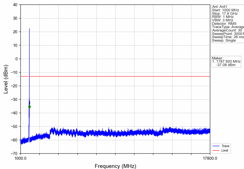
n66_15kHz_SISO_NTNV_35MHz_DFT-s-OFDM QPSK_1762.5MHz_Edge_1RB_Right
