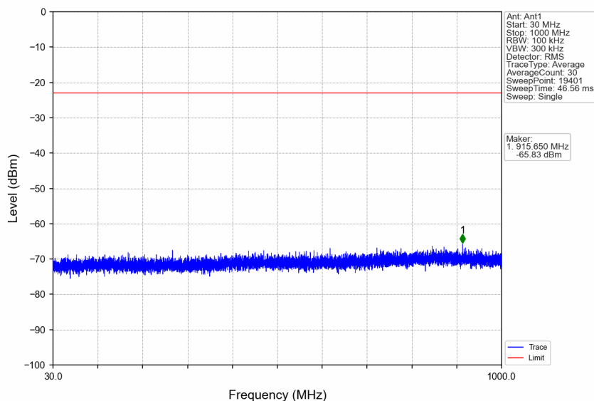
n66_15kHz_SISO_NTNV_35MHz_DFT-s-OFDM QPSK_1762.5MHz_Edge_1RB_Right
