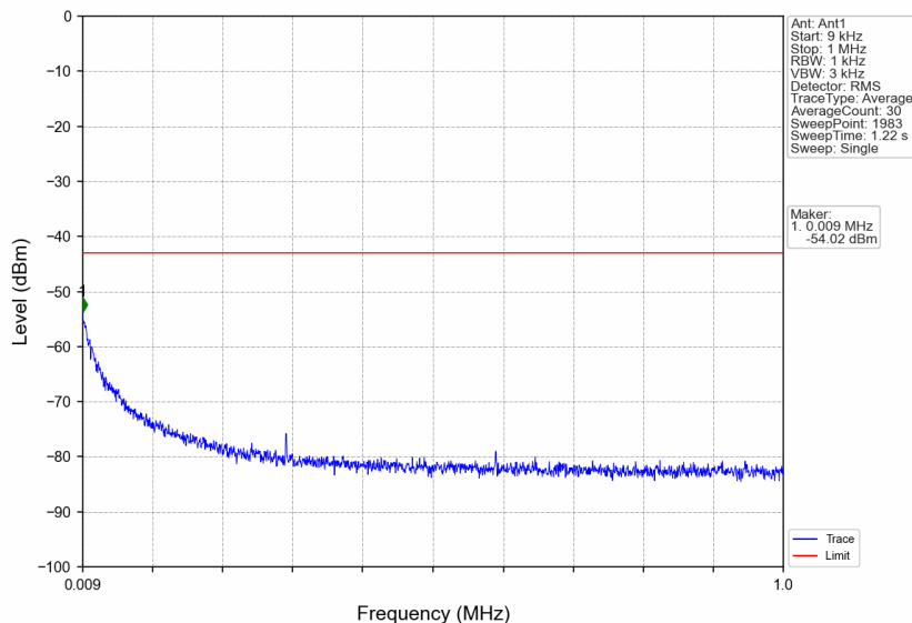
n66_15kHz_SISO_NTNV_15MHz_CP-OFDM QPSK_1772.5MHz_Edge_1RB_Right
