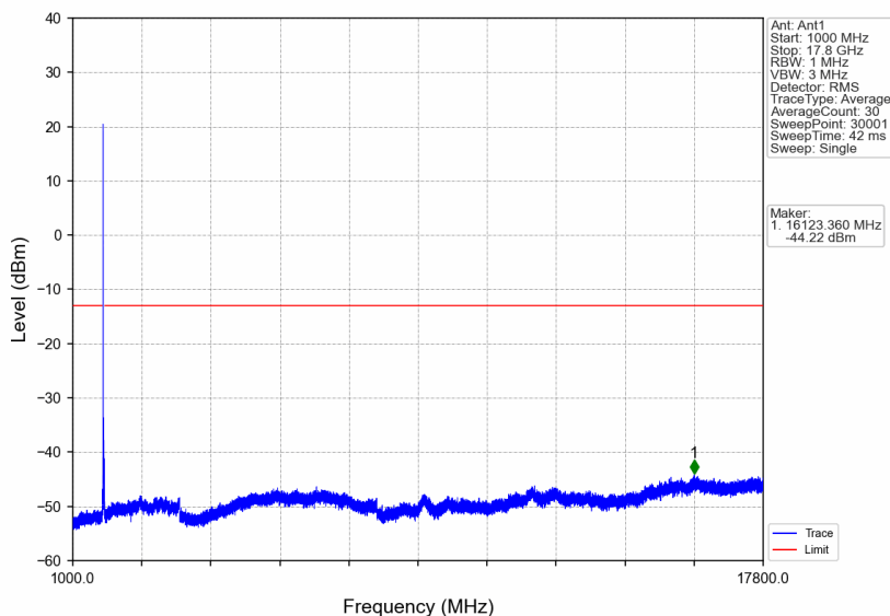
n66_15kHz_SISO_NTNV_20MHz_CP-OFDM QPSK_1770MHz_Edge_1RB_Right
