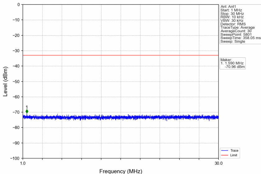
n66_15kHz_SISO_NTNV_25MHz_DFT-s-OFDM QPSK_1722.5MHz_Edge_1RB_Left
