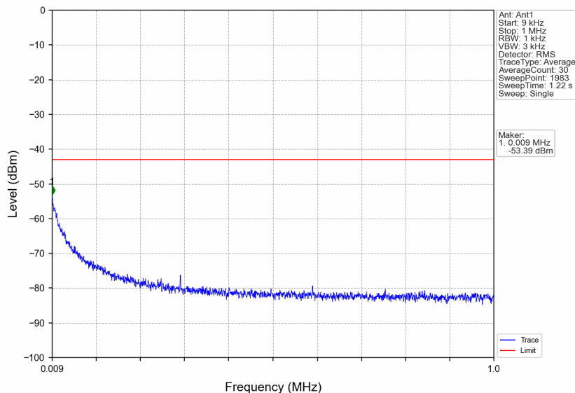
n66_15kHz_SISO_NTNV_20MHz_CP-OFDM QPSK_1770MHz_Edge_1RB_Right
