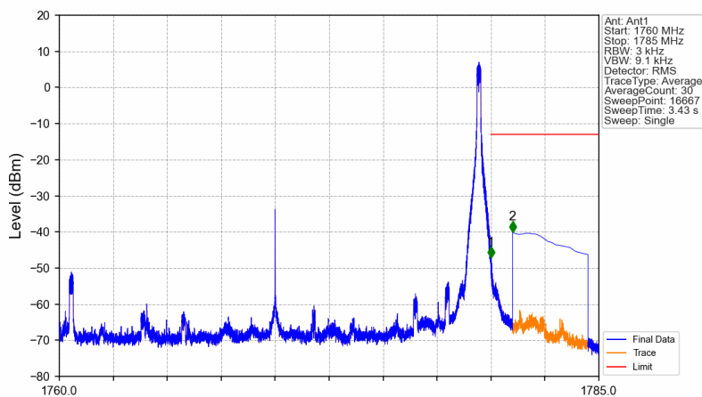
n66_15kHz_SISO_NTNV_20MHz_CP-OFDM QPSK_1770MHz_Edge_1RB_Right
