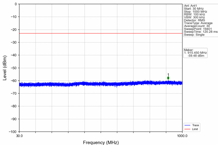
n66_15kHz_SISO_NTNV_15MHz_CP-OFDM QPSK_1717.5MHz_Edge_1RB_Left
