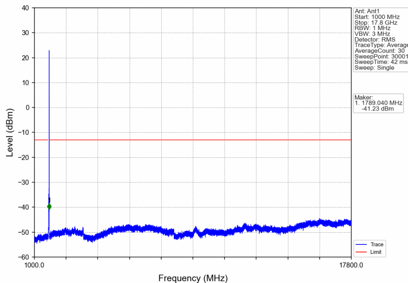
n66_15kHz_SISO_NTNV_20MHz_DFT-s-OFDM QPSK_1770MHz_Edge_1RB_Right
