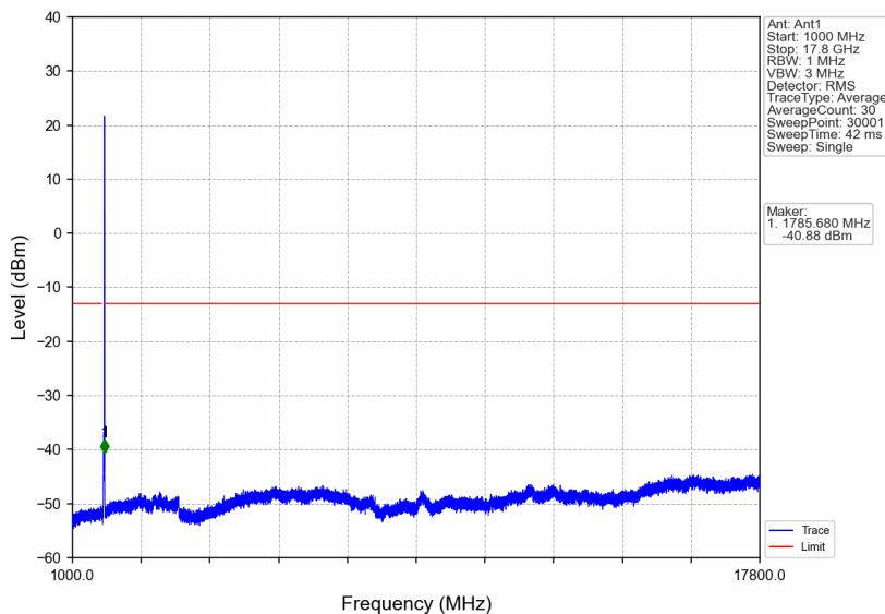
n66_15kHz_SISO_NTNV_15MHz_CP-OFDM QPSK_1772.5MHz_Edge_1RB_Right
