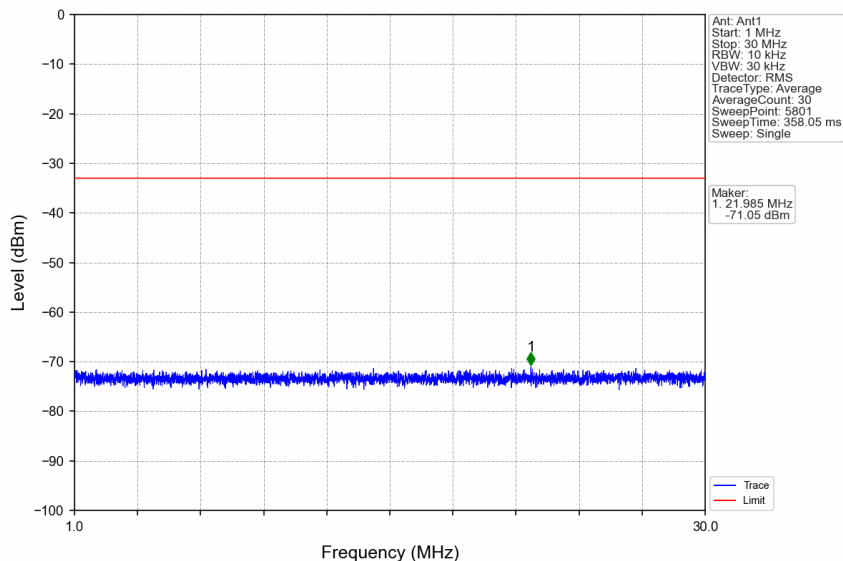
n66_15kHz_SISO_NTNV_15MHz_CP-OFDM QPSK_1745MHz_Edge_1RB_Left
