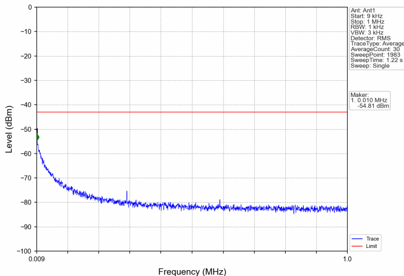
n66_15kHz_SISO_NTNV_20MHz_DFT-s-OFDM QPSK_1770MHz_Edge_1RB_Right
