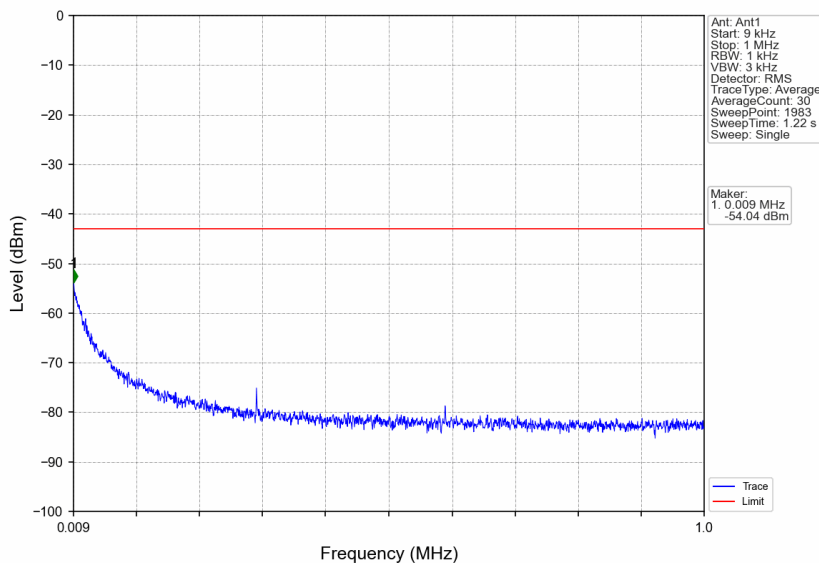
n66_15kHz_SISO_NTNV_15MHz_CP-OFDM QPSK_1745MHz_Edge_1RB_Left
