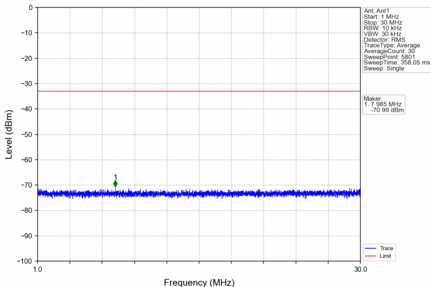
n66_15kHz_SISO_NTNV_20MHz_CP-OFDM QPSK_1745MHz_Edge_1RB_Left
