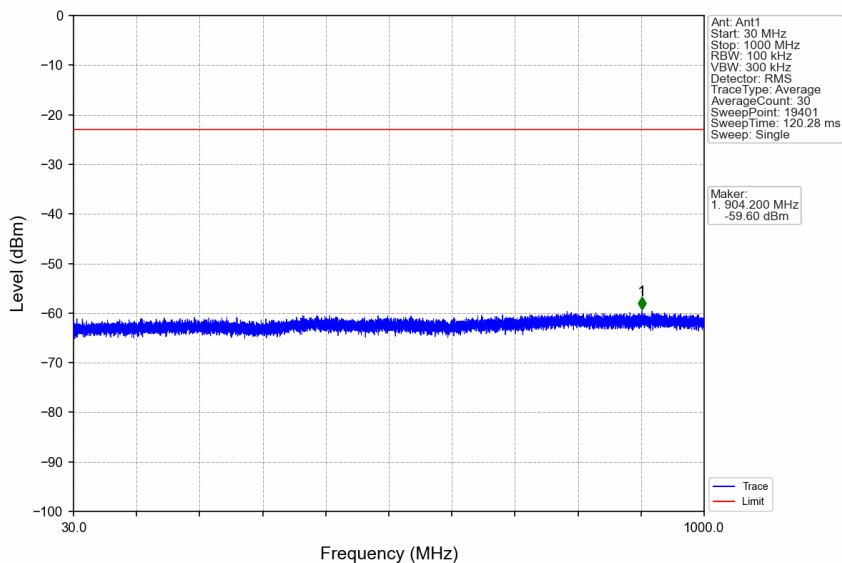
n66_15kHz_SISO_NTNV_20MHz_CP-OFDM QPSK_1745MHz_Edge_1RB_Left
