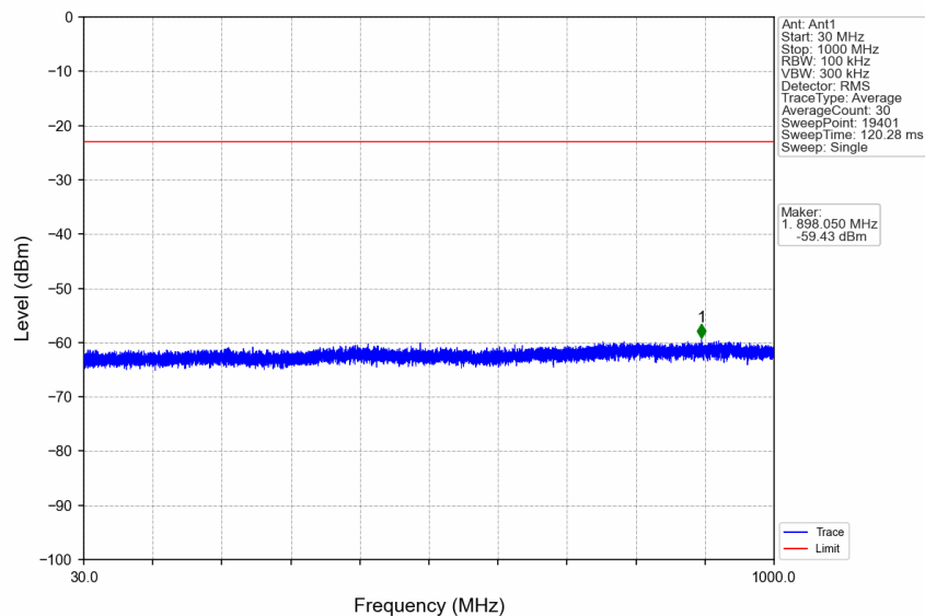
n66_15kHz_SISO_NTNV_20MHz_DFT-s-OFDM QPSK_1745MHz_Edge_1RB_Left
