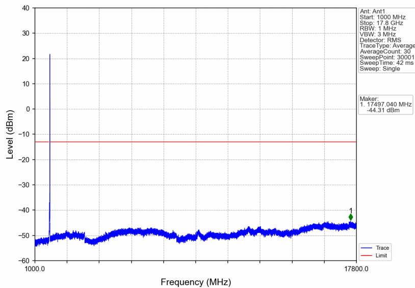
n66_15kHz_SISO_NTNV_20MHz_CP-OFDM QPSK_1770MHz_Edge_1RB_Right
