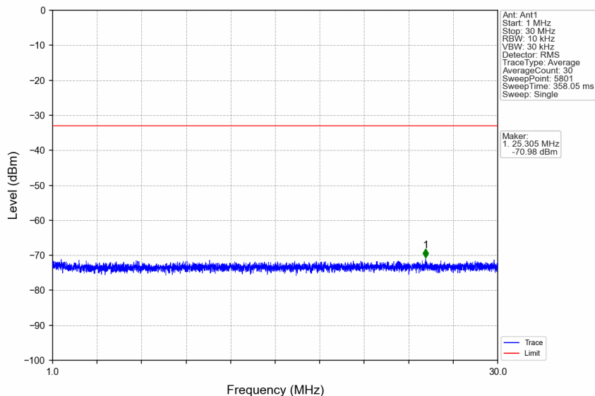
n66_15kHz_SISO_NTNV_15MHz_CP-OFDM QPSK_1717.5MHz_Edge_1RB_Left
