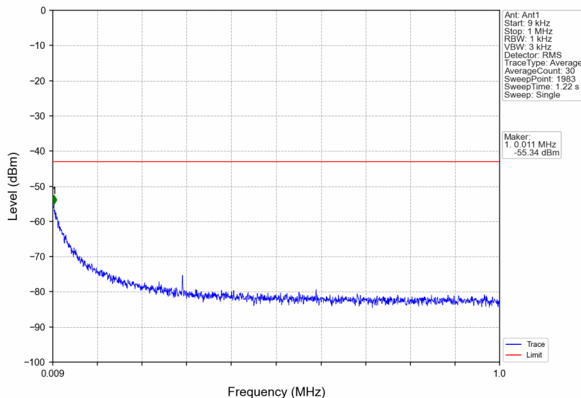
n66_15kHz_SISO_NTNV_15MHz_DFT-s-OFDM QPSK_1772.5MHz_Edge_1RB_Right
