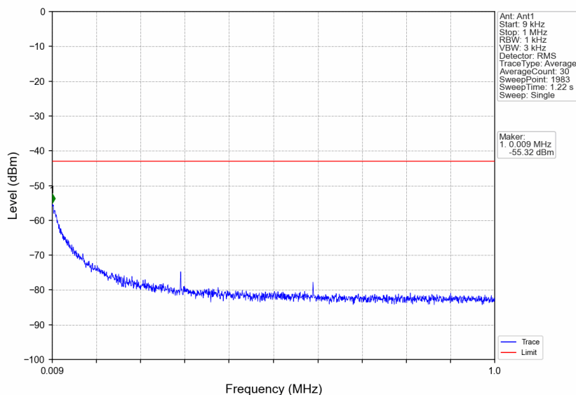
n66_15kHz_SISO_NTNV_10MHz_DFT-s-OFDM_QPSK_1775MHz_Edge_1RB_Right
