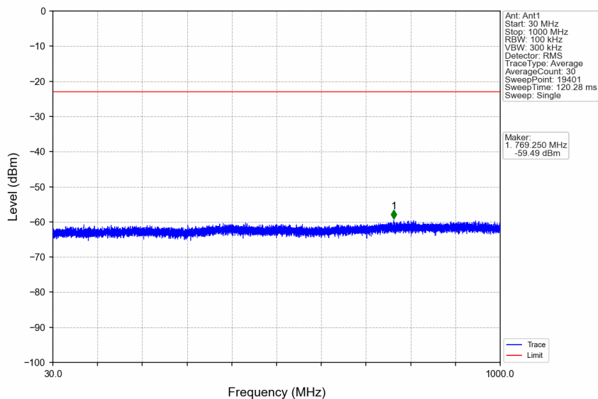
n66_15kHz_SISO_NTNV_15MHz_DFT-s-OFDM_QPSK_1717.5MHz_Edge_1RB_Left
