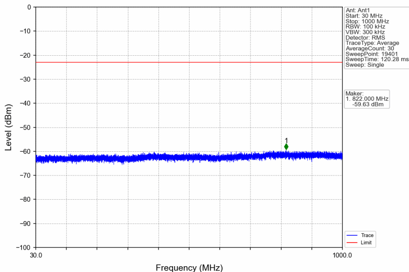
n66_15kHz_SISO_NTNV_5MHz_CP-OFDM QPSK_1777.5MHz_Edge_1RB_Right
