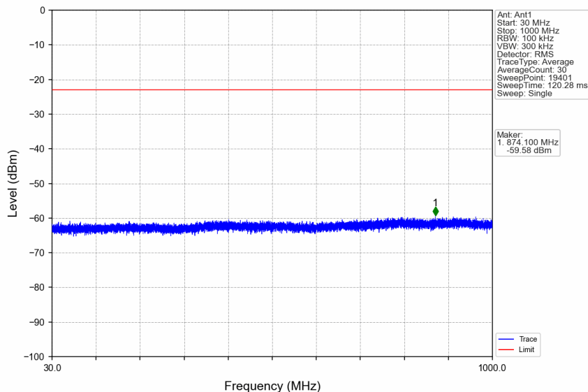
n66_15kHz_SISO_NTNV_10MHz_CP-OFDM QPSK_1775MHz_Edge_1RB_Right
