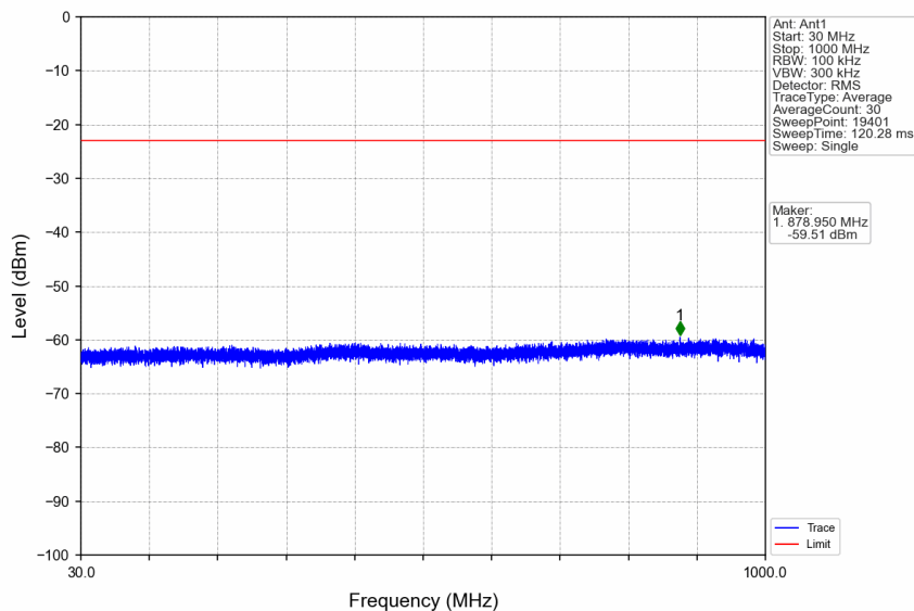
n66_15kHz_SISO_NTNV_10MHz_CP-OFDM QPSK_1715MHz_Edge_1RB_Left
