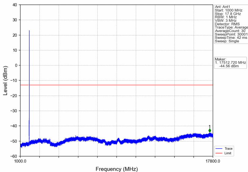
n66_15kHz_SISO_NTNV_10MHz_DFT-s-OFDM_QPSK_1775MHz_Edge_1RB_Right
