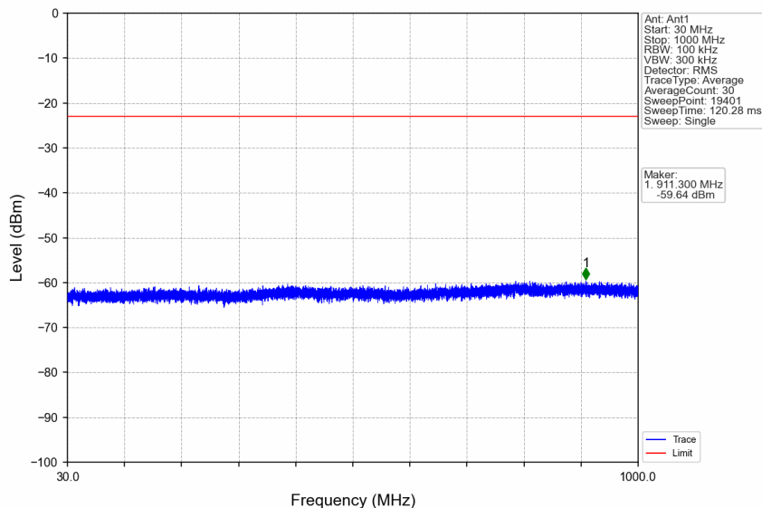
n66_15kHz_SISO_NTNV_10MHz_DFT-s-OFDM_QPSK_1775MHz_Edge_1RB_Right
