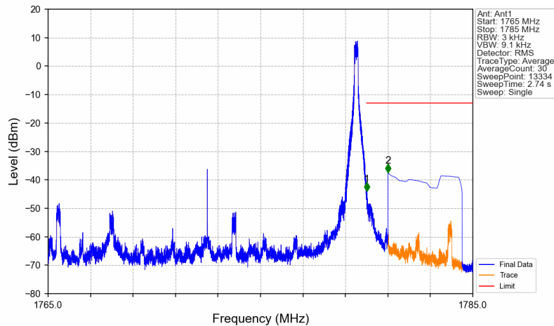
n66_15kHz_SISO_NTNV_15MHz_DFT-s-OFDM QPSK_1772.5MHz_Edge_1RB_Right
