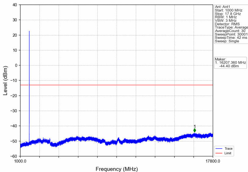
n66_15kHz_SISO_NTNV_5MHz_CP-OFDM QPSK_1777.5MHz_Edge_1RB_Right
