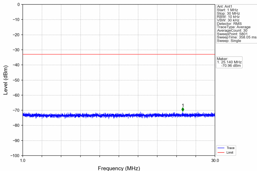
n66_15kHz_SISO_NTNV_10MHz_DFT-s-OFDM QPSK_1745MHz_Edge_1RB_Left
