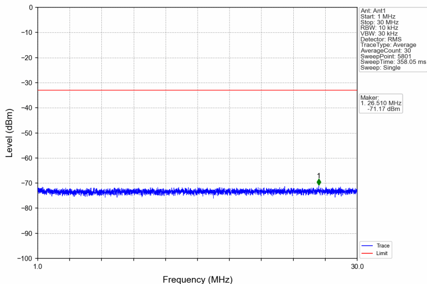
n66_15kHz_SISO_NTNV_10MHz_CP-OFDM QPSK_1745MHz_Edge_1RB_Left
