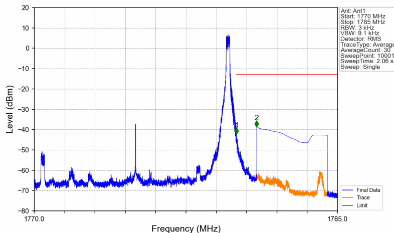
n66_15kHz_SISO_NTNV_10MHz_CP-OFDM QPSK_1775MHz_Edge_1RB_Right
