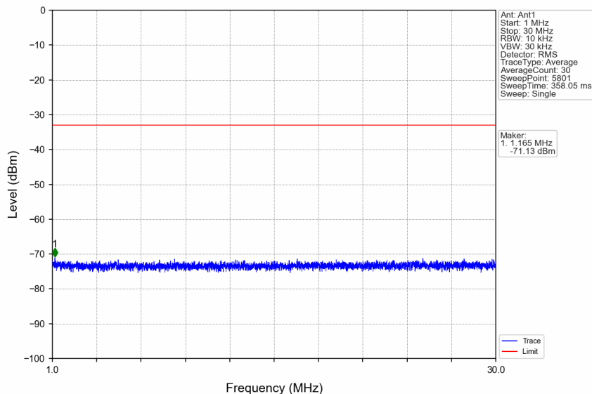
n66_15kHz_SISO_NTNV_10MHz_CP-OFDM QPSK_1715MHz_Edge_1RB_Left
