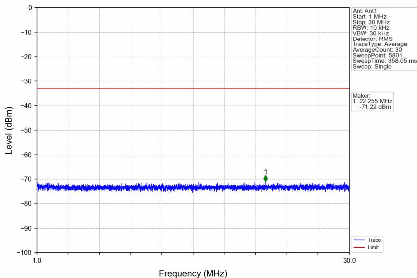
n66_15kHz_SISO_NTNV_15MHz_DFT-s-OFDM QPSK_1772.5MHz_Edge_1RB_Right
