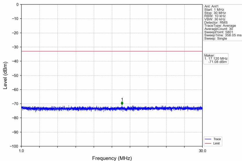
n66_15kHz_SISO_NTNV_10MHz_CP-OFDM QPSK_1775MHz_Edge_1RB_Right
