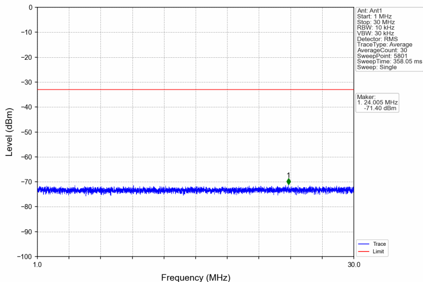
n66_15kHz_SISO_NTNV_15MHz_DFT-s-OFDM QPSK_1745MHz_Edge_1RB_Left
