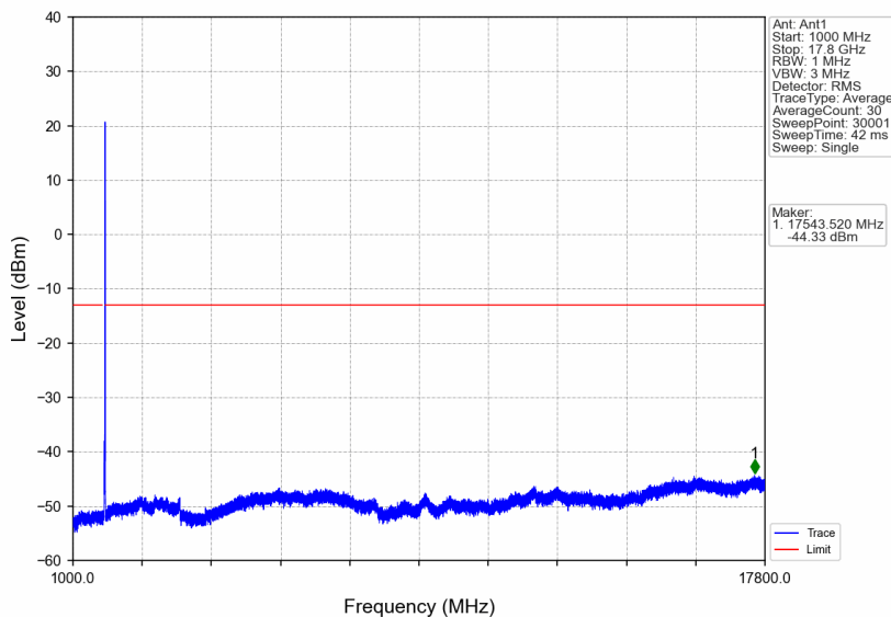
n66_15kHz_SISO_NTNV_10MHz_CP-OFDM QPSK_1775MHz_Edge_1RB_Right
