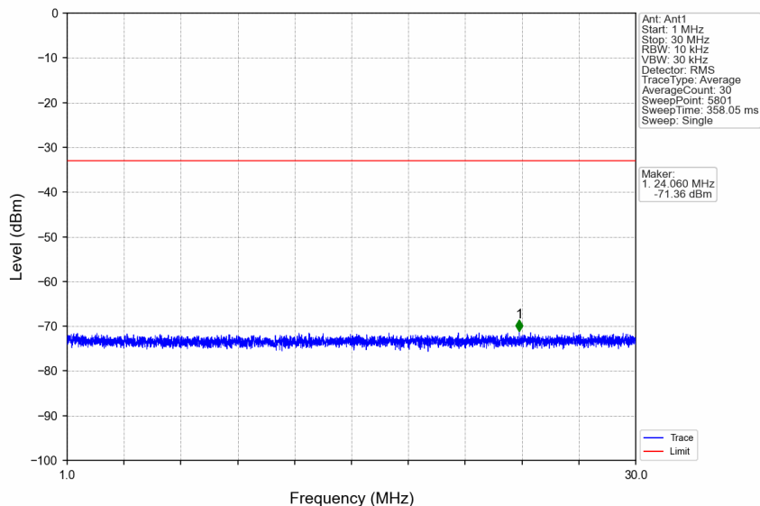
n66_15kHz_SISO_NTNV_10MHz_DFT-s-OFDM QPSK_1715MHz_Edge_1RB_Left
