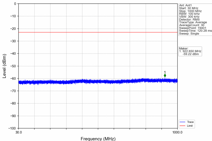
n66_15kHz_SISO_NTNV_15MHz_DFT-s-OFDM QPSK_1772.5MHz_Edge_1RB_Right
