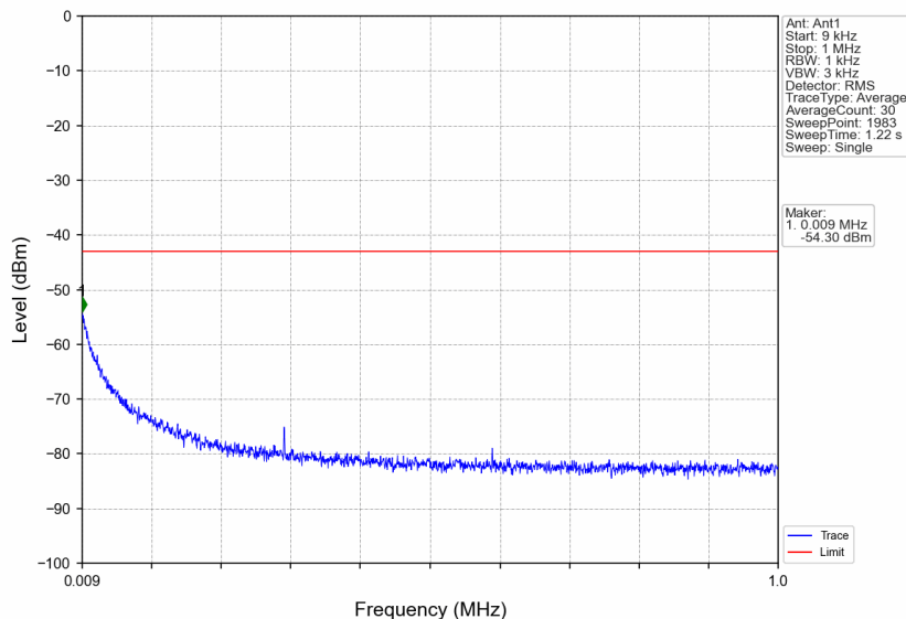
n66_15kHz_SISO_NTNV_10MHz_CP-OFDM QPSK_1775MHz_Edge_1RB_Right
