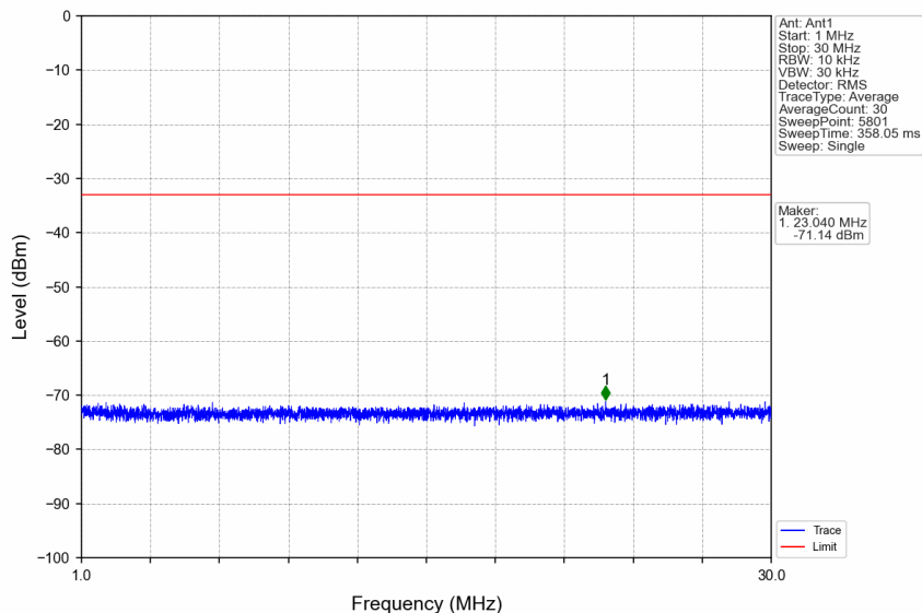
n66_15kHz_SISO_NTNV_15MHz_DFT-s-OFDM_QPSK_1717.5MHz_Edge_1RB_Left
