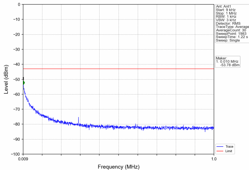
n66_15kHz_SISO_NTNV_5MHz_CP-OFDM QPSK_1777.5MHz_Edge_1RB_Right
