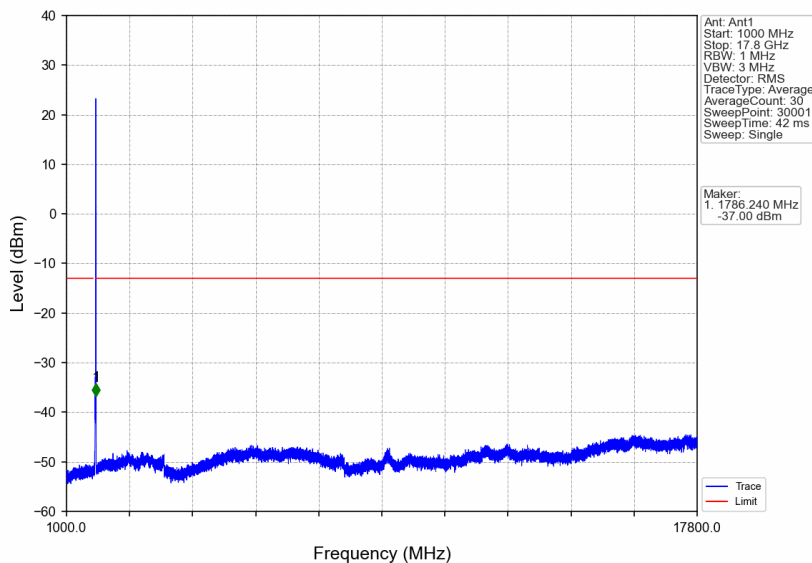
n66_15kHz_SISO_NTNV_15MHz_DFT-s-OFDM QPSK_1772.5MHz_Edge_1RB_Right
