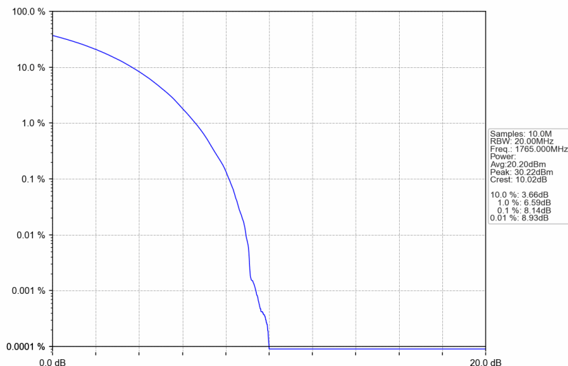
n66_30kHz_SISO_NTNV_30MHz_CP-OFDM 16 QAM_1765MHz_Outer_Full
