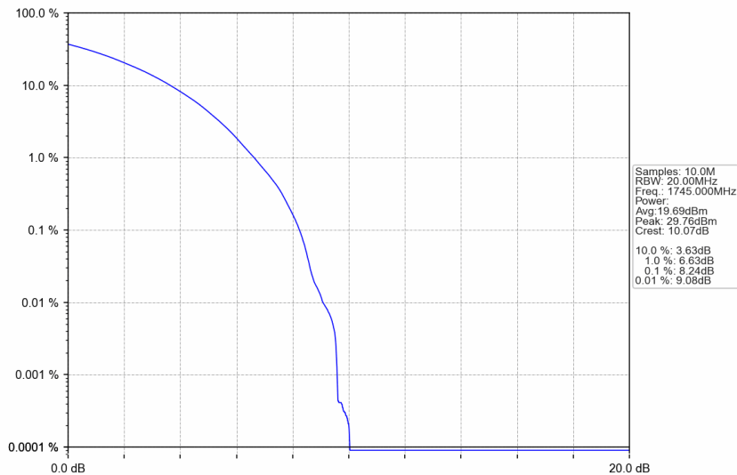
n66_30kHz_SISO_NTNV_30MHz_CP-OFDM 64 QAM_1745MHz_Outer_Full
