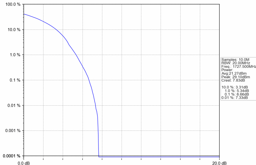
n66_30kHz_SISO_NTNV_35MHz_DFT-s-OFDM 64 QAM_1727.5MHz_Outer_Full
