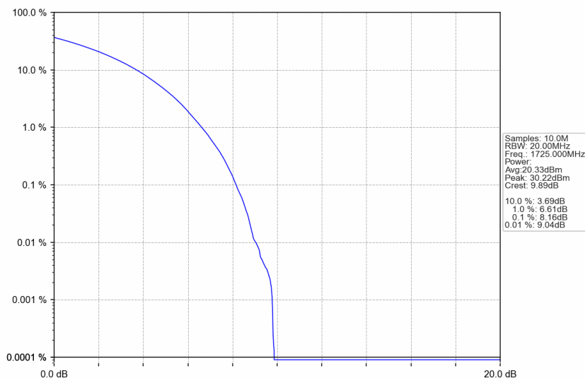
n66_30kHz_SISO_NTNV_30MHz_CP-OFDM QPSK_1725MHz_Outer_Full
