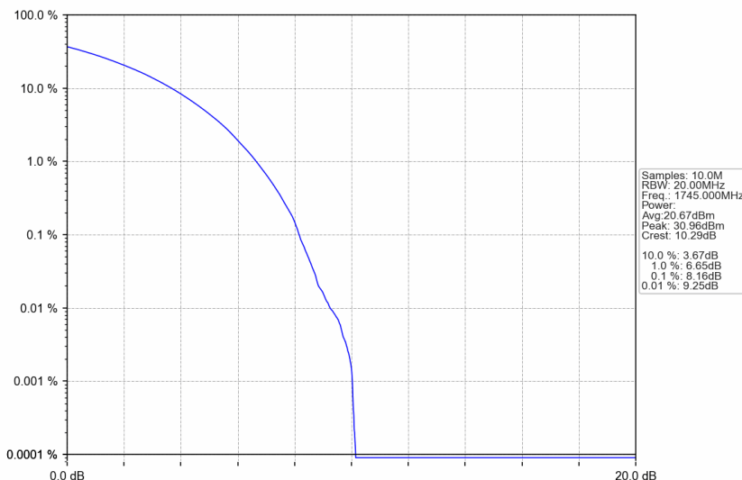
n66_30kHz_SISO_NTNV_35MHz_CP-OFDM QPSK_1745MHz_Outer_Full
