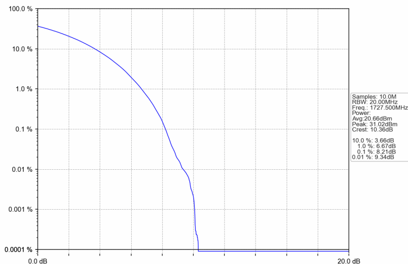
n66_30kHz_SISO_NTNV_35MHz_CP-OFDM QPSK_1727.5MHz_Outer_Full
