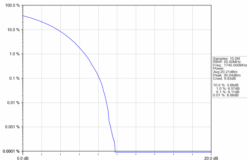
n66_30kHz_SISO_NTNV_30MHz_CP-OFDM 16 QAM_1745MHz_Outer_Full
