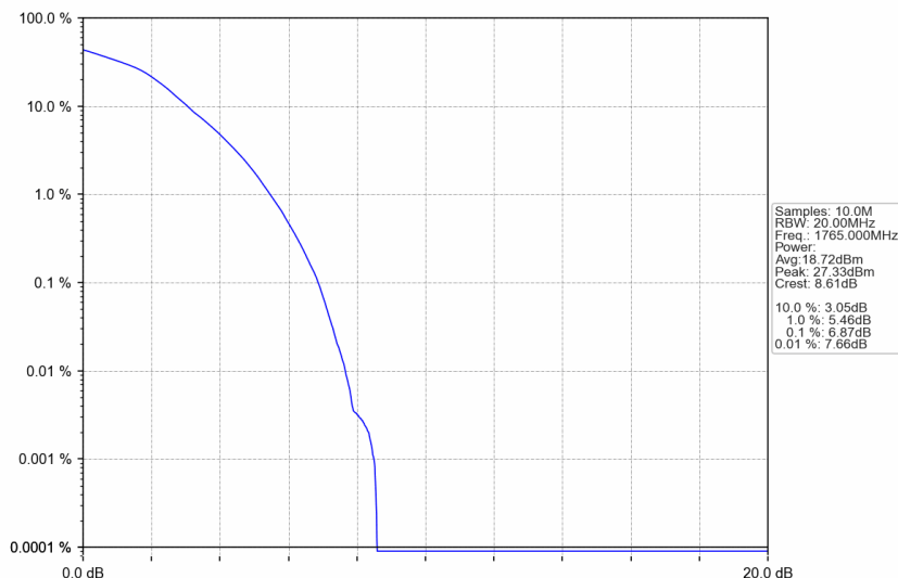
n66_30kHz_SISO_NTNV_30MHz_DFT-s-OFDM 256 QAM_1765MHz_Outer_Full
