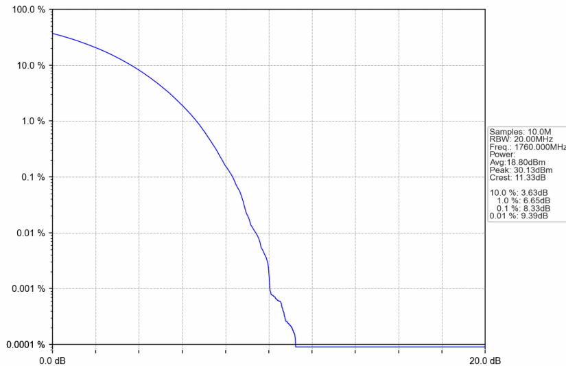
n66_30kHz_SISO_NTNV_40MHz_CP-OFDM QPSK_1760MHz_Outer_Full
