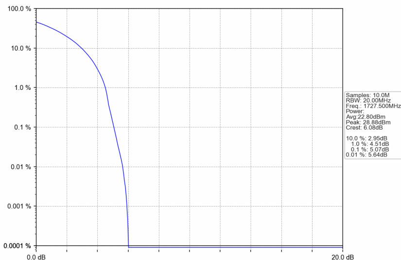
n66_30kHz_SISO_NTNV_35MHz_DFT-s-OFDM QPSK_1727.5MHz_Outer_Full
