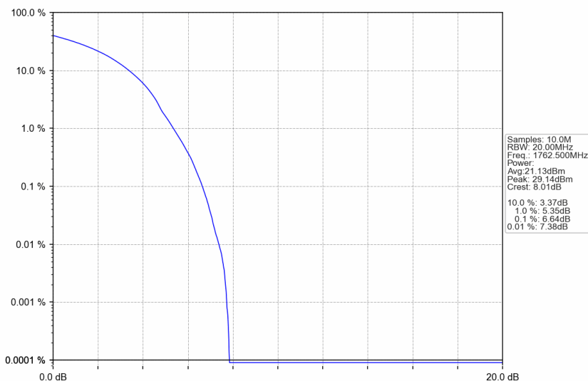
n66_30kHz_SISO_NTNV_35MHz_DFT-s-OFDM 64 QAM_1762.5MHz_Outer_Full
