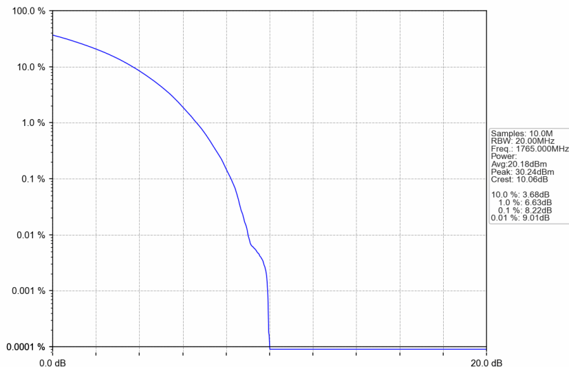
n66_30kHz_SISO_NTNV_30MHz_CP-OFDM QPSK_1765MHz_Outer_Full
