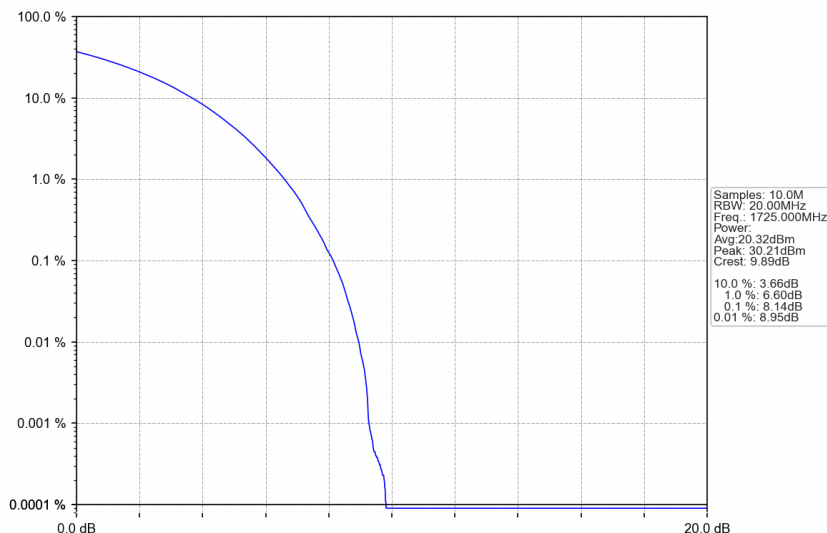
n66_30kHz_SISO_NTNV_30MHz_CP-OFDM 16 QAM_1725MHz_Outer_Full
