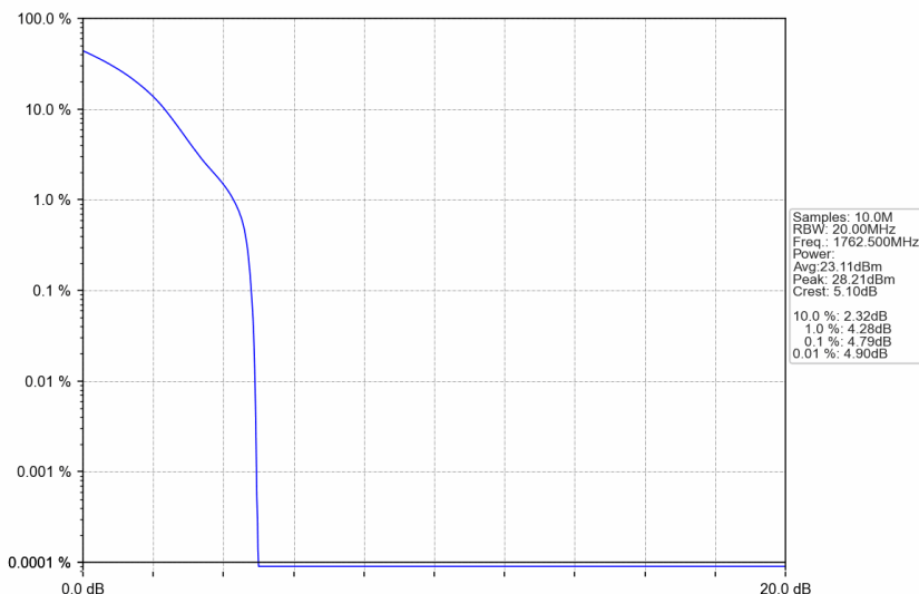
n66_30kHz_SISO_NTNV_35MHz_DFT-s-OFDM PI/2 BPSK_1762.5MHz_Outer_Full
