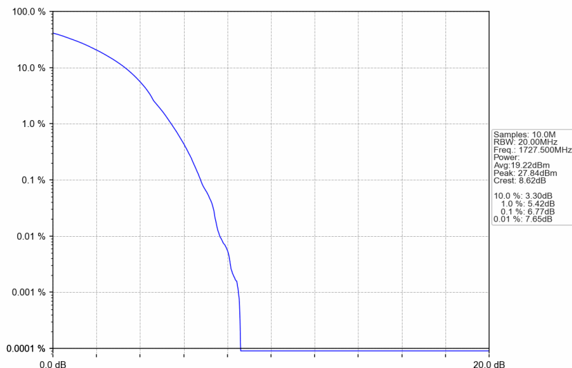
n66_30kHz_SISO_NTNV_35MHz_DFT-s-OFDM 256 QAM_1727.5MHz_Outer_Full
