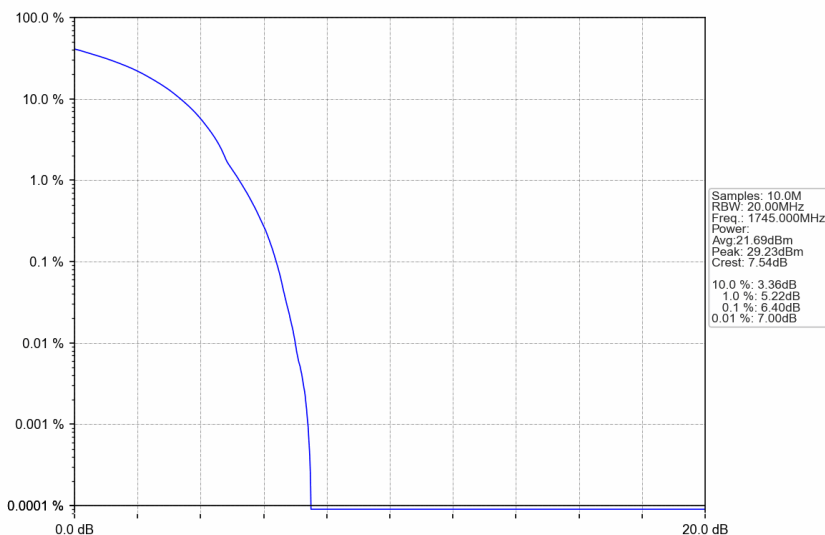
n66_30kHz_SISO_NTNV_35MHz_DFT-s-OFDM 16 QAM_1745MHz_Outer_Full
