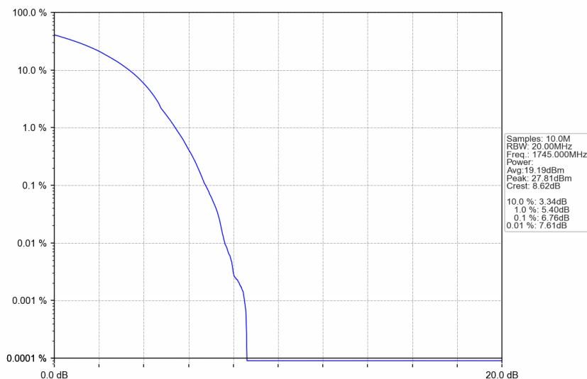
n66_30kHz_SISO_NTNV_35MHz_DFT-s-OFDM 256 QAM_1745MHz_Outer_Full
