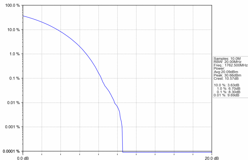
n66_30kHz_SISO_NTNV_35MHz_CP-OFDM 64 QAM_1762.5MHz_Outer_Full
