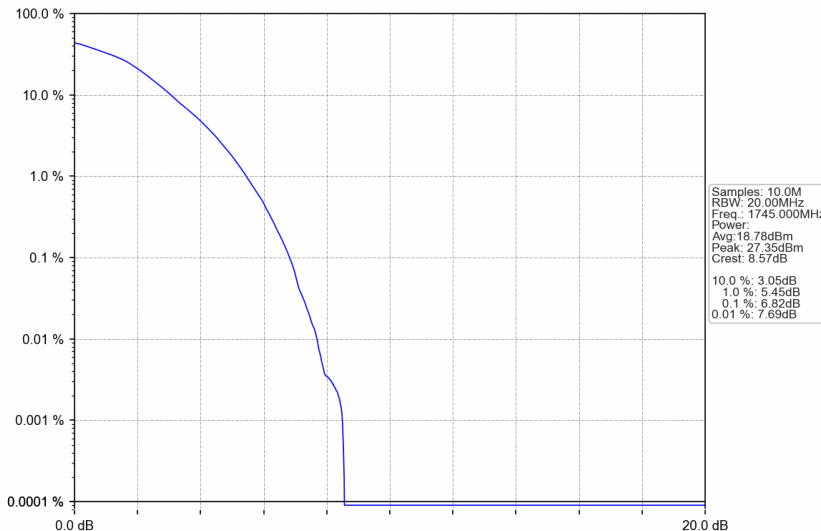
n66_30kHz_SISO_NTNV_30MHz_DFT-s-OFDM 256 QAM_1745MHz_Outer_Full
