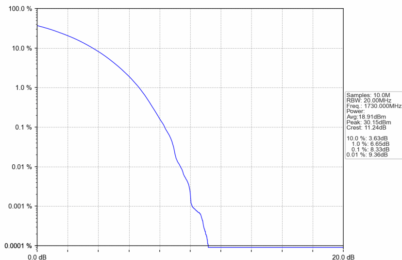
n66_30kHz_SISO_NTNV_40MHz_CP-OFDM QPSK_1730MHz_Outer_Full
