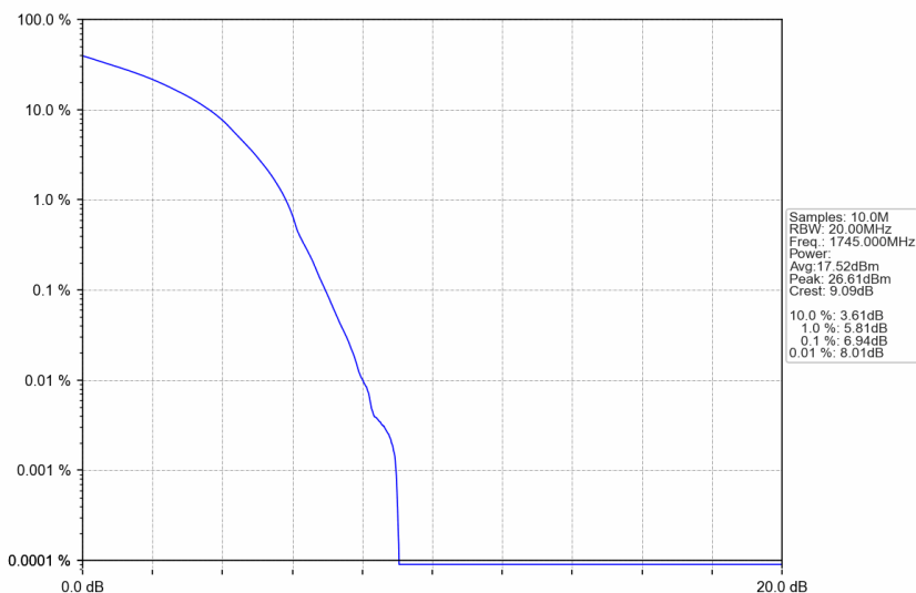
n66_30kHz_SISO_NTNV_40MHz_DFT-s-OFDM 256 QAM_1745MHz_Outer_Full
