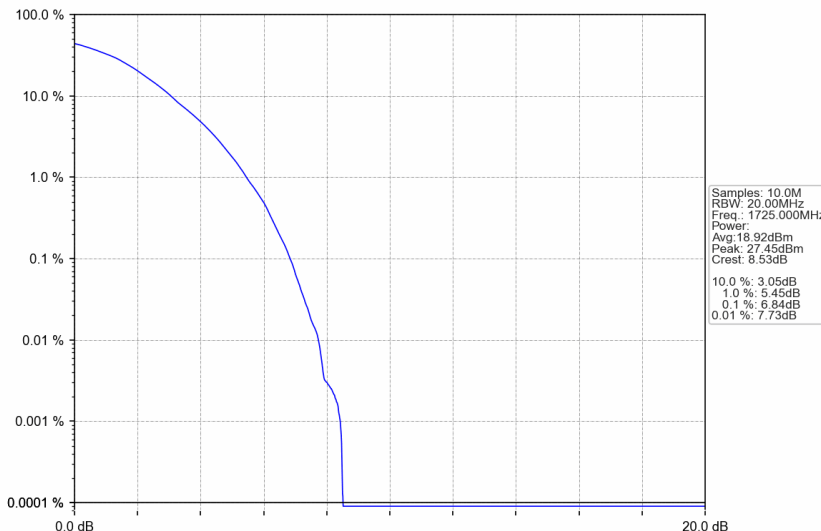
n66_30kHz_SISO_NTNV_30MHz_DFT-s-OFDM 256 QAM_1725MHz_Outer_Full
