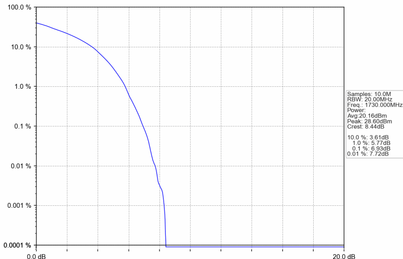
n66_30kHz_SISO_NTNV_40MHz_DFT-s-OFDM 16 QAM_1730MHz_Outer_Full
