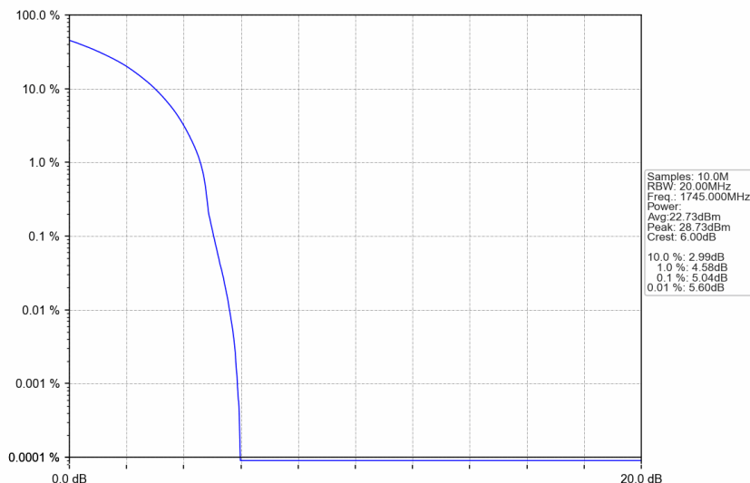
n66_30kHz_SISO_NTNV_35MHz_DFT-s-OFDM QPSK_1745MHz_Outer_Full
