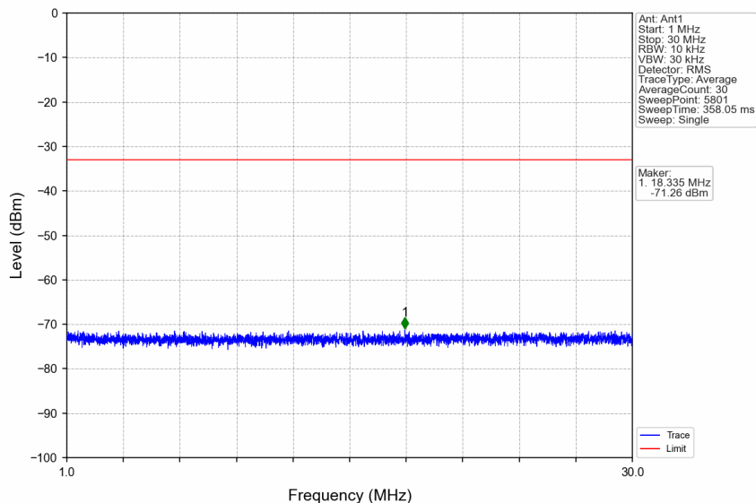
n66_15kHz_SISO_NTNV_5MHz_DFT-s-OFDM QPSK_1745MHz_Edge_1RB_Left
