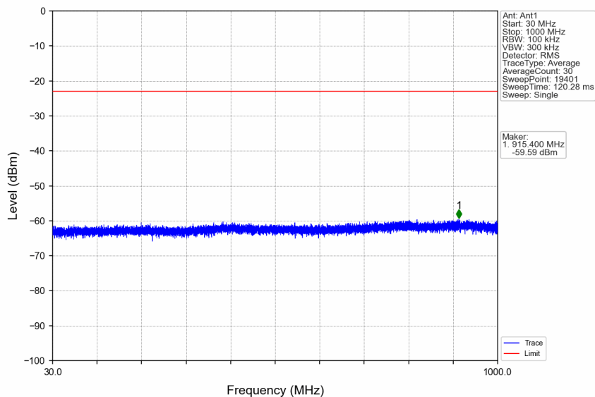
n66_15kHz_SISO_NTNV_5MHz_DFT-s-OFDM QPSK_1745MHz_Edge_1RB_Left
