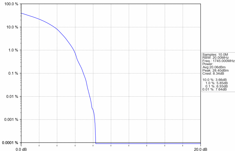
n66_30kHz_SISO_NTNV_40MHz_DFT-s-OFDM 16 QAM_1745MHz_Outer_Full
