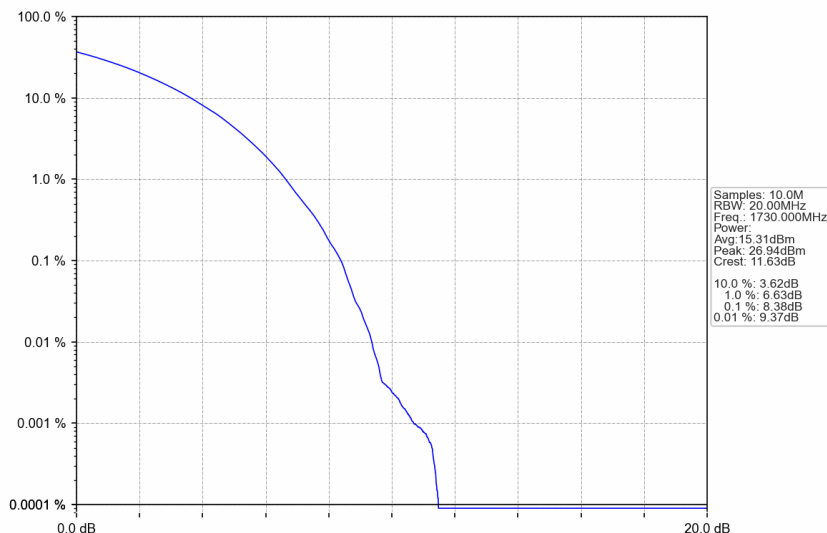
n66_30kHz_SISO_NTNV_40MHz_CP-OFDM 256 QAM_1730MHz_Outer_Full
