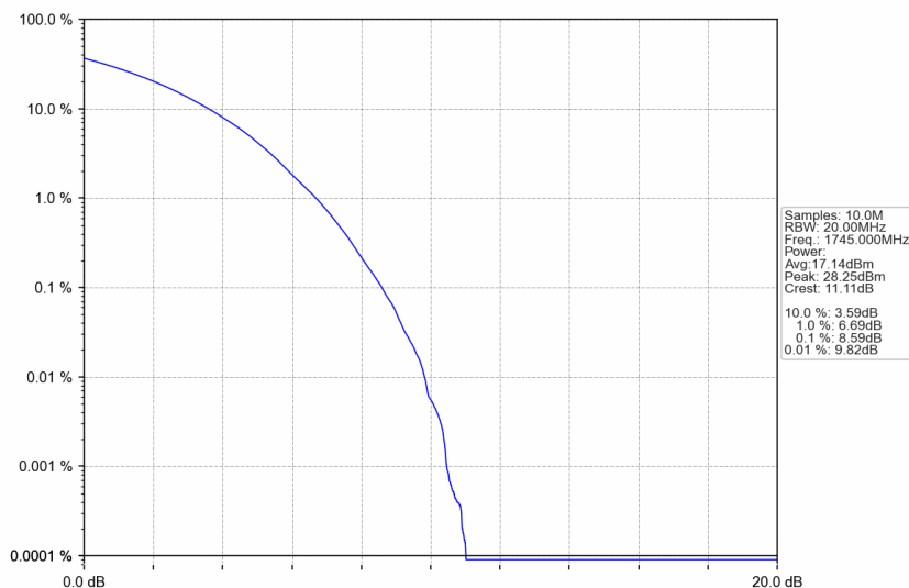
n66_30kHz_SISO_NTNV_35MHz_CP-OFDM 256 QAM_1745MHz_Outer_Full
