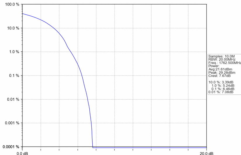
n66_30kHz_SISO_NTNV_35MHz_DFT-s-OFDM 16 QAM_1762.5MHz_Outer_Full
