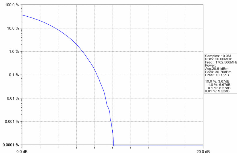
n66_30kHz_SISO_NTNV_35MHz_CP-OFDM 16 QAM_1762.5MHz_Outer_Full
