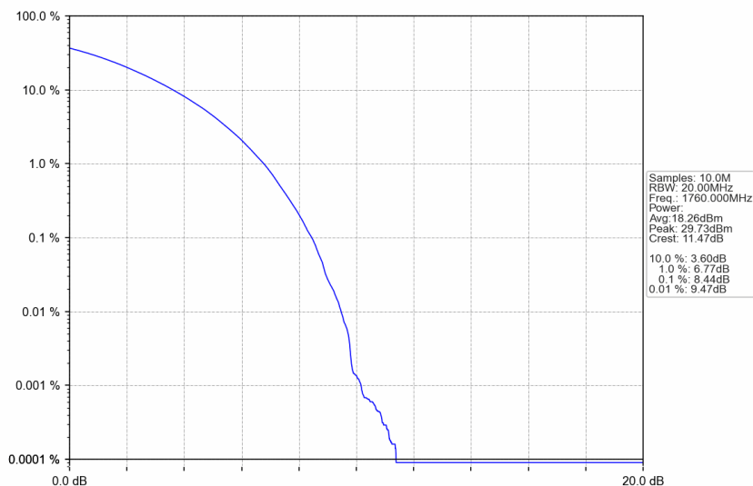
n66_30kHz_SISO_NTNV_40MHz_CP-OFDM 64 QAM_1760MHz_Outer_Full
