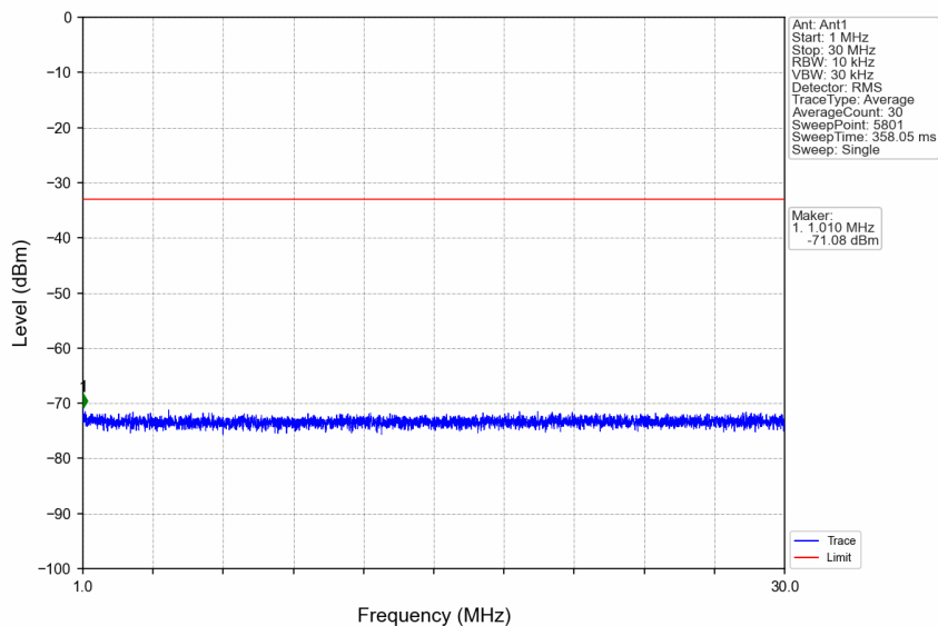
n66_15kHz_SISO_NTNV_5MHz_DFT-s-OFDM QPSK_1777.5MHz_Edge_1RB_Right
