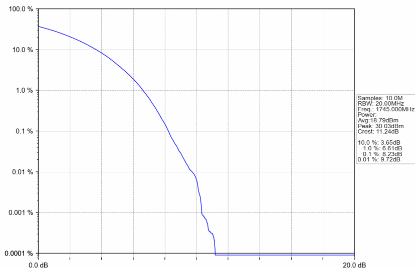
n66_30kHz_SISO_NTNV_40MHz_CP-OFDM 16 QAM_1745MHz_Outer_Full
