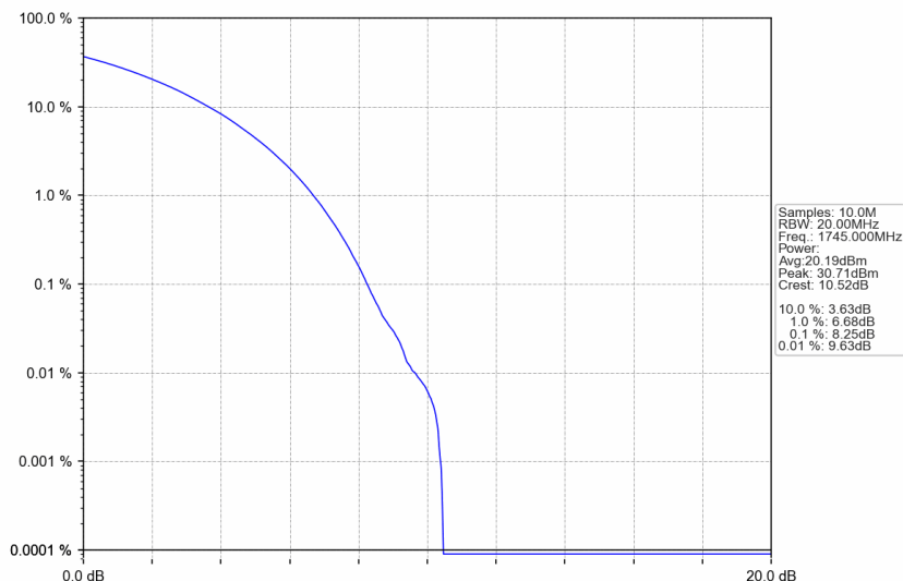
n66_30kHz_SISO_NTNV_35MHz_CP-OFDM 64 QAM_1745MHz_Outer_Full
