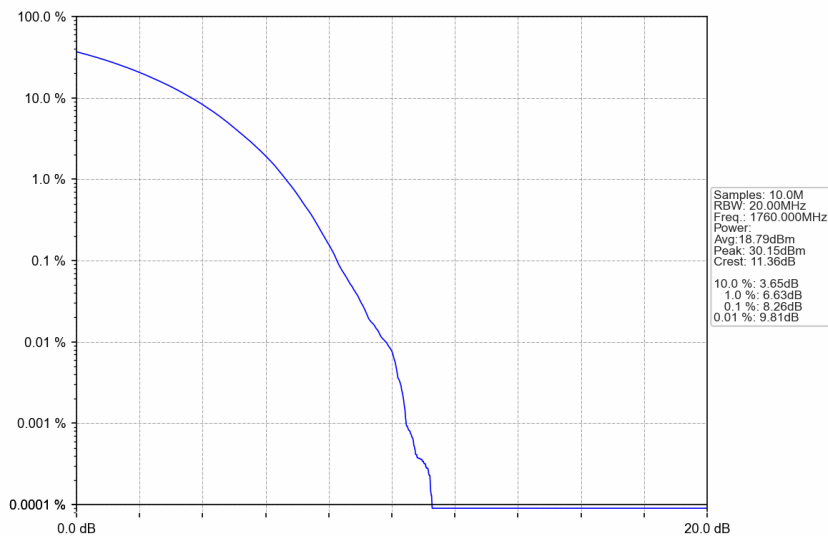
n66_30kHz_SISO_NTNV_40MHz_CP-OFDM 16 QAM_1760MHz_Outer_Full
