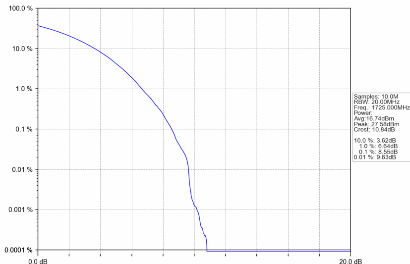
n66_30kHz_SISO_NTNV_30MHz_CP-OFDM 256 QAM_1725MHz_Outer_Full
