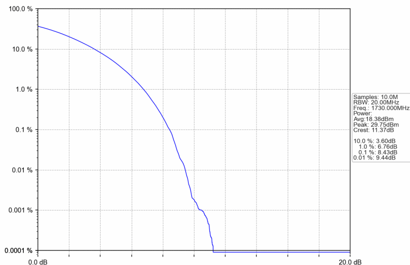
n66_30kHz_SISO_NTNV_40MHz_CP-OFDM 64 QAM_1730MHz_Outer_Full
