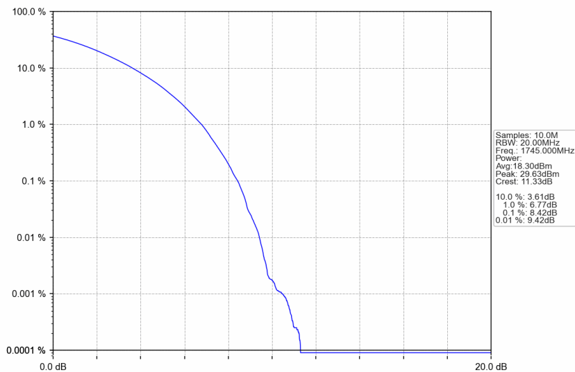
n66_30kHz_SISO_NTNV_40MHz_CP-OFDM 64 QAM_1745MHz_Outer_Full
