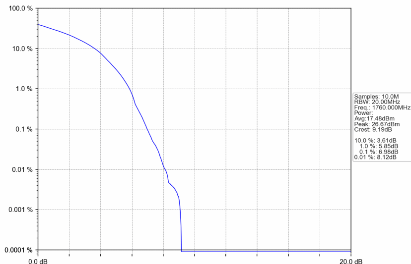
n66_30kHz_SISO_NTNV_40MHz_DFT-s-OFDM 256 QAM_1760MHz_Outer_Full
