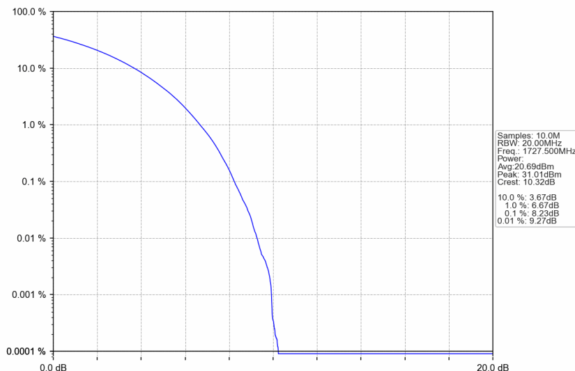
n66_30kHz_SISO_NTNV_35MHz_CP-OFDM 16 QAM_1727.5MHz_Outer_Full
