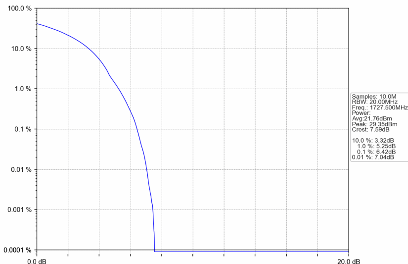
n66_30kHz_SISO_NTNV_35MHz_DFT-s-OFDM 16 QAM_1727.5MHz_Outer_Full
