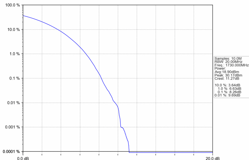
n66_30kHz_SISO_NTNV_40MHz_CP-OFDM 16 QAM_1730MHz_Outer_Full
