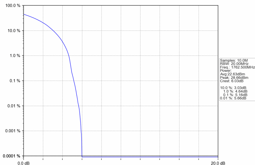
n66_30kHz_SISO_NTNV_35MHz_DFT-s-OFDM QPSK_1762.5MHz_Outer_Full
