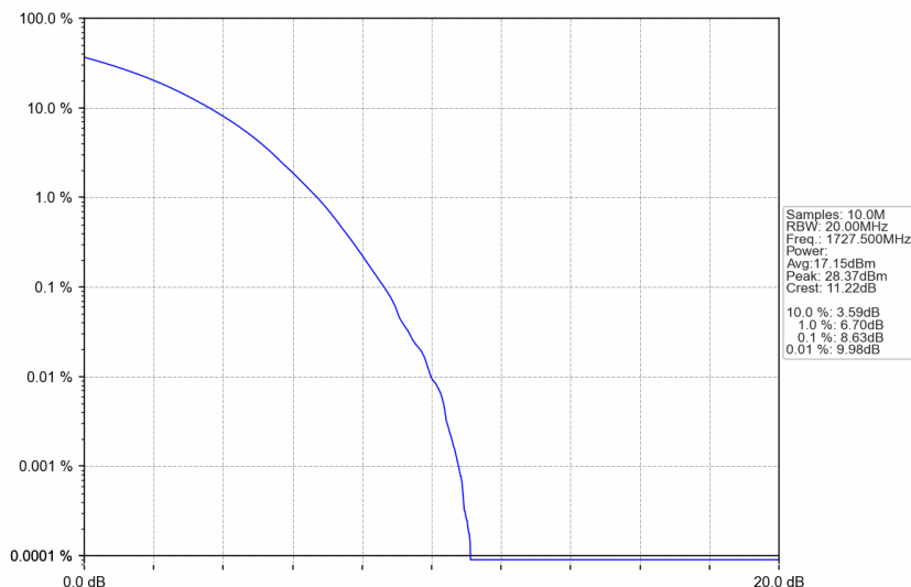
n66_30kHz_SISO_NTNV_35MHz_CP-OFDM 256 QAM_1727.5MHz_Outer_Full
