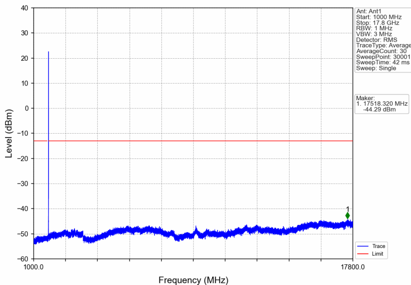
n66_15kHz_SISO_NTNV_5MHz_DFT-s-OFDM_QPSK_1777.5MHz_Edge_1RB_Right
