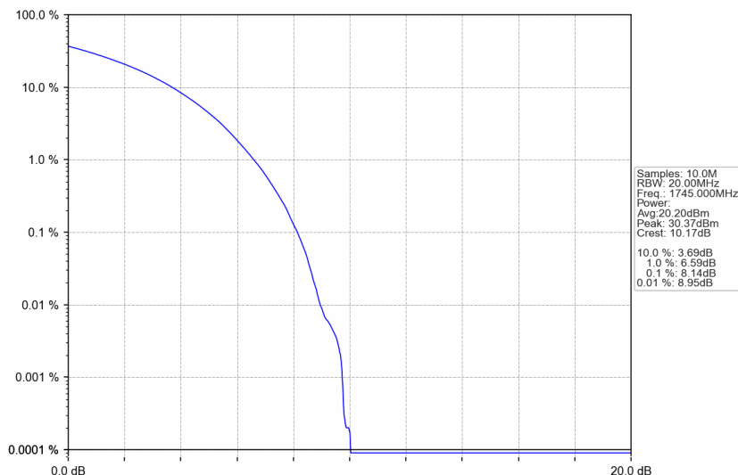
n66_30kHz_SISO_NTNV_30MHz_CP-OFDM QPSK_1745MHz_Outer_Full
