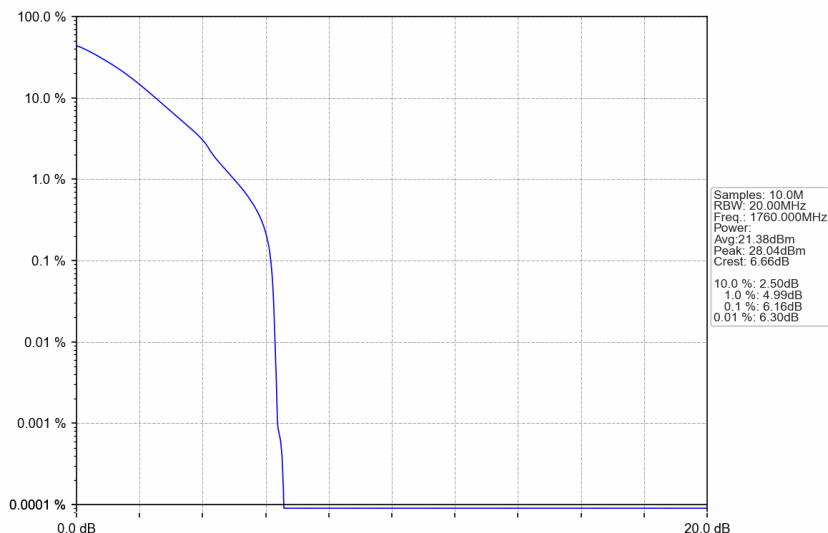
n66_30kHz_SISO_NTNV_40MHz_DFT-s-OFDM PI/2 BPSK_1760MHz_Outer_Full
