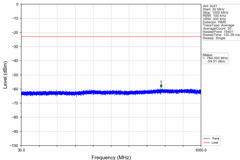
n66_15kHz_SISO_NTNV_5MHz_DFT-s-OFDM_QPSK_1777.5MHz_Edge_1RB_Right
