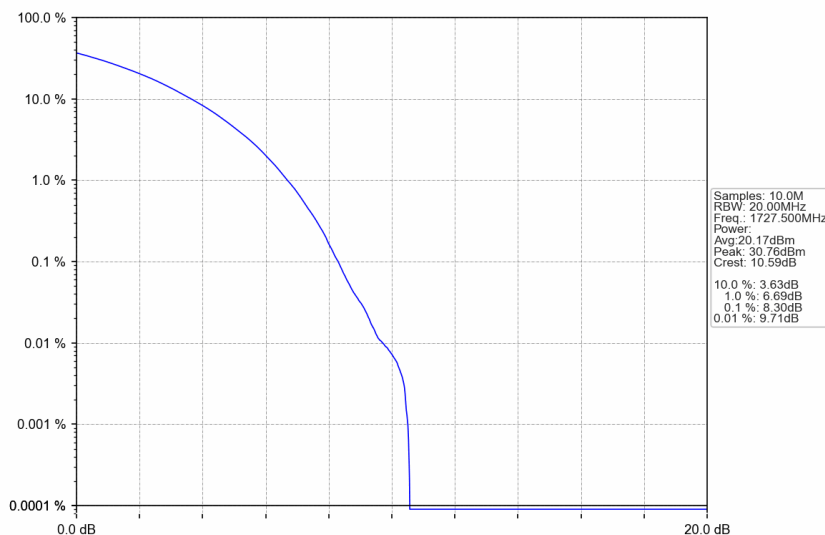
n66_30kHz_SISO_NTNV_35MHz_CP-OFDM 64 QAM_1727.5MHz_Outer_Full
