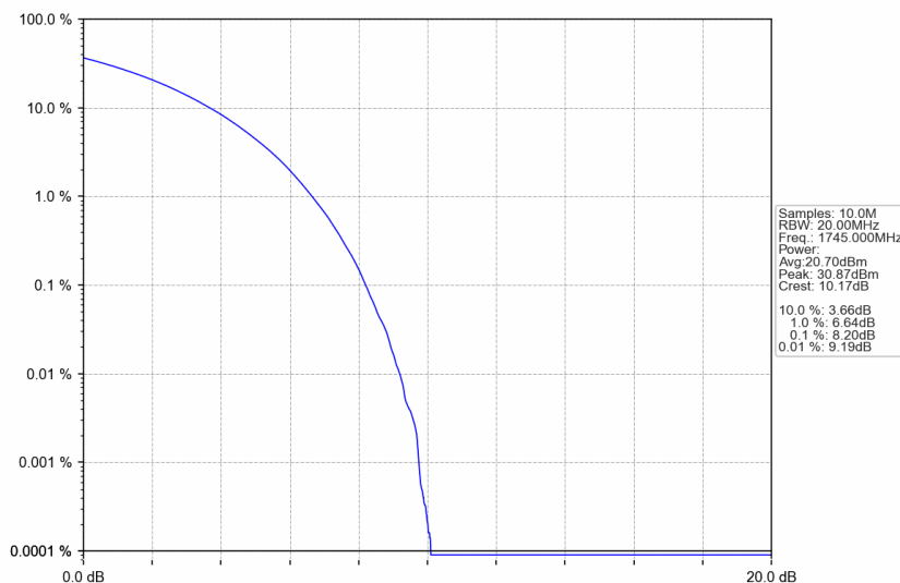
n66_30kHz_SISO_NTNV_35MHz_CP-OFDM 16 QAM_1745MHz_Outer_Full
