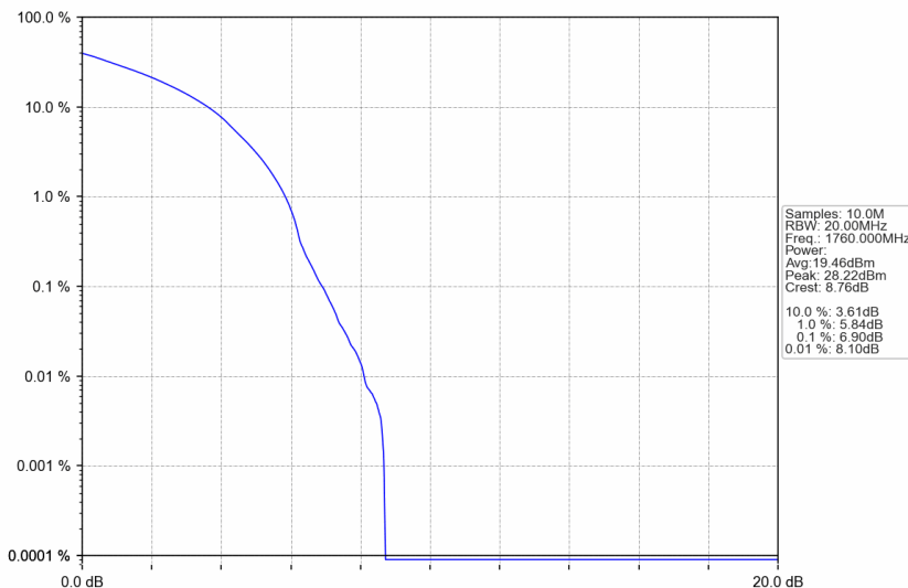
n66_30kHz_SISO_NTNV_40MHz_DFT-s-OFDM 64 QAM_1760MHz_Outer_Full
