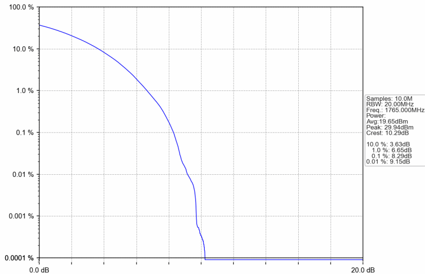
n66_30kHz_SISO_NTNV_30MHz_CP-OFDM 64 QAM_1765MHz_Outer_Full
