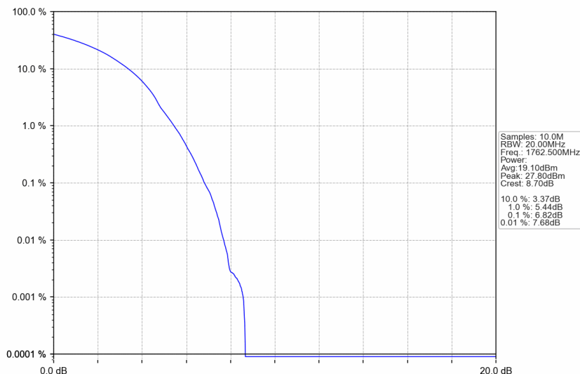
n66_30kHz_SISO_NTNV_35MHz_DFT-s-OFDM 256 QAM_1762.5MHz_Outer_Full
