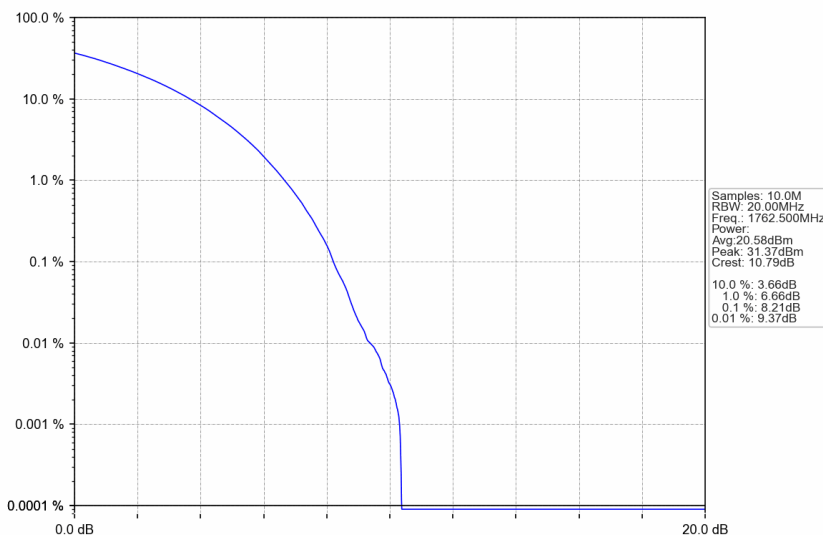
n66_30kHz_SISO_NTNV_35MHz_CP-OFDM QPSK_1762.5MHz_Outer_Full
