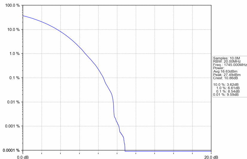
n66_30kHz_SISO_NTNV_30MHz_CP-OFDM 256 QAM_1745MHz_Outer_Full
