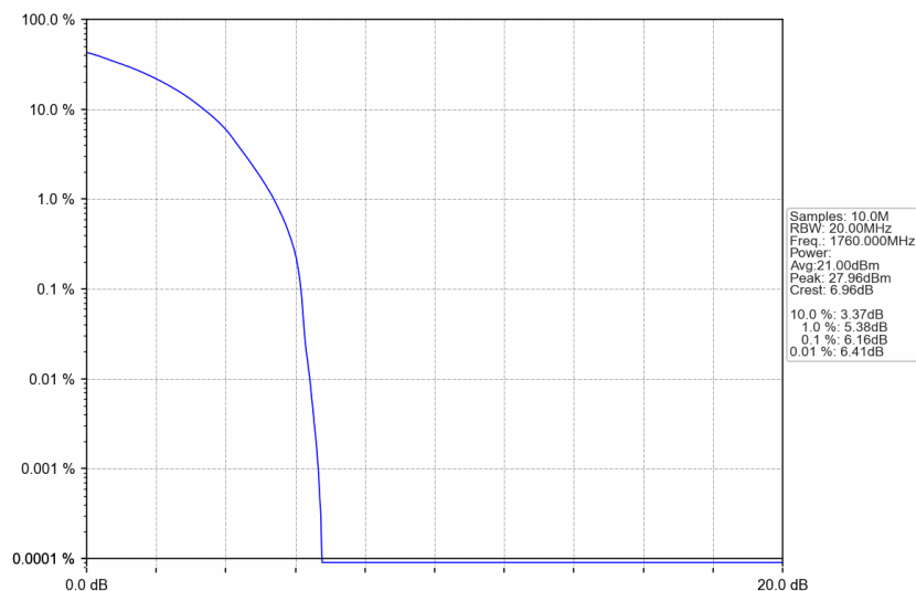
n66_30kHz_SISO_NTNV_40MHz_DFT-s-OFDM QPSK_1760MHz_Outer_Full
