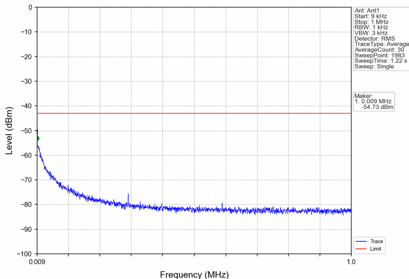
n66_15kHz_SISO_NTNV_5MHz_DFT-s-OFDM QPSK_1777.5MHz_Edge_1RB_Right
