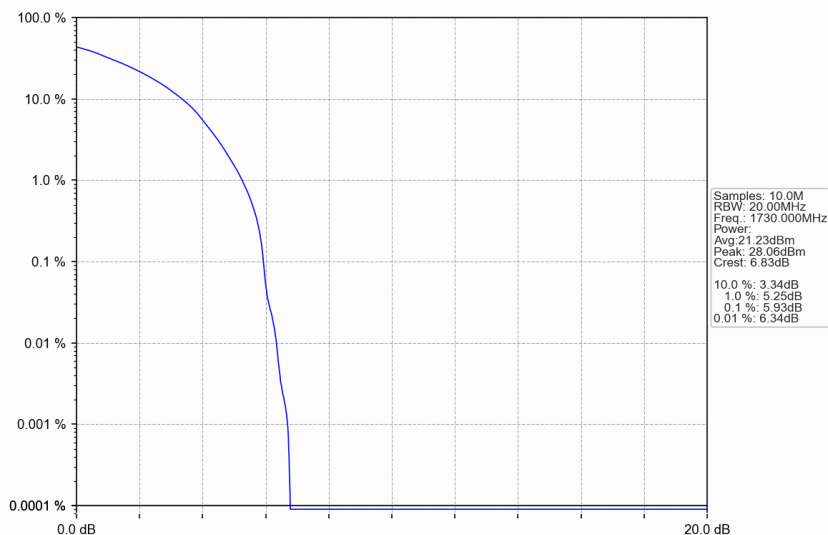
n66_30kHz_SISO_NTNV_40MHz_DFT-s-OFDM QPSK_1730MHz_Outer_Full
