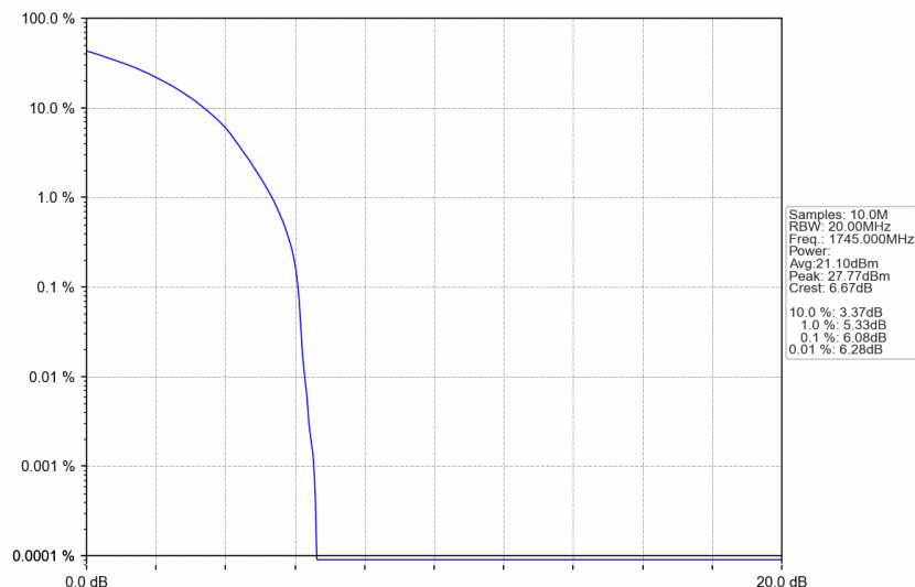
n66_30kHz_SISO_NTNV_40MHz_DFT-s-OFDM QPSK_1745MHz_Outer_Full
