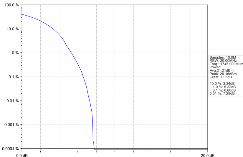
n66_30kHz_SISO_NTNV_35MHz_DFT-s-OFDM 64 QAM_1745MHz_Outer_Full
