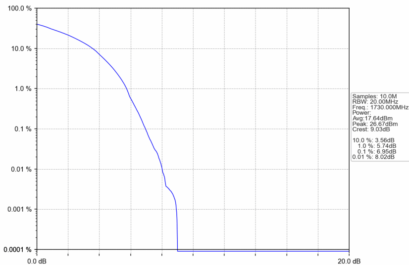
n66_30kHz_SISO_NTNV_40MHz_DFT-s-OFDM 256 QAM_1730MHz_Outer_Full
