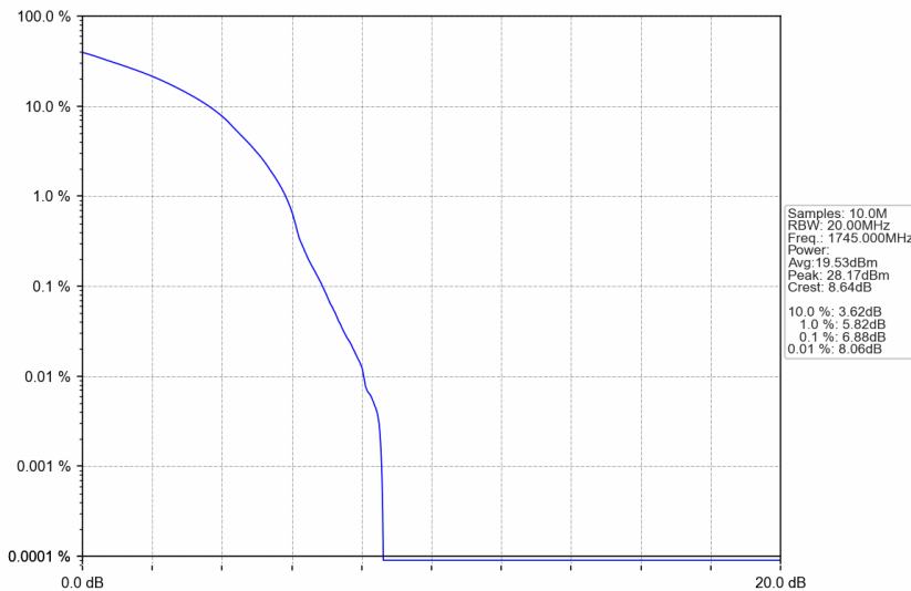
n66_30kHz_SISO_NTNV_40MHz_DFT-s-OFDM 64 QAM_1745MHz_Outer_Full
