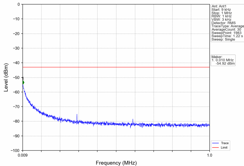
n66_15kHz_SISO_NTNV_5MHz_DFT-s-OFDM PI/2 BPSK_1777.5MHz_Edge_1RB_Right
