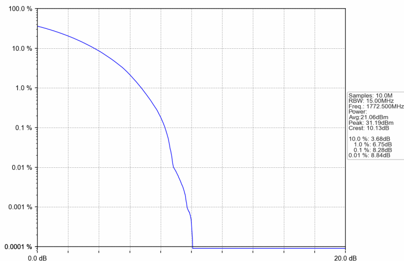
n66_30kHz_SISO_NTNV_15MHz_CP-OFDM 64 QAM_1772.5MHz_Outer_Full
