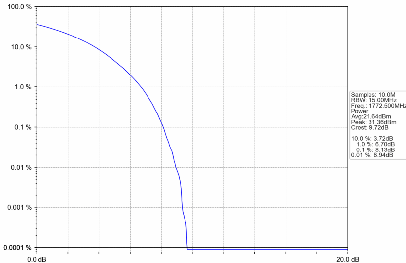
n66_30kHz_SISO_NTNV_15MHz_CP-OFDM QPSK_1772.5MHz_Outer_Full
