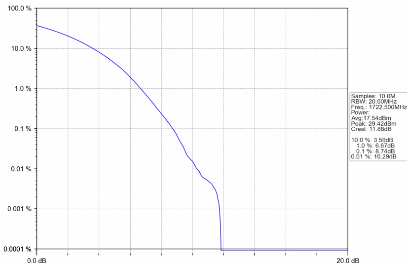
n66_30kHz_SISO_NTNV_25MHz_CP-OFDM 256 QAM_1722.5MHz_Outer_Full
