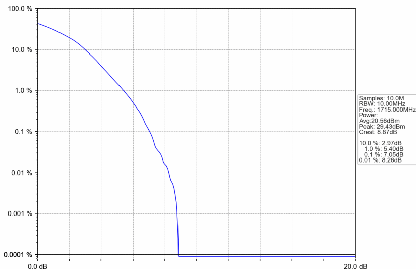
n66_30kHz_SISO_NTNV_10MHz_DFT-s-OFDM 256 QAM_1715MHz_Outer_Full
