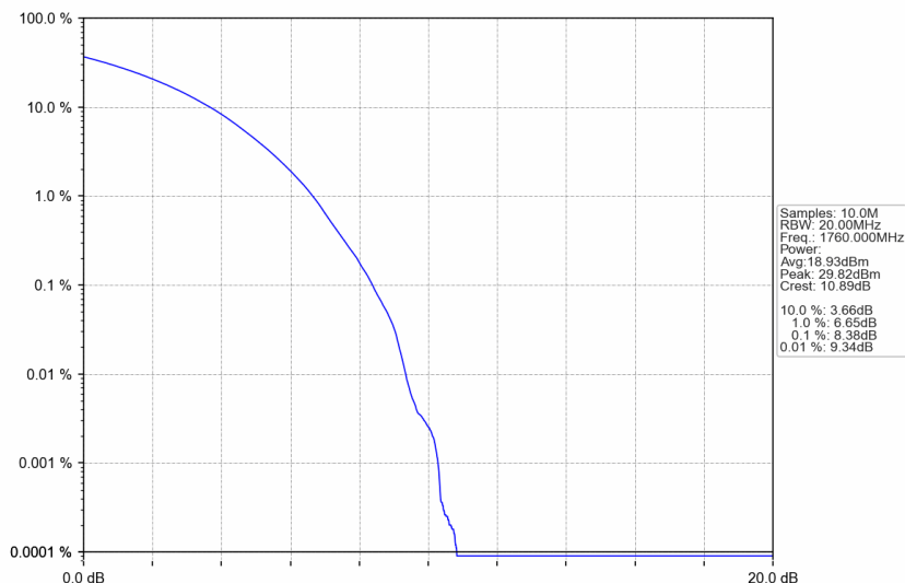
n66_15kHz_SISO_NTNV_40MHz_CP-OFDM 16 QAM_1760MHz_Outer_Full
