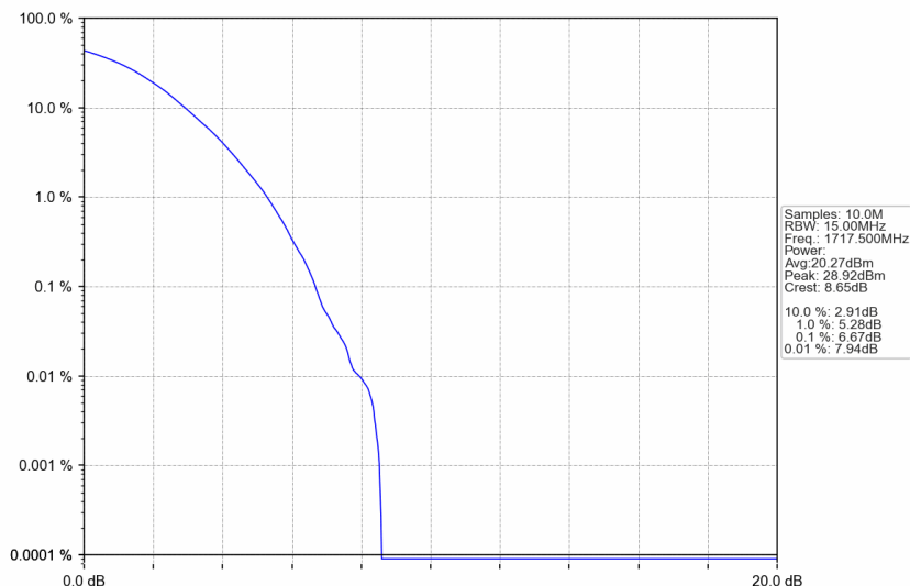
n66_30kHz_SISO_NTNV_15MHz_DFT-s-OFDM 256 QAM_1717.5MHz_Outer_Full
