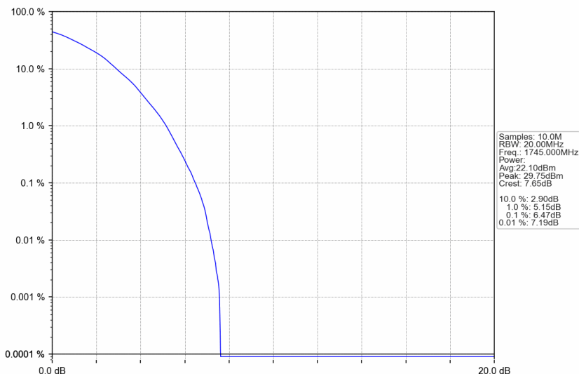
n66_30kHz_SISO_NTNV_20MHz_DFT-s-OFDM 64 QAM_1745MHz_Outer_Full
