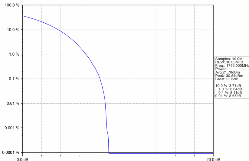
n66_30kHz_SISO_NTNV_10MHz_CP-OFDM QPSK_1745MHz_Outer_Full
