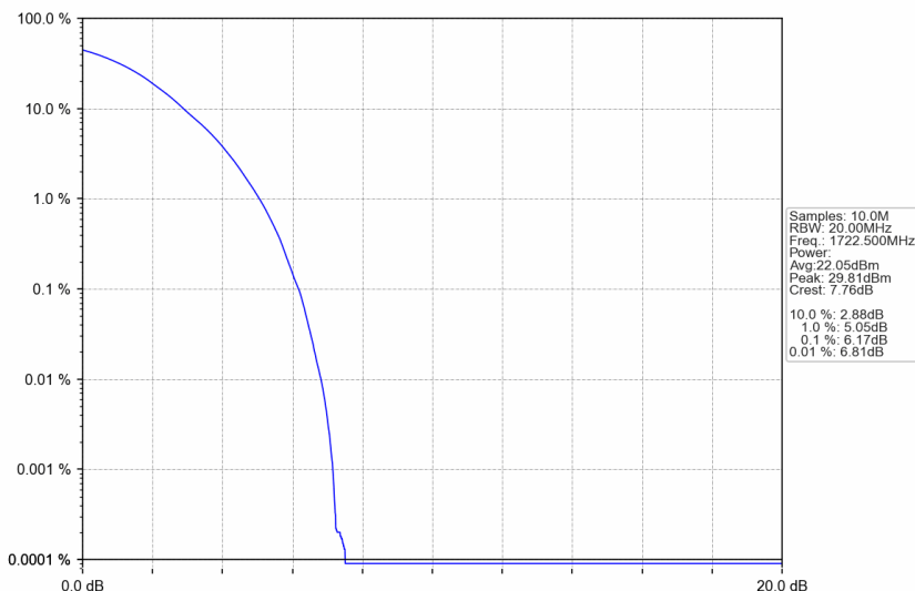
n66_30kHz_SISO_NTNV_25MHz_DFT-s-OFDM 16 QAM_1722.5MHz_Outer_Full
