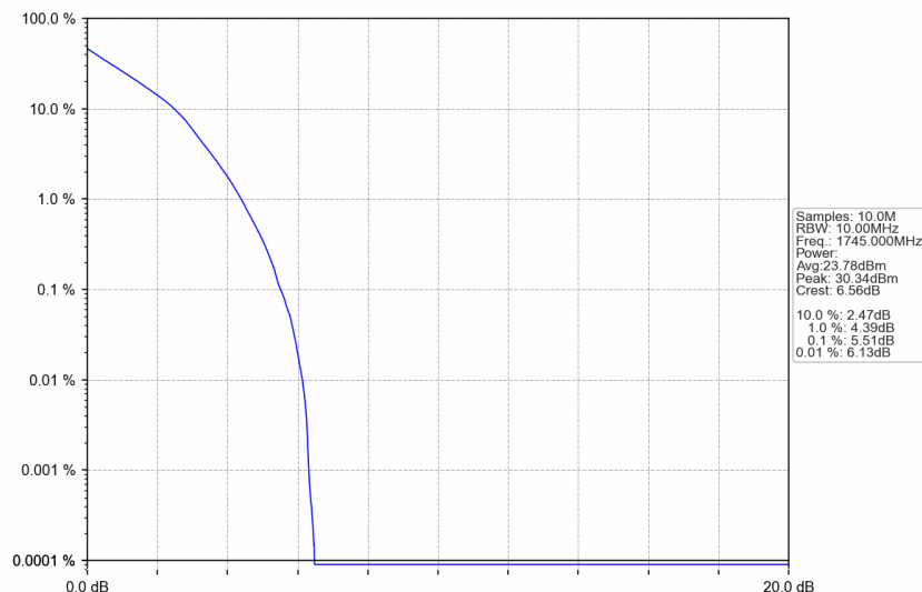
n66_30kHz_SISO_NTNV_10MHz_DFT-s-OFDM QPSK_1745MHz_Outer_Full
