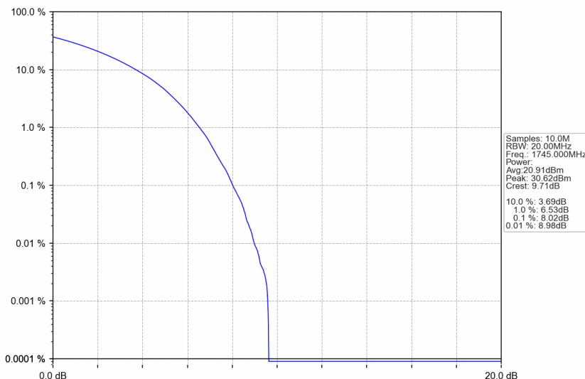
n66_30kHz_SISO_NTNV_25MHz_CP-OFDM QPSK_1745MHz_Outer_Full
