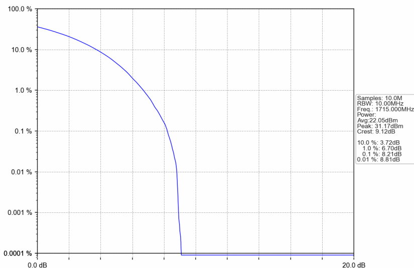
n66_30kHz_SISO_NTNV_10MHz_CP-OFDM QPSK_1715MHz_Outer_Full
