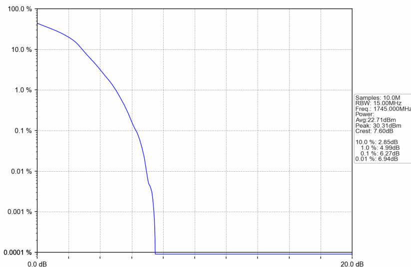
n66_30kHz_SISO_NTNV_15MHz_DFT-s-OFDM 16 QAM_1745MHz_Outer_Full
