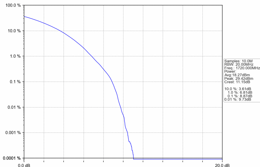
n66_30kHz_SISO_NTNV_20MHz_CP-OFDM 256 QAM_1720MHz_Outer_Full
