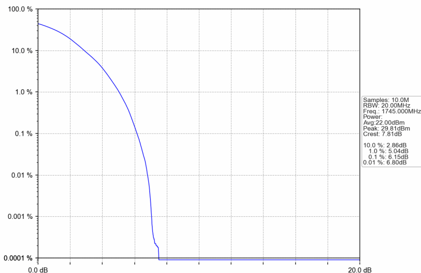
n66_30kHz_SISO_NTNV_25MHz_DFT-s-OFDM 16 QAM_1745MHz_Outer_Full
