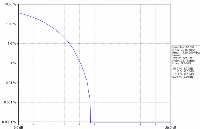
n66_30kHz_SISO_NTNV_20MHz_CP-OFDM QPSK_1720MHz_Outer_Full
