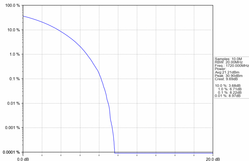
n66_30kHz_SISO_NTNV_20MHz_CP-OFDM 64 QAM_1720MHz_Outer_Full
