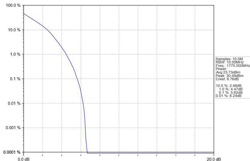
n66_30kHz_SISO_NTNV_10MHz_DFT-s-OFDM QPSK_1775MHz_Outer_Full
