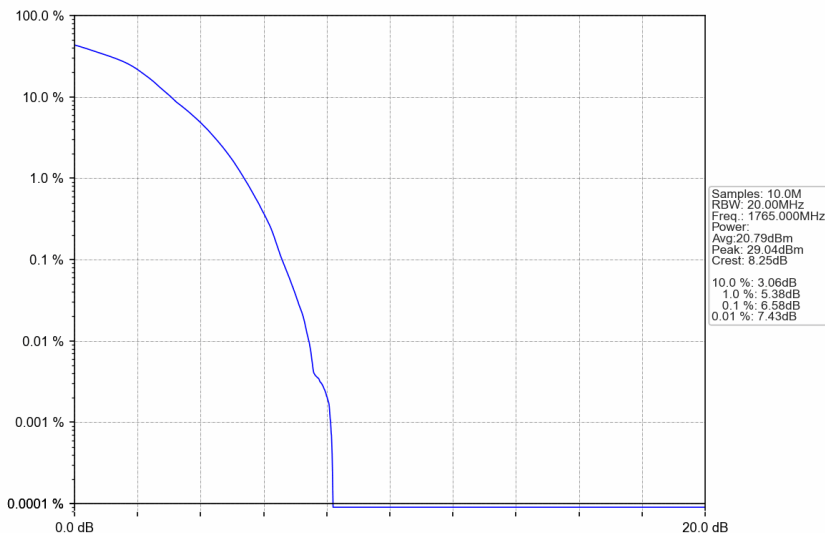
n66_30kHz_SISO_NTNV_30MHz_DFT-s-OFDM 64 QAM_1765MHz_Outer_Full
