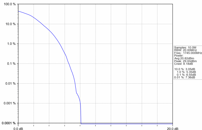
n66_30kHz_SISO_NTNV_30MHz_DFT-s-OFDM 64 QAM_1745MHz_Outer_Full
