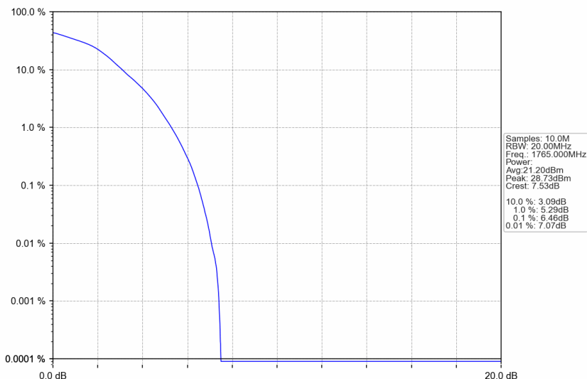
n66_30kHz_SISO_NTNV_30MHz_DFT-s-OFDM 16 QAM_1765MHz_Outer_Full
