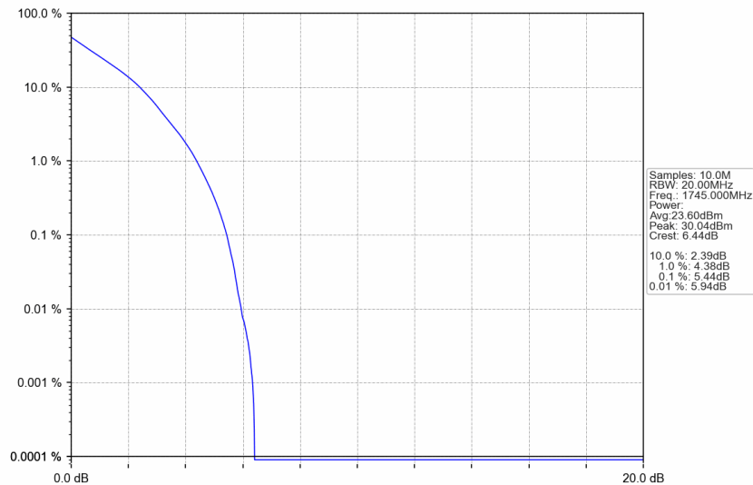
n66_30kHz_SISO_NTNV_20MHz_DFT-s-OFDM QPSK_1745MHz_Outer_Full
