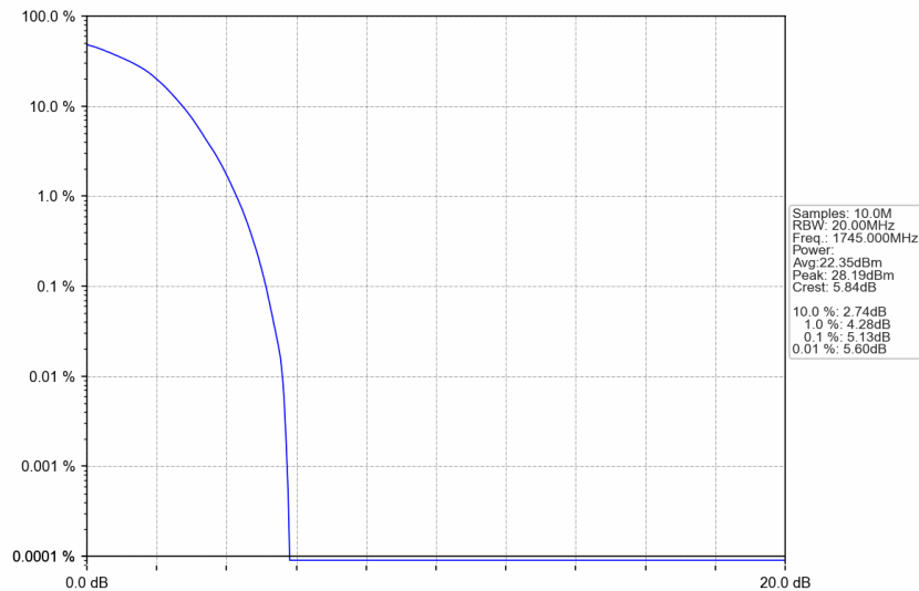
n66_30kHz_SISO_NTNV_30MHz_DFT-s-OFDM QPSK_1745MHz_Outer_Full
