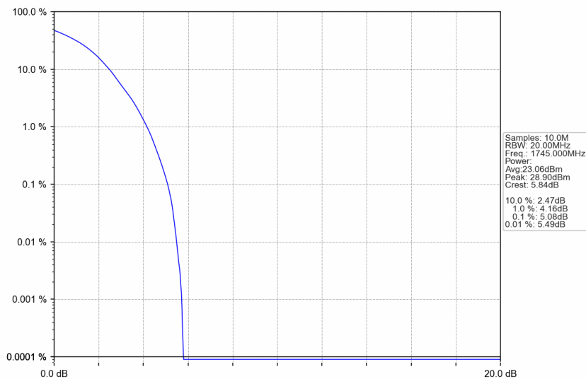
n66_30kHz_SISO_NTNV_25MHz_DFT-s-OFDM QPSK_1745MHz_Outer_Full
