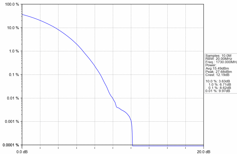
n66_15kHz_SISO_NTNV_40MHz_CP-OFDM 256 QAM_1730MHz_Outer_Full
