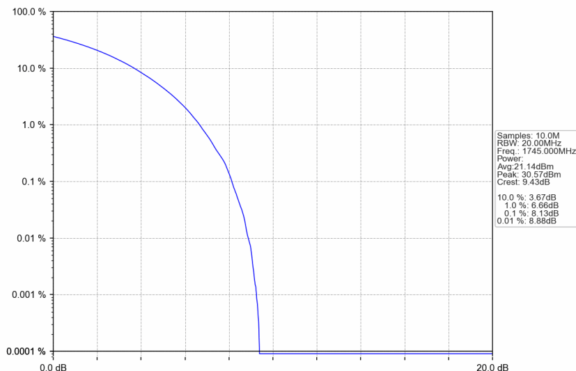
n66_30kHz_SISO_NTNV_20MHz_CP-OFDM 64 QAM_1745MHz_Outer_Full
