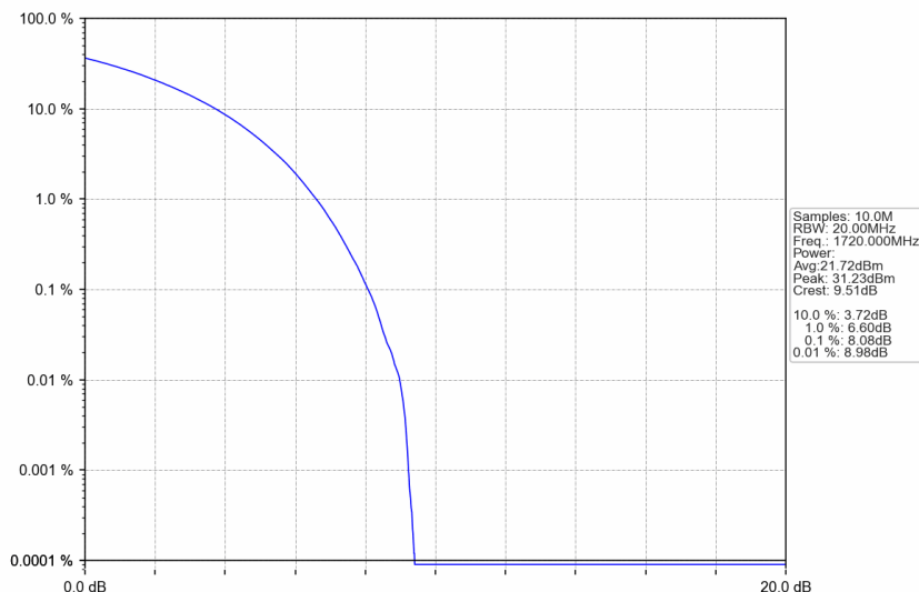
n66_30kHz_SISO_NTNV_20MHz_CP-OFDM 16 QAM_1720MHz_Outer_Full
