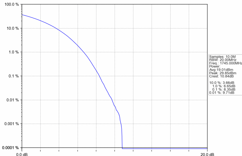
n66_15kHz_SISO_NTNV_40MHz_CP-OFDM QPSK_1745MHz_Outer_Full
