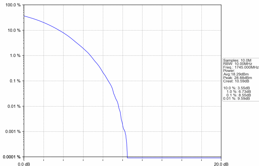
n66_30kHz_SISO_NTNV_10MHz_CP-OFDM 256 QAM_1745MHz_Outer_Full
