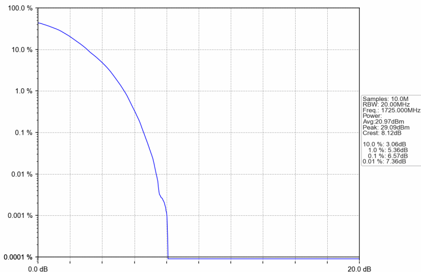
n66_30kHz_SISO_NTNV_30MHz_DFT-s-OFDM 64 QAM_1725MHz_Outer_Full
