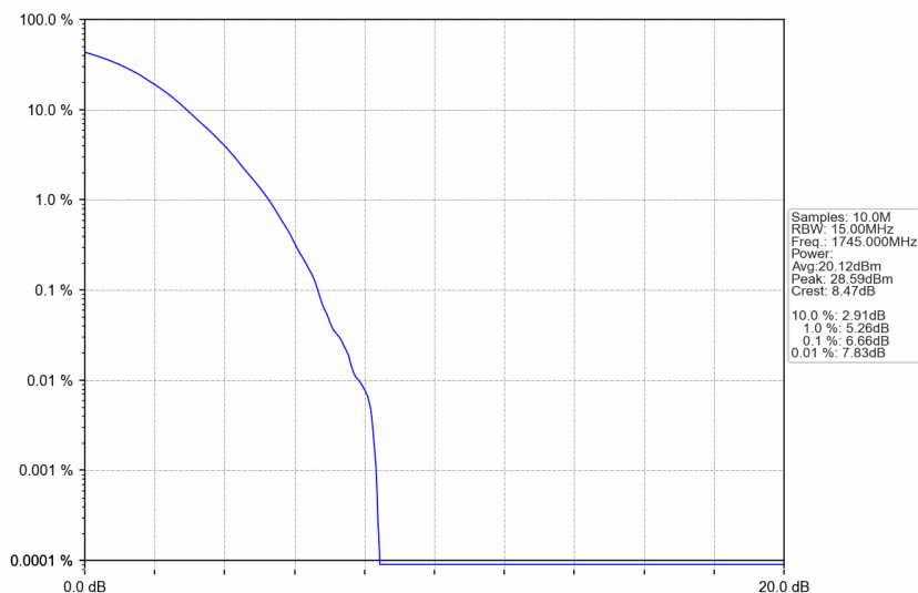
n66_30kHz_SISO_NTNV_15MHz_DFT-s-OFDM 256 QAM_1745MHz_Outer_Full
