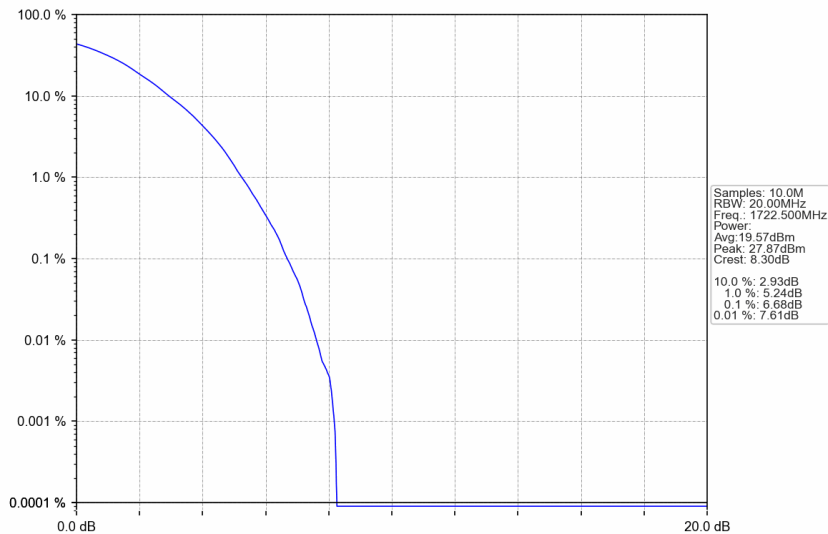
n66_30kHz_SISO_NTNV_25MHz_DFT-s-OFDM 256 QAM_1722.5MHz_Outer_Full
