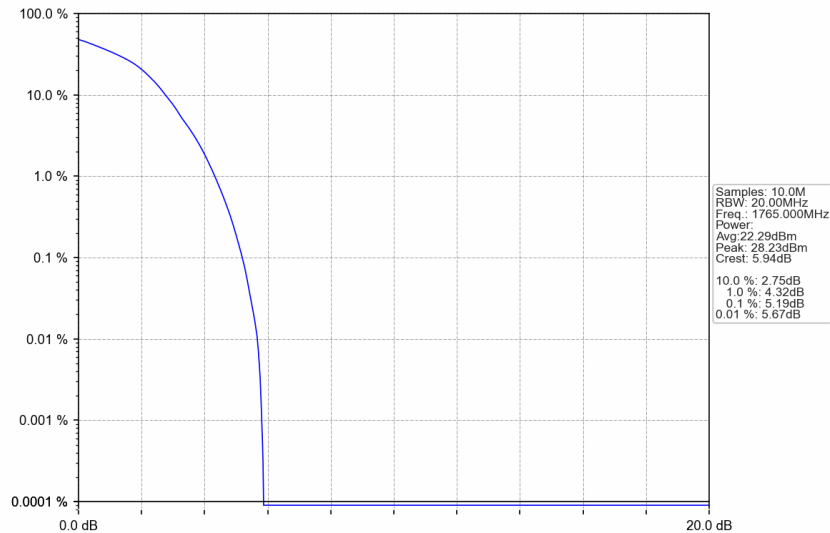
n66_30kHz_SISO_NTNV_30MHz_DFT-s-OFDM QPSK_1765MHz_Outer_Full
