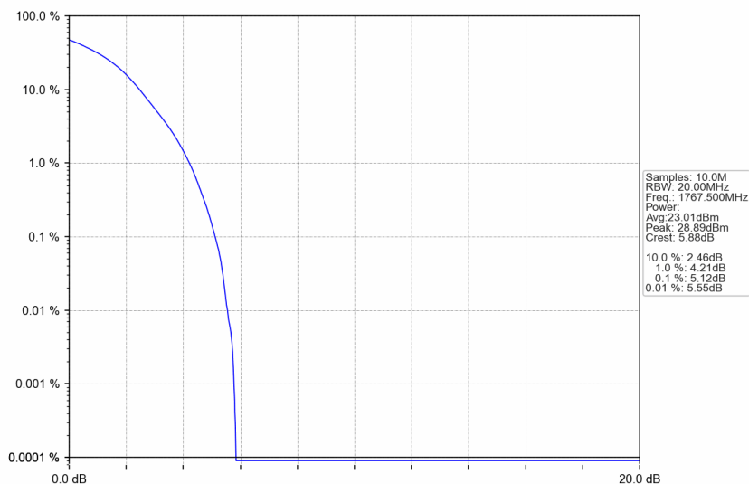
n66_30kHz_SISO_NTNV_25MHz_DFT-s-OFDM QPSK_1767.5MHz_Outer_Full
