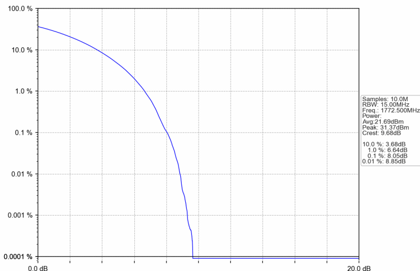
n66_30kHz_SISO_NTNV_15MHz_CP-OFDM 16 QAM_1772.5MHz_Outer_Full
