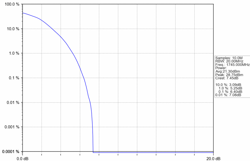
n66_30kHz_SISO_NTNV_30MHz_DFT-s-OFDM 16 QAM_1745MHz_Outer_Full
