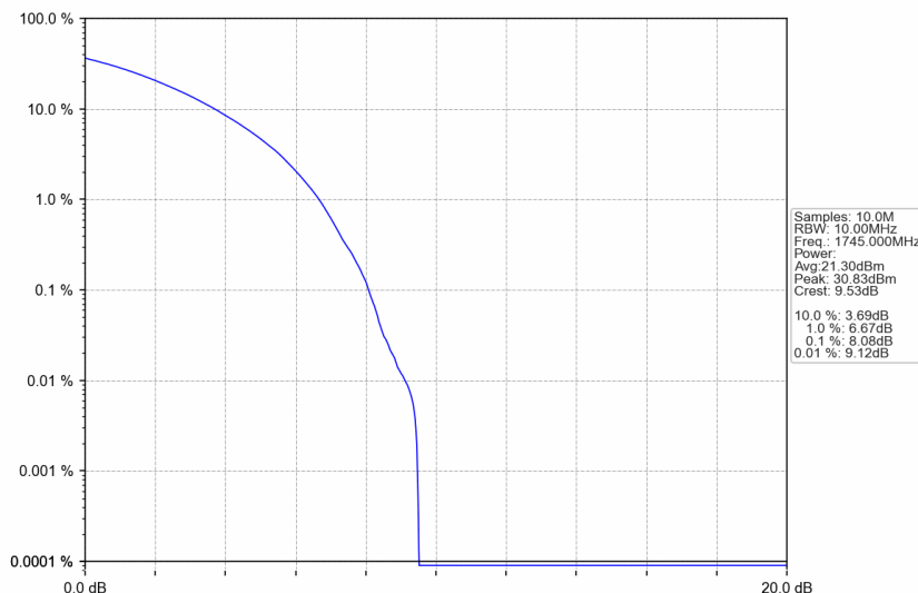
n66_30kHz_SISO_NTNV_10MHz_CP-OFDM 64 QAM_1745MHz_Outer_Full
