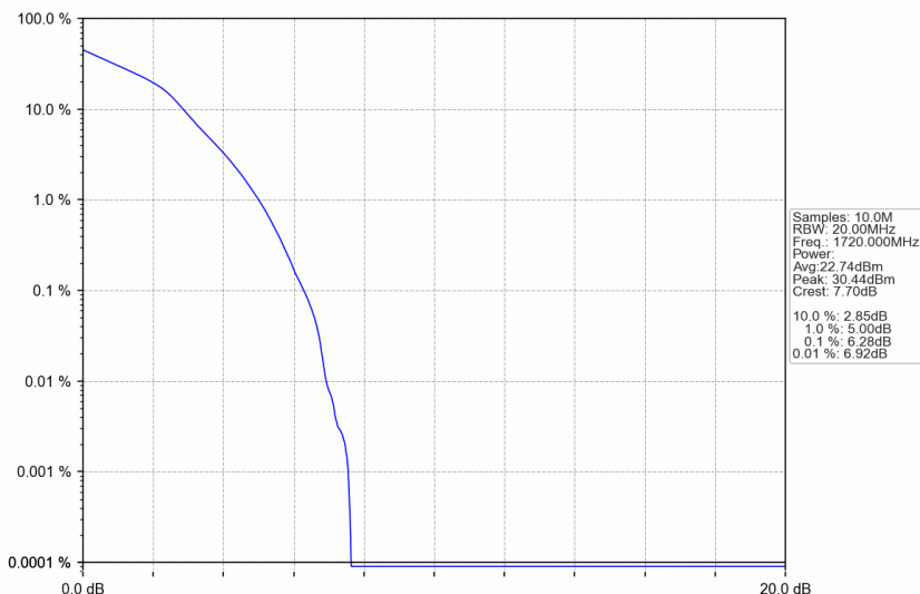
n66_30kHz_SISO_NTNV_20MHz_DFT-s-OFDM 16 QAM_1720MHz_Outer_Full
