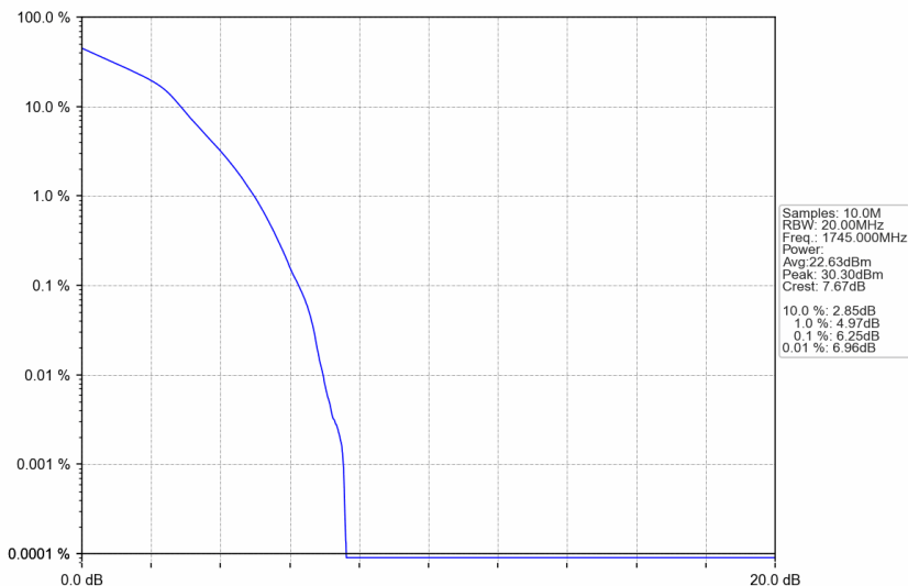
n66_30kHz_SISO_NTNV_20MHz_DFT-s-OFDM 16 QAM_1745MHz_Outer_Full
