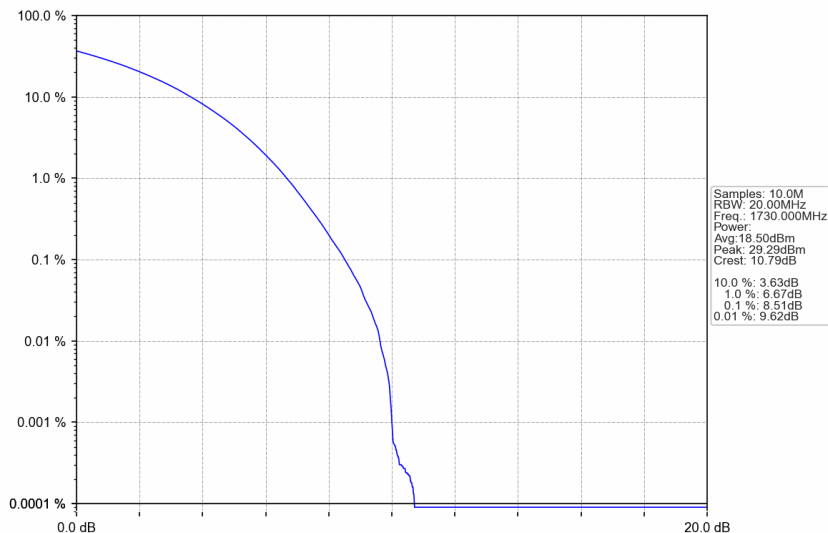
n66_15kHz_SISO_NTNV_40MHz_CP-OFDM 64 QAM_1730MHz_Outer_Full
