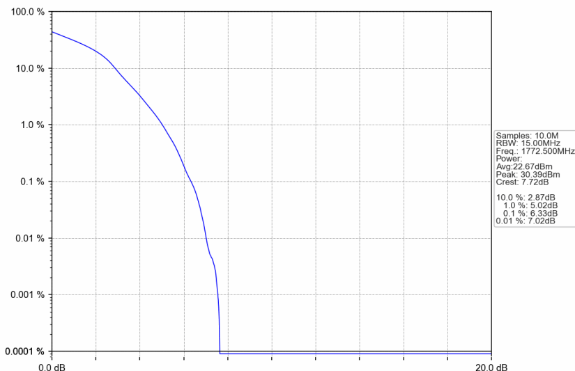
n66_30kHz_SISO_NTNV_15MHz_DFT-s-OFDM 16 QAM_1772.5MHz_Outer_Full
