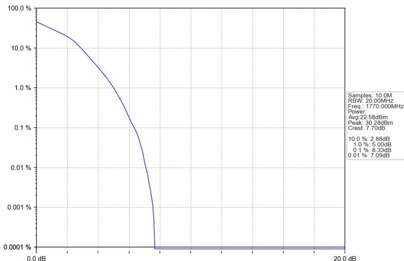
n66_30kHz_SISO_NTNV_20MHz_DFT-s-OFDM 16 QAM_1770MHz_Outer_Full
