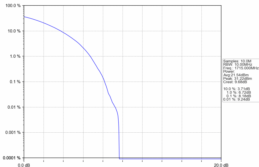
n66_30kHz_SISO_NTNV_10MHz_CP-OFDM 64 QAM_1715MHz_Outer_Full
