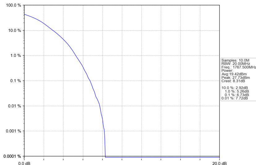
n66_30kHz_SISO_NTNV_25MHz_DFT-s-OFDM 256 QAM_1767.5MHz_Outer_Full
