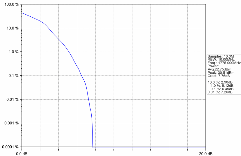
n66_30kHz_SISO_NTNV_10MHz_DFT-s-OFDM 16 QAM_1775MHz_Outer_Full
