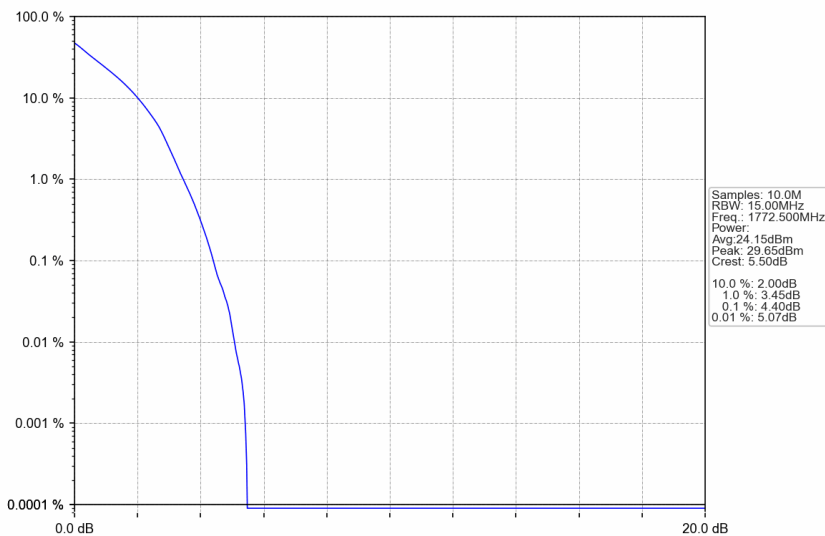
n66_30kHz_SISO_NTNV_15MHz_DFT-s-OFDM PI/2 BPSK_1772.5MHz_Outer_Full
