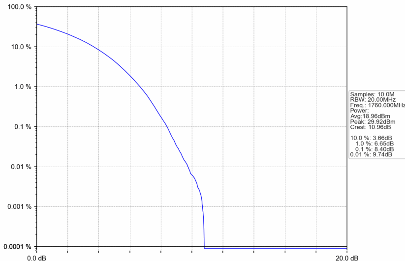
n66_15kHz_SISO_NTNV_40MHz_CP-OFDM QPSK_1760MHz_Outer_Full
