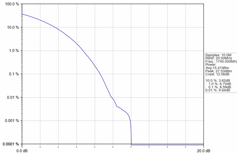
n66_15kHz_SISO_NTNV_40MHz_CP-OFDM 256 QAM_1745MHz_Outer_Full
