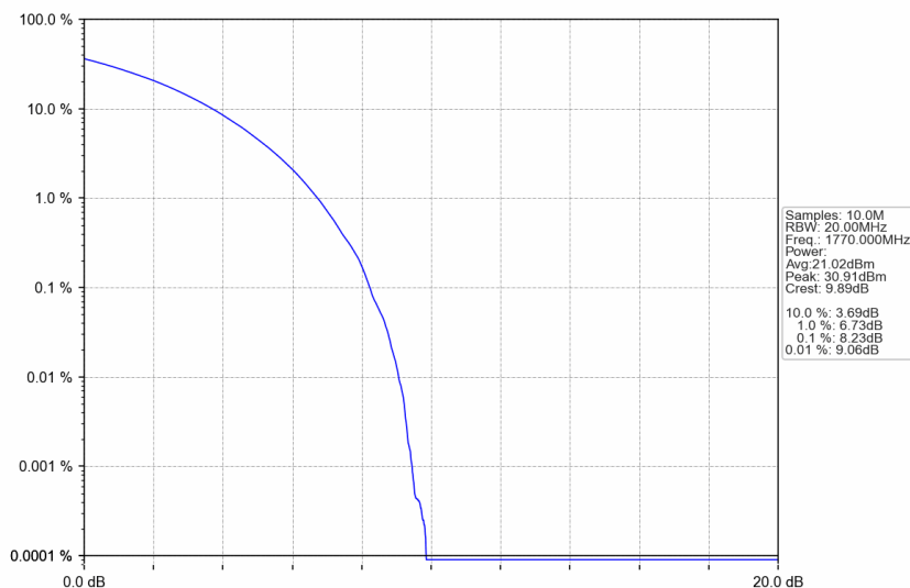
n66_30kHz_SISO_NTNV_20MHz_CP-OFDM 64 QAM_1770MHz_Outer_Full
