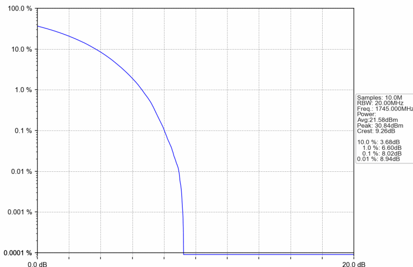
n66_30kHz_SISO_NTNV_20MHz_CP-OFDM QPSK_1745MHz_Outer_Full
