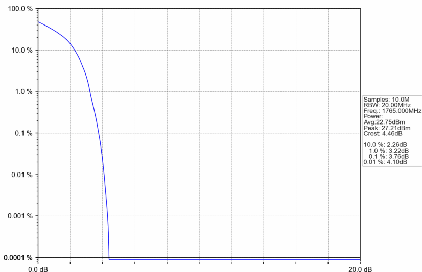
n66_30kHz_SISO_NTNV_30MHz_DFT-s-OFDM PI/2 BPSK_1765MHz_Outer_Full
