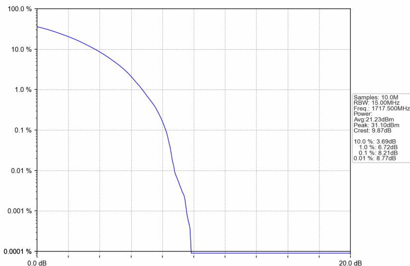
n66_30kHz_SISO_NTNV_15MHz_CP-OFDM 64 QAM_1717.5MHz_Outer_Full
