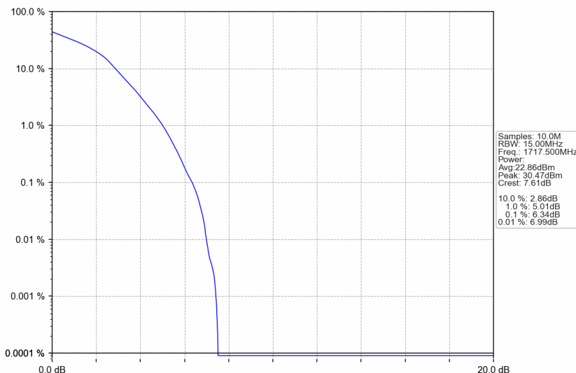
n66_30kHz_SISO_NTNV_15MHz_DFT-s-OFDM 16 QAM_1717.5MHz_Outer_Full
