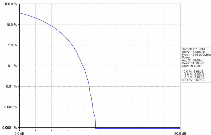
n66_30kHz_SISO_NTNV_15MHz_CP-OFDM 16 QAM_1745MHz_Outer_Full
