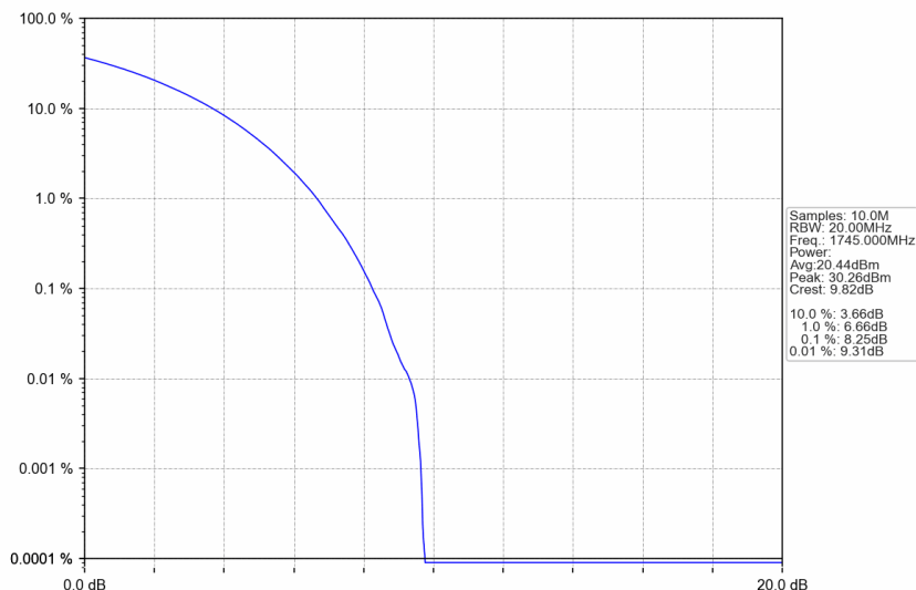
n66_30kHz_SISO_NTNV_25MHz_CP-OFDM 64 QAM_1745MHz_Outer_Full
