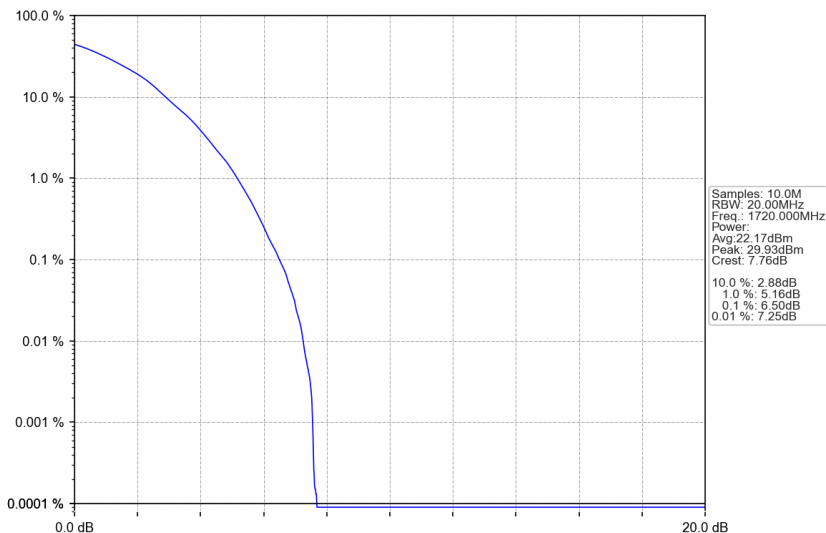
n66_30kHz_SISO_NTNV_20MHz_DFT-s-OFDM 64 QAM_1720MHz_Outer_Full
