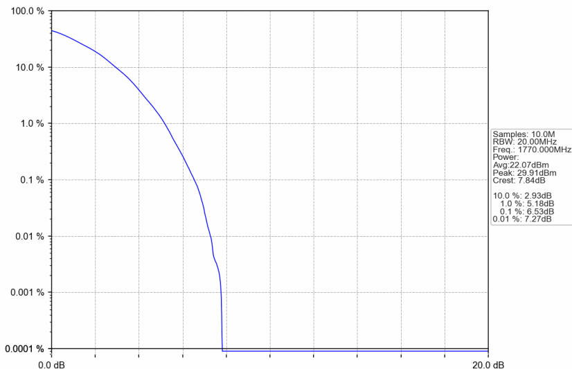
n66_30kHz_SISO_NTNV_20MHz_DFT-s-OFDM 64 QAM_1770MHz_Outer_Full
