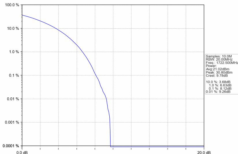
n66_30kHz_SISO_NTNV_25MHz_CP-OFDM 16 QAM_1722.5MHz_Outer_Full
