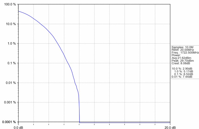
n66_30kHz_SISO_NTNV_25MHz_DFT-s-OFDM 64 QAM_1722.5MHz_Outer_Full
