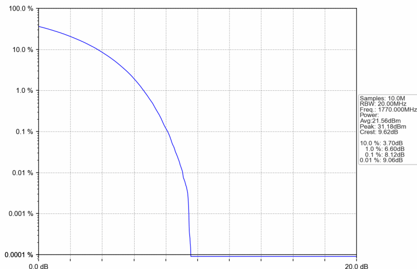
n66_30kHz_SISO_NTNV_20MHz_CP-OFDM 16 QAM_1770MHz_Outer_Full
