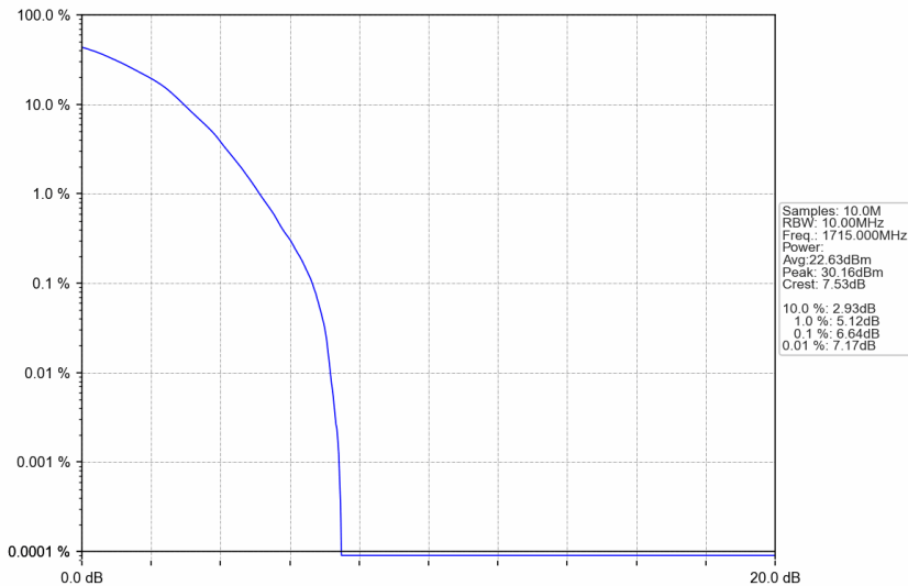
n66_30kHz_SISO_NTNV_10MHz_DFT-s-OFDM 64 QAM_1715MHz_Outer_Full
