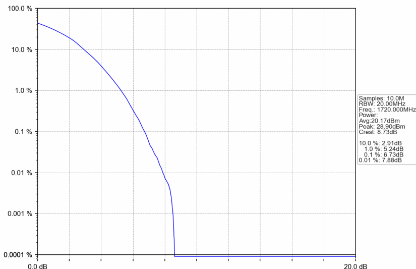
n66_30kHz_SISO_NTNV_20MHz_DFT-s-OFDM 256 QAM_1720MHz_Outer_Full
