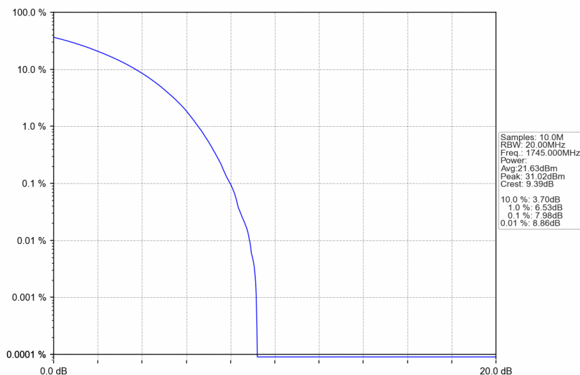
n66_30kHz_SISO_NTNV_20MHz_CP-OFDM 16 QAM_1745MHz_Outer_Full
