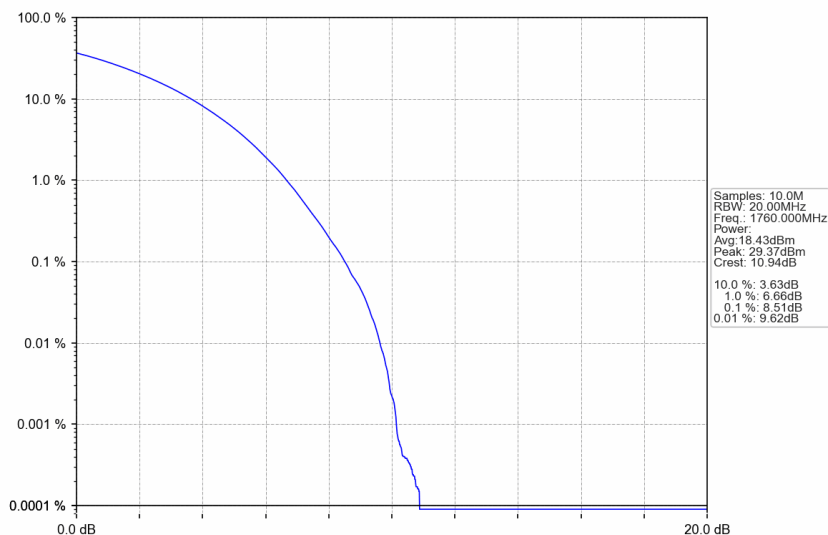
n66_15kHz_SISO_NTNV_40MHz_CP-OFDM 64 QAM_1760MHz_Outer_Full
