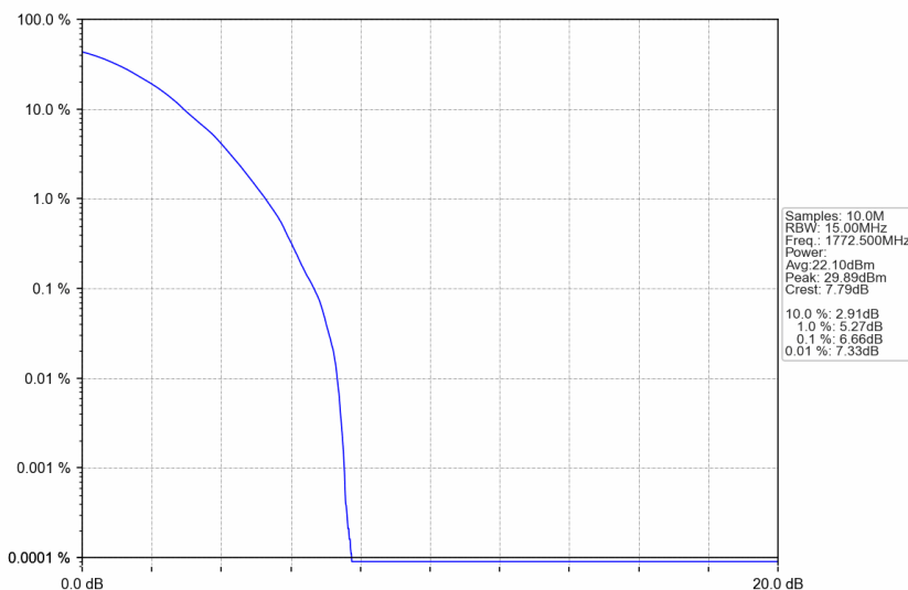
n66_30kHz_SISO_NTNV_15MHz_DFT-s-OFDM 64 QAM_1772.5MHz_Outer_Full
