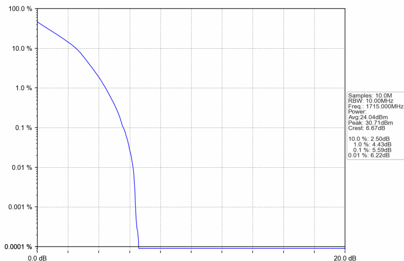
n66_30kHz_SISO_NTNV_10MHz_DFT-s-OFDM QPSK_1715MHz_Outer_Full
