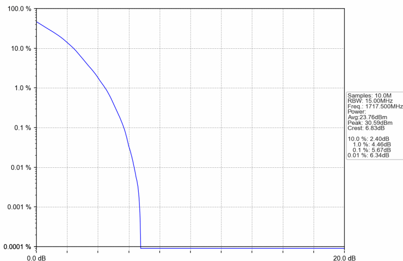
n66_30kHz_SISO_NTNV_15MHz_DFT-s-OFDM QPSK_1717.5MHz_Outer_Full
