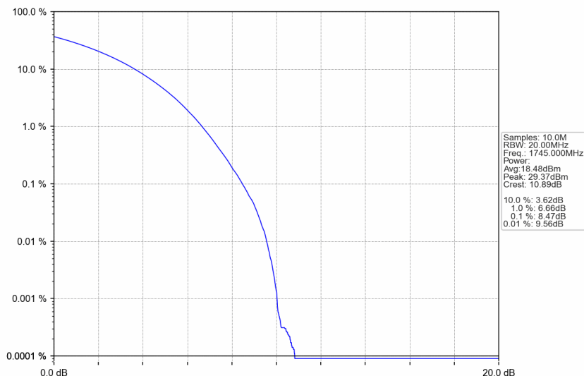
n66_15kHz_SISO_NTNV_40MHz_CP-OFDM 64 QAM_1745MHz_Outer_Full
