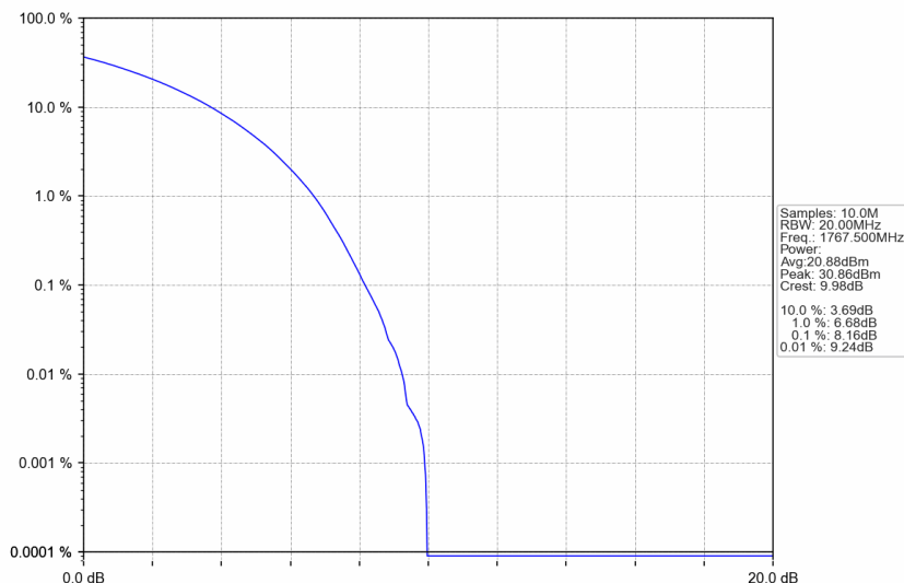
n66_30kHz_SISO_NTNV_25MHz_CP-OFDM 16 QAM_1767.5MHz_Outer_Full
