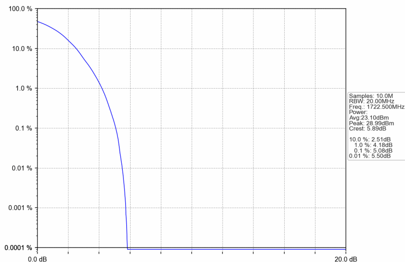
n66_30kHz_SISO_NTNV_25MHz_DFT-s-OFDM QPSK_1722.5MHz_Outer_Full
