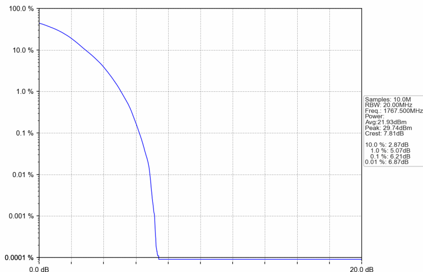
n66_30kHz_SISO_NTNV_25MHz_DFT-s-OFDM 16 QAM_1767.5MHz_Outer_Full
