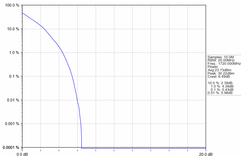
n66_30kHz_SISO_NTNV_20MHz_DFT-s-OFDM QPSK_1720MHz_Outer_Full
