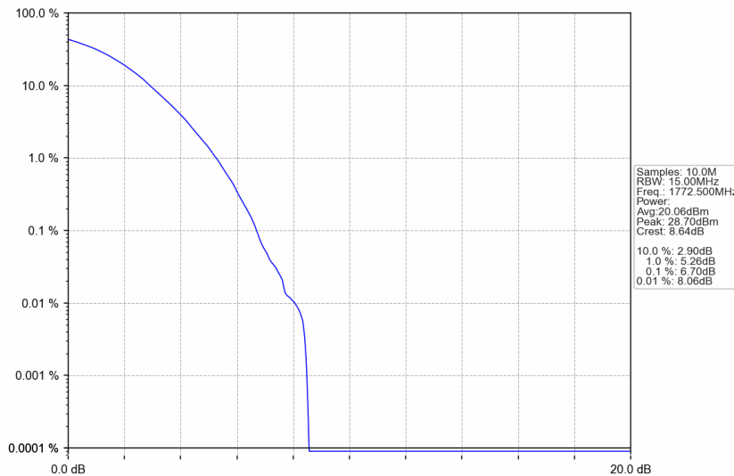
n66_30kHz_SISO_NTNV_15MHz_DFT-s-OFDM 256 QAM_1772.5MHz_Outer_Full
