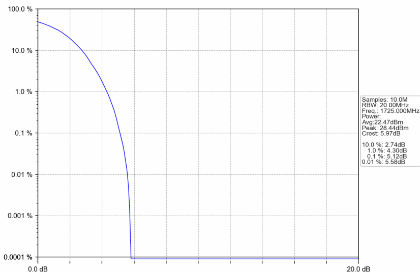
n66_30kHz_SISO_NTNV_30MHz_DFT-s-OFDM QPSK_1725MHz_Outer_Full
