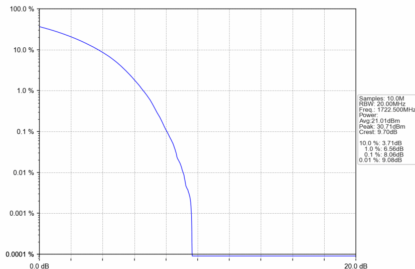
n66_30kHz_SISO_NTNV_25MHz_CP-OFDM QPSK_1722.5MHz_Outer_Full
