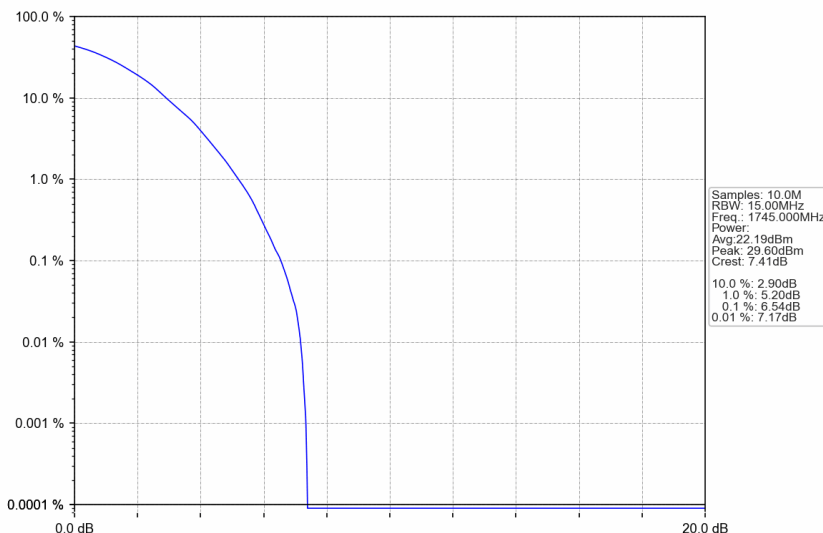
n66_30kHz_SISO_NTNV_15MHz_DFT-s-OFDM 64 QAM_1745MHz_Outer_Full
