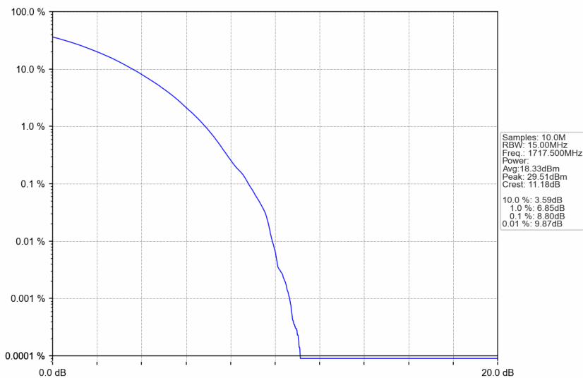
n66_30kHz_SISO_NTNV_15MHz_CP-OFDM 256 QAM_1717.5MHz_Outer_Full
