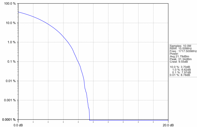
n66_30kHz_SISO_NTNV_15MHz_CP-OFDM 16 QAM_1717.5MHz_Outer_Full
