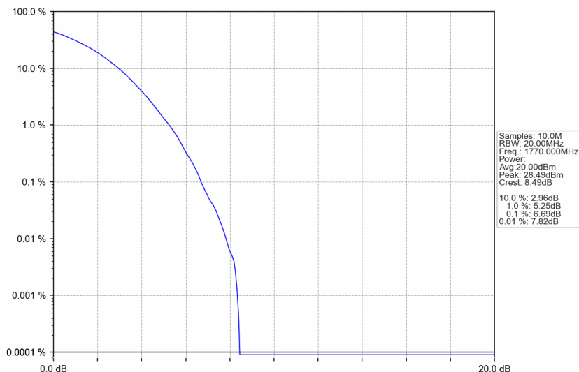
n66_30kHz_SISO_NTNV_20MHz_DFT-s-OFDM 256 QAM_1770MHz_Outer_Full
