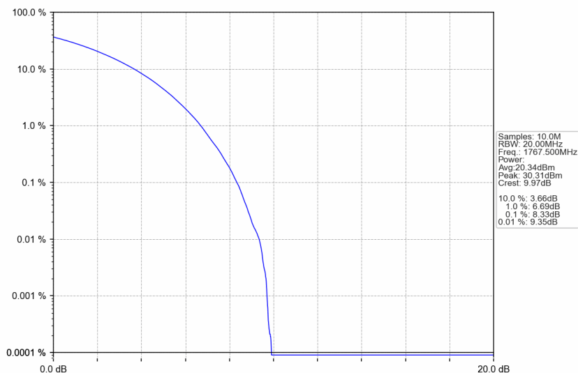
n66_30kHz_SISO_NTNV_25MHz_CP-OFDM 64 QAM_1767.5MHz_Outer_Full
