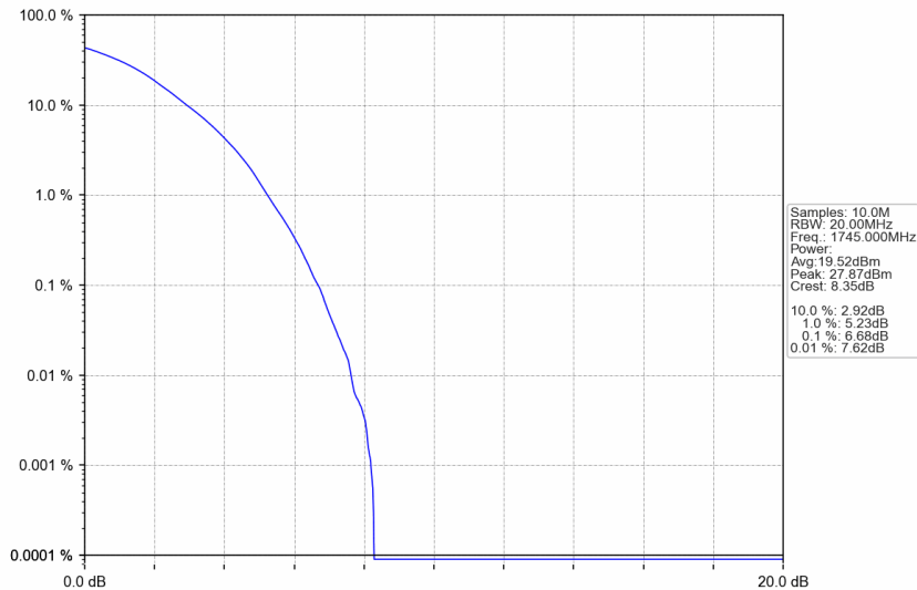
n66_30kHz_SISO_NTNV_25MHz_DFT-s-OFDM 256 QAM_1745MHz_Outer_Full
