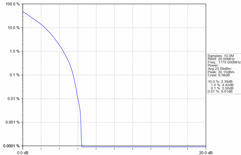
n66_30kHz_SISO_NTNV_20MHz_DFT-s-OFDM QPSK_1770MHz_Outer_Full
