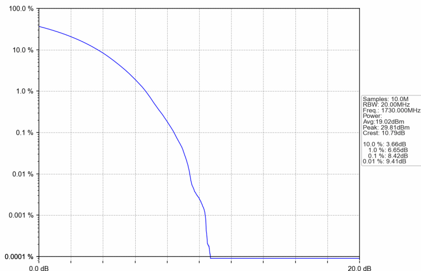
n66_15kHz_SISO_NTNV_40MHz_CP-OFDM 16 QAM_1730MHz_Outer_Full
