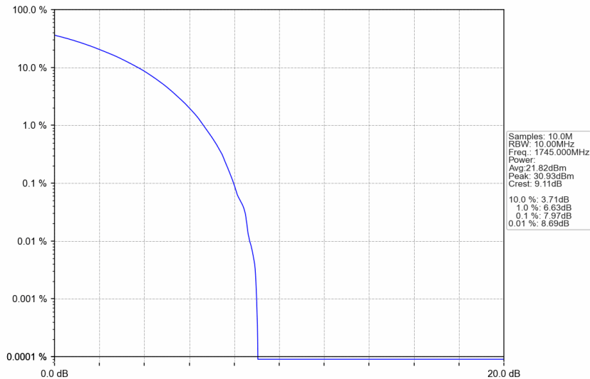
n66_30kHz_SISO_NTNV_10MHz_CP-OFDM 16 QAM_1745MHz_Outer_Full
