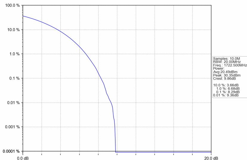
n66_30kHz_SISO_NTNV_25MHz_CP-OFDM 64 QAM_1722.5MHz_Outer_Full
