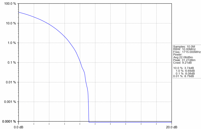
n66_30kHz_SISO_NTNV_10MHz_CP-OFDM 16 QAM_1715MHz_Outer_Full
