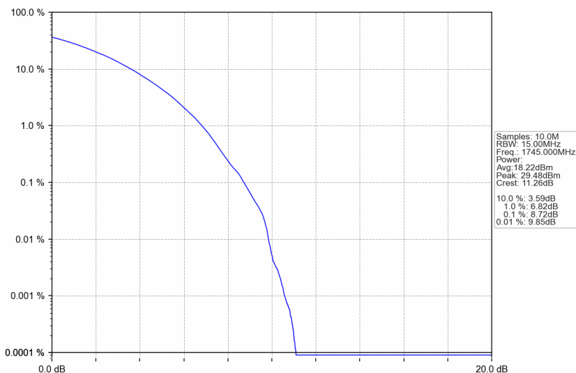
n66_30kHz_SISO_NTNV_15MHz_CP-OFDM 256 QAM_1745MHz_Outer_Full
