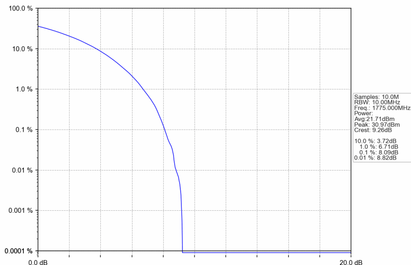
n66_30kHz_SISO_NTNV_10MHz_CP-OFDM 16 QAM_1775MHz_Outer_Full
