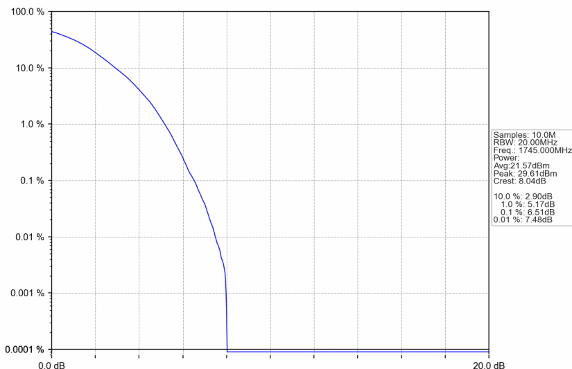
n66_30kHz_SISO_NTNV_25MHz_DFT-s-OFDM 64 QAM_1745MHz_Outer_Full
