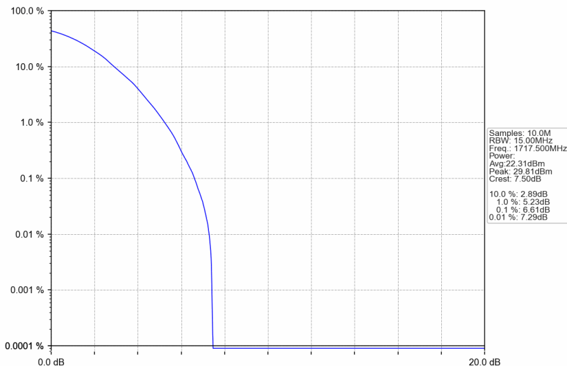
n66_30kHz_SISO_NTNV_15MHz_DFT-s-OFDM 64 QAM_1717.5MHz_Outer_Full
