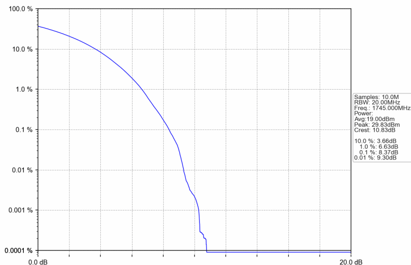
n66_15kHz_SISO_NTNV_40MHz_CP-OFDM 16 QAM_1745MHz_Outer_Full
