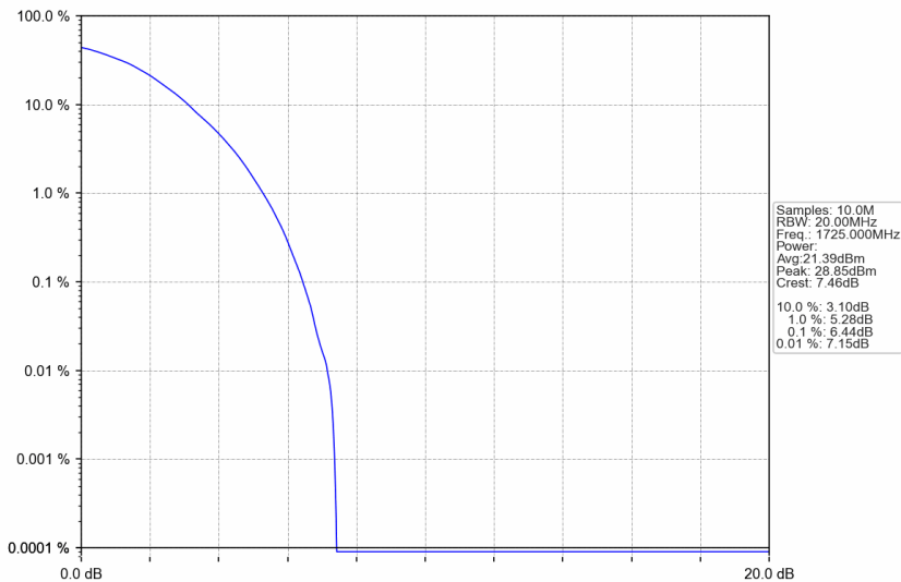
n66_30kHz_SISO_NTNV_30MHz_DFT-s-OFDM 16 QAM_1725MHz_Outer_Full
