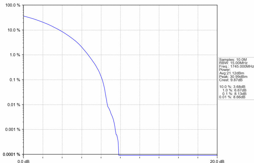
n66_30kHz_SISO_NTNV_15MHz_CP-OFDM 64 QAM_1745MHz_Outer_Full
