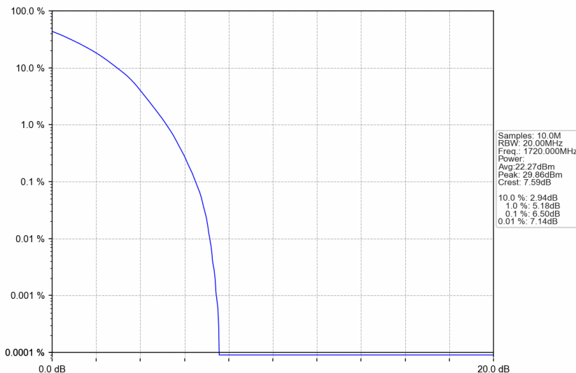
n66_15kHz_SISO_NTNV_20MHz_DFT-s-OFDM 64 QAM_1720MHz_Outer_Full
