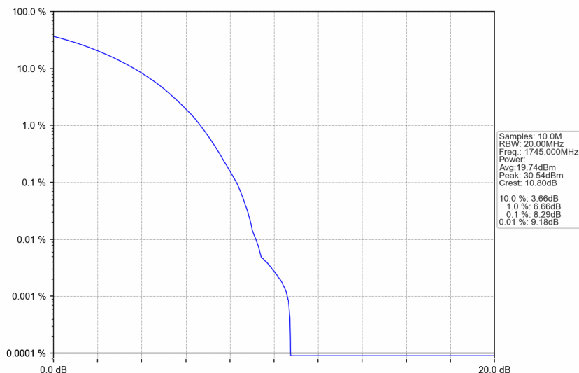
n66_15kHz_SISO_NTNV_30MHz_CP-OFDM 64 QAM_1745MHz_Outer_Full
