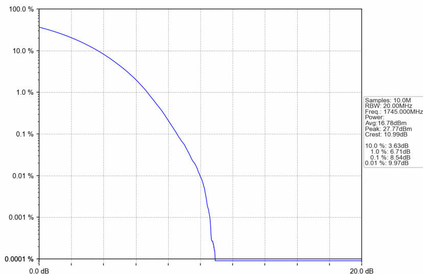
n66_15kHz_SISO_NTNV_35MHz_CP-OFDM 256 QAM_1745MHz_Outer_Full
