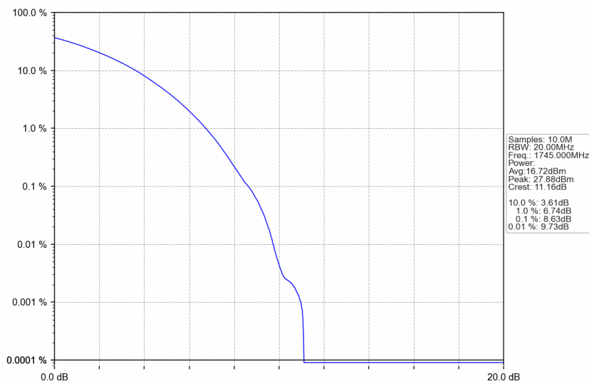
n66_15kHz_SISO_NTNV_30MHz_CP-OFDM 256 QAM_1745MHz_Outer_Full
