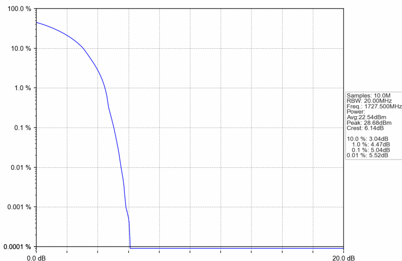
n66_15kHz_SISO_NTNV_35MHz_DFT-s-OFDM QPSK_1727.5MHz_Outer_Full
