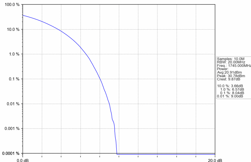
n66_15kHz_SISO_NTNV_25MHz_CP-OFDM QPSK_1745MHz_Outer_Full
