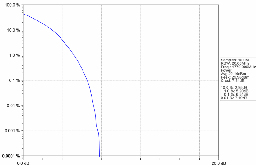
n66_15kHz_SISO_NTNV_20MHz_DFT-s-OFDM 64 QAM_1770MHz_Outer_Full
