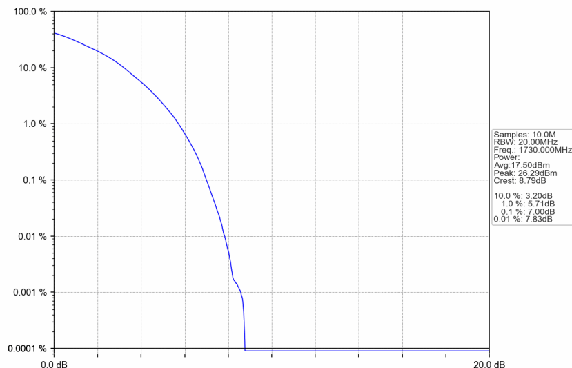
n66_15kHz_SISO_NTNV_40MHz_DFT-s-OFDM 256 QAM_1730MHz_Outer_Full
