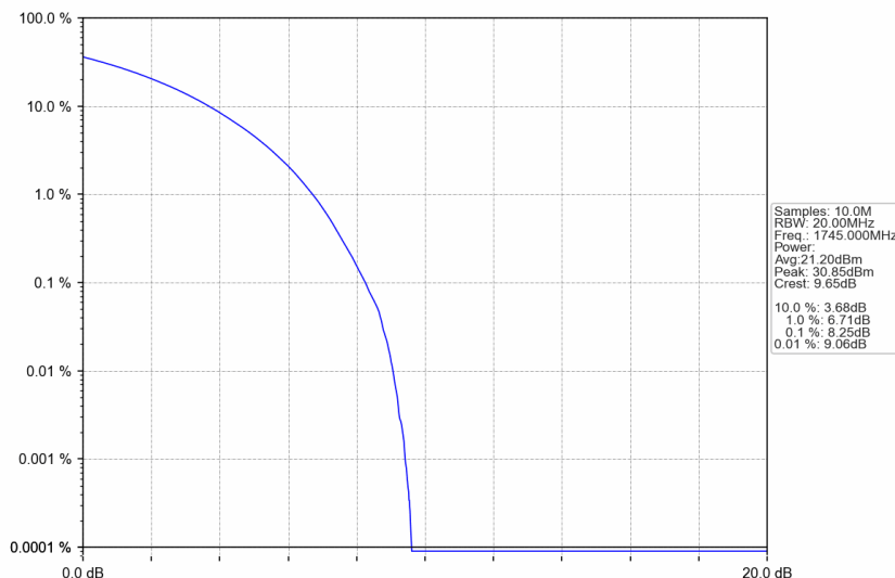
n66_15kHz_SISO_NTNV_20MHz_CP-OFDM 64 QAM_1745MHz_Outer_Full
