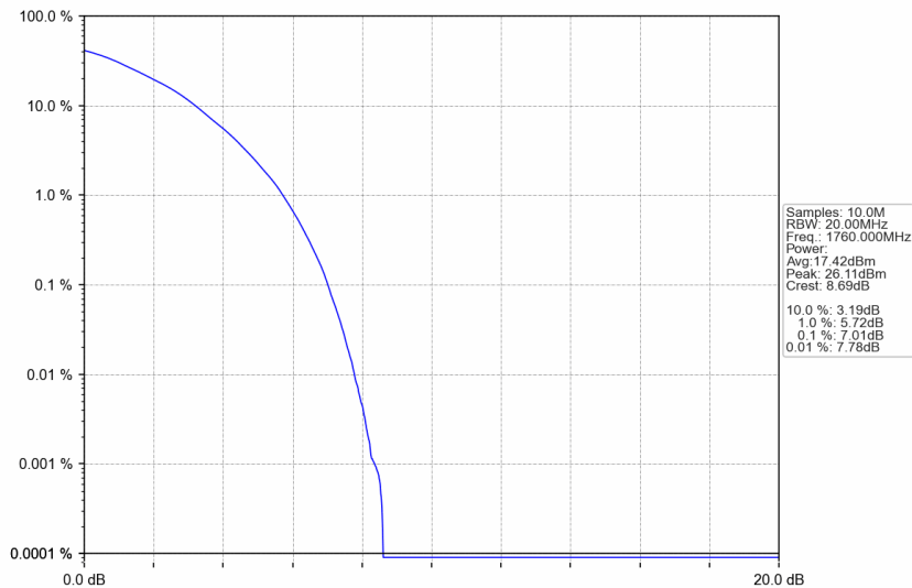
n66_15kHz_SISO_NTNV_40MHz_DFT-s-OFDM 256 QAM_1760MHz_Outer_Full
