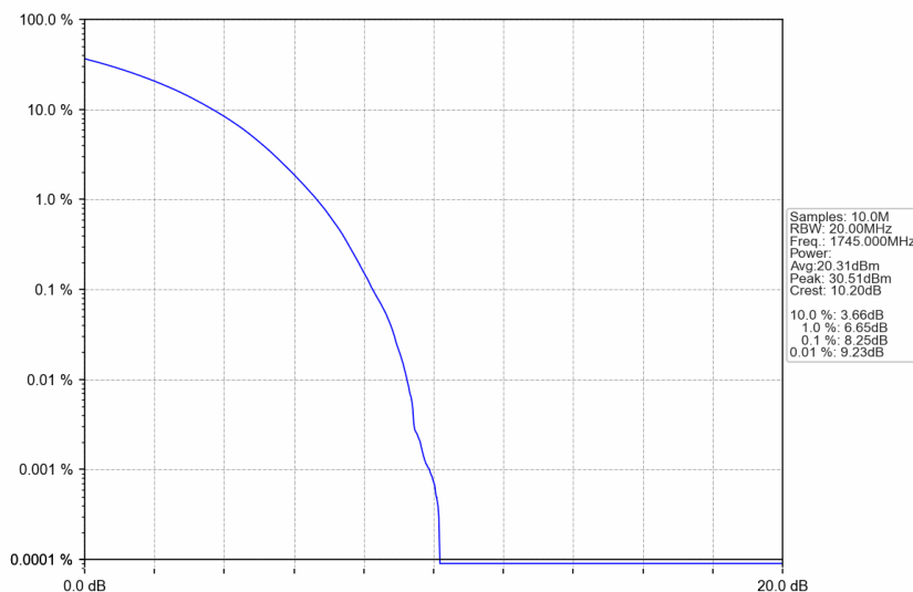
n66_15kHz_SISO_NTNV_35MHz_CP-OFDM 16 QAM_1745MHz_Outer_Full
