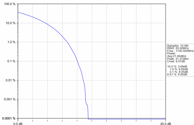
n66_15kHz_SISO_NTNV_20MHz_CP-OFDM 16 QAM_1720MHz_Outer_Full
