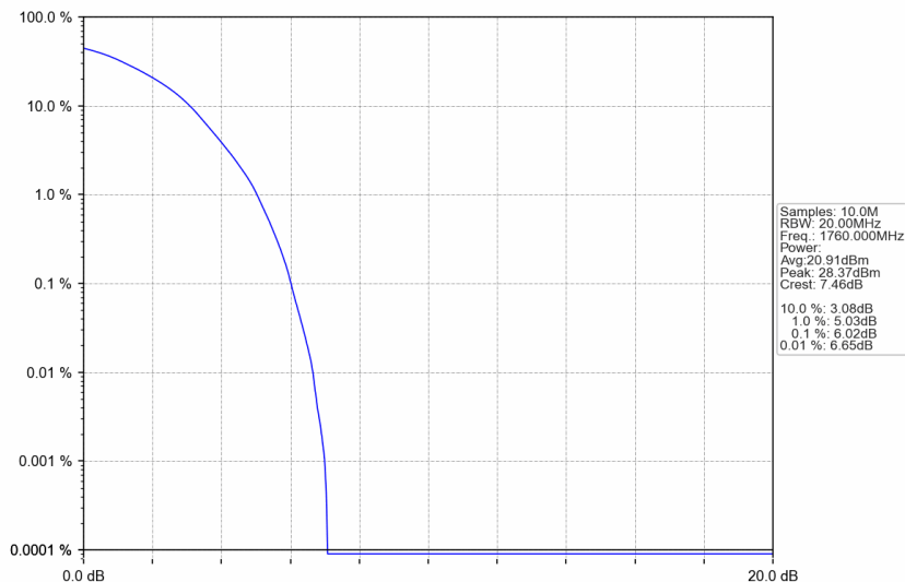
n66_15kHz_SISO_NTNV_40MHz_DFT-s-OFDM_QPSK_1760MHz_Outer_Full
