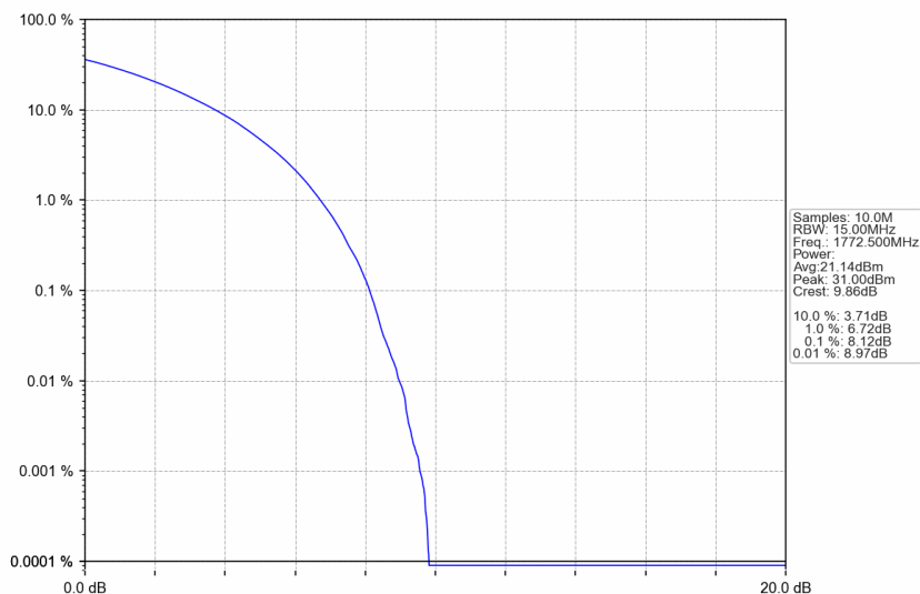
n66_15kHz_SISO_NTNV_15MHz_CP-OFDM 64 QAM_1772.5MHz_Outer_Full
