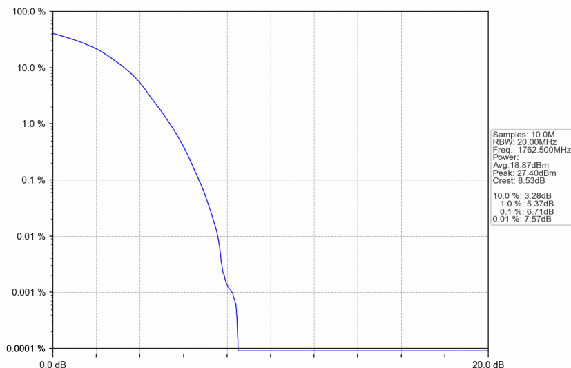
n66_15kHz_SISO_NTNV_35MHz_DFT-s-OFDM 256 QAM_1762.5MHz_Outer_Full
