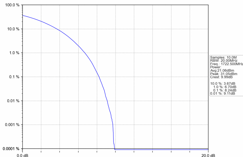
n66_15kHz_SISO_NTNV_25MHz_CP-OFDM 16 QAM_1722.5MHz_Outer_Full
