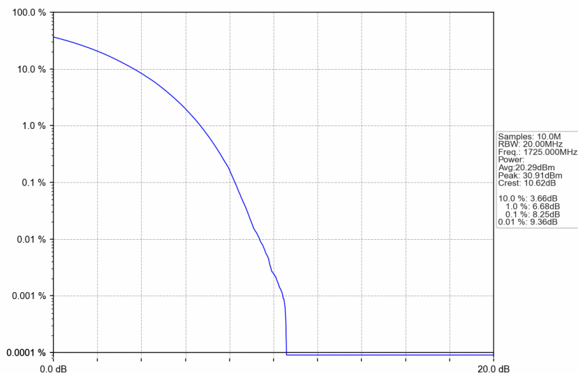
n66_15kHz_SISO_NTNV_30MHz_CP-OFDM QPSK_1725MHz_Outer_Full
