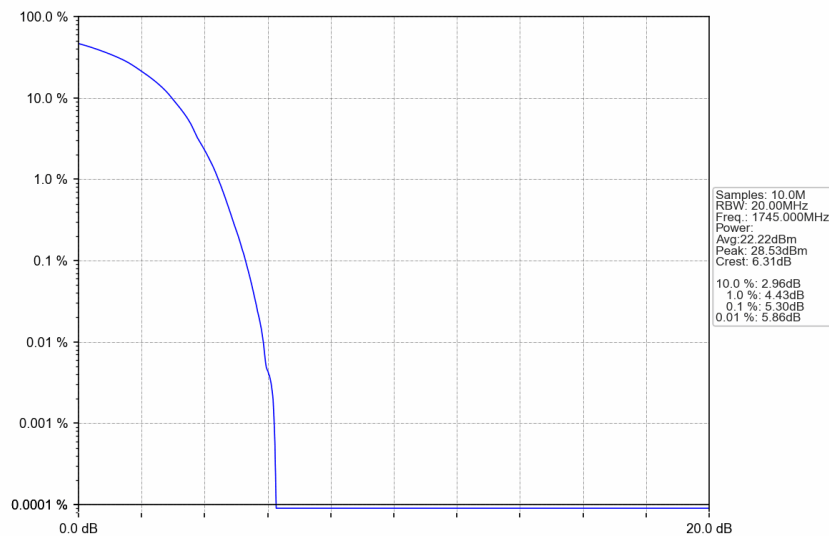
n66_15kHz_SISO_NTNV_30MHz_DFT-s-OFDM QPSK_1745MHz_Outer_Full
