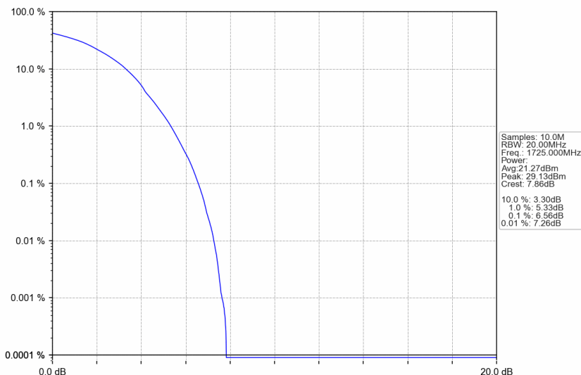
n66_15kHz_SISO_NTNV_30MHz_DFT-s-OFDM 16 QAM_1725MHz_Outer_Full
