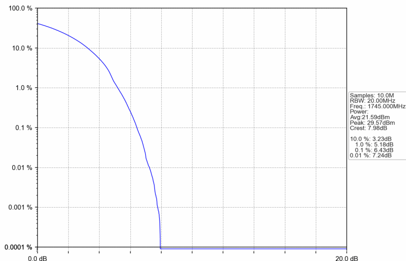
n66_15kHz_SISO_NTNV_25MHz_DFT-s-OFDM 64 QAM_1745MHz_Outer_Full
