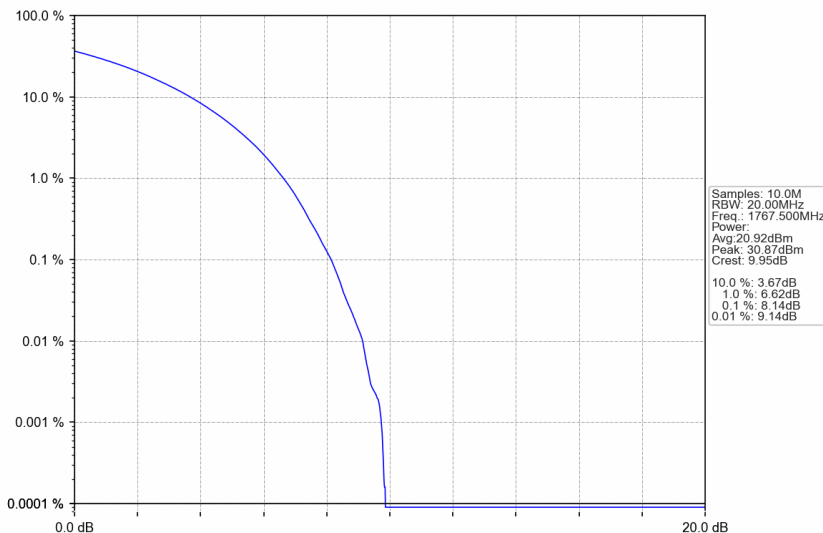
n66_15kHz_SISO_NTNV_25MHz_CP-OFDM QPSK_1767.5MHz_Outer_Full
