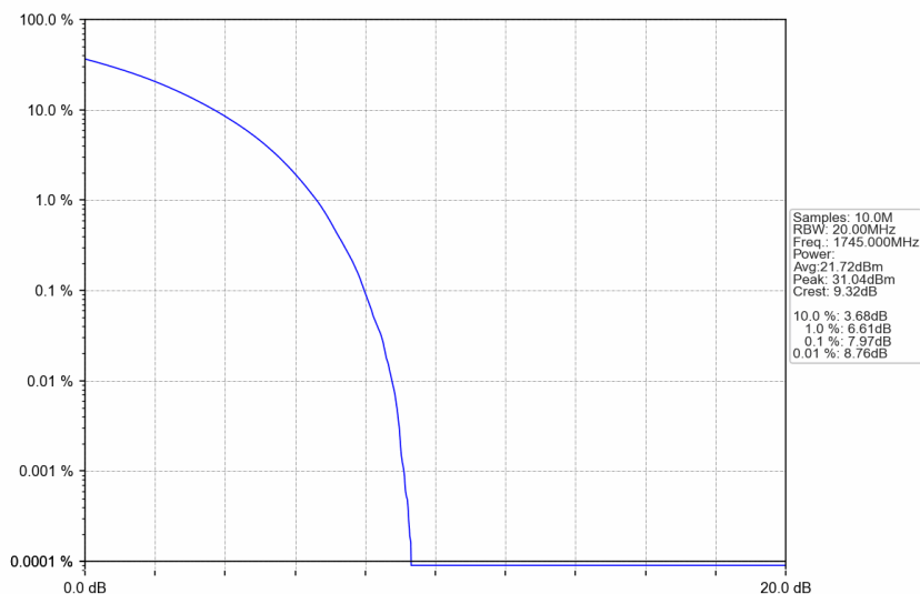
n66_15kHz_SISO_NTNV_20MHz_CP-OFDM 16 QAM_1745MHz_Outer_Full
