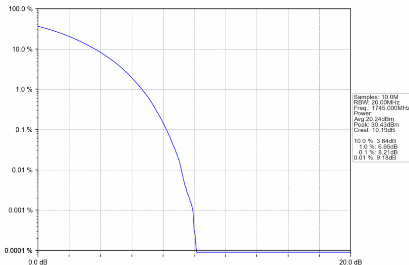
n66_15kHz_SISO_NTNV_30MHz_CP-OFDM 16 QAM_1745MHz_Outer_Full
