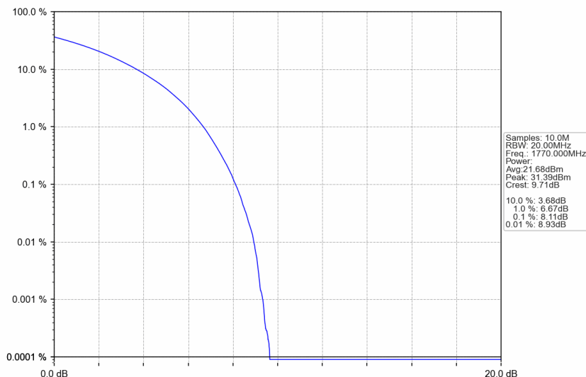
n66_15kHz_SISO_NTNV_20MHz_CP-OFDM 16 QAM_1770MHz_Outer_Full
