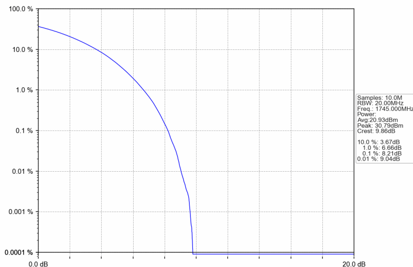
n66_15kHz_SISO_NTNV_25MHz_CP-OFDM 16 QAM_1745MHz_Outer_Full
