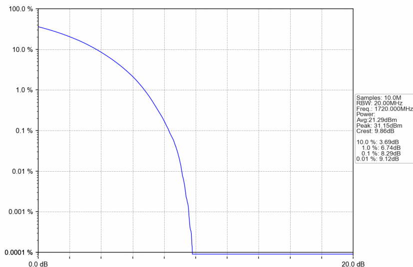
n66_15kHz_SISO_NTNV_20MHz_CP-OFDM 64 QAM_1720MHz_Outer_Full
