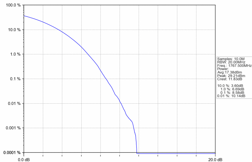
n66_15kHz_SISO_NTNV_25MHz_CP-OFDM 256 QAM_1767.5MHz_Outer_Full
