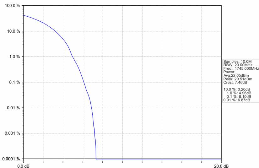
n66_15kHz_SISO_NTNV_25MHz_DFT-s-OFDM 16 QAM_1745MHz_Outer_Full
