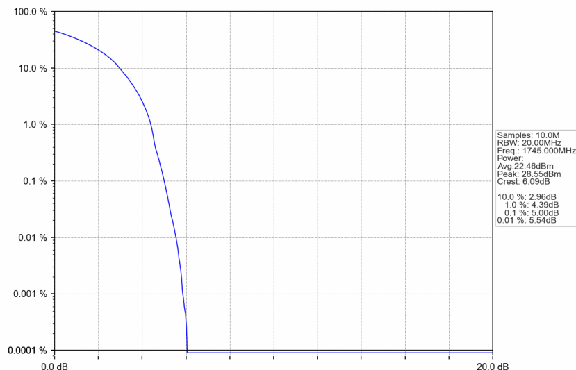
n66_15kHz_SISO_NTNV_35MHz_DFT-s-OFDM QPSK_1745MHz_Outer_Full
