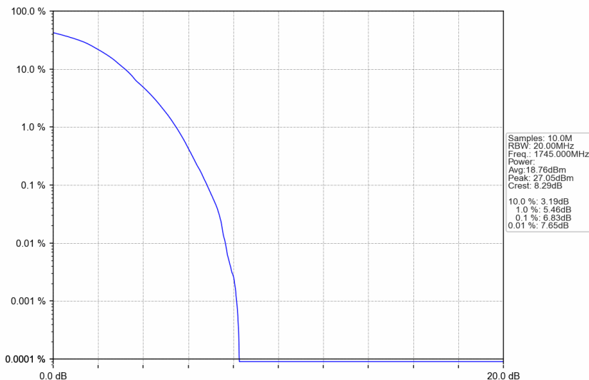
n66_15kHz_SISO_NTNV_30MHz_DFT-s-OFDM 256 QAM_1745MHz_Outer_Full
