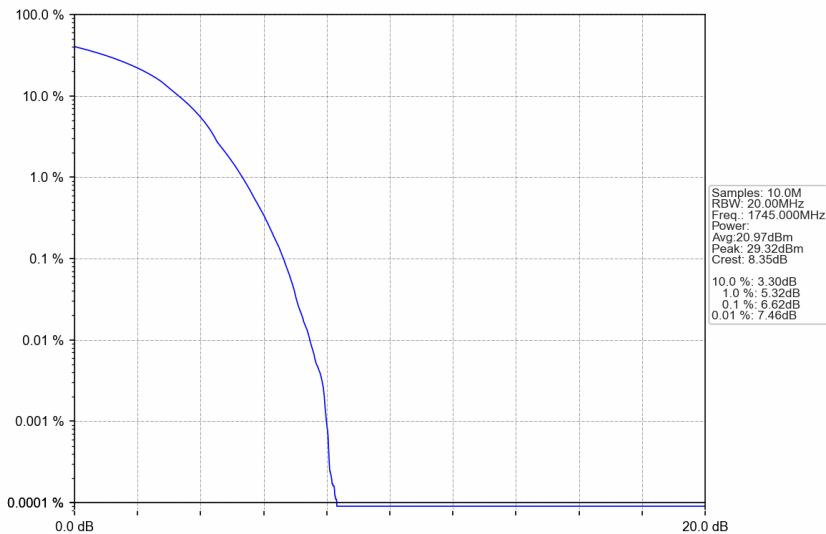
n66_15kHz_SISO_NTNV_35MHz_DFT-s-OFDM 64 QAM_1745MHz_Outer_Full
