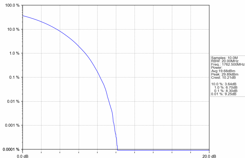
n66_15kHz_SISO_NTNV_35MHz_CP-OFDM 64 QAM_1762.5MHz_Outer_Full
