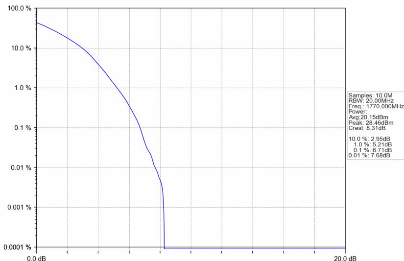
n66_15kHz_SISO_NTNV_20MHz_DFT-s-OFDM 256 QAM_1770MHz_Outer_Full
