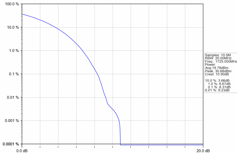
n66_15kHz_SISO_NTNV_30MHz_CP-OFDM 64 QAM_1725MHz_Outer_Full
