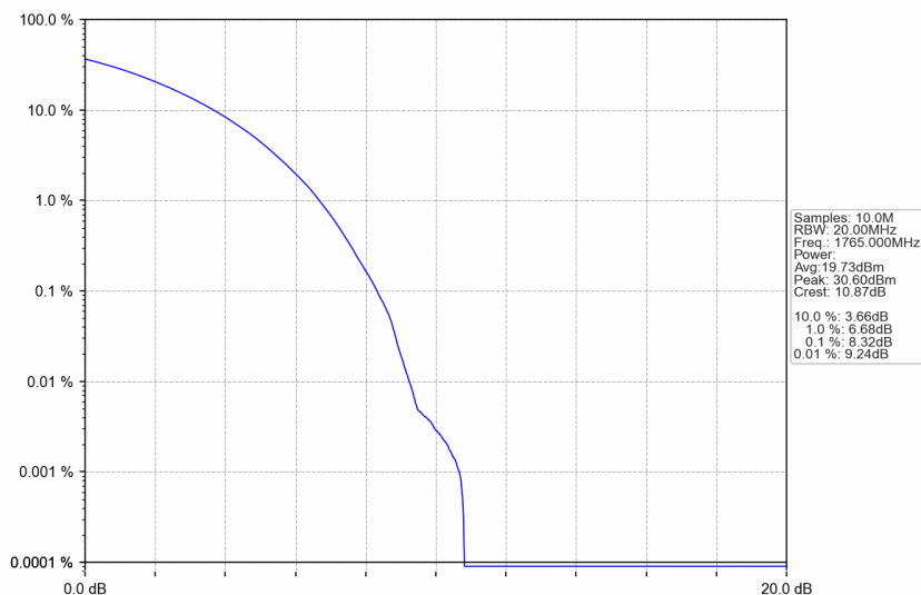
n66_15kHz_SISO_NTNV_30MHz_CP-OFDM 64 QAM_1765MHz_Outer_Full
