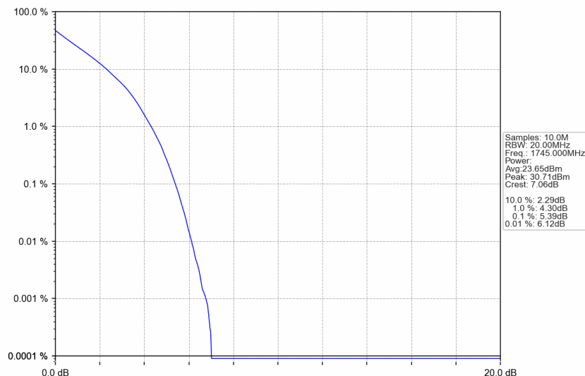
n66_15kHz_SISO_NTNV_20MHz_DFT-s-OFDM QPSK_1745MHz_Outer_Full
