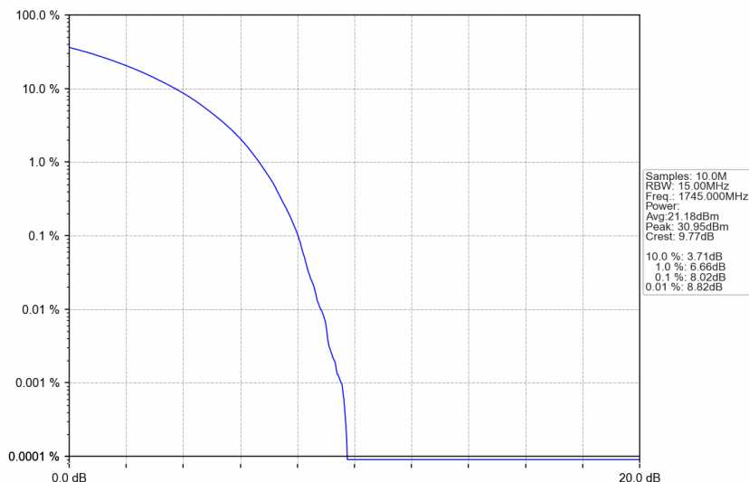
n66_15kHz_SISO_NTNV_15MHz_CP-OFDM 64 QAM_1745MHz_Outer_Full
