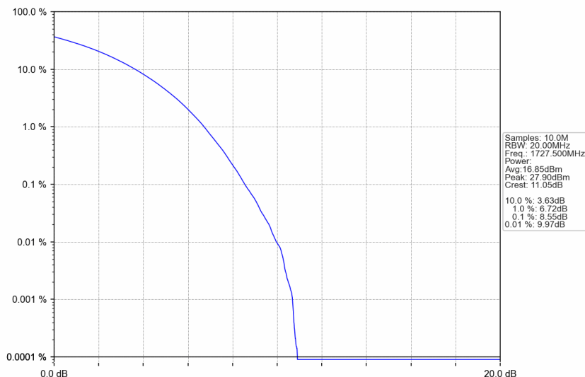
n66_15kHz_SISO_NTNV_35MHz_CP-OFDM 256 QAM_1727.5MHz_Outer_Full
