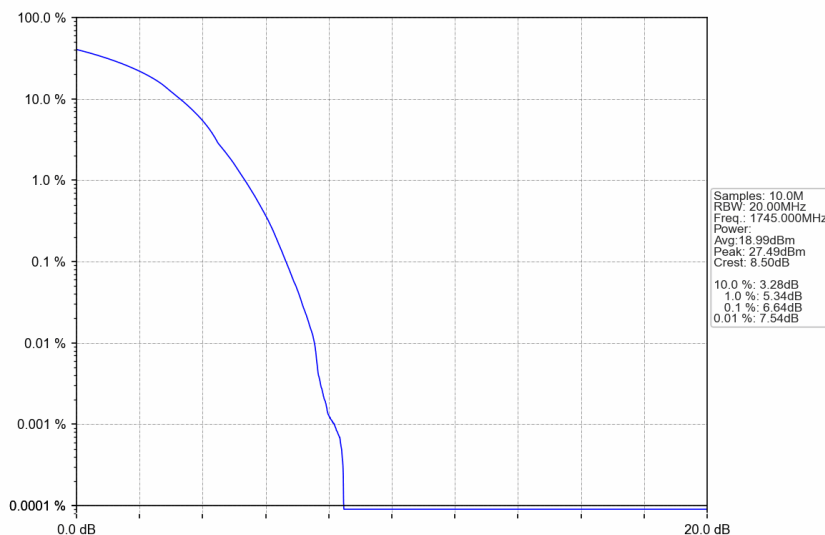
n66_15kHz_SISO_NTNV_35MHz_DFT-s-OFDM 256 QAM_1745MHz_Outer_Full
