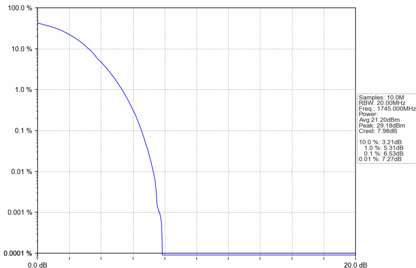
n66_15kHz_SISO_NTNV_30MHz_DFT-s-OFDM 16 QAM_1745MHz_Outer_Full
