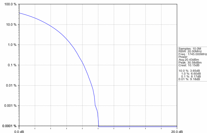
n66_15kHz_SISO_NTNV_25MHz_CP-OFDM 64 QAM_1745MHz_Outer_Full
