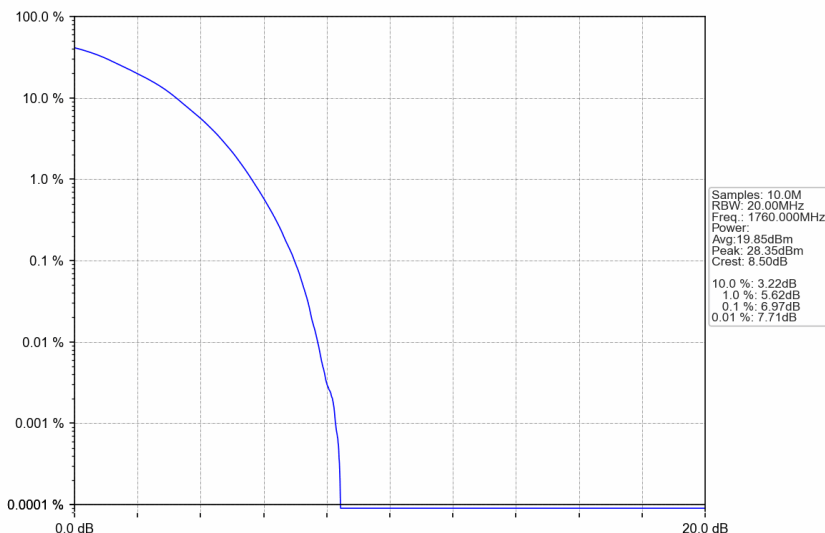
n66_15kHz_SISO_NTNV_40MHz_DFT-s-OFDM 16 QAM_1760MHz_Outer_Full
