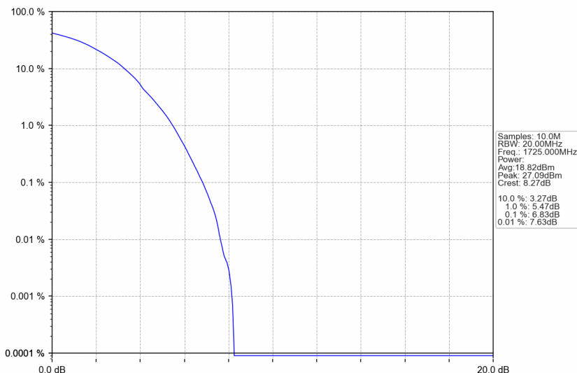
n66_15kHz_SISO_NTNV_30MHz_DFT-s-OFDM 256 QAM_1725MHz_Outer_Full
