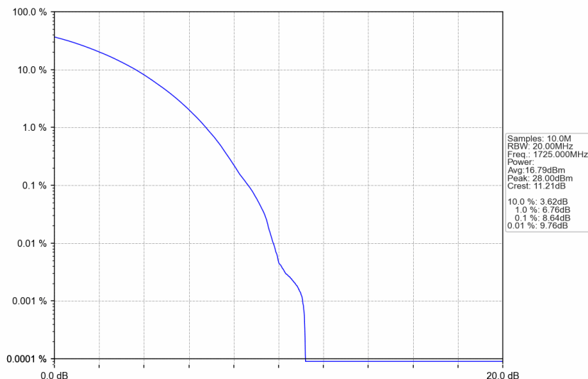
n66_15kHz_SISO_NTNV_30MHz_CP-OFDM 256 QAM_1725MHz_Outer_Full
