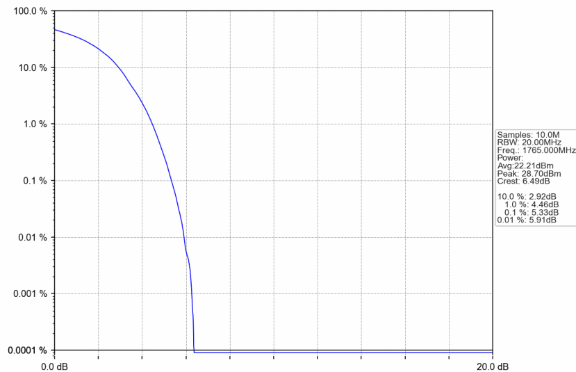
n66_15kHz_SISO_NTNV_30MHz_DFT-s-OFDM QPSK_1765MHz_Outer_Full
