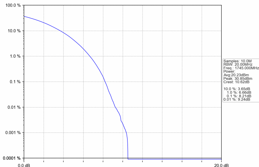
n66_15kHz_SISO_NTNV_30MHz_CP-OFDM QPSK_1745MHz_Outer_Full
