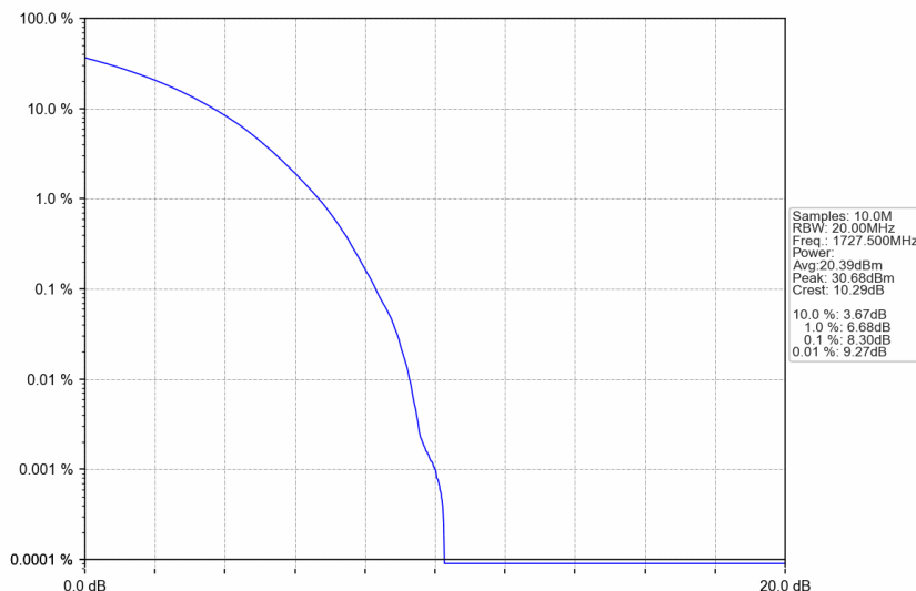
n66_15kHz_SISO_NTNV_35MHz_CP-OFDM 16 QAM_1727.5MHz_Outer_Full
