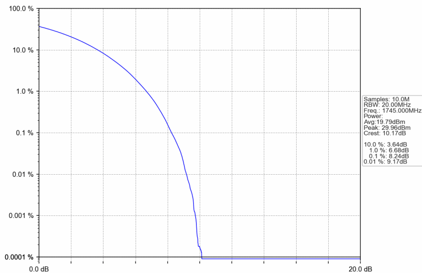
n66_15kHz_SISO_NTNV_35MHz_CP-OFDM 64 QAM_1745MHz_Outer_Full
