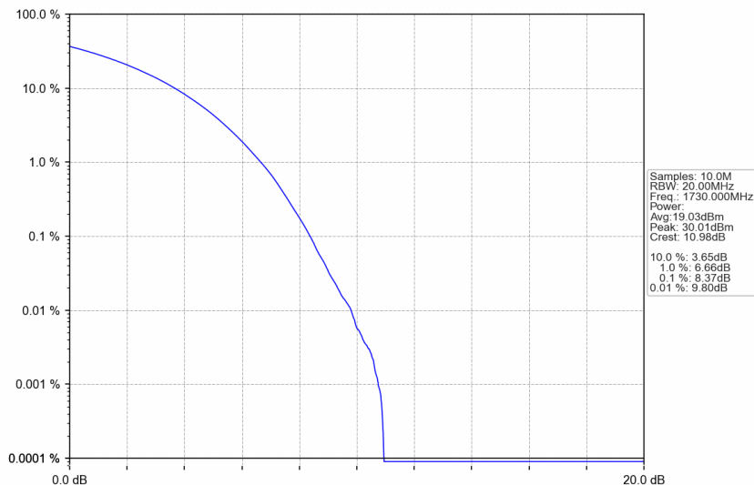
n66_15kHz_SISO_NTNV_40MHz_CP-OFDM QPSK_1730MHz_Outer_Full
