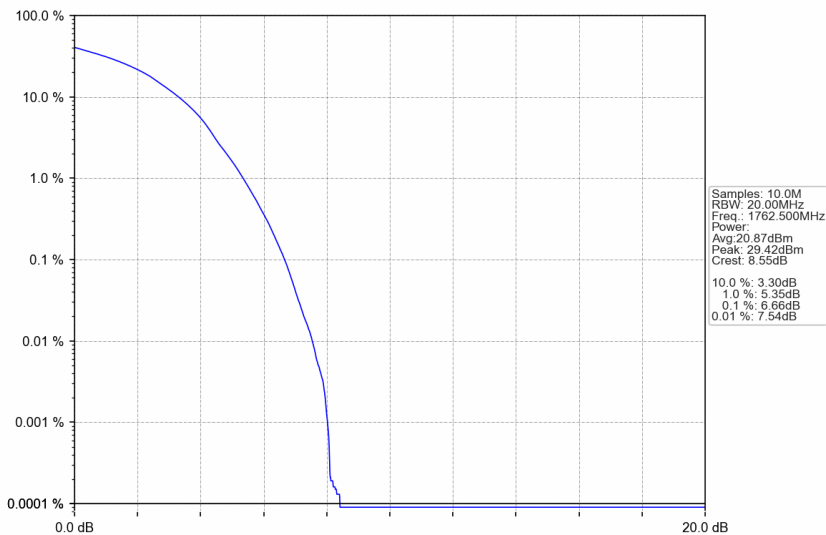
n66_15kHz_SISO_NTNV_35MHz_DFT-s-OFDM 64 QAM_1762.5MHz_Outer_Full
