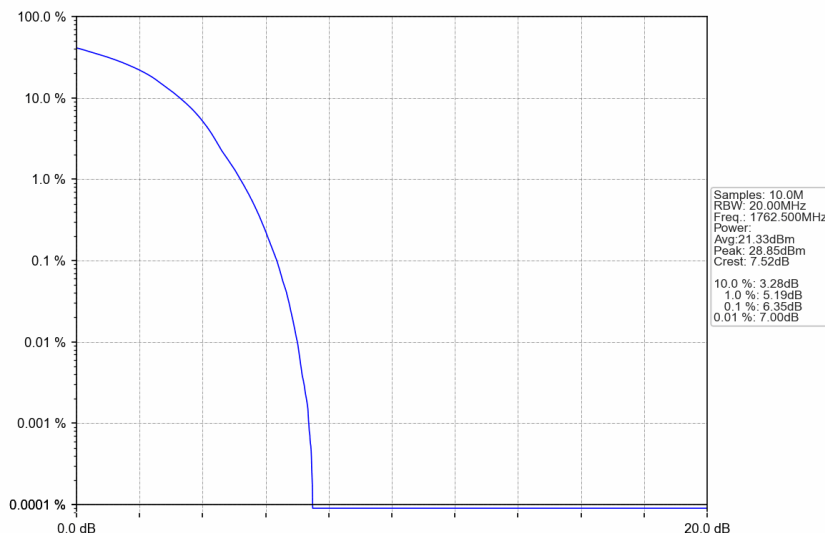
n66_15kHz_SISO_NTNV_35MHz_DFT-s-OFDM 16 QAM_1762.5MHz_Outer_Full
