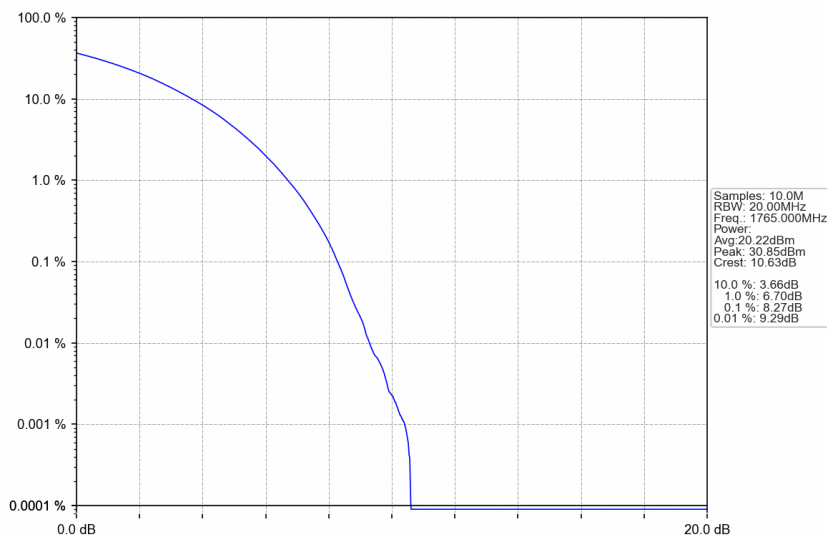
n66_15kHz_SISO_NTNV_30MHz_CP-OFDM QPSK_1765MHz_Outer_Full
