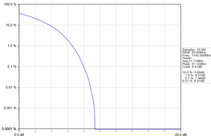
n66_15kHz_SISO_NTNV_20MHz_CP-OFDM QPSK_1745MHz_Outer_Full
