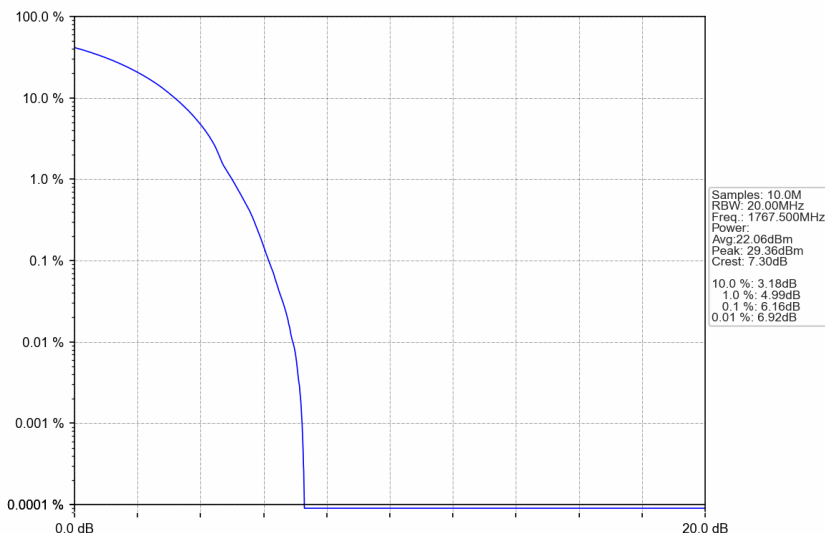
n66_15kHz_SISO_NTNV_25MHz_DFT-s-OFDM 16 QAM_1767.5MHz_Outer_Full
