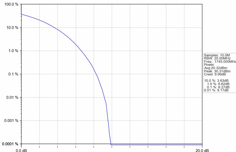
n66_15kHz_SISO_NTNV_35MHz_CP-OFDM QPSK_1745MHz_Outer_Full
