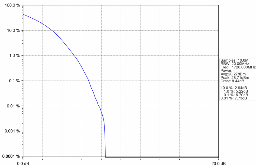
n66_15kHz_SISO_NTNV_20MHz_DFT-s-OFDM 256 QAM_1720MHz_Outer_Full
