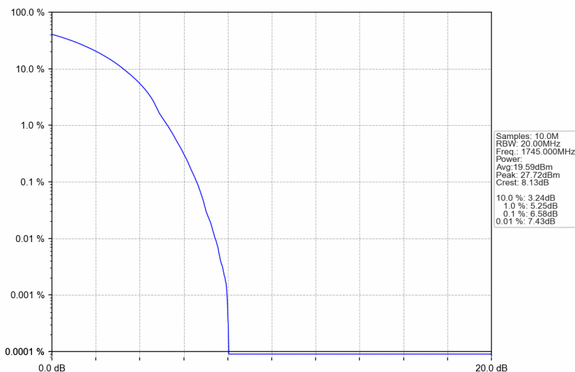
n66_15kHz_SISO_NTNV_25MHz_DFT-s-OFDM 256 QAM_1745MHz_Outer_Full
