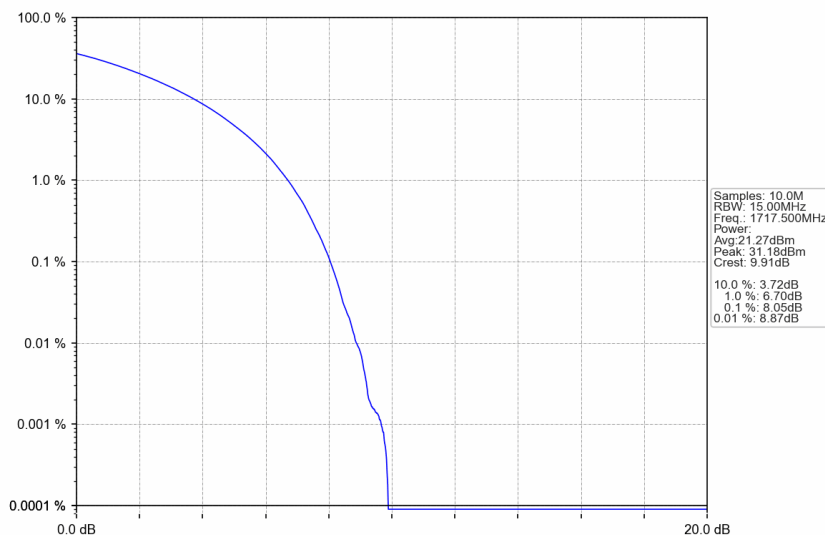
n66_15kHz_SISO_NTNV_15MHz_CP-OFDM 64 QAM_1717.5MHz_Outer_Full
