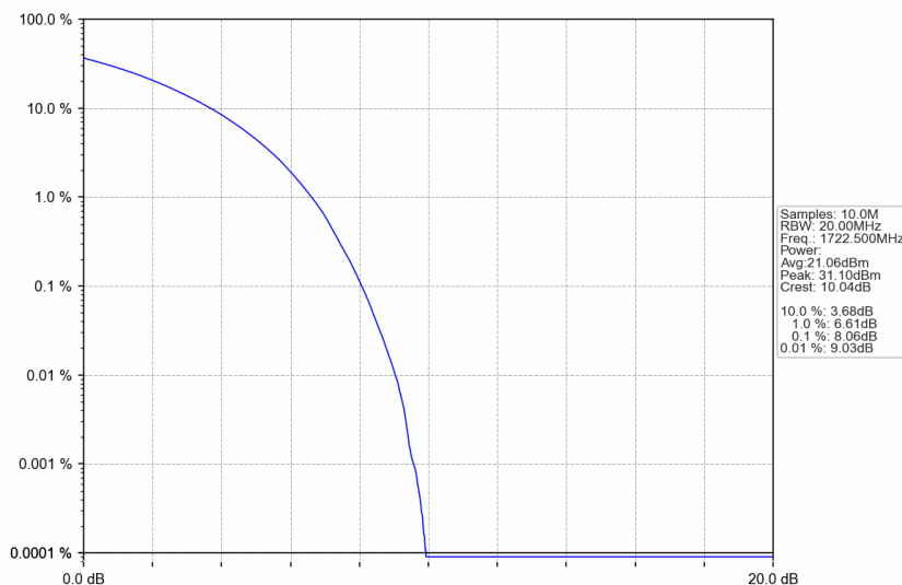
n66_15kHz_SISO_NTNV_25MHz_CP-OFDM QPSK_1722.5MHz_Outer_Full
