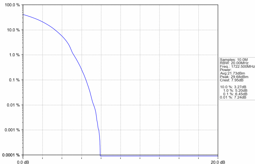
n66_15kHz_SISO_NTNV_25MHz_DFT-s-OFDM 64 QAM_1722.5MHz_Outer_Full
