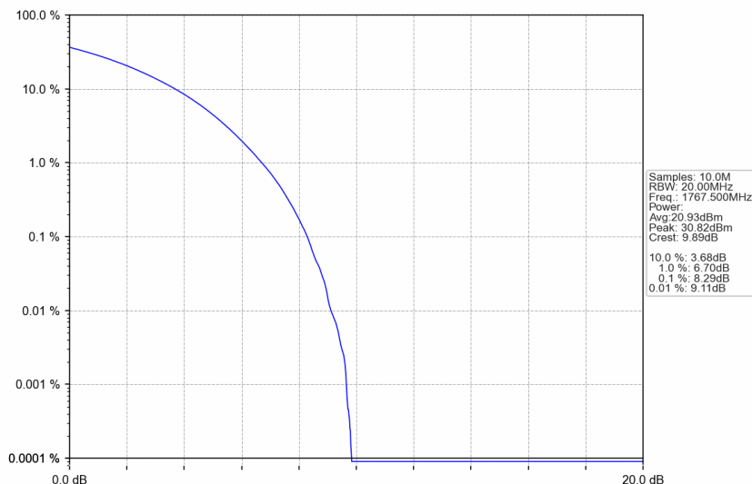
n66_15kHz_SISO_NTNV_25MHz_CP-OFDM 16 QAM_1767.5MHz_Outer_Full
