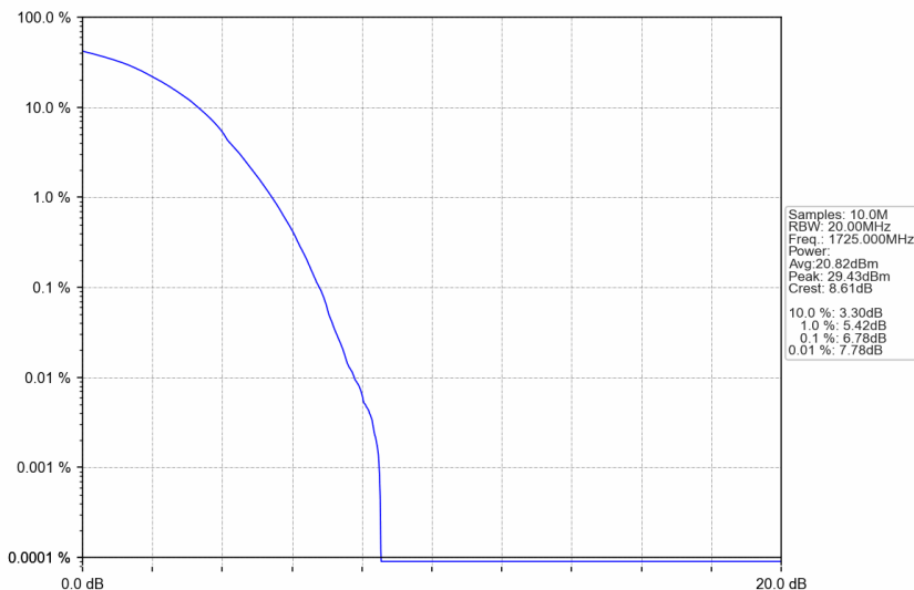
n66_15kHz_SISO_NTNV_30MHz_DFT-s-OFDM 64 QAM_1725MHz_Outer_Full
