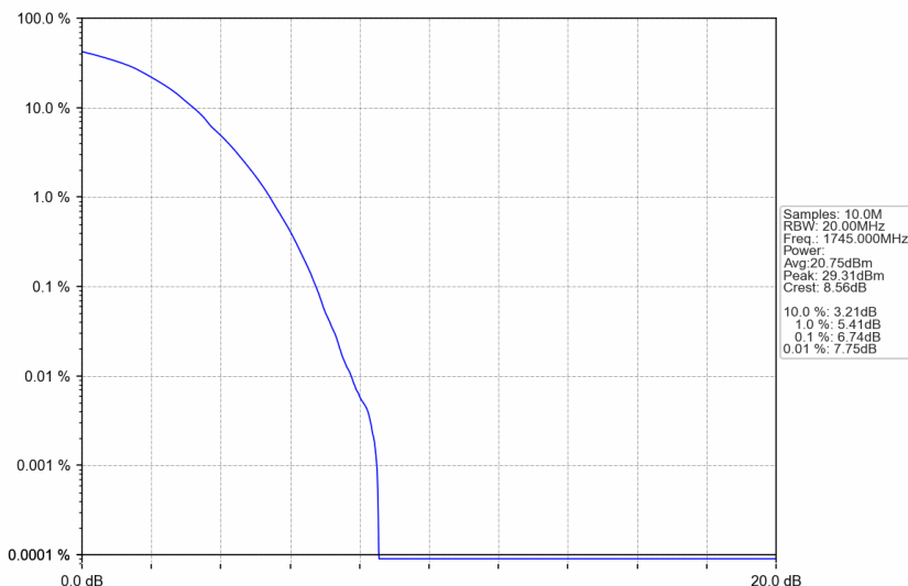
n66_15kHz_SISO_NTNV_30MHz_DFT-s-OFDM 64 QAM_1745MHz_Outer_Full
