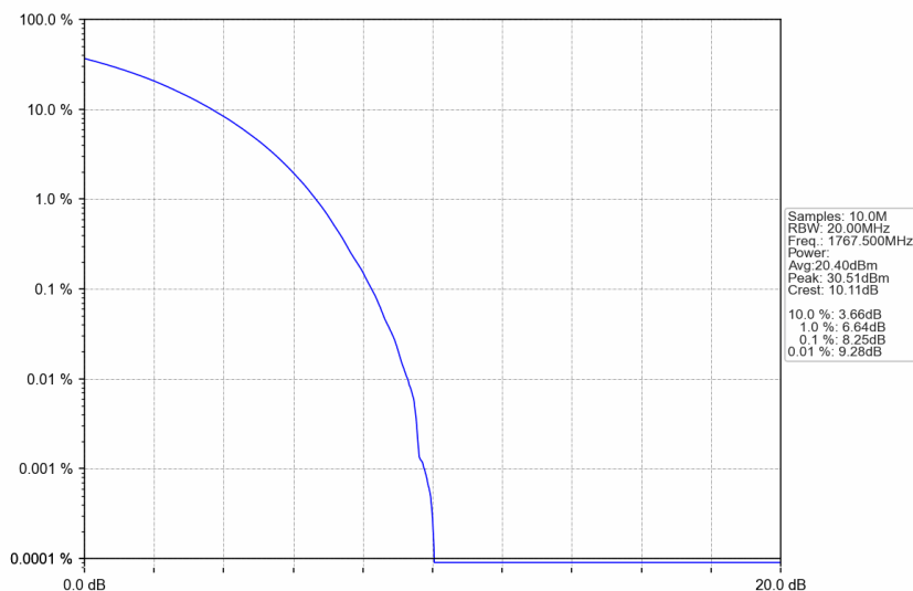
n66_15kHz_SISO_NTNV_25MHz_CP-OFDM 64 QAM_1767.5MHz_Outer_Full
