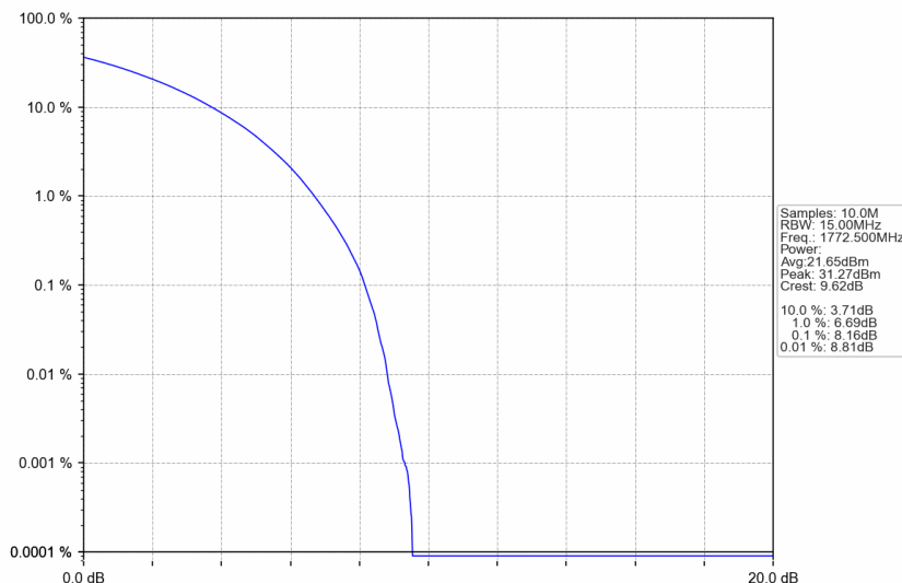
n66_15kHz_SISO_NTNV_15MHz_CP-OFDM 16 QAM_1772.5MHz_Outer_Full
