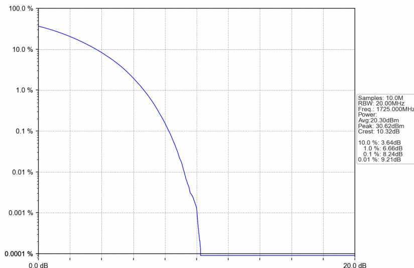
n66_15kHz_SISO_NTNV_30MHz_CP-OFDM 16 QAM_1725MHz_Outer_Full
