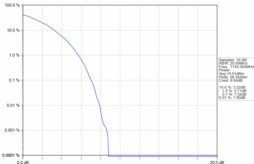
n66_15kHz_SISO_NTNV_40MHz_DFT-s-OFDM 64 QAM_1745MHz_Outer_Full
