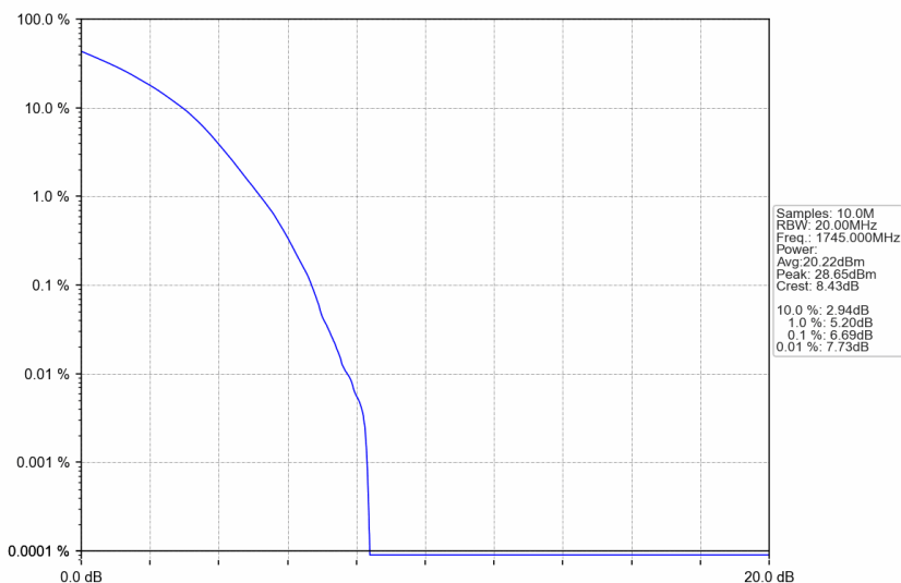
n66_15kHz_SISO_NTNV_20MHz_DFT-s-OFDM 256 QAM_1745MHz_Outer_Full
