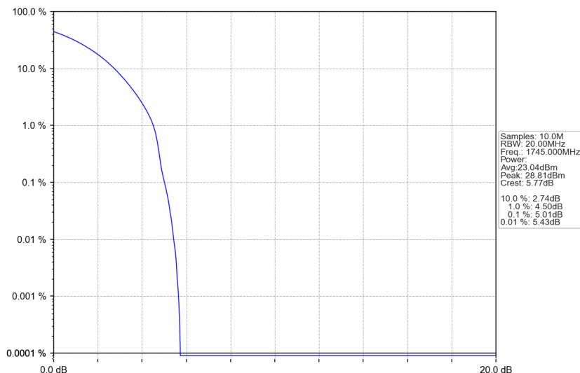
n66_15kHz_SISO_NTNV_25MHz_DFT-s-OFDM QPSK_1745MHz_Outer_Full
