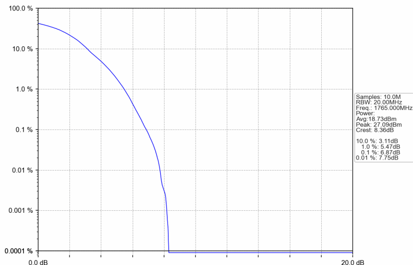
n66_15kHz_SISO_NTNV_30MHz_DFT-s-OFDM 256 QAM_1765MHz_Outer_Full
