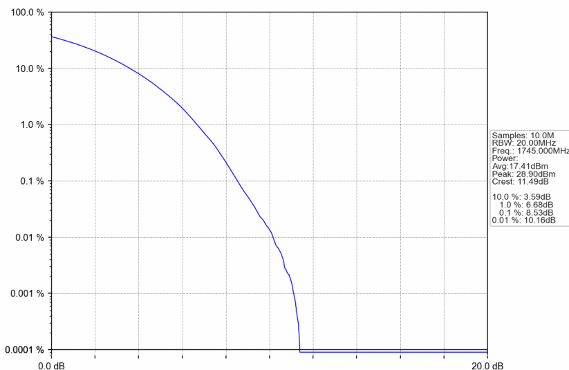
n66_15kHz_SISO_NTNV_25MHz_CP-OFDM 256 QAM_1745MHz_Outer_Full
