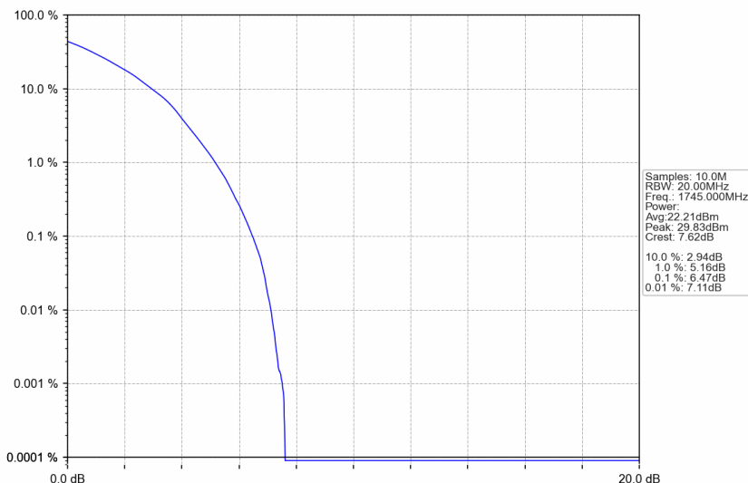
n66_15kHz_SISO_NTNV_20MHz_DFT-s-OFDM 64 QAM_1745MHz_Outer_Full
