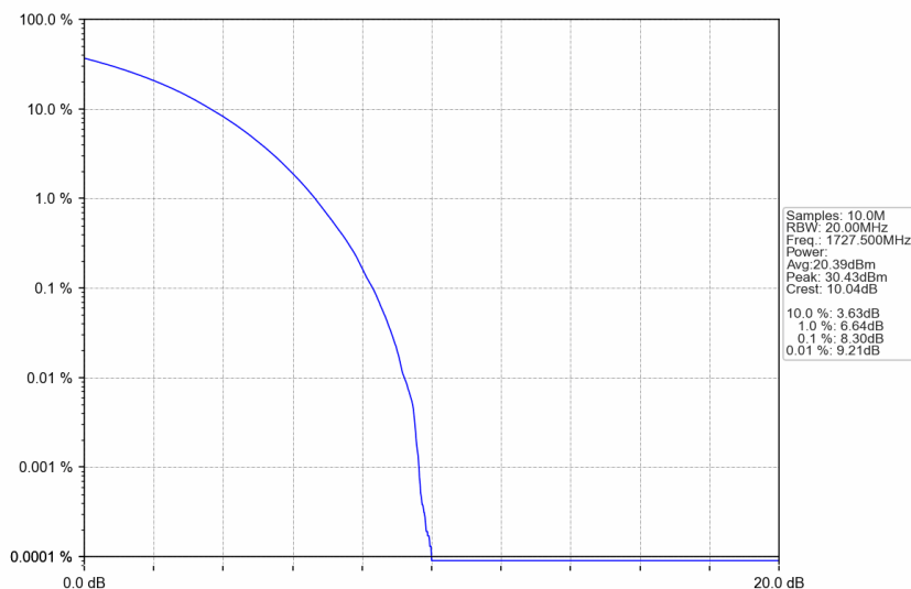
n66_15kHz_SISO_NTNV_35MHz_CP-OFDM QPSK_1727.5MHz_Outer_Full
