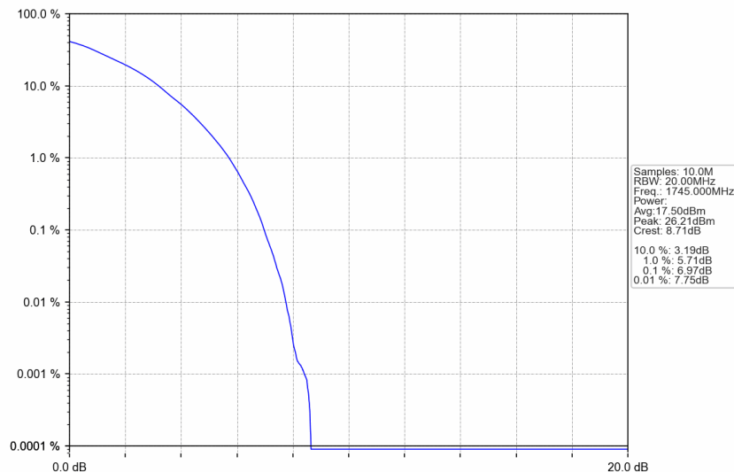
n66_15kHz_SISO_NTNV_40MHz_DFT-s-OFDM 256 QAM_1745MHz_Outer_Full
