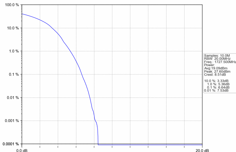
n66_15kHz_SISO_NTNV_35MHz_DFT-s-OFDM 256 QAM_1727.5MHz_Outer_Full
