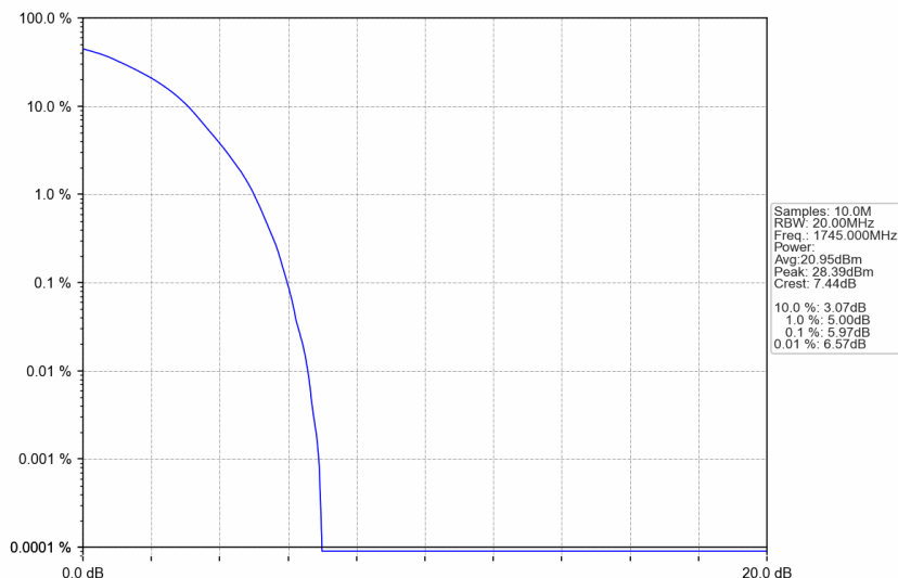
n66_15kHz_SISO_NTNV_40MHz_DFT-s-OFDM_QPSK_1745MHz_Outer_Full
