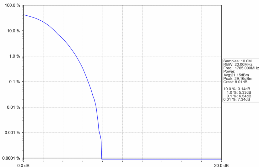
n66_15kHz_SISO_NTNV_30MHz_DFT-s-OFDM 16 QAM_1765MHz_Outer_Full
