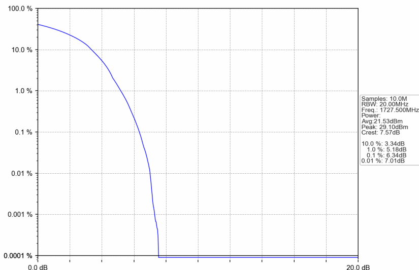
n66_15kHz_SISO_NTNV_35MHz_DFT-s-OFDM 16 QAM_1727.5MHz_Outer_Full
