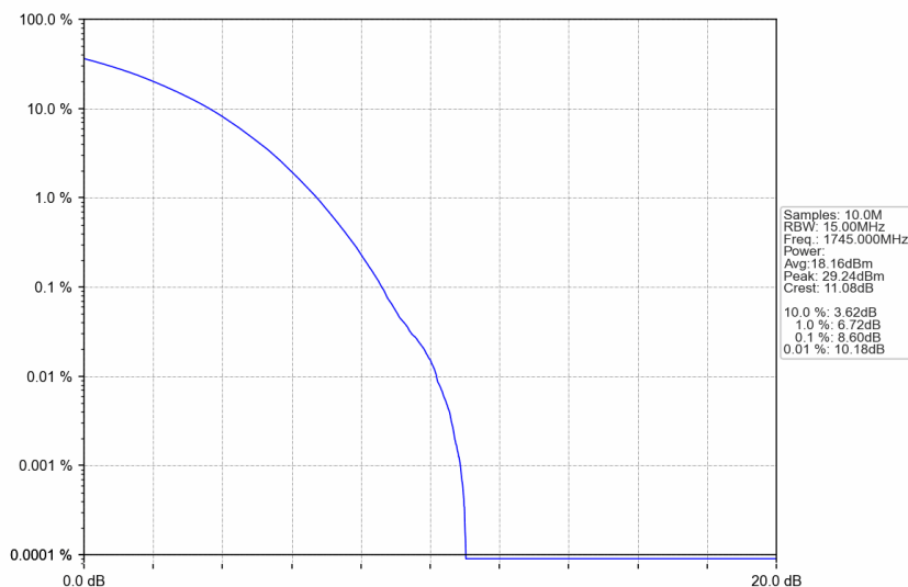
n66_15kHz_SISO_NTNV_15MHz_CP-OFDM 256 QAM_1745MHz_Outer_Full
