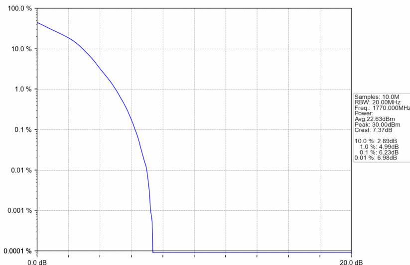
n66_15kHz_SISO_NTNV_20MHz_DFT-s-OFDM 16 QAM_1770MHz_Outer_Full
