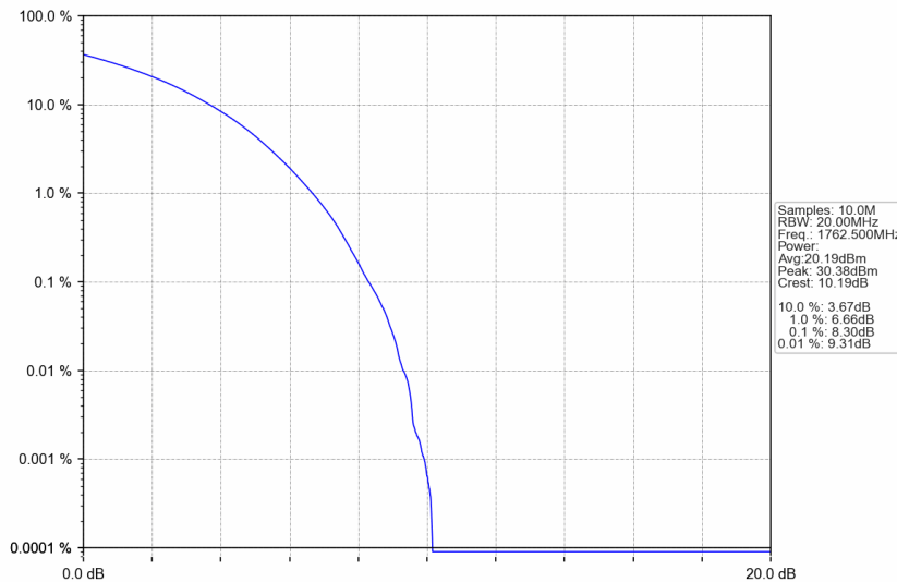
n66_15kHz_SISO_NTNV_35MHz_CP-OFDM 16 QAM_1762.5MHz_Outer_Full
