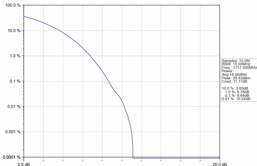
n66_15kHz_SISO_NTNV_15MHz_CP-OFDM 256 QAM_1717.5MHz_Outer_Full
