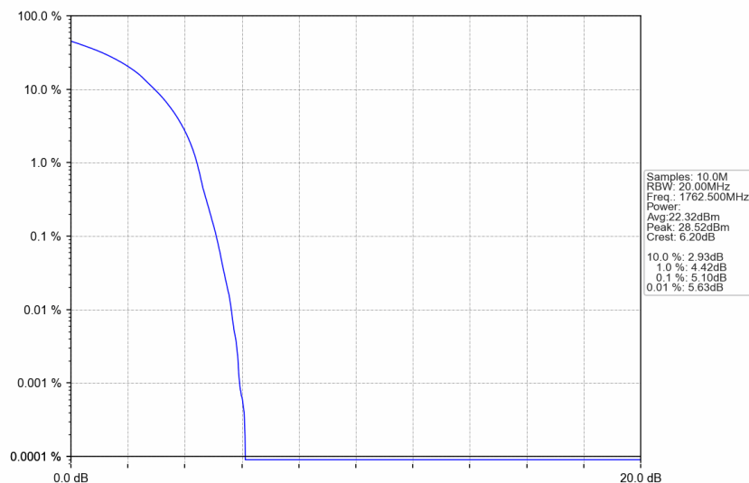
n66_15kHz_SISO_NTNV_35MHz_DFT-s-OFDM QPSK_1762.5MHz_Outer_Full
