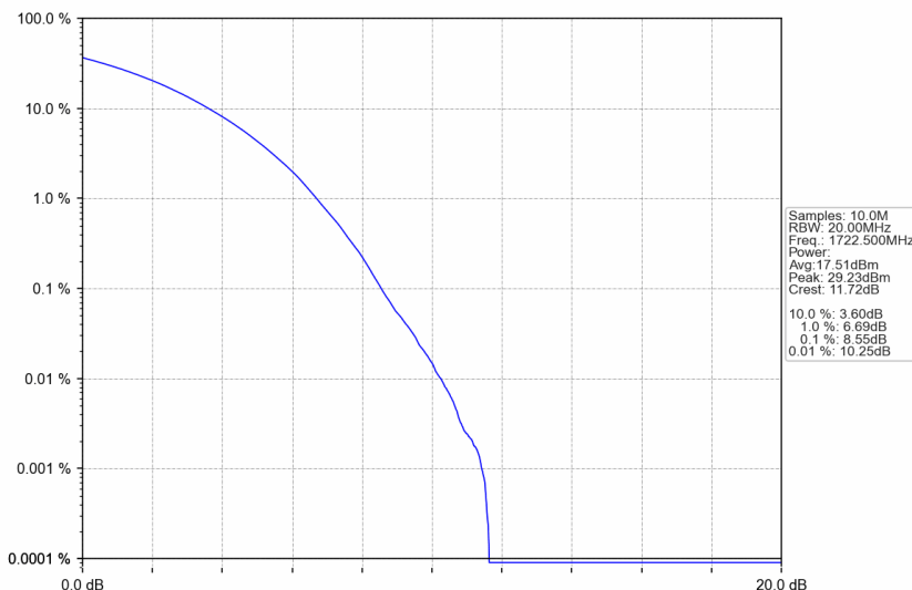
n66_15kHz_SISO_NTNV_25MHz_CP-OFDM 256 QAM_1722.5MHz_Outer_Full
