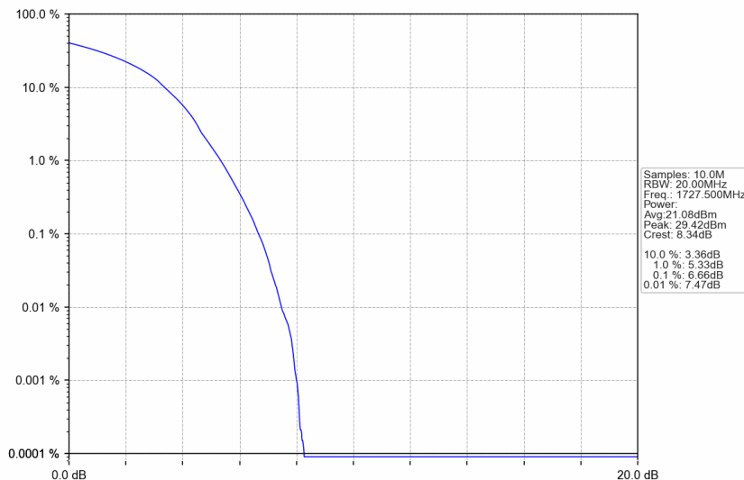
n66_15kHz_SISO_NTNV_35MHz_DFT-s-OFDM 64 QAM_1727.5MHz_Outer_Full
