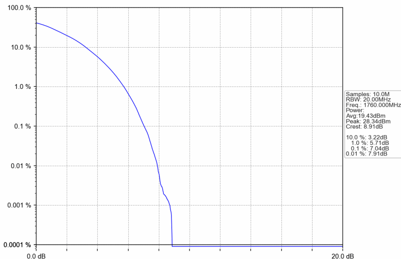
n66_15kHz_SISO_NTNV_40MHz_DFT-s-OFDM 64 QAM_1760MHz_Outer_Full
