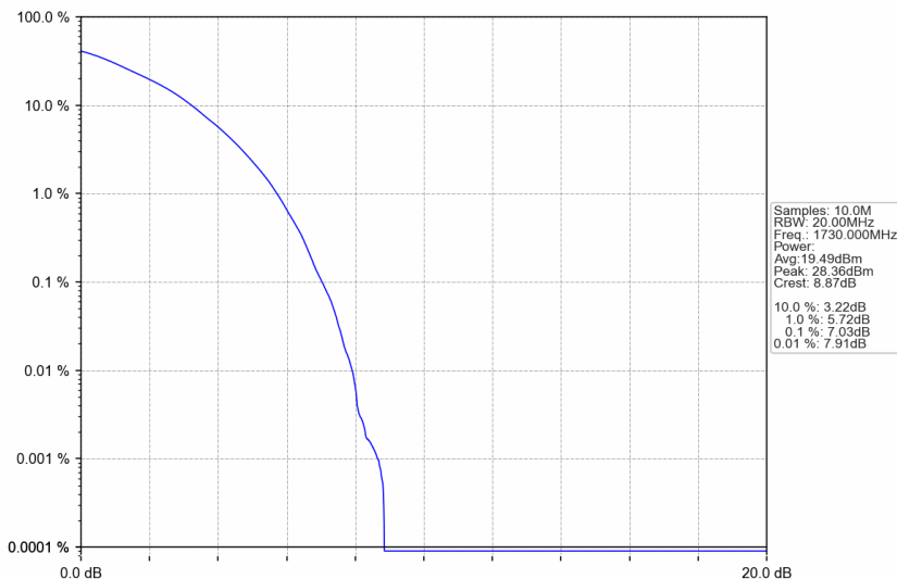
n66_15kHz_SISO_NTNV_40MHz_DFT-s-OFDM 64 QAM_1730MHz_Outer_Full
