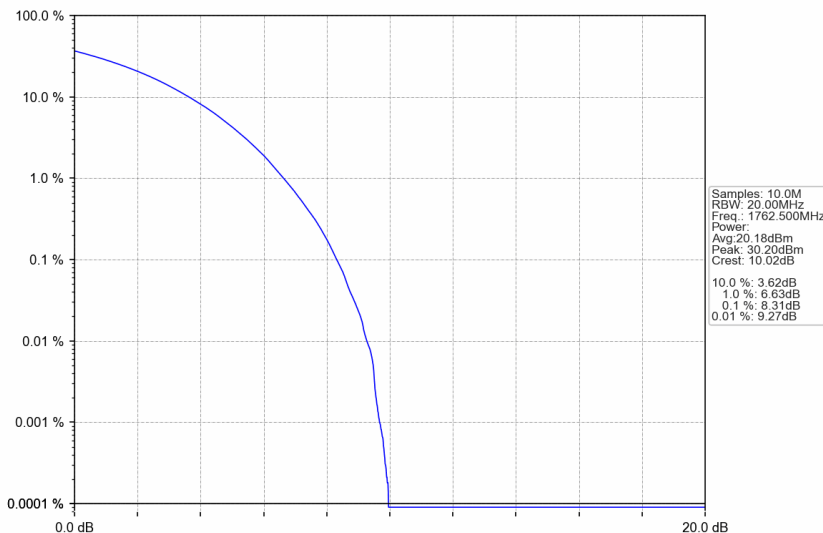
n66_15kHz_SISO_NTNV_35MHz_CP-OFDM QPSK_1762.5MHz_Outer_Full
