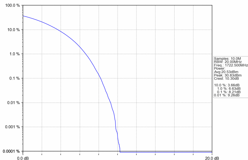
n66_15kHz_SISO_NTNV_25MHz_CP-OFDM 64 QAM_1722.5MHz_Outer_Full
