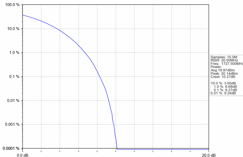
n66_15kHz_SISO_NTNV_35MHz_CP-OFDM 64 QAM_1727.5MHz_Outer_Full
