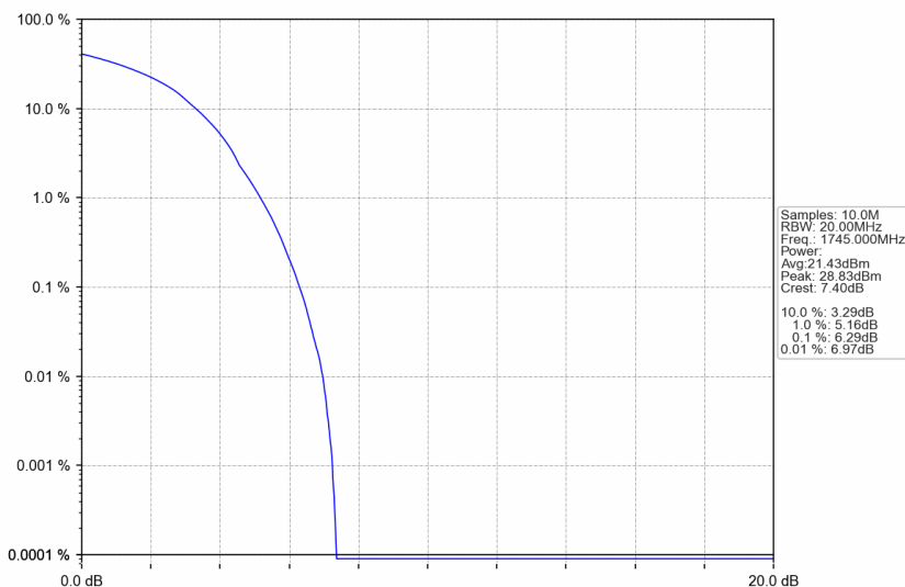
n66_15kHz_SISO_NTNV_35MHz_DFT-s-OFDM 16 QAM_1745MHz_Outer_Full
