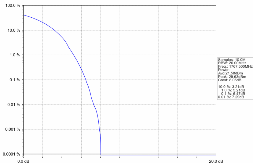
n66_15kHz_SISO_NTNV_25MHz_DFT-s-OFDM 64 QAM_1767.5MHz_Outer_Full
