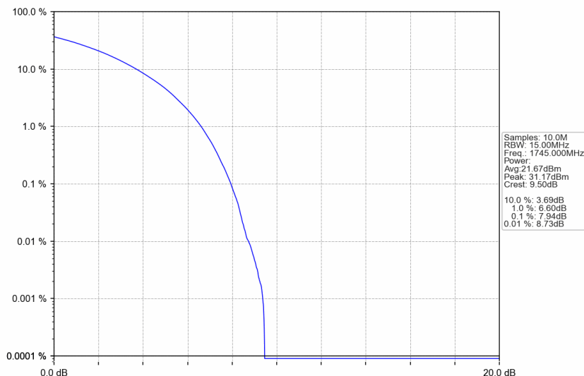
n66_15kHz_SISO_NTNV_15MHz_CP-OFDM QPSK_1745MHz_Outer_Full
