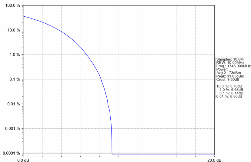
n66_15kHz_SISO_NTNV_10MHz_CP-OFDM 16 QAM_1745MHz_Outer_Full
