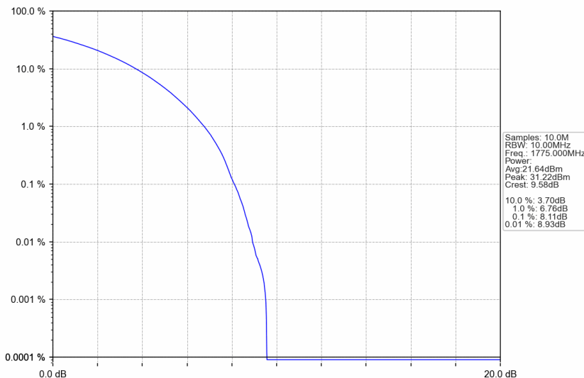
n66_15kHz_SISO_NTNV_10MHz_CP-OFDM QPSK_1775MHz_Outer_Full
