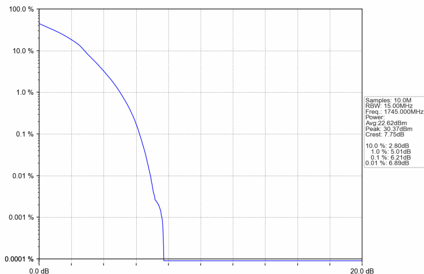
n66_15kHz_SISO_NTNV_15MHz_DFT-s-OFDM 16 QAM_1745MHz_Outer_Full
