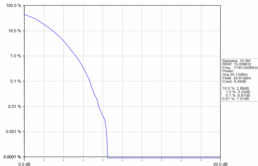
n66_15kHz_SISO_NTNV_15MHz_DFT-s-OFDM 256 QAM_1745MHz_Outer_Full
