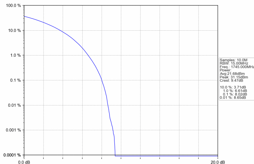
n66_15kHz_SISO_NTNV_15MHz_CP-OFDM 16 QAM_1745MHz_Outer_Full
