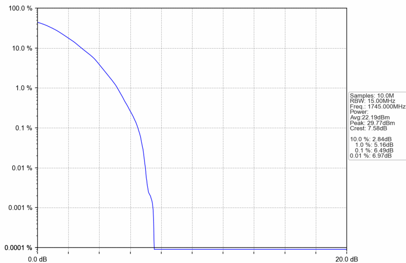
n66_15kHz_SISO_NTNV_15MHz_DFT-s-OFDM 64 QAM_1745MHz_Outer_Full
