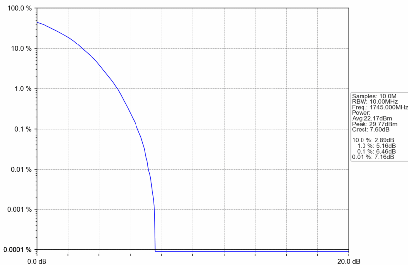
n66_15kHz_SISO_NTNV_10MHz_DFT-s-OFDM 64 QAM_1745MHz_Outer_Full
