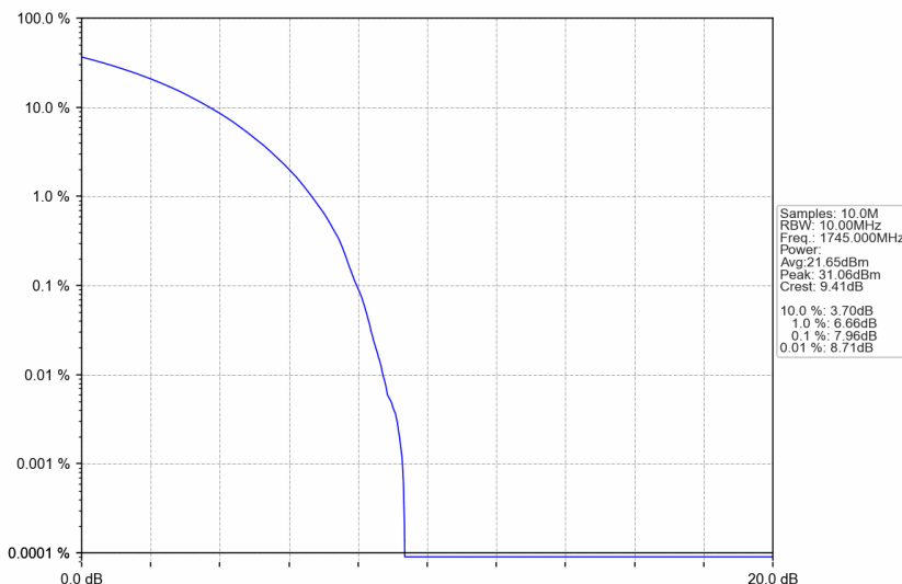
n66_15kHz_SISO_NTNV_10MHz_CP-OFDM QPSK_1745MHz_Outer_Full
