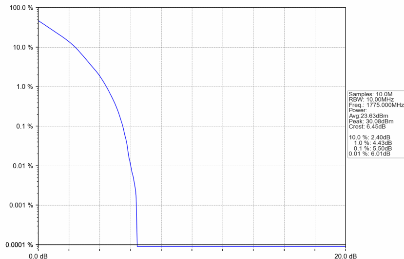
n66_15kHz_SISO_NTNV_10MHz_DFT-s-OFDM QPSK_1775MHz_Outer_Full
