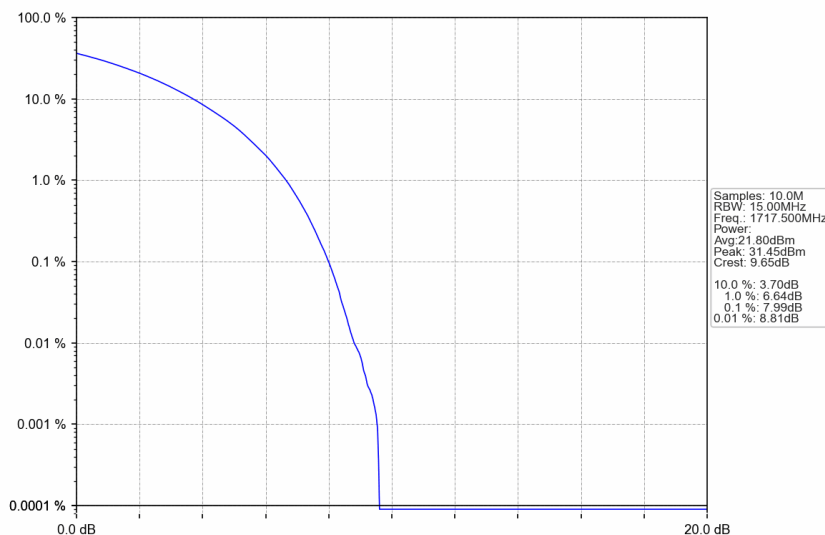
n66_15kHz_SISO_NTNV_15MHz_CP-OFDM QPSK_1717.5MHz_Outer_Full
