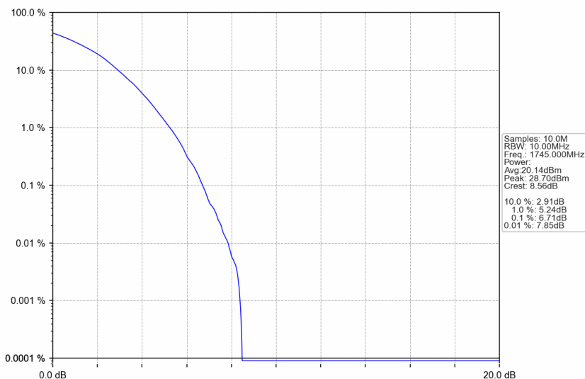
n66_15kHz_SISO_NTNV_10MHz_DFT-s-OFDM 256 QAM_1745MHz_Outer_Full
