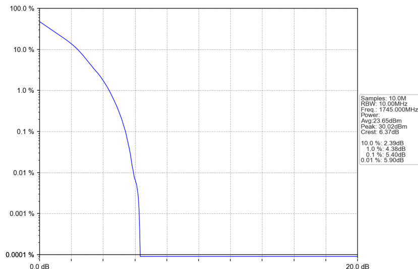
n66_15kHz_SISO_NTNV_10MHz_DFT-s-OFDM QPSK_1745MHz_Outer_Full
