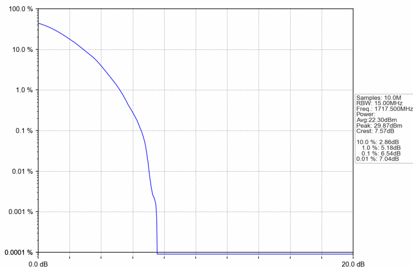
n66_15kHz_SISO_NTNV_15MHz_DFT-s-OFDM 64 QAM_1717.5MHz_Outer_Full
