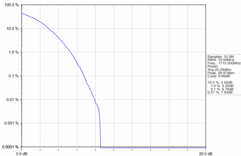
n66_15kHz_SISO_NTNV_10MHz_DFT-s-OFDM 256 QAM_1715MHz_Outer_Full
