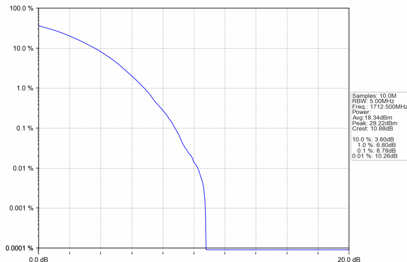
n66_15kHz_SISO_NTNV_5MHz_CP-OFDM 256 QAM_1712.5MHz_Outer_Full
