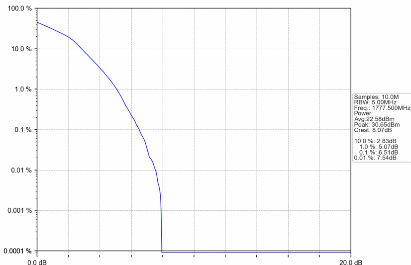
n66_15kHz_SISO_NTNV_5MHz_DFT-s-OFDM 16 QAM_1777.5MHz_Outer_Full
