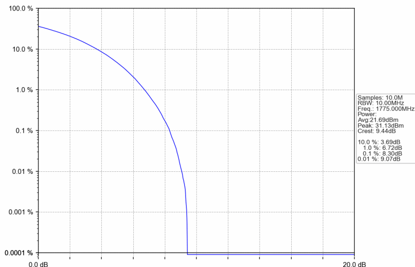
n66_15kHz_SISO_NTNV_10MHz_CP-OFDM 16 QAM_1775MHz_Outer_Full
