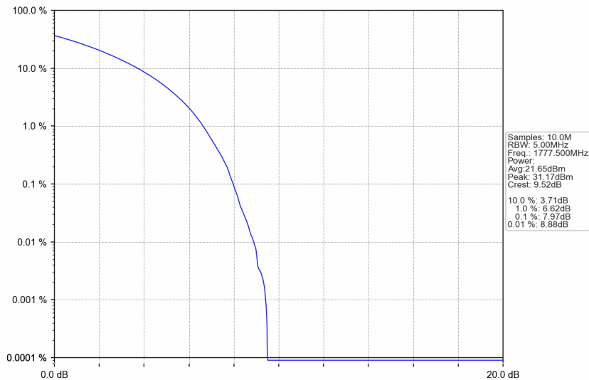
n66_15kHz_SISO_NTNV_5MHz_CP-OFDM 16 QAM_1777.5MHz_Outer_Full
