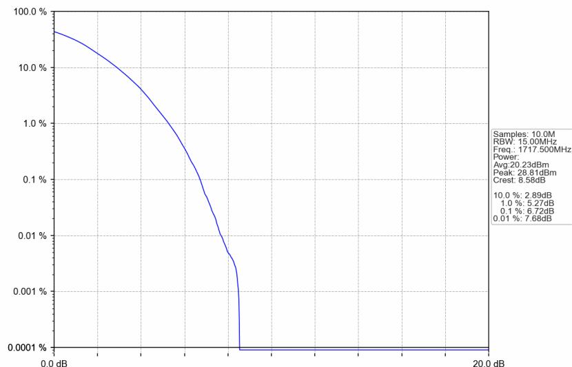
n66_15kHz_SISO_NTNV_15MHz_DFT-s-OFDM 256 QAM_1717.5MHz_Outer_Full
