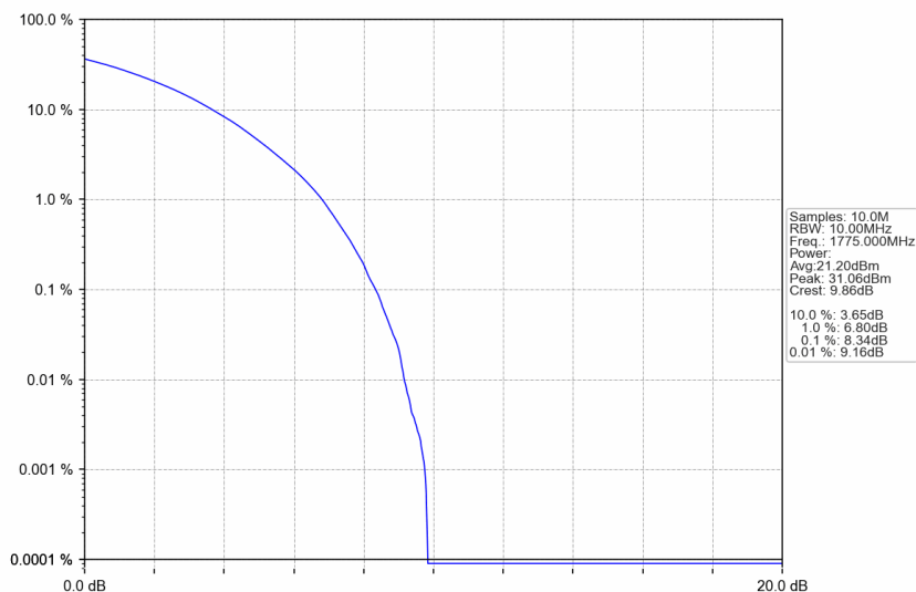
n66_15kHz_SISO_NTNV_10MHz_CP-OFDM 64 QAM_1775MHz_Outer_Full
