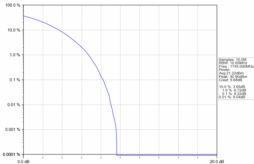
n66_15kHz_SISO_NTNV_10MHz_CP-OFDM 64 QAM_1745MHz_Outer_Full
