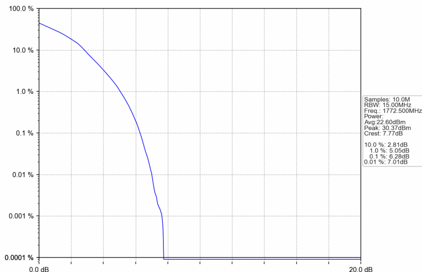
n66_15kHz_SISO_NTNV_15MHz_DFT-s-OFDM 16 QAM_1772.5MHz_Outer_Full
