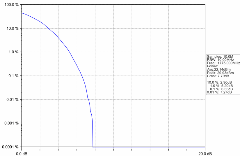
n66_15kHz_SISO_NTNV_10MHz_DFT-s-OFDM 64 QAM_1775MHz_Outer_Full
