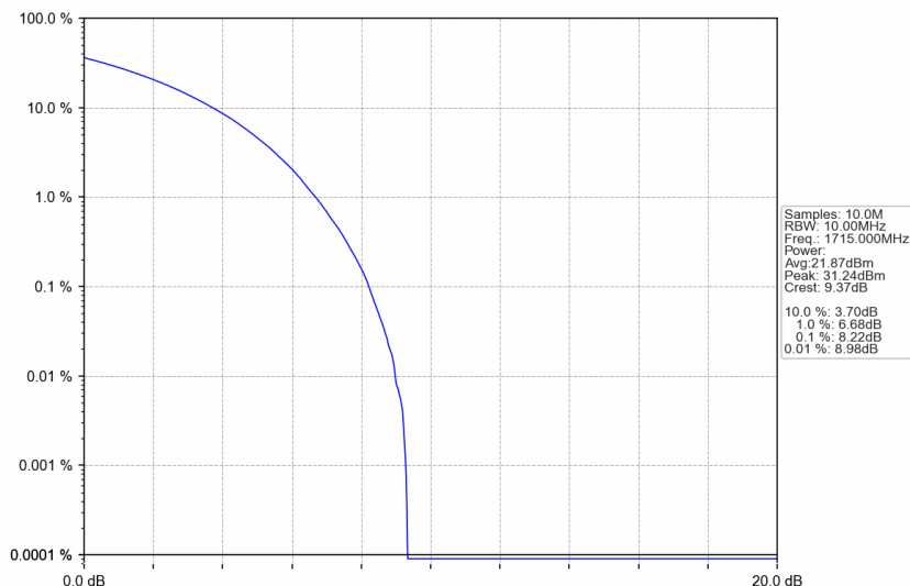
n66_15kHz_SISO_NTNV_10MHz_CP-OFDM 16 QAM_1715MHz_Outer_Full
