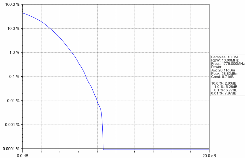
n66_15kHz_SISO_NTNV_10MHz_DFT-s-OFDM 256 QAM_1775MHz_Outer_Full
