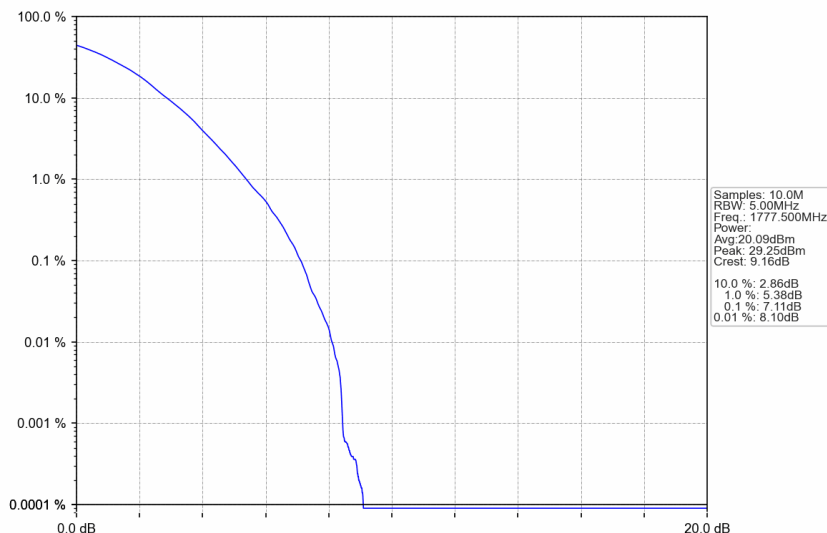
n66_15kHz_SISO_NTNV_5MHz_DFT-s-OFDM 256 QAM_1777.5MHz_Outer_Full
