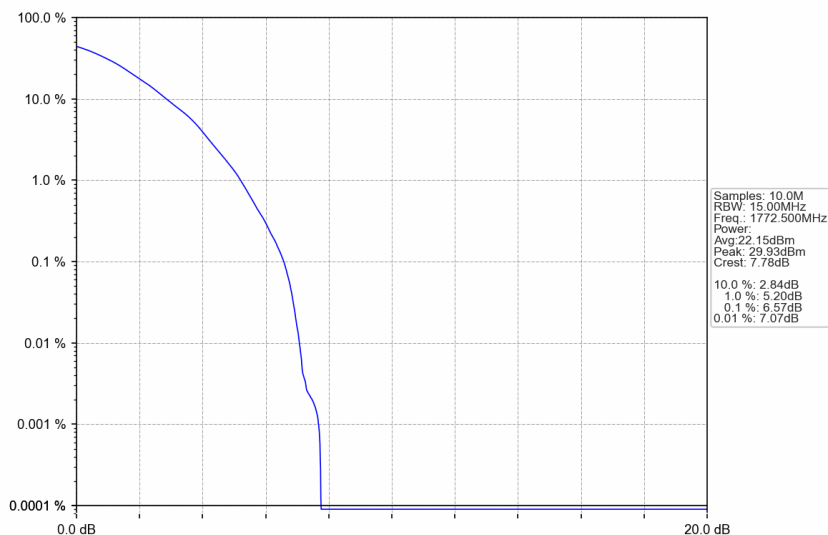
n66_15kHz_SISO_NTNV_15MHz_DFT-s-OFDM 64 QAM_1772.5MHz_Outer_Full
