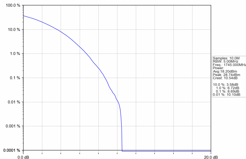
n66_15kHz_SISO_NTNV_5MHz_CP-OFDM 256 QAM_1745MHz_Outer_Full
