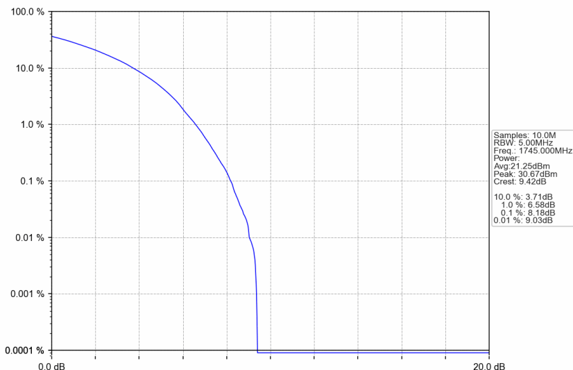
n66_15kHz_SISO_NTNV_5MHz_CP-OFDM 64 QAM_1745MHz_Outer_Full
