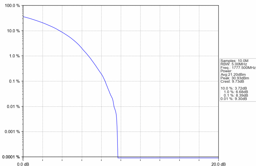
n66_15kHz_SISO_NTNV_5MHz_CP-OFDM 64 QAM_1777.5MHz_Outer_Full
