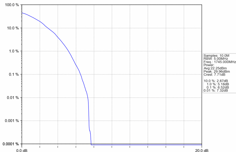
n66_15kHz_SISO_NTNV_5MHz_DFT-s-OFDM 64 QAM_1745MHz_Outer_Full
