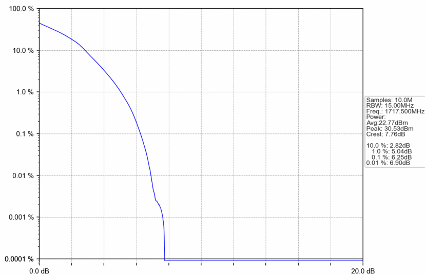
n66_15kHz_SISO_NTNV_15MHz_DFT-s-OFDM 16 QAM_1717.5MHz_Outer_Full
