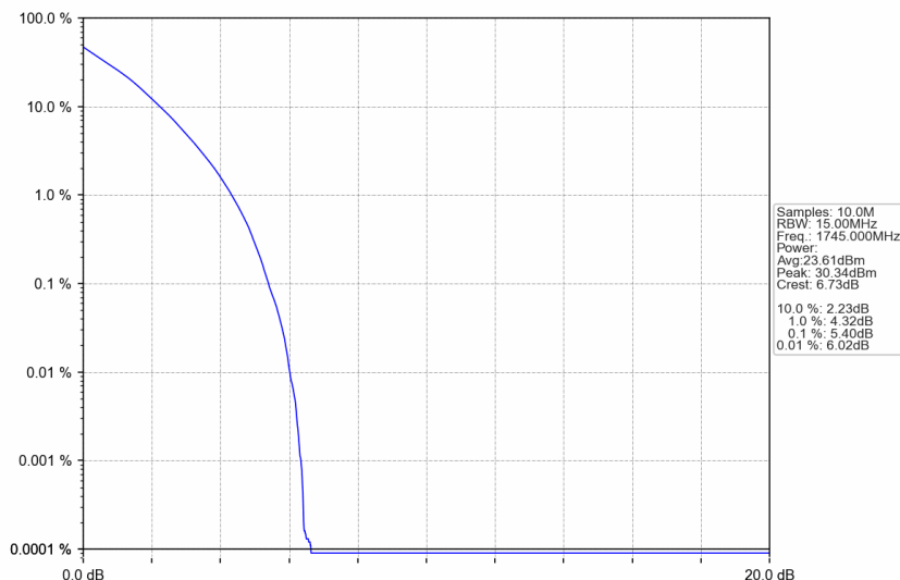
n66_15kHz_SISO_NTNV_15MHz_DFT-s-OFDM QPSK_1745MHz_Outer_Full
