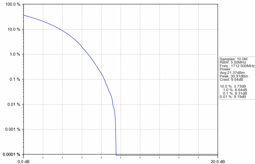
n66_15kHz_SISO_NTNV_5MHz_CP-OFDM 64 QAM_1712.5MHz_Outer_Full
