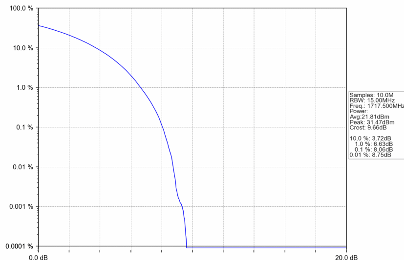
n66_15kHz_SISO_NTNV_15MHz_CP-OFDM 16 QAM_1717.5MHz_Outer_Full
