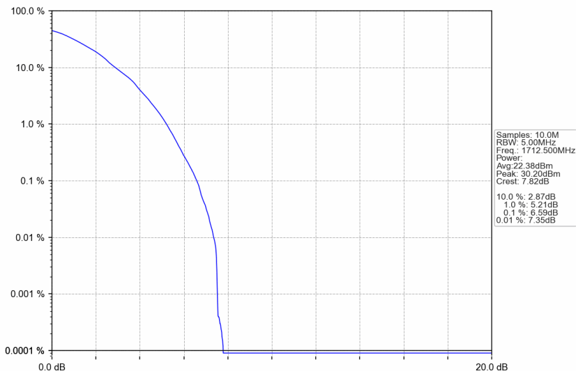
n66_15kHz_SISO_NTNV_5MHz_DFT-s-OFDM 64 QAM_1712.5MHz_Outer_Full
