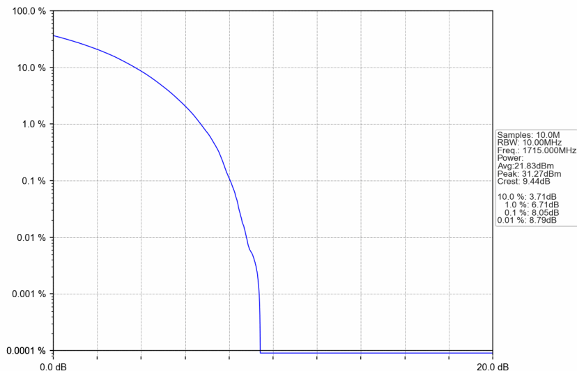
n66_15kHz_SISO_NTNV_10MHz_CP-OFDM QPSK_1715MHz_Outer_Full
