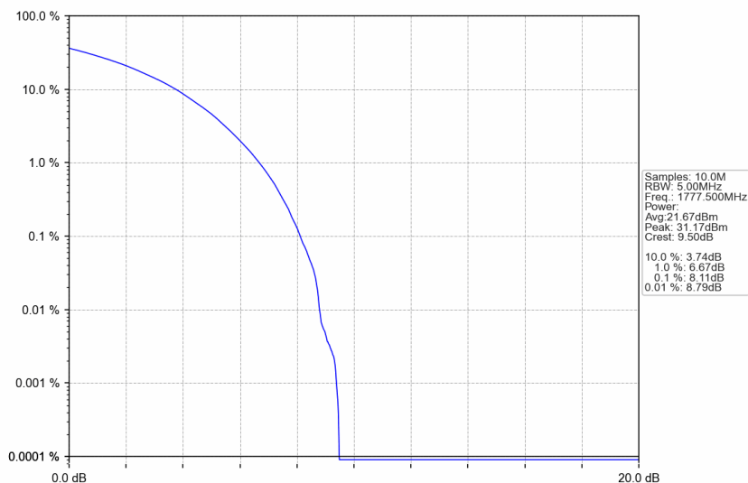
n66_15kHz_SISO_NTNV_5MHz_CP-OFDM QPSK_1777.5MHz_Outer_Full
