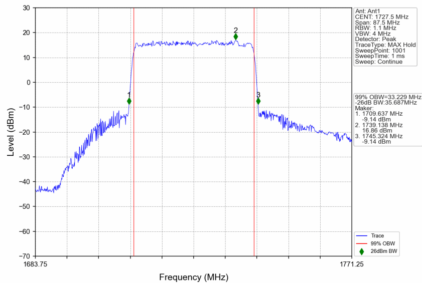
n66_30kHz_SISO_NTNV_35MHz_CP-OFDM 64 QAM_1727.5MHz_Outer_Full
