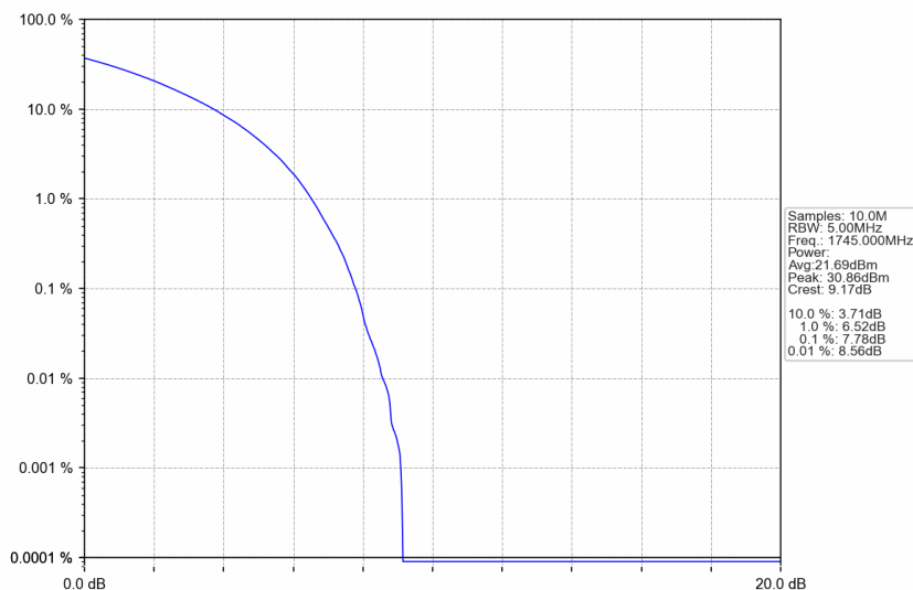
n66_15kHz_SISO_NTNV_5MHz_CP-OFDM 16 QAM_1745MHz_Outer_Full
