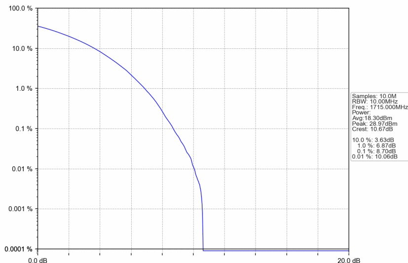
n66_15kHz_SISO_NTNV_10MHz_CP-OFDM 256 QAM_1715MHz_Outer_Full
