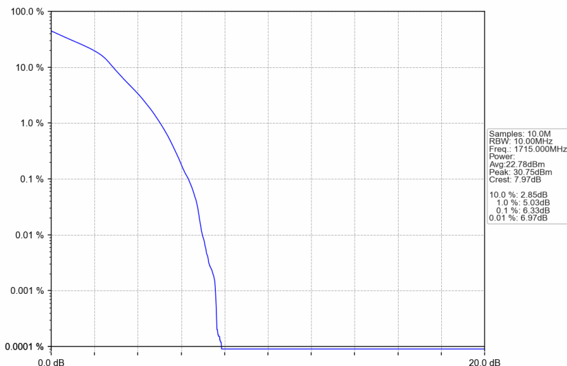
n66_15kHz_SISO_NTNV_10MHz_DFT-s-OFDM 16 QAM_1715MHz_Outer_Full
