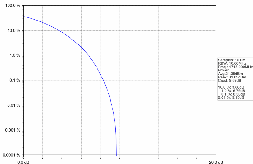
n66_15kHz_SISO_NTNV_10MHz_CP-OFDM 64 QAM_1715MHz_Outer_Full
