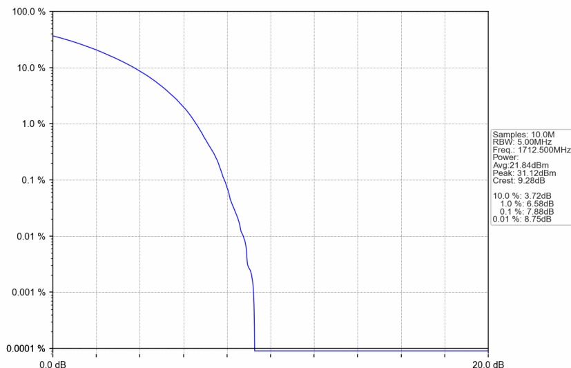
n66_15kHz_SISO_NTNV_5MHz_CP-OFDM 16 QAM_1712.5MHz_Outer_Full
