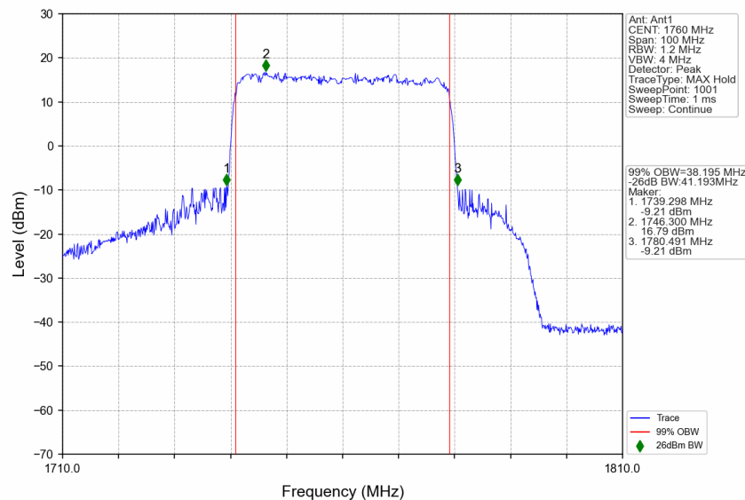
n66_30kHz_SISO_NTNV_40MHz_CP-OFDM 64 QAM_1760MHz_Outer_Full
