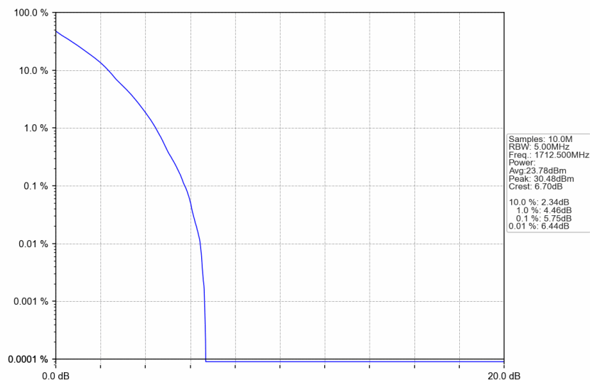
n66_15kHz_SISO_NTNV_5MHz_DFT-s-OFDM QPSK_1712.5MHz_Outer_Full
