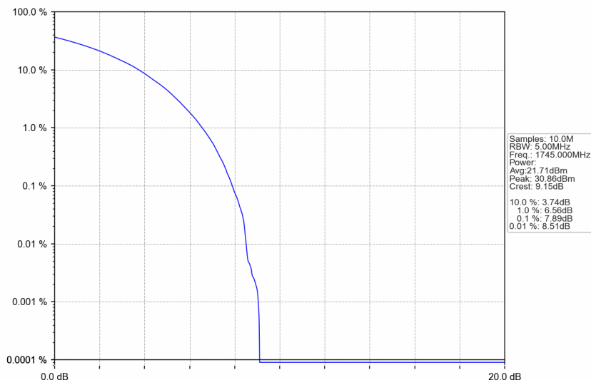
n66_15kHz_SISO_NTNV_5MHz_CP-OFDM QPSK_1745MHz_Outer_Full
