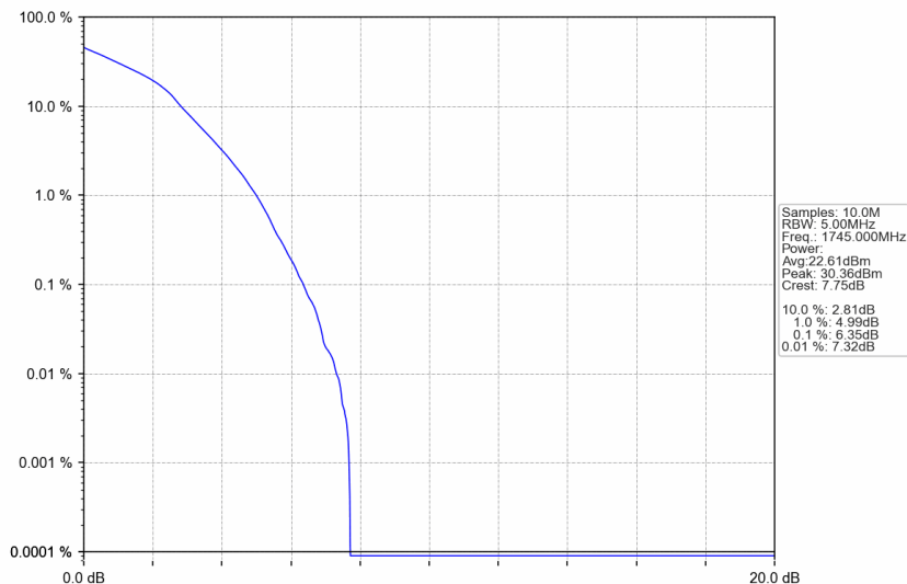
n66_15kHz_SISO_NTNV_5MHz_DFT-s-OFDM 16 QAM_1745MHz_Outer_Full
