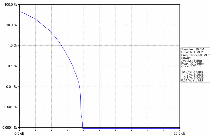
n66_15kHz_SISO_NTNV_5MHz_DFT-s-OFDM 64 QAM_1777.5MHz_Outer_Full
