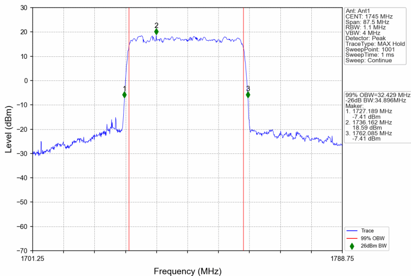
n66_30kHz_SISO_NTNV_35MHz_DFT-s-OFDM 16 QAM_1745MHz_Outer_Full
