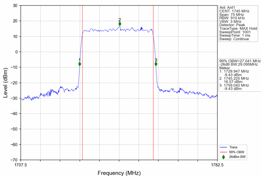
n66_30kHz_SISO_NTNV_30MHz_DFT-s-OFDM 256 QAM_1745MHz_Outer_Full
