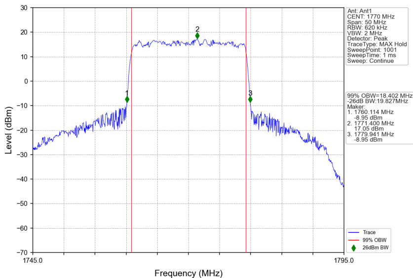
n66_30kHz_SISO_NTNV_20MHz_CP-OFDM 64 QAM_1770MHz_Outer_Full
