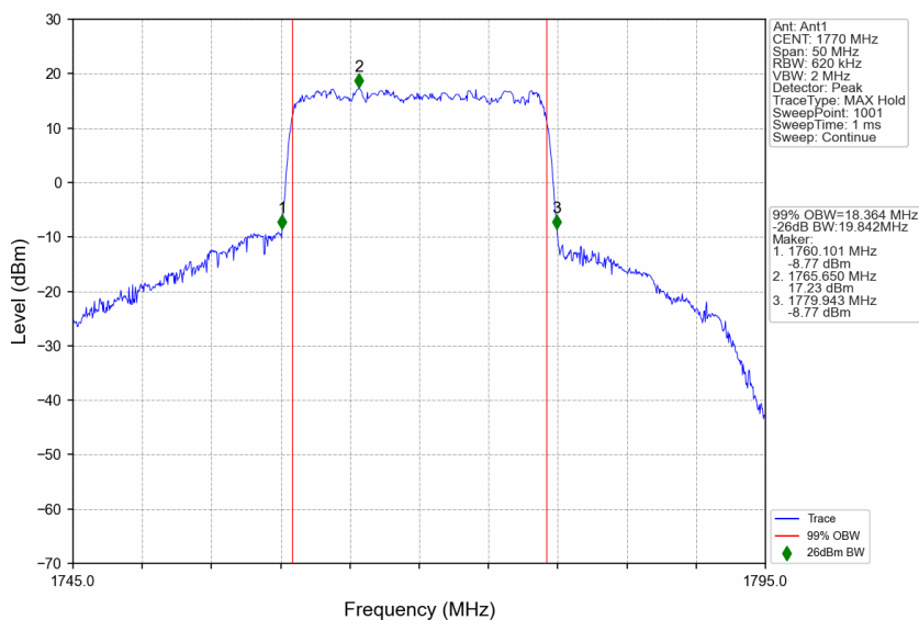
n66_30kHz_SISO_NTNV_20MHz_CP-OFDM QPSK_1770MHz_Outer_Full
