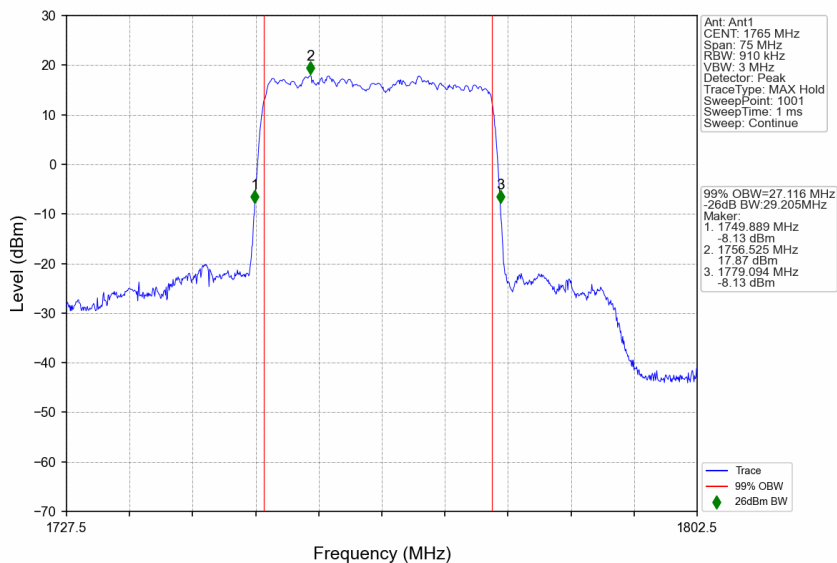
n66_30kHz_SISO_NTNV_30MHz_DFT-s-OFDM 64 QAM_1765MHz_Outer_Full
