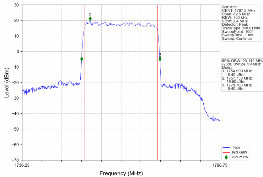
n66_30kHz_SISO_NTNV_25MHz_DFT-s-OFDM QPSK_1767.5MHz_Outer_Full
