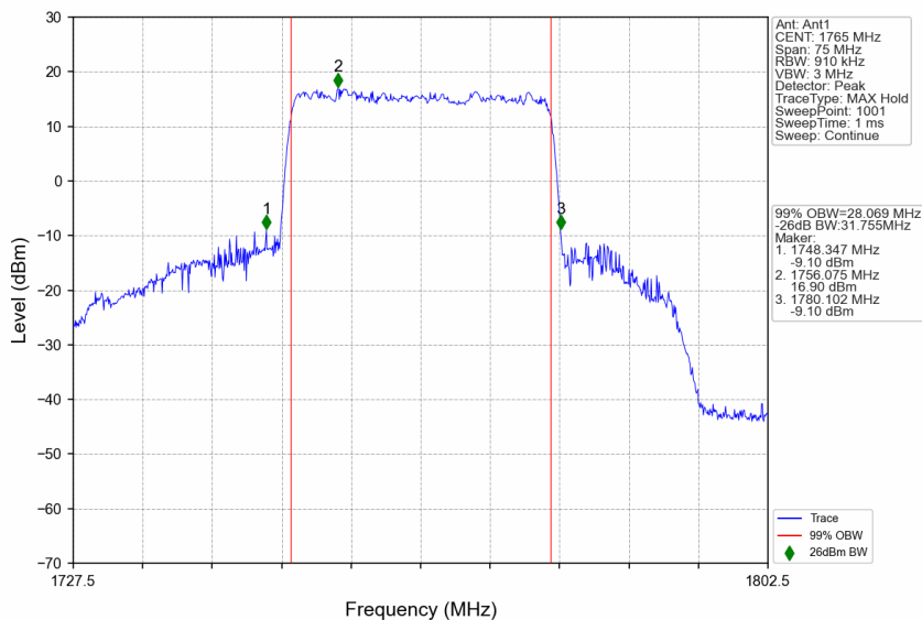
n66_30kHz_SISO_NTNV_30MHz_CP-OFDM 64 QAM_1765MHz_Outer_Full
