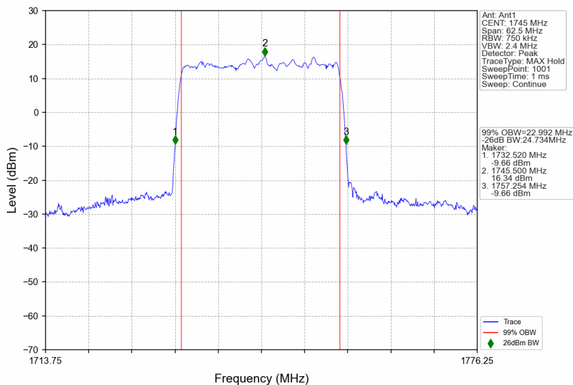
n66_30kHz_SISO_NTNV_25MHz_DFT-s-OFDM 256 QAM_1745MHz_Outer_Full
