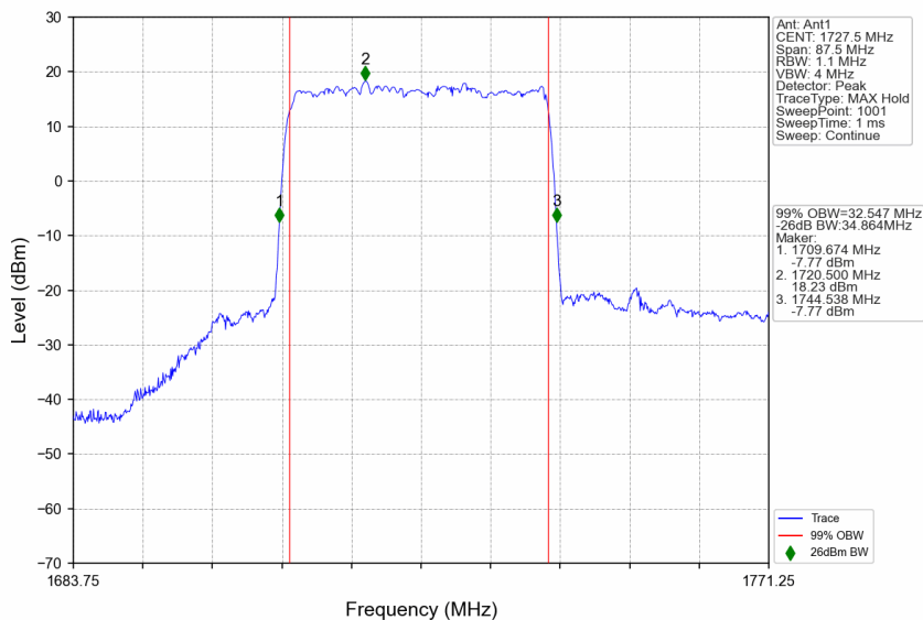
n66_30kHz_SISO_NTNV_35MHz_DFT-s-OFDM 64 QAM_1727.5MHz_Outer_Full
