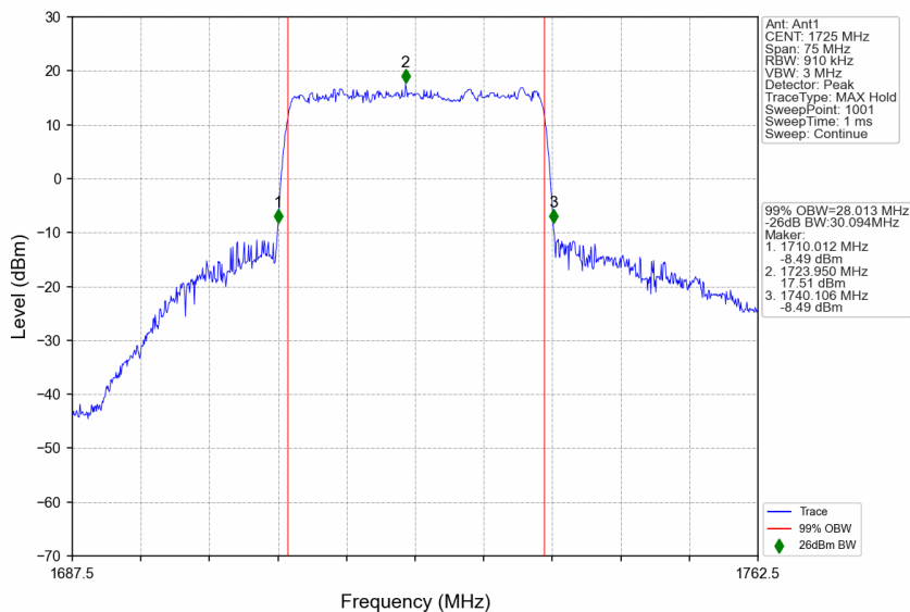
n66_30kHz_SISO_NTNV_30MHz_CP-OFDM 64 QAM_1725MHz_Outer_Full
