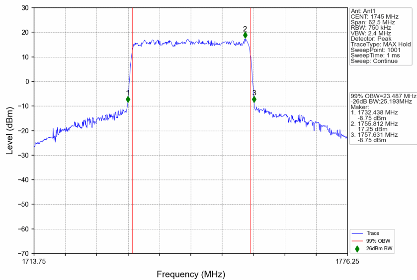
n66_30kHz_SISO_NTNV_25MHz_CP-OFDM 16 QAM_1745MHz_Outer_Full
