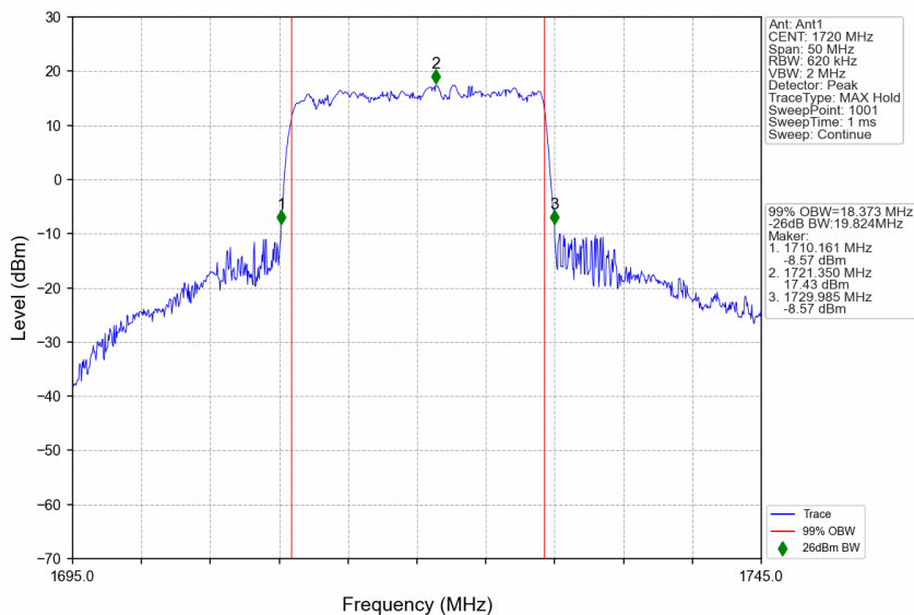
n66_30kHz_SISO_NTNV_20MHz_CP-OFDM 64 QAM_1720MHz_Outer_Full
