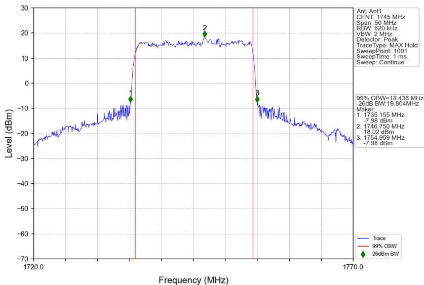
n66_30kHz_SISO_NTNV_20MHz_CP-OFDM 16 QAM_1745MHz_Outer_Full
