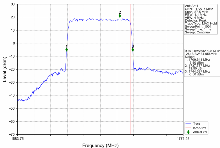
n66_30kHz_SISO_NTNV_35MHz_DFT-s-OFDM QPSK_1727.5MHz_Outer_Full
