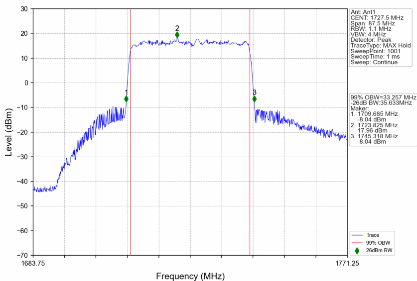
n66_30kHz_SISO_NTNV_35MHz_CP-OFDM QPSK_1727.5MHz_Outer_Full
