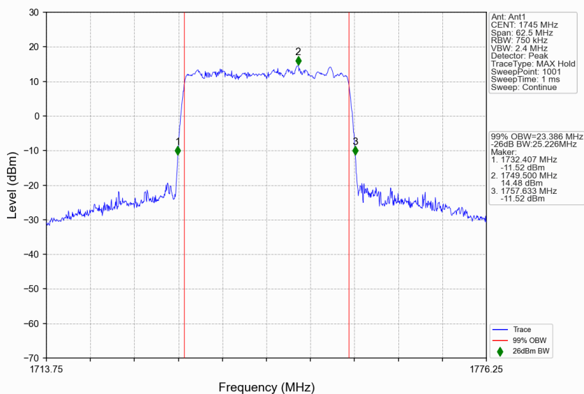
n66_30kHz_SISO_NTNV_25MHz_CP-OFDM 256 QAM_1745MHz_Outer_Full
