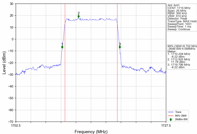
n66_30kHz_SISO_NTNV_10MHz_DFT-s-OFDM 64 QAM_1715MHz_Outer_Full
