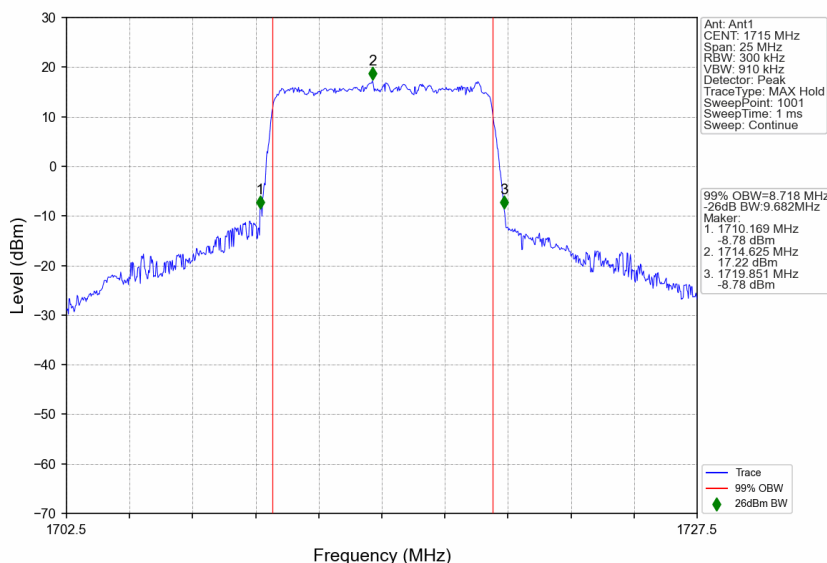
n66_30kHz_SISO_NTNV_10MHz_CP-OFDM QPSK_1715MHz_Outer_Full
