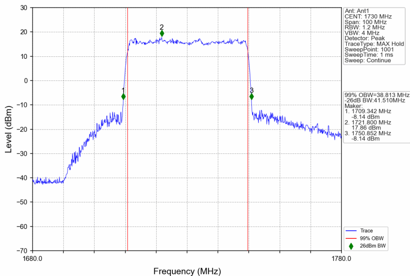
n66_15kHz_SISO_NTNV_40MHz_CP-OFDM 64 QAM_1730MHz_Outer_Full
