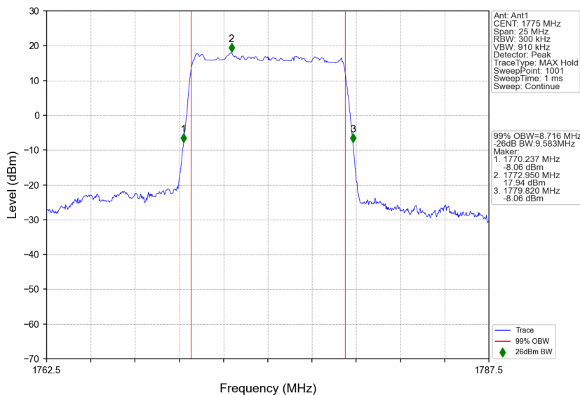
n66_30kHz_SISO_NTNV_10MHz_DFT-s-OFDM 64 QAM_1775MHz_Outer_Full
