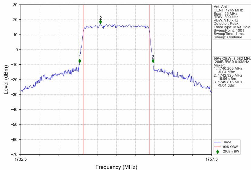
n66_30kHz_SISO_NTNV_10MHz_CP-OFDM 16 QAM_1745MHz_Outer_Full
