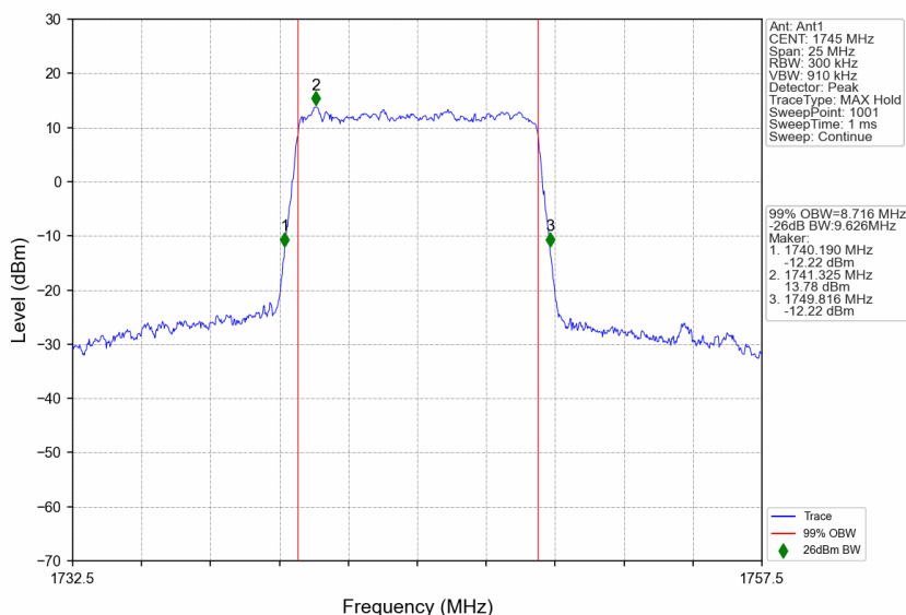
n66_30kHz_SISO_NTNV_10MHz_CP-OFDM 256 QAM_1745MHz_Outer_Full
