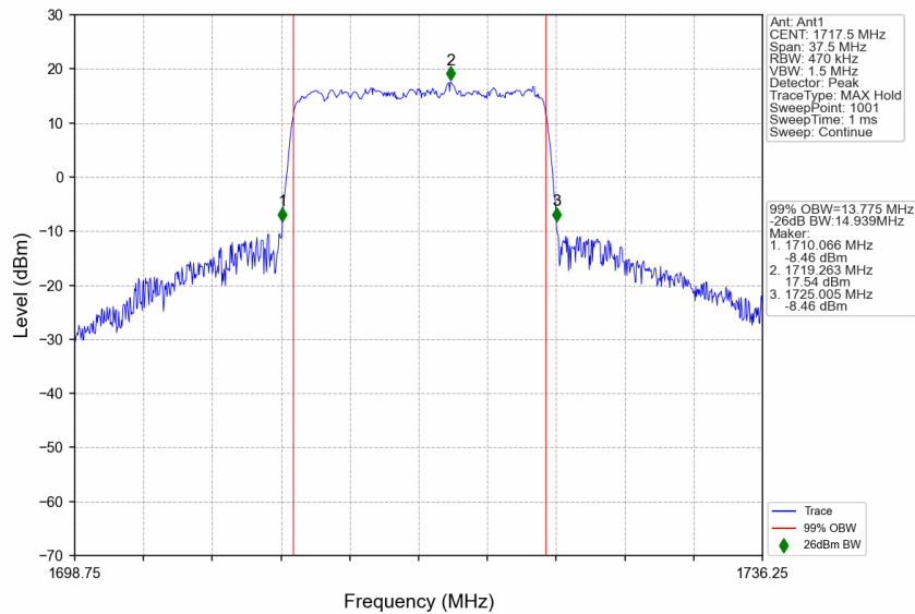
n66_30kHz_SISO_NTNV_15MHz_CP-OFDM 64 QAM_1717.5MHz_Outer_Full
