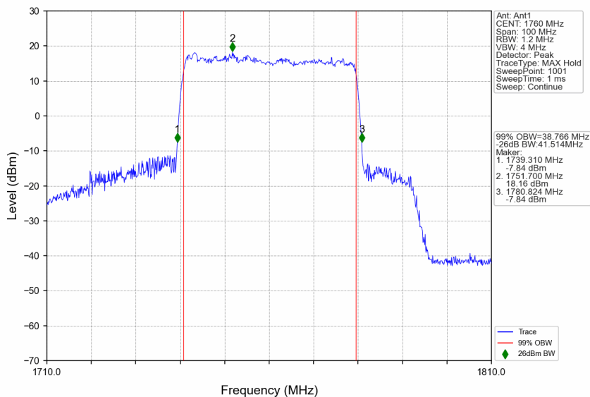
n66_15kHz_SISO_NTNV_40MHz_CP-OFDM 64 QAM_1760MHz_Outer_Full
