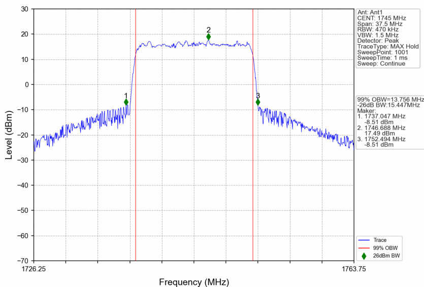
n66_30kHz_SISO_NTNV_15MHz_CP-OFDM 16 QAM_1745MHz_Outer_Full
