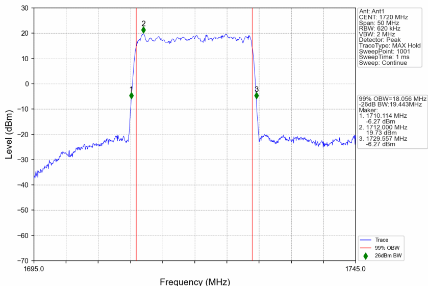
n66_30kHz_SISO_NTNV_20MHz_DFT-s-OFDM QPSK_1720MHz_Outer_Full
