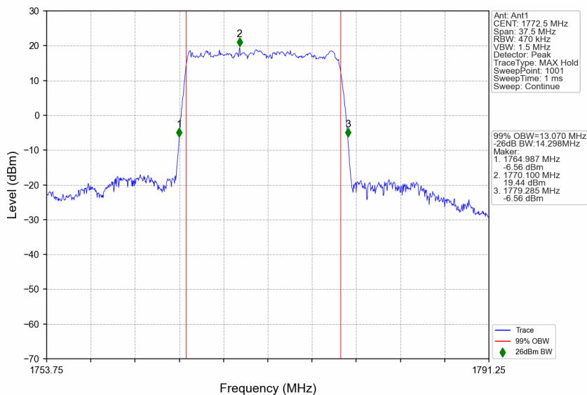
n66_30kHz_SISO_NTNV_15MHz_DFT-s-OFDM QPSK_1772.5MHz_Outer_Full
