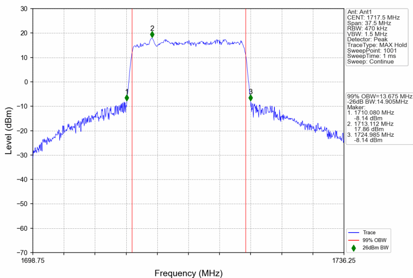
n66_30kHz_SISO_NTNV_15MHz_CP-OFDM QPSK_1717.5MHz_Outer_Full
