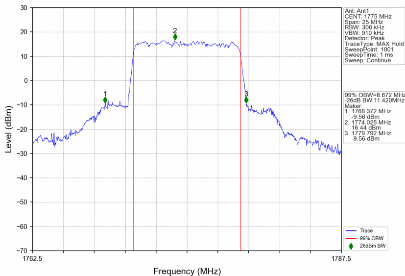
n66_30kHz_SISO_NTNV_10MHz_CP-OFDM 64 QAM_1775MHz_Outer_Full
