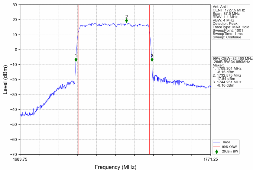
n66_15kHz_SISO_NTNV_35MHz_DFT-s-OFDM 64 QAM_1727.5MHz_Outer_Full
