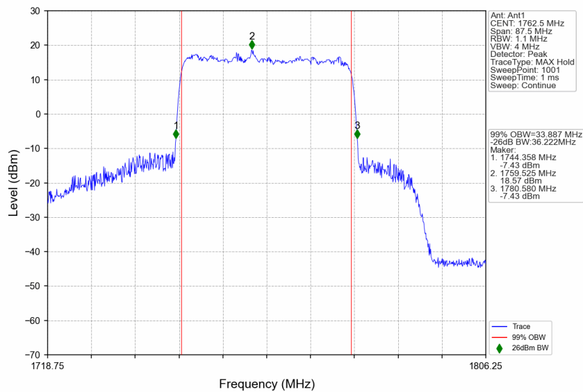
n66_15kHz_SISO_NTNV_35MHz_CP-OFDM 64 QAM_1762.5MHz_Outer_Full
