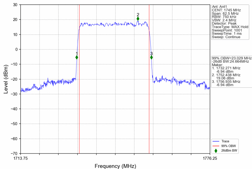
n66_15kHz_SISO_NTNV_25MHz_DFT-s-OFDM 16 QAM_1745MHz_Outer_Full
