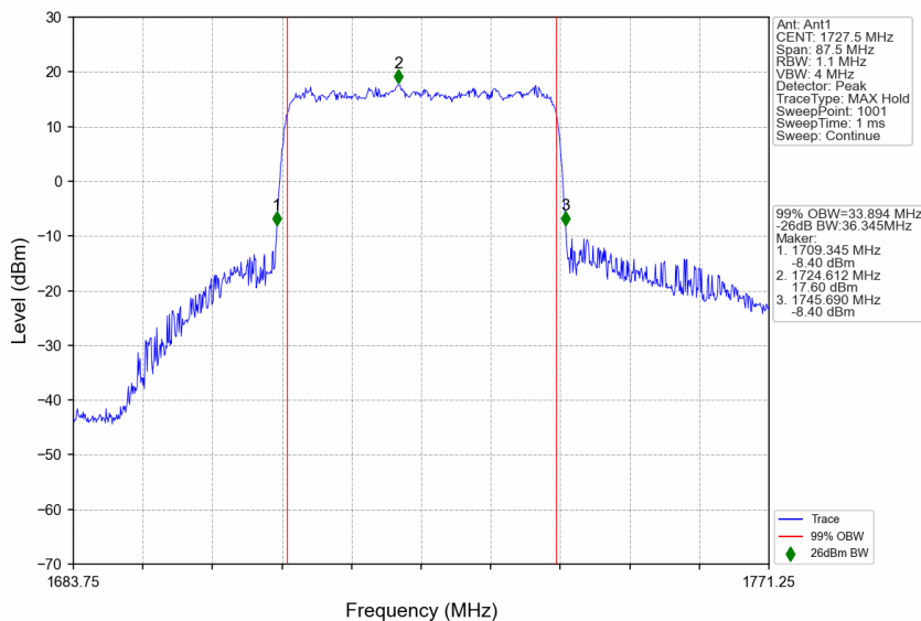
n66_15kHz_SISO_NTNV_35MHz_CP-OFDM 64 QAM_1727.5MHz_Outer_Full
