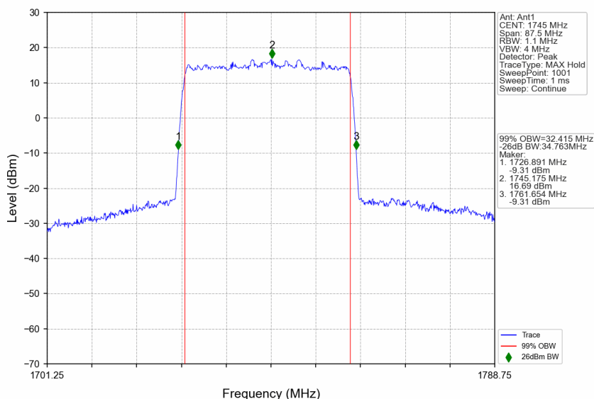
n66_15kHz_SISO_NTNV_35MHz_DFT-s-OFDM 256 QAM_1745MHz_Outer_Full
