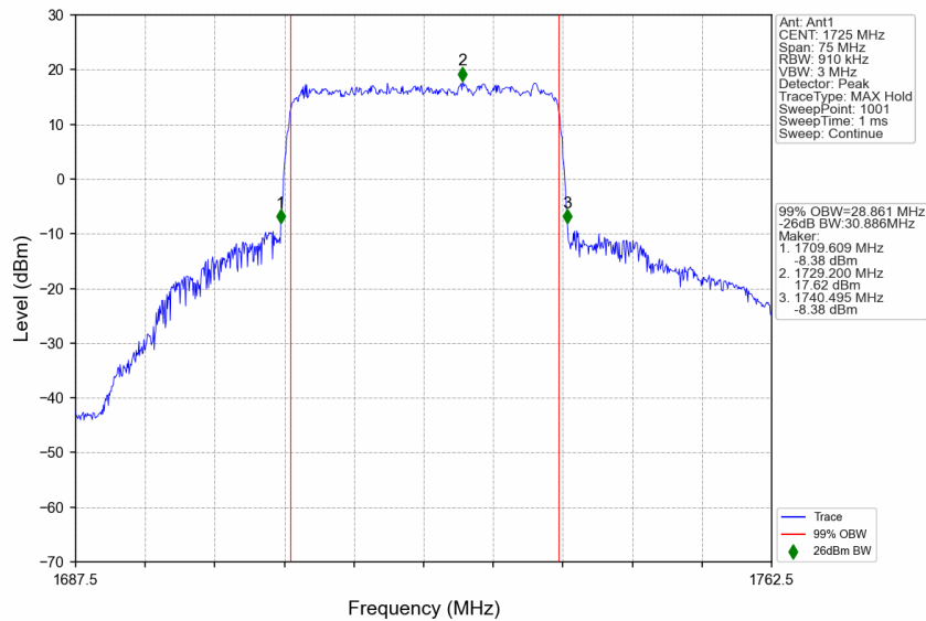
n66_15kHz_SISO_NTNV_30MHz_CP-OFDM QPSK_1725MHz_Outer_Full
