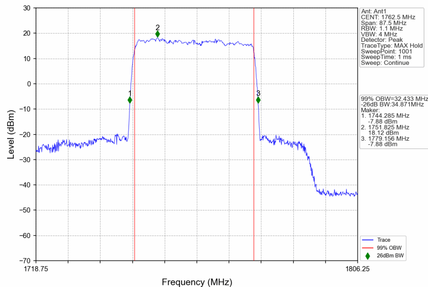
n66_15kHz_SISO_NTNV_35MHz_DFT-s-OFDM 64 QAM_1762.5MHz_Outer_Full
