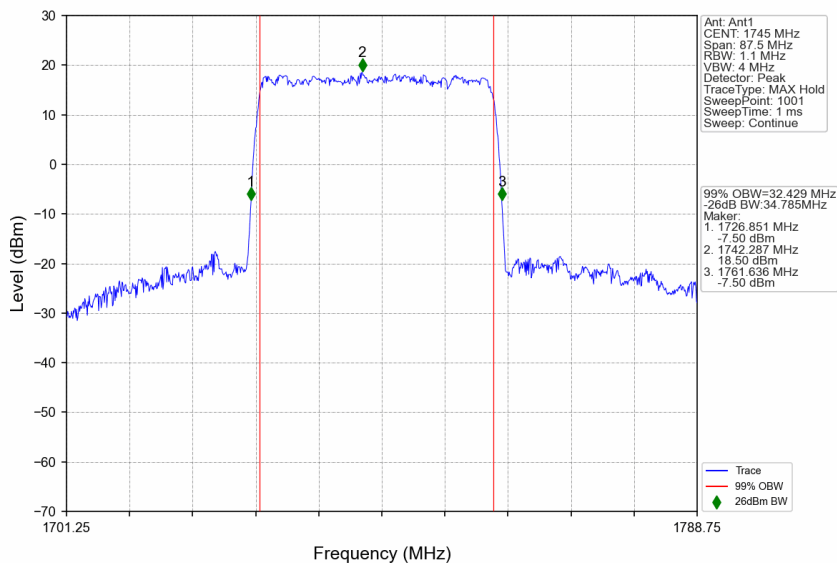
n66_15kHz_SISO_NTNV_35MHz_DFT-s-OFDM 16 QAM_1745MHz_Outer_Full
