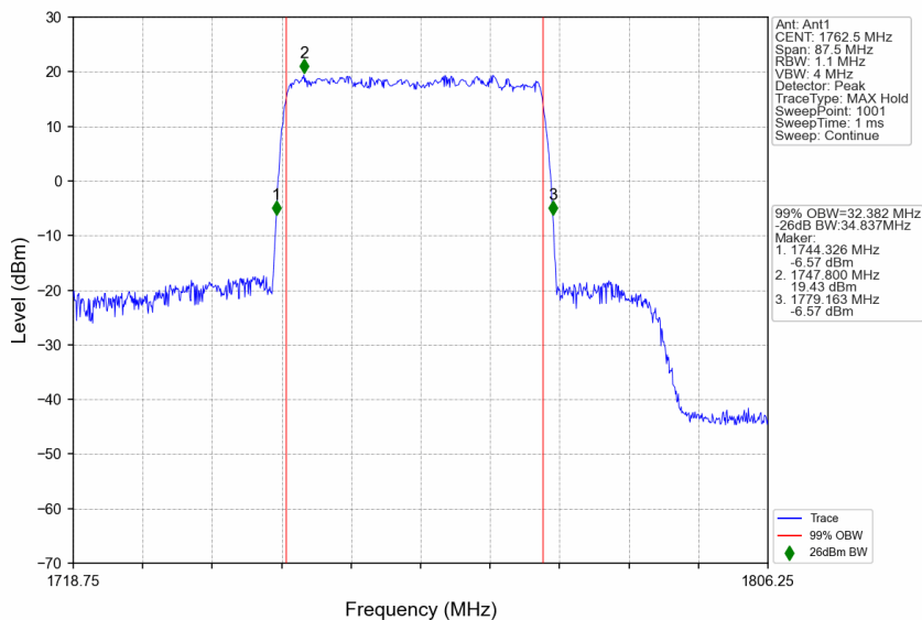
n66_15kHz_SISO_NTNV_35MHz_DFT-s-OFDM QPSK_1762.5MHz_Outer_Full
