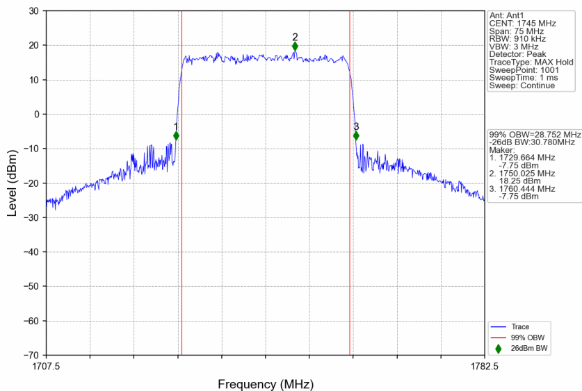
n66_15kHz_SISO_NTNV_30MHz_CP-OFDM 16 QAM_1745MHz_Outer_Full
