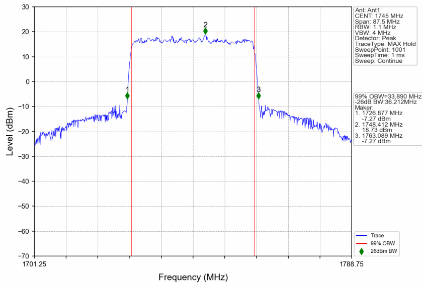
n66_15kHz_SISO_NTNV_35MHz_CP-OFDM 16 QAM_1745MHz_Outer_Full
