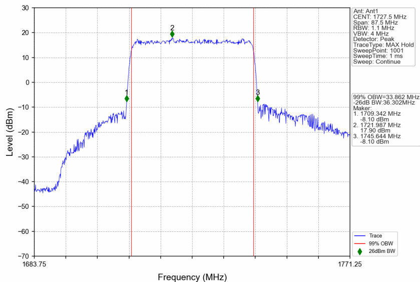
n66_15kHz_SISO_NTNV_35MHz_CP-OFDM QPSK_1727.5MHz_Outer_Full
