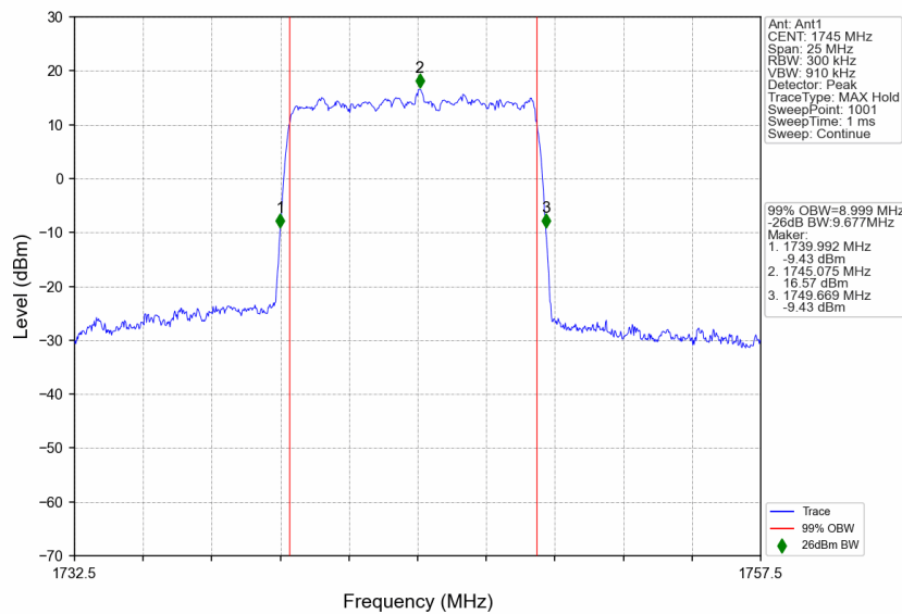
n66_15kHz_SISO_NTNV_10MHz_DFT-s-OFDM 256 QAM_1745MHz_Outer_Full
