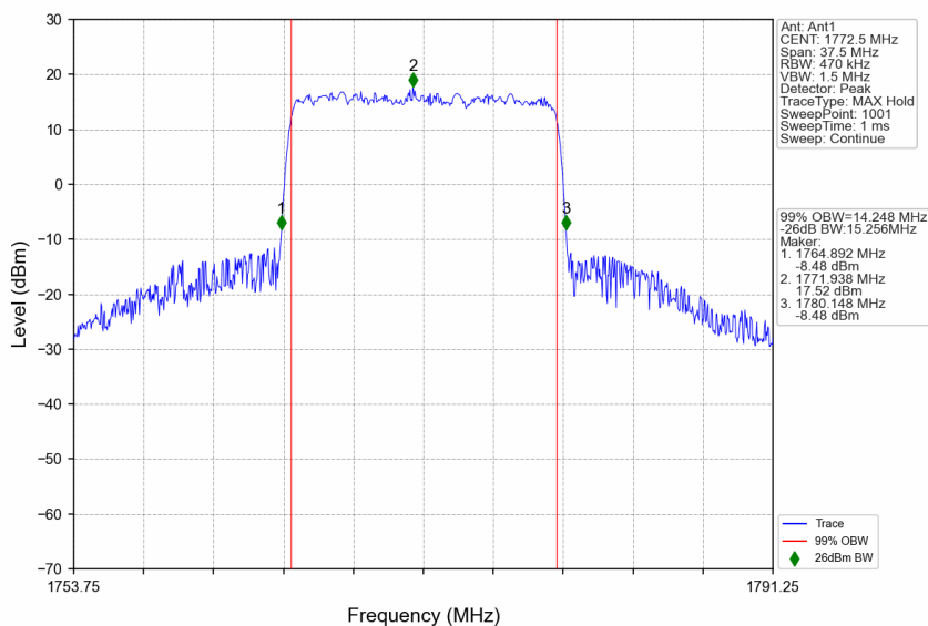
n66_15kHz_SISO_NTNV_15MHz_CP-OFDM 64 QAM_1772.5MHz_Outer_Full
