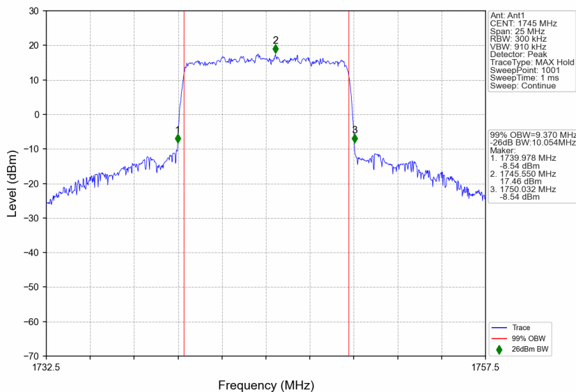
n66_15kHz_SISO_NTNV_10MHz_CP-OFDM 16 QAM_1745MHz_Outer_Full
