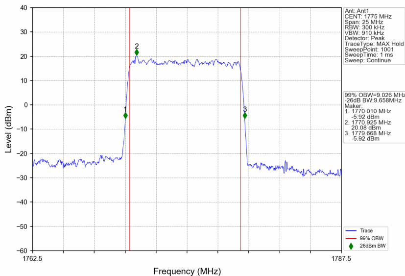
n66_15kHz_SISO_NTNV_10MHz_DFT-s-OFDM QPSK_1775MHz_Outer_Full
