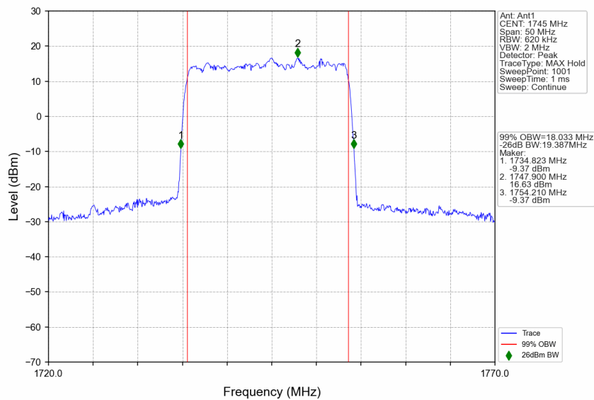
n66_15kHz_SISO_NTNV_20MHz_DFT-s-OFDM 256 QAM_1745MHz_Outer_Full
