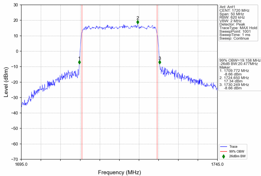
n66_15kHz_SISO_NTNV_20MHz_CP-OFDM 64 QAM_1720MHz_Outer_Full
