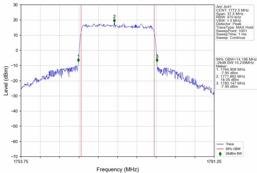
n66_15kHz_SISO_NTNV_15MHz_CP-OFDM QPSK_1772.5MHz_Outer_Full
