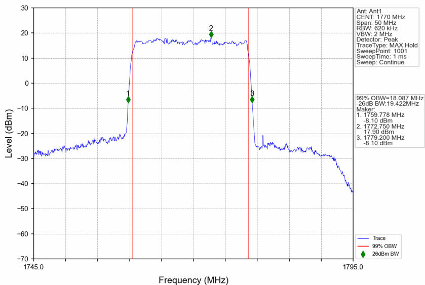
n66_15kHz_SISO_NTNV_20MHz_DFT-s-OFDM 64 QAM_1770MHz_Outer_Full
