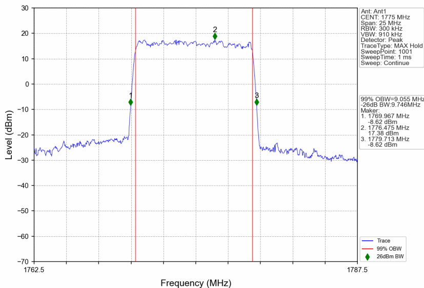
n66_15kHz_SISO_NTNV_10MHz_DFT-s-OFDM 64 QAM_1775MHz_Outer_Full
