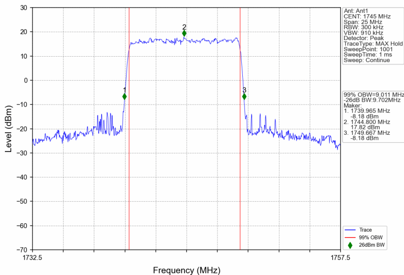
n66_15kHz_SISO_NTNV_10MHz_DFT-s-OFDM 16 QAM_1745MHz_Outer_Full
