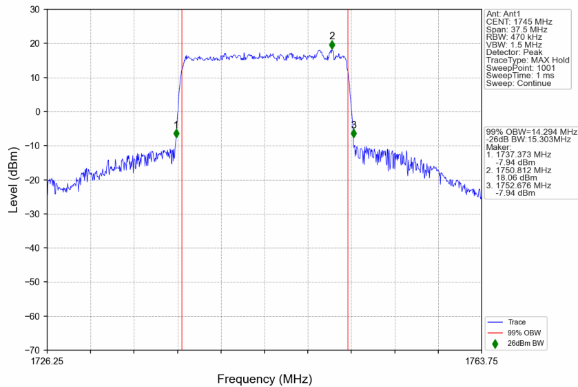
n66_15kHz_SISO_NTNV_15MHz_CP-OFDM 16 QAM_1745MHz_Outer_Full
