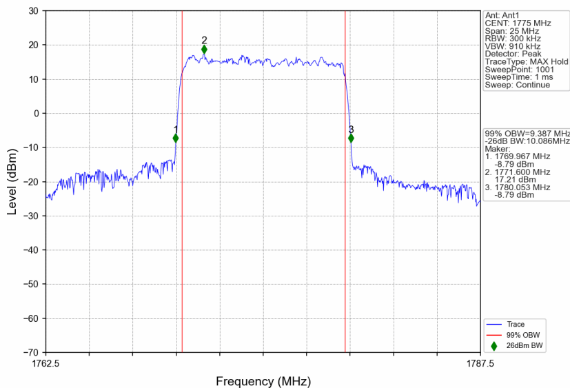
n66_15kHz_SISO_NTNV_10MHz_CP-OFDM 64 QAM_1775MHz_Outer_Full
