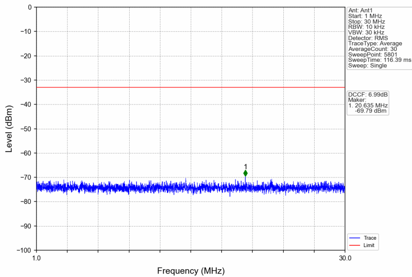
n41_30kHz_SISO_NTNV_100MHz_CP-OFDM QPSK_2592.99MHz_Edge_1RB_Left
