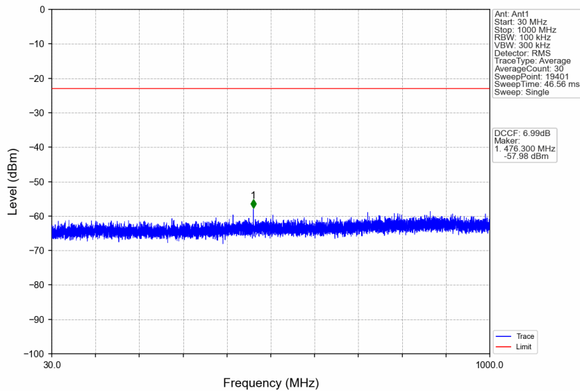
n41_30kHz_SISO_NTNV_100MHz_DFT-s-OFDM_QPSK_2546.01MHz_Edge_1RB_Left
