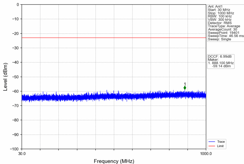
n41_30kHz_SISO_NTNV_100MHz_CP-OFDM QPSK_2546.01MHz_Edge_1RB_Left
