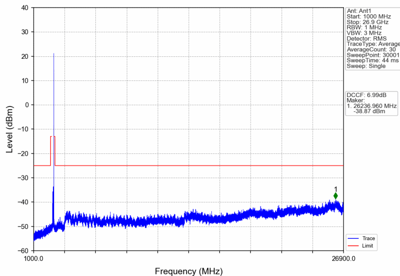
n41_30kHz_SISO_NTNV_90MHz_CP-OFDM QPSK_2644.98MHz_Edge_1RB_Right
