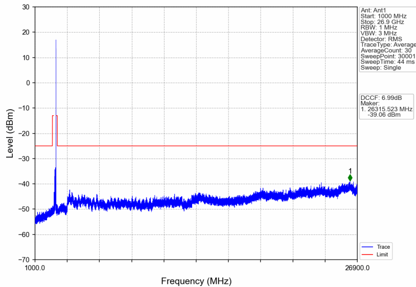
n41_30kHz_SISO_NTNV_100MHz_CP-OFDM QPSK_2640MHz_Edge_1RB_Right
