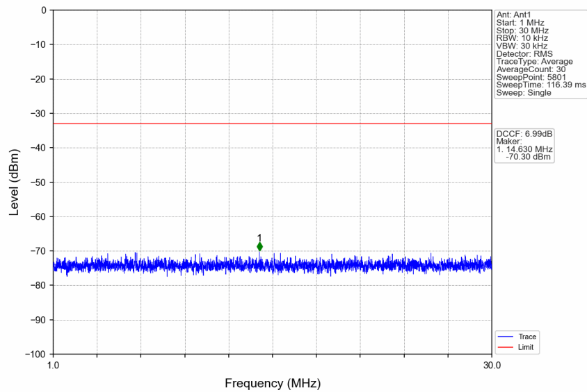
n41_30kHz_SISO_NTNV_100MHz_DFT-s-OFDM_QPSK_2592.99MHz_Edge_1RB_Left
