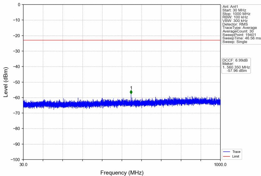
n41_30kHz_SISO_NTNV_90MHz_DFT-s-OFDM_QPSK_2644.98MHz_Edge_1RB_Right
