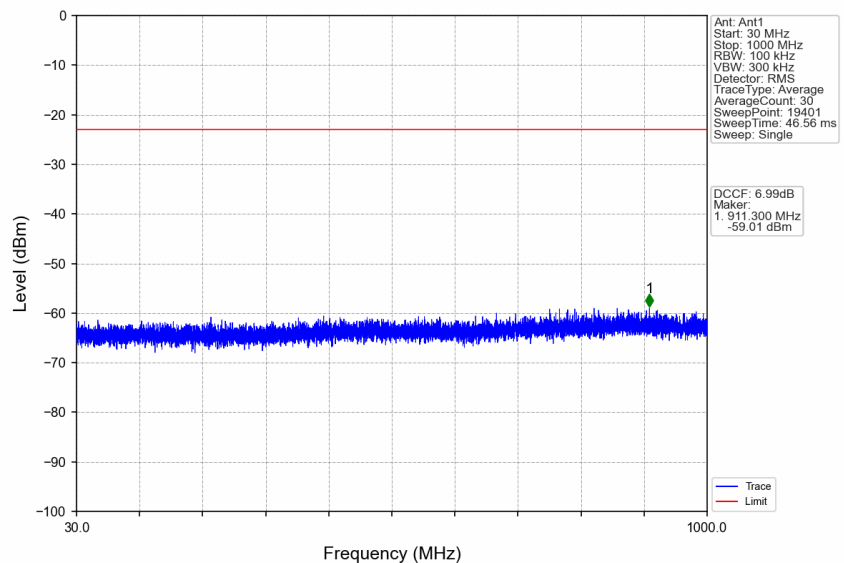
n41_30kHz_SISO_NTNV_80MHz_CP-OFDM QPSK_2592.99MHz_Edge_1RB_Left
