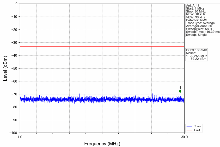
n41_30kHz_SISO_NTNV_80MHz_DFT-s-OFDM QPSK_2592.99MHz_Edge_1RB_Left
