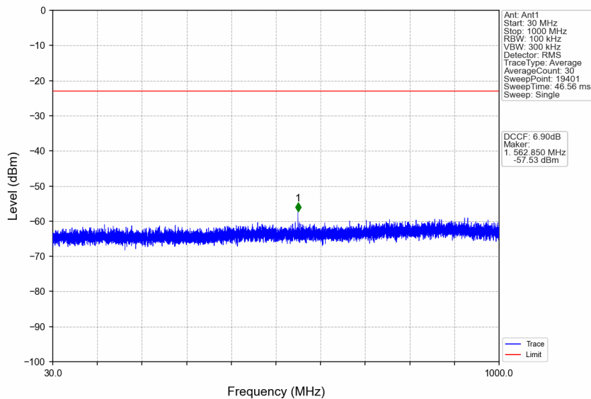
n41_30kHz_SISO_NTNV_80MHz_DFT-s-OFDM_QPSK_2649.99MHz_Edge_1RB_Right
