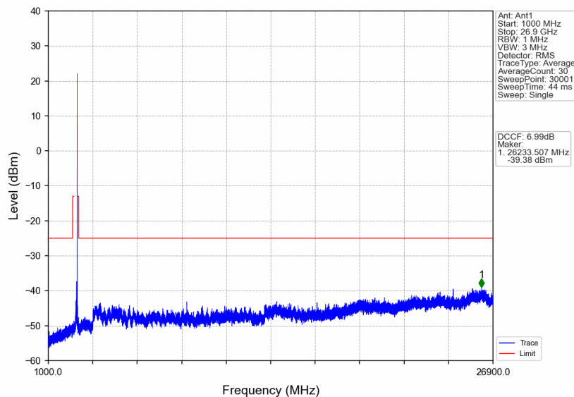
n41_30kHz_SISO_NTNV_80MHz_CP-OFDM QPSK_2649.99MHz_Edge_1RB_Right
