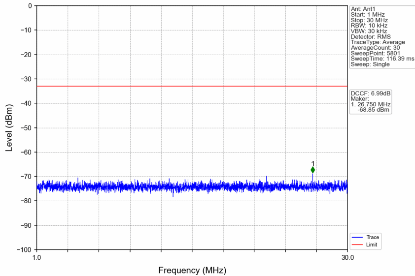
n41_30kHz_SISO_NTNV_80MHz_CP-OFDM QPSK_2649.99MHz_Edge_1RB_Right
