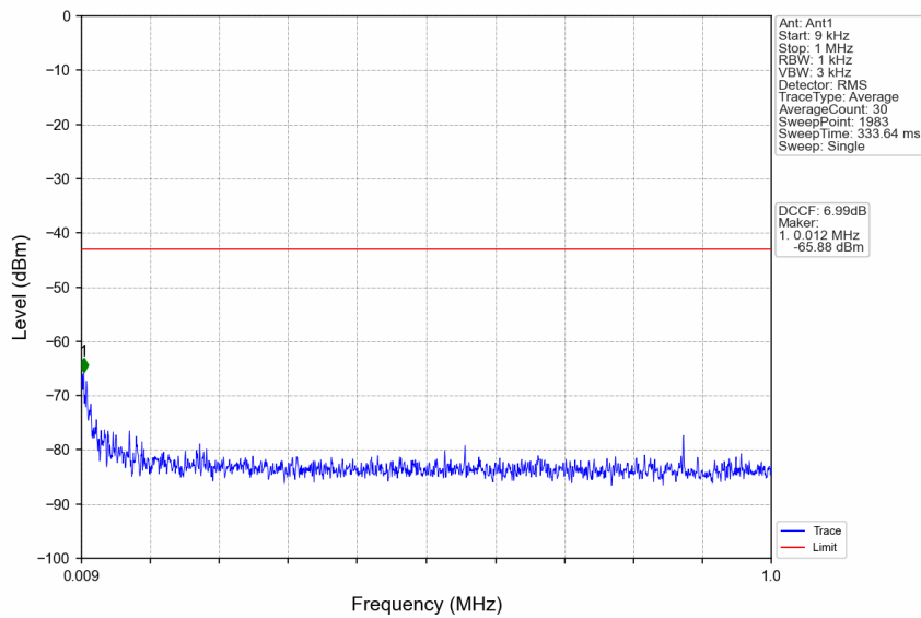
n41_30kHz_SISO_NTNV_90MHz_DFT-s-OFDM_QPSK_2644.98MHz_Edge_1RB_Right
