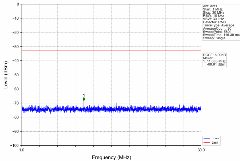
n41_30kHz_SISO_NTNV_80MHz_CP-OFDM QPSK_2536.02MHz_Edge_1RB_Left
