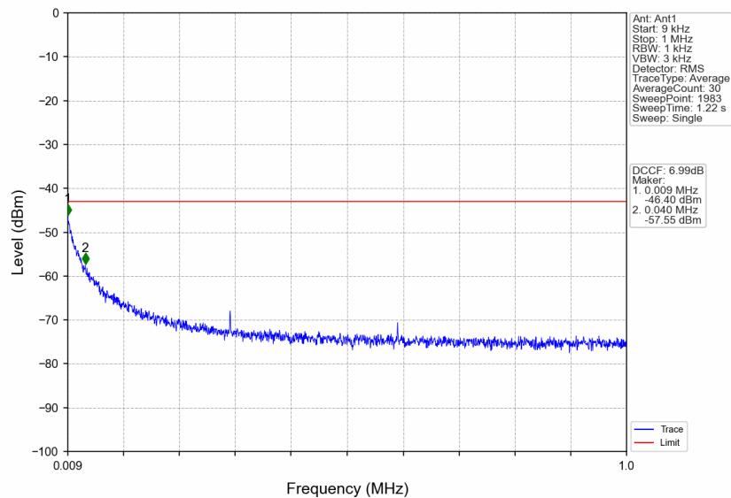
n41_30kHz_SISO_NTNV_60MHz_DFT-s-OFDM_QPSK_2659.98MHz_Edge_1RB_Right
