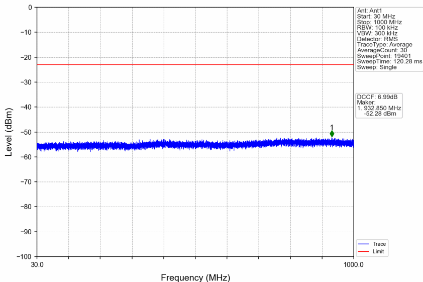
n41_30kHz_SISO_NTNV_60MHz_CP-OFDM QPSK_2659.98MHz_Edge_1RB_Right
