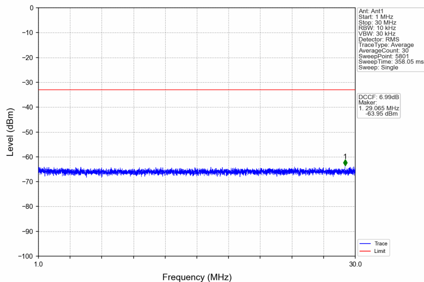
n41_30kHz_SISO_NTNV_60MHz_DFT-s-OFDM_QPSK_2659.98MHz_Edge_1RB_Right
