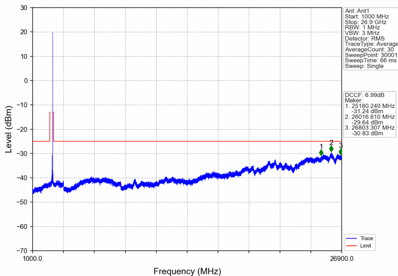
n41_30kHz_SISO_NTNV_60MHz_CP-OFDM QPSK_2659.98MHz_Edge_1RB_Right
