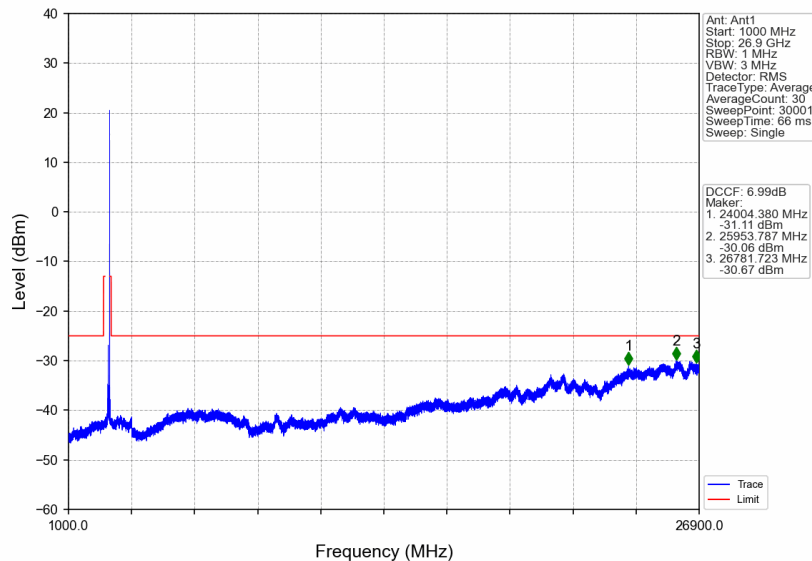
n41_30kHz_SISO_NTNV_60MHz_DFT-s-OFDM_QPSK_2659.98MHz_Edge_1RB_Right
