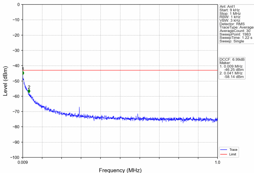
n41_30kHz_SISO_NTNV_60MHz_CP-OFDM QPSK_2659.98MHz_Edge_1RB_Right
