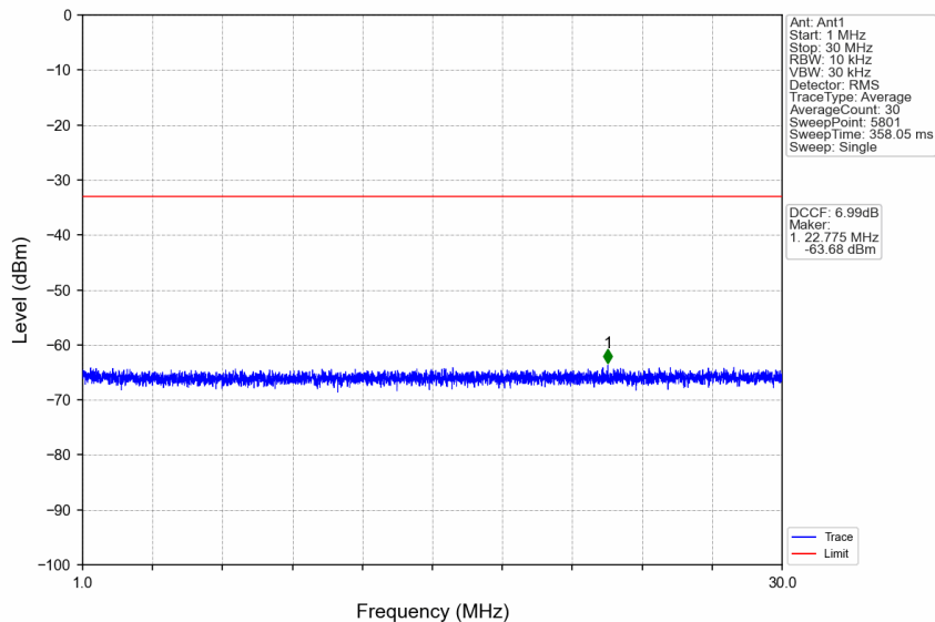
n41_30kHz_SISO_NTNV_50MHz_CP-OFDM QPSK_2664.99MHz_Edge_1RB_Right
