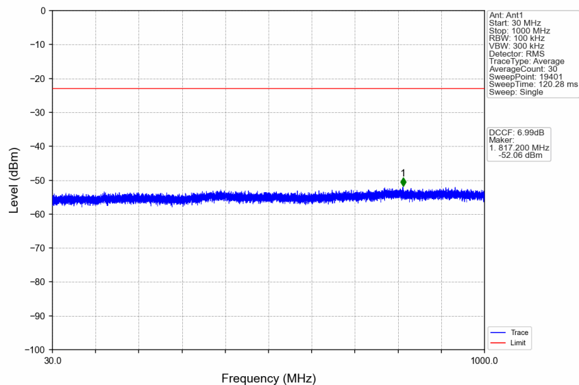
n41_30kHz_SISO_NTNV_50MHz_DFT-s-OFDM QPSK_2592.99MHz_Edge_1RB_Left
