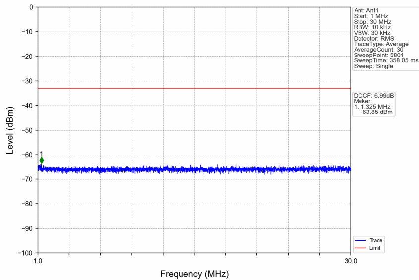
n41_30kHz_SISO_NTNV_40MHz_CP-OFDM QPSK_2592.99MHz_Edge_1RB_Left
