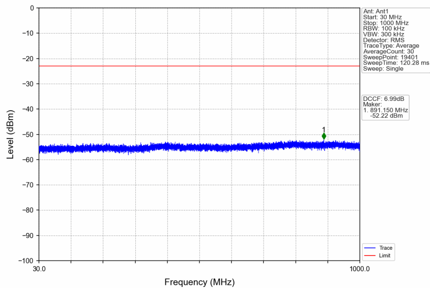
n41_30kHz_SISO_NTNV_50MHz_CP-OFDM QPSK_2521.02MHz_Edge_1RB_Left
