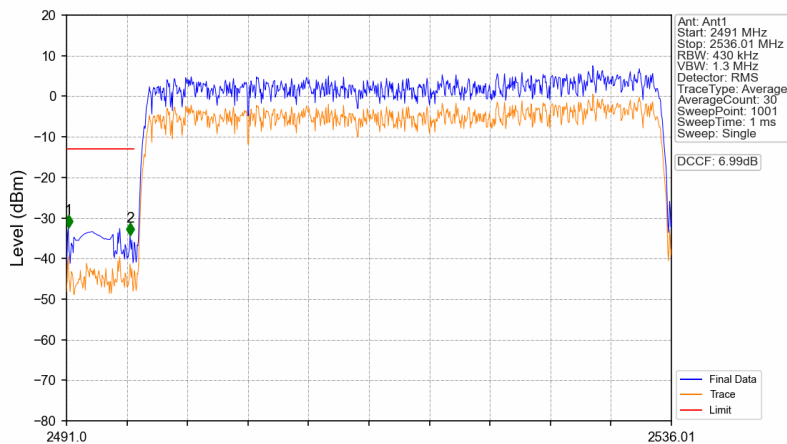
n41_30kHz_SISO_NTNV_40MHz_CP-OFDM QPSK_2516.01MHz_Outer_Full
