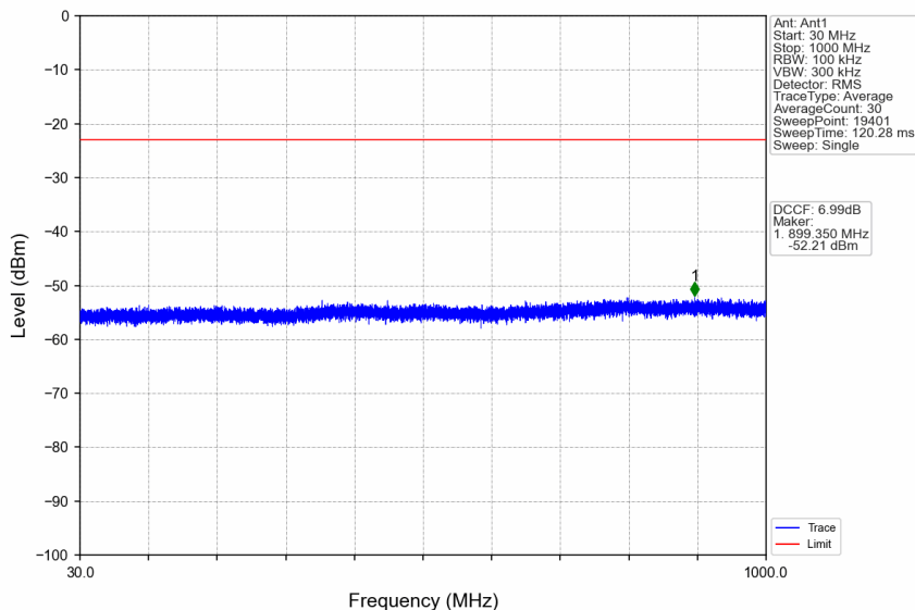
n41_30kHz_SISO_NTNV_50MHz_CP-OFDM QPSK_2664.99MHz_Edge_1RB_Right
