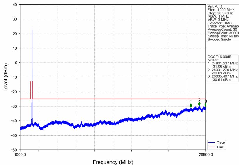
n41_30kHz_SISO_NTNV_50MHz_DFT-s-OFDM PI/2 BPSK_2664.99MHz_Edge_1RB_Right
