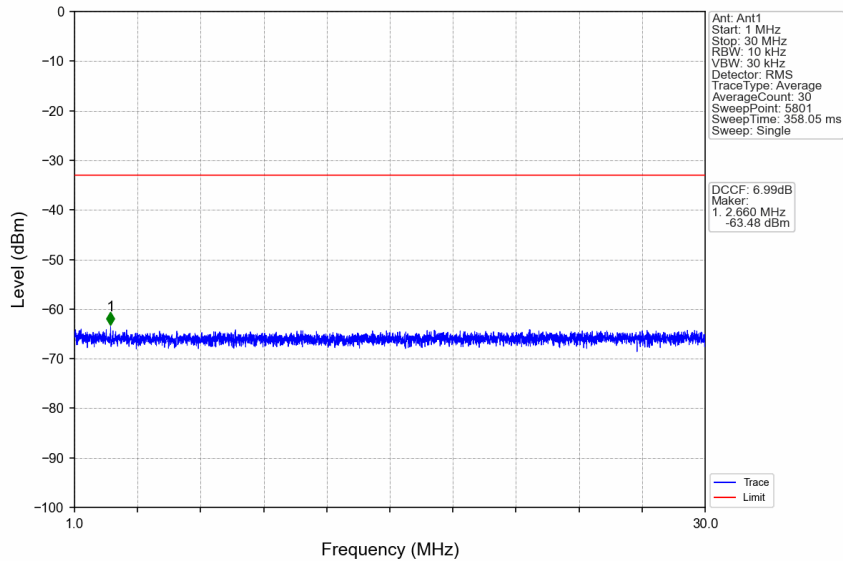
n41_30kHz_SISO_NTNV_50MHz_DFT-s-OFDM_QPSK_2664.99MHz_Edge_1RB_Right
