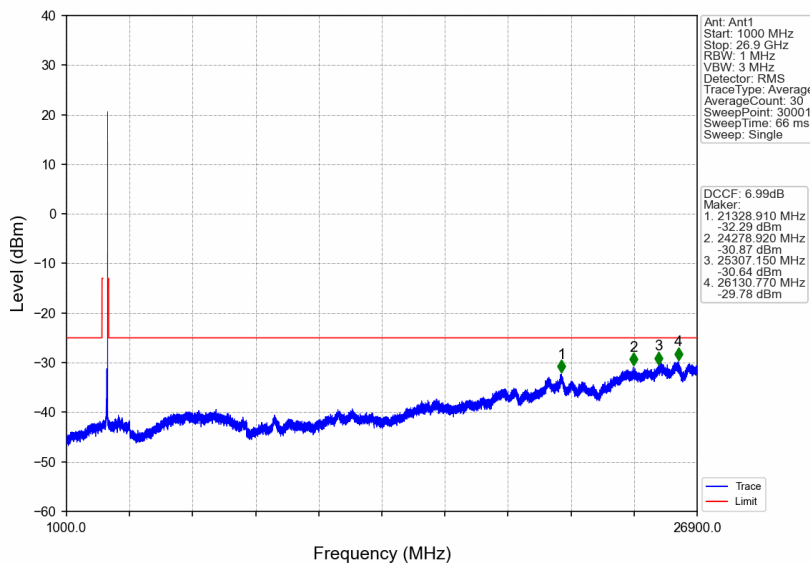
n41_30kHz_SISO_NTNV_40MHz_CP-OFDM QPSK_2670MHz_Edge_1RB_Right
