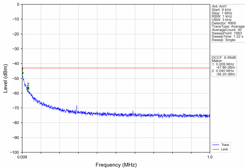
n41_30kHz_SISO_NTNV_60MHz_DFT-s-OFDM PI/2 BPSK_2659.98MHz_Edge_1RB_Right
