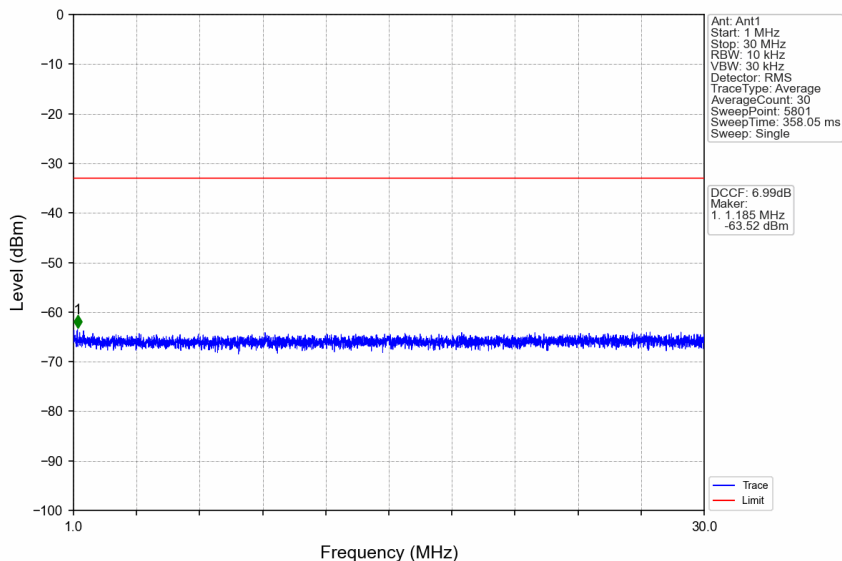
n41_30kHz_SISO_NTNV_40MHz_CP-OFDM QPSK_2516.01MHz_Edge_1RB_Left
