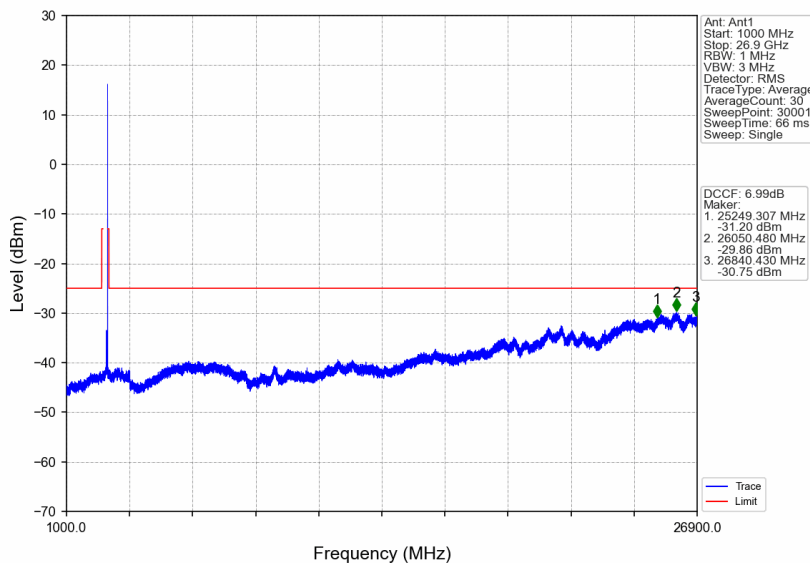
n41_30kHz_SISO_NTNV_50MHz_CP-OFDM QPSK_2664.99MHz_Edge_1RB_Right
