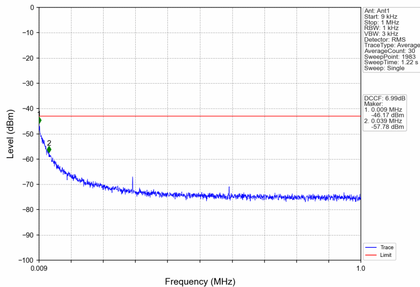
n41_30kHz_SISO_NTNV_40MHz_CP-OFDM QPSK_2670MHz_Edge_1RB_Right
