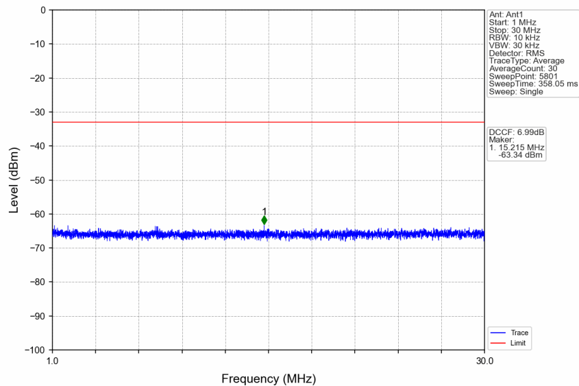
n41_30kHz_SISO_NTNV_50MHz_DFT-s-OFDM PI/2 BPSK_2592.99MHz_Edge_1RB_Left
