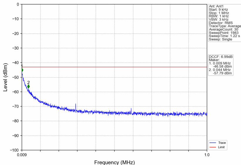
n41_30kHz_SISO_NTNV_50MHz_CP-OFDM QPSK_2664.99MHz_Edge_1RB_Right
