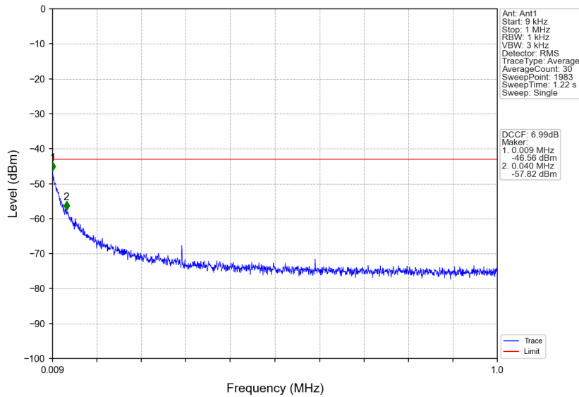
n41_30kHz_SISO_NTNV_50MHz_DFT-s-OFDM_QPSK_2664.99MHz_Edge_1RB_Right
