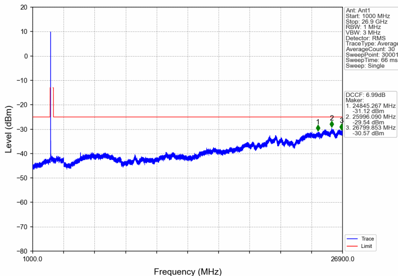
n41_30kHz_SISO_NTNV_40MHz_CP-OFDM QPSK_2516.01MHz_Outer_Full
