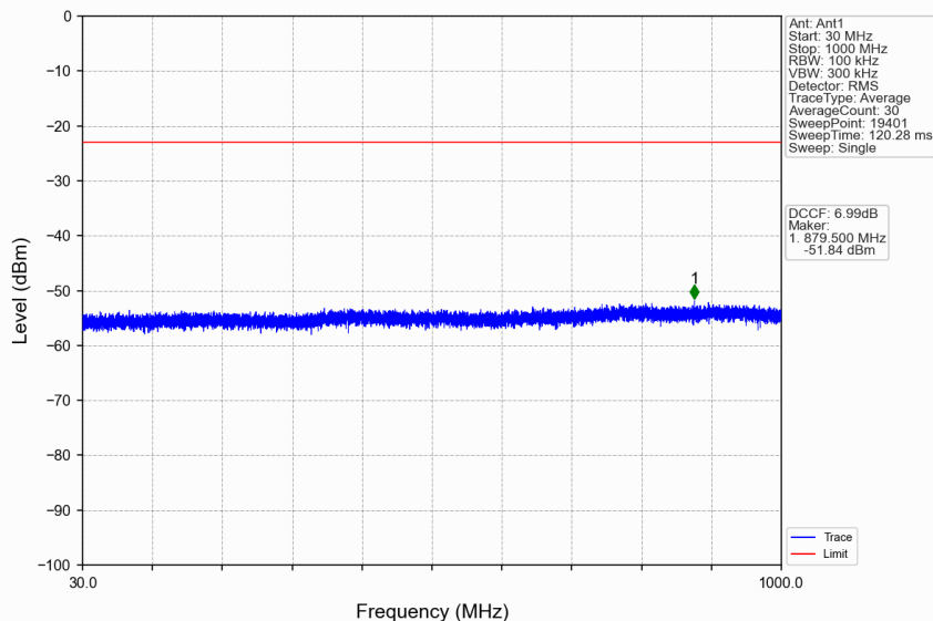
n41_30kHz_SISO_NTNV_40MHz_CP-OFDM QPSK_2670MHz_Edge_1RB_Right
