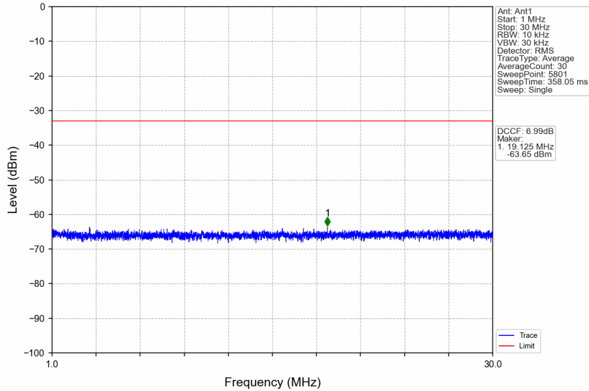
n41_30kHz_SISO_NTNV_50MHz_DFT-s-OFDM QPSK_2521.02MHz_Edge_1RB_Left
