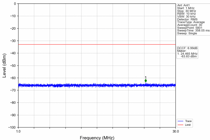
n41_30kHz_SISO_NTNV_30MHz_CP-OFDM QPSK_2511MHz_Edge_1RB_Left
