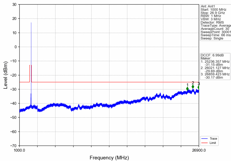
n41_30kHz_SISO_NTNV_40MHz_DFT-s-OFDM QPSK_2670MHz_Edge_1RB_Right
