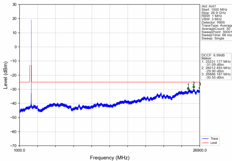
n41_30kHz_SISO_NTNV_30MHz_DFT-s-OFDM_QPSK_2674.98MHz_Edge_1RB_Right
