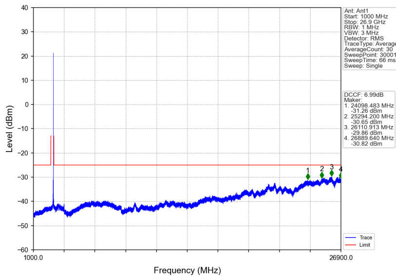
n41_30kHz_SISO_NTNV_30MHz_DFT-s-OFDM PI/2 BPSK_2674.98MHz_Edge_1RB_Right
