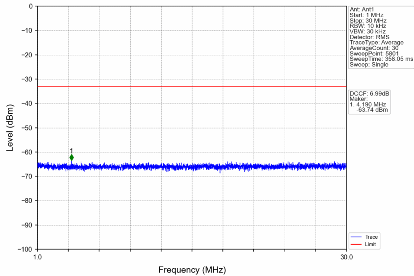
n41_30kHz_SISO_NTNV_30MHz_DFT-s-OFDM QPSK_2511MHz_Edge_1RB_Left
