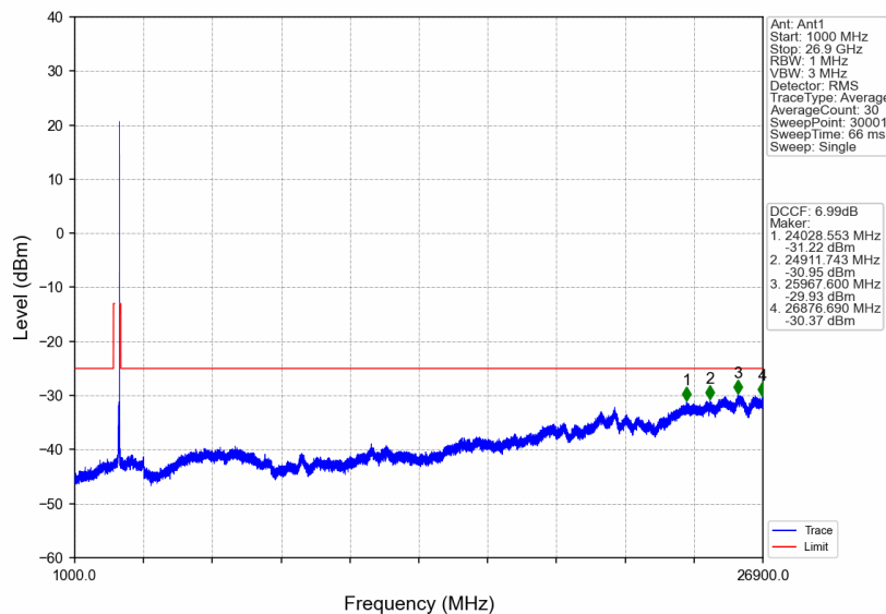
n41_30kHz_SISO_NTNV_40MHz_DFT-s-OFDM PI/2 BPSK_2670MHz_Edge_1RB_Right
