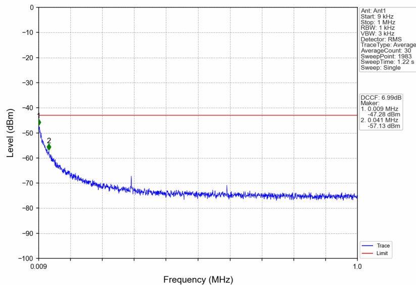
n41_30kHz_SISO_NTNV_30MHz_CP-OFDM QPSK_2674.98MHz_Edge_1RB_Right
