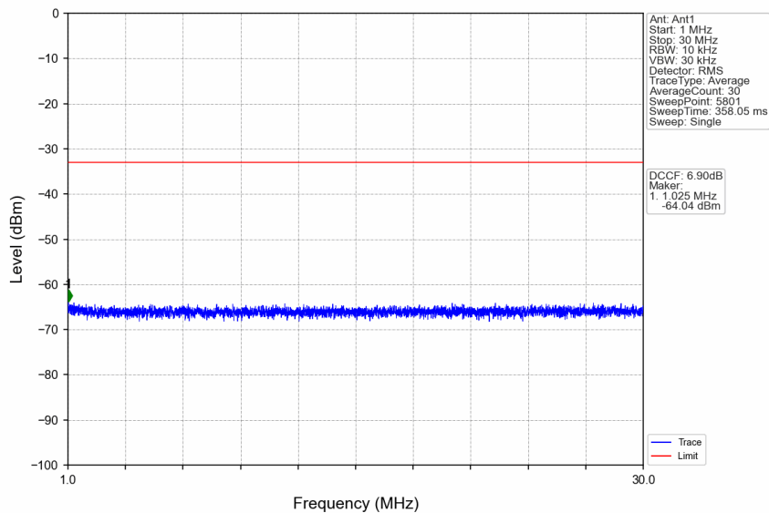
n41_30kHz_SISO_NTNV_40MHz_DFT-s-OFDM QPSK_2516.01MHz_Edge_1RB_Left
