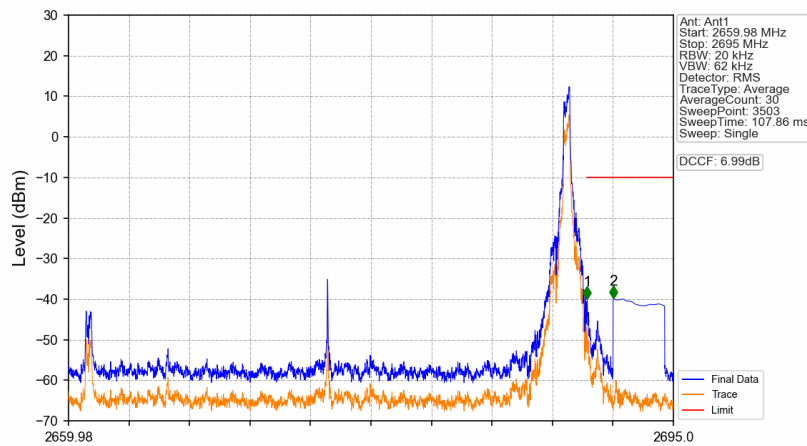
n41_30kHz_SISO_NTNV_30MHz_CP-OFDM QPSK_2674.98MHz_Edge_1RB_Right
