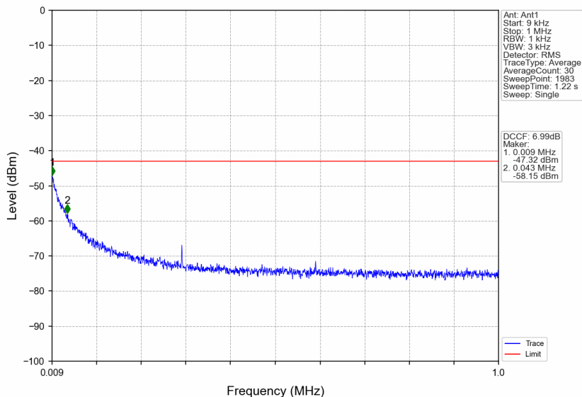
n41_30kHz_SISO_NTNV_30MHz_DFT-s-OFDM_QPSK_2674.98MHz_Edge_1RB_Right
