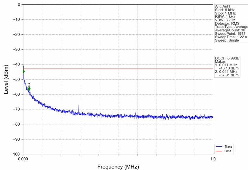
n41_30kHz_SISO_NTNV_25MHz_DFT-s-OFDM QPSK_2677.5MHz_Edge_1RB_Right
