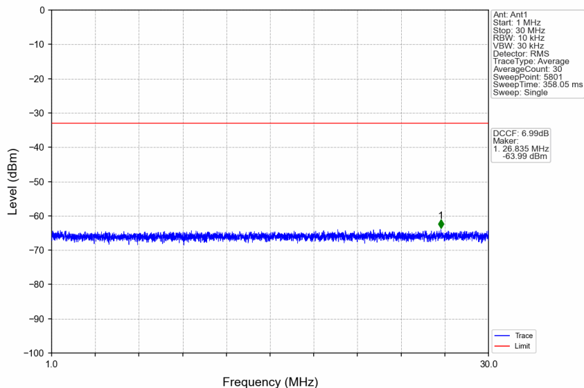
n41_30kHz_SISO_NTNV_25MHz_CP-OFDM QPSK_2592.99MHz_Edge_1RB_Left
