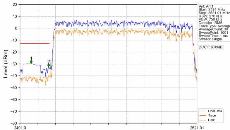
n41_30kHz_SISO_NTNV_25MHz_CP-OFDM QPSK_2508.51MHz_Outer_Full
