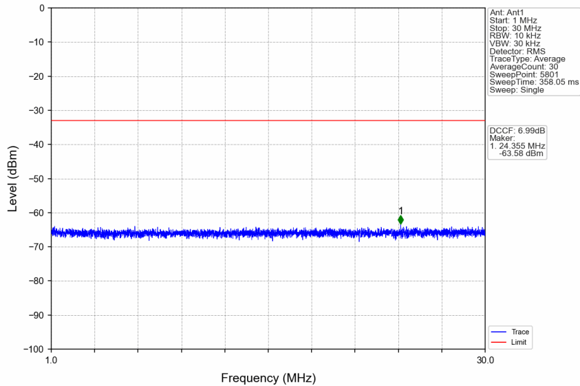
n41_30kHz_SISO_NTNV_20MHz_DFT-s-OFDM_QPSK_2679.99MHz_Edge_1RB_Right
