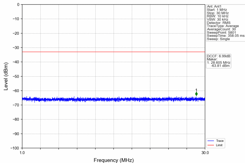
n41_30kHz_SISO_NTNV_25MHz_CP-OFDM QPSK_2677.5MHz_Edge_1RB_Right
