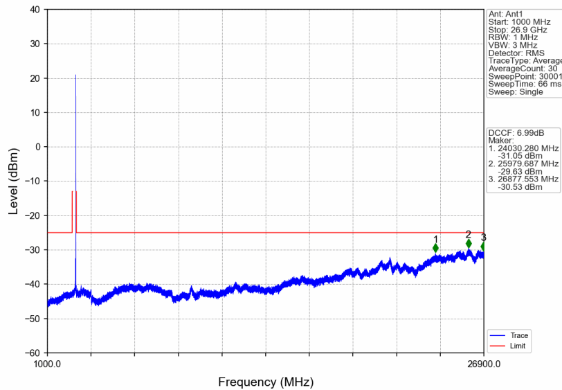
n41_30kHz_SISO_NTNV_25MHz_CP-OFDM QPSK_2677.5MHz_Edge_1RB_Right
