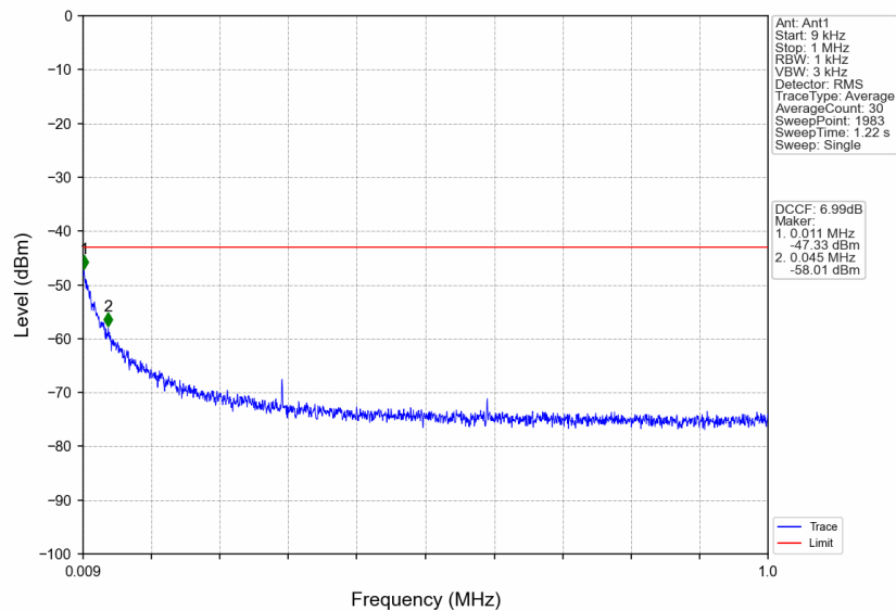
n41_30kHz_SISO_NTNV_20MHz_CP-OFDM QPSK_2679.99MHz_Edge_1RB_Right
