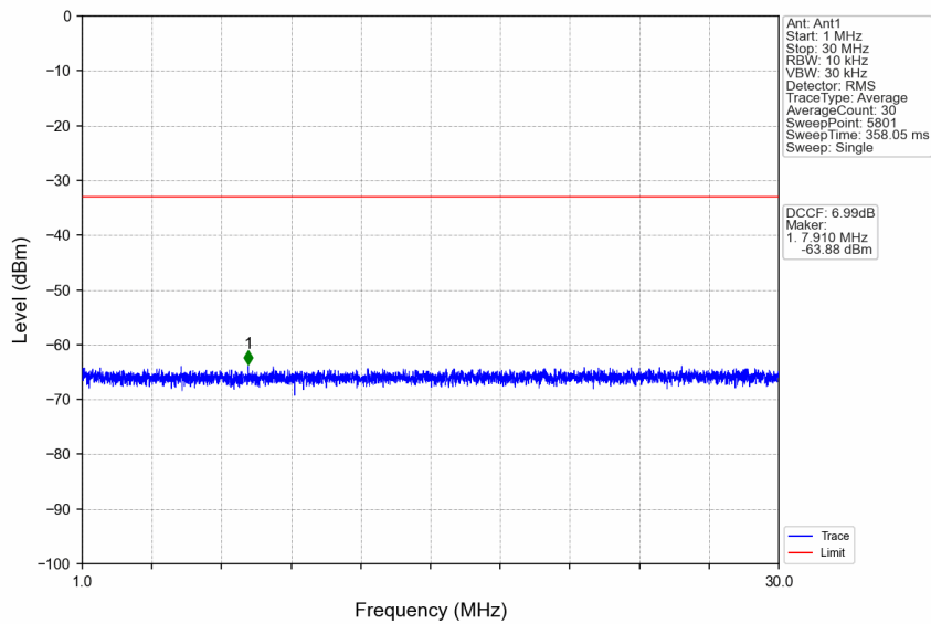
n41_30kHz_SISO_NTNV_25MHz_DFT-s-OFDM QPSK_2592.99MHz_Edge_1RB_Left
