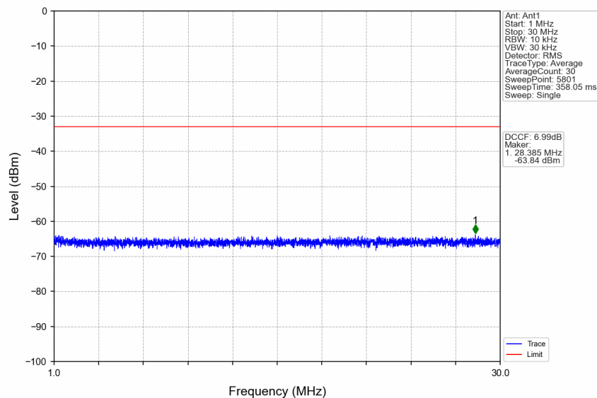
n41_30kHz_SISO_NTNV_25MHz_DFT-s-OFDM QPSK_2677.5MHz_Edge_1RB_Right
