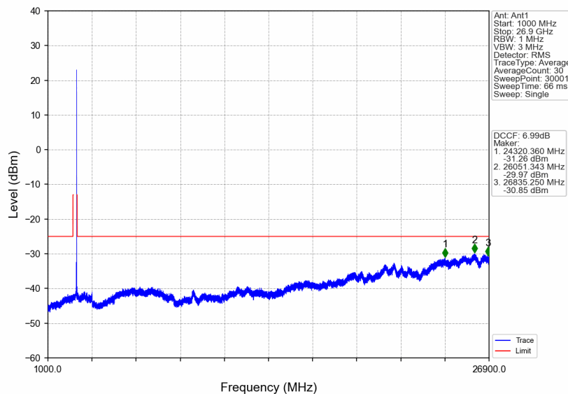
n41_30kHz_SISO_NTNV_25MHz_DFT-s-OFDM QPSK_2677.5MHz_Edge_1RB_Right
