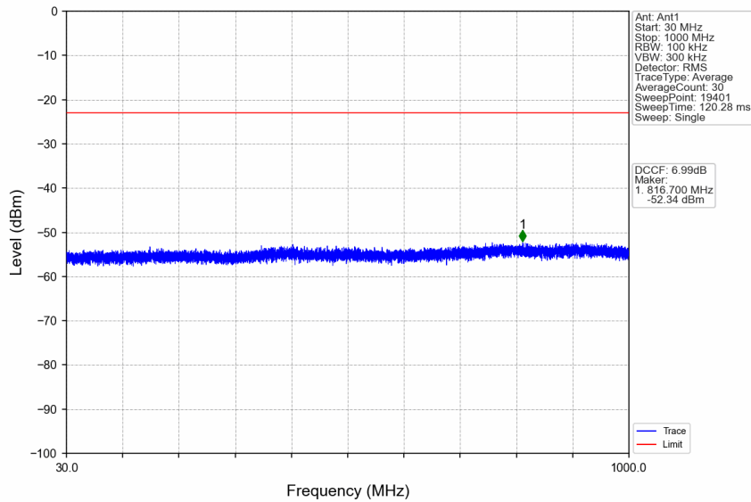
n41_30kHz_SISO_NTNV_20MHz_DFT-s-OFDM_QPSK_2679.99MHz_Edge_1RB_Right
