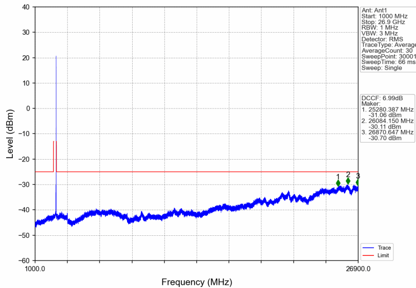
n41_30kHz_SISO_NTNV_20MHz_CP-OFDM QPSK_2679.99MHz_Edge_1RB_Right
