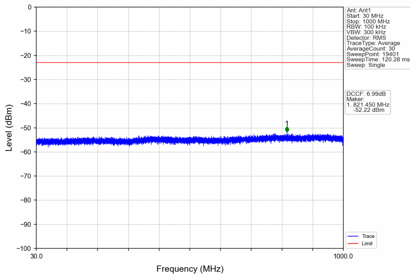
n41_30kHz_SISO_NTNV_25MHz_DFT-s-OFDM PI/2 BPSK_2677.5MHz_Edge_1RB_Right
