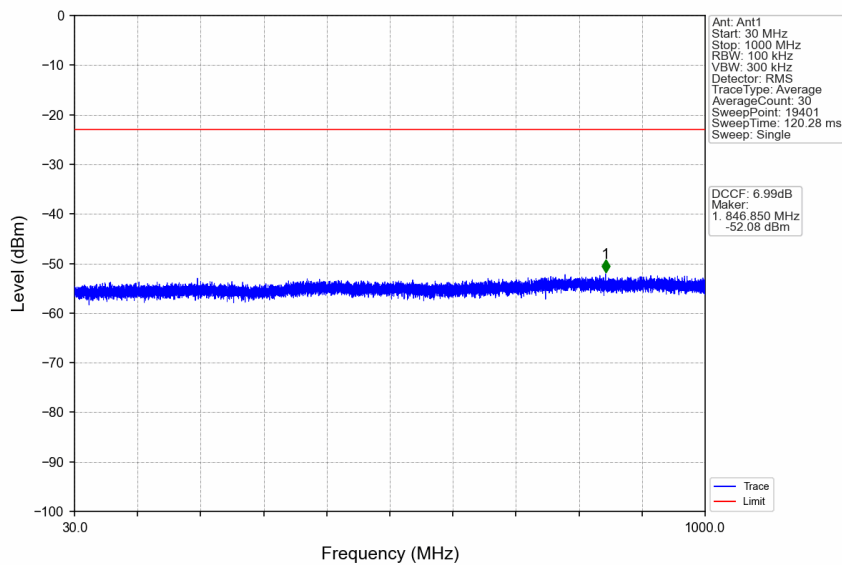
n41_30kHz_SISO_NTNV_25MHz_DFT-s-OFDM PI/2 BPSK_2592.99MHz_Edge_1RB_Left
