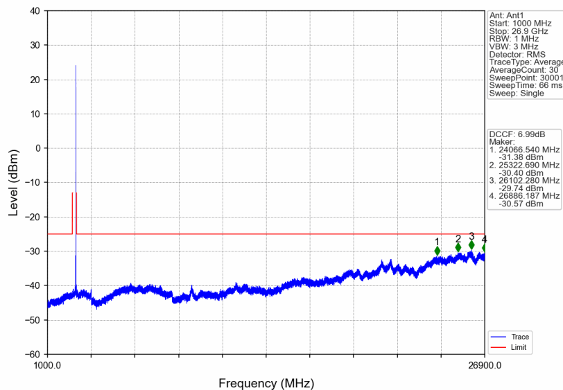
n41_30kHz_SISO_NTNV_25MHz_DFT-s-OFDM PI/2 BPSK_2677.5MHz_Edge_1RB_Right
