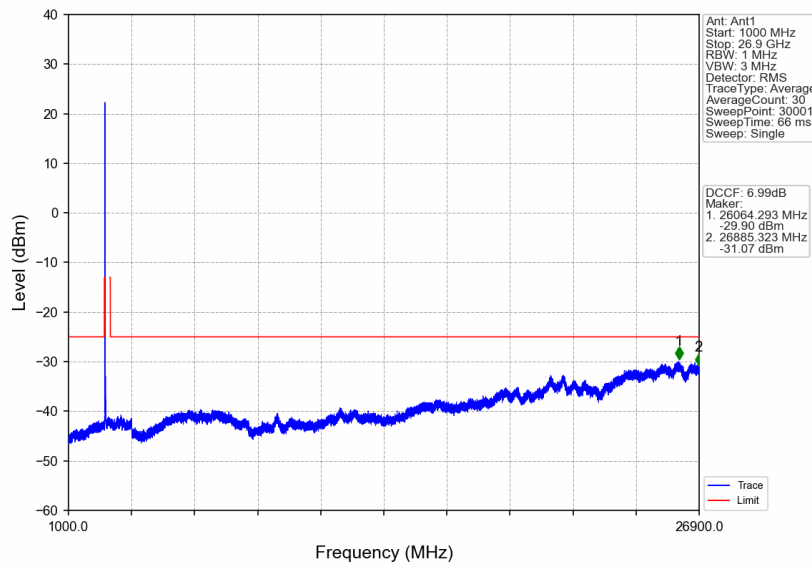
n41_30kHz_SISO_NTNV_25MHz_CP-OFDM QPSK_2508.51MHz_Outer_Full
