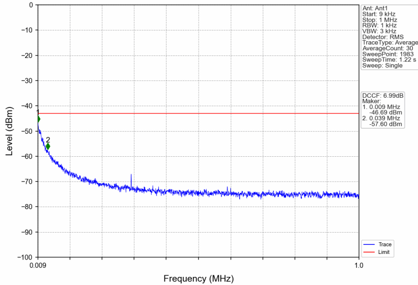
n41_30kHz_SISO_NTNV_20MHz_DFT-s-OFDM_QPSK_2679.99MHz_Edge_1RB_Right
