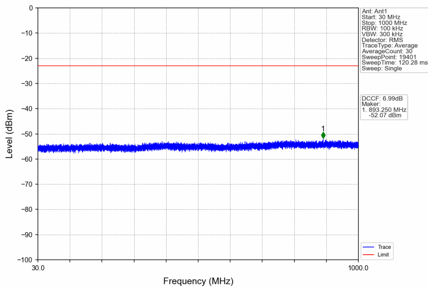
n41_30kHz_SISO_NTNV_20MHz_DFT-s-OFDM QPSK_2592.99MHz_Edge_1RB_Left
