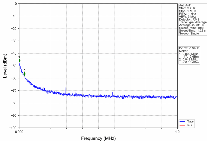
n41_30kHz_SISO_NTNV_25MHz_CP-OFDM QPSK_2677.5MHz_Edge_1RB_Right
