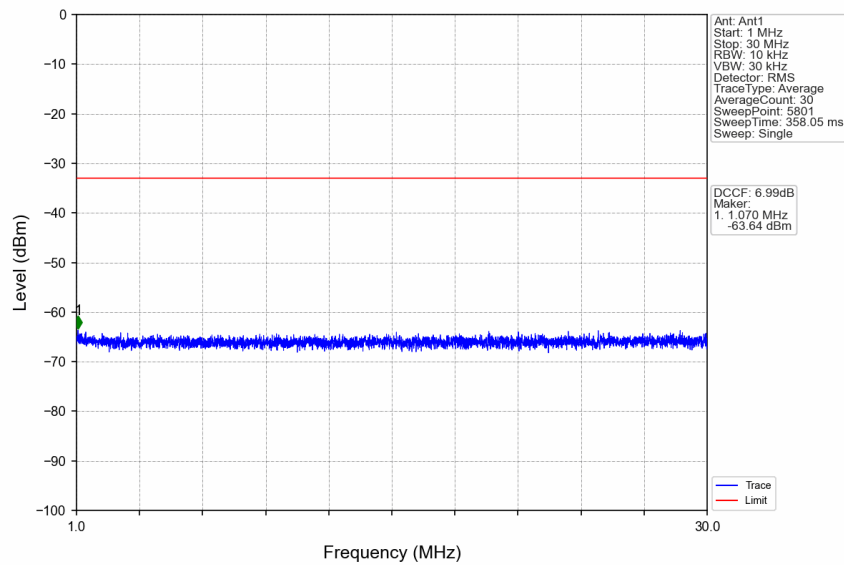
n41_30kHz_SISO_NTNV_15MHz_DFT-s-OFDM PI/2 BPSK_2592.99MHz_Edge_1RB_Left
