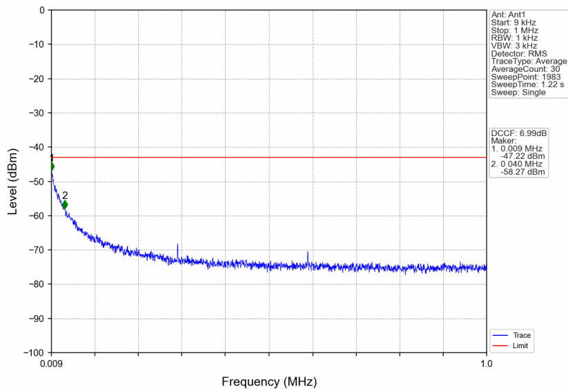
n41_30kHz_SISO_NTNV_15MHz_DFT-s-OFDM PI/2 BPSK_2682.48MHz_Edge_1RB_Right
