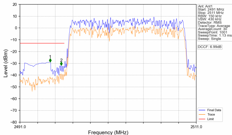
n41_30kHz_SISO_NTNV_15MHz_DFT-s-OFDM PI/2 BPSK_2503.5MHz_Outer_Full
