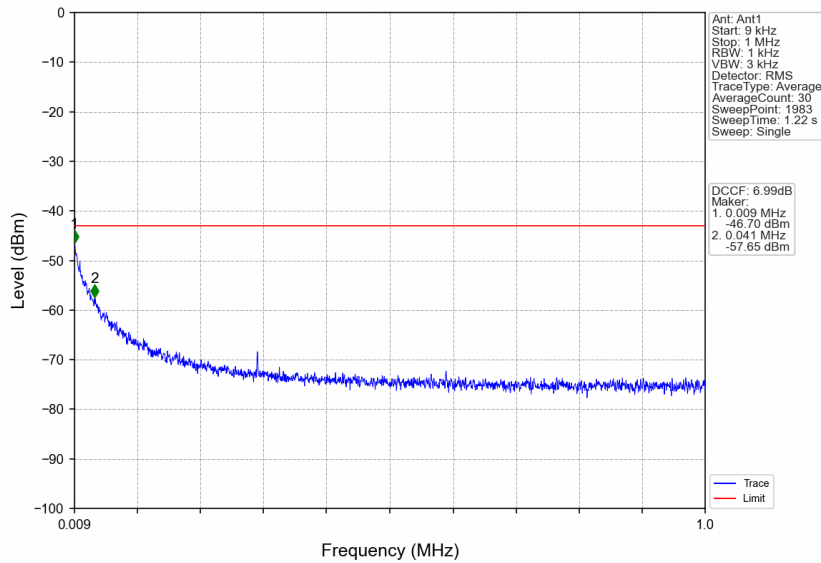
n41_15kHz_SISO_NTNV_50MHz_CP-OFDM QPSK_2664.99MHz_Edge_1RB_Right
