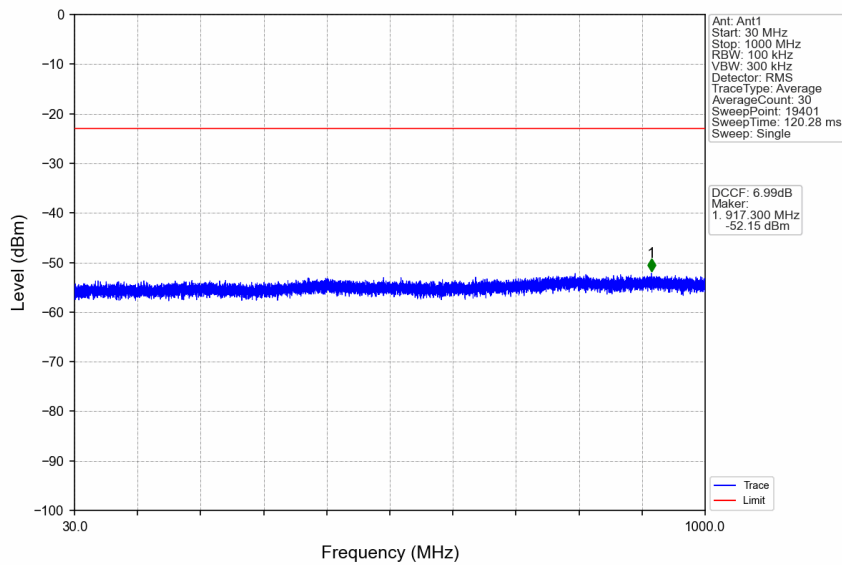
n41_15kHz_SISO_NTNV_50MHz_DFT-s-OFDM_QPSK_2664.99MHz_Edge_1RB_Right
