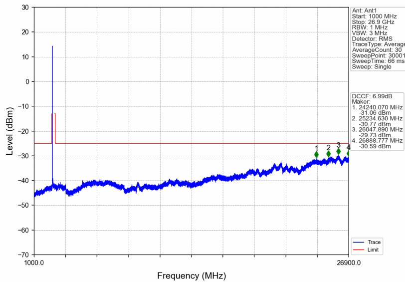
n41_15kHz_SISO_NTNV_50MHz_CP-OFDM QPSK_2521.005MHz_Outer_Full
