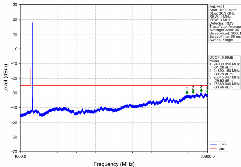
n41_15kHz_SISO_NTNV_50MHz_CP-OFDM QPSK_2664.99MHz_Edge_1RB_Right
