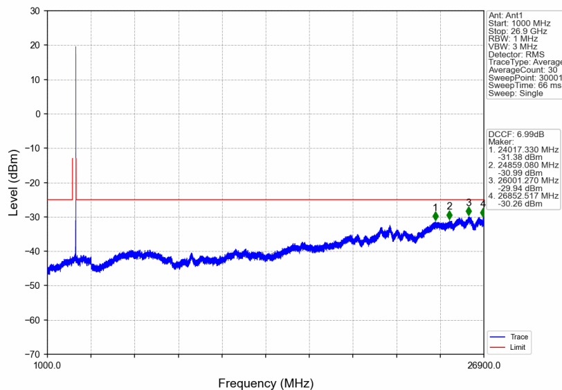
n41_30kHz_SISO_NTNV_10MHz_DFT-s-OFDM QPSK_2685MHz_Edge_1RB_Right
