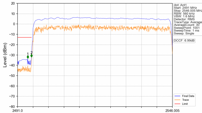
n41_15kHz_SISO_NTNV_50MHz_CP-OFDM QPSK_2521.005MHz_Outer_Full
