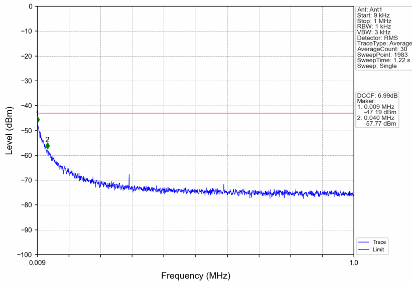
n41_15kHz_SISO_NTNV_50MHz_DFT-s-OFDM_QPSK_2664.99MHz_Edge_1RB_Right
