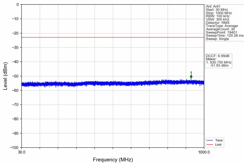
n41_30kHz_SISO_NTNV_10MHz_DFT-s-OFDM PI/2 BPSK_2592.99MHz_Edge_1RB_Left
