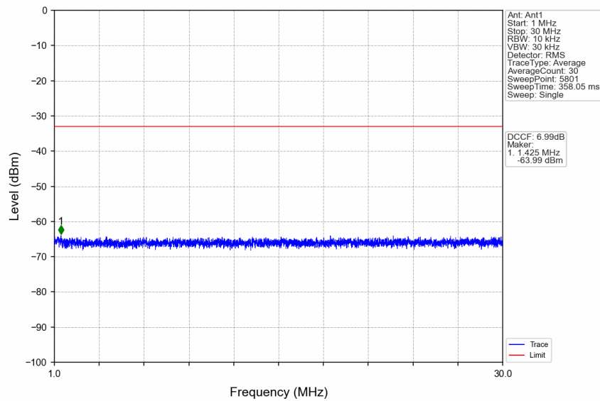
n41_30kHz_SISO_NTNV_10MHz_DFT-s-OFDM QPSK_2592.99MHz_Edge_1RB_Left
