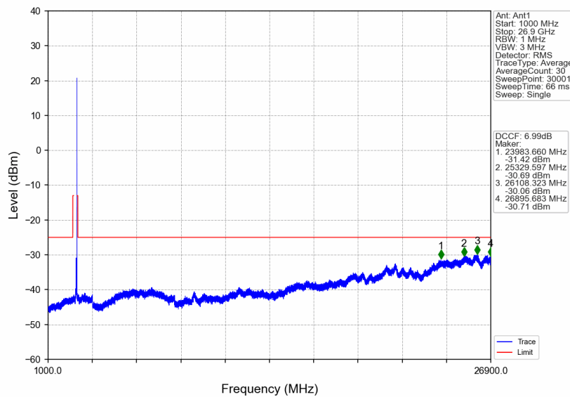
n41_15kHz_SISO_NTNV_50MHz_DFT-s-OFDM_QPSK_2664.99MHz_Edge_1RB_Right
