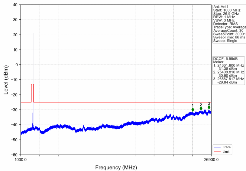
n41_15kHz_SISO_NTNV_50MHz_DFT-s-OFDM PI/2 BPSK_2664.99MHz_Edge_1RB_Right
