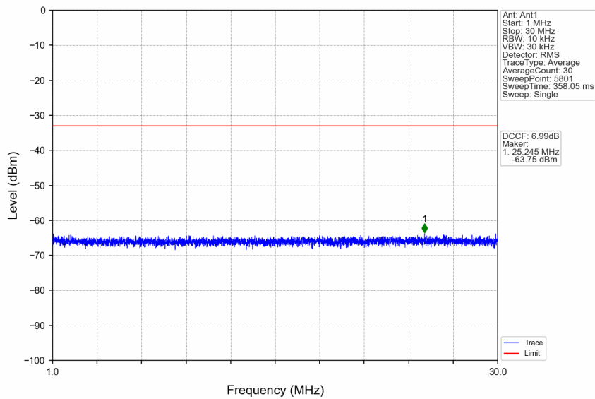
n41_30kHz_SISO_NTNV_10MHz_DFT-s-OFDM QPSK_2501.01MHz_Edge_1RB_Left
