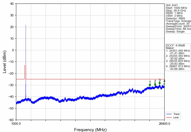
n41_30kHz_SISO_NTNV_10MHz_DFT-s-OFDM PI/2 BPSK_2685MHz_Edge_1RB_Right
