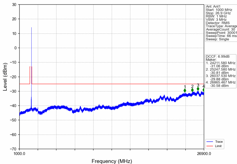
n41_15kHz_SISO_NTNV_40MHz_CP-OFDM QPSK_2670MHz_Edge_1RB_Right
