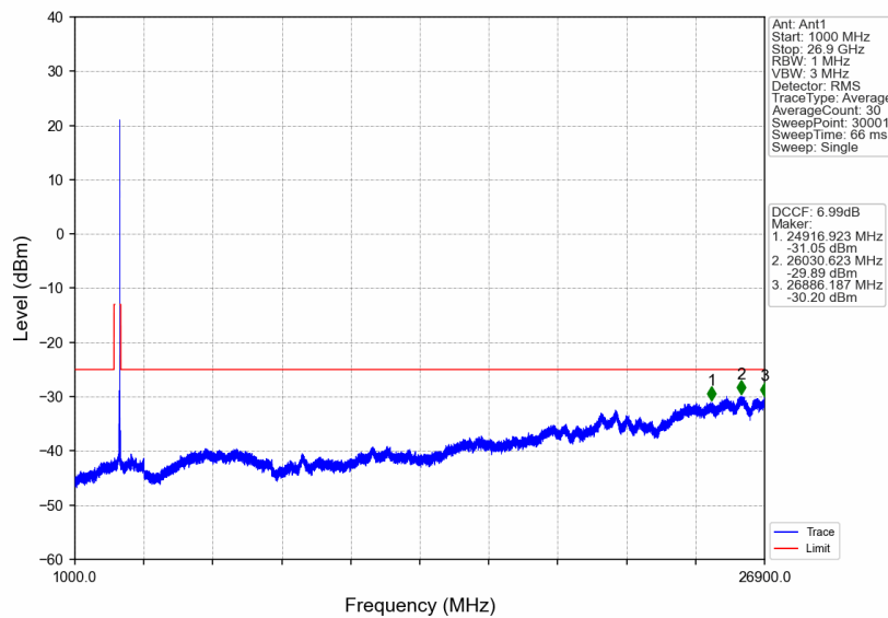
n41_15kHz_SISO_NTNV_30MHz_DFT-s-OFDM_PI/2_BPSK_2674.995MHz_Edge_1RB_Right
