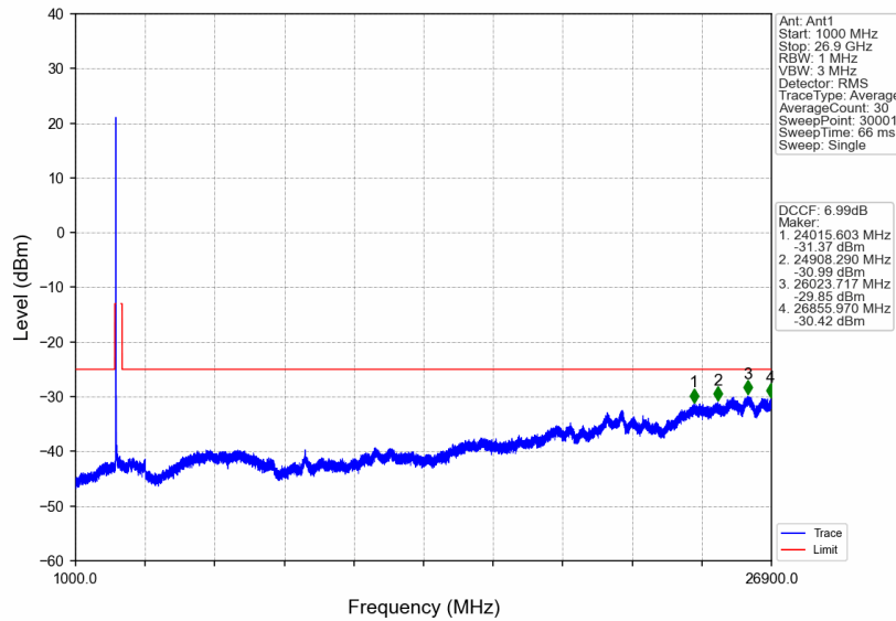
n41_15kHz_SISO_NTNV_40MHz_CP-OFDM QPSK_2516.01MHz_Outer_Full
