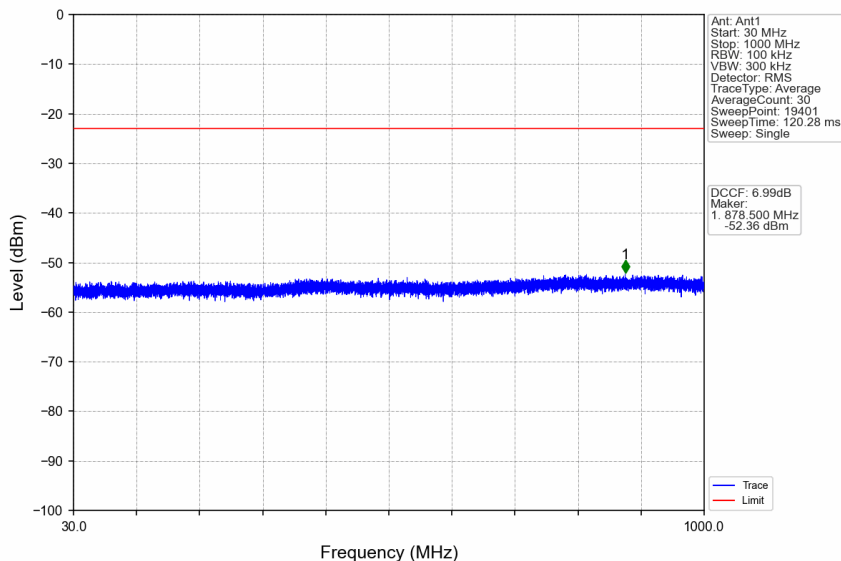
n41_15kHz_SISO_NTNV_30MHz_CP-OFDM QPSK_2674.995MHz_Edge_1RB_Right
