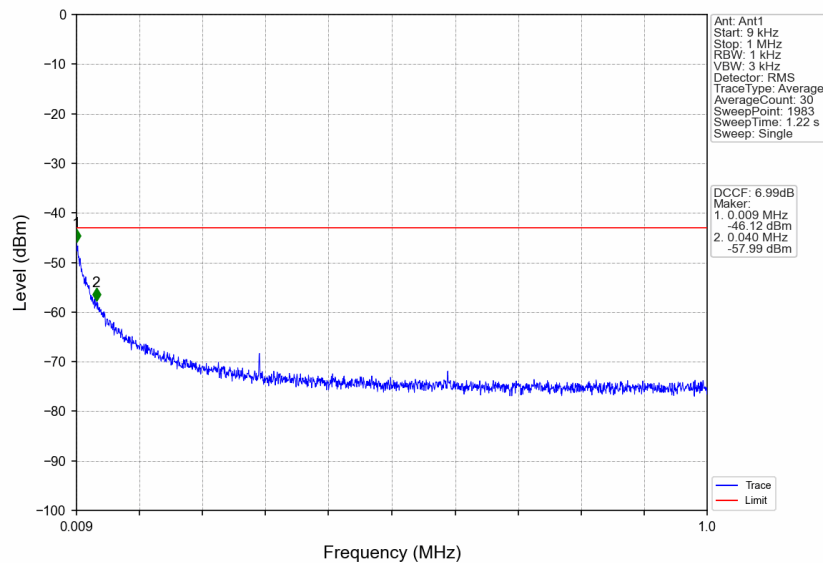
n41_15kHz_SISO_NTNV_40MHz_DFT-s-OFDM QPSK_2670MHz_Edge_1RB_Right
