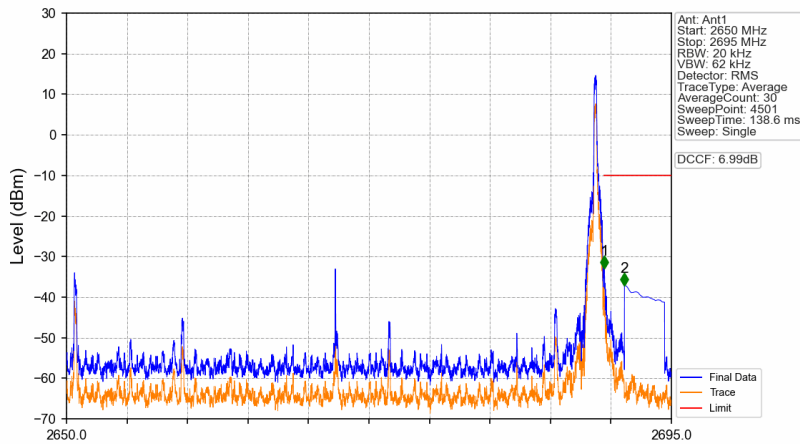
n41_15kHz_SISO_NTNV_40MHz_DFT-s-OFDM QPSK_2670MHz_Edge_1RB_Right
