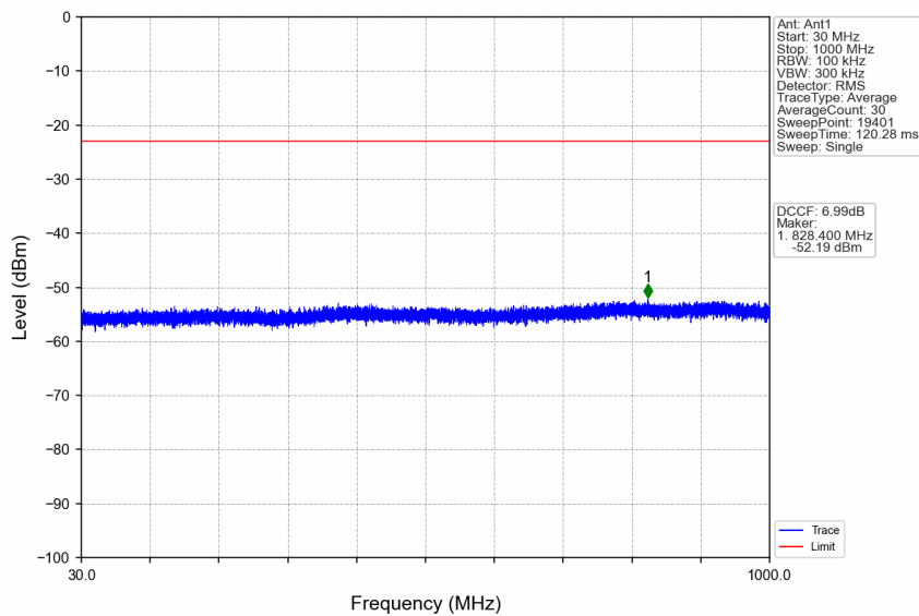
n41_15kHz_SISO_NTNV_40MHz_DFT-s-OFDM QPSK_2516.01MHz_Edge_1RB_Left
