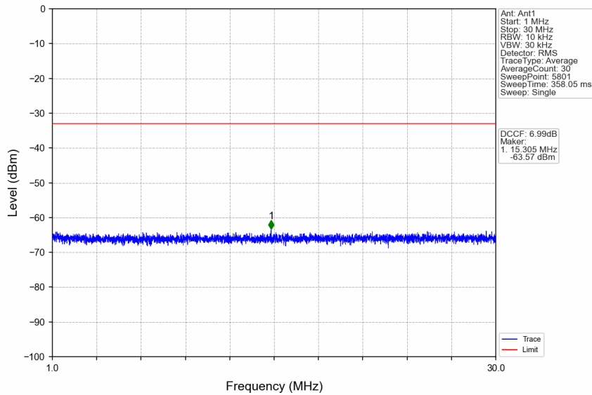
n41_15kHz_SISO_NTNV_30MHz_DFT-s-OFDM_QPSK_2593.005MHz_Edge_1RB_Left
