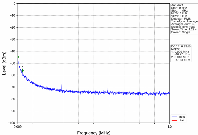
n41_15kHz_SISO_NTNV_40MHz_CP-OFDM QPSK_2670MHz_Edge_1RB_Right
