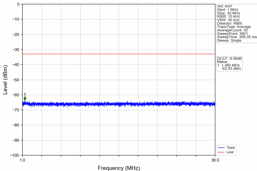
n41_15kHz_SISO_NTNV_40MHz_CP-OFDM QPSK_2670MHz_Edge_1RB_Right
