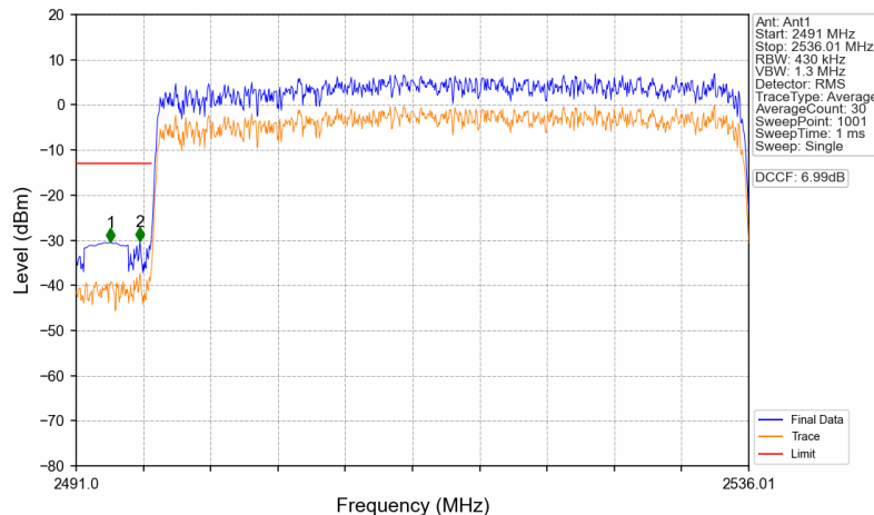
n41_15kHz_SISO_NTNV_40MHz_CP-OFDM QPSK_2516.01MHz_Outer_Full
