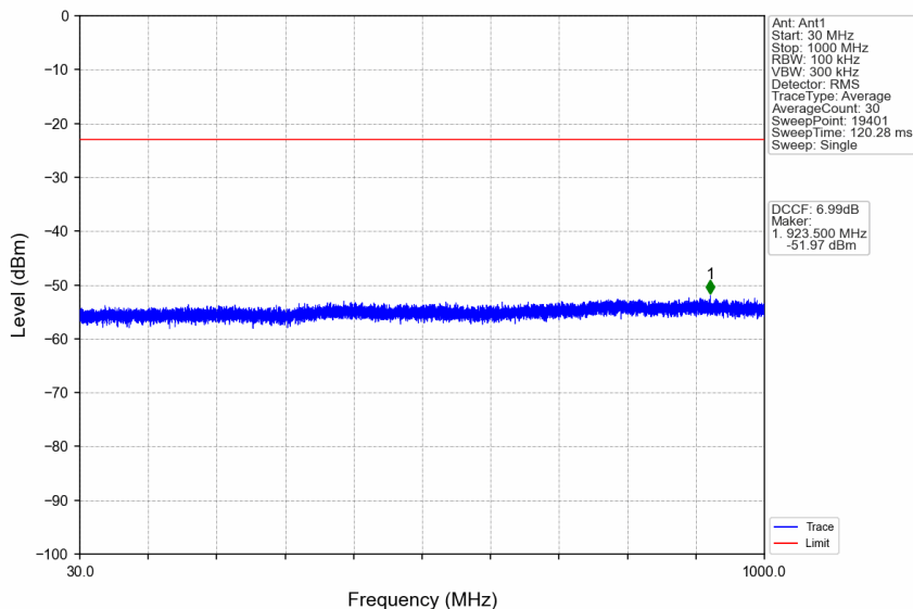
n41_15kHz_SISO_NTNV_30MHz_DFT-s-OFDM QPSK_2674.995MHz_Edge_1RB_Right
