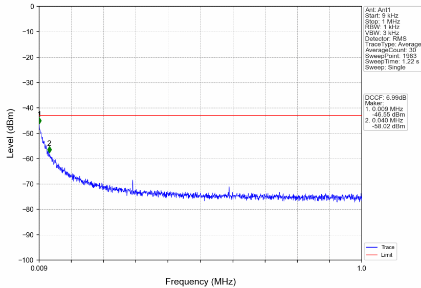
n41_15kHz_SISO_NTNV_30MHz_CP-OFDM QPSK_2674.995MHz_Edge_1RB_Right
