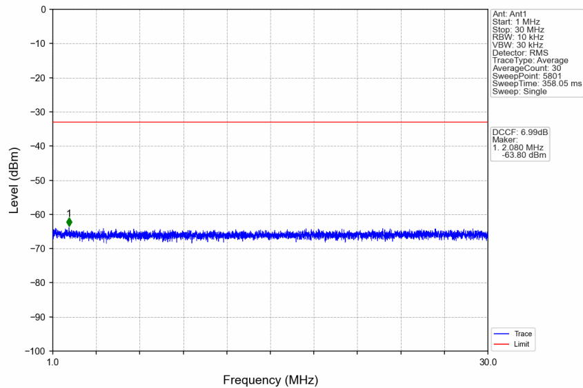
n41_15kHz_SISO_NTNV_30MHz_CP-OFDM QPSK_2674.995MHz_Edge_1RB_Right
