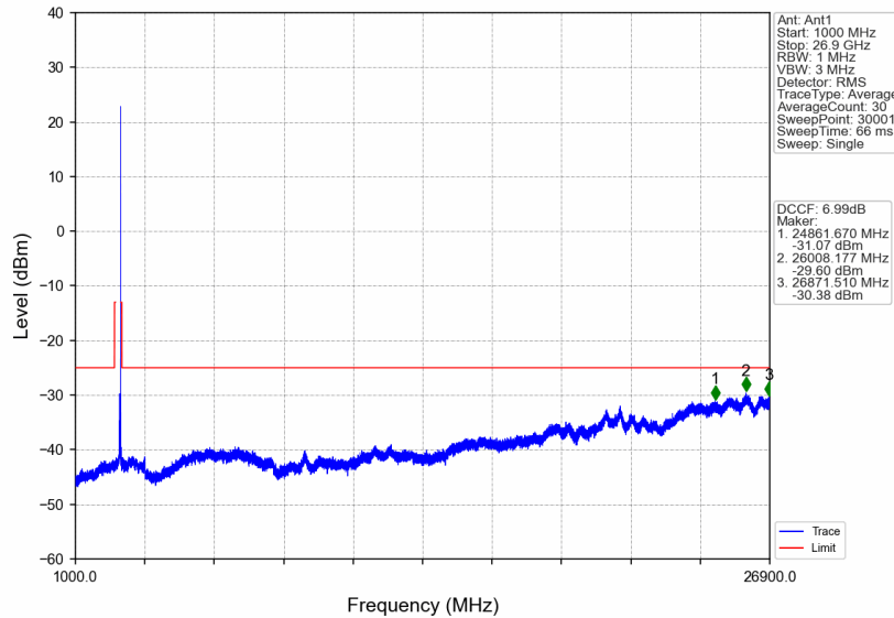
n41_15kHz_SISO_NTNV_40MHz_DFT-s-OFDM PI/2 BPSK_2670MHz_Edge_1RB_Right
