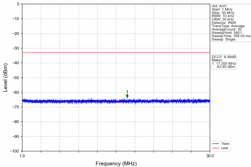
n41_15kHz_SISO_NTNV_30MHz_DFT-s-OFDM QPSK_2674.995MHz_Edge_1RB_Right
