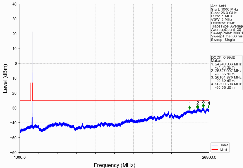
n41_15kHz_SISO_NTNV_30MHz_DFT-s-OFDM QPSK_2674.995MHz_Edge_1RB_Right
