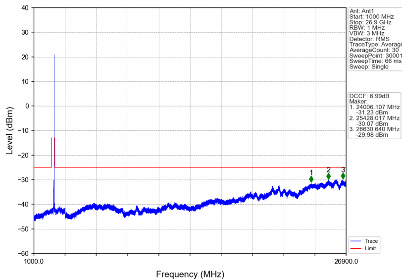
n41_15kHz_SISO_NTNV_40MHz_DFT-s-OFDM QPSK_2670MHz_Edge_1RB_Right
