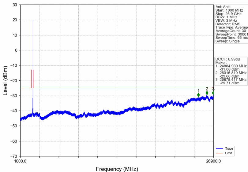
n41_15kHz_SISO_NTNV_30MHz_CP-OFDM QPSK_2674.995MHz_Edge_1RB_Right
