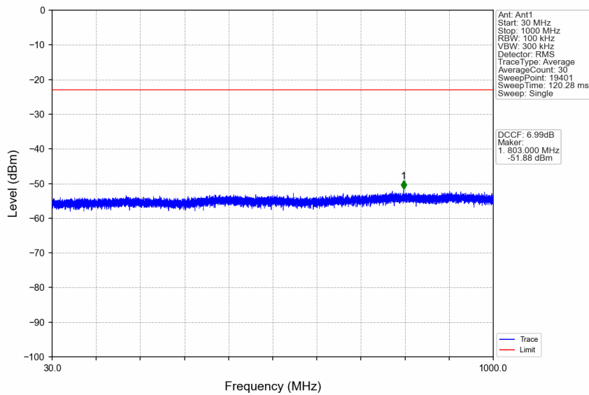
n41_15kHz_SISO_NTNV_30MHz_DFT-s-OFDM_PI/2_BPSK_2674.995MHz_Edge_1RB_Right
