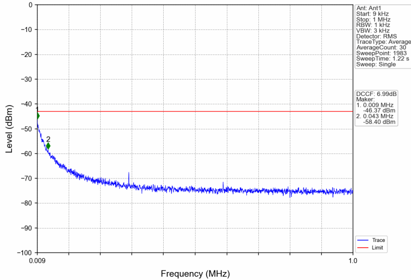
n41_15kHz_SISO_NTNV_30MHz_DFT-s-OFDM QPSK_2674.995MHz_Edge_1RB_Right
