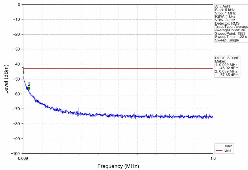
n41_15kHz_SISO_NTNV_25MHz_CP-OFDM QPSK_2677.5MHz_Edge_1RB_Right
