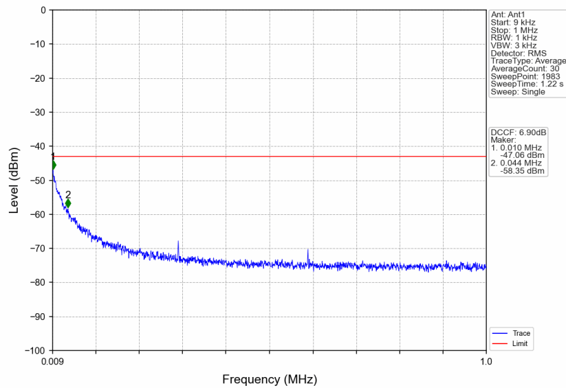
n41_15kHz_SISO_NTNV_20MHz_DFT-s-OFDM_QPSK_2679.99MHz_Edge_1RB_Right
