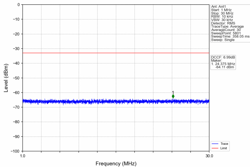
n41_15kHz_SISO_NTNV_25MHz_CP-OFDM QPSK_2677.5MHz_Edge_1RB_Right
