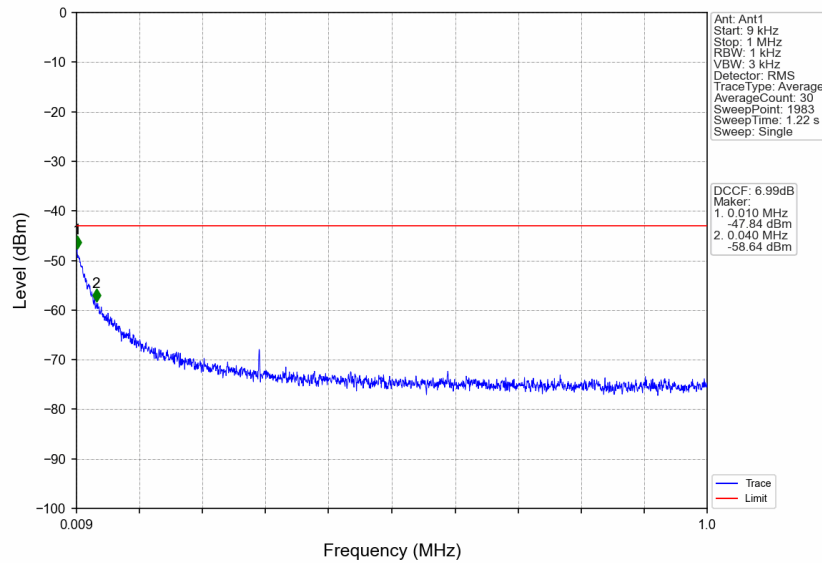
n41_15kHz_SISO_NTNV_20MHz_CP-OFDM QPSK_2679.99MHz_Edge_1RB_Right
