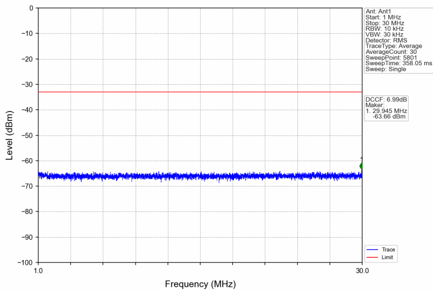
n41_15kHz_SISO_NTNV_25MHz_DFT-s-OFDM QPSK_2677.5MHz_Edge_1RB_Right
