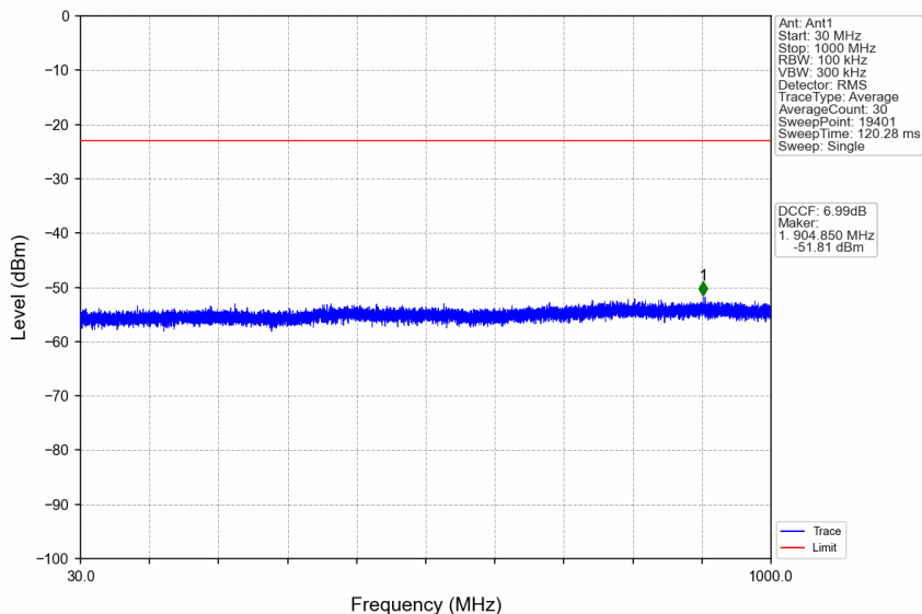
n41_15kHz_SISO_NTNV_25MHz_CP-OFDM QPSK_2677.5MHz_Edge_1RB_Right
