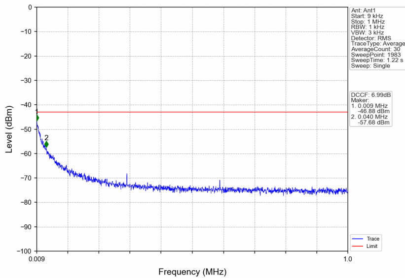
n41_15kHz_SISO_NTNV_25MHz_DFT-s-OFDM QPSK_2677.5MHz_Edge_1RB_Right
