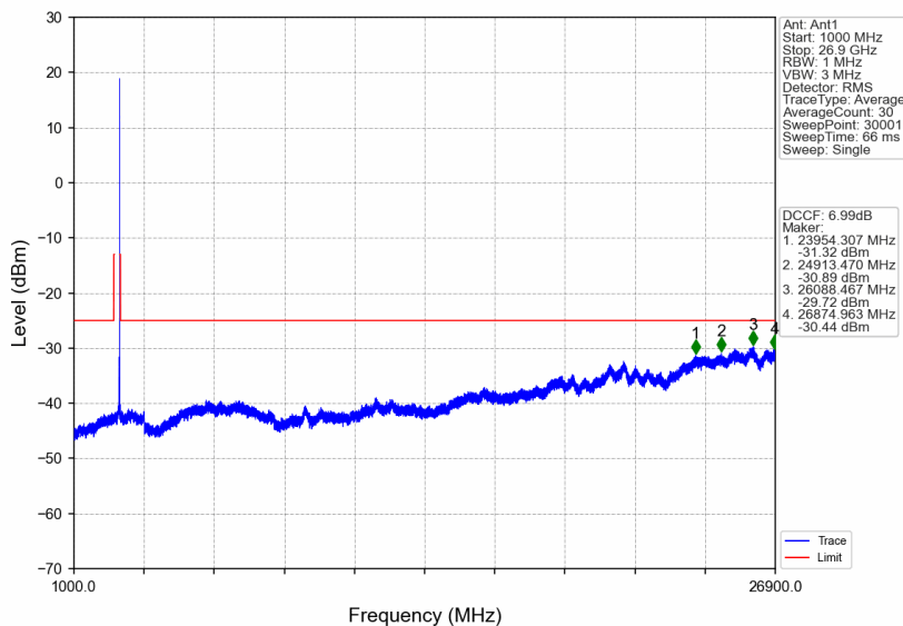
n41_15kHz_SISO_NTNV_25MHz_CP-OFDM QPSK_2677.5MHz_Edge_1RB_Right
