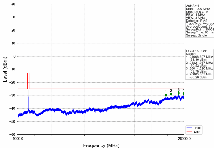
n41_15kHz_SISO_NTNV_25MHz_DFT-s-OFDM QPSK_2677.5MHz_Edge_1RB_Right
