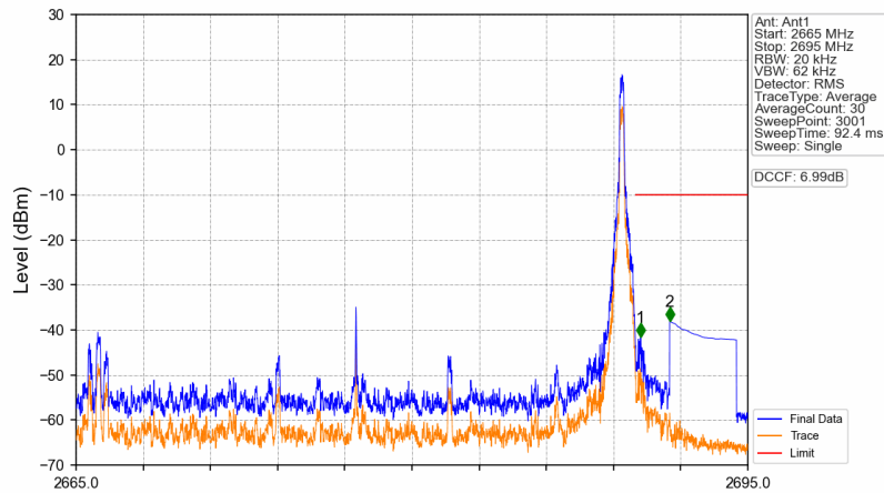
n41_15kHz_SISO_NTNV_25MHz_DFT-s-OFDM QPSK_2677.5MHz_Edge_1RB_Right
