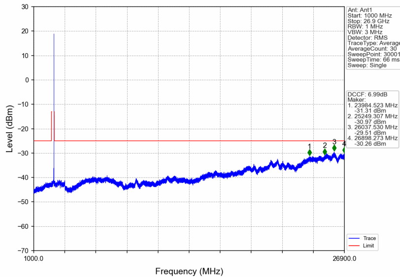
n41_15kHz_SISO_NTNV_20MHz_CP-OFDM QPSK_2679.99MHz_Edge_1RB_Right
