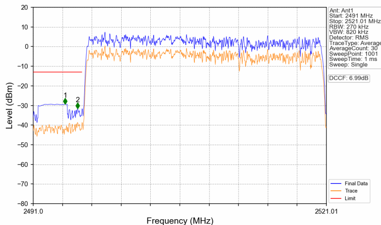
n41_15kHz_SISO_NTNV_25MHz_CP-OFDM QPSK_2508.51MHz_Outer_Full
