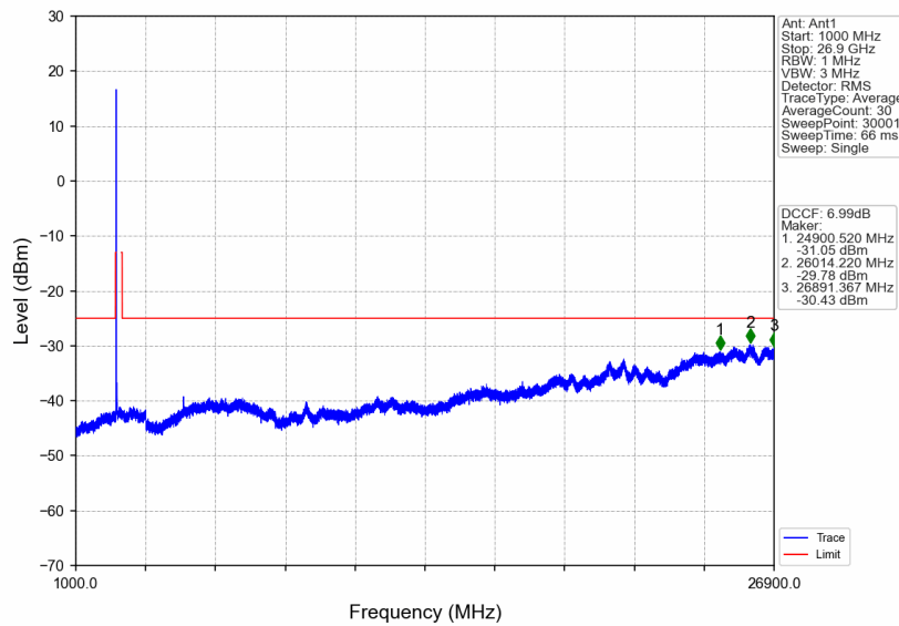
n41_15kHz_SISO_NTNV_25MHz_CP-OFDM QPSK_2508.51MHz_Outer_Full
