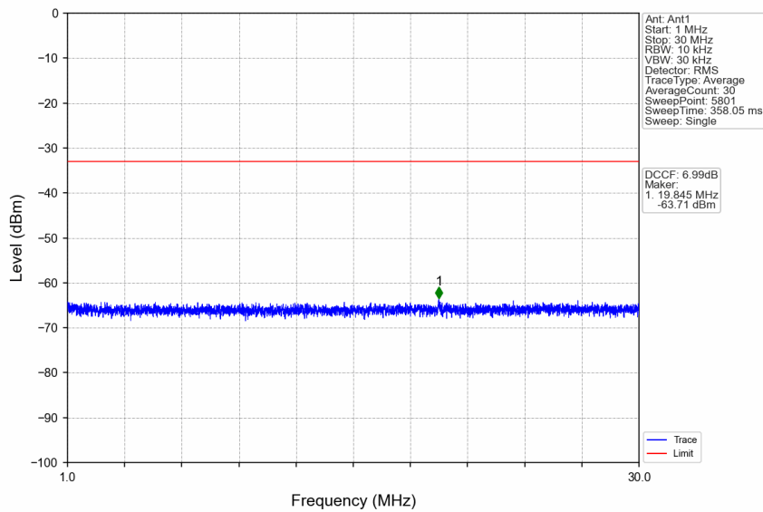
n41_15kHz_SISO_NTNV_25MHz_DFT-s-OFDM QPSK_2593.005MHz_Edge_1RB_Left
