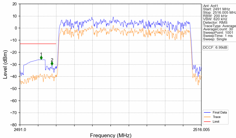
n41_15kHz_SISO_NTNV_20MHz_DFT-s-OFDM QPSK_2506.005MHz_Outer_Full
