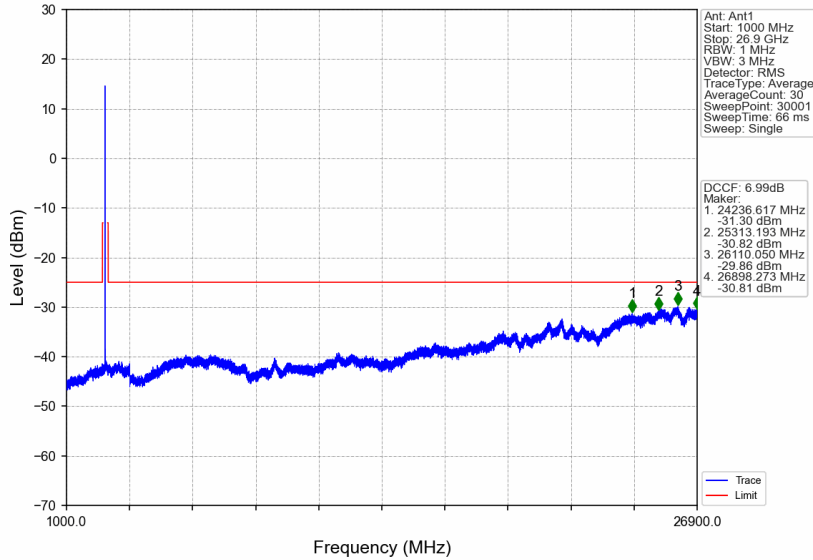
n41_15kHz_SISO_NTNV_20MHz_DFT-s-OFDM QPSK_2679.99MHz_Edge_1RB_Right
