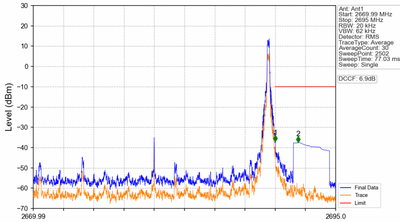
n41_15kHz_SISO_NTNV_20MHz_DFT-s-OFDM QPSK_2679.99MHz_Edge_1RB_Right
