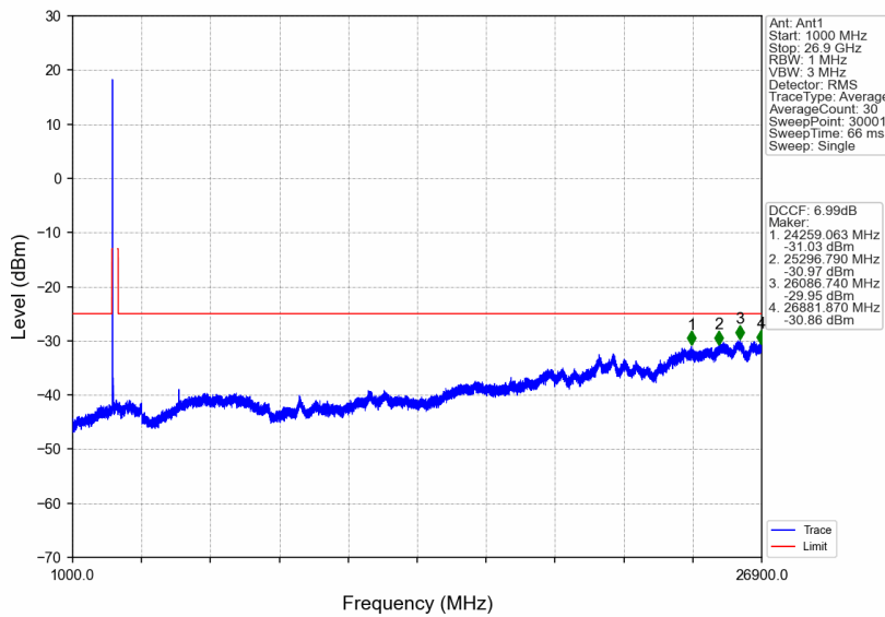
n41_15kHz_SISO_NTNV_20MHz_DFT-s-OFDM QPSK_2506.005MHz_Outer_Full
