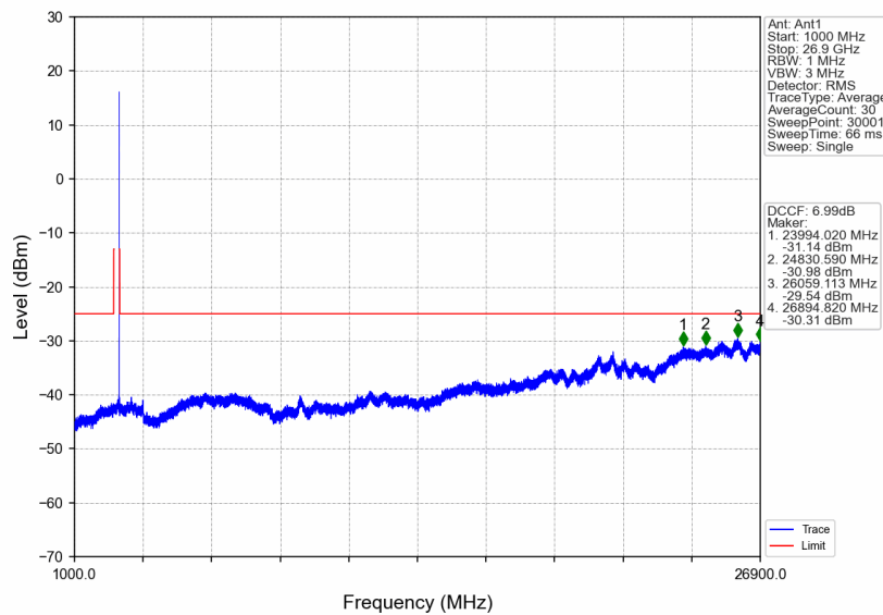
n41_15kHz_SISO_NTNV_15MHz_CP-OFDM QPSK_2682.495MHz_Edge_1RB_Right
