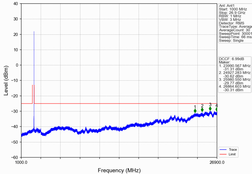
n41_15kHz_SISO_NTNV_20MHz_DFT-s-OFDM PI/2 BPSK_2679.99MHz_Edge_1RB_Right
