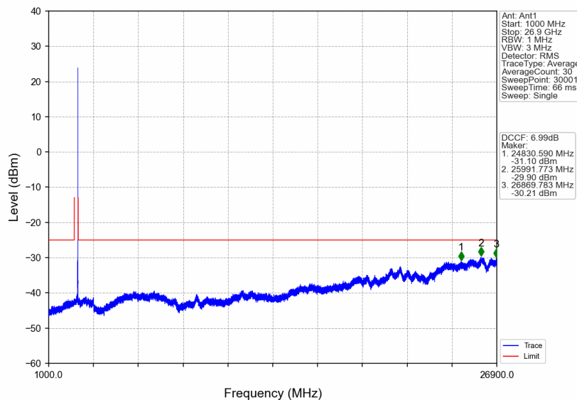
n41_15kHz_SISO_NTNV_15MHz_DFT-s-OFDM QPSK_2682.495MHz_Edge_1RB_Right
