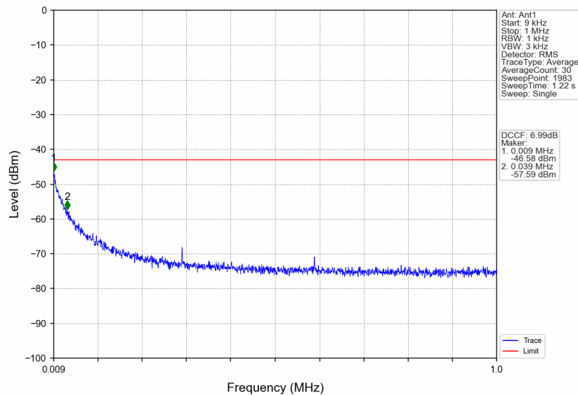
n41_15kHz_SISO_NTNV_15MHz_CP-OFDM QPSK_2682.495MHz_Edge_1RB_Right
