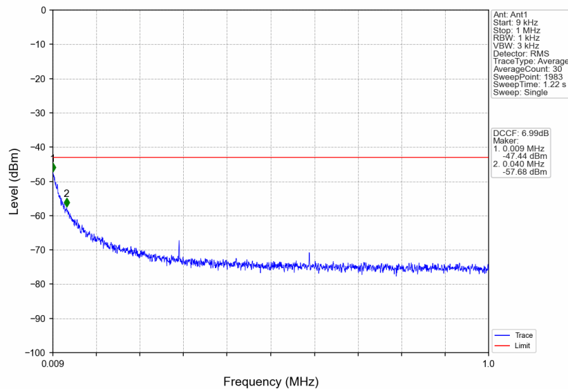
n41_15kHz_SISO_NTNV_15MHz_DFT-s-OFDM QPSK_2682.495MHz_Edge_1RB_Right
