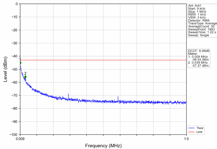
n41_15kHz_SISO_NTNV_15MHz_DFT-s-OFDM PI/2 BPSK_2682.495MHz_Edge_1RB_Right
