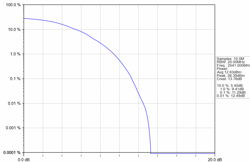
n41_30kHz_SISO_NTNV_90MHz_DFT-s-OFDM 64 QAM_2541MHz_Outer_Full
