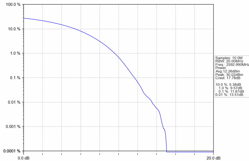
n41_30kHz_SISO_NTNV_80MHz_CP-OFDM 64 QAM_2592.99MHz_Outer_Full
