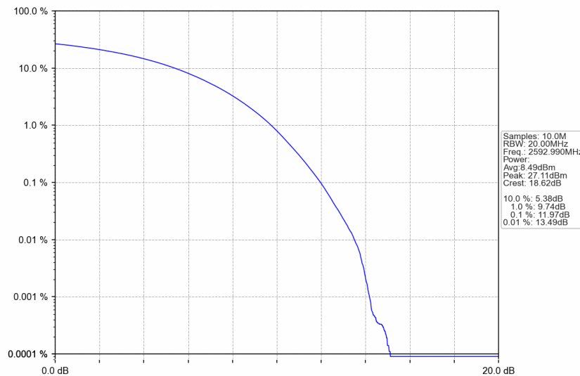
n41_30kHz_SISO_NTNV_90MHz_CP-OFDM 256 QAM_2592.99MHz_Outer_Full
