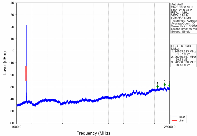
n41_15kHz_SISO_NTNV_10MHz_DFT-s-OFDM_QPSK_2685MHz_Edge_1RB_Right
