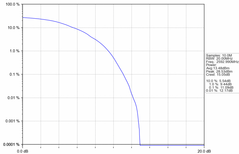
n41_30kHz_SISO_NTNV_90MHz_DFT-s-OFDM QPSK_2592.99MHz_Outer_Full
