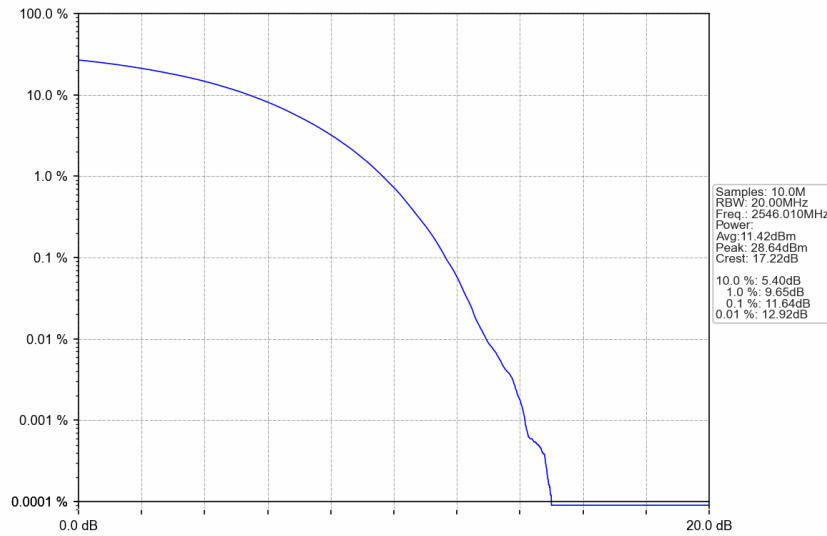
n41_30kHz_SISO_NTNV_100MHz_CP-OFDM 64 QAM_2546.01MHz_Outer_Full
