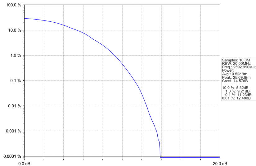
n41_30kHz_SISO_NTNV_90MHz_DFT-s-OFDM 256 QAM_2592.99MHz_Outer_Full
