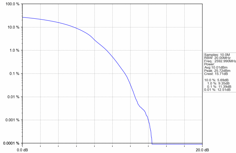
n41_30kHz_SISO_NTNV_100MHz_DFT-s-OFDM 256 QAM_2592.99MHz_Outer_Full
