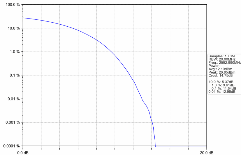
n41_30kHz_SISO_NTNV_90MHz_CP-OFDM 16 QAM_2592.99MHz_Outer_Full
