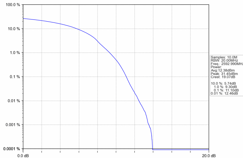
n41_30kHz_SISO_NTNV_100MHz_DFT-s-OFDM 16 QAM_2592.99MHz_Outer_Full
