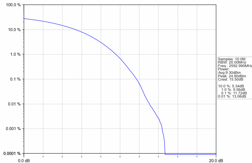
n41_30kHz_SISO_NTNV_80MHz_CP-OFDM 256 QAM_2592.99MHz_Outer_Full
