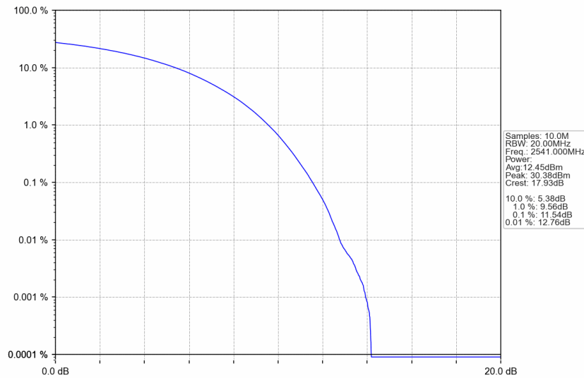
n41_30kHz_SISO_NTNV_90MHz_CP-OFDM 16 QAM_2541MHz_Outer_Full
