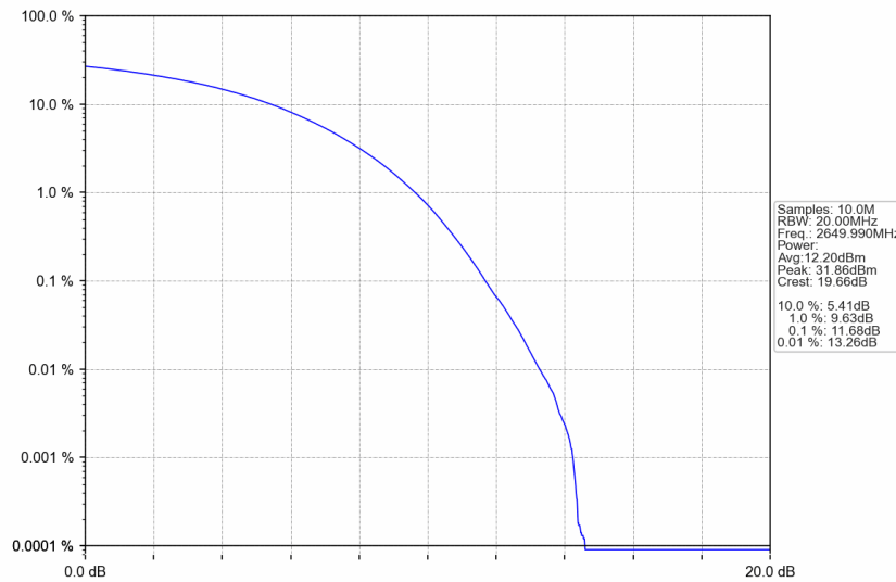
n41_30kHz_SISO_NTNV_80MHz_CP-OFDM 16 QAM_2649.99MHz_Outer_Full
