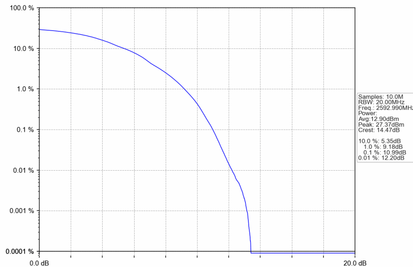
n41_30kHz_SISO_NTNV_90MHz_DFT-s-OFDM 16 QAM_2592.99MHz_Outer_Full
