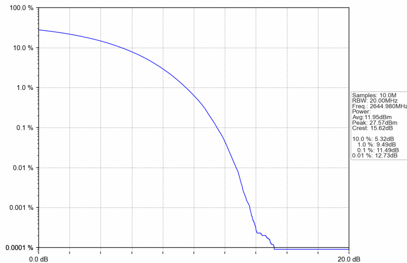
n41_30kHz_SISO_NTNV_90MHz_CP-OFDM QPSK_2644.98MHz_Outer_Full
