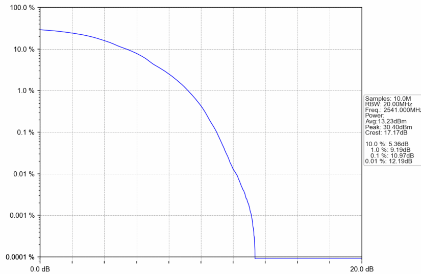
n41_30kHz_SISO_NTNV_90MHz_DFT-s-OFDM 16 QAM_2541MHz_Outer_Full
