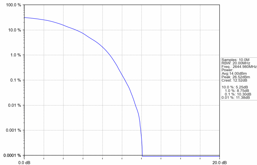
n41_30kHz_SISO_NTNV_90MHz_DFT-s-OFDM QPSK_2644.98MHz_Outer_Full
