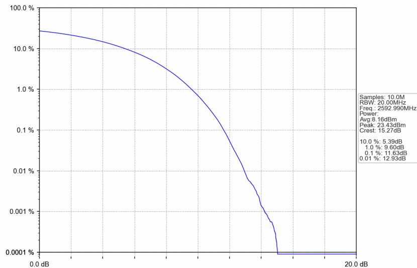
n41_30kHz_SISO_NTNV_100MHz_CP-OFDM 256 QAM_2592.99MHz_Outer_Full
