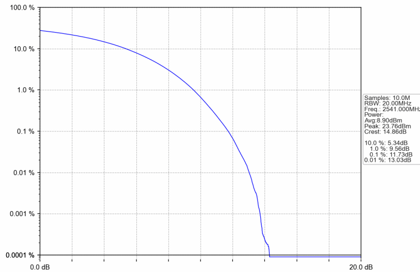
n41_30kHz_SISO_NTNV_90MHz_CP-OFDM 256 QAM_2541MHz_Outer_Full
