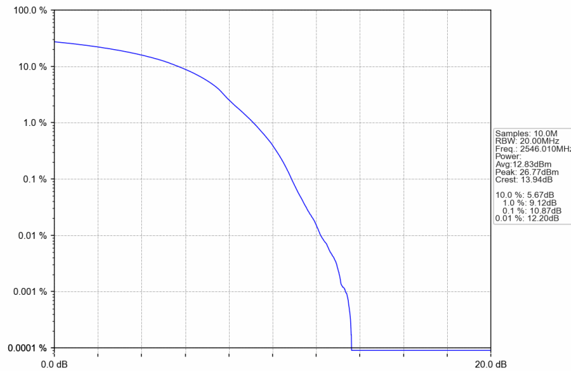
n41_30kHz_SISO_NTNV_100MHz_DFT-s-OFDM 16 QAM_2546.01MHz_Outer_Full
