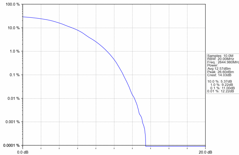
n41_30kHz_SISO_NTNV_90MHz_DFT-s-OFDM 16 QAM_2644.98MHz_Outer_Full
