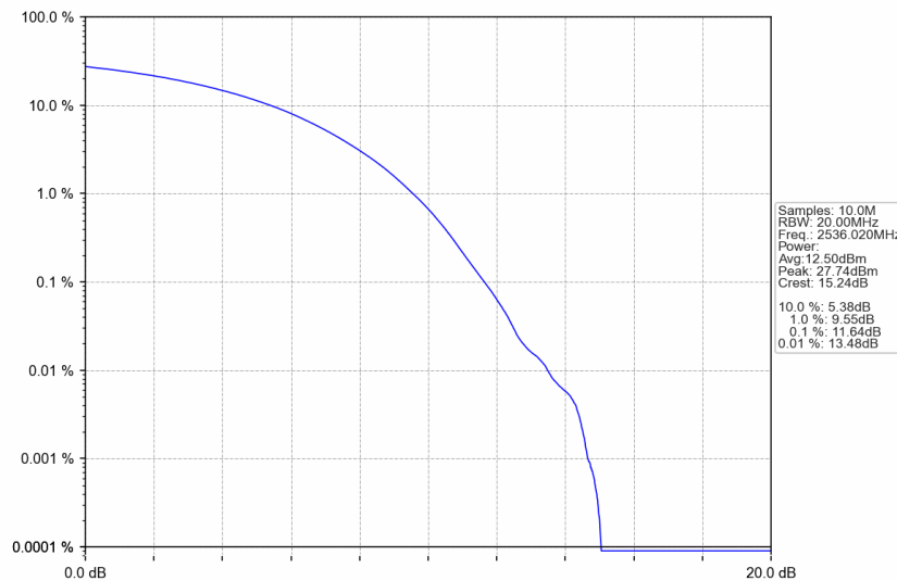
n41_30kHz_SISO_NTNV_80MHz_CP-OFDM 64 QAM_2536.02MHz_Outer_Full
