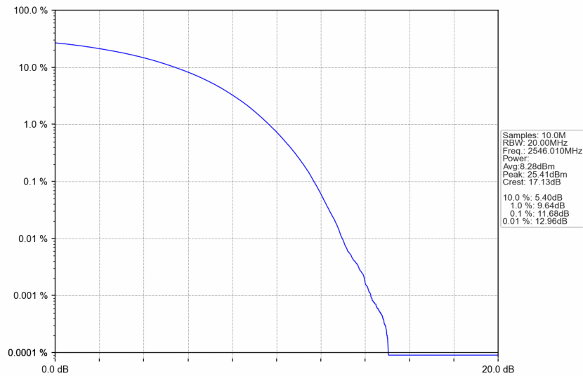
n41_30kHz_SISO_NTNV_100MHz_CP-OFDM 256 QAM_2546.01MHz_Outer_Full
