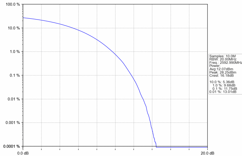
n41_30kHz_SISO_NTNV_90MHz_CP-OFDM QPSK_2592.99MHz_Outer_Full
