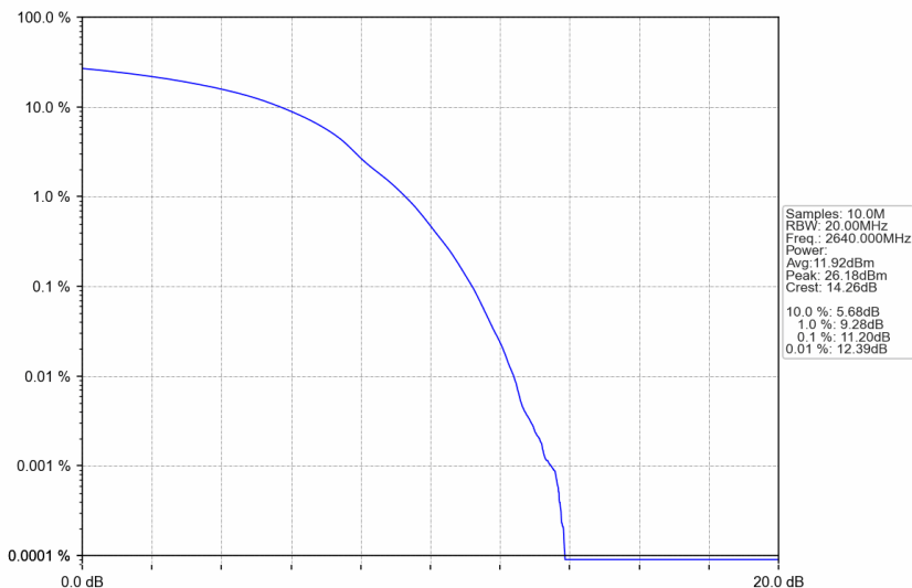
n41_30kHz_SISO_NTNV_100MHz_DFT-s-OFDM 64 QAM_2640MHz_Outer_Full
