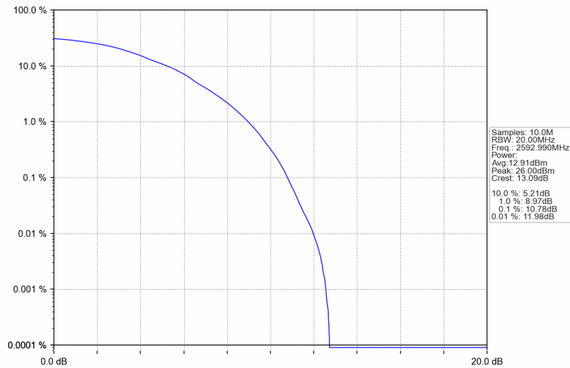
n41_30kHz_SISO_NTNV_90MHz_DFT-s-OFDM 64 QAM_2592.99MHz_Outer_Full
