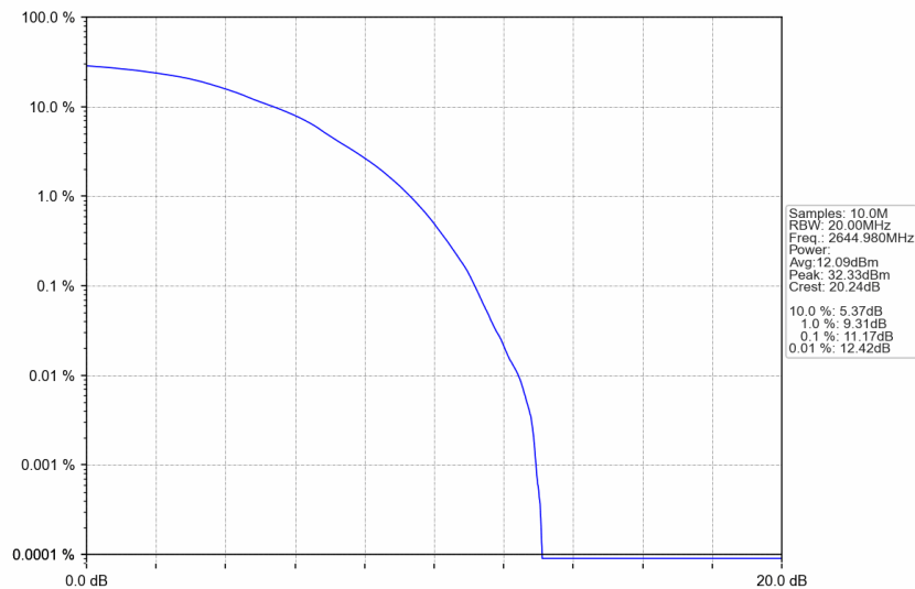
n41_30kHz_SISO_NTNV_90MHz_DFT-s-OFDM 64 QAM_2644.98MHz_Outer_Full
