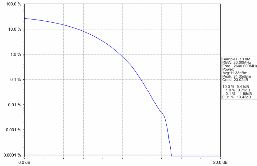
n41_30kHz_SISO_NTNV_100MHz_CP-OFDM 16 QAM_2640MHz_Outer_Full
