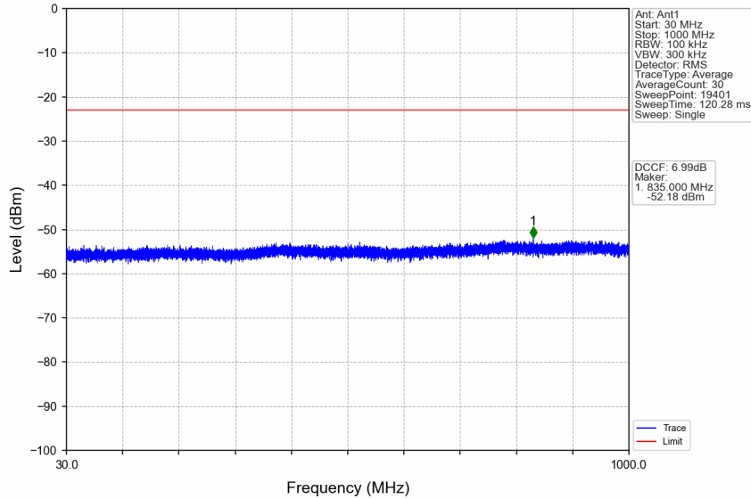
n41_15kHz_SISO_NTNV_10MHz_DFT-s-OFDM_QPSK_2685MHz_Edge_1RB_Right
