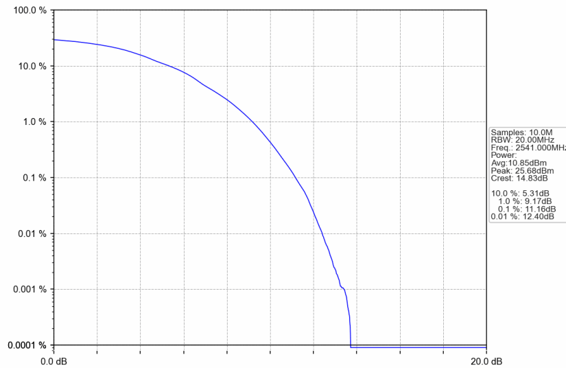
n41_30kHz_SISO_NTNV_90MHz_DFT-s-OFDM 256 QAM_2541MHz_Outer_Full
