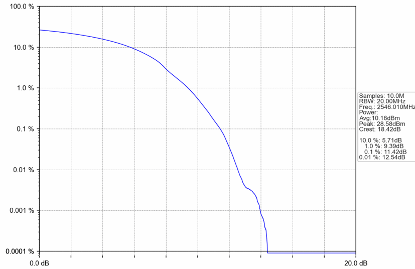
n41_30kHz_SISO_NTNV_100MHz_DFT-s-OFDM 256 QAM_2546.01MHz_Outer_Full
