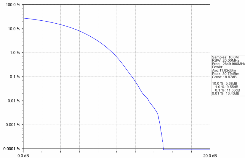
n41_30kHz_SISO_NTNV_80MHz_CP-OFDM 64 QAM_2649.99MHz_Outer_Full
