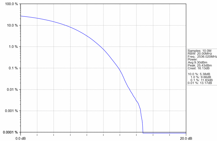
n41_30kHz_SISO_NTNV_80MHz_CP-OFDM 256 QAM_2536.02MHz_Outer_Full
