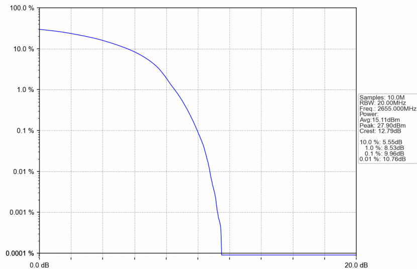
n41_30kHz_SISO_NTNV_70MHz_DFT-s-OFDM QPSK_2655MHz_Outer_Full
