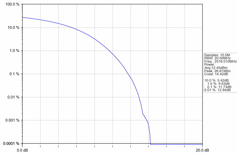
n41_30kHz_SISO_NTNV_40MHz_CP-OFDM 256 QAM_2516.01MHz_Outer_Full
