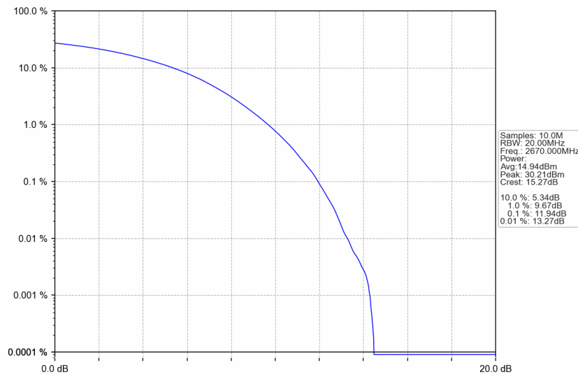
n41_30kHz_SISO_NTNV_40MHz_CP-OFDM 64 QAM_2670MHz_Outer_Full
