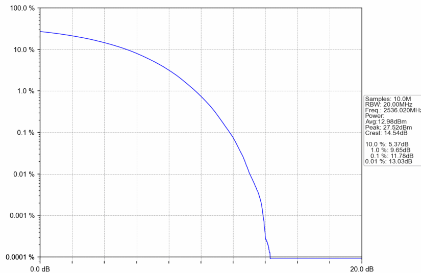
n41_30kHz_SISO_NTNV_80MHz_CP-OFDM QPSK_2536.02MHz_Outer_Full
