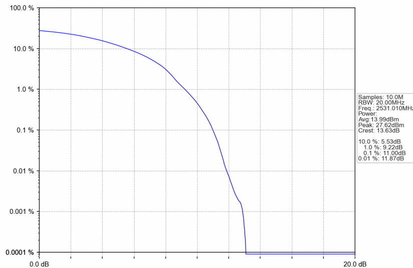
n41_30kHz_SISO_NTNV_70MHz_DFT-s-OFDM 64 QAM_2531.01MHz_Outer_Full
