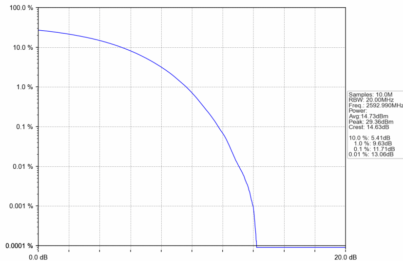
n41_30kHz_SISO_NTNV_50MHz_CP-OFDM 16 QAM_2592.99MHz_Outer_Full
