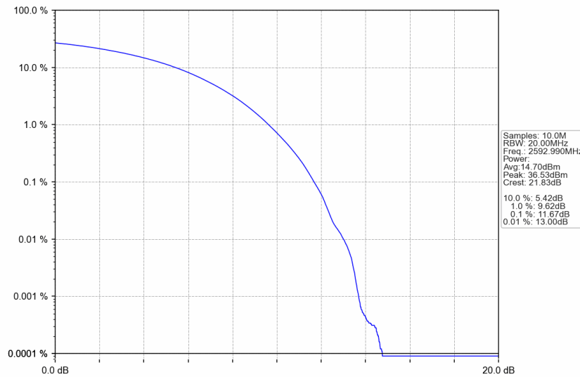
n41_30kHz_SISO_NTNV_50MHz_CP-OFDM QPSK_2592.99MHz_Outer_Full
