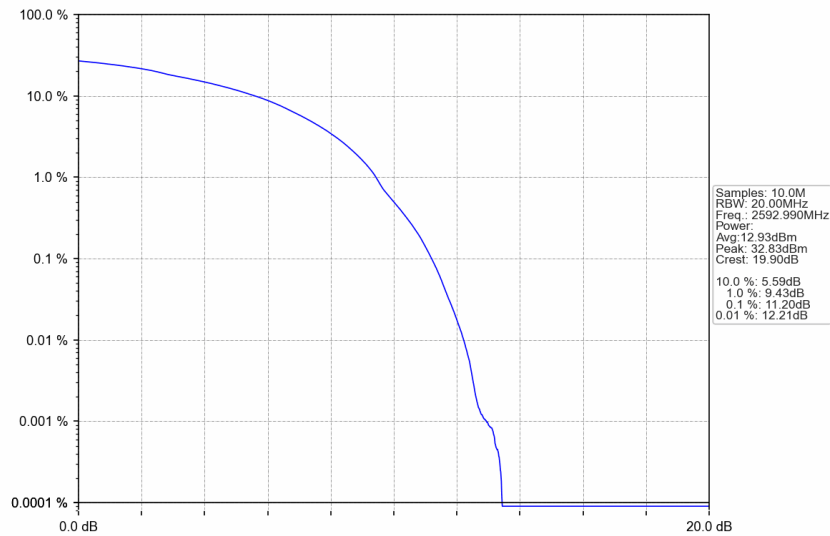
n41_30kHz_SISO_NTNV_80MHz_DFT-s-OFDM 64 QAM_2592.99MHz_Outer_Full
