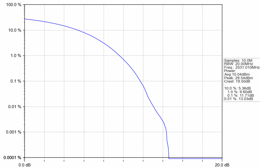
n41_30kHz_SISO_NTNV_70MHz_CP-OFDM 256 QAM_2531.01MHz_Outer_Full
