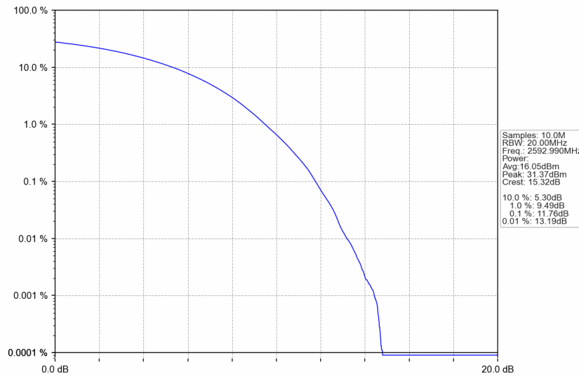
n41_30kHz_SISO_NTNV_40MHz_CP-OFDM QPSK_2592.99MHz_Outer_Full
