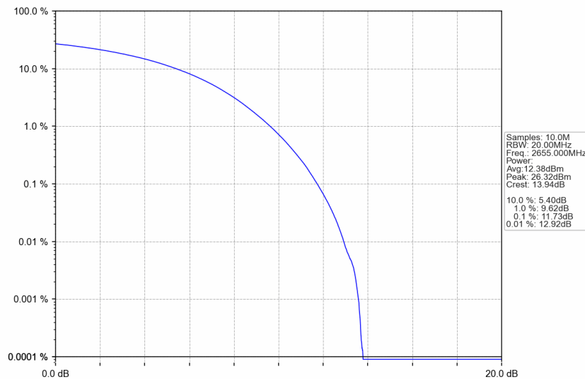
n41_30kHz_SISO_NTNV_70MHz_CP-OFDM 64 QAM_2655MHz_Outer_Full
