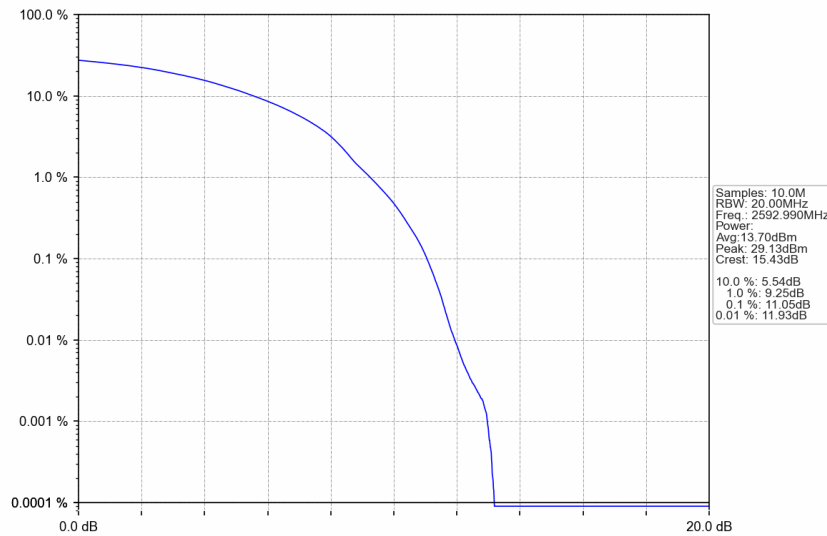
n41_30kHz_SISO_NTNV_70MHz_DFT-s-OFDM 64 QAM_2592.99MHz_Outer_Full
