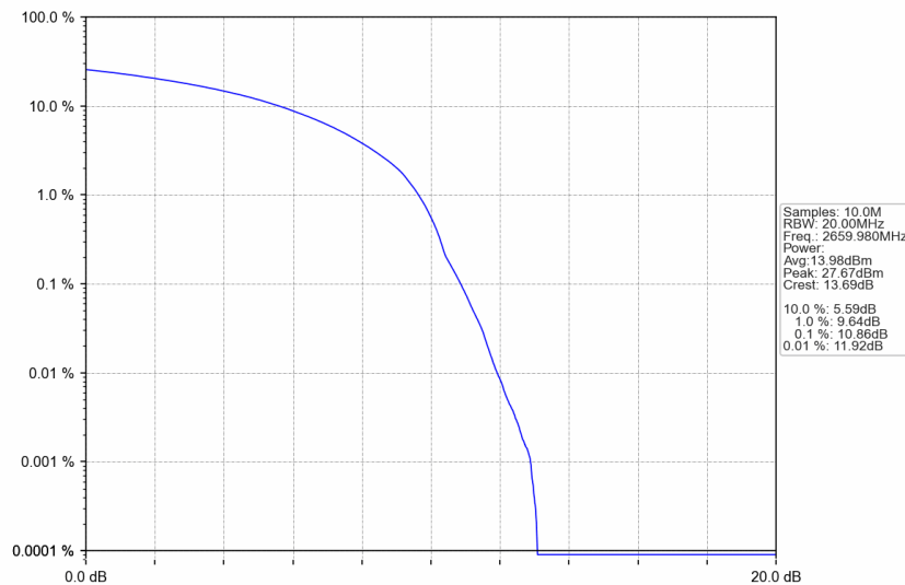
n41_30kHz_SISO_NTNV_60MHz_DFT-s-OFDM 64 QAM_2659.98MHz_Outer_Full
