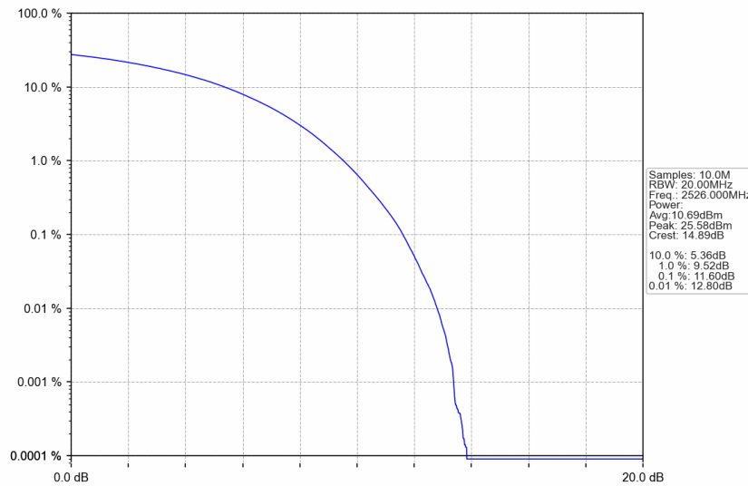
n41_30kHz_SISO_NTNV_60MHz_CP-OFDM 256 QAM_2526MHz_Outer_Full
