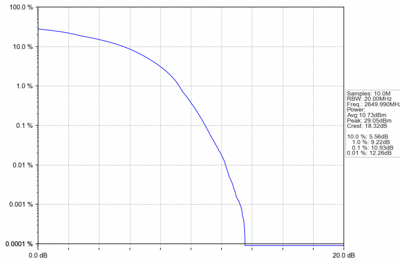
n41_30kHz_SISO_NTNV_80MHz_DFT-s-OFDM 256 QAM_2649.99MHz_Outer_Full
