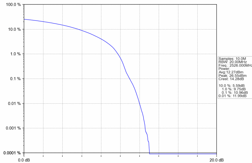
n41_30kHz_SISO_NTNV_60MHz_DFT-s-OFDM_256_QAM_2526MHz_Outer_Full
