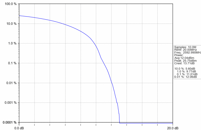
n41_30kHz_SISO_NTNV_60MHz_DFT-s-OFDM_256_QAM_2592.99MHz_Outer_Full
