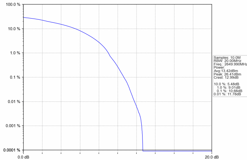
n41_30kHz_SISO_NTNV_80MHz_DFT-s-OFDM 16 QAM_2649.99MHz_Outer_Full
