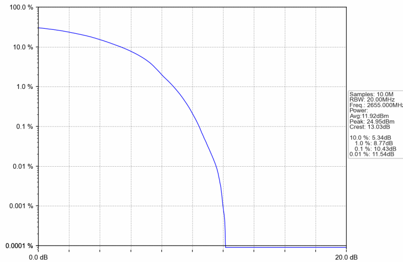
n41_30kHz_SISO_NTNV_70MHz_DFT-s-OFDM 256 QAM_2655MHz_Outer_Full
