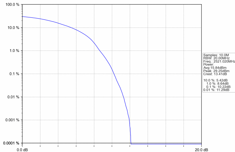
n41_30kHz_SISO_NTNV_50MHz_DFT-s-OFDM 64 QAM_2521.02MHz_Outer_Full
