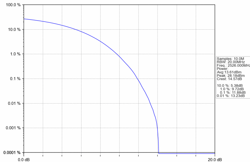
n41_30kHz_SISO_NTNV_60MHz_CP-OFDM 64 QAM_2526MHz_Outer_Full
