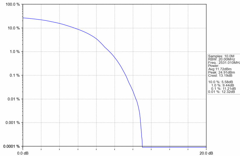
n41_30kHz_SISO_NTNV_70MHz_DFT-s-OFDM 256 QAM_2531.01MHz_Outer_Full
