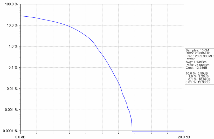
n41_30kHz_SISO_NTNV_80MHz_DFT-s-OFDM 256 QAM_2592.99MHz_Outer_Full
