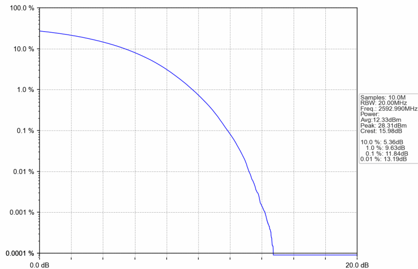
n41_30kHz_SISO_NTNV_40MHz_CP-OFDM 256 QAM_2592.99MHz_Outer_Full
