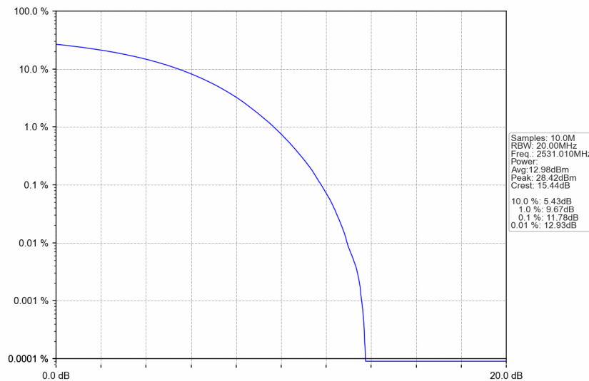
n41_30kHz_SISO_NTNV_70MHz_CP-OFDM 64 QAM_2531.01MHz_Outer_Full
