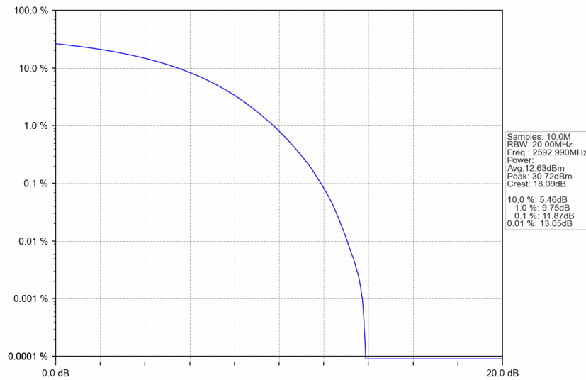
n41_30kHz_SISO_NTNV_70MHz_CP-OFDM 64 QAM_2592.99MHz_Outer_Full
