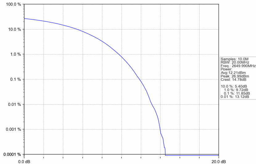
n41_30kHz_SISO_NTNV_80MHz_CP-OFDM QPSK_2649.99MHz_Outer_Full
