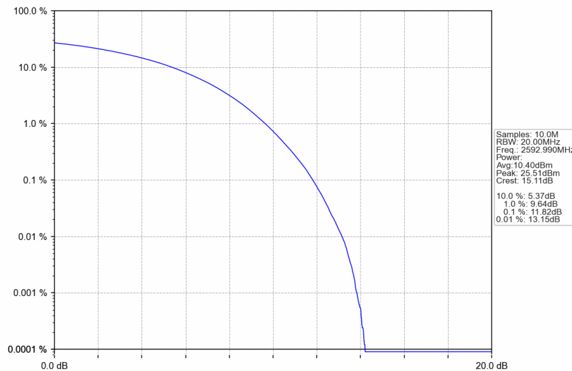
n41_30kHz_SISO_NTNV_60MHz_CP-OFDM 256 QAM_2592.99MHz_Outer_Full
