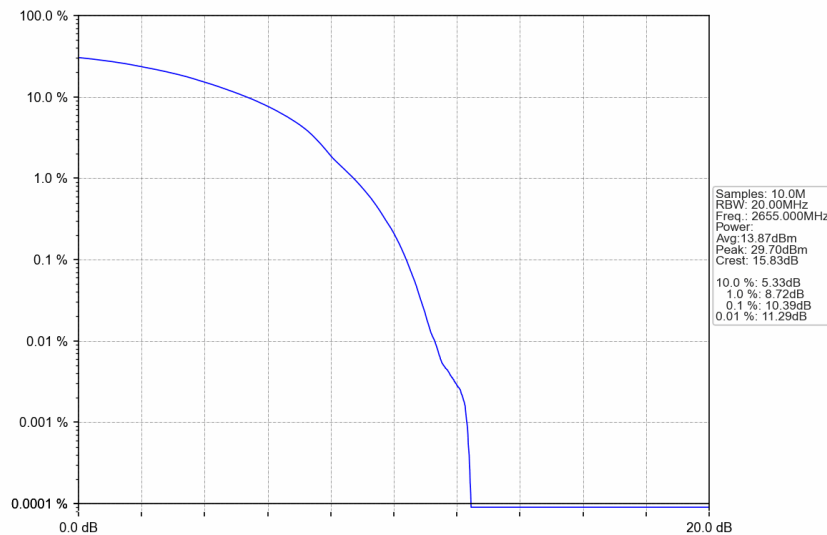
n41_30kHz_SISO_NTNV_70MHz_DFT-s-OFDM 64 QAM_2655MHz_Outer_Full
