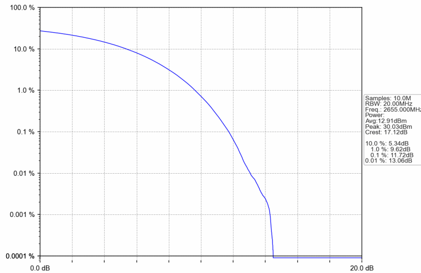
n41_30kHz_SISO_NTNV_70MHz_CP-OFDM 16 QAM_2655MHz_Outer_Full
