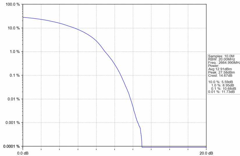
n41_30kHz_SISO_NTNV_50MHz_DFT-s-OFDM 256 QAM_2664.99MHz_Outer_Full
