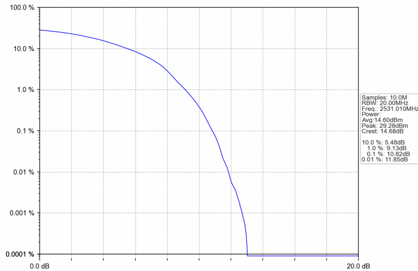
n41_30kHz_SISO_NTNV_70MHz_DFT-s-OFDM 16 QAM_2531.01MHz_Outer_Full
