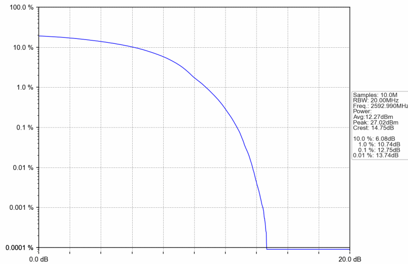
n41_30kHz_SISO_NTNV_50MHz_DFT-s-OFDM 64 QAM_2592.99MHz_Outer_Full
