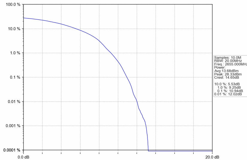
n41_30kHz_SISO_NTNV_70MHz_DFT-s-OFDM 16 QAM_2655MHz_Outer_Full
