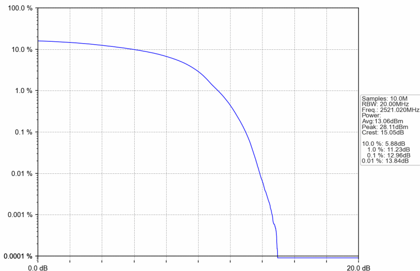
n41_30kHz_SISO_NTNV_50MHz_DFT-s-OFDM QPSK_2521.02MHz_Outer_Full
