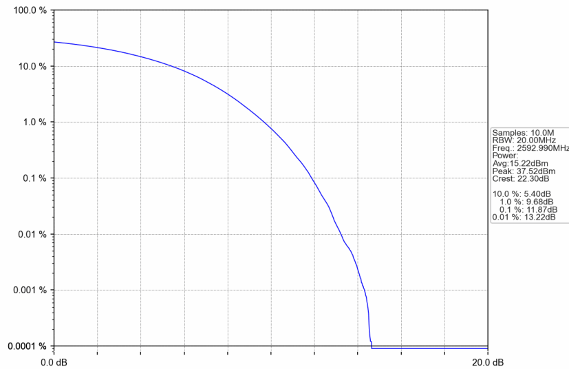
n41_30kHz_SISO_NTNV_40MHz_CP-OFDM 64 QAM_2592.99MHz_Outer_Full
