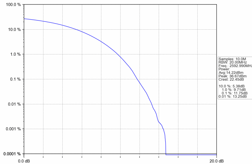
n41_30kHz_SISO_NTNV_50MHz_CP-OFDM 64 QAM_2592.99MHz_Outer_Full
