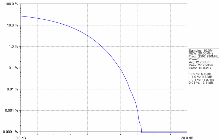
n41_30kHz_SISO_NTNV_80MHz_CP-OFDM QPSK_2592.99MHz_Outer_Full
