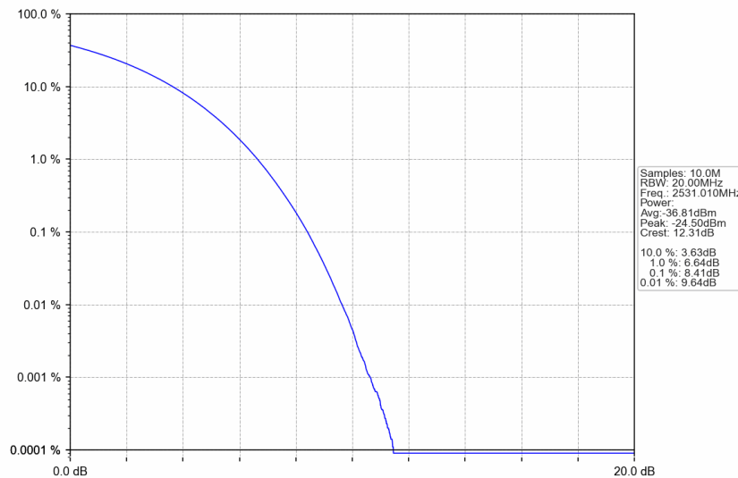
n41_30kHz_SISO_NTNV_70MHz_DFT-s-OFDM QPSK_2531.01MHz_Outer_Full
