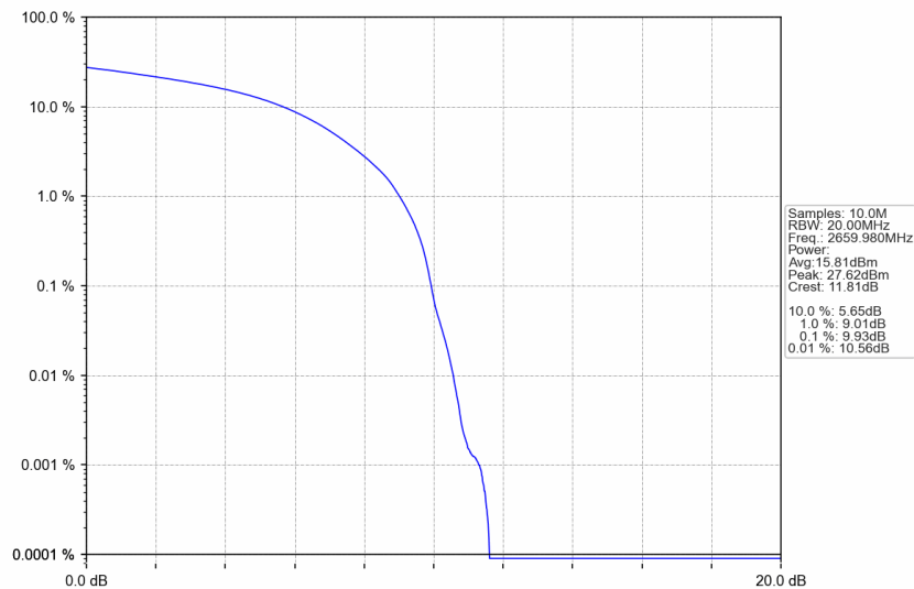
n41_30kHz_SISO_NTNV_60MHz_DFT-s-OFDM QPSK_2659.98MHz_Outer_Full
