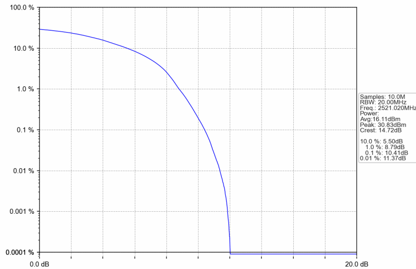
n41_30kHz_SISO_NTNV_50MHz_DFT-s-OFDM 16 QAM_2521.02MHz_Outer_Full
