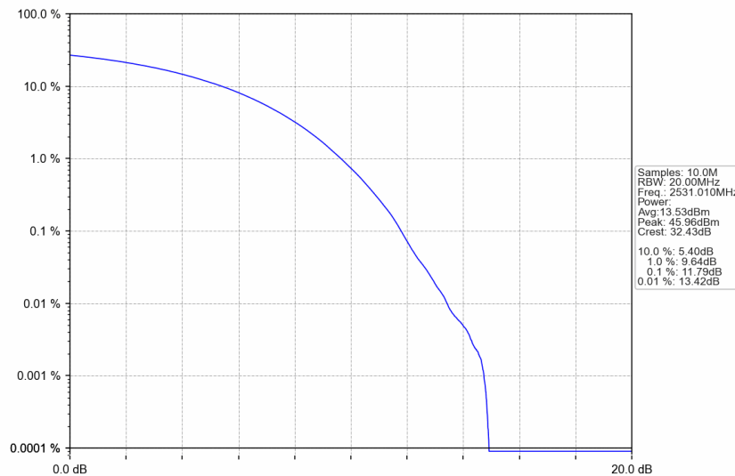
n41_30kHz_SISO_NTNV_70MHz_CP-OFDM QPSK_2531.01MHz_Outer_Full
