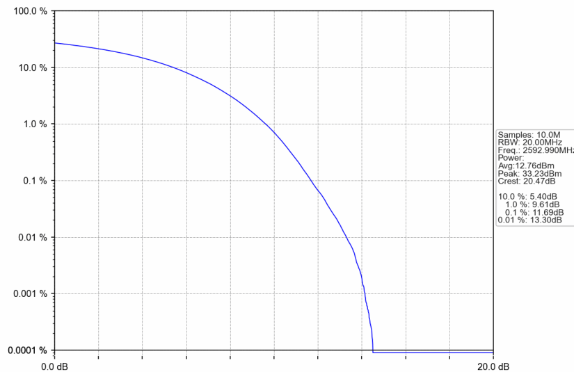
n41_30kHz_SISO_NTNV_80MHz_CP-OFDM 16 QAM_2592.99MHz_Outer_Full
