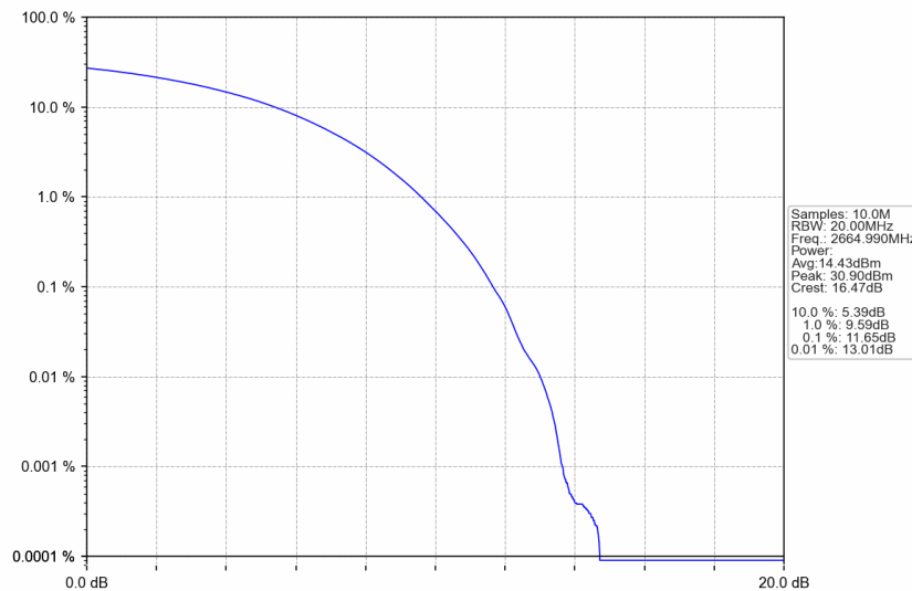
n41_30kHz_SISO_NTNV_50MHz_CP-OFDM QPSK_2664.99MHz_Outer_Full
