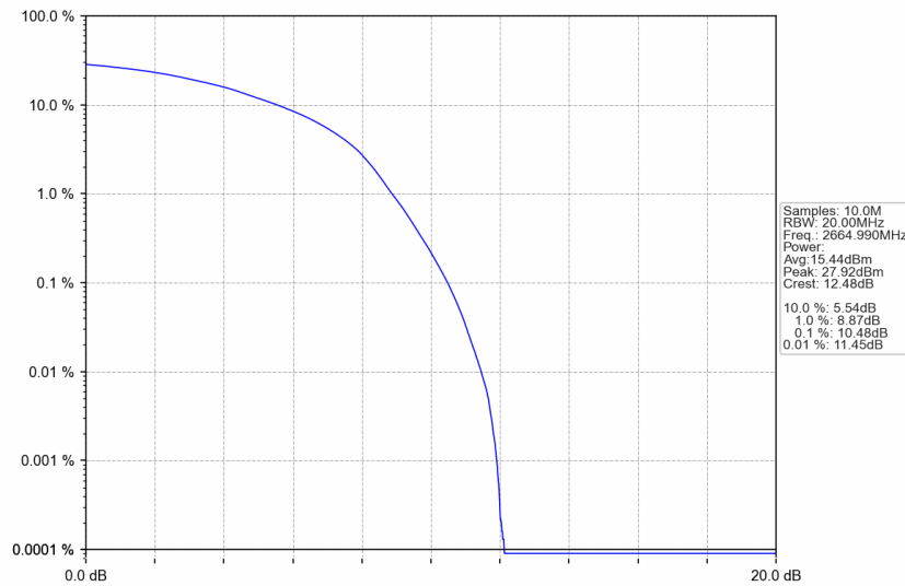
n41_30kHz_SISO_NTNV_50MHz_DFT-s-OFDM 16 QAM_2664.99MHz_Outer_Full
