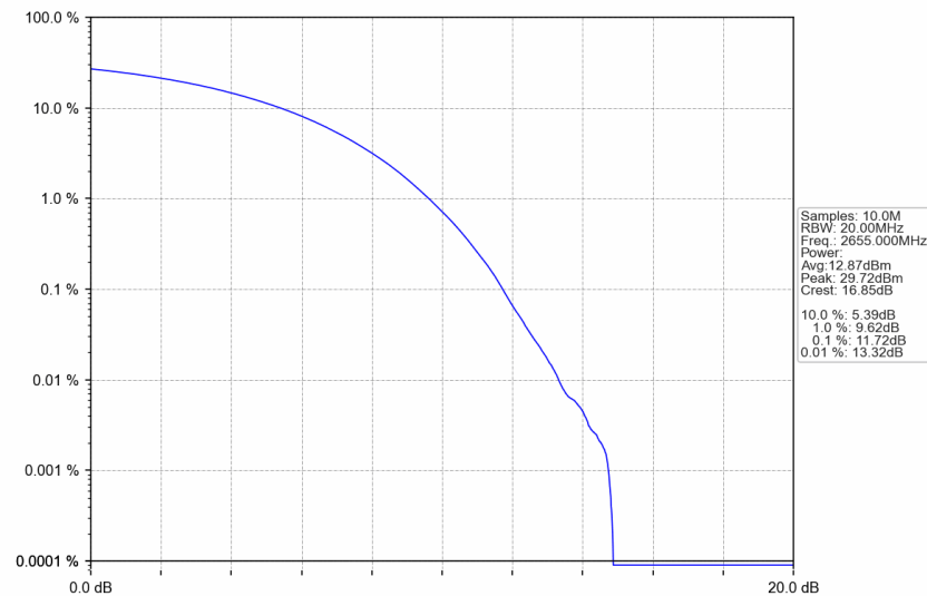
n41_30kHz_SISO_NTNV_70MHz_CP-OFDM QPSK_2655MHz_Outer_Full
