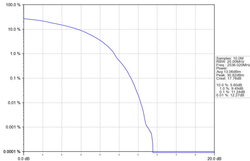
n41_30kHz_SISO_NTNV_80MHz_DFT-s-OFDM 64 QAM_2536.02MHz_Outer_Full
