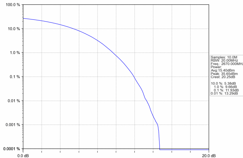
n41_30kHz_SISO_NTNV_40MHz_CP-OFDM QPSK_2670MHz_Outer_Full
