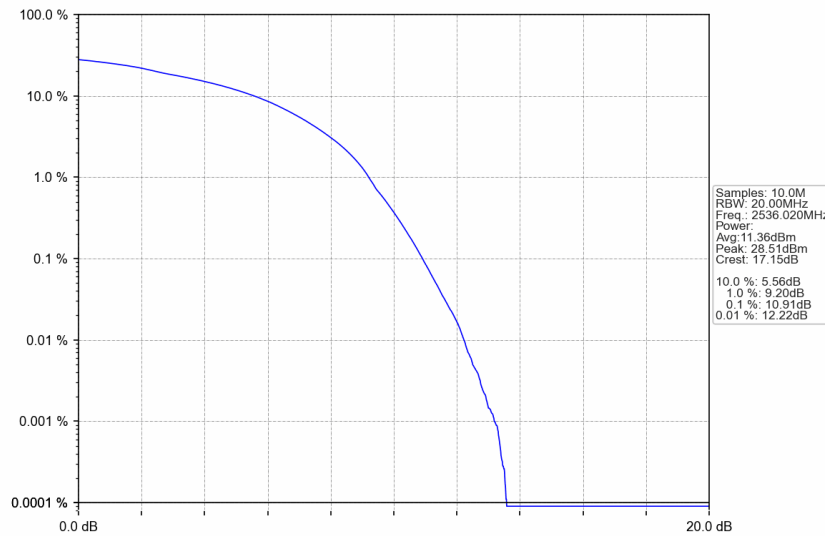
n41_30kHz_SISO_NTNV_80MHz_DFT-s-OFDM 256 QAM_2536.02MHz_Outer_Full
