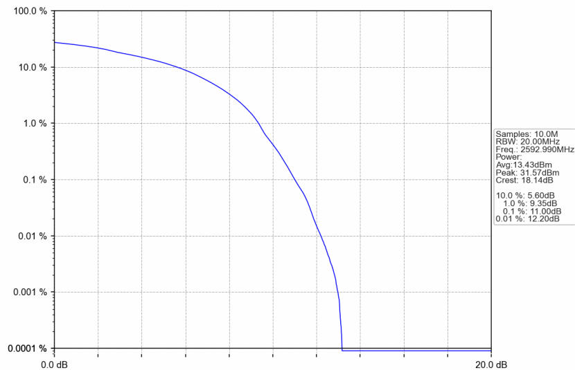
n41_30kHz_SISO_NTNV_80MHz_DFT-s-OFDM 16 QAM_2592.99MHz_Outer_Full
