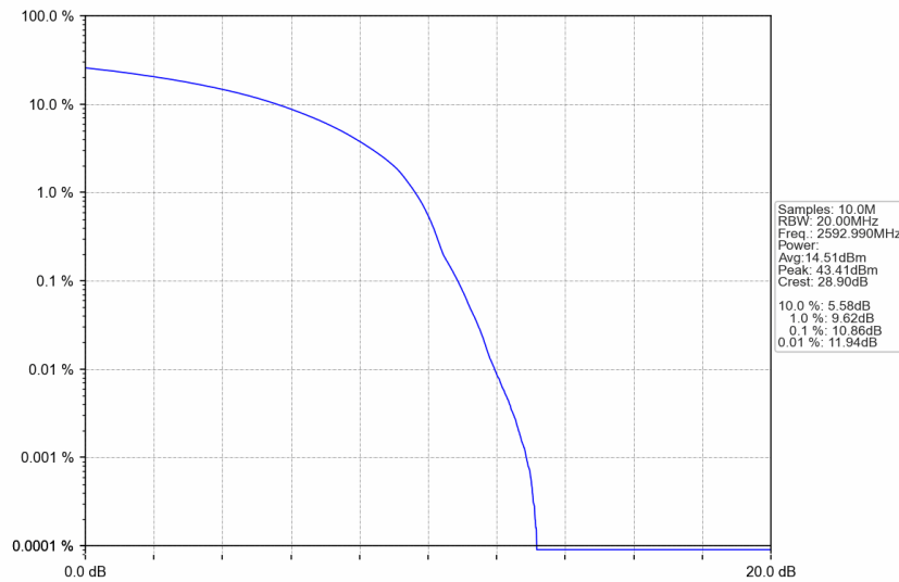
n41_30kHz_SISO_NTNV_60MHz_DFT-s-OFDM 64 QAM_2592.99MHz_Outer_Full
