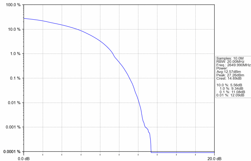
n41_30kHz_SISO_NTNV_80MHz_DFT-s-OFDM 64 QAM_2649.99MHz_Outer_Full
