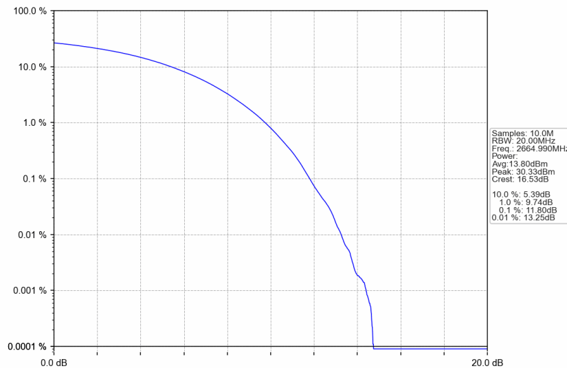
n41_30kHz_SISO_NTNV_50MHz_CP-OFDM 64 QAM_2664.99MHz_Outer_Full
