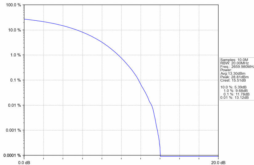
n41_30kHz_SISO_NTNV_60MHz_CP-OFDM 64 QAM_2659.98MHz_Outer_Full
