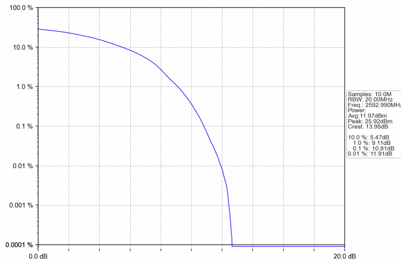
n41_30kHz_SISO_NTNV_70MHz_DFT-s-OFDM 256 QAM_2592.99MHz_Outer_Full
