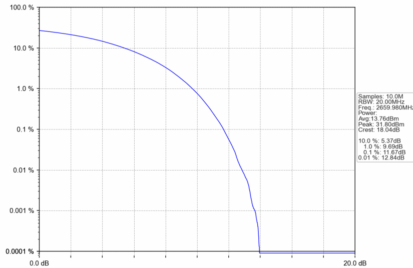
n41_30kHz_SISO_NTNV_60MHz_CP-OFDM 16 QAM_2659.98MHz_Outer_Full
