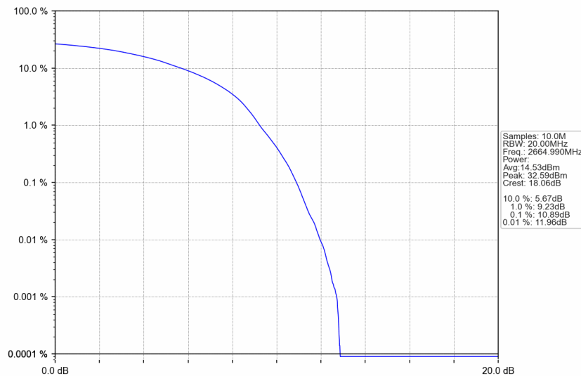
n41_30kHz_SISO_NTNV_50MHz_DFT-s-OFDM 64 QAM_2664.99MHz_Outer_Full
