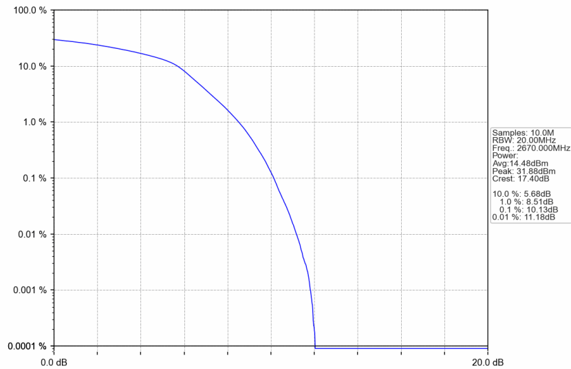
n41_30kHz_SISO_NTNV_40MHz_DFT-s-OFDM 256 QAM_2670MHz_Outer_Full
