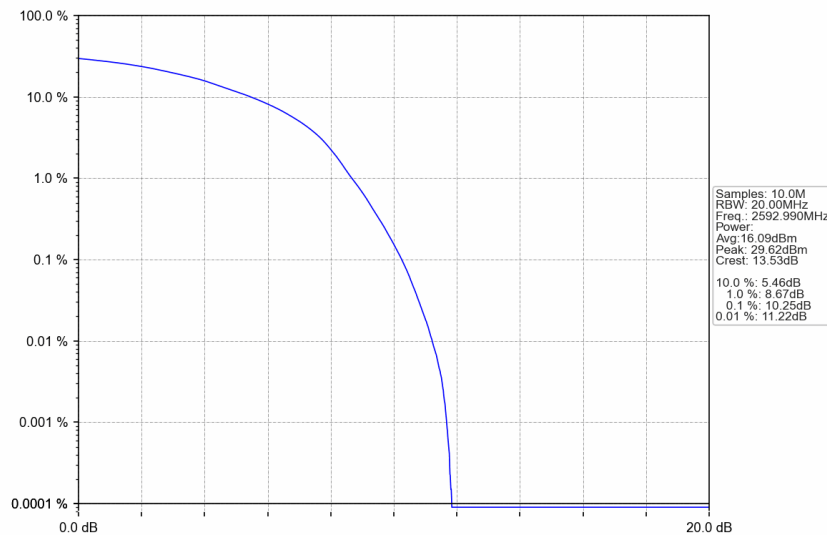
n41_30kHz_SISO_NTNV_50MHz_DFT-s-OFDM 16 QAM_2592.99MHz_Outer_Full
