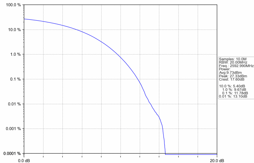
n41_30kHz_SISO_NTNV_70MHz_CP-OFDM 256 QAM_2592.99MHz_Outer_Full
