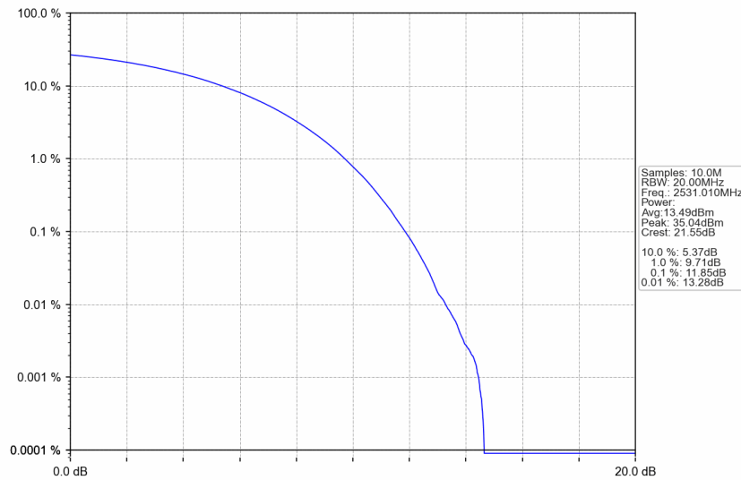
n41_30kHz_SISO_NTNV_70MHz_CP-OFDM 16 QAM_2531.01MHz_Outer_Full
