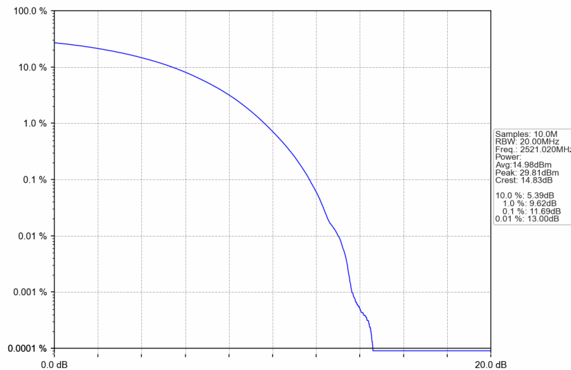
n41_30kHz_SISO_NTNV_50MHz_CP-OFDM QPSK_2521.02MHz_Outer_Full
