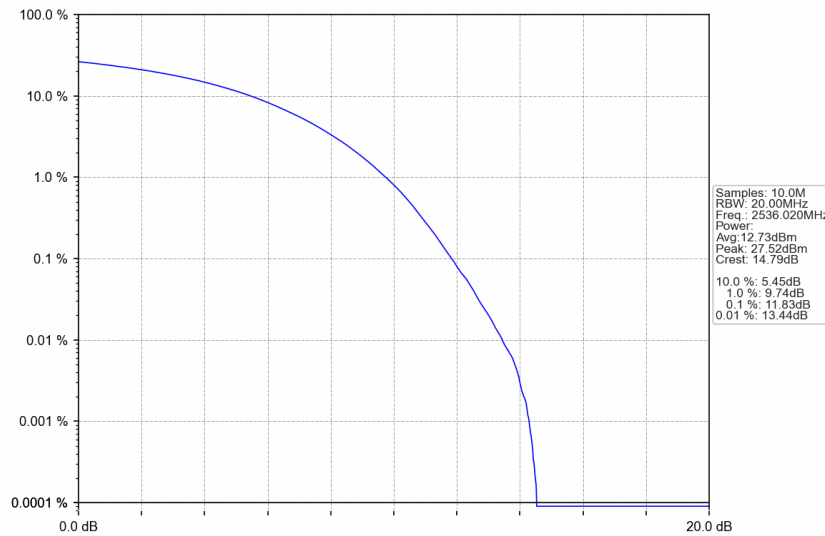
n41_30kHz_SISO_NTNV_80MHz_CP-OFDM 16 QAM_2536.02MHz_Outer_Full
