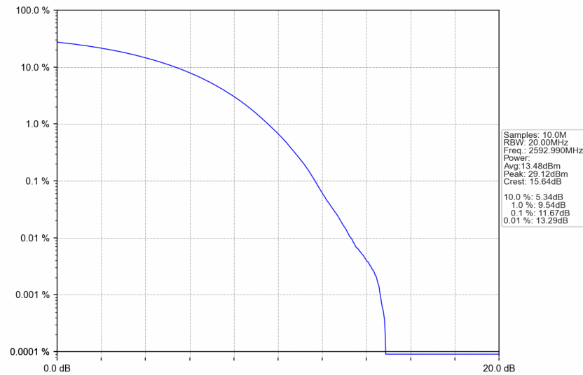
n41_30kHz_SISO_NTNV_70MHz_CP-OFDM QPSK_2592.99MHz_Outer_Full
