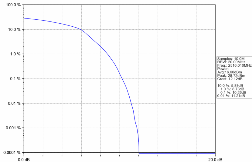
n41_30kHz_SISO_NTNV_40MHz_DFT-s-OFDM 64 QAM_2516.01MHz_Outer_Full
