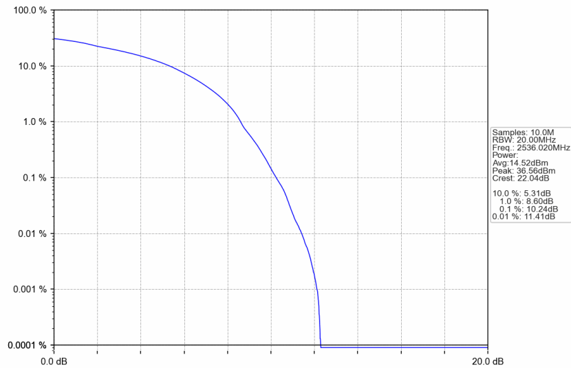
n41_30kHz_SISO_NTNV_80MHz_DFT-s-OFDM 16 QAM_2536.02MHz_Outer_Full
