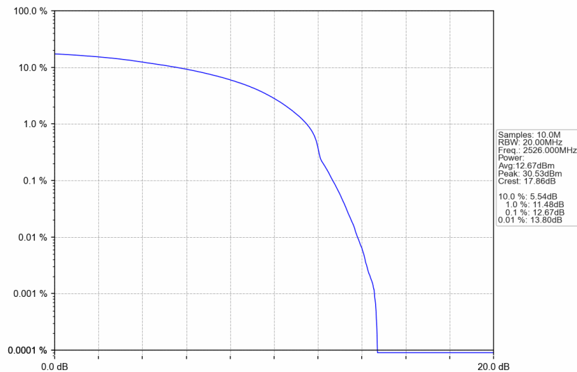
n41_30kHz_SISO_NTNV_60MHz_DFT-s-OFDM QPSK_2526MHz_Outer_Full
