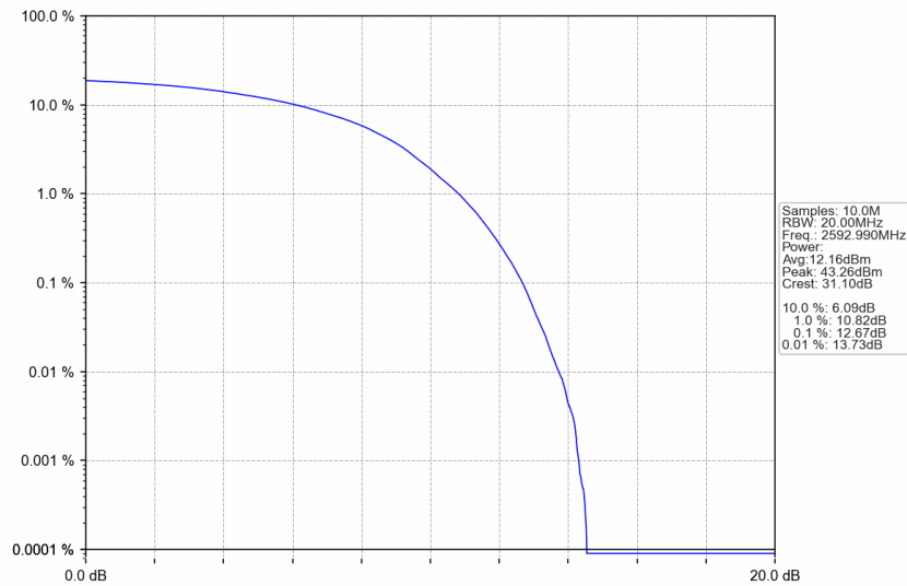
n41_30kHz_SISO_NTNV_70MHz_DFT-s-OFDM QPSK_2592.99MHz_Outer_Full
