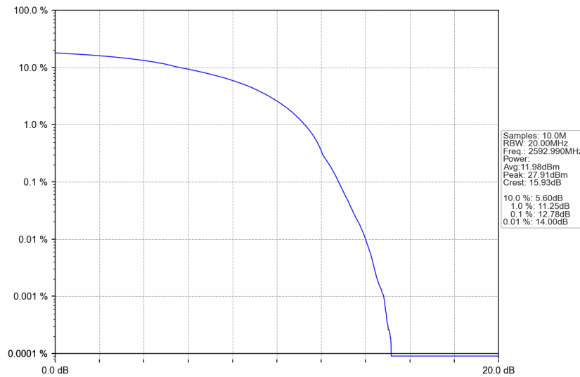
n41_30kHz_SISO_NTNV_80MHz_DFT-s-OFDM QPSK_2592.99MHz_Outer_Full
