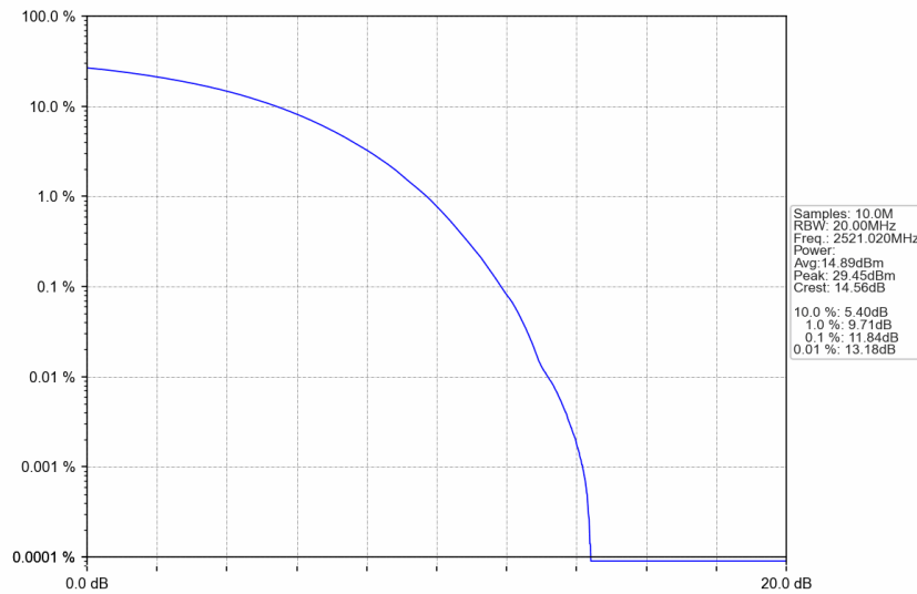
n41_30kHz_SISO_NTNV_50MHz_CP-OFDM 16 QAM_2521.02MHz_Outer_Full
