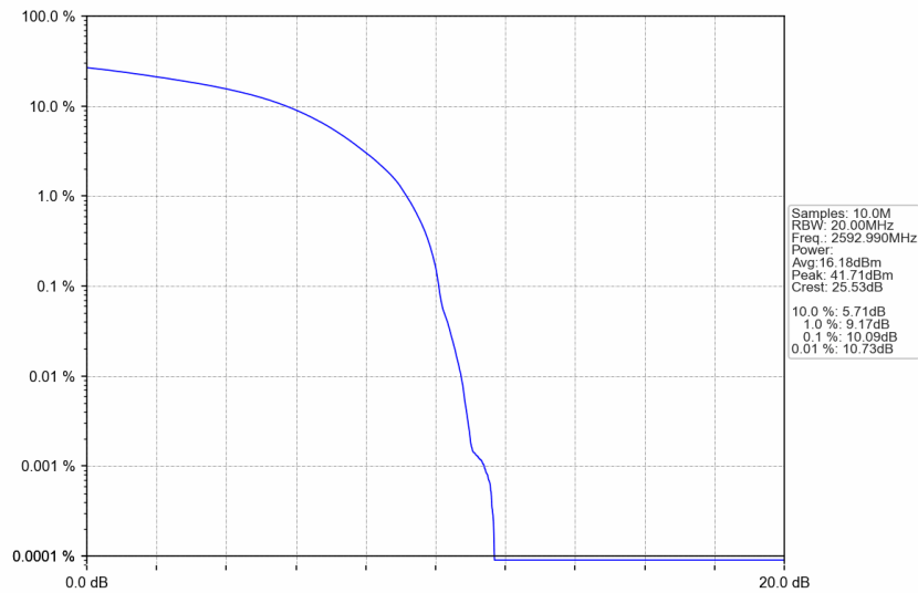
n41_30kHz_SISO_NTNV_60MHz_DFT-s-OFDM QPSK_2592.99MHz_Outer_Full
