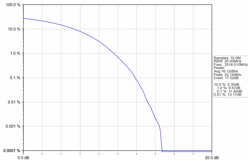
n41_30kHz_SISO_NTNV_40MHz_CP-OFDM QPSK_2516.01MHz_Outer_Full
