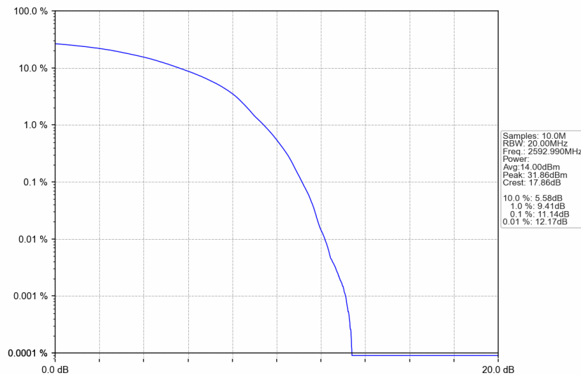
n41_30kHz_SISO_NTNV_70MHz_DFT-s-OFDM 16 QAM_2592.99MHz_Outer_Full
