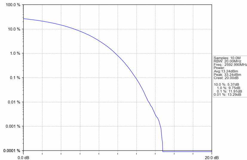
n41_30kHz_SISO_NTNV_70MHz_CP-OFDM 16 QAM_2592.99MHz_Outer_Full
