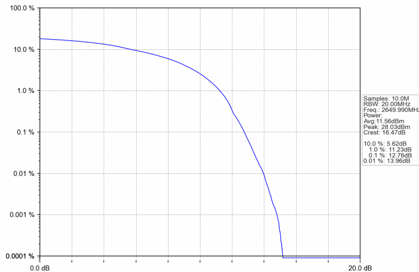
n41_30kHz_SISO_NTNV_80MHz_DFT-s-OFDM QPSK_2649.99MHz_Outer_Full
