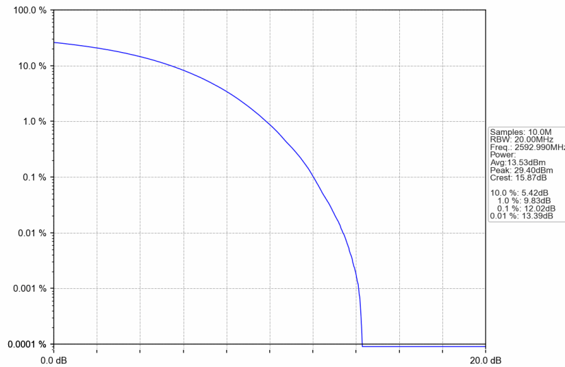
n41_30kHz_SISO_NTNV_60MHz_CP-OFDM 64 QAM_2592.99MHz_Outer_Full
