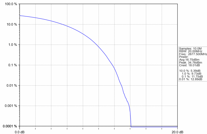
n41_30kHz_SISO_NTNV_25MHz_CP-OFDM 64 QAM_2677.5MHz_Outer_Full
