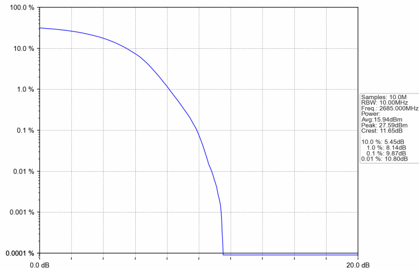
n41_30kHz_SISO_NTNV_10MHz_DFT-s-OFDM 256 QAM_2685MHz_Outer_Full
