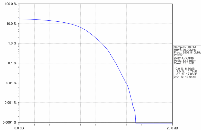
n41_30kHz_SISO_NTNV_25MHz_DFT-s-OFDM 64 QAM_2508.51MHz_Outer_Full
