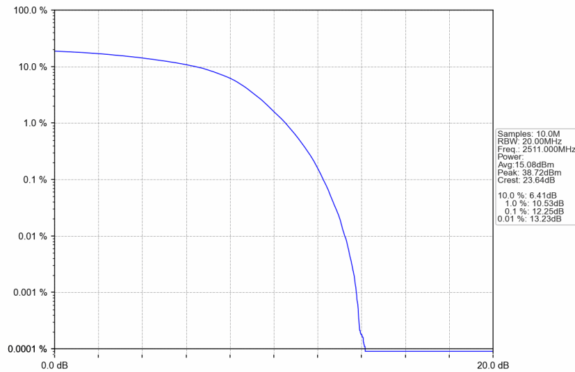
n41_30kHz_SISO_NTNV_30MHz_DFT-s-OFDM 16 QAM_2511MHz_Outer_Full
