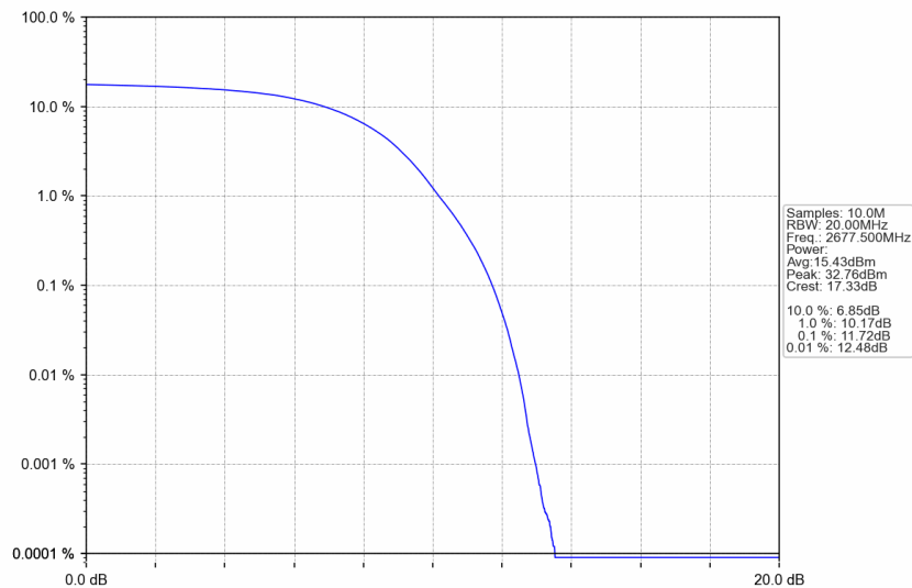
n41_30kHz_SISO_NTNV_25MHz_DFT-s-OFDM QPSK_2677.5MHz_Outer_Full
