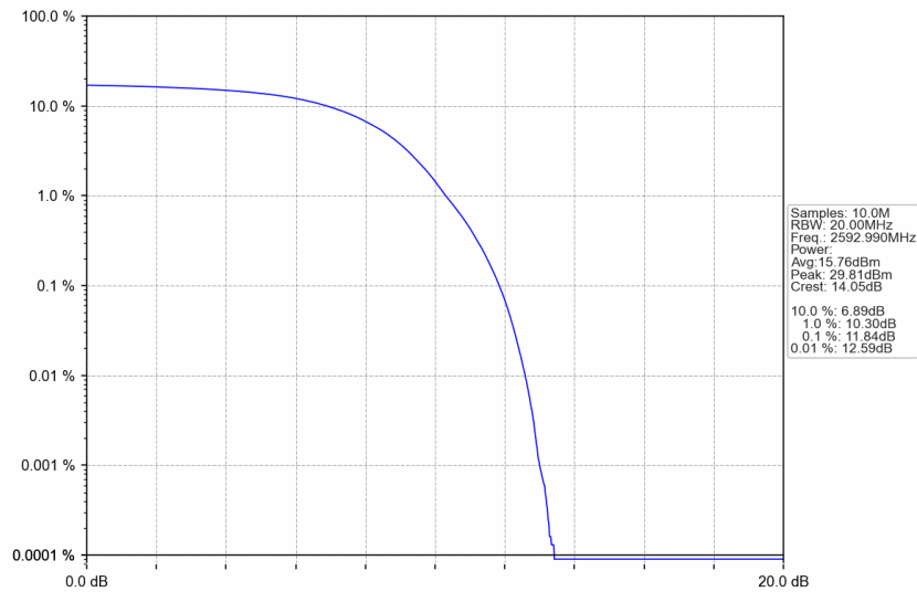
n41_30kHz_SISO_NTNV_25MHz_DFT-s-OFDM QPSK_2592.99MHz_Outer_Full
