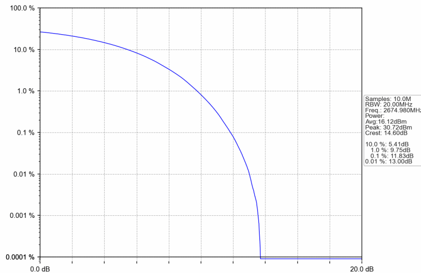
n41_30kHz_SISO_NTNV_30MHz_CP-OFDM 64 QAM_2674.98MHz_Outer_Full
