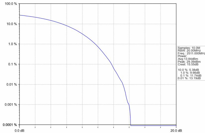
n41_30kHz_SISO_NTNV_30MHz_CP-OFDM 256 QAM_2511MHz_Outer_Full
