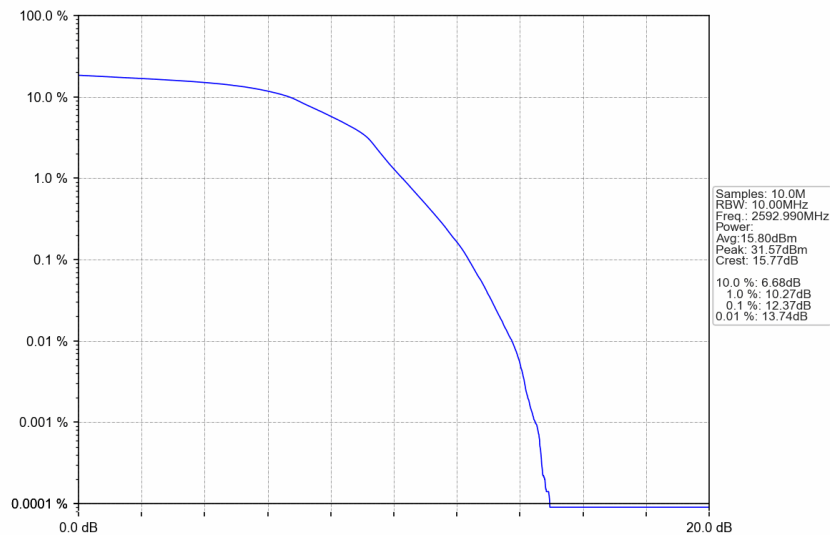
n41_30kHz_SISO_NTNV_10MHz_DFT-s-OFDM 16 QAM_2592.99MHz_Outer_Full
