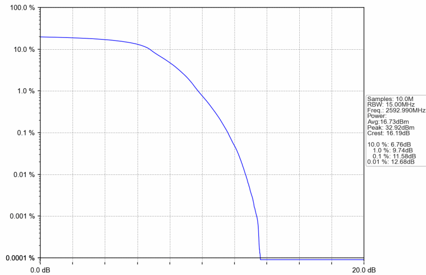
n41_30kHz_SISO_NTNV_15MHz_DFT-s-OFDM QPSK_2592.99MHz_Outer_Full
