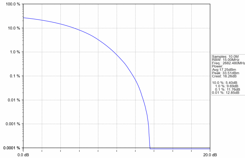
n41_30kHz_SISO_NTNV_15MHz_CP-OFDM QPSK_2682.48MHz_Outer_Full
