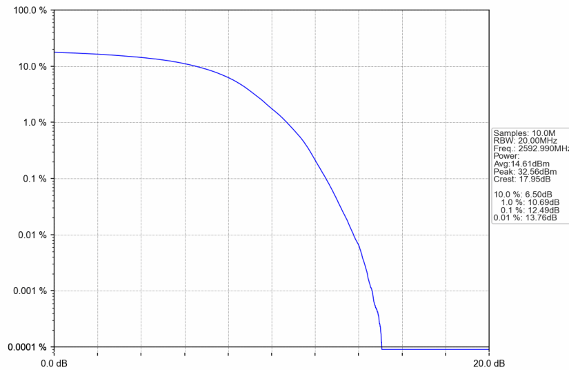
n41_30kHz_SISO_NTNV_25MHz_DFT-s-OFDM 64 QAM_2592.99MHz_Outer_Full
