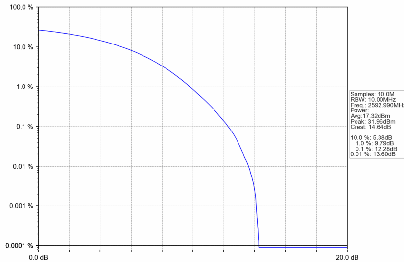
n41_30kHz_SISO_NTNV_10MHz_CP-OFDM QPSK_2592.99MHz_Outer_Full
