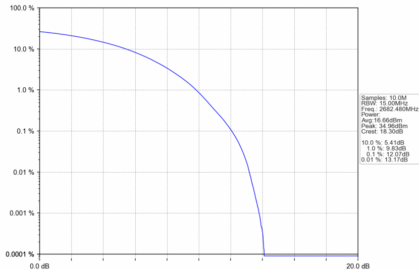
n41_30kHz_SISO_NTNV_15MHz_CP-OFDM 64 QAM_2682.48MHz_Outer_Full
