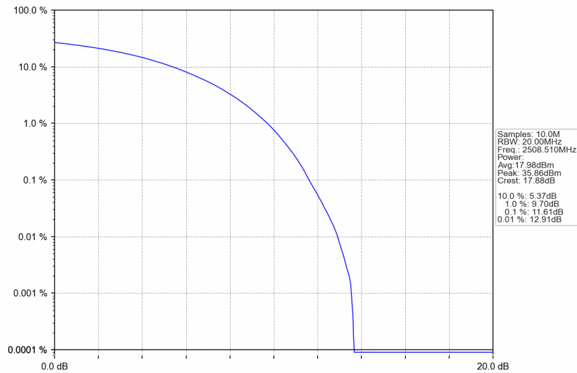
n41_30kHz_SISO_NTNV_25MHz_CP-OFDM 16 QAM_2508.51MHz_Outer_Full
