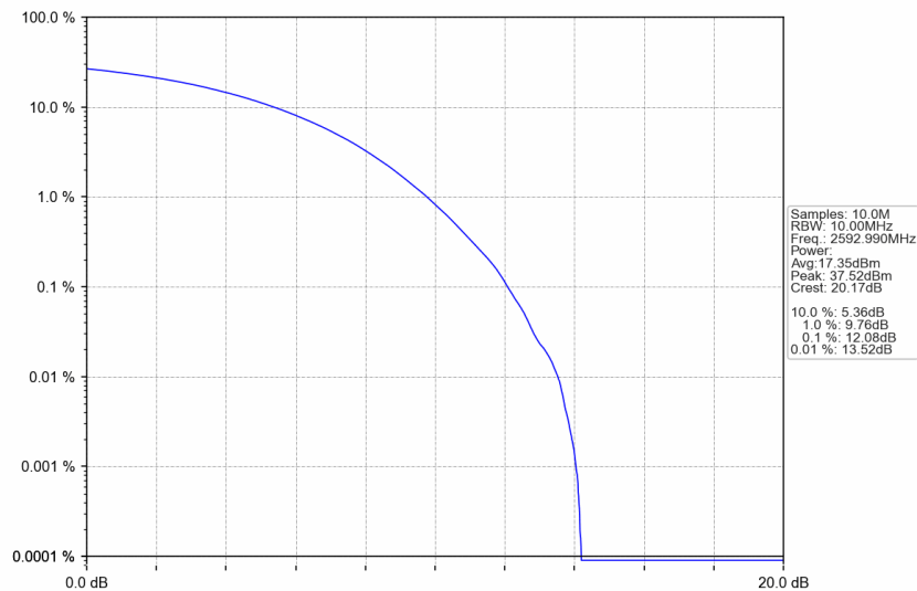
n41_30kHz_SISO_NTNV_10MHz_CP-OFDM 16 QAM_2592.99MHz_Outer_Full
