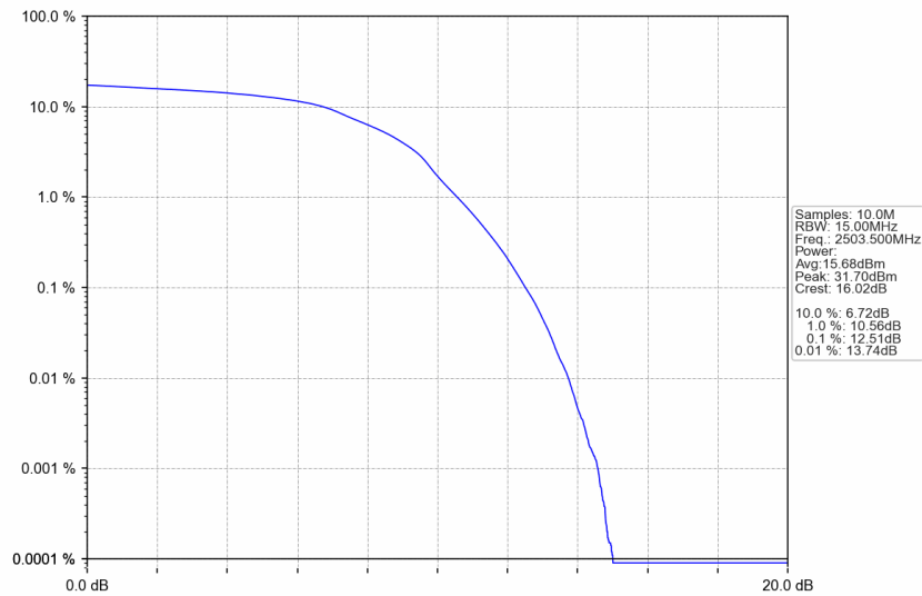
n41_30kHz_SISO_NTNV_15MHz_DFT-s-OFDM 16 QAM_2503.5MHz_Outer_Full
