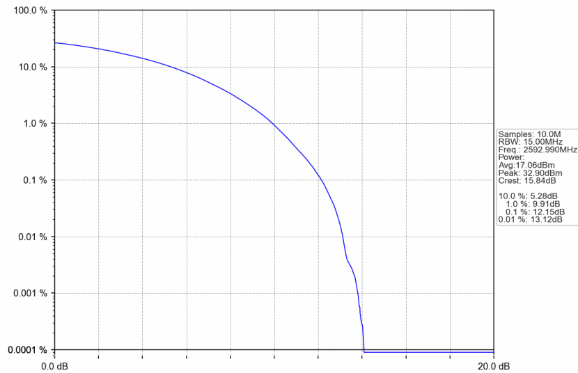
n41_30kHz_SISO_NTNV_15MHz_CP-OFDM 64 QAM_2592.99MHz_Outer_Full
