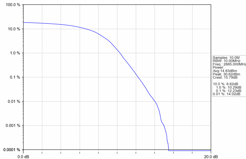
n41_30kHz_SISO_NTNV_10MHz_DFT-s-OFDM 64 QAM_2685MHz_Outer_Full
