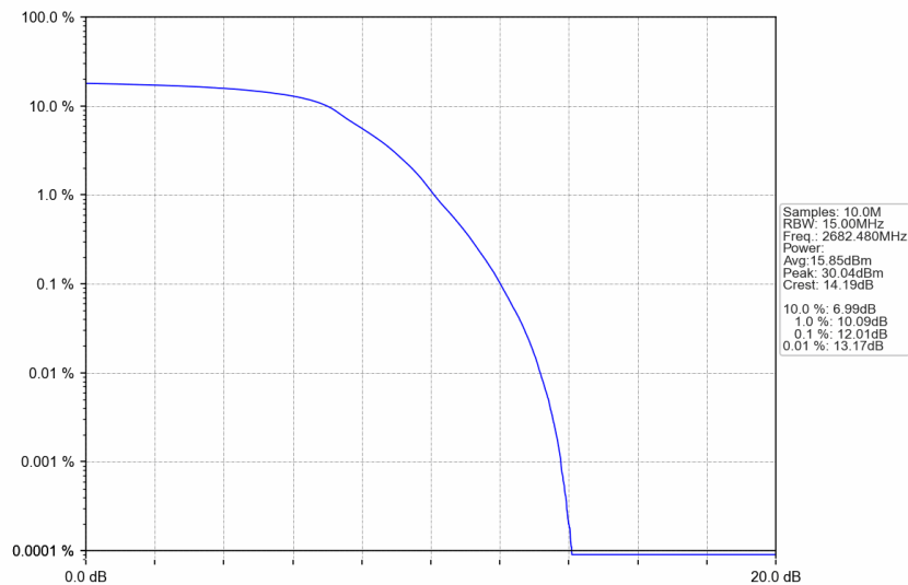
n41_30kHz_SISO_NTNV_15MHz_DFT-s-OFDM QPSK_2682.48MHz_Outer_Full
