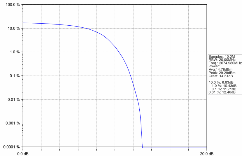
n41_30kHz_SISO_NTNV_30MHz_DFT-s-OFDM QPSK_2674.98MHz_Outer_Full
