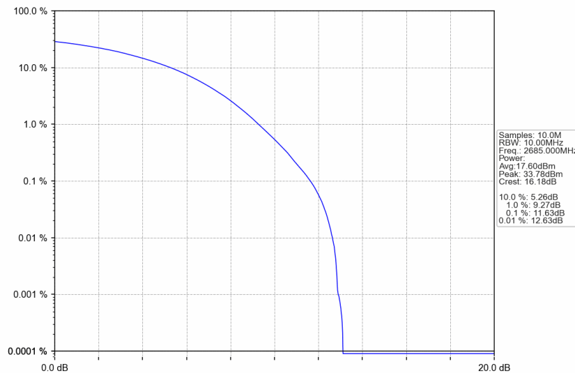
n41_30kHz_SISO_NTNV_10MHz_CP-OFDM QPSK_2685MHz_Outer_Full
