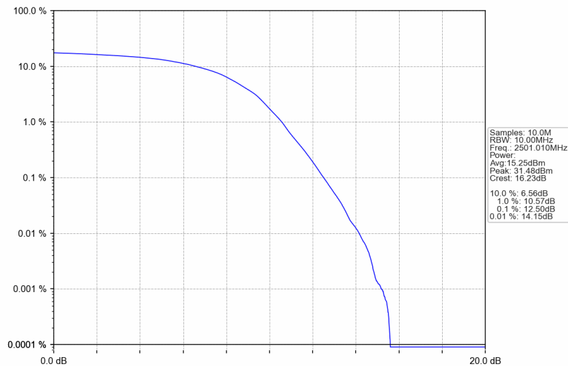
n41_30kHz_SISO_NTNV_10MHz_DFT-s-OFDM 64 QAM_2501.01MHz_Outer_Full
