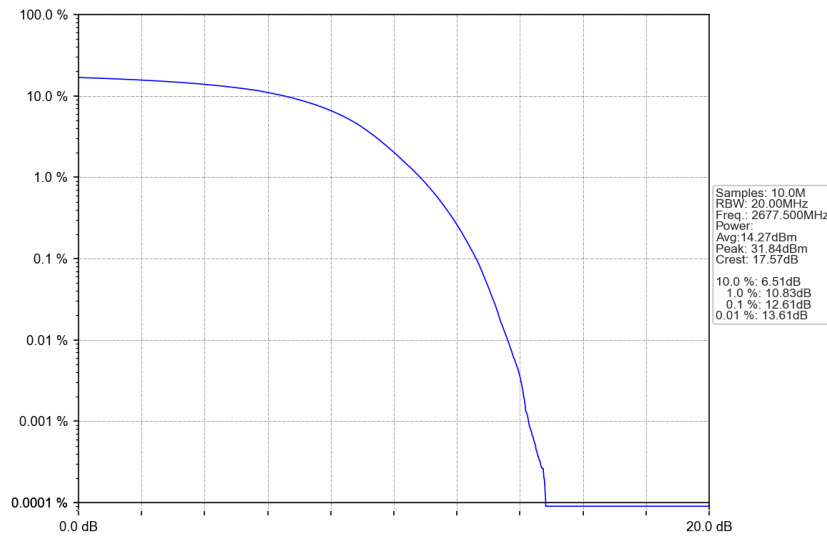
n41_30kHz_SISO_NTNV_25MHz_DFT-s-OFDM 16 QAM_2677.5MHz_Outer_Full
