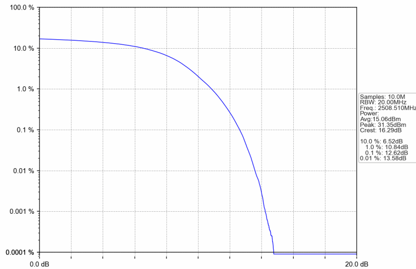
n41_30kHz_SISO_NTNV_25MHz_DFT-s-OFDM 16 QAM_2508.51MHz_Outer_Full
