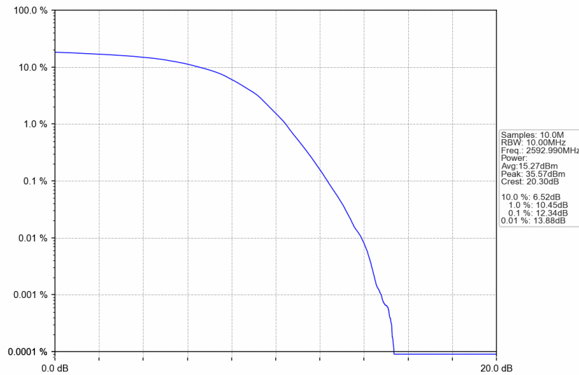
n41_30kHz_SISO_NTNV_10MHz_DFT-s-OFDM 64 QAM_2592.99MHz_Outer_Full
