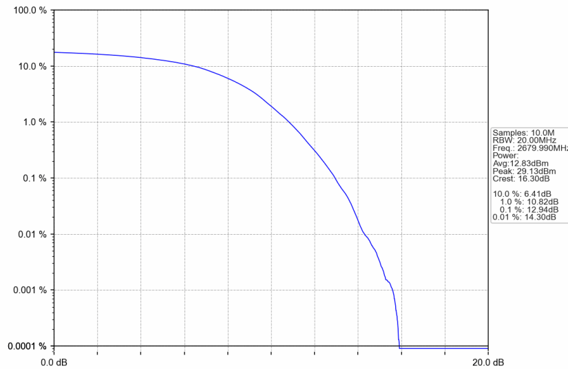
n41_30kHz_SISO_NTNV_20MHz_DFT-s-OFDM 256 QAM_2679.99MHz_Outer_Full
