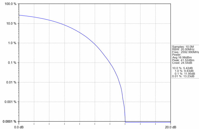
n41_30kHz_SISO_NTNV_30MHz_CP-OFDM 16 QAM_2592.99MHz_Outer_Full
