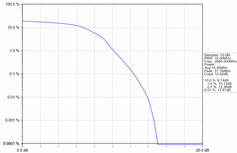
n41_30kHz_SISO_NTNV_10MHz_DFT-s-OFDM 16 QAM_2685MHz_Outer_Full
