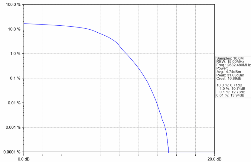
n41_30kHz_SISO_NTNV_15MHz_DFT-s-OFDM 16 QAM_2682.48MHz_Outer_Full
