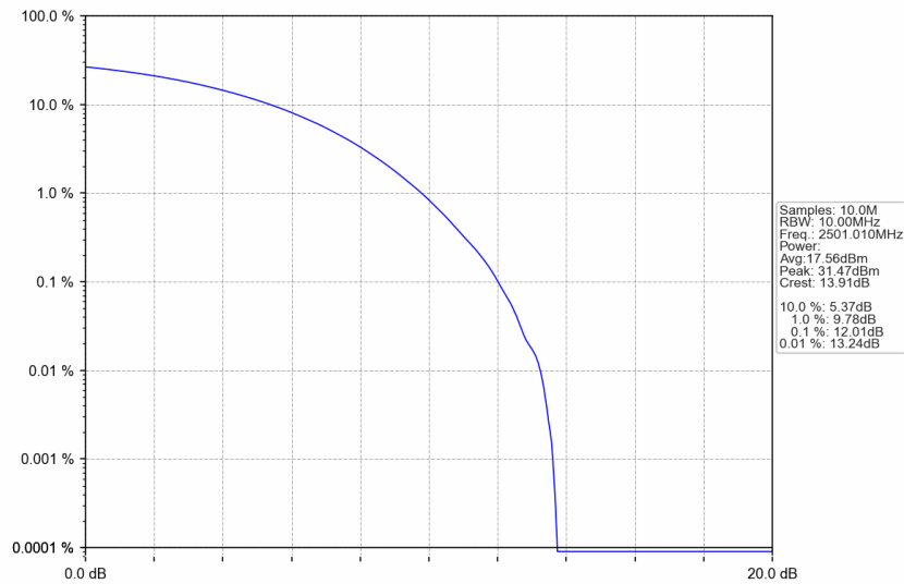
n41_30kHz_SISO_NTNV_10MHz_CP-OFDM 16 QAM_2501.01MHz_Outer_Full
