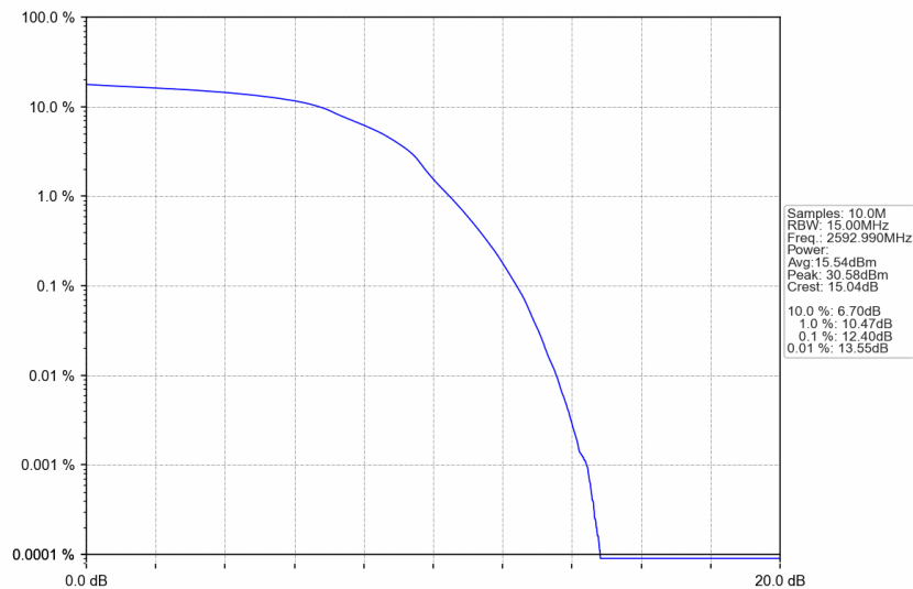
n41_30kHz_SISO_NTNV_15MHz_DFT-s-OFDM 16 QAM_2592.99MHz_Outer_Full
