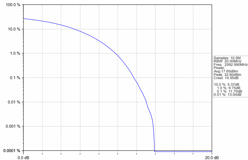
n41_30kHz_SISO_NTNV_25MHz_CP-OFDM 16 QAM_2592.99MHz_Outer_Full
