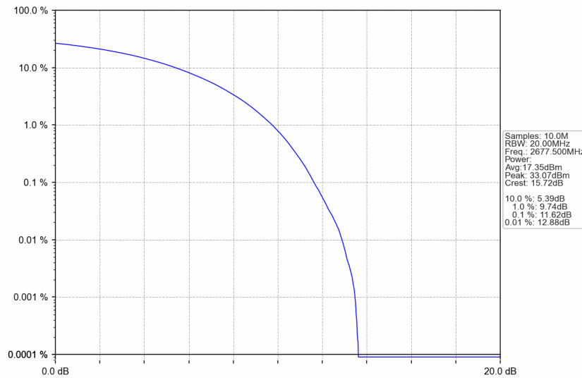
n41_30kHz_SISO_NTNV_25MHz_CP-OFDM 16 QAM_2677.5MHz_Outer_Full
