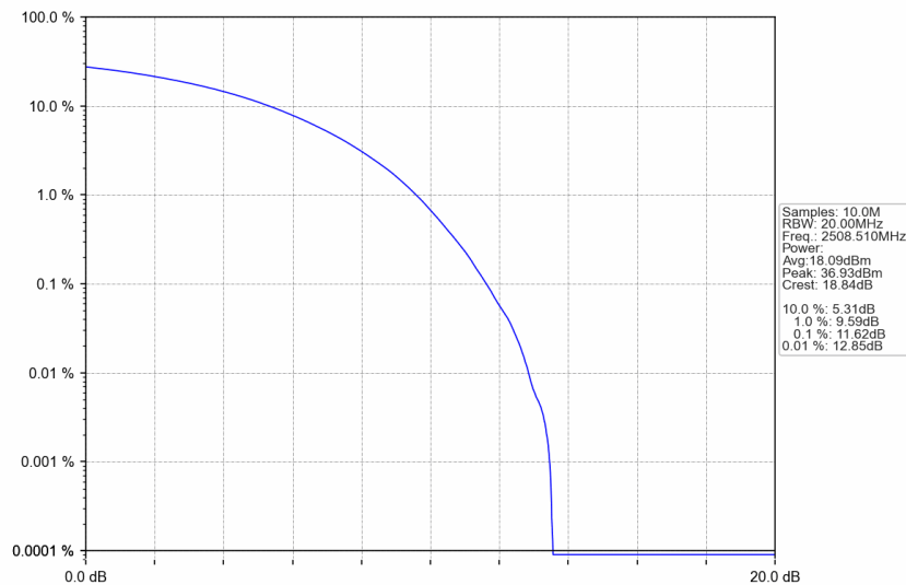
n41_30kHz_SISO_NTNV_25MHz_CP-OFDM QPSK_2508.51MHz_Outer_Full
