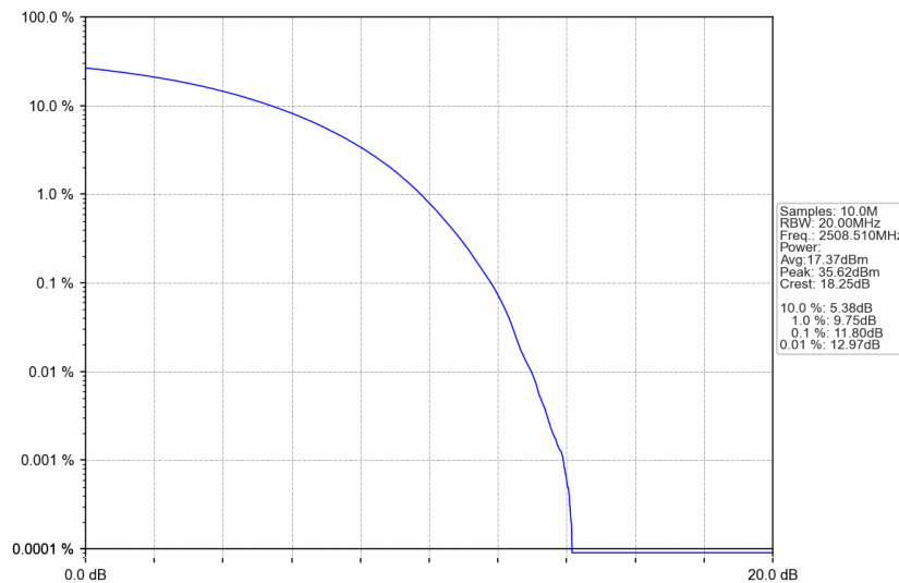
n41_30kHz_SISO_NTNV_25MHz_CP-OFDM 64 QAM_2508.51MHz_Outer_Full
