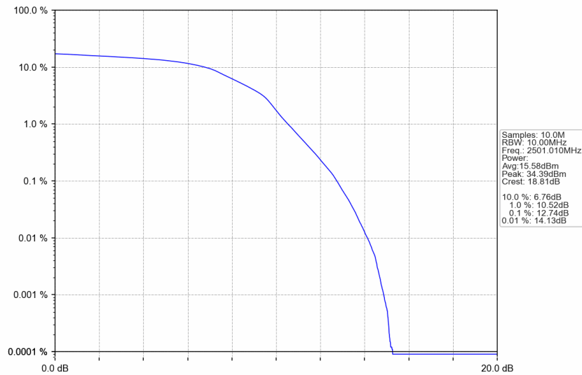
n41_30kHz_SISO_NTNV_10MHz_DFT-s-OFDM 16 QAM_2501.01MHz_Outer_Full
