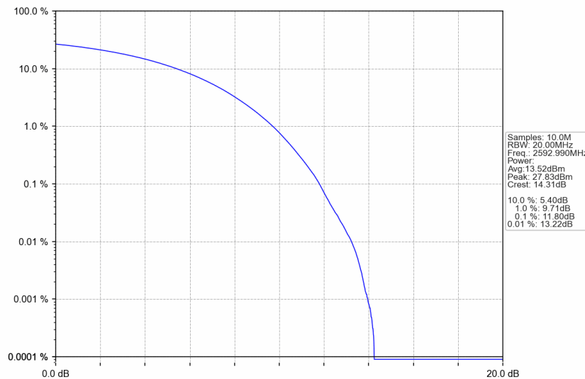
n41_30kHz_SISO_NTNV_30MHz_CP-OFDM 256 QAM_2592.99MHz_Outer_Full
