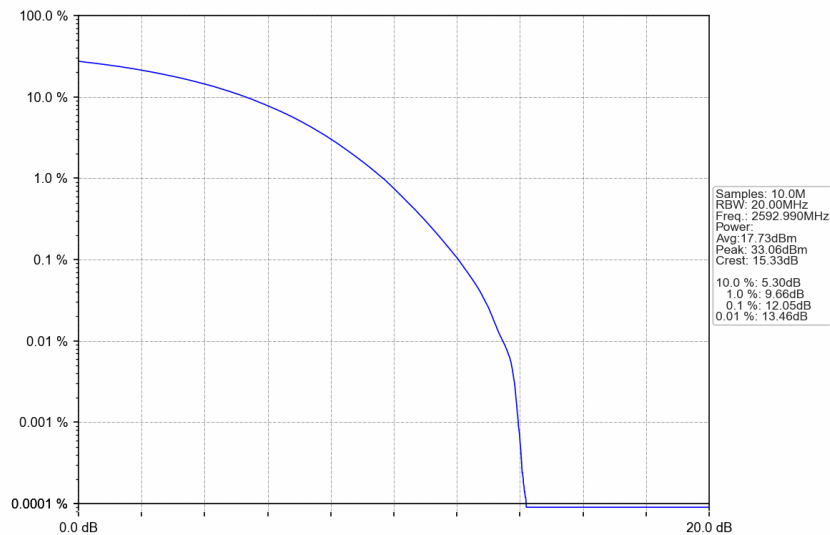
n41_30kHz_SISO_NTNV_20MHz_CP-OFDM 16 QAM_2592.99MHz_Outer_Full
