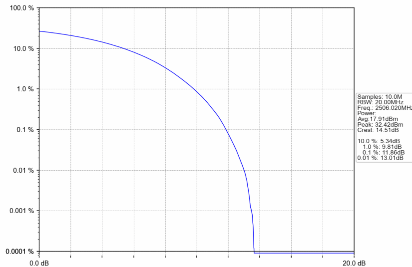
n41_30kHz_SISO_NTNV_20MHz_CP-OFDM QPSK_2506.02MHz_Outer_Full
