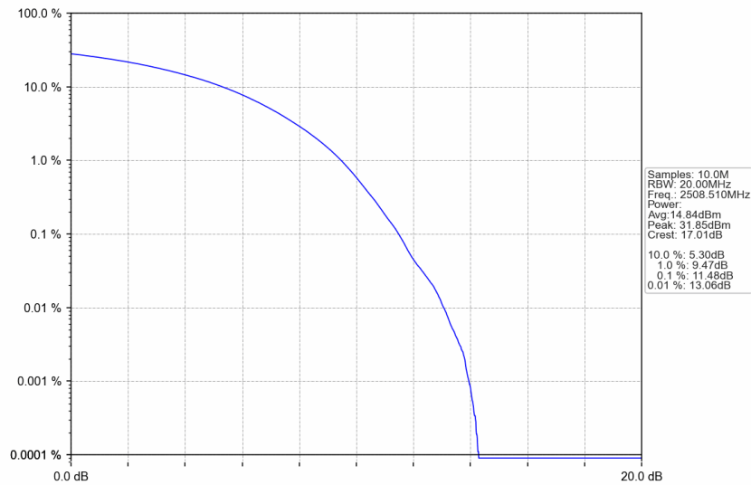
n41_30kHz_SISO_NTNV_25MHz_CP-OFDM 256 QAM_2508.51MHz_Outer_Full
