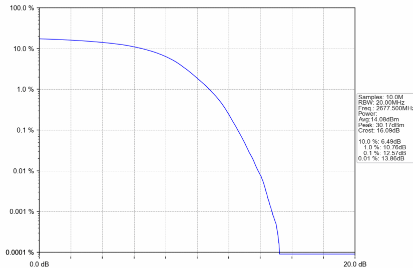
n41_30kHz_SISO_NTNV_25MHz_DFT-s-OFDM 64 QAM_2677.5MHz_Outer_Full
