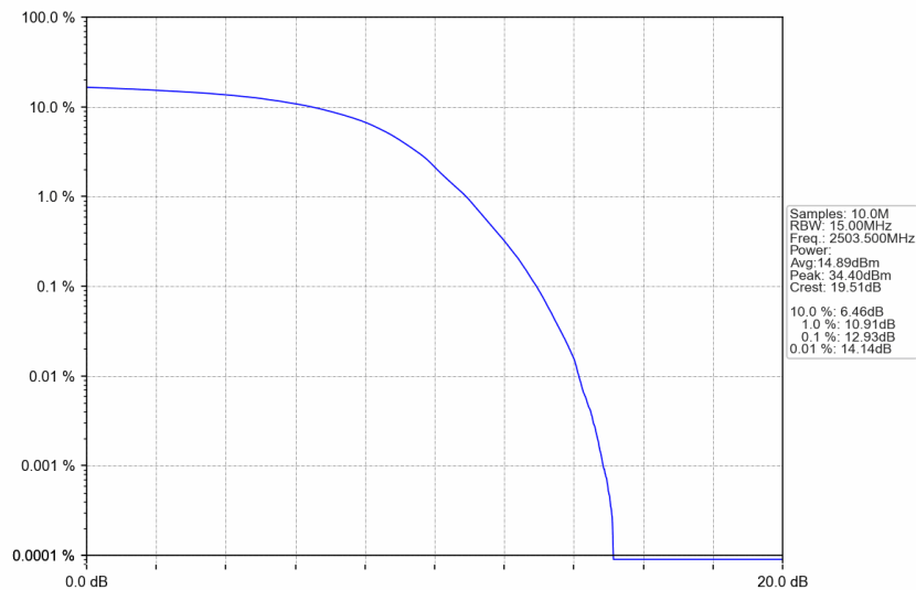
n41_30kHz_SISO_NTNV_15MHz_DFT-s-OFDM 64 QAM_2503.5MHz_Outer_Full
