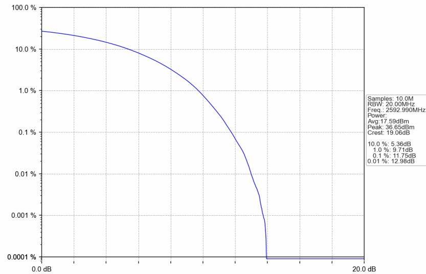
n41_30kHz_SISO_NTNV_25MHz_CP-OFDM QPSK_2592.99MHz_Outer_Full
