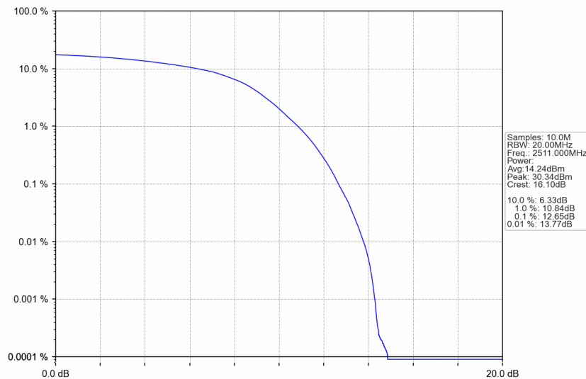
n41_30kHz_SISO_NTNV_30MHz_DFT-s-OFDM 64 QAM_2511MHz_Outer_Full
