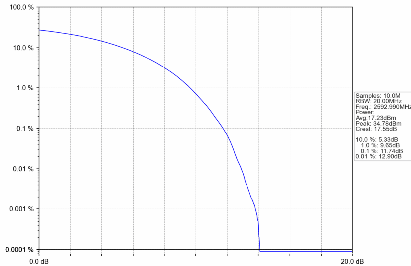
n41_30kHz_SISO_NTNV_25MHz_CP-OFDM 64 QAM_2592.99MHz_Outer_Full
