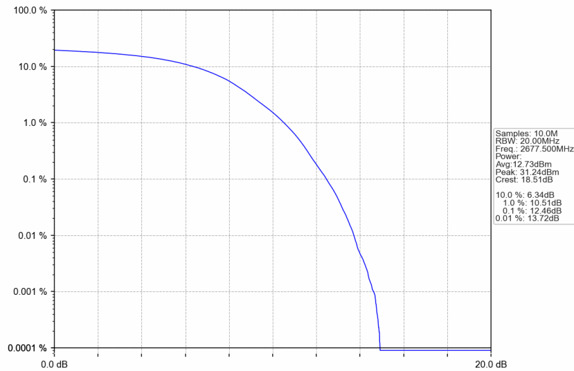
n41_30kHz_SISO_NTNV_25MHz_DFT-s-OFDM 256 QAM_2677.5MHz_Outer_Full
