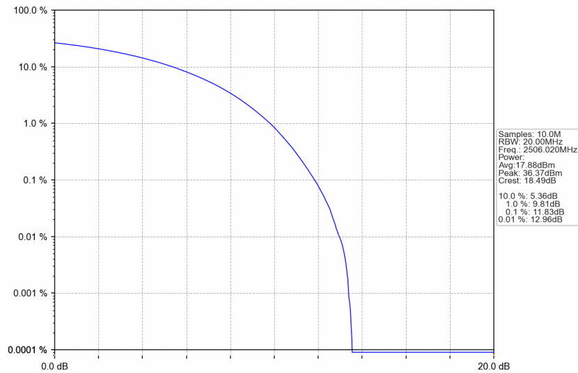
n41_30kHz_SISO_NTNV_20MHz_CP-OFDM 16 QAM_2506.02MHz_Outer_Full
