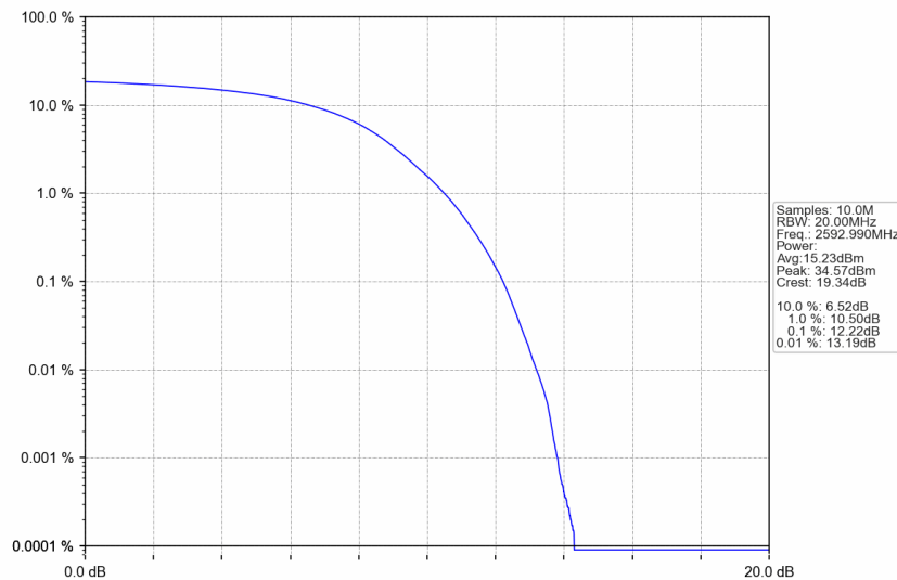
n41_30kHz_SISO_NTNV_25MHz_DFT-s-OFDM 16 QAM_2592.99MHz_Outer_Full
