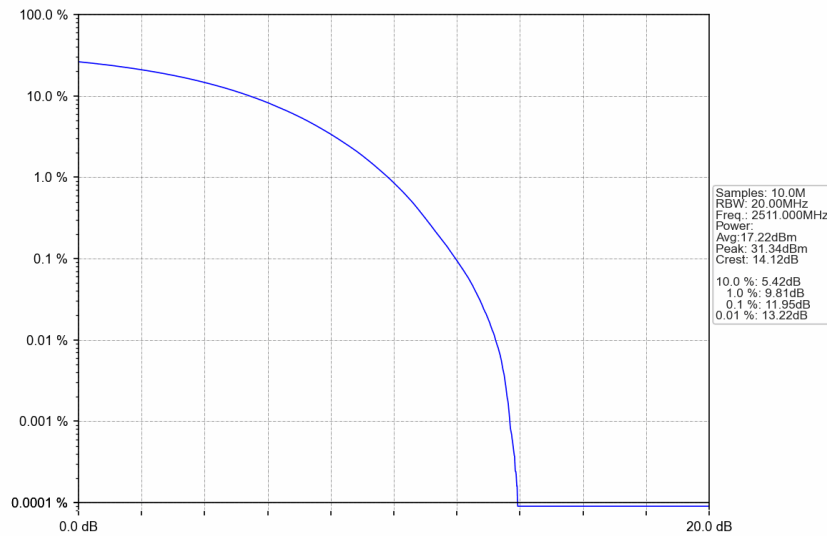
n41_30kHz_SISO_NTNV_30MHz_CP-OFDM 16 QAM_2511MHz_Outer_Full
