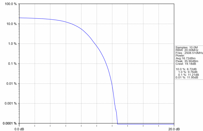
n41_30kHz_SISO_NTNV_25MHz_DFT-s-OFDM QPSK_2508.51MHz_Outer_Full
