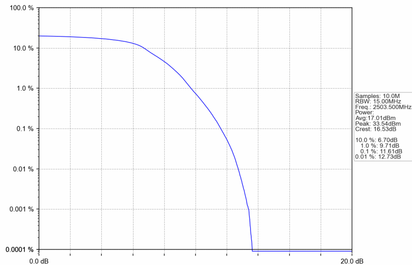
n41_30kHz_SISO_NTNV_15MHz_DFT-s-OFDM QPSK_2503.5MHz_Outer_Full
