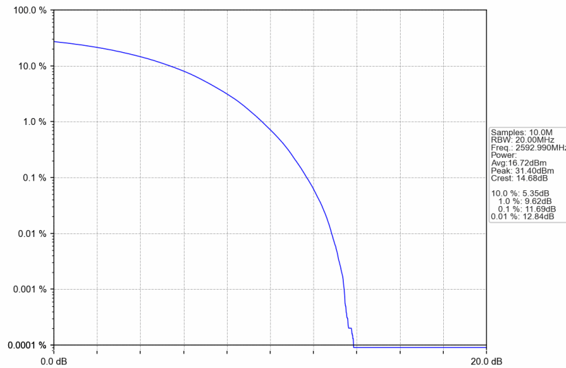
n41_30kHz_SISO_NTNV_30MHz_CP-OFDM 64 QAM_2592.99MHz_Outer_Full
