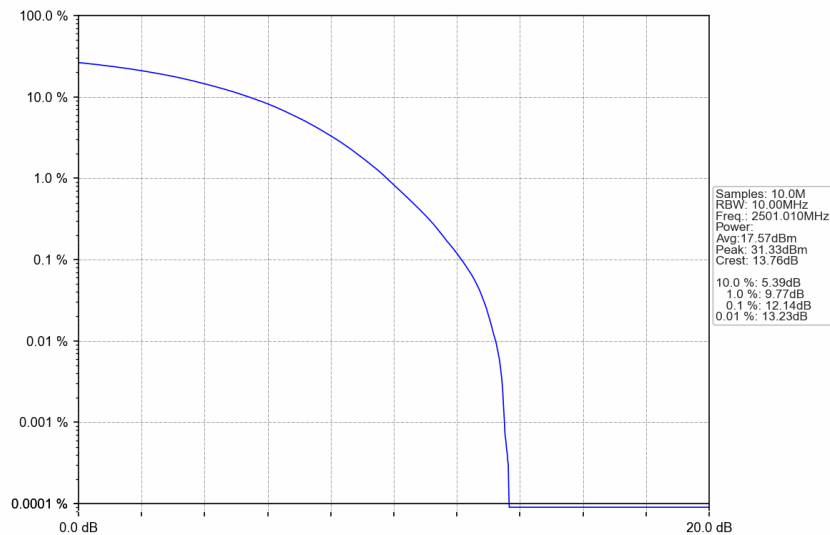
n41_30kHz_SISO_NTNV_10MHz_CP-OFDM QPSK_2501.01MHz_Outer_Full
