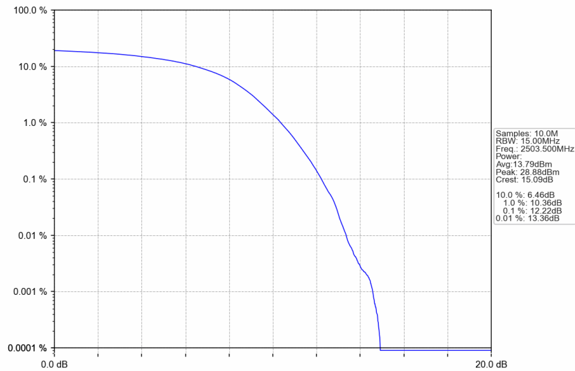
n41_30kHz_SISO_NTNV_15MHz_DFT-s-OFDM 256 QAM_2503.5MHz_Outer_Full
