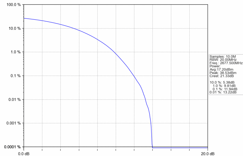
n41_30kHz_SISO_NTNV_25MHz_CP-OFDM QPSK_2677.5MHz_Outer_Full
