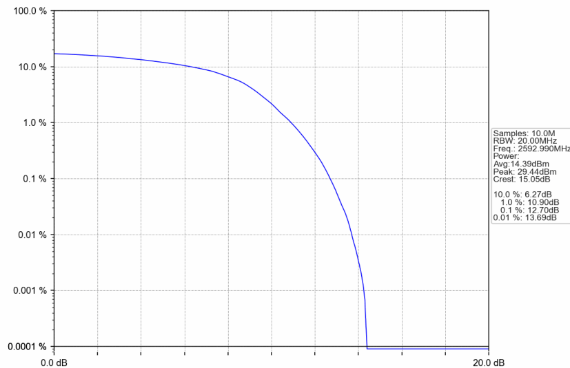
n41_30kHz_SISO_NTNV_30MHz_DFT-s-OFDM 16 QAM_2592.99MHz_Outer_Full
