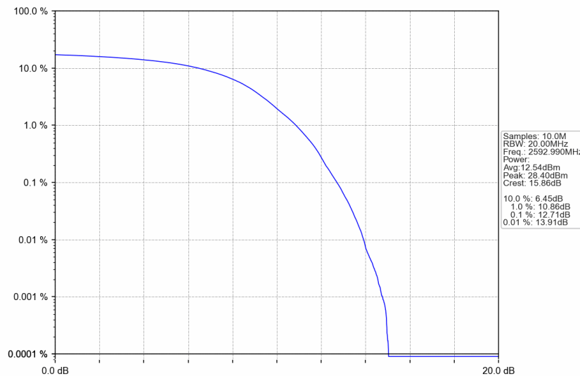
n41_30kHz_SISO_NTNV_25MHz_DFT-s-OFDM 256 QAM_2592.99MHz_Outer_Full
