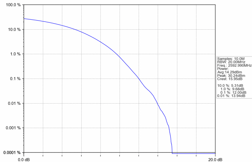
n41_30kHz_SISO_NTNV_25MHz_CP-OFDM 256 QAM_2592.99MHz_Outer_Full
