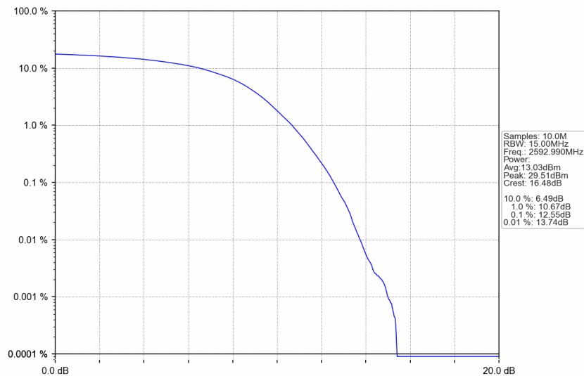
n41_30kHz_SISO_NTNV_15MHz_DFT-s-OFDM 256 QAM_2592.99MHz_Outer_Full
