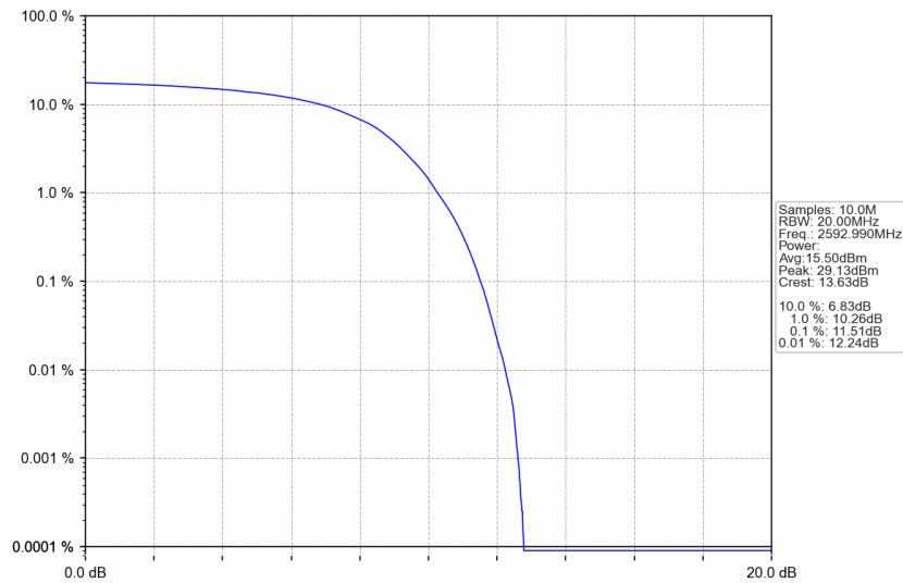
n41_30kHz_SISO_NTNV_30MHz_DFT-s-OFDM QPSK_2592.99MHz_Outer_Full
