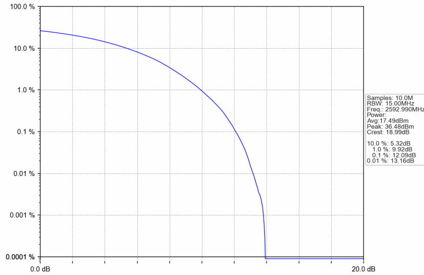
n41_30kHz_SISO_NTNV_15MHz_CP-OFDM QPSK_2592.99MHz_Outer_Full
