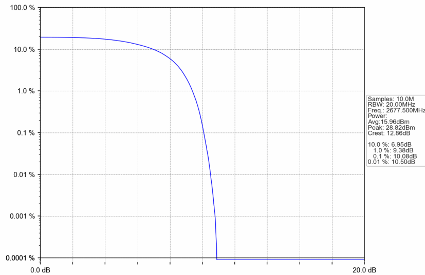
n41_30kHz_SISO_NTNV_25MHz_DFT-s-OFDM PI/2 BPSK_2677.5MHz_Outer_Full
