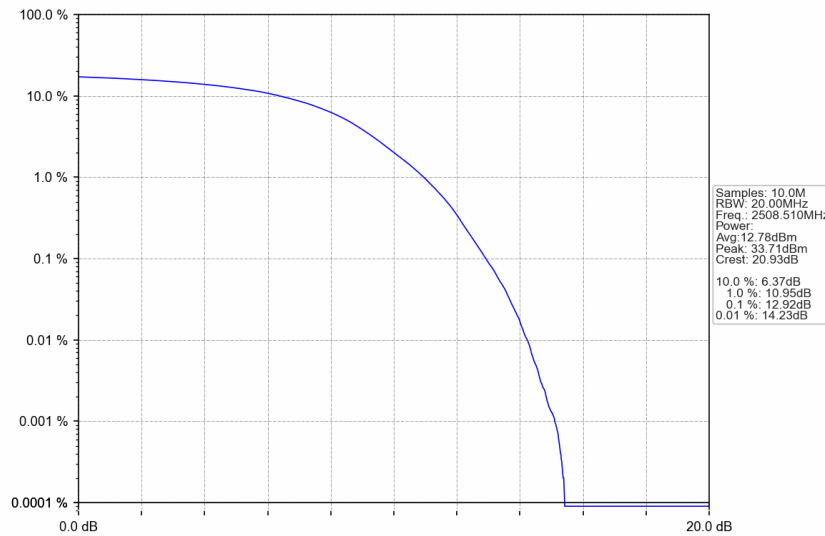
n41_30kHz_SISO_NTNV_25MHz_DFT-s-OFDM 256 QAM_2508.51MHz_Outer_Full
