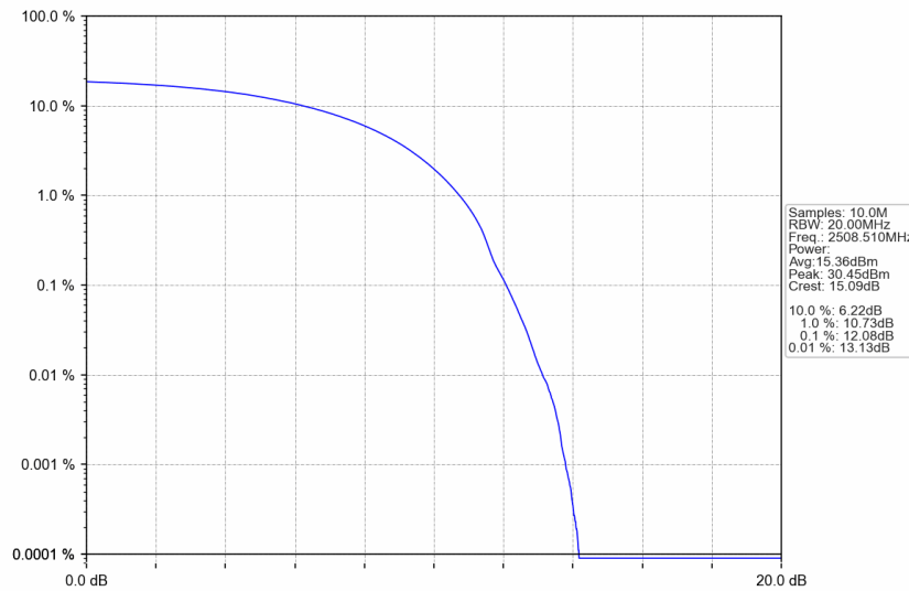
n41_15kHz_SISO_NTNV_25MHz_DFT-s-OFDM 16 QAM_2508.51MHz_Outer_Full
