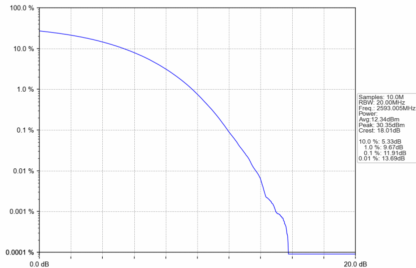
n41_15kHz_SISO_NTNV_40MHz_CP-OFDM 256 QAM_2593.005MHz_Outer_Full
