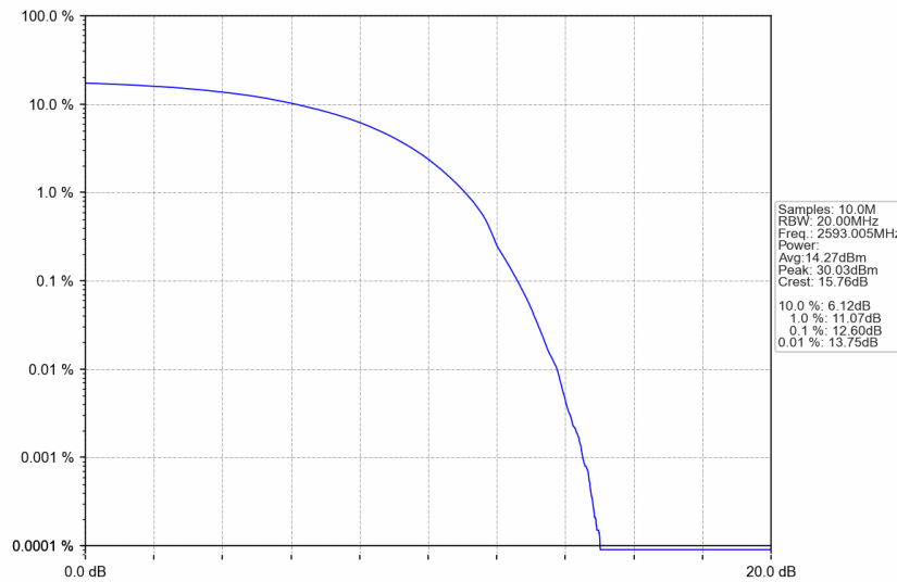
n41_15kHz_SISO_NTNV_25MHz_DFT-s-OFDM 64 QAM_2593.005MHz_Outer_Full
