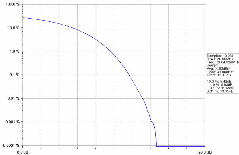
n41_15kHz_SISO_NTNV_50MHz_CP-OFDM 16 QAM_2664.99MHz_Outer_Full
