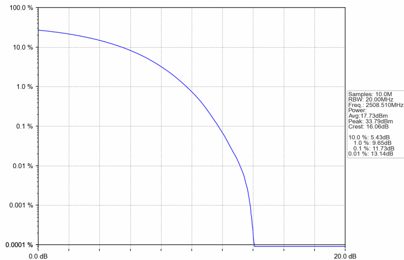
n41_15kHz_SISO_NTNV_25MHz_CP-OFDM QPSK_2508.51MHz_Outer_Full
