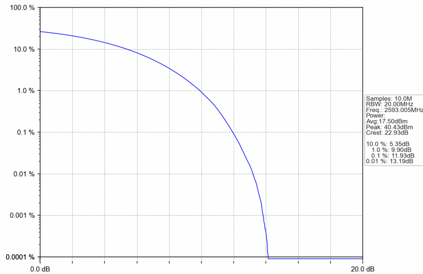
n41_15kHz_SISO_NTNV_25MHz_CP-OFDM QPSK_2593.005MHz_Outer_Full
