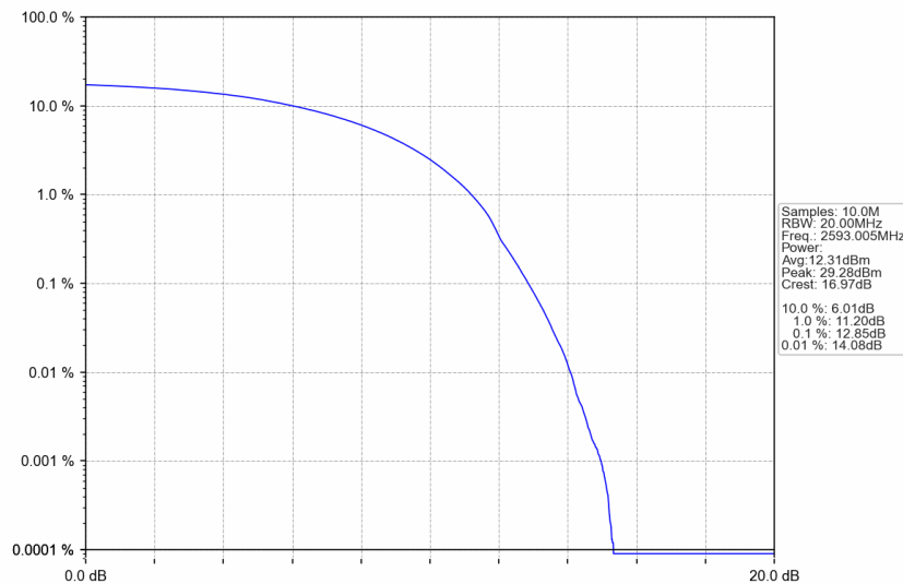
n41_15kHz_SISO_NTNV_25MHz_DFT-s-OFDM 256 QAM_2593.005MHz_Outer_Full
