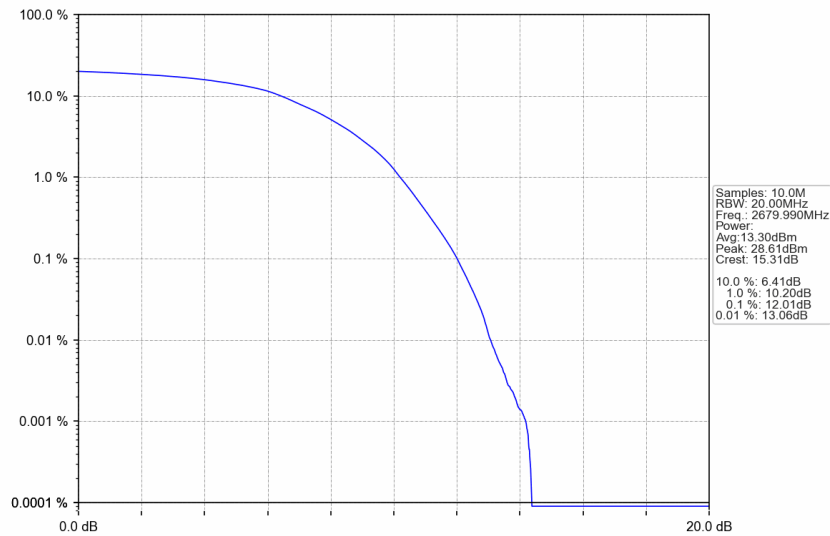
n41_15kHz_SISO_NTNV_20MHz_DFT-s-OFDM 256 QAM_2679.99MHz_Outer_Full
