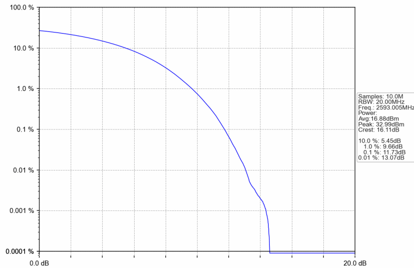
n41_15kHz_SISO_NTNV_30MHz_CP-OFDM QPSK_2593.005MHz_Outer_Full
