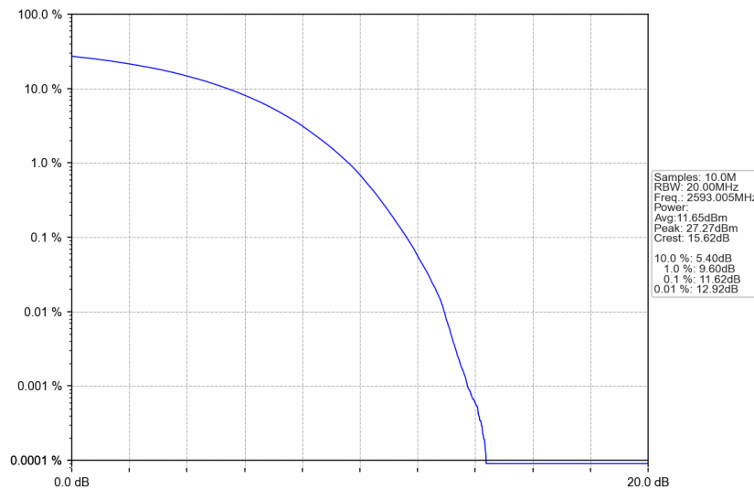
n41_15kHz_SISO_NTNV_50MHz_CP-OFDM 256 QAM_2593.005MHz_Outer_Full
