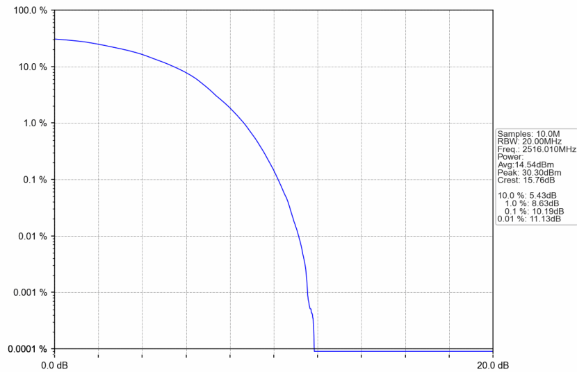
n41_15kHz_SISO_NTNV_40MHz_DFT-s-OFDM 256 QAM_2516.01MHz_Outer_Full
