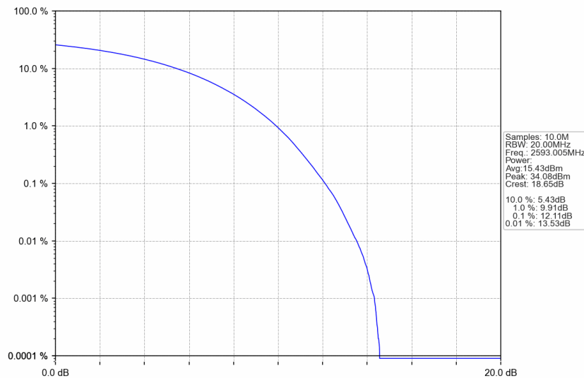
n41_15kHz_SISO_NTNV_40MHz_CP-OFDM 16 QAM_2593.005MHz_Outer_Full
