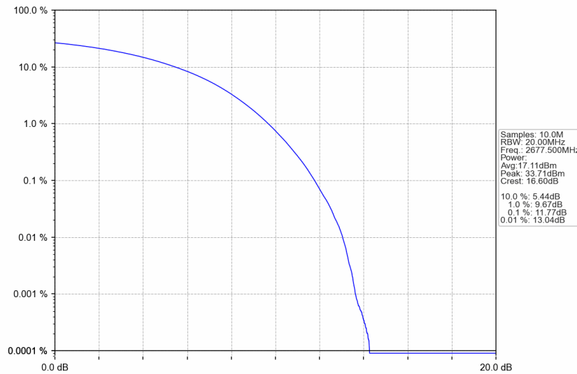
n41_15kHz_SISO_NTNV_25MHz_CP-OFDM 16 QAM_2677.5MHz_Outer_Full
