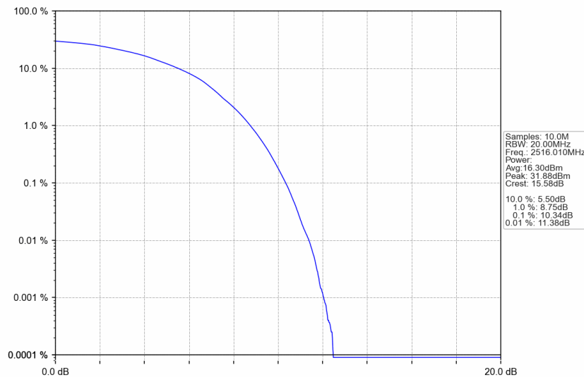
n41_15kHz_SISO_NTNV_40MHz_DFT-s-OFDM 64 QAM_2516.01MHz_Outer_Full
