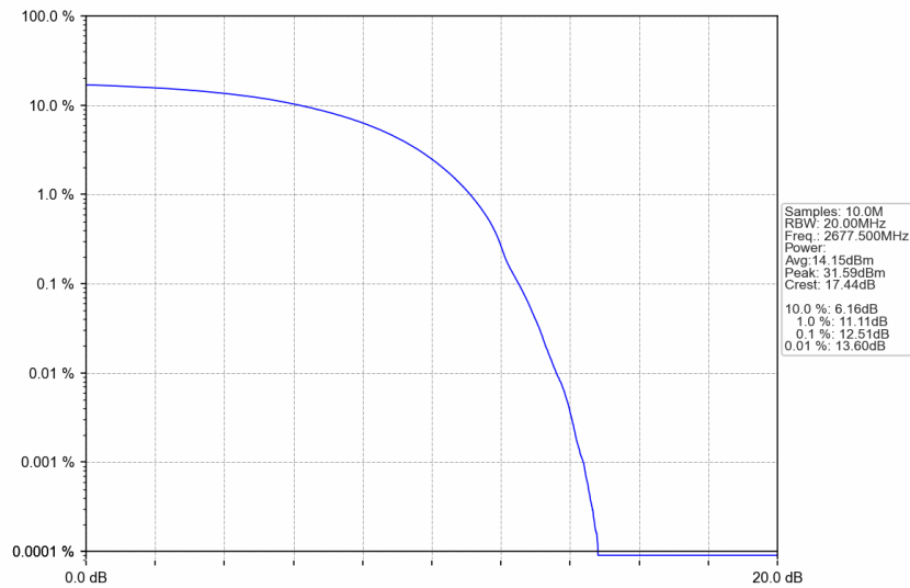
n41_15kHz_SISO_NTNV_25MHz_DFT-s-OFDM 16 QAM_2677.5MHz_Outer_Full
