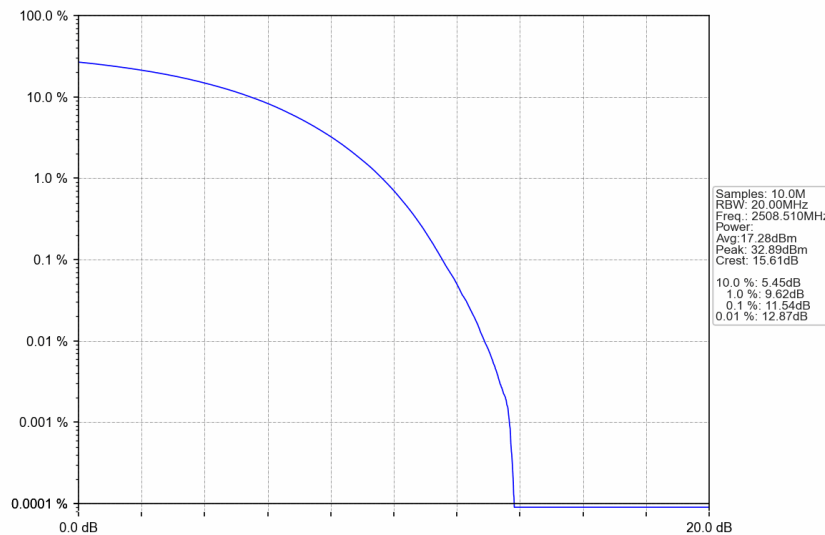
n41_15kHz_SISO_NTNV_25MHz_CP-OFDM 64 QAM_2508.51MHz_Outer_Full
