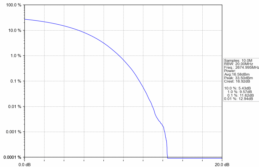
n41_15kHz_SISO_NTNV_30MHz_CP-OFDM QPSK_2674.995MHz_Outer_Full
