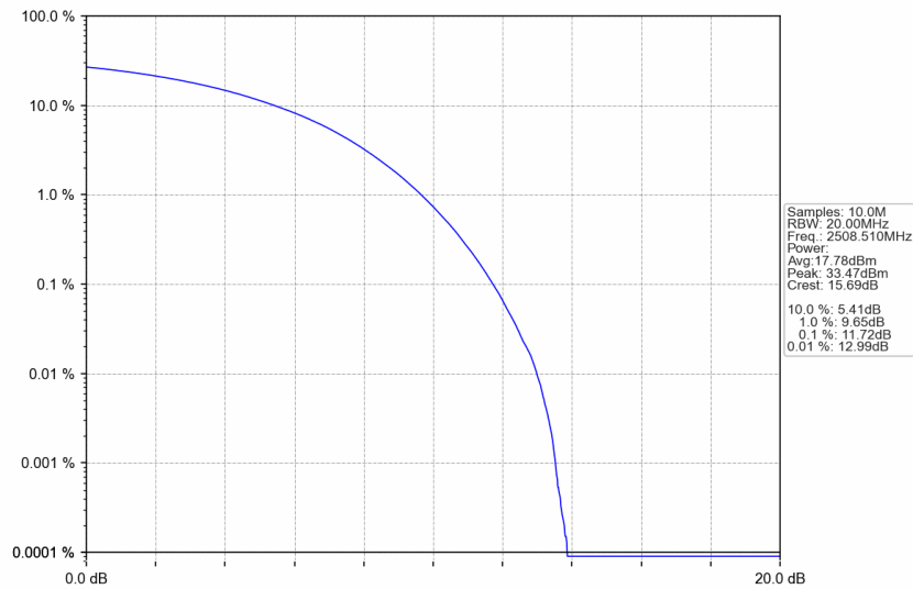
n41_15kHz_SISO_NTNV_25MHz_CP-OFDM 16 QAM_2508.51MHz_Outer_Full
