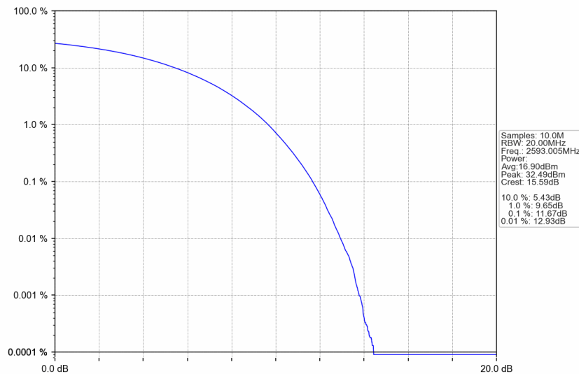
n41_15kHz_SISO_NTNV_30MHz_CP-OFDM 16 QAM_2593.005MHz_Outer_Full
