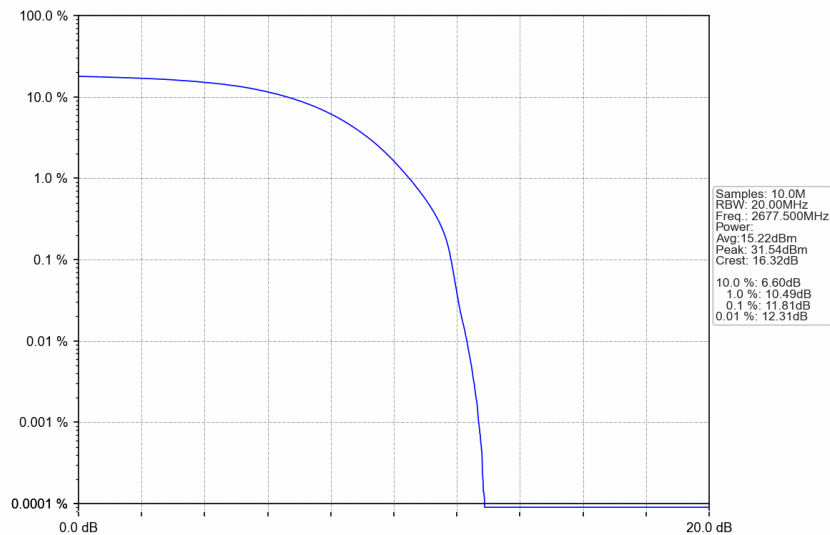
n41_15kHz_SISO_NTNV_25MHz_DFT-s-OFDM QPSK_2677.5MHz_Outer_Full
