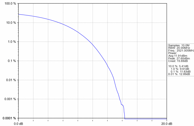
n41_15kHz_SISO_NTNV_50MHz_CP-OFDM 256 QAM_2521.005MHz_Outer_Full
