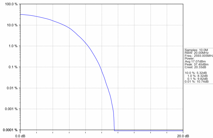
n41_15kHz_SISO_NTNV_40MHz_DFT-s-OFDM 16 QAM_2593.005MHz_Outer_Full
