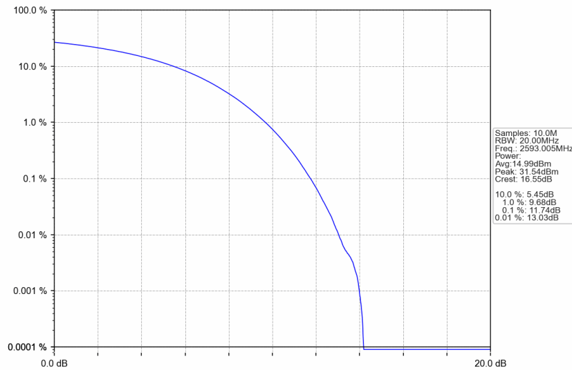
n41_15kHz_SISO_NTNV_50MHz_CP-OFDM QPSK_2593.005MHz_Outer_Full
