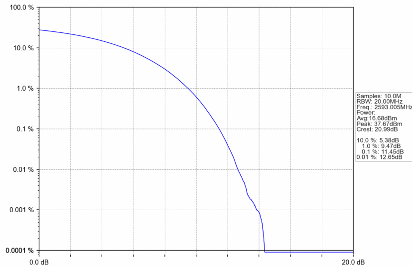
n41_15kHz_SISO_NTNV_30MHz_CP-OFDM 64 QAM_2593.005MHz_Outer_Full
