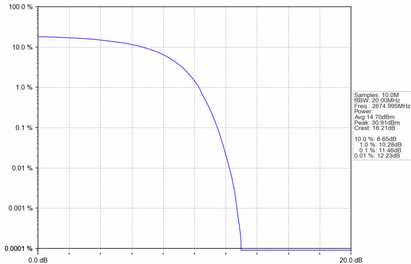
n41_15kHz_SISO_NTNV_30MHz_DFT-s-OFDM QPSK_2674.995MHz_Outer_Full
