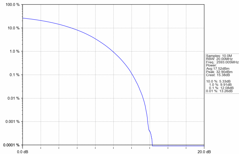
n41_15kHz_SISO_NTNV_25MHz_CP-OFDM 16 QAM_2593.005MHz_Outer_Full
