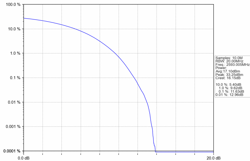
n41_15kHz_SISO_NTNV_20MHz_CP-OFDM 64 QAM_2593.005MHz_Outer_Full
