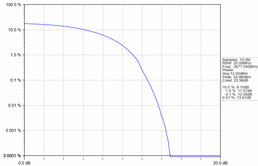
n41_15kHz_SISO_NTNV_25MHz_DFT-s-OFDM 256 QAM_2677.5MHz_Outer_Full
