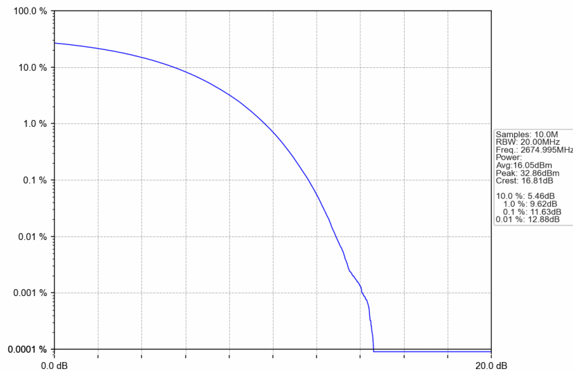
n41_15kHz_SISO_NTNV_30MHz_CP-OFDM 64 QAM_2674.995MHz_Outer_Full
