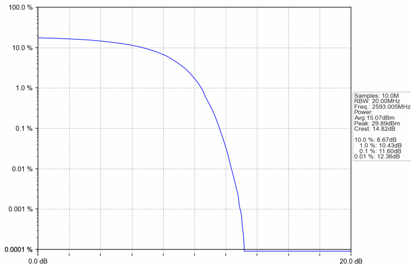
n41_15kHz_SISO_NTNV_30MHz_DFT-s-OFDM QPSK_2593.005MHz_Outer_Full
