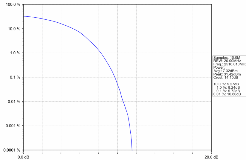
n41_15kHz_SISO_NTNV_40MHz_DFT-s-OFDM 16 QAM_2516.01MHz_Outer_Full
