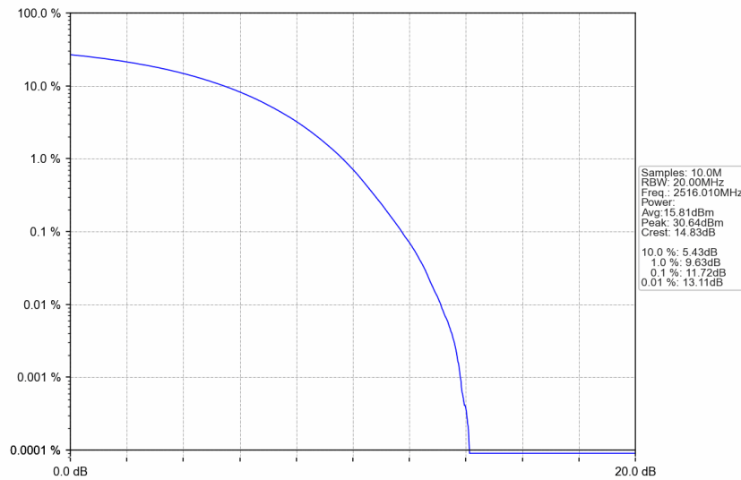
n41_15kHz_SISO_NTNV_40MHz_CP-OFDM 16 QAM_2516.01MHz_Outer_Full
