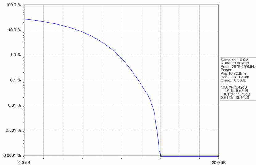
n41_15kHz_SISO_NTNV_20MHz_CP-OFDM 64 QAM_2679.99MHz_Outer_Full
