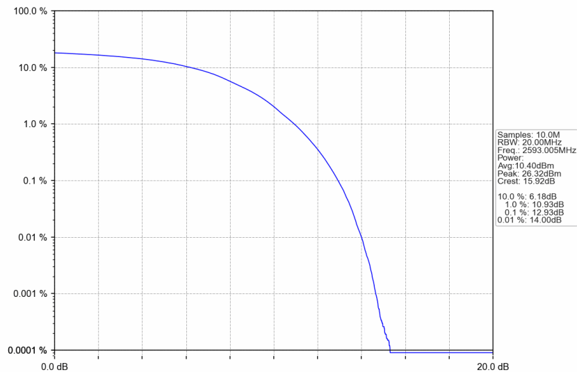
n41_15kHz_SISO_NTNV_40MHz_DFT-s-OFDM 256 QAM_2593.005MHz_Outer_Full
