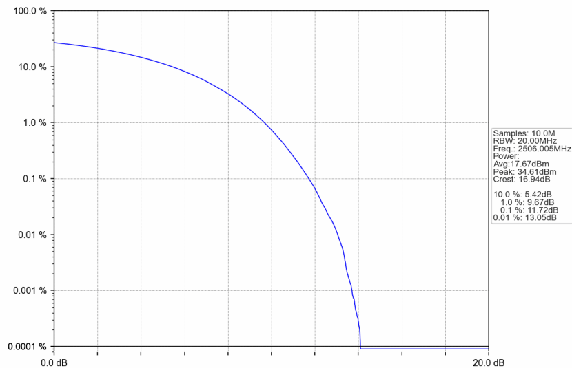
n41_15kHz_SISO_NTNV_20MHz_CP-OFDM QPSK_2506.005MHz_Outer_Full
