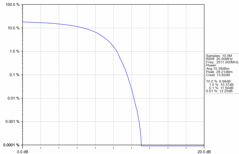
n41_15kHz_SISO_NTNV_30MHz_DFT-s-OFDM QPSK_2511MHz_Outer_Full
