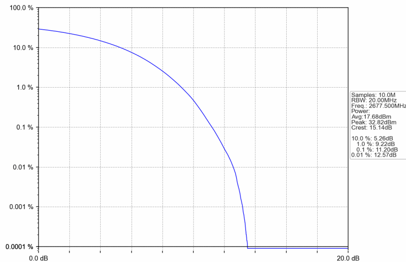
n41_15kHz_SISO_NTNV_25MHz_CP-OFDM QPSK_2677.5MHz_Outer_Full
