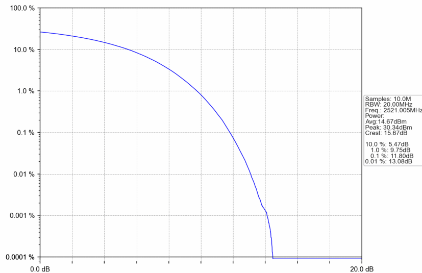
n41_15kHz_SISO_NTNV_50MHz_CP-OFDM 64 QAM_2521.005MHz_Outer_Full
