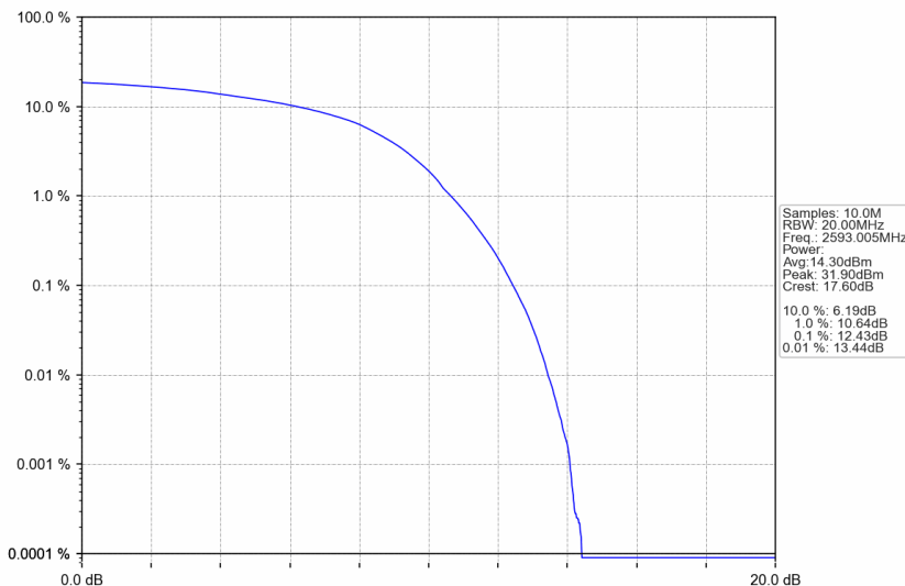
n41_15kHz_SISO_NTNV_30MHz_DFT-s-OFDM 16 QAM_2593.005MHz_Outer_Full
