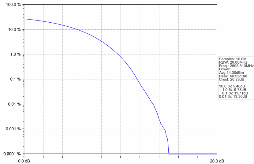
n41_15kHz_SISO_NTNV_25MHz_CP-OFDM 256 QAM_2508.51MHz_Outer_Full
