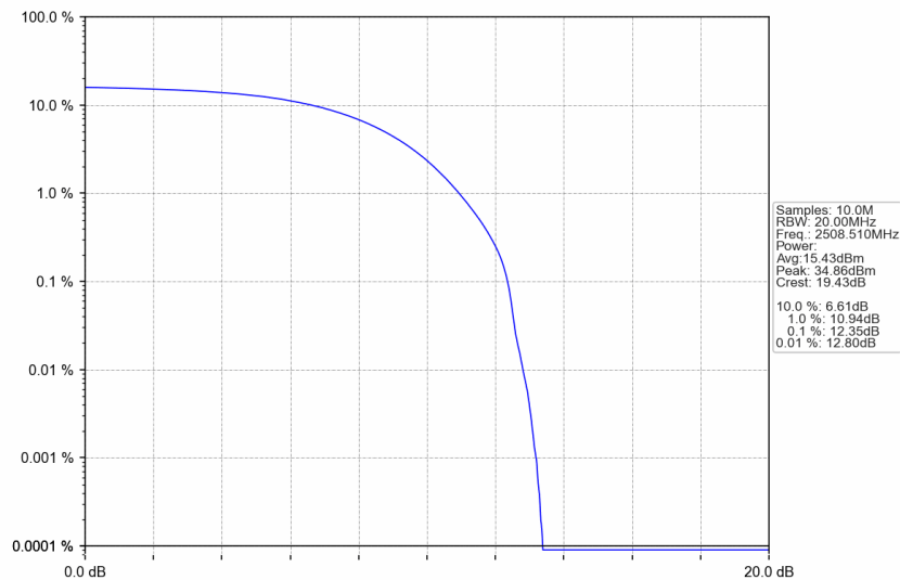
n41_15kHz_SISO_NTNV_25MHz_DFT-s-OFDM QPSK_2508.51MHz_Outer_Full
