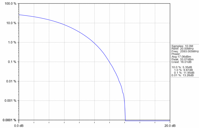
n41_15kHz_SISO_NTNV_25MHz_CP-OFDM 64 QAM_2593.005MHz_Outer_Full
