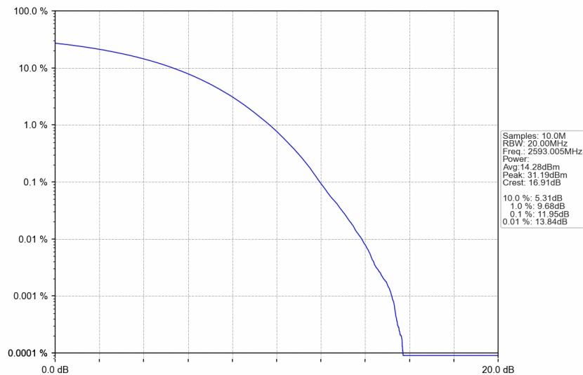
n41_15kHz_SISO_NTNV_25MHz_CP-OFDM 256 QAM_2593.005MHz_Outer_Full
