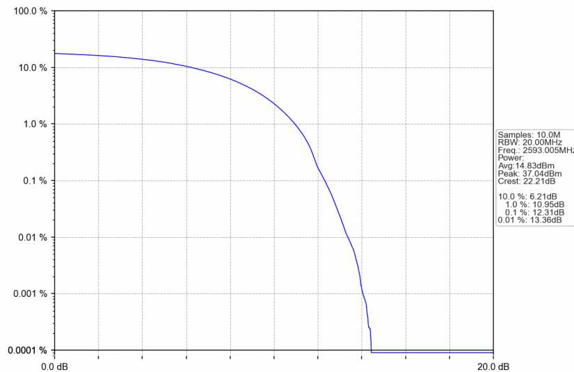
n41_15kHz_SISO_NTNV_25MHz_DFT-s-OFDM 16 QAM_2593.005MHz_Outer_Full
