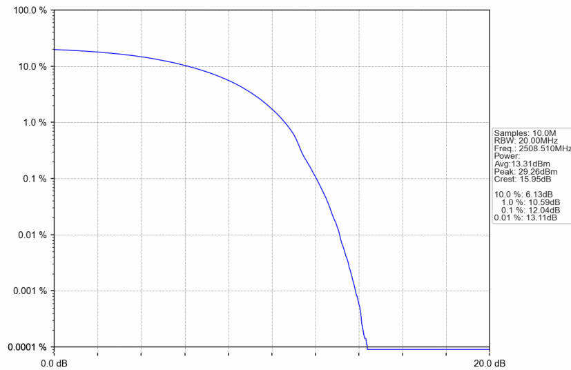
n41_15kHz_SISO_NTNV_25MHz_DFT-s-OFDM 256 QAM_2508.51MHz_Outer_Full
