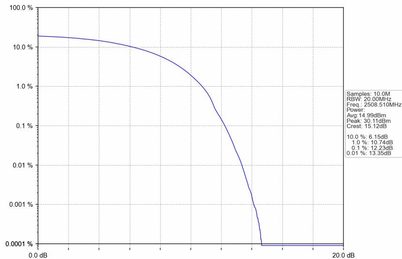
n41_15kHz_SISO_NTNV_25MHz_DFT-s-OFDM 64 QAM_2508.51MHz_Outer_Full
