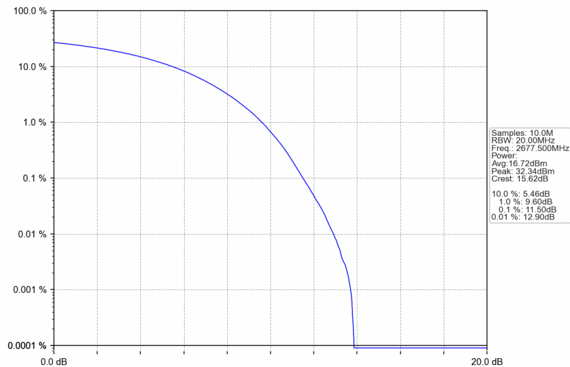
n41_15kHz_SISO_NTNV_25MHz_CP-OFDM 64 QAM_2677.5MHz_Outer_Full
