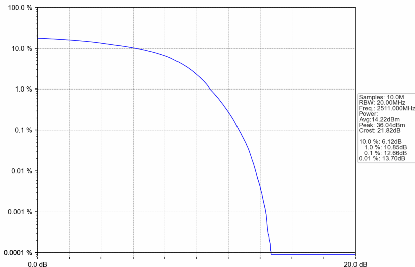
n41_15kHz_SISO_NTNV_30MHz_DFT-s-OFDM 16 QAM_2511MHz_Outer_Full
