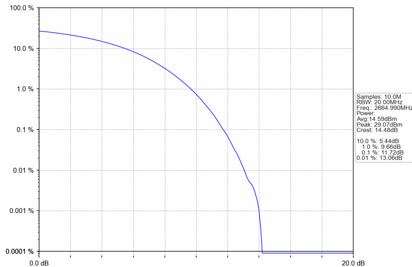
n41_15kHz_SISO_NTNV_50MHz_CP-OFDM QPSK_2664.99MHz_Outer_Full
