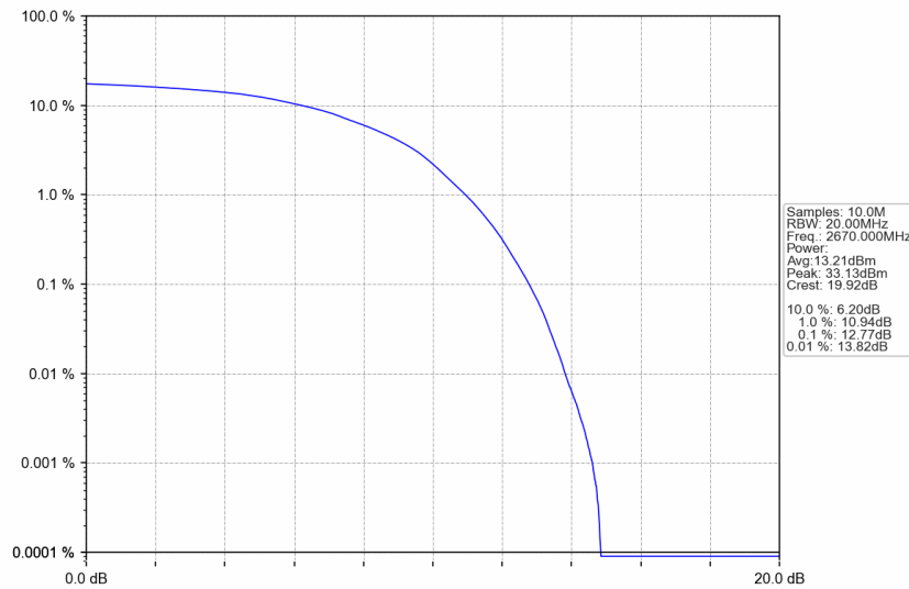
n41_15kHz_SISO_NTNV_40MHz_DFT-s-OFDM 16 QAM_2670MHz_Outer_Full
