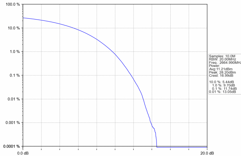
n41_15kHz_SISO_NTNV_50MHz_CP-OFDM 256 QAM_2664.99MHz_Outer_Full
