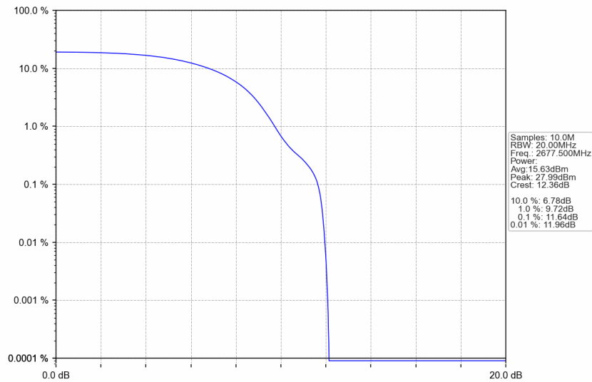
n41_15kHz_SISO_NTNV_25MHz_DFT-s-OFDM PI/2 BPSK_2677.5MHz_Outer_Full
