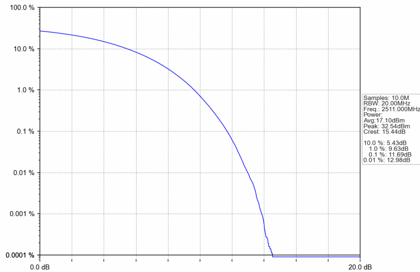
n41_15kHz_SISO_NTNV_30MHz_CP-OFDM 16 QAM_2511MHz_Outer_Full
