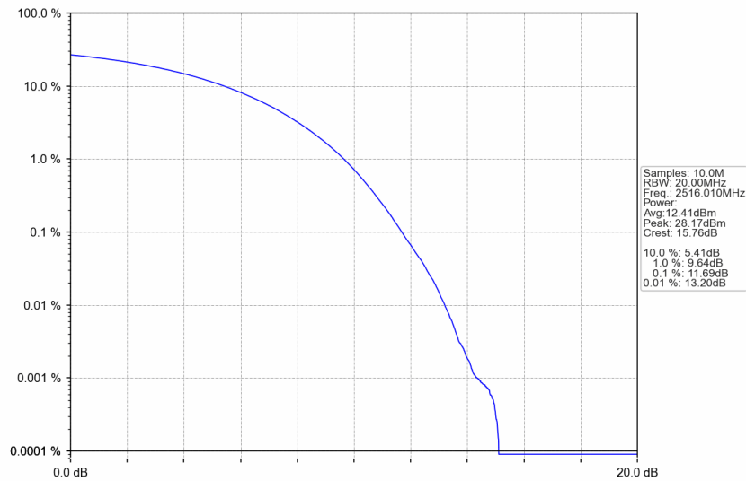
n41_15kHz_SISO_NTNV_40MHz_CP-OFDM 256 QAM_2516.01MHz_Outer_Full
