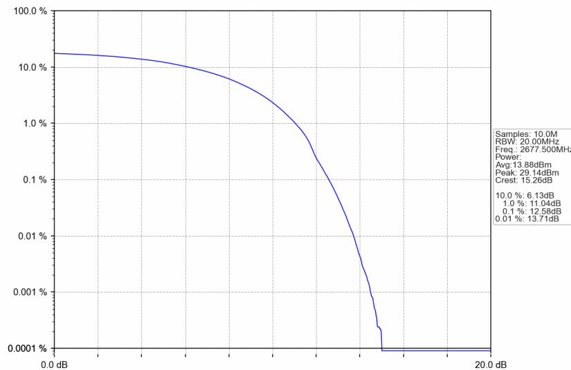
n41_15kHz_SISO_NTNV_25MHz_DFT-s-OFDM 64 QAM_2677.5MHz_Outer_Full
