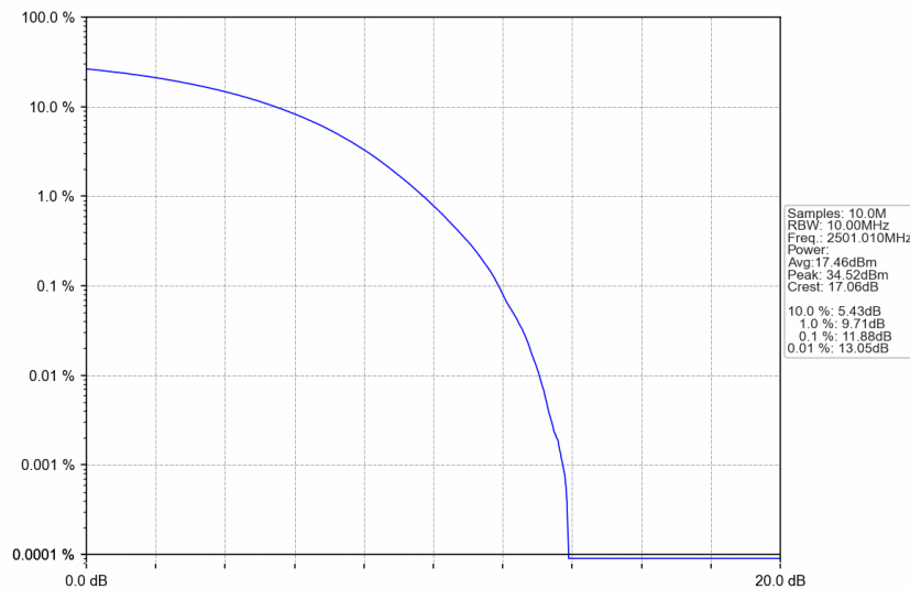
n41_15kHz_SISO_NTNV_10MHz_CP-OFDM QPSK_2501.01MHz_Outer_Full
