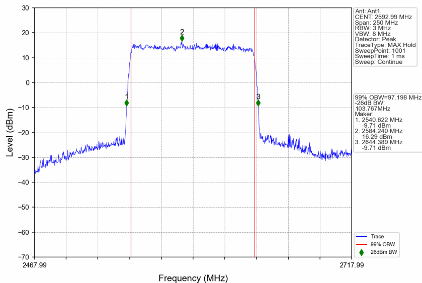
n41_30kHz_SISO_NTNV_100MHz_DFT-s-OFDM 256 QAM_2592.99MHz_Outer_Full
