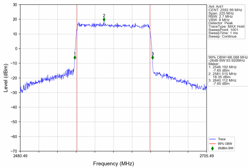
n41_30kHz_SISO_NTNV_90MHz_CP-OFDM 16 QAM_2592.99MHz_Outer_Full
