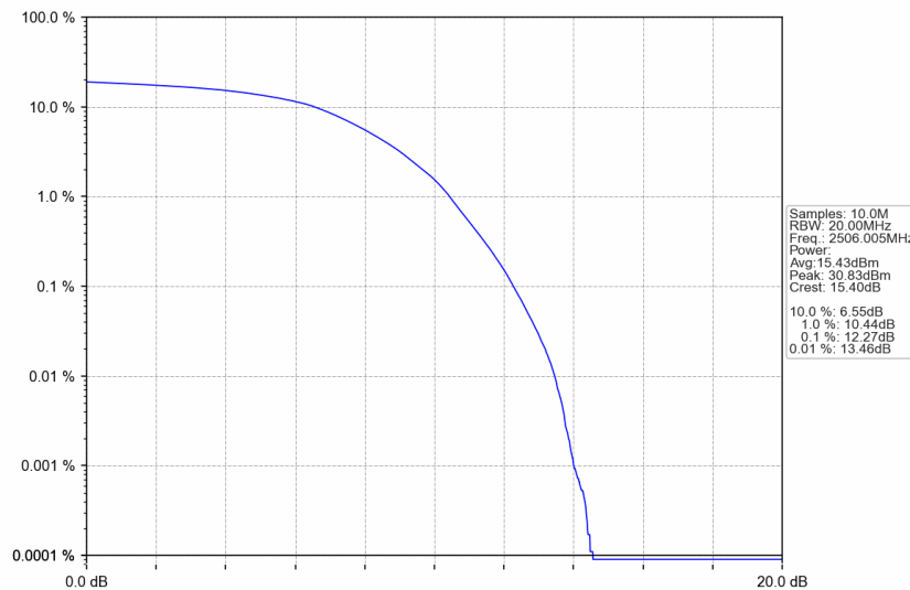
n41_15kHz_SISO_NTNV_20MHz_DFT-s-OFDM 64 QAM_2506.005MHz_Outer_Full
