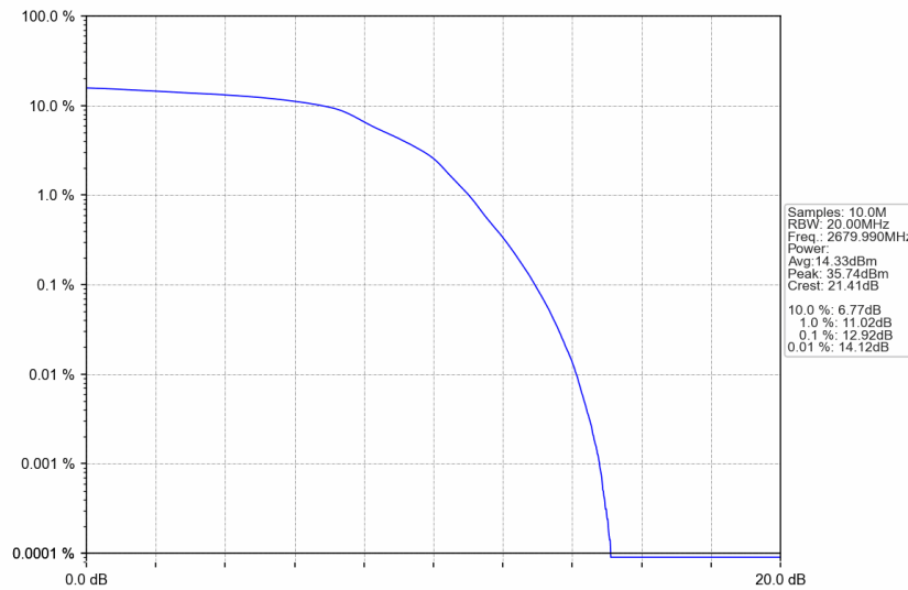
n41_15kHz_SISO_NTNV_20MHz_DFT-s-OFDM 16 QAM_2679.99MHz_Outer_Full
