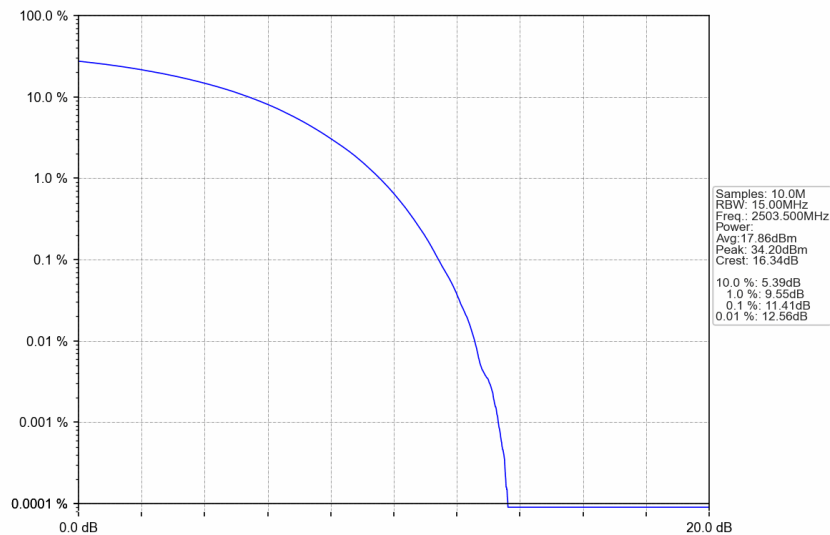
n41_15kHz_SISO_NTNV_15MHz_CP-OFDM QPSK_2503.5MHz_Outer_Full
