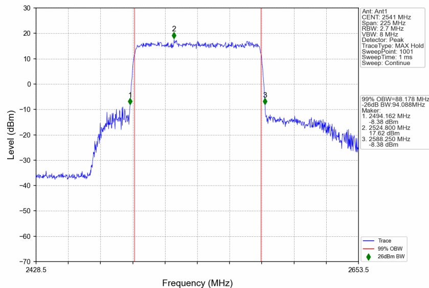
n41_30kHz_SISO_NTNV_90MHz_CP-OFDM 64 QAM_2541MHz_Outer_Full
