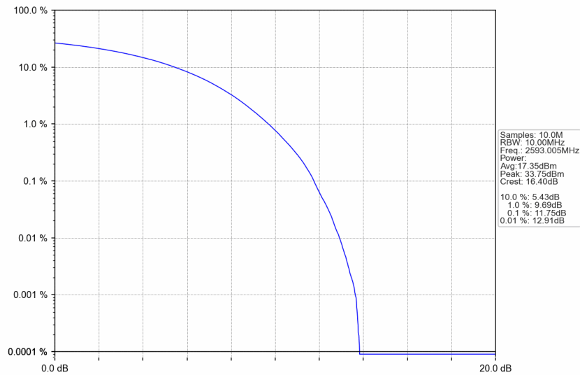
n41_15kHz_SISO_NTNV_10MHz_CP-OFDM QPSK_2593.005MHz_Outer_Full
