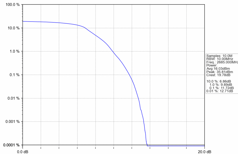
n41_15kHz_SISO_NTNV_10MHz_DFT-s-OFDM QPSK_2685MHz_Outer_Full
