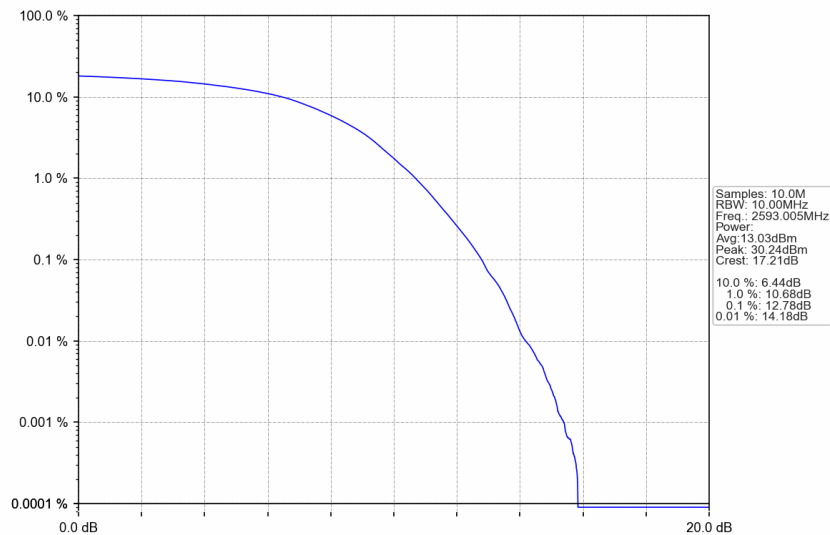
n41_15kHz_SISO_NTNV_10MHz_DFT-s-OFDM 256 QAM_2593.005MHz_Outer_Full
