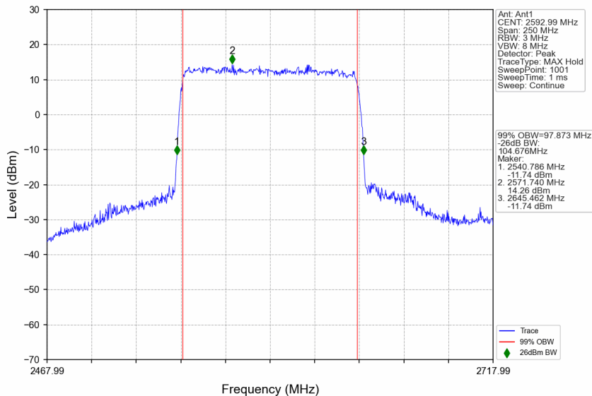
n41_30kHz_SISO_NTNV_100MHz_CP-OFDM 256 QAM_2592.99MHz_Outer_Full
