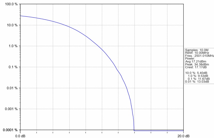
n41_15kHz_SISO_NTNV_10MHz_CP-OFDM 64 QAM_2501.01MHz_Outer_Full
