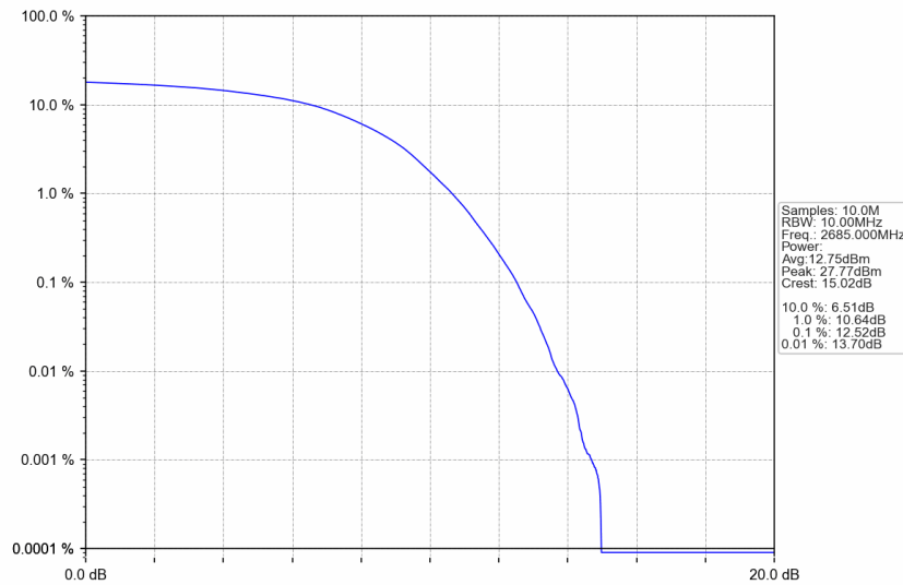
n41_15kHz_SISO_NTNV_10MHz_DFT-s-OFDM 256 QAM_2685MHz_Outer_Full
