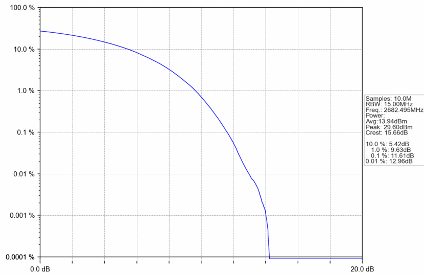
n41_15kHz_SISO_NTNV_15MHz_CP-OFDM 256 QAM_2682.495MHz_Outer_Full
