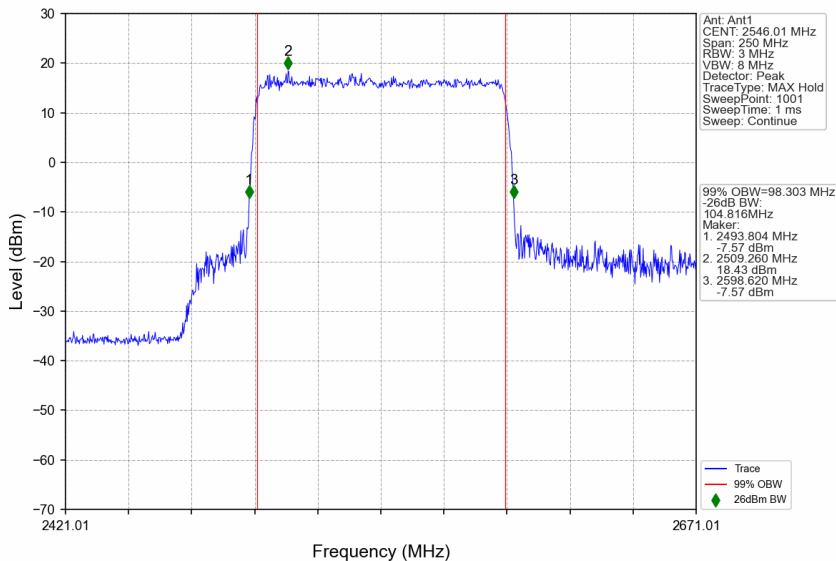
n41_30kHz_SISO_NTNV_100MHz_CP-OFDM QPSK_2546.01MHz_Outer_Full
