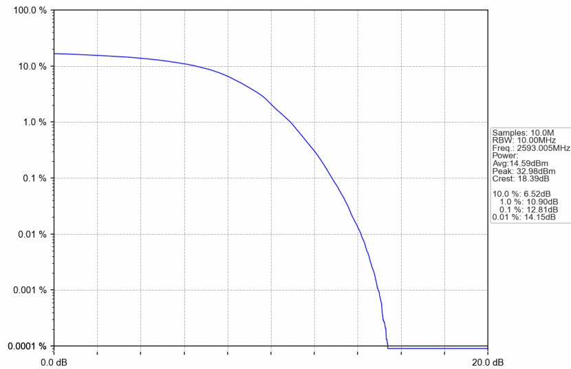
n41_15kHz_SISO_NTNV_10MHz_DFT-s-OFDM 64 QAM_2593.005MHz_Outer_Full
