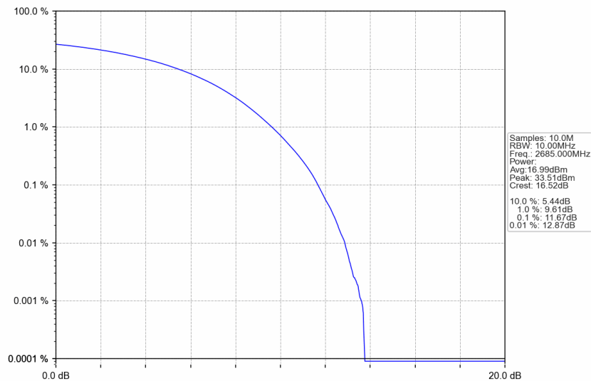
n41_15kHz_SISO_NTNV_10MHz_CP-OFDM QPSK_2685MHz_Outer_Full
