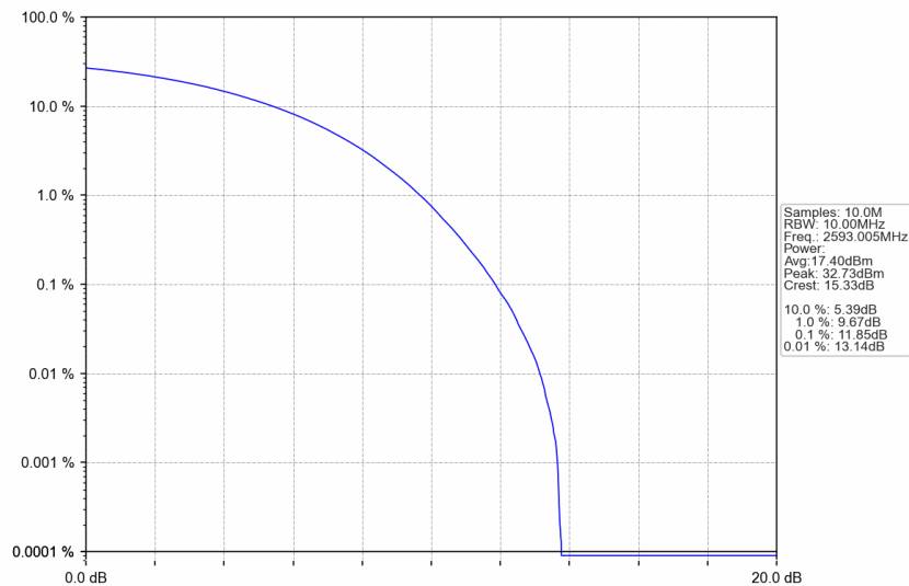
n41_15kHz_SISO_NTNV_10MHz_CP-OFDM 16 QAM_2593.005MHz_Outer_Full
