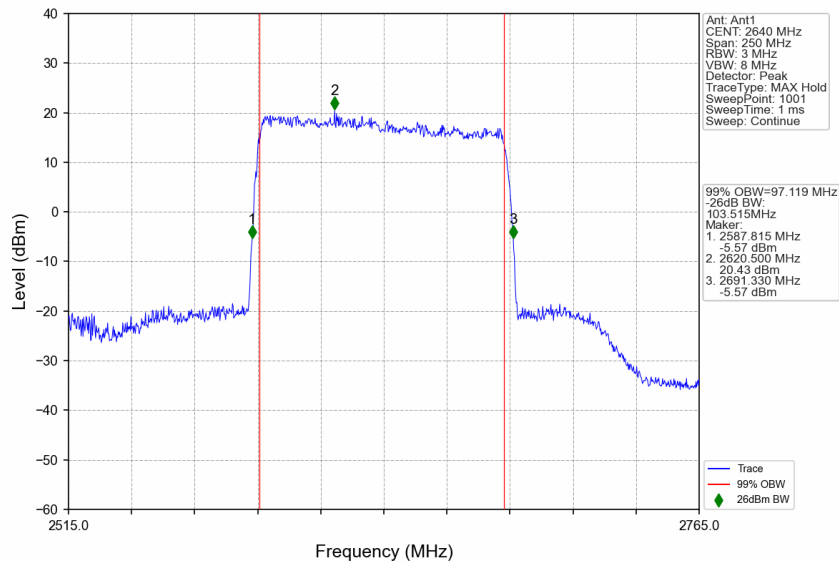
n41_30kHz_SISO_NTNV_100MHz_DFT-s-OFDM QPSK_2640MHz_Outer_Full
