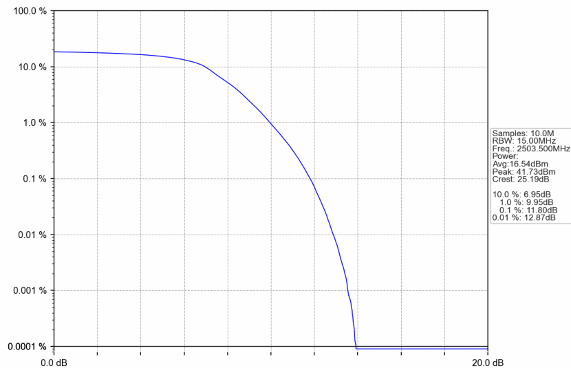
n41_15kHz_SISO_NTNV_15MHz_DFT-s-OFDM QPSK_2503.5MHz_Outer_Full
