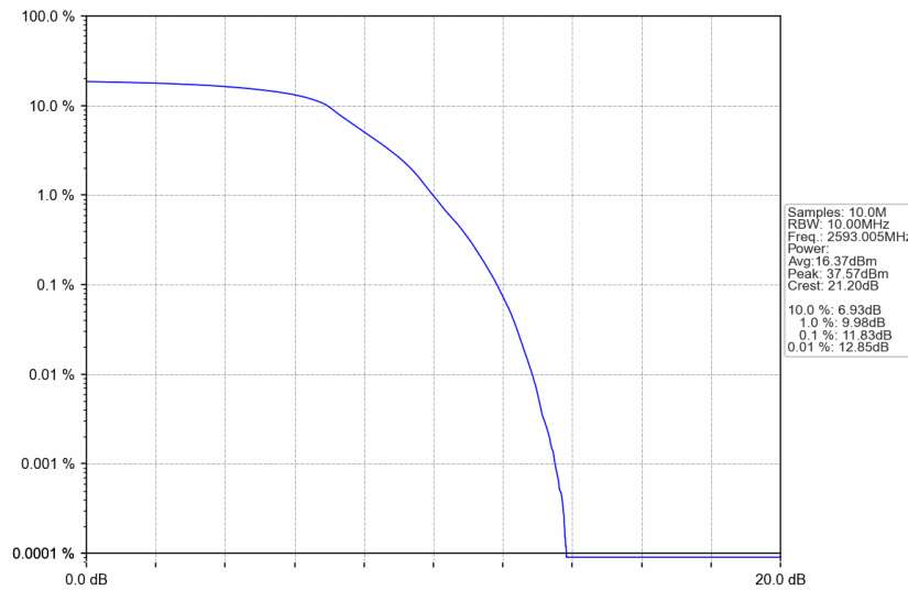
n41_15kHz_SISO_NTNV_10MHz_DFT-s-OFDM QPSK_2593.005MHz_Outer_Full
