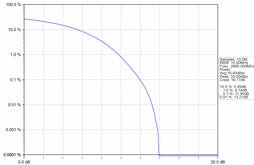
n41_15kHz_SISO_NTNV_10MHz_CP-OFDM 16 QAM_2685MHz_Outer_Full
