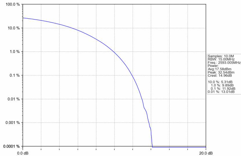
n41_15kHz_SISO_NTNV_15MHz_CP-OFDM QPSK_2593.005MHz_Outer_Full
