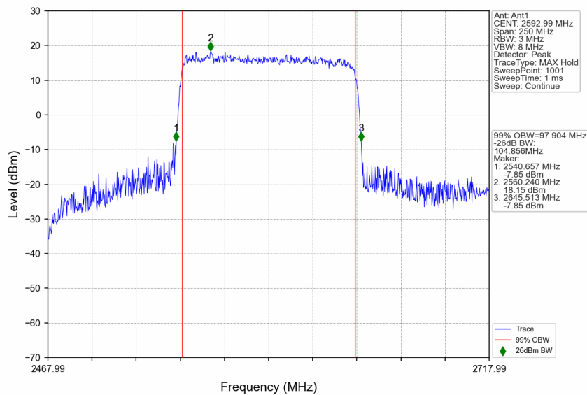
n41_30kHz_SISO_NTNV_100MHz_CP-OFDM 16 QAM_2592.99MHz_Outer_Full
