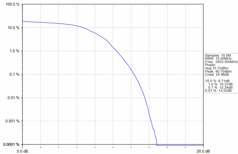
n41_15kHz_SISO_NTNV_15MHz_DFT-s-OFDM 16 QAM_2503.5MHz_Outer_Full
