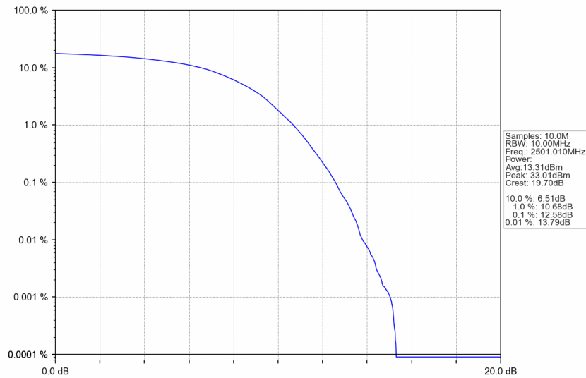
n41_15kHz_SISO_NTNV_10MHz_DFT-s-OFDM 256 QAM_2501.01MHz_Outer_Full
