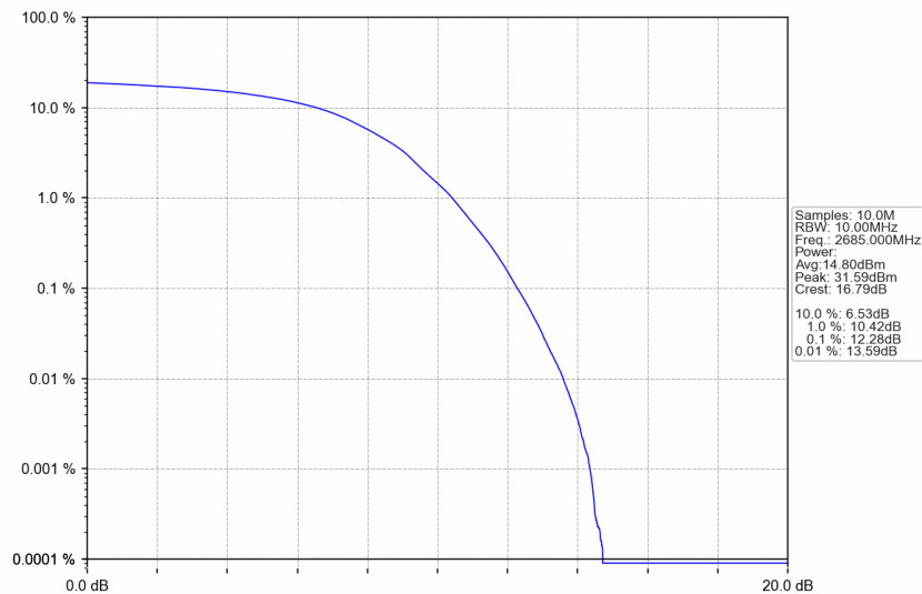
n41_15kHz_SISO_NTNV_10MHz_DFT-s-OFDM 64 QAM_2685MHz_Outer_Full
