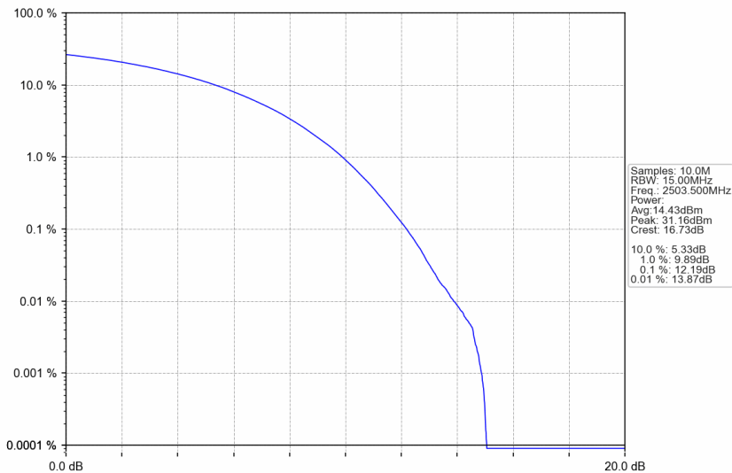
n41_15kHz_SISO_NTNV_15MHz_CP-OFDM 256 QAM_2503.5MHz_Outer_Full
