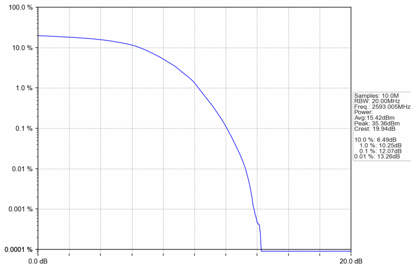
n41_15kHz_SISO_NTNV_20MHz_DFT-s-OFDM 64 QAM_2593.005MHz_Outer_Full
