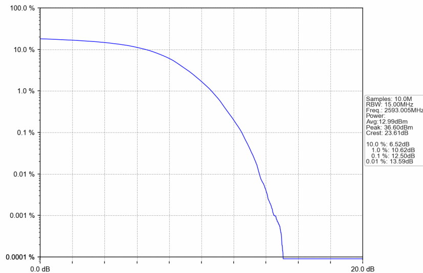
n41_15kHz_SISO_NTNV_15MHz_DFT-s-OFDM 256 QAM_2593.005MHz_Outer_Full
