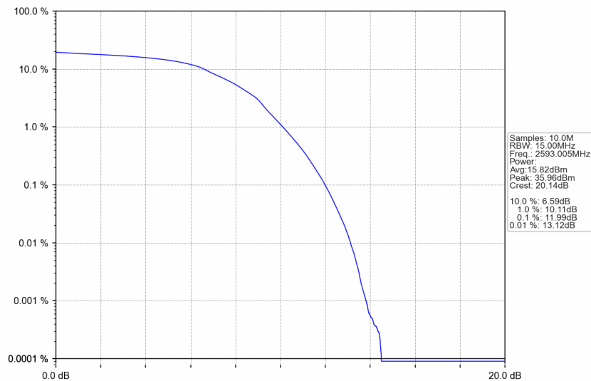
n41_15kHz_SISO_NTNV_15MHz_DFT-s-OFDM 16 QAM_2593.005MHz_Outer_Full
