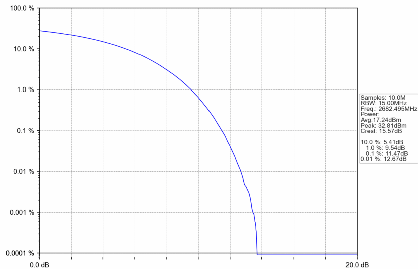
n41_15kHz_SISO_NTNV_15MHz_CP-OFDM QPSK_2682.495MHz_Outer_Full
