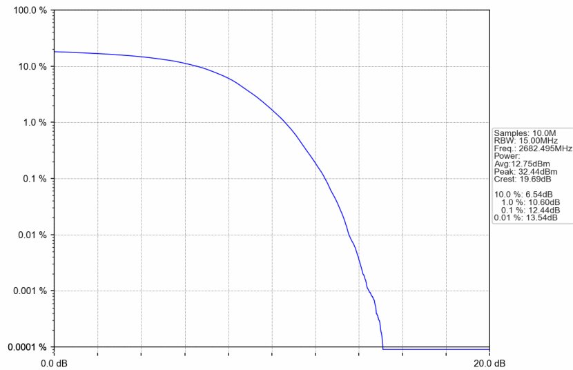
n41_15kHz_SISO_NTNV_15MHz_DFT-s-OFDM 256 QAM_2682.495MHz_Outer_Full
