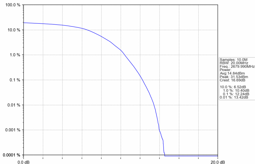
n41_15kHz_SISO_NTNV_20MHz_DFT-s-OFDM 64 QAM_2679.99MHz_Outer_Full
