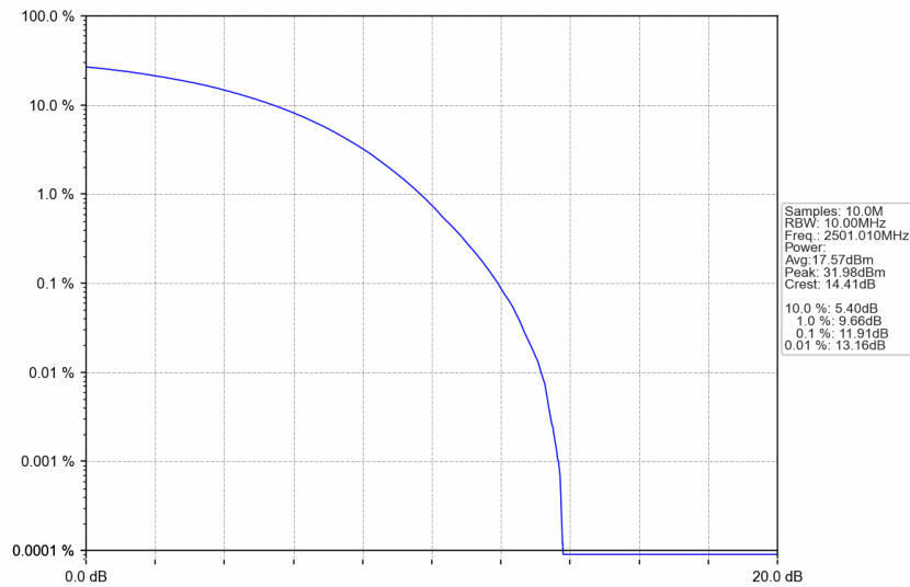
n41_15kHz_SISO_NTNV_10MHz_CP-OFDM 16 QAM_2501.01MHz_Outer_Full
