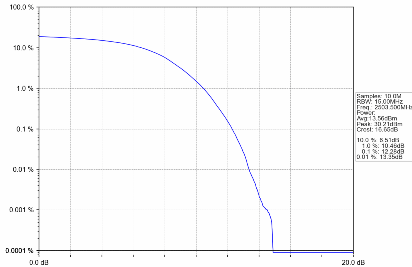
n41_15kHz_SISO_NTNV_15MHz_DFT-s-OFDM 256 QAM_2503.5MHz_Outer_Full
