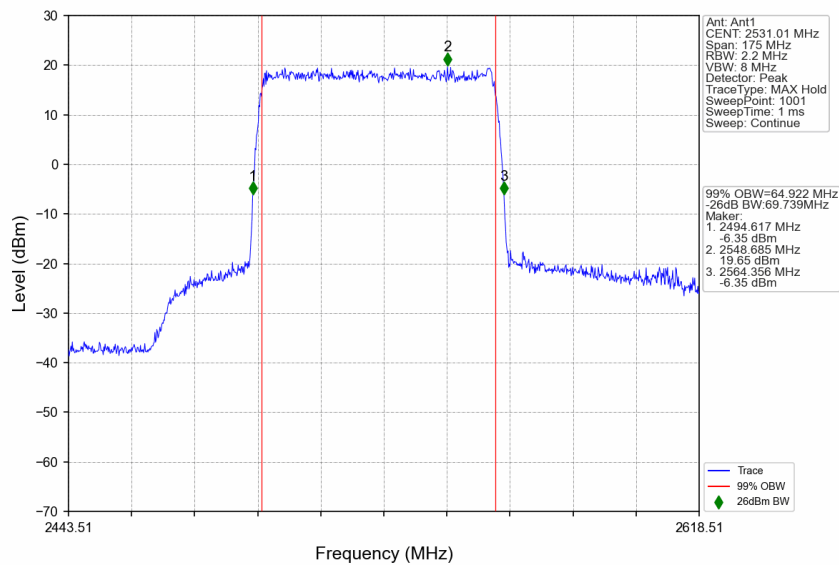
n41_30kHz_SISO_NTNV_70MHz_DFT-s-OFDM QPSK_2531.01MHz_Outer_Full
