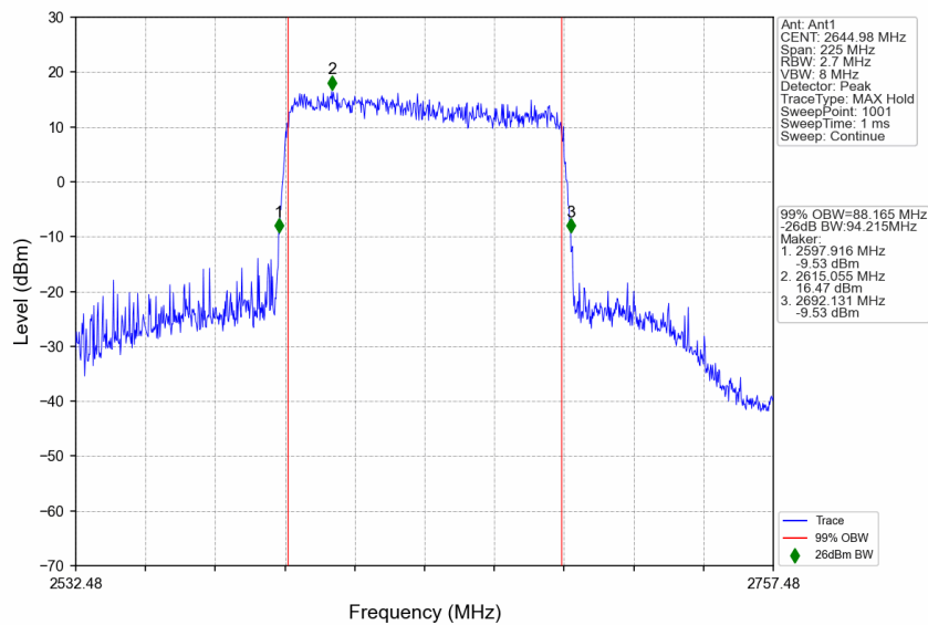
n41_30kHz_SISO_NTNV_90MHz_CP-OFDM QPSK_2644.98MHz_Outer_Full
