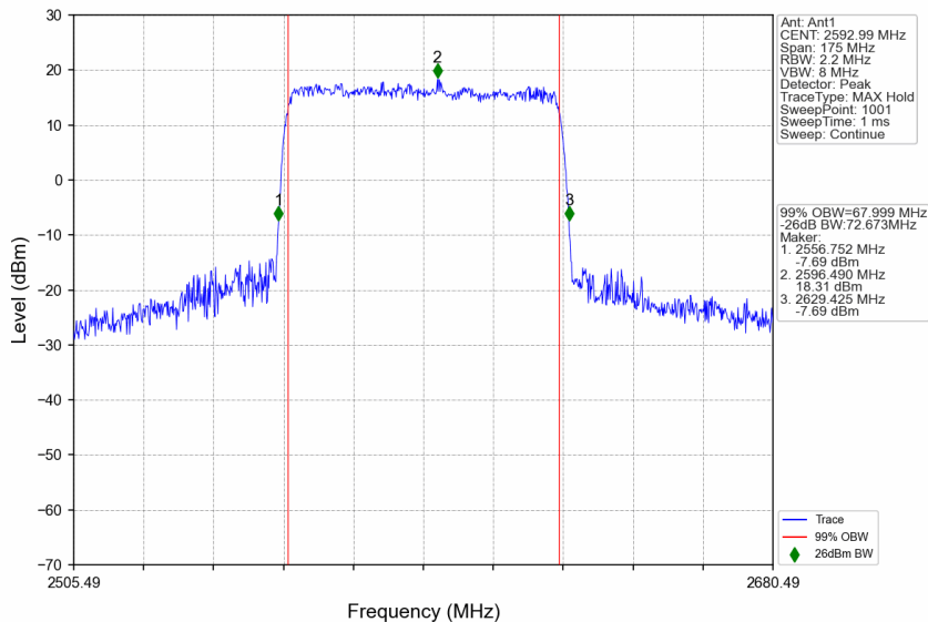
n41_30kHz_SISO_NTNV_70MHz_CP-OFDM 16 QAM_2592.99MHz_Outer_Full
