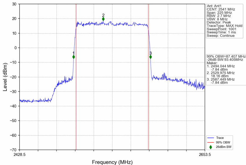
n41_30kHz_SISO_NTNV_90MHz_DFT-s-OFDM 64 QAM_2541MHz_Outer_Full
