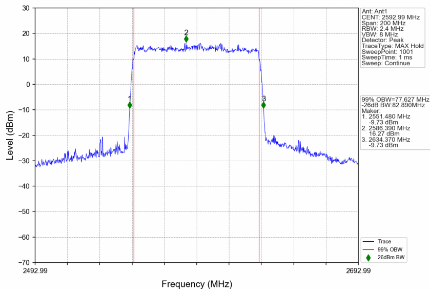
n41_30kHz_SISO_NTNV_80MHz_DFT-s-OFDM 256 QAM_2592.99MHz_Outer_Full
