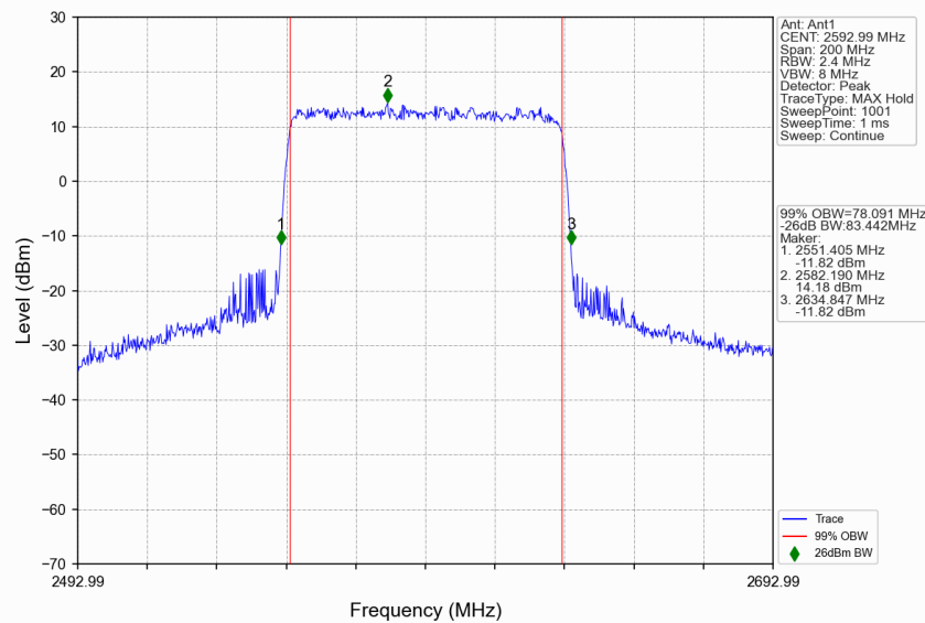
n41_30kHz_SISO_NTNV_80MHz_CP-OFDM 256 QAM_2592.99MHz_Outer_Full
