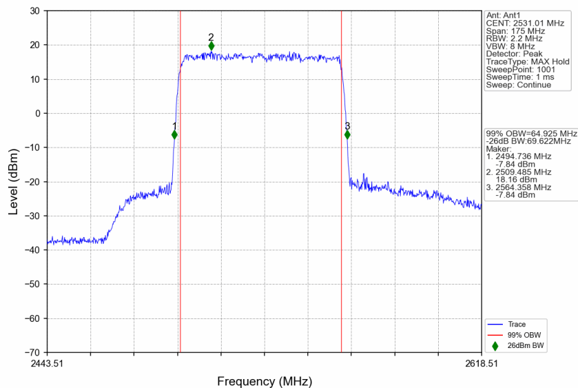
n41_30kHz_SISO_NTNV_70MHz_DFT-s-OFDM 64 QAM_2531.01MHz_Outer_Full
