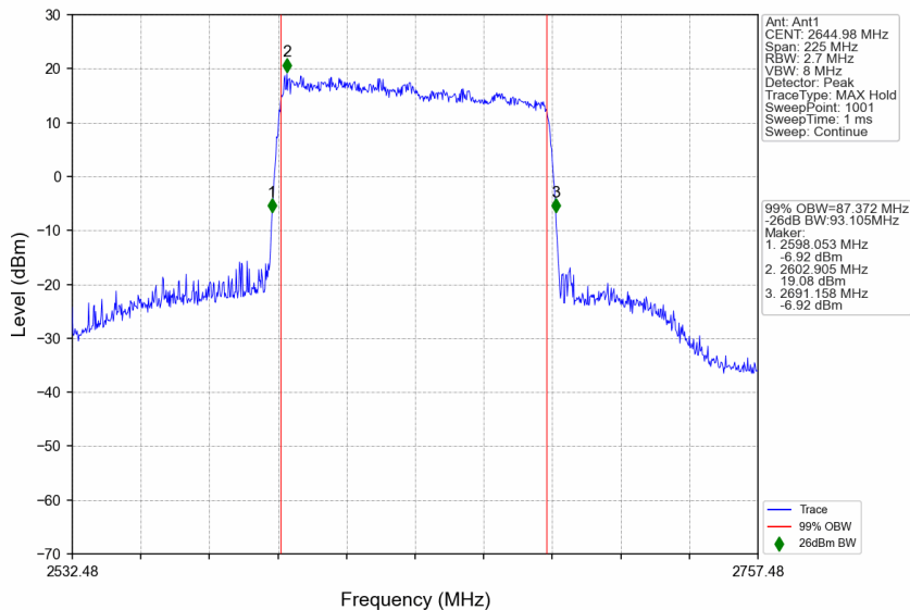
n41_30kHz_SISO_NTNV_90MHz_DFT-s-OFDM 64 QAM_2644.98MHz_Outer_Full
