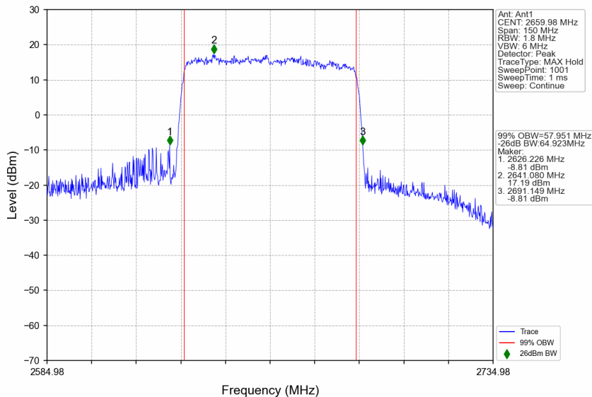
n41_30kHz_SISO_NTNV_60MHz_CP-OFDM QPSK_2659.98MHz_Outer_Full
