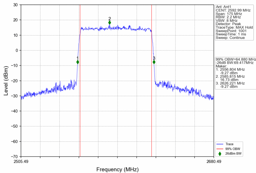
n41_30kHz_SISO_NTNV_70MHz_DFT-s-OFDM 256 QAM_2592.99MHz_Outer_Full
