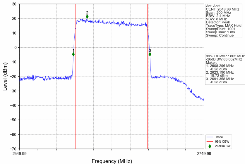
n41_30kHz_SISO_NTNV_80MHz_DFT-s-OFDM QPSK_2649.99MHz_Outer_Full
