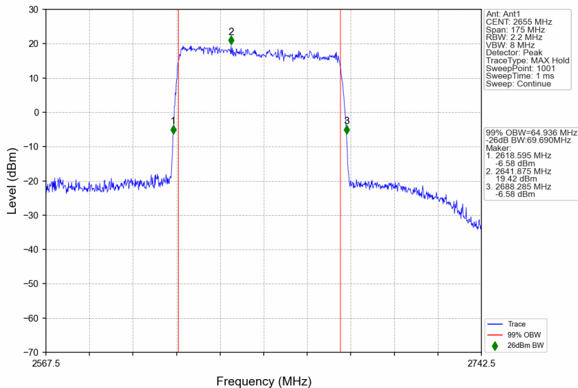
n41_30kHz_SISO_NTNV_70MHz_DFT-s-OFDM QPSK_2655MHz_Outer_Full
