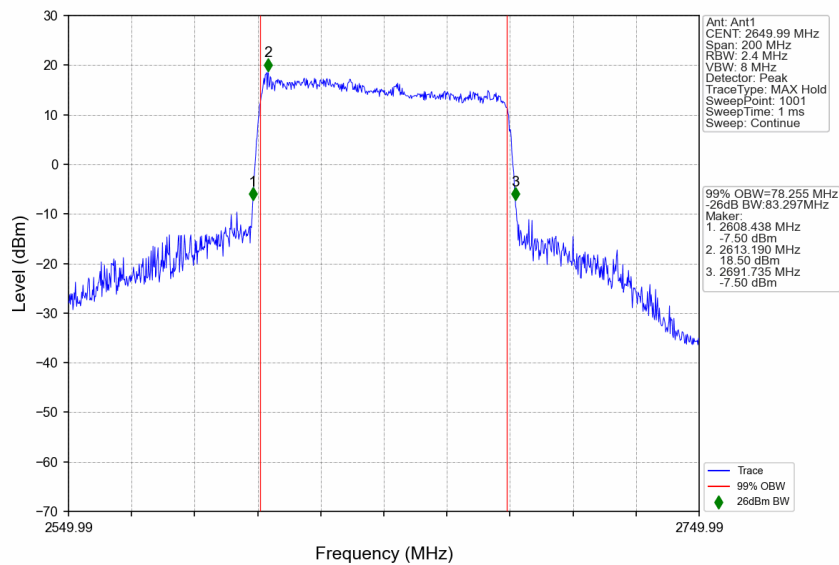
n41_30kHz_SISO_NTNV_80MHz_CP-OFDM 64 QAM_2649.99MHz_Outer_Full
