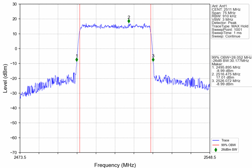
n41_30kHz_SISO_NTNV_30MHz_CP-OFDM 64 QAM_2511MHz_Outer_Full
