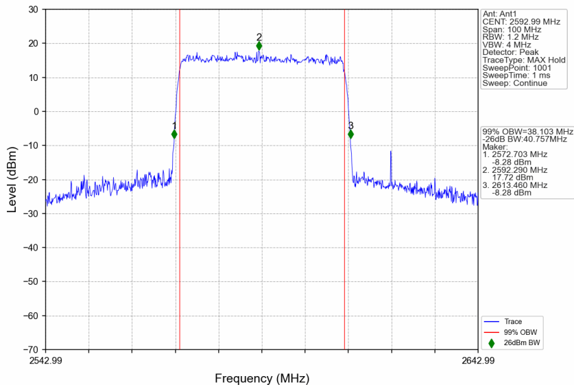
n41_30kHz_SISO_NTNV_40MHz_CP-OFDM 16 QAM_2592.99MHz_Outer_Full
