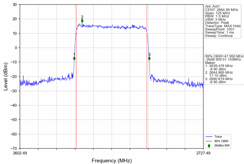
n41_30kHz_SISO_NTNV_50MHz_CP-OFDM 64 QAM_2664.99MHz_Outer_Full
