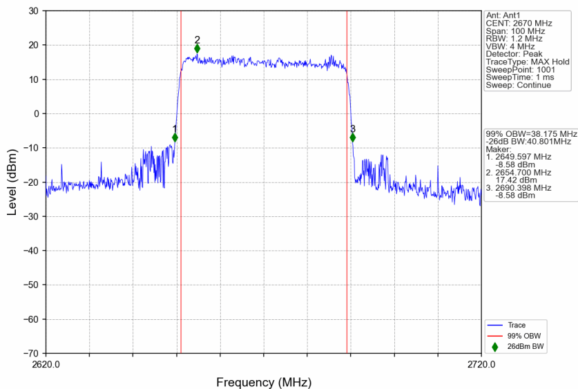
n41_30kHz_SISO_NTNV_40MHz_CP-OFDM QPSK_2670MHz_Outer_Full
