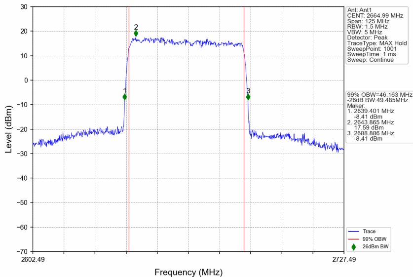
n41_30kHz_SISO_NTNV_50MHz_DFT-s-OFDM 64 QAM_2664.99MHz_Outer_Full
