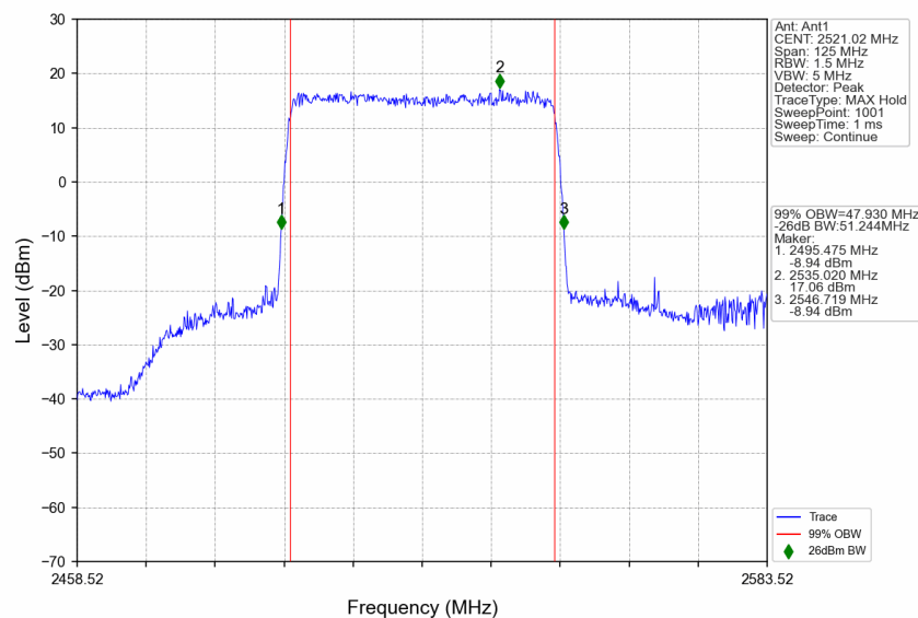
n41_30kHz_SISO_NTNV_50MHz_CP-OFDM 64 QAM_2521.02MHz_Outer_Full
