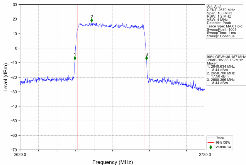
n41_30kHz_SISO_NTNV_40MHz_DFT-s-OFDM 64 QAM_2670MHz_Outer_Full
