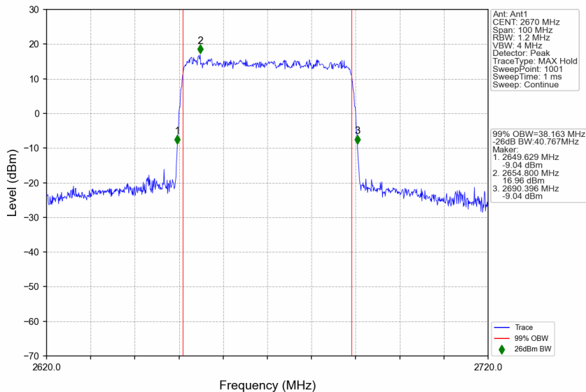
n41_30kHz_SISO_NTNV_40MHz_CP-OFDM 64 QAM_2670MHz_Outer_Full
