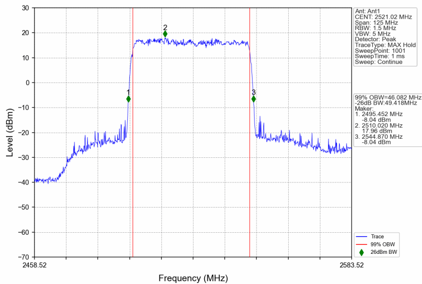
n41_30kHz_SISO_NTNV_50MHz_DFT-s-OFDM 64 QAM_2521.02MHz_Outer_Full
