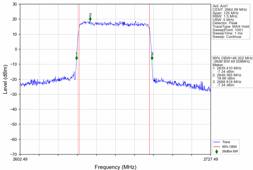
n41_30kHz_SISO_NTNV_50MHz_DFT-s-OFDM QPSK_2664.99MHz_Outer_Full
