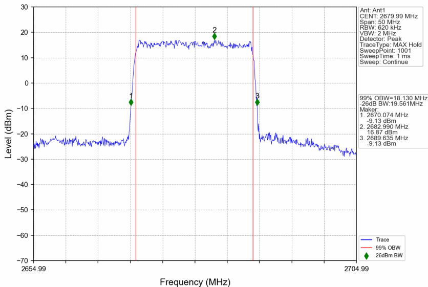
n41_30kHz_SISO_NTNV_20MHz_DFT-s-OFDM 64 QAM_2679.99MHz_Outer_Full
