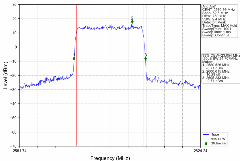
n41_30kHz_SISO_NTNV_25MHz_DFT-s-OFDM 256 QAM_2592.99MHz_Outer_Full
