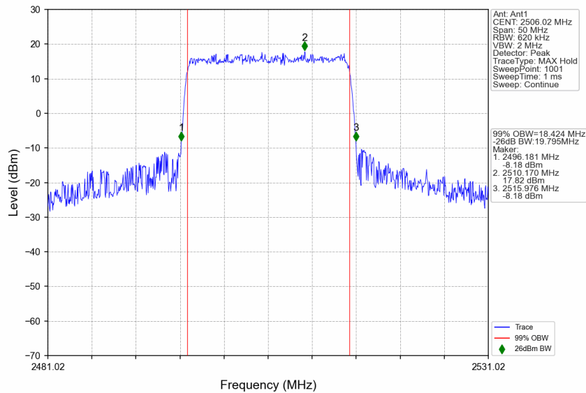
n41_30kHz_SISO_NTNV_20MHz_CP-OFDM QPSK_2506.02MHz_Outer_Full
