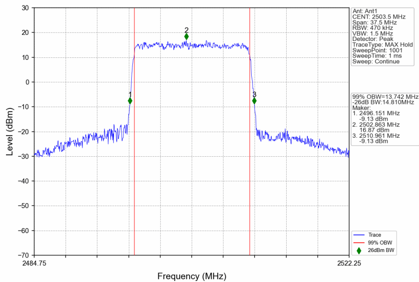
n41_30kHz_SISO_NTNV_15MHz_CP-OFDM 64 QAM_2503.5MHz_Outer_Full
