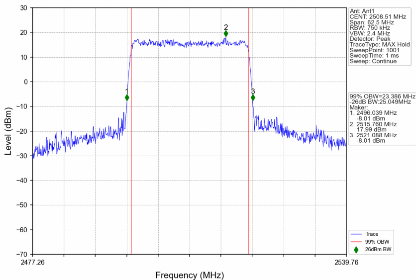
n41_30kHz_SISO_NTNV_25MHz_CP-OFDM QPSK_2508.51MHz_Outer_Full
