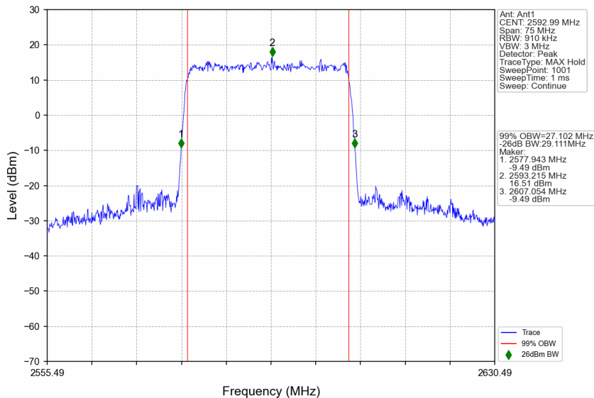
n41_30kHz_SISO_NTNV_30MHz_DFT-s-OFDM 256 QAM_2592.99MHz_Outer_Full
