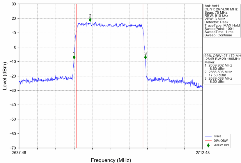
n41_30kHz_SISO_NTNV_30MHz_DFT-s-OFDM 64 QAM_2674.98MHz_Outer_Full
