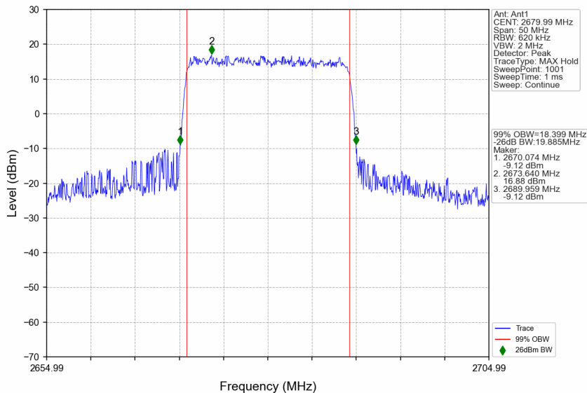
n41_30kHz_SISO_NTNV_20MHz_CP-OFDM QPSK_2679.99MHz_Outer_Full
