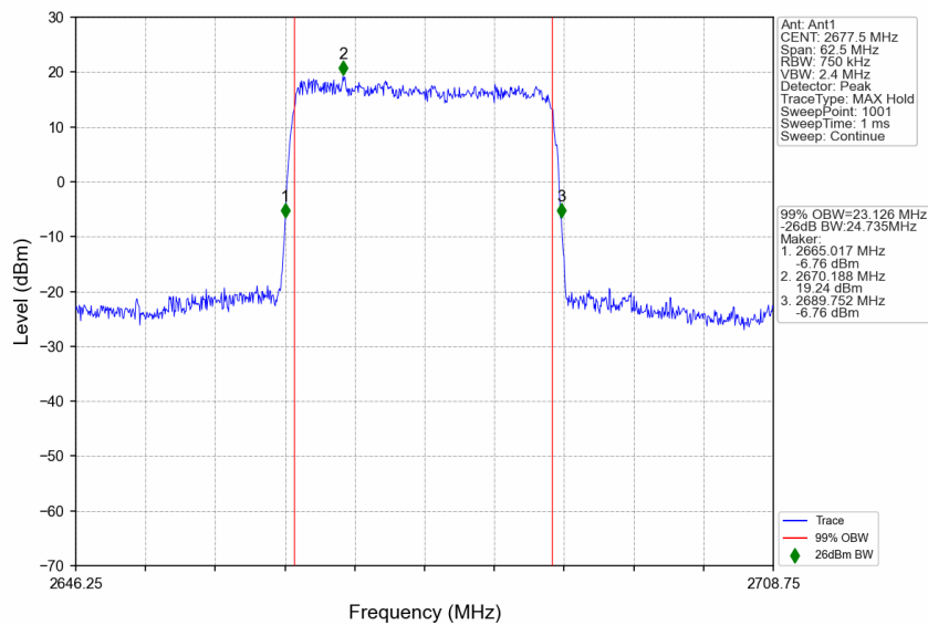
n41_30kHz_SISO_NTNV_25MHz_DFT-s-OFDM QPSK_2677.5MHz_Outer_Full
