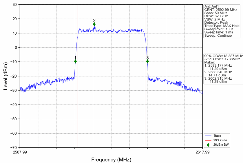
n41_30kHz_SISO_NTNV_20MHz_CP-OFDM 256 QAM_2592.99MHz_Outer_Full
