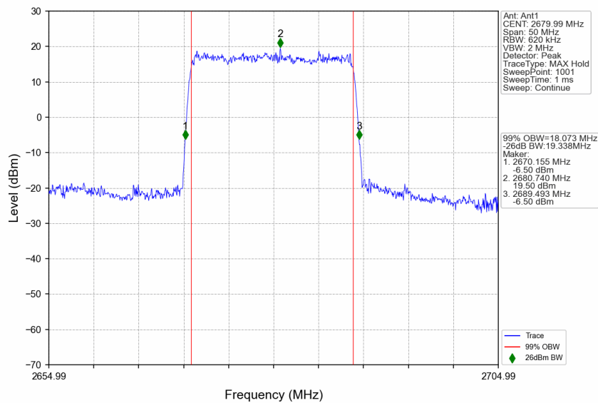
n41_30kHz_SISO_NTNV_20MHz_DFT-s-OFDM QPSK_2679.99MHz_Outer_Full
