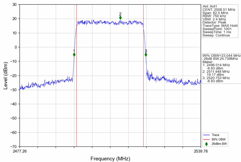
n41_30kHz_SISO_NTNV_25MHz_DFT-s-OFDM QPSK_2508.51MHz_Outer_Full
