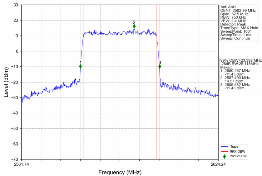
n41_30kHz_SISO_NTNV_25MHz_CP-OFDM 256 QAM_2592.99MHz_Outer_Full
