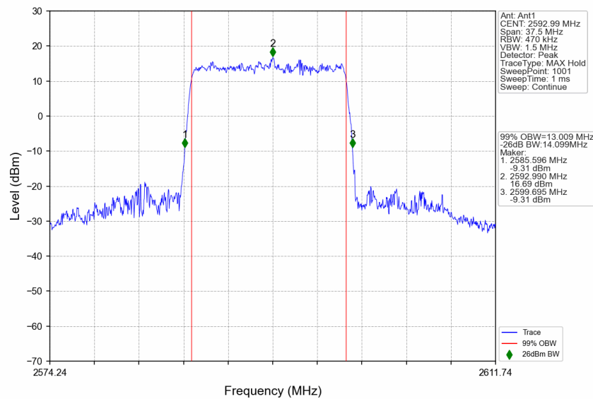
n41_30kHz_SISO_NTNV_15MHz_DFT-s-OFDM 256 QAM_2592.99MHz_Outer_Full
