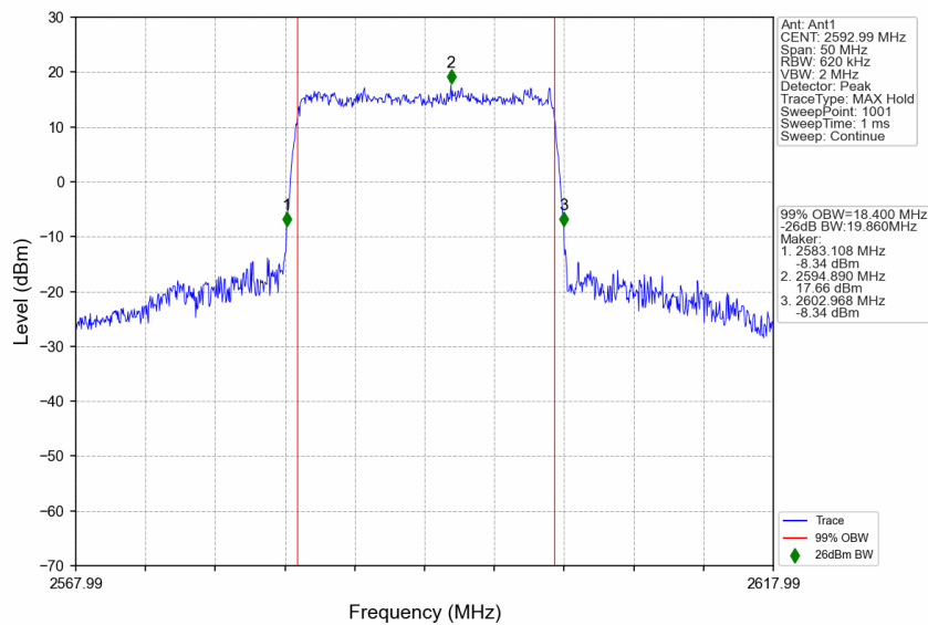
n41_30kHz_SISO_NTNV_20MHz_CP-OFDM 16 QAM_2592.99MHz_Outer_Full
