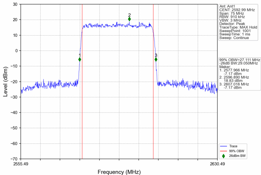
n41_30kHz_SISO_NTNV_30MHz_DFT-s-OFDM 16 QAM_2592.99MHz_Outer_Full
