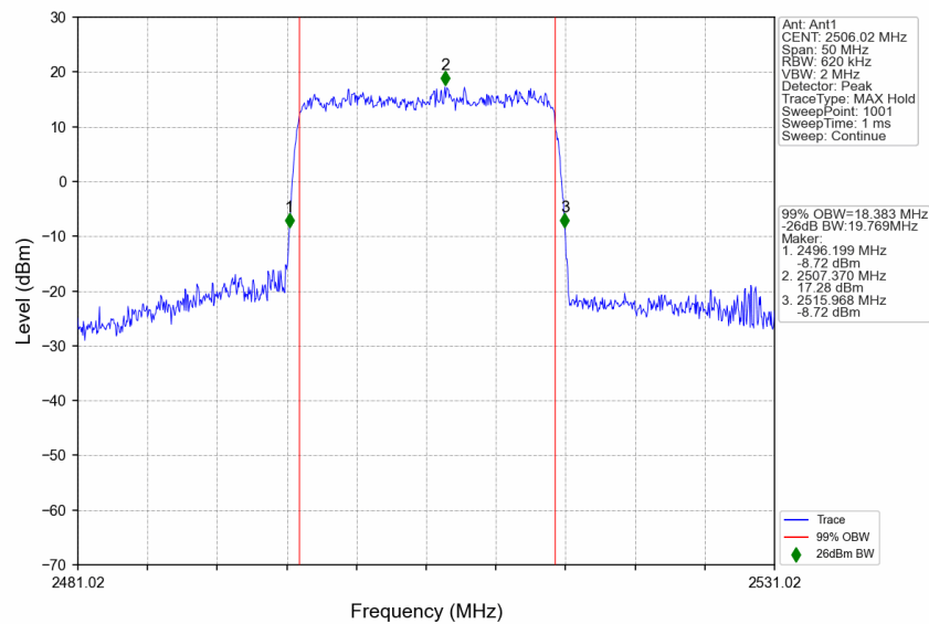
n41_30kHz_SISO_NTNV_20MHz_CP-OFDM 64 QAM_2506.02MHz_Outer_Full
