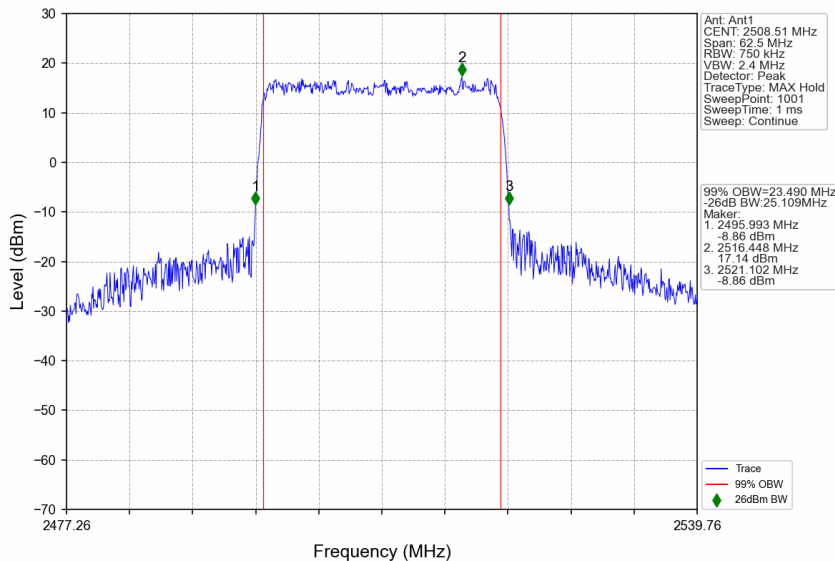
n41_30kHz_SISO_NTNV_25MHz_CP-OFDM 64 QAM_2508.51MHz_Outer_Full
