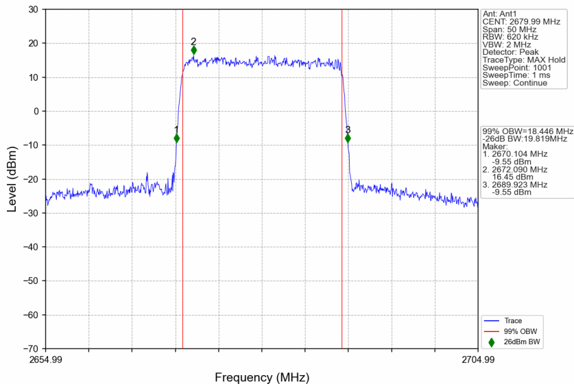
n41_30kHz_SISO_NTNV_20MHz_CP-OFDM 64 QAM_2679.99MHz_Outer_Full
