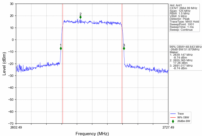
n41_15kHz_SISO_NTNV_50MHz_CP-OFDM 64 QAM_2664.99MHz_Outer_Full
