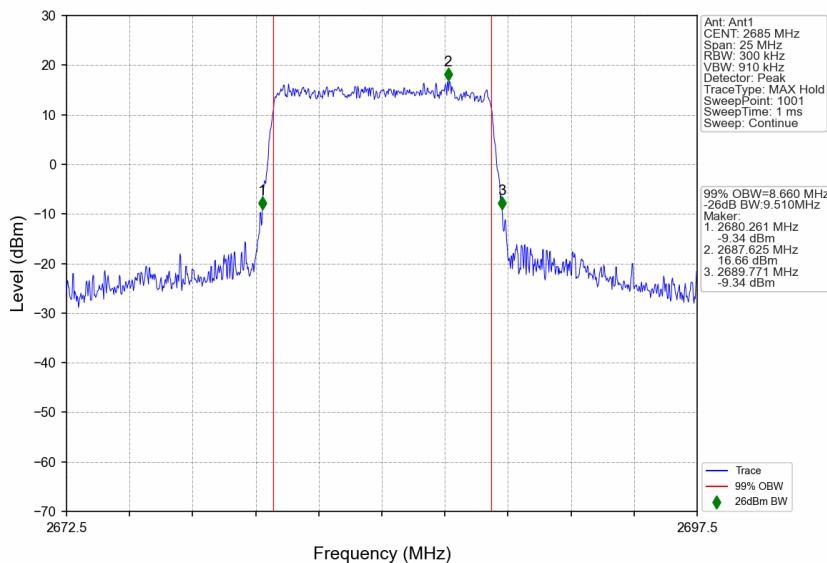
n41_30kHz_SISO_NTNV_10MHz_CP-OFDM QPSK_2685MHz_Outer_Full
