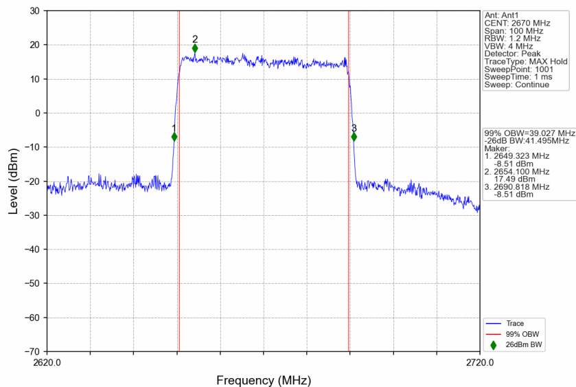
n41_15kHz_SISO_NTNV_40MHz_DFT-s-OFDM 64 QAM_2670MHz_Outer_Full
