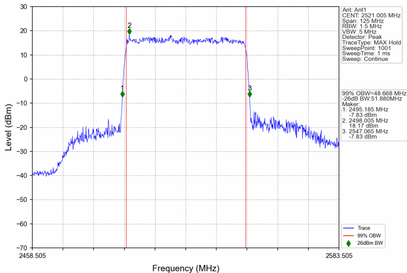
n41_15kHz_SISO_NTNV_50MHz_DFT-s-OFDM 64 QAM_2521.005MHz_Outer_Full
