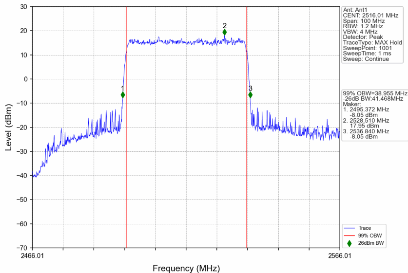
n41_15kHz_SISO_NTNV_40MHz_CP-OFDM QPSK_2516.01MHz_Outer_Full
