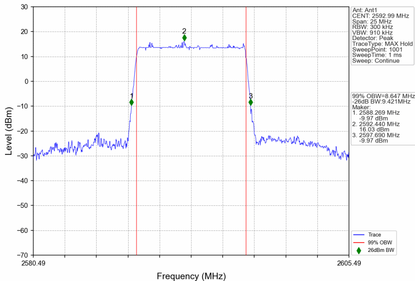
n41_30kHz_SISO_NTNV_10MHz_DFT-s-OFDM 256 QAM_2592.99MHz_Outer_Full
