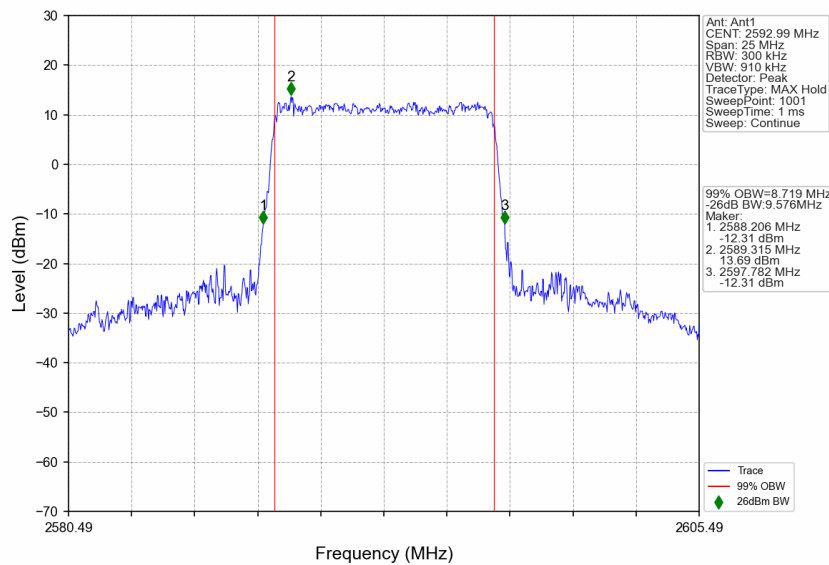
n41_30kHz_SISO_NTNV_10MHz_CP-OFDM 256 QAM_2592.99MHz_Outer_Full
