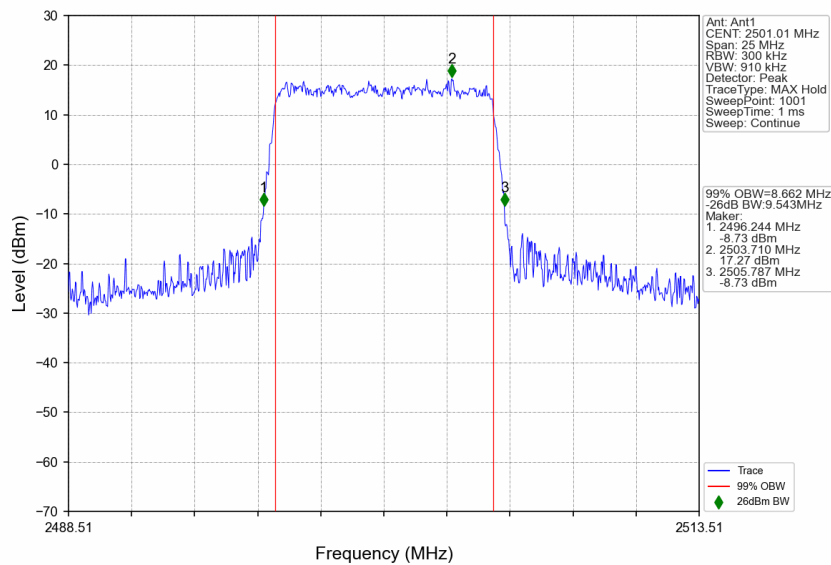
n41_30kHz_SISO_NTNV_10MHz_CP-OFDM QPSK_2501.01MHz_Outer_Full
