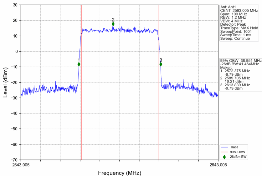
n41_15kHz_SISO_NTNV_40MHz_DFT-s-OFDM 256 QAM_2593.005MHz_Outer_Full
