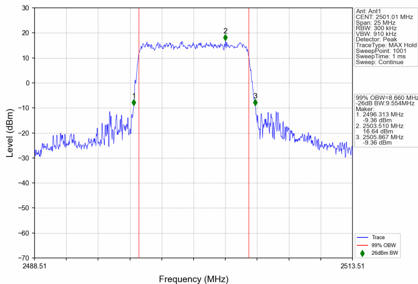
n41_30kHz_SISO_NTNV_10MHz_CP-OFDM 64 QAM_2501.01MHz_Outer_Full
