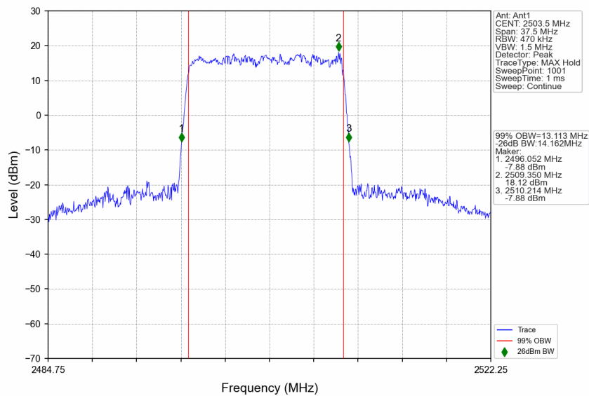
n41_30kHz_SISO_NTNV_15MHz_DFT-s-OFDM 64 QAM_2503.5MHz_Outer_Full
