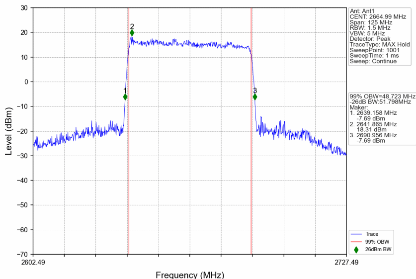
n41_15kHz_SISO_NTNV_50MHz_DFT-s-OFDM 64 QAM_2664.99MHz_Outer_Full
