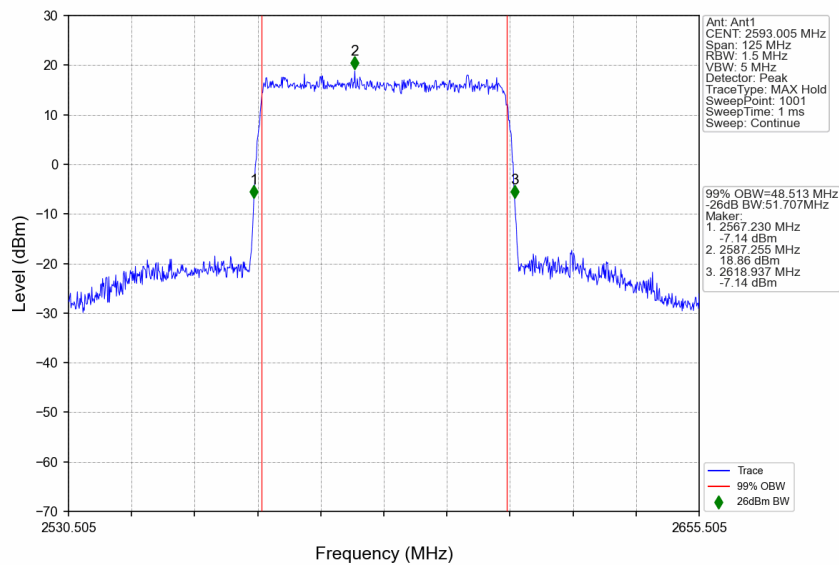
n41_15kHz_SISO_NTNV_50MHz_DFT-s-OFDM 16 QAM_2593.005MHz_Outer_Full
