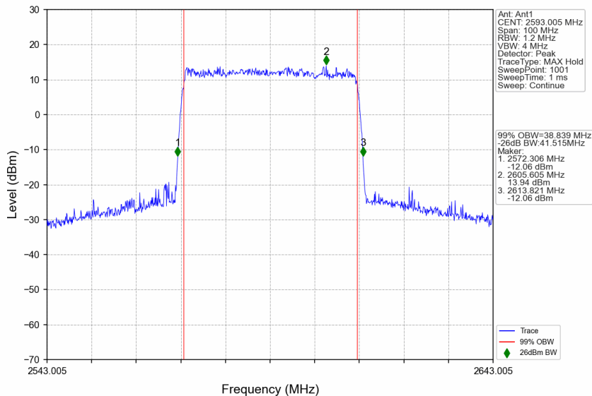
n41_15kHz_SISO_NTNV_40MHz_CP-OFDM 256 QAM_2593.005MHz_Outer_Full
