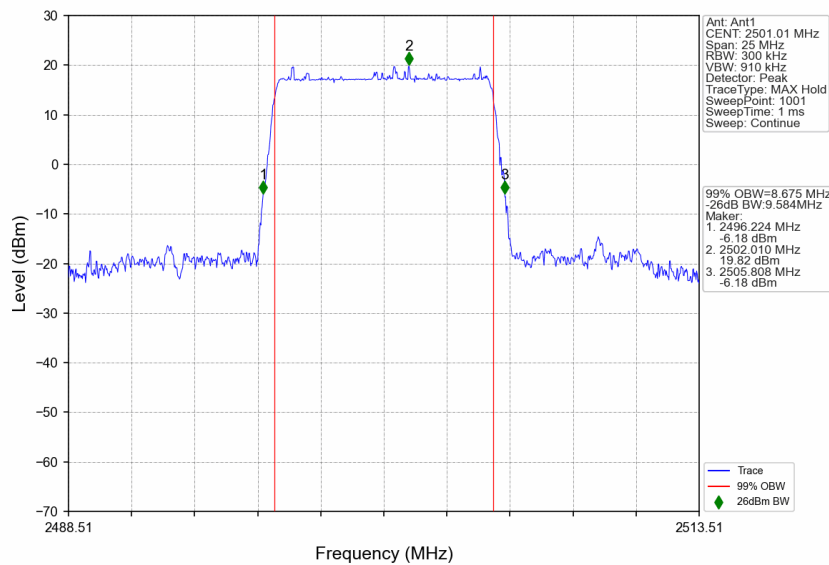
n41_30kHz_SISO_NTNV_10MHz_DFT-s-OFDM QPSK_2501.01MHz_Outer_Full
