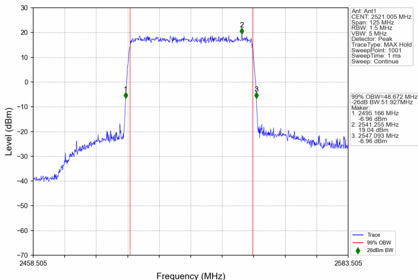
n41_15kHz_SISO_NTNV_50MHz_DFT-s-OFDM QPSK_2521.005MHz_Outer_Full
