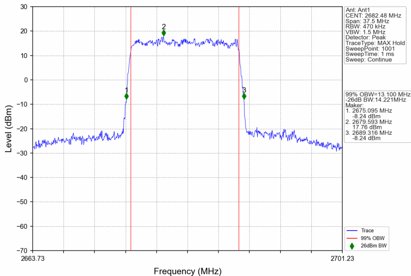
n41_30kHz_SISO_NTNV_15MHz_DFT-s-OFDM 64 QAM_2682.48MHz_Outer_Full
