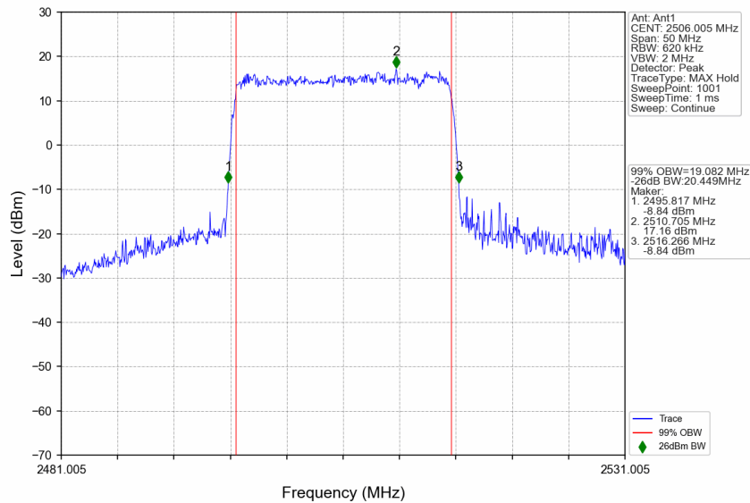
n41_15kHz_SISO_NTNV_20MHz_CP-OFDM 64 QAM_2506.005MHz_Outer_Full
