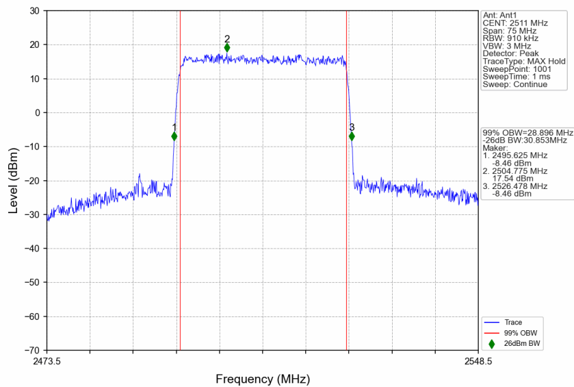
n41_15kHz_SISO_NTNV_30MHz_DFT-s-OFDM 64 QAM_2511MHz_Outer_Full
