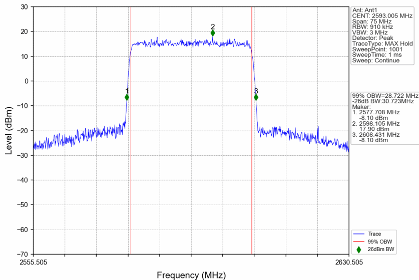
n41_15kHz_SISO_NTNV_30MHz_CP-OFDM 16 QAM_2593.005MHz_Outer_Full
