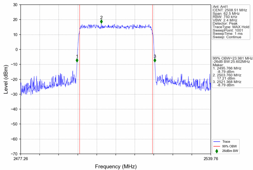
n41_15kHz_SISO_NTNV_25MHz_CP-OFDM QPSK_2508.51MHz_Outer_Full
