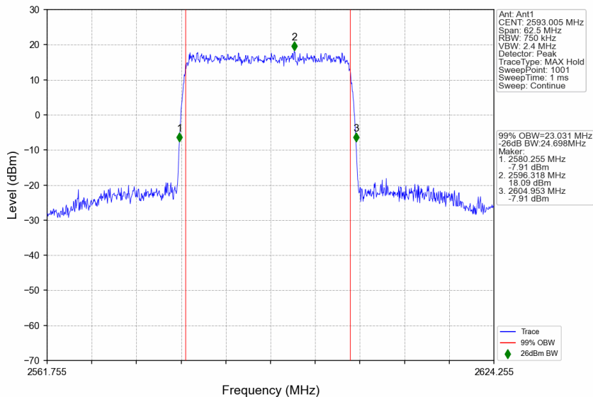
n41_15kHz_SISO_NTNV_25MHz_DFT-s-OFDM 16 QAM_2593.005MHz_Outer_Full
