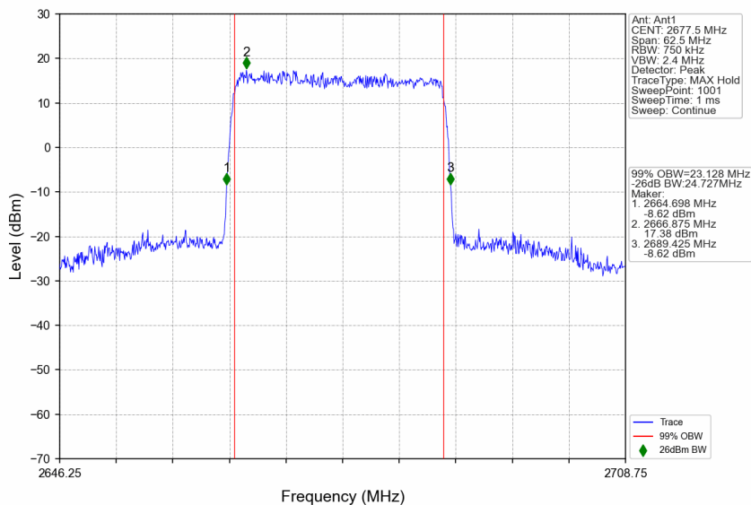
n41_15kHz_SISO_NTNV_25MHz_DFT-s-OFDM 64 QAM_2677.5MHz_Outer_Full
