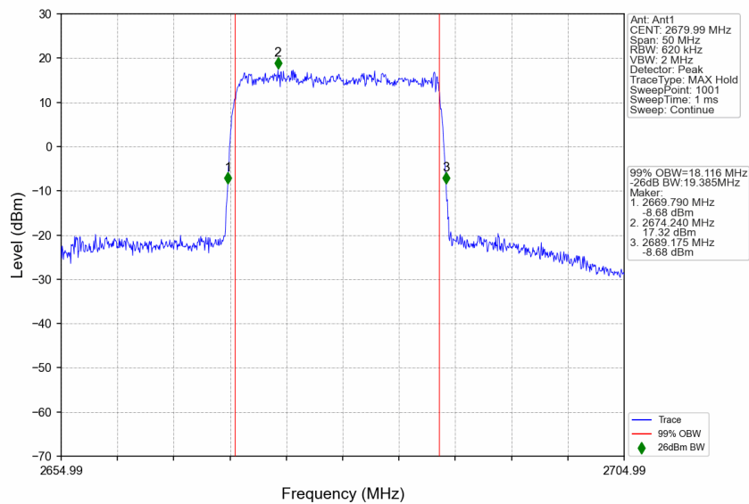
n41_15kHz_SISO_NTNV_20MHz_DFT-s-OFDM 64 QAM_2679.99MHz_Outer_Full
