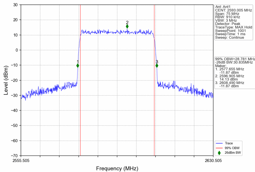
n41_15kHz_SISO_NTNV_30MHz_CP-OFDM 256 QAM_2593.005MHz_Outer_Full
