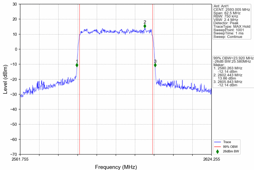
n41_15kHz_SISO_NTNV_25MHz_CP-OFDM 256 QAM_2593.005MHz_Outer_Full
