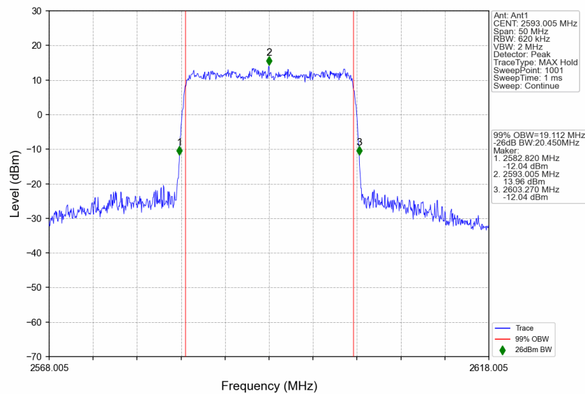
n41_15kHz_SISO_NTNV_20MHz_CP-OFDM 256 QAM_2593.005MHz_Outer_Full
