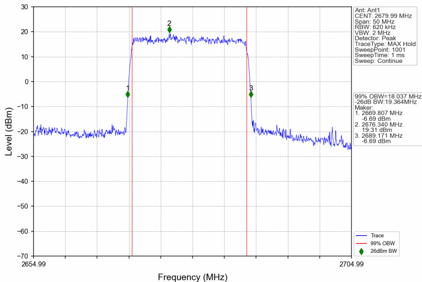
n41_15kHz_SISO_NTNV_20MHz_DFT-s-OFDM QPSK_2679.99MHz_Outer_Full
