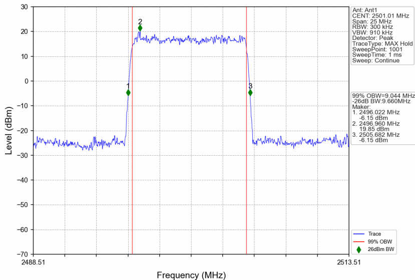
n41_15kHz_SISO_NTNV_10MHz_DFT-s-OFDM QPSK_2501.01MHz_Outer_Full
