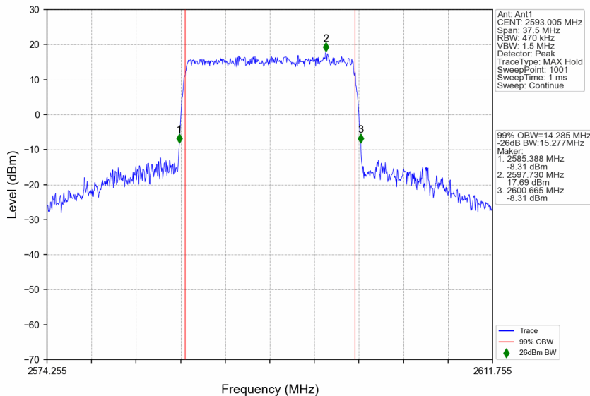
n41_15kHz_SISO_NTNV_15MHz_CP-OFDM 16 QAM_2593.005MHz_Outer_Full
