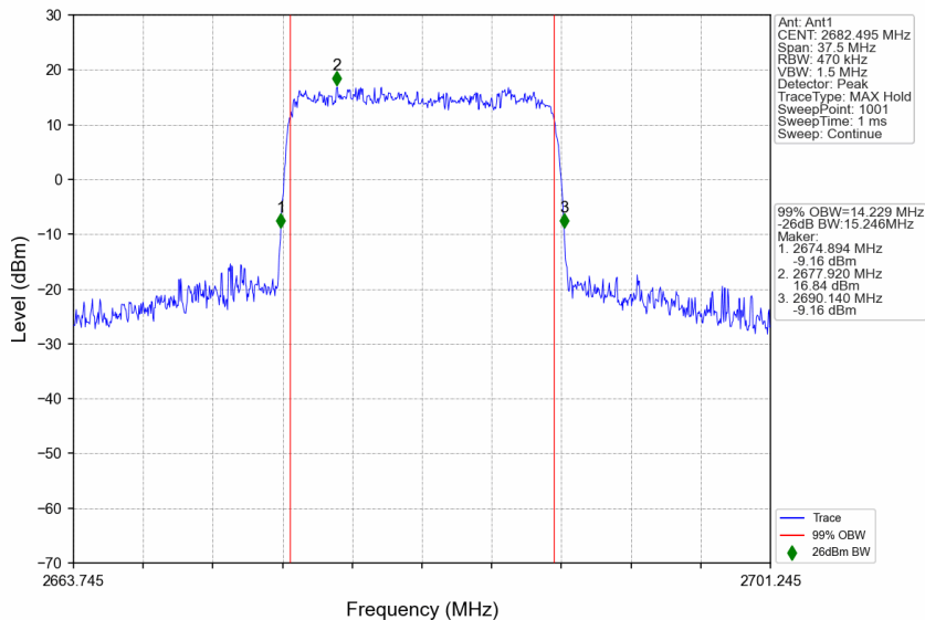
n41_15kHz_SISO_NTNV_15MHz_CP-OFDM QPSK_2682.495MHz_Outer_Full
