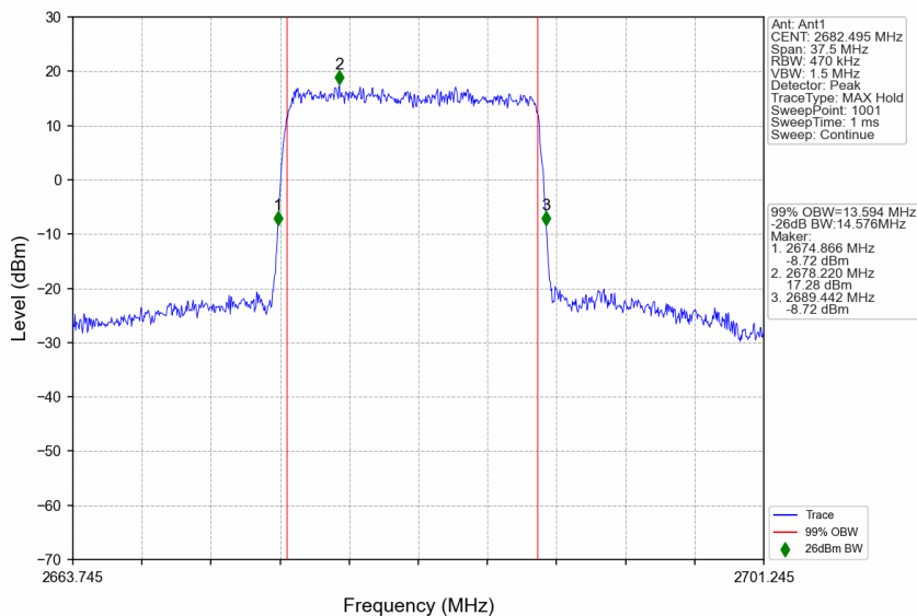
n41_15kHz_SISO_NTNV_15MHz_DFT-s-OFDM 64 QAM_2682.495MHz_Outer_Full
