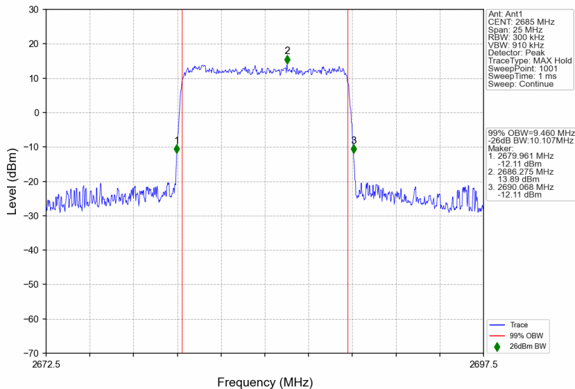
n41_15kHz_SISO_NTNV_10MHz_CP-OFDM 64 QAM_2685MHz_Outer_Full
