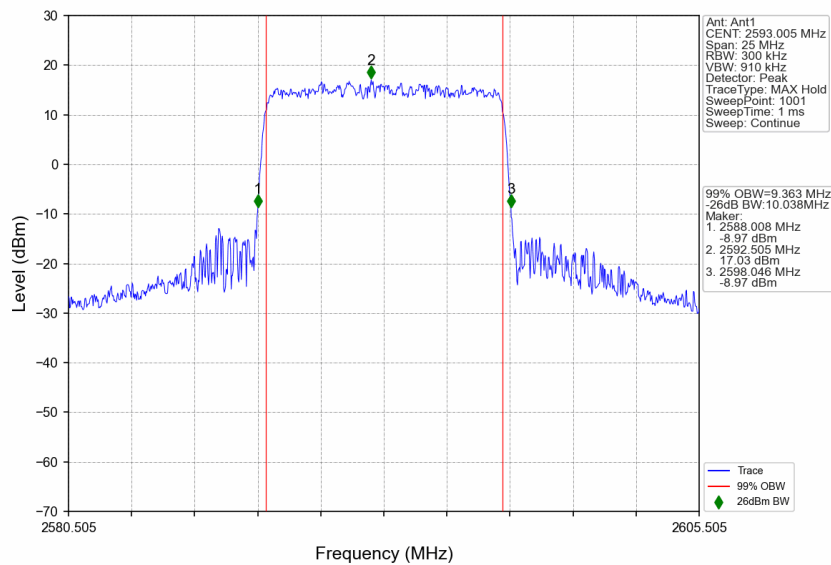
n41_15kHz_SISO_NTNV_10MHz_CP-OFDM 16 QAM_2593.005MHz_Outer_Full
