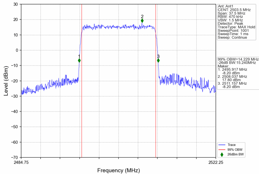
n41_15kHz_SISO_NTNV_15MHz_CP-OFDM QPSK_2503.5MHz_Outer_Full
