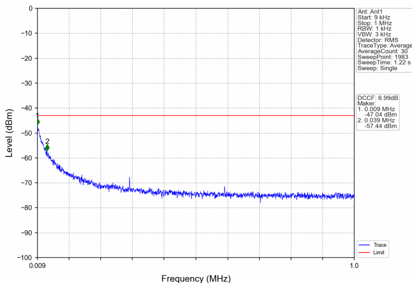
n38_30kHz_SISO_NTNV_40MHz_DFT-s-OFDM QPSK_2600MHz_Edge_1RB_Right
