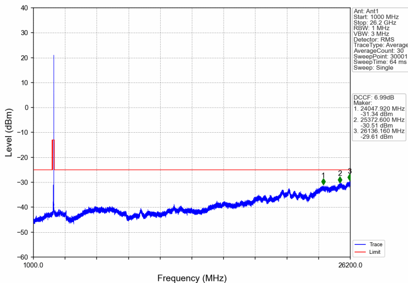
n38_30kHz_SISO_NTNV_40MHz_DFT-s-OFDM QPSK_2600MHz_Edge_1RB_Right
