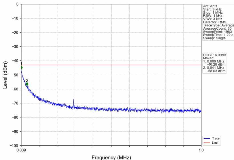
n38_30kHz_SISO_NTNV_40MHz_CP-OFDM QPSK_2600MHz_Edge_1RB_Right
