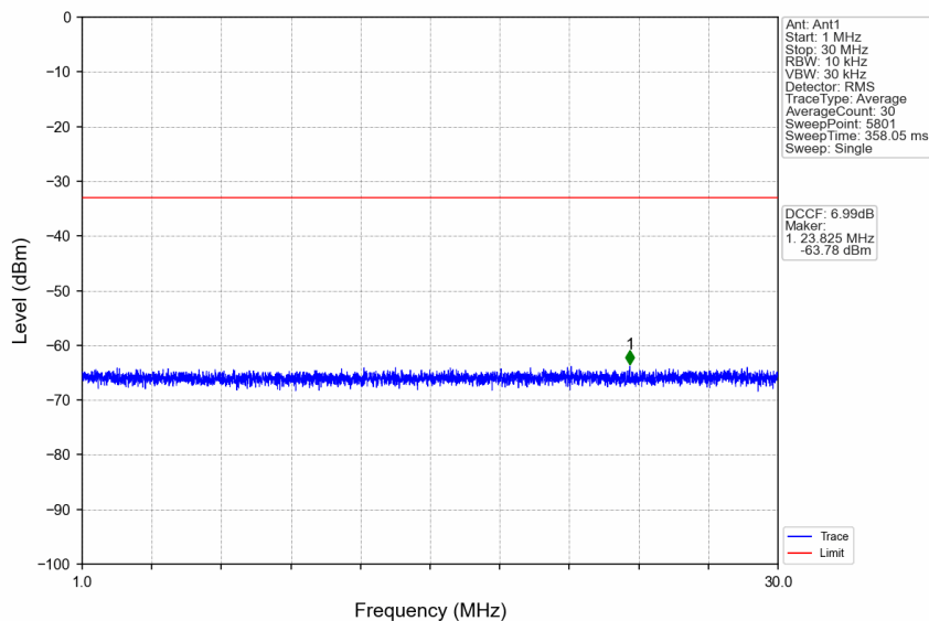
n38_30kHz_SISO_NTNV_30MHz_CP-OFDM QPSK_2605MHz_Edge_1RB_Right
