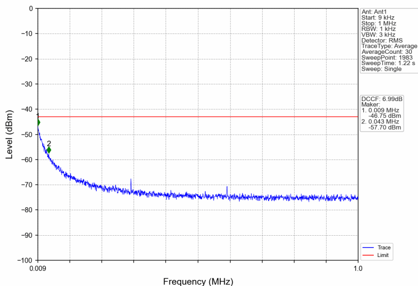
n38_30kHz_SISO_NTNV_30MHz_DFT-s-OFDM QPSK_2605MHz_Edge_1RB_Right
