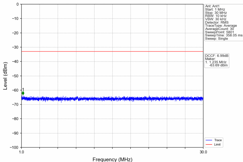
n38_30kHz_SISO_NTNV_30MHz_DFT-s-OFDM QPSK_2585MHz_Edge_1RB_Left
