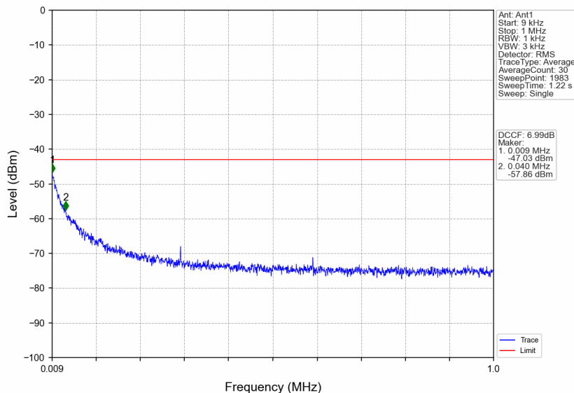
n38_30kHz_SISO_NTNV_30MHz_CP-OFDM QPSK_2605MHz_Edge_1RB_Right
