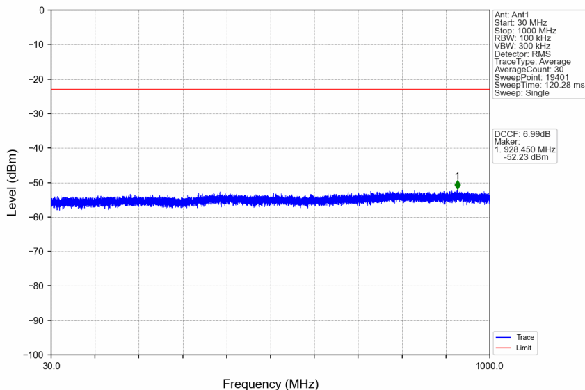
n38_30kHz_SISO_NTNV_25MHz_CP-OFDM QPSK_2607.5MHz_Edge_1RB_Right
