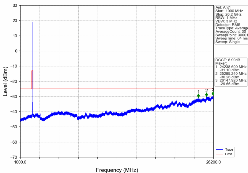
n38_30kHz_SISO_NTNV_30MHz_DFT-s-OFDM QPSK_2605MHz_Edge_1RB_Right
