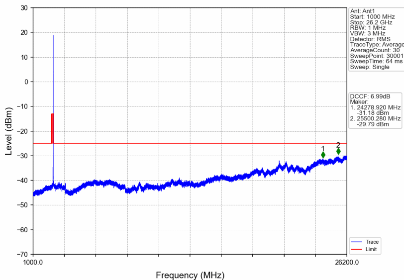
n38_30kHz_SISO_NTNV_25MHz_CP-OFDM QPSK_2607.5MHz_Edge_1RB_Right
