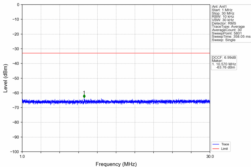
n38_30kHz_SISO_NTNV_25MHz_CP-OFDM QPSK_2607.5MHz_Edge_1RB_Right
