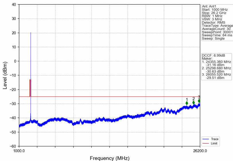
n38_30kHz_SISO_NTNV_30MHz_CP-OFDM QPSK_2605MHz_Edge_1RB_Right
