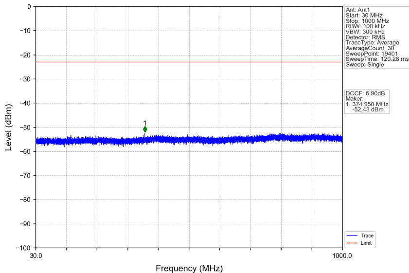
n38_30kHz_SISO_NTNV_30MHz_DFT-s-OFDM QPSK_2595MHz_Edge_1RB_Left
