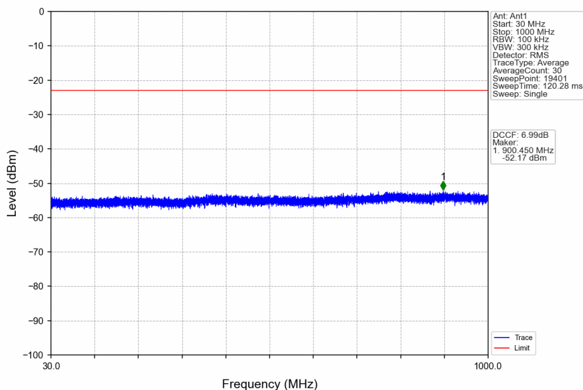
n38_30kHz_SISO_NTNV_30MHz_CP-OFDM QPSK_2605MHz_Edge_1RB_Right
