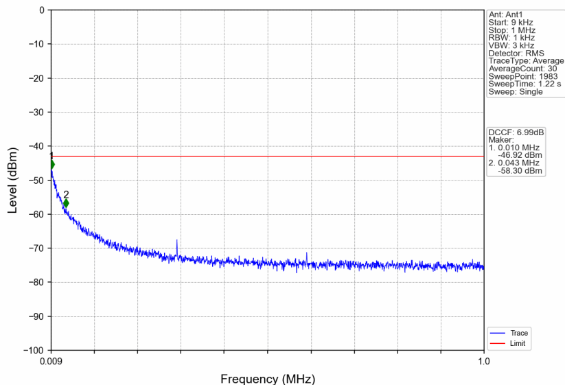
n38_30kHz_SISO_NTNV_25MHz_CP-OFDM QPSK_2607.5MHz_Edge_1RB_Right
