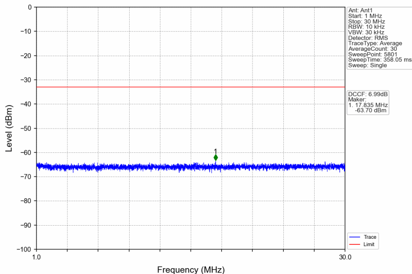
n38_30kHz_SISO_NTNV_25MHz_CP-OFDM QPSK_2595MHz_Edge_1RB_Left
