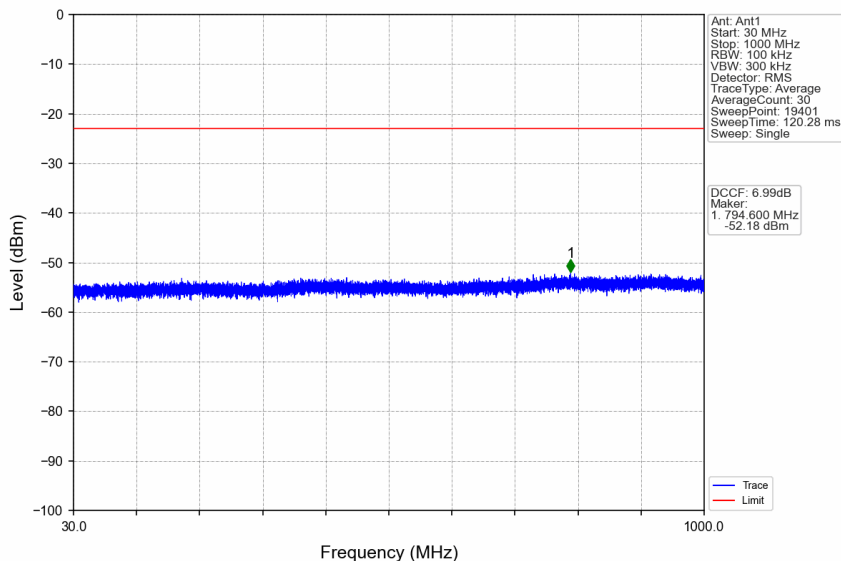
n38_30kHz_SISO_NTNV_25MHz_DFT-s-OFDM QPSK_2607.5MHz_Edge_1RB_Right
