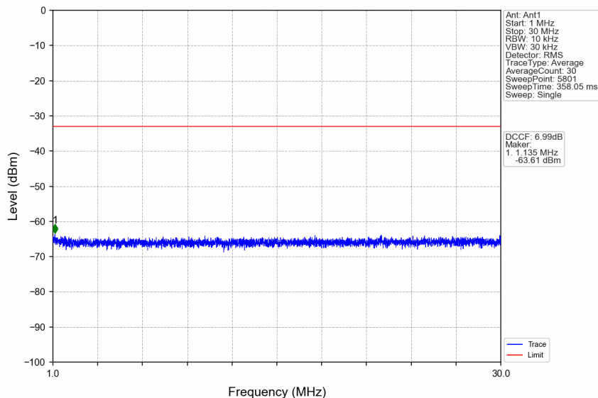
n38_30kHz_SISO_NTNV_25MHz_DFT-s-OFDM QPSK_2595MHz_Edge_1RB_Left
