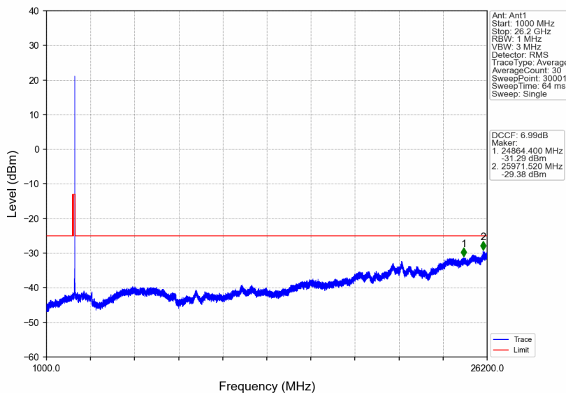
n38_30kHz_SISO_NTNV_20MHz_CP-OFDM QPSK_2610MHz_Edge_1RB_Right
