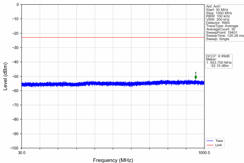
n38_30kHz_SISO_NTNV_25MHz_DFT-s-OFDM_QPSK_2582.5MHz_Edge_1RB_Left
