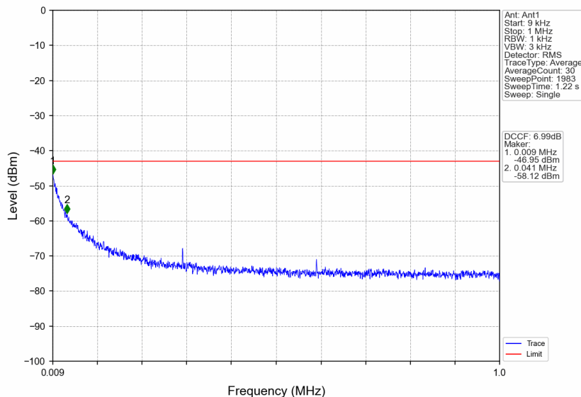
n38_30kHz_SISO_NTNV_20MHz_CP-OFDM QPSK_2610MHz_Edge_1RB_Right
