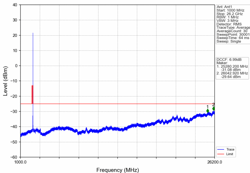
n38_30kHz_SISO_NTNV_25MHz_DFT-s-OFDM QPSK_2607.5MHz_Edge_1RB_Right
