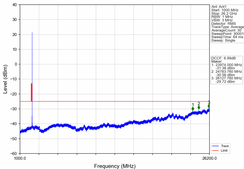
n38_30kHz_SISO_NTNV_20MHz_DFT-s-OFDM QPSK_2610MHz_Edge_1RB_Right
