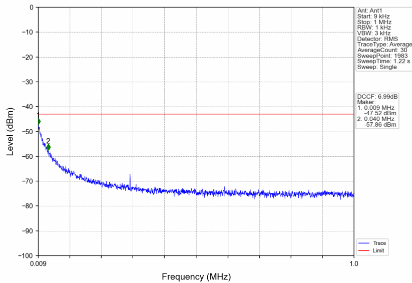
n38_30kHz_SISO_NTNV_25MHz_DFT-s-OFDM PI/2 BPSK_2607.5MHz_Edge_1RB_Right
