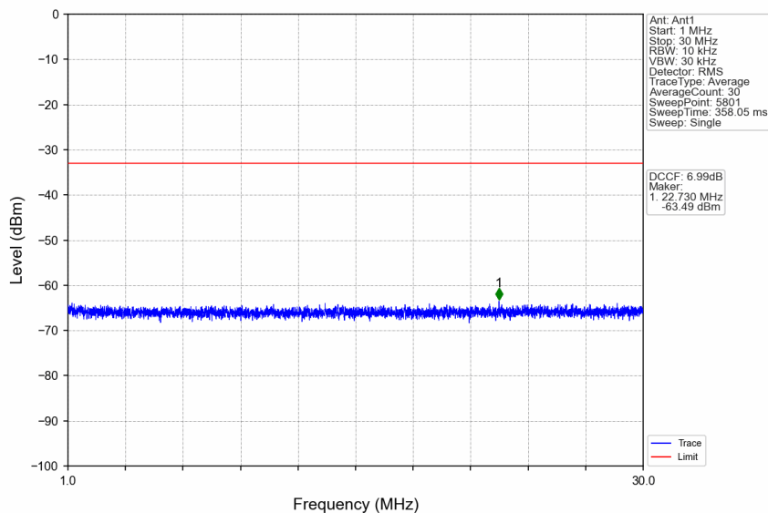
n38_30kHz_SISO_NTNV_20MHz_CP-OFDM QPSK_2610MHz_Edge_1RB_Right
