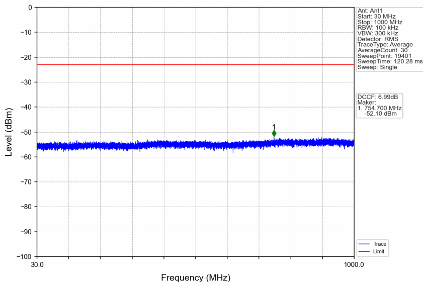
n38_30kHz_SISO_NTNV_20MHz_CP-OFDM QPSK_2610MHz_Edge_1RB_Right
