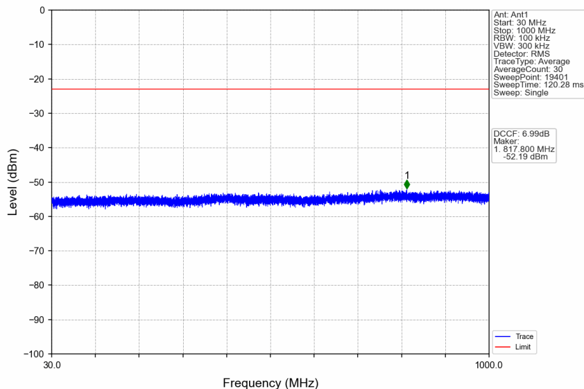
n38_30kHz_SISO_NTNV_25MHz_DFT-s-OFDM PI/2 BPSK_2607.5MHz_Edge_1RB_Right
