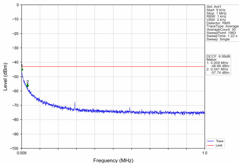
n38_30kHz_SISO_NTNV_20MHz_DFT-s-OFDM QPSK_2610MHz_Edge_1RB_Right
