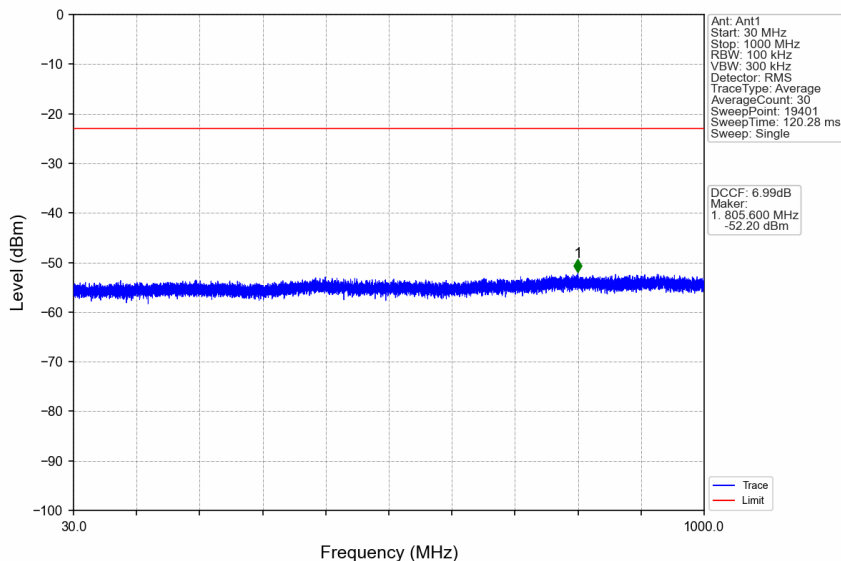
n38_30kHz_SISO_NTNV_20MHz_DFT-s-OFDM QPSK_2610MHz_Edge_1RB_Right
