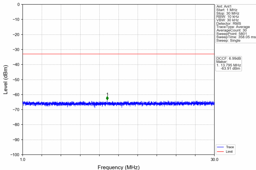
n38_30kHz_SISO_NTNV_25MHz_DFT-s-OFDM_QPSK_2582.5MHz_Edge_1RB_Left
