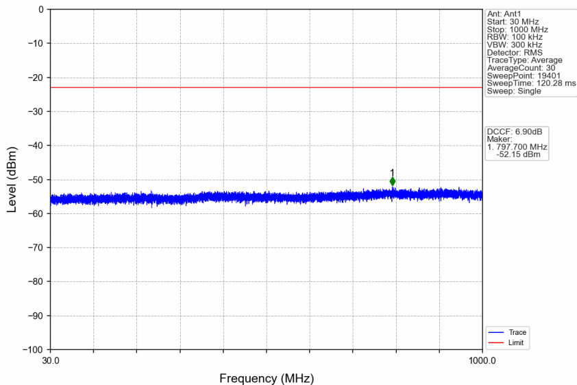
n38_30kHz_SISO_NTNV_25MHz_CP-OFDM QPSK_2582.5MHz_Edge_1RB_Left
