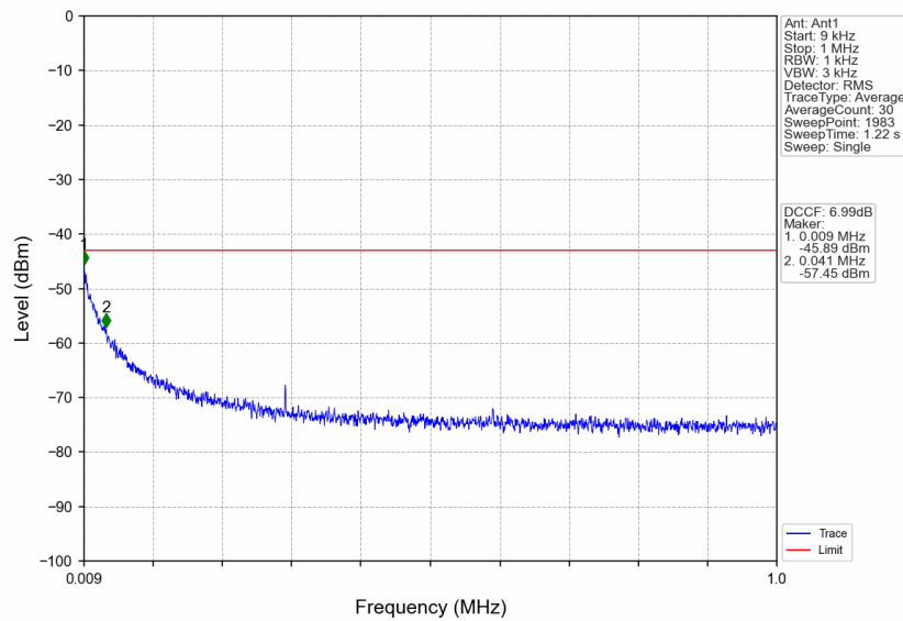
n38_30kHz_SISO_NTNV_25MHz_DFT-s-OFDM QPSK_2607.5MHz_Edge_1RB_Right
