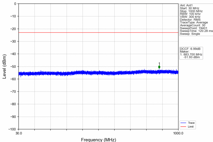
n38_30kHz_SISO_NTNV_15MHz_CP-OFDM QPSK_2612.5MHz_Edge_1RB_Right
