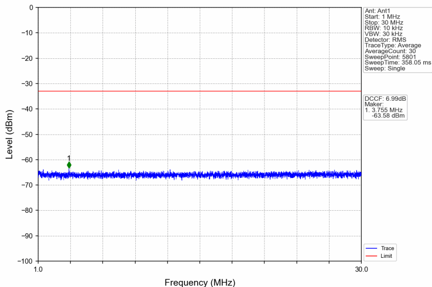
n38_30kHz_SISO_NTNV_15MHz_CP-OFDM QPSK_2595MHz_Edge_1RB_Left
