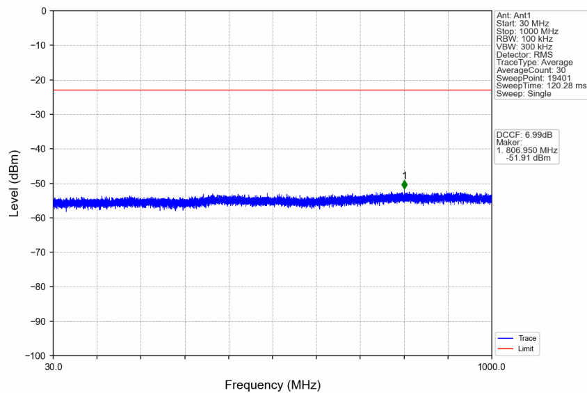
n38_30kHz_SISO_NTNV_10MHz_CP-OFDM QPSK_2575MHz_Edge_1RB_Left
