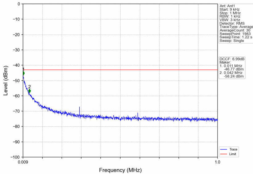
n38_30kHz_SISO_NTNV_10MHz_CP-OFDM QPSK_2615MHz_Edge_1RB_Right
