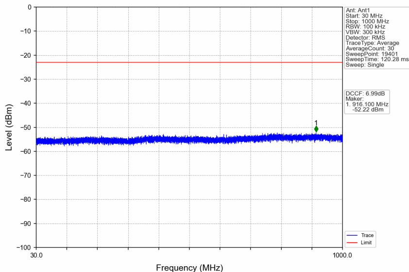
n38_30kHz_SISO_NTNV_15MHz_DFT-s-OFDM QPSK_2612.5MHz_Edge_1RB_Right
