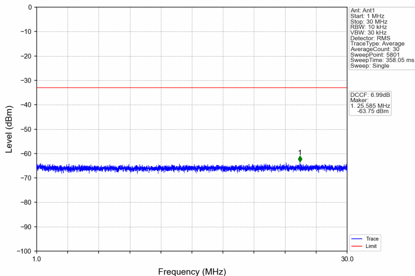
n38_30kHz_SISO_NTNV_15MHz_DFT-s-OFDM QPSK_2595MHz_Edge_1RB_Left
