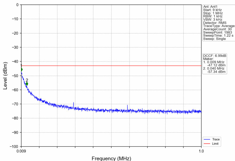
n38_30kHz_SISO_NTNV_10MHz_DFT-s-OFDM QPSK_2615MHz_Edge_1RB_Right
