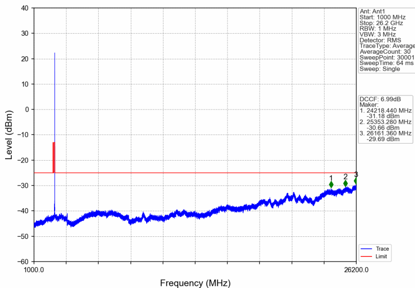
n38_30kHz_SISO_NTNV_15MHz_CP-OFDM QPSK_2612.5MHz_Edge_1RB_Right
