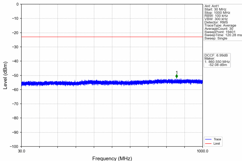
n38_30kHz_SISO_NTNV_10MHz_DFT-s-OFDM QPSK_2615MHz_Edge_1RB_Right
