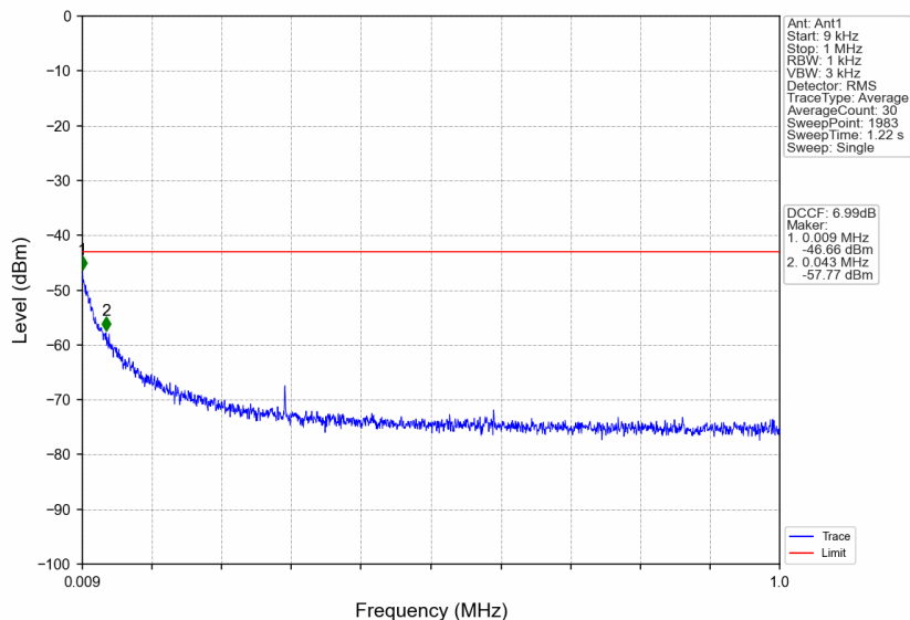
n38_30kHz_SISO_NTNV_15MHz_CP-OFDM QPSK_2612.5MHz_Edge_1RB_Right
