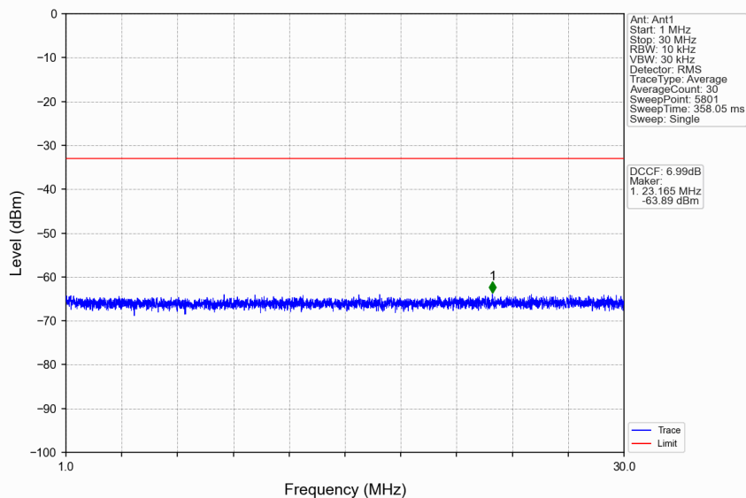
n38_30kHz_SISO_NTNV_15MHz_CP-OFDM QPSK_2612.5MHz_Edge_1RB_Right
