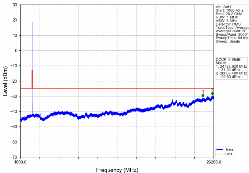
n38_30kHz_SISO_NTNV_10MHz_CP-OFDM QPSK_2615MHz_Edge_1RB_Right
