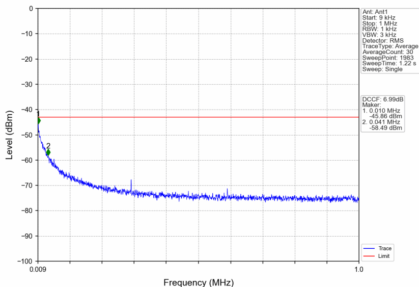
n38_30kHz_SISO_NTNV_15MHz_DFT-s-OFDM QPSK_2612.5MHz_Edge_1RB_Right
