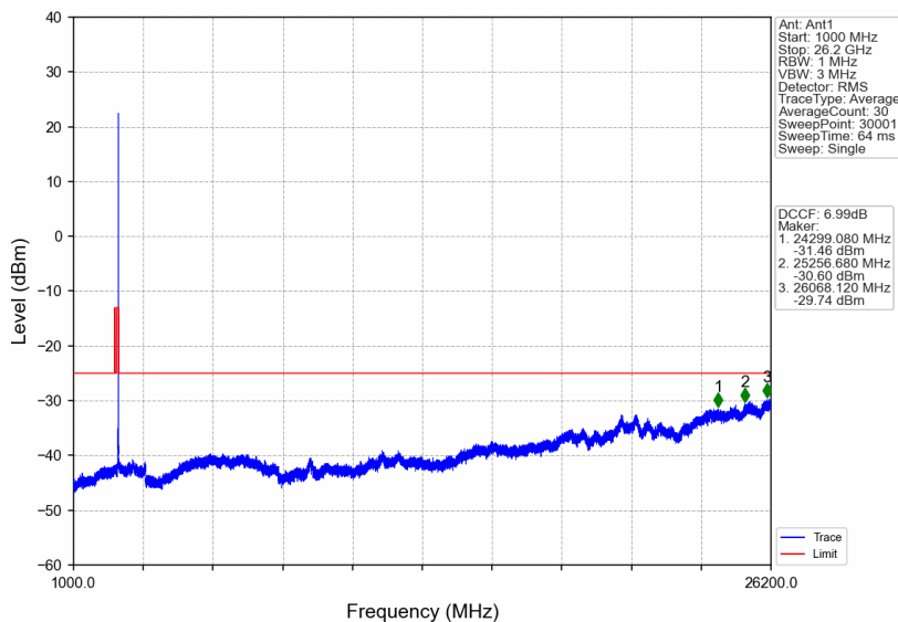
n38_30kHz_SISO_NTNV_15MHz_DFT-s-OFDM QPSK_2612.5MHz_Edge_1RB_Right
