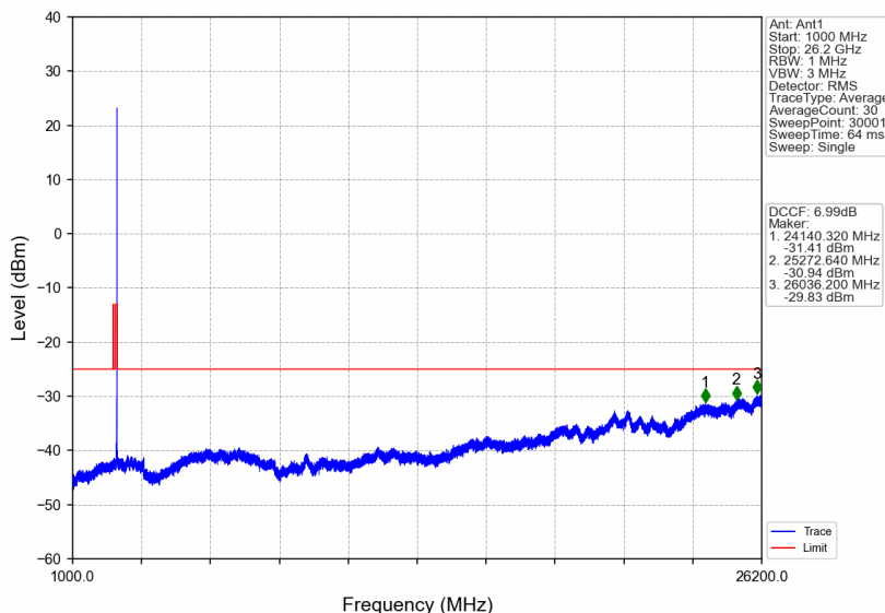
n38_30kHz_SISO_NTNV_10MHz_DFT-s-OFDM QPSK_2615MHz_Edge_1RB_Right
