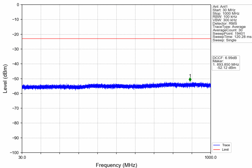
n38_30kHz_SISO_NTNV_15MHz_DFT-s-OFDM_QPSK_2577.5MHz_Edge_1RB_Left
