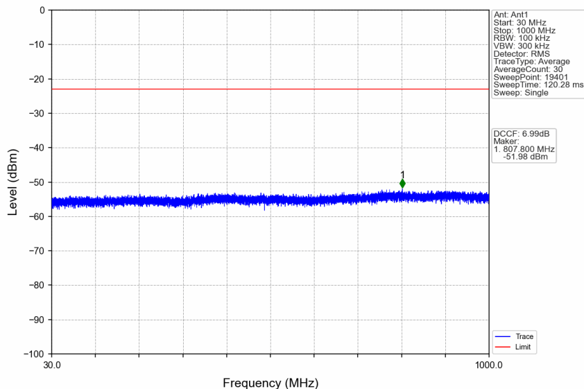
n38_30kHz_SISO_NTNV_10MHz_CP-OFDM QPSK_2615MHz_Edge_1RB_Right
