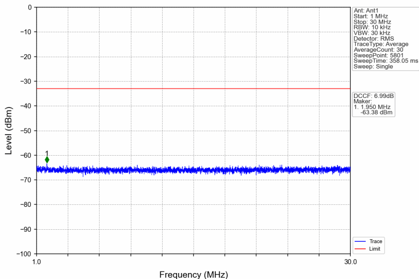
n38_30kHz_SISO_NTNV_15MHz_DFT-s-OFDM_QPSK_2577.5MHz_Edge_1RB_Left
