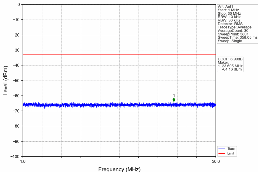
n38_15kHz_SISO_NTNV_40MHz_DFT-s-OFDM QPSK_2595MHz_Edge_1RB_Left
