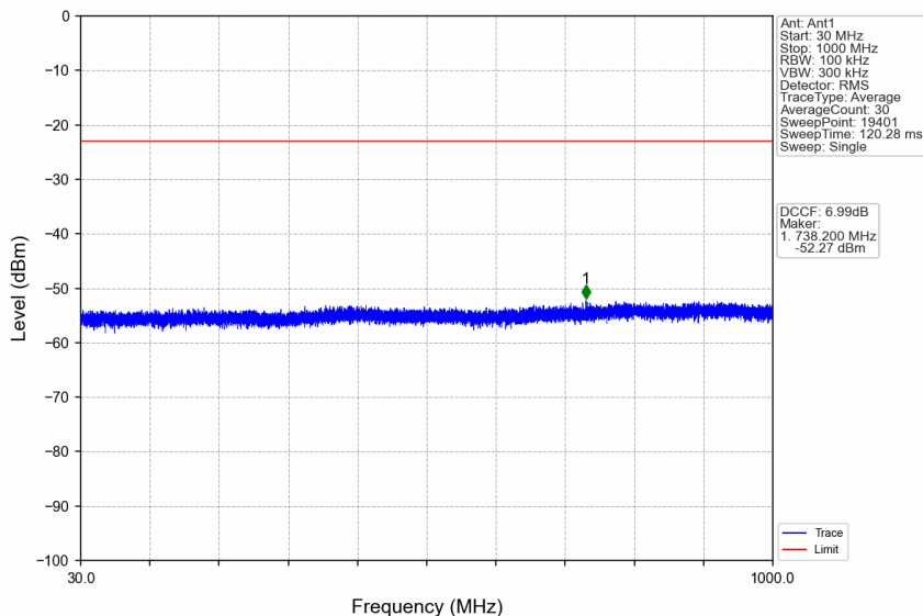
n38_15kHz_SISO_NTNV_30MHz_CP-OFDM QPSK_2605MHz_Edge_1RB_Right
