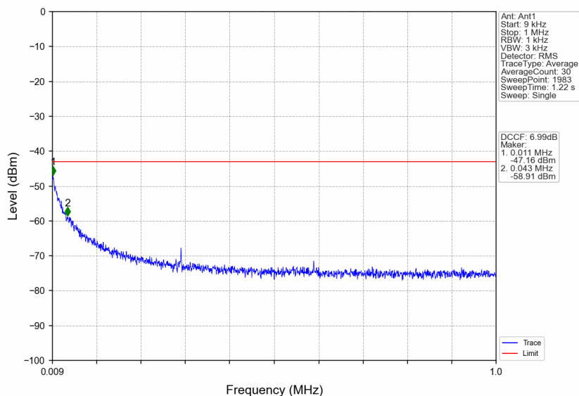
n38_15kHz_SISO_NTNV_40MHz_CP-OFDM QPSK_2600MHz_Edge_1RB_Right
