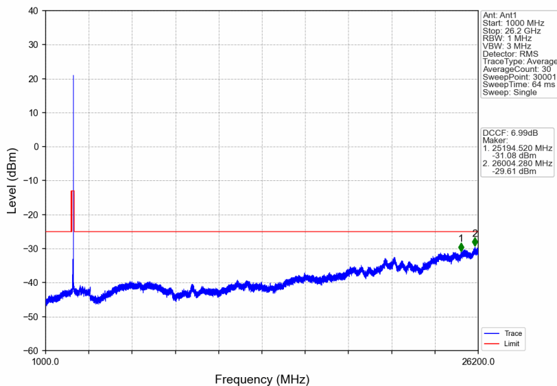
n38_15kHz_SISO_NTNV_40MHz_DFT-s-OFDM QPSK_2600MHz_Edge_1RB_Right
