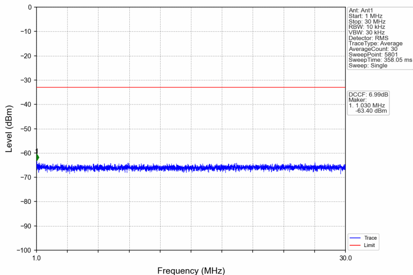
n38_30kHz_SISO_NTNV_10MHz_DFT-s-OFDM QPSK_2575MHz_Edge_1RB_Left
