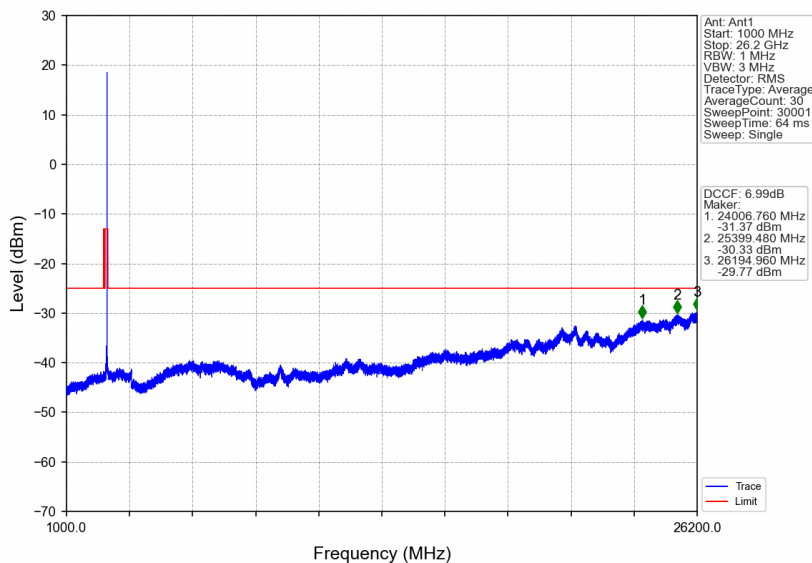
n38_15kHz_SISO_NTNV_30MHz_CP-OFDM QPSK_2605MHz_Edge_1RB_Right
