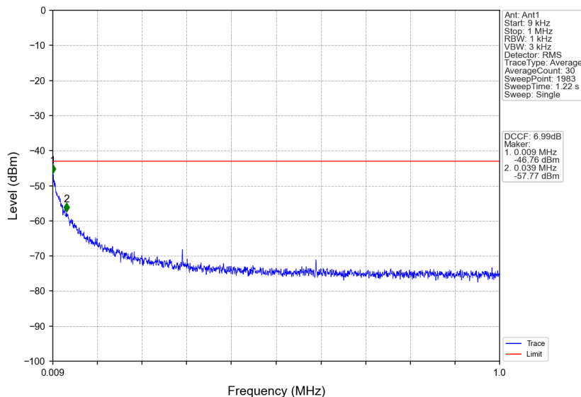
n38_15kHz_SISO_NTNV_30MHz_CP-OFDM QPSK_2605MHz_Edge_1RB_Right
