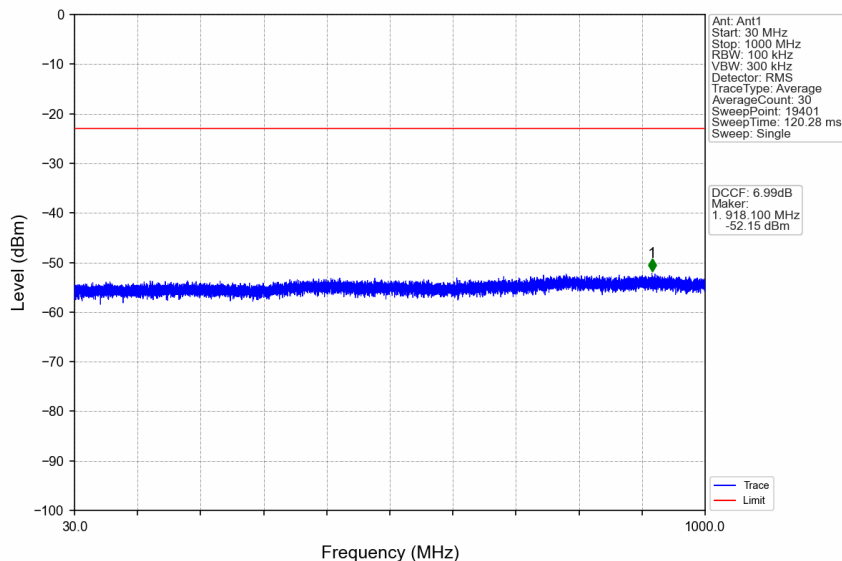
n38_15kHz_SISO_NTNV_40MHz_DFT-s-OFDM QPSK_2600MHz_Edge_1RB_Right
