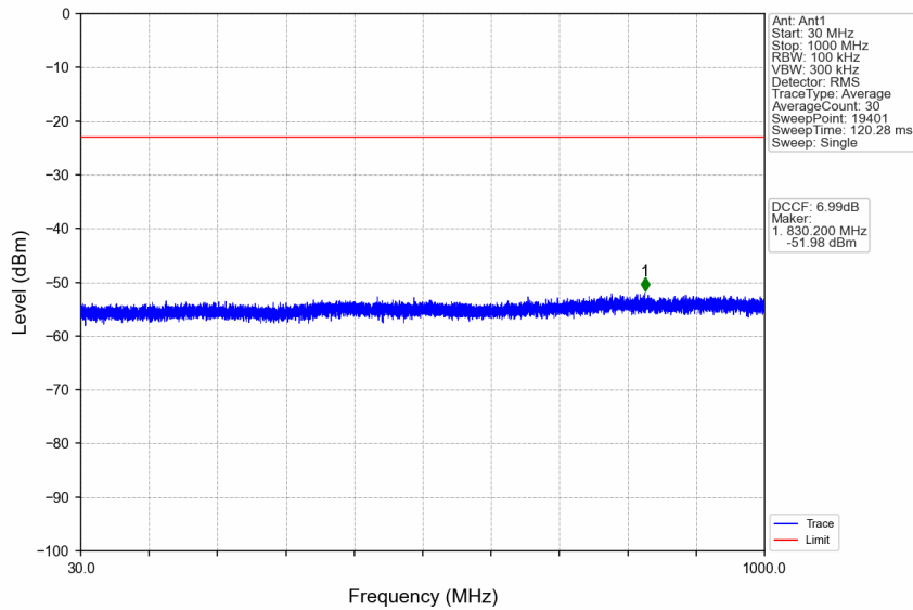
n38_15kHz_SISO_NTNV_40MHz_CP-OFDM QPSK_2600MHz_Edge_1RB_Right
