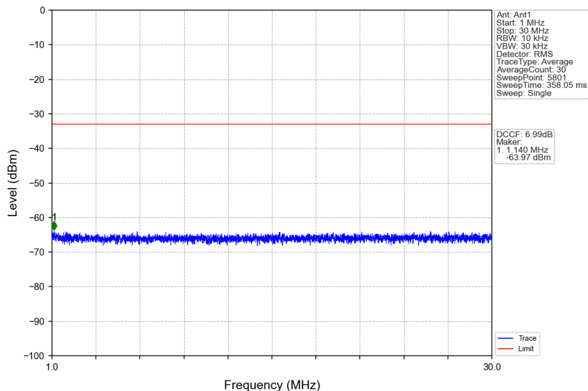
n38_15kHz_SISO_NTNV_30MHz_CP-OFDM QPSK_2595MHz_Edge_1RB_Left
