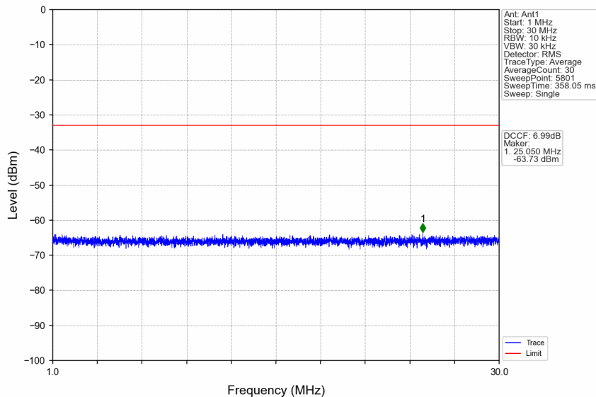
n38_15kHz_SISO_NTNV_30MHz_CP-OFDM QPSK_2605MHz_Edge_1RB_Right
