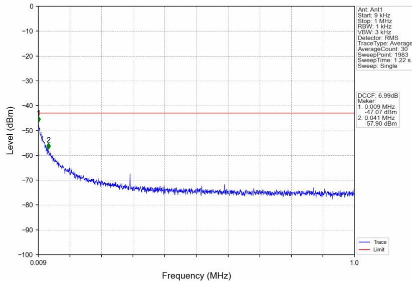
n38_15kHz_SISO_NTNV_40MHz_DFT-s-OFDM QPSK_2600MHz_Edge_1RB_Right
