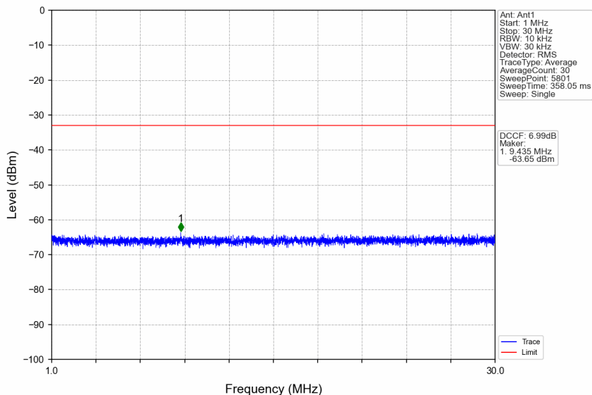
n38_15kHz_SISO_NTNV_30MHz_DFT-s-OFDM QPSK_2585MHz_Edge_1RB_Left
