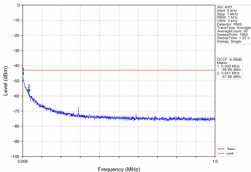
n38_15kHz_SISO_NTNV_25MHz_DFT-s-OFDM QPSK_2607.5MHz_Edge_1RB_Right
