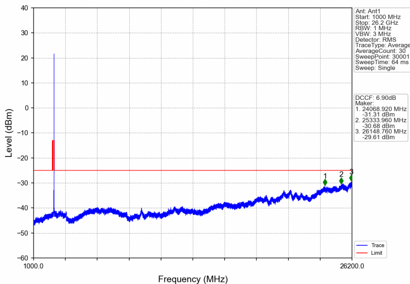
n38_15kHz_SISO_NTNV_25MHz_CP-OFDM QPSK_2607.5MHz_Edge_1RB_Right
