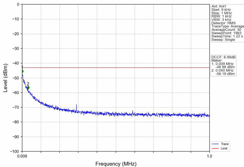
n38_15kHz_SISO_NTNV_30MHz_DFT-s-OFDM QPSK_2605MHz_Edge_1RB_Right
