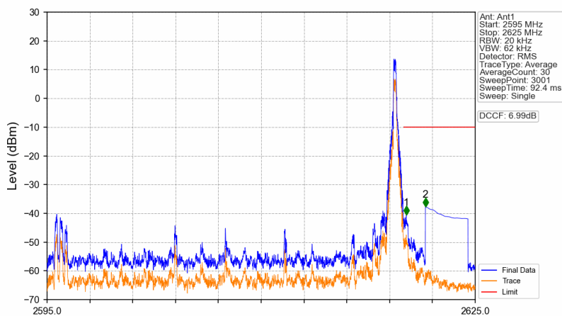
n38_15kHz_SISO_NTNV_25MHz_DFT-s-OFDM PI/2 BPSK_2607.5MHz_Edge_1RB_Right
