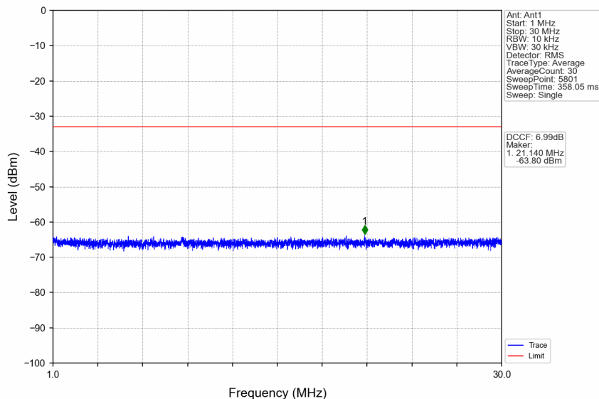
n38_15kHz_SISO_NTNV_25MHz_DFT-s-OFDM QPSK_2582.5MHz_Edge_1RB_Left
