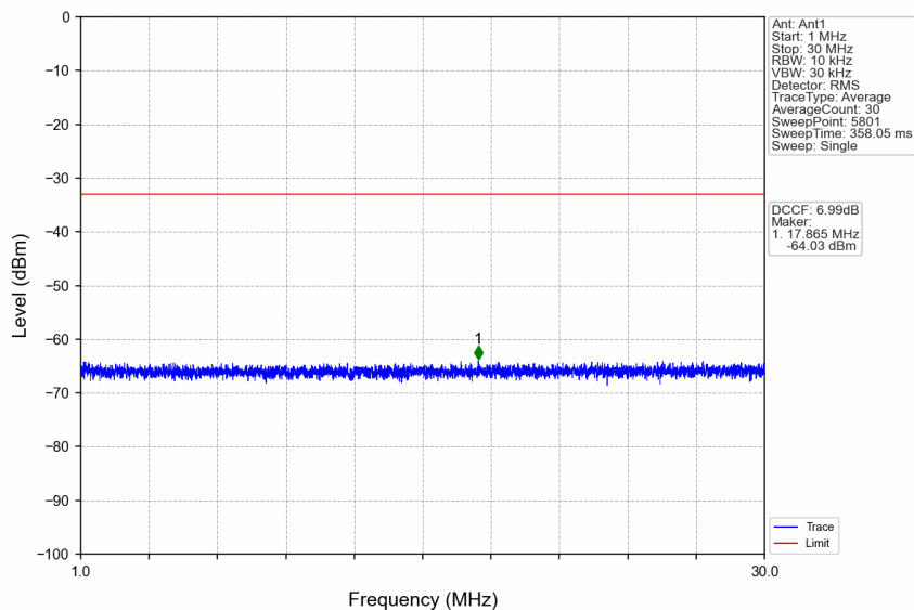
n38_15kHz_SISO_NTNV_25MHz_DFT-s-OFDM QPSK_2607.5MHz_Edge_1RB_Right
