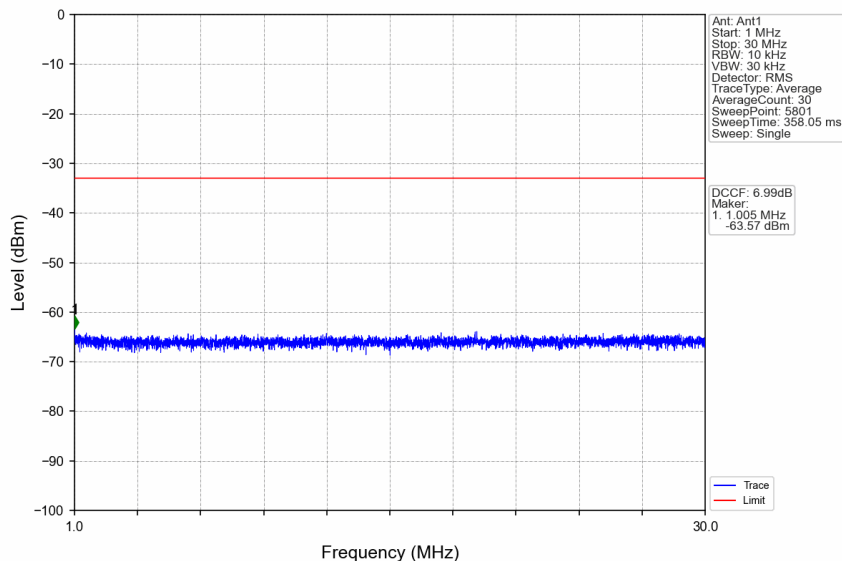
n38_15kHz_SISO_NTNV_30MHz_DFT-s-OFDM QPSK_2595MHz_Edge_1RB_Left
