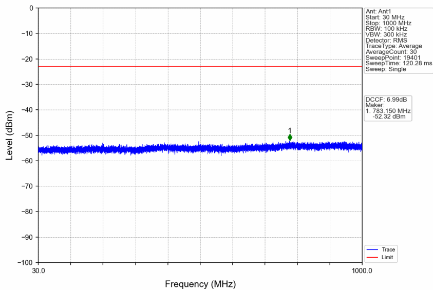
n38_15kHz_SISO_NTNV_30MHz_CP-OFDM QPSK_2585MHz_Edge_1RB_Left
