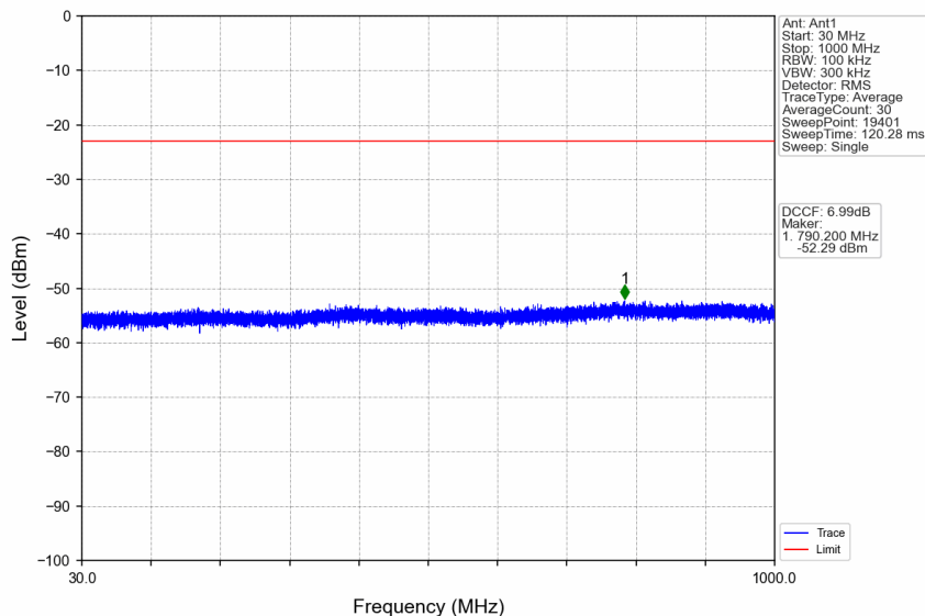
n38_15kHz_SISO_NTNV_25MHz_DFT-s-OFDM QPSK_2607.5MHz_Edge_1RB_Right
