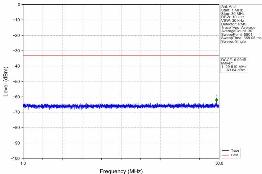
n38_15kHz_SISO_NTNV_25MHz_CP-OFDM QPSK_2595MHz_Edge_1RB_Left
