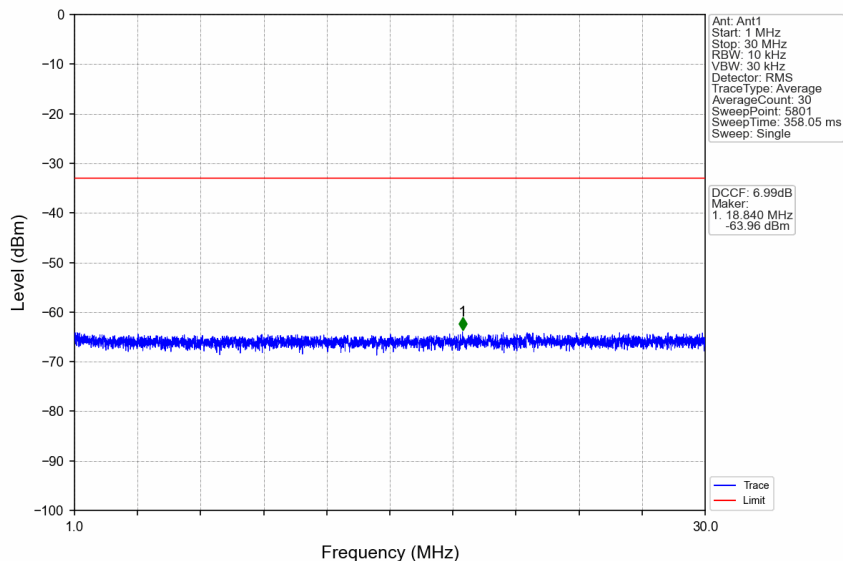
n38_15kHz_SISO_NTNV_25MHz_DFT-s-OFDM QPSK_2595MHz_Edge_1RB_Left
