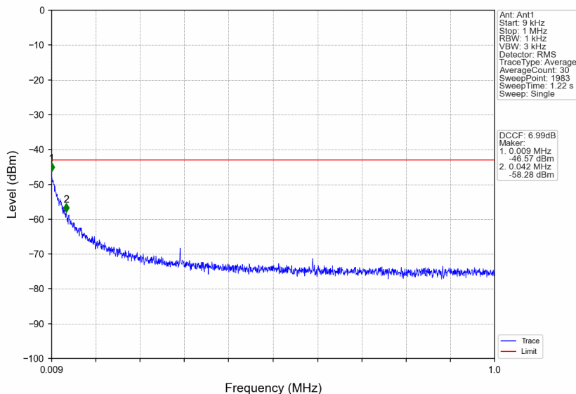
n38_15kHz_SISO_NTNV_20MHz_CP-OFDM QPSK_2610MHz_Edge_1RB_Right
