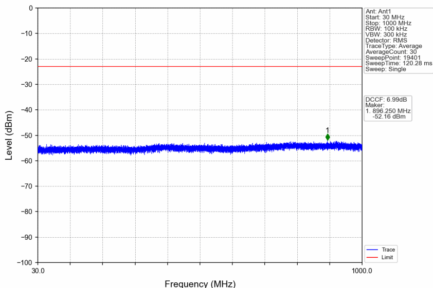
n38_15kHz_SISO_NTNV_15MHz_CP-OFDM QPSK_2595MHz_Edge_1RB_Left
