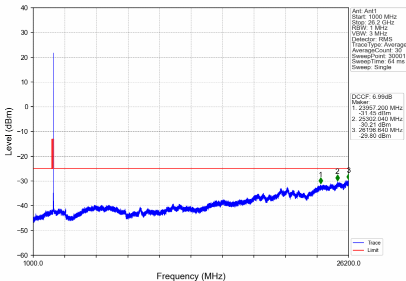
n38_15kHz_SISO_NTNV_20MHz_DFT-s-OFDM QPSK_2610MHz_Edge_1RB_Right
