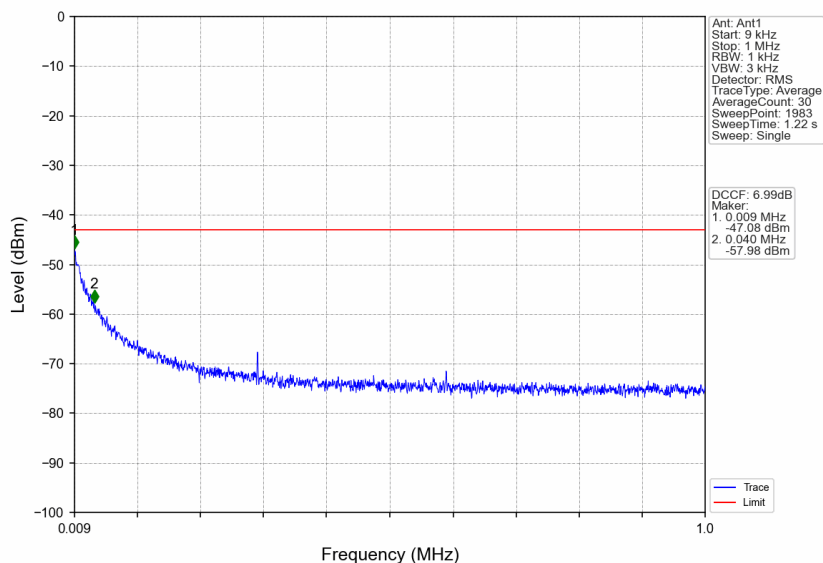
n38_15kHz_SISO_NTNV_15MHz_CP-OFDM QPSK_2612.5MHz_Edge_1RB_Right
