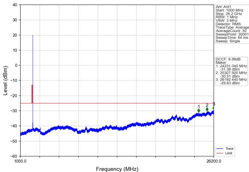
n38_15kHz_SISO_NTNV_15MHz_CP-OFDM QPSK_2612.5MHz_Edge_1RB_Right
