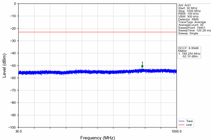
n38_15kHz_SISO_NTNV_20MHz_CP-OFDM QPSK_2610MHz_Edge_1RB_Right
