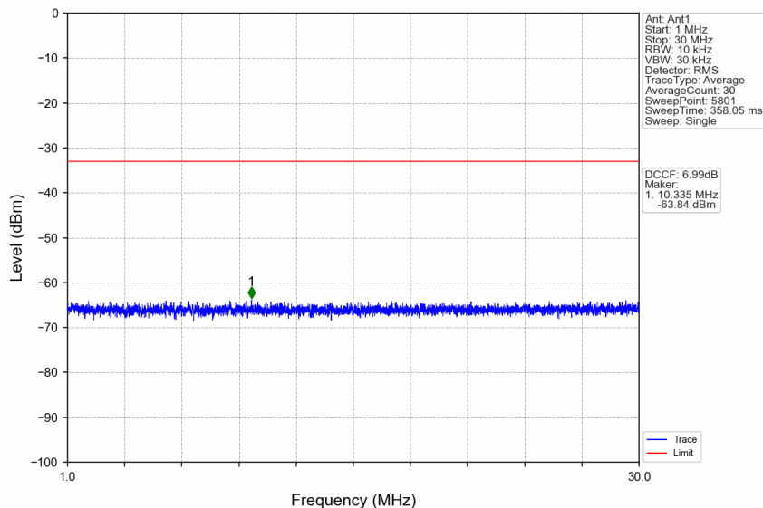
n38_15kHz_SISO_NTNV_15MHz_DFT-s-OFDM QPSK_2577.5MHz_Edge_1RB_Left
