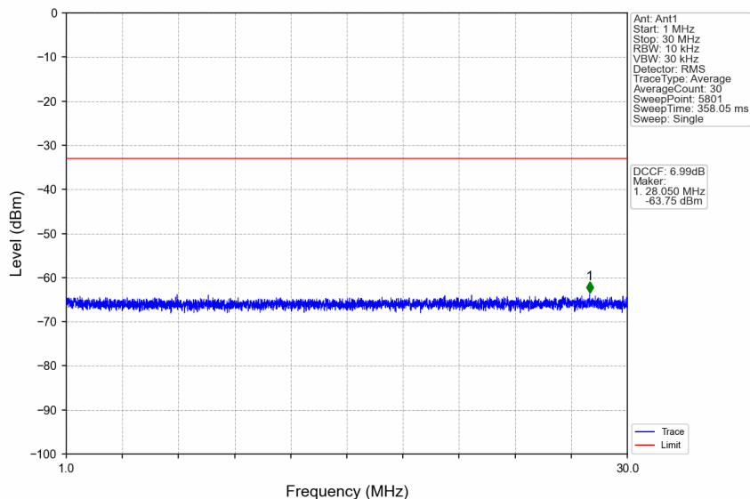
n38_15kHz_SISO_NTNV_15MHz_DFT-s-OFDM QPSK_2595MHz_Edge_1RB_Left
