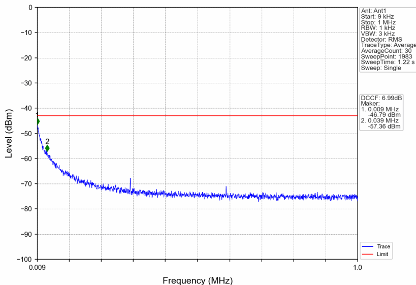
n38_15kHz_SISO_NTNV_20MHz_DFT-s-OFDM QPSK_2610MHz_Edge_1RB_Right
