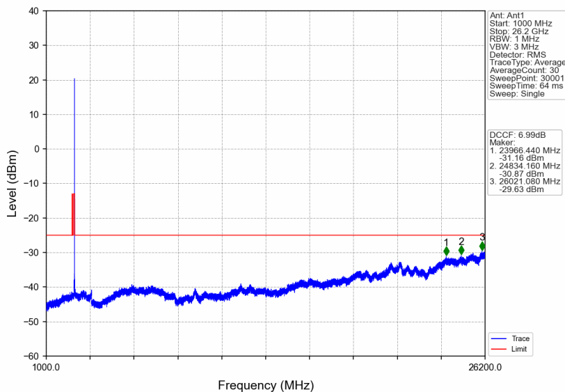
n38_15kHz_SISO_NTNV_15MHz_DFT-s-OFDM QPSK_2612.5MHz_Edge_1RB_Right
