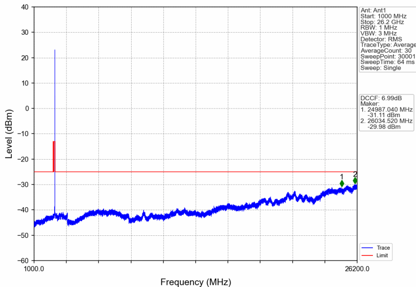
n38_15kHz_SISO_NTNV_20MHz_CP-OFDM QPSK_2610MHz_Edge_1RB_Right
