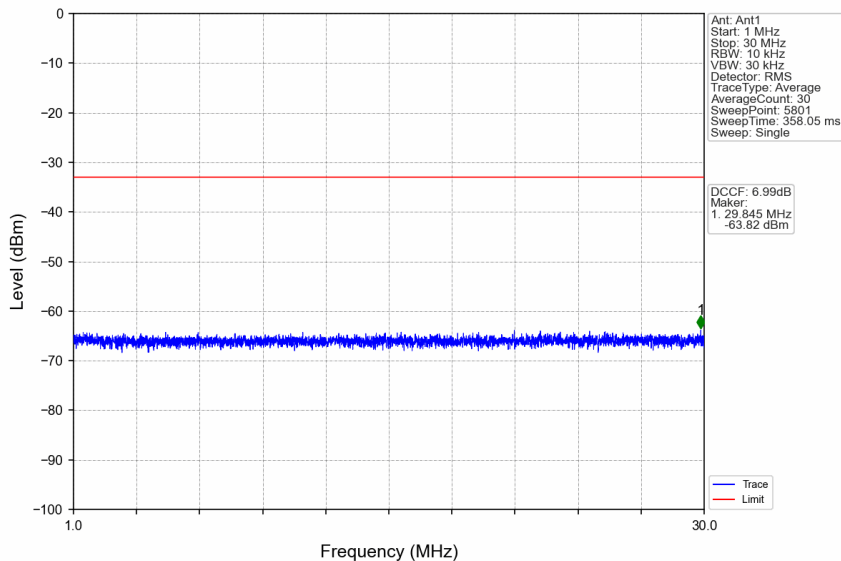
n38_15kHz_SISO_NTNV_20MHz_DFT-s-OFDM QPSK_2610MHz_Edge_1RB_Right
