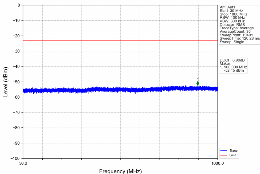
n38_15kHz_SISO_NTNV_20MHz_DFT-s-OFDM QPSK_2610MHz_Edge_1RB_Right
