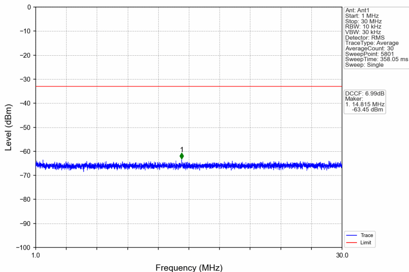
n38_15kHz_SISO_NTNV_15MHz_CP-OFDM QPSK_2577.5MHz_Edge_1RB_Left
