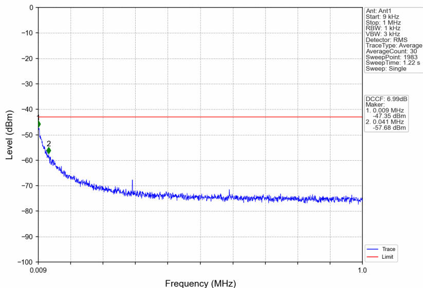
n38_15kHz_SISO_NTNV_15MHz_DFT-s-OFDM QPSK_2612.5MHz_Edge_1RB_Right
