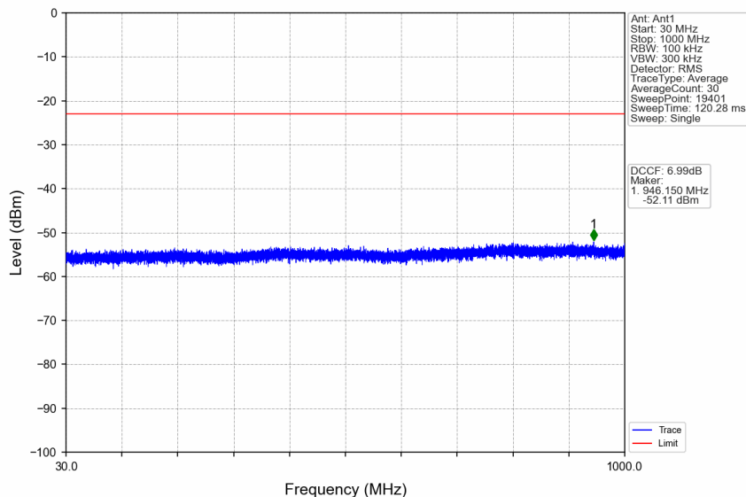
n38_15kHz_SISO_NTNV_15MHz_DFT-s-OFDM QPSK_2612.5MHz_Edge_1RB_Right
