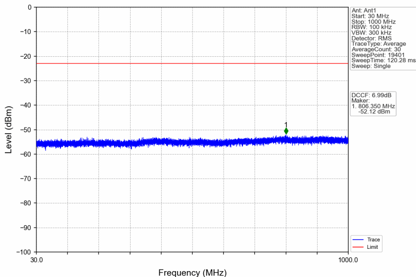
n38_15kHz_SISO_NTNV_15MHz_CP-OFDM QPSK_2612.5MHz_Edge_1RB_Right
