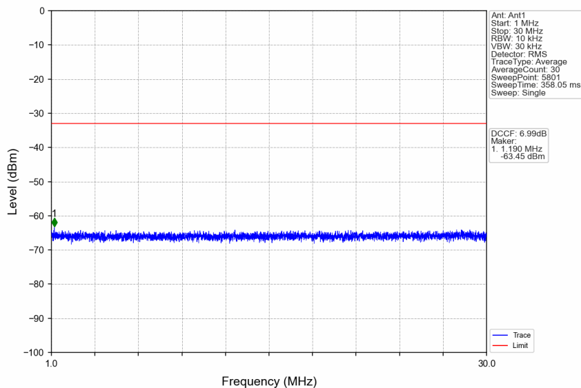
n38_15kHz_SISO_NTNV_5MHz_CP-OFDM QPSK_2617.5MHz_Edge_1RB_Right
