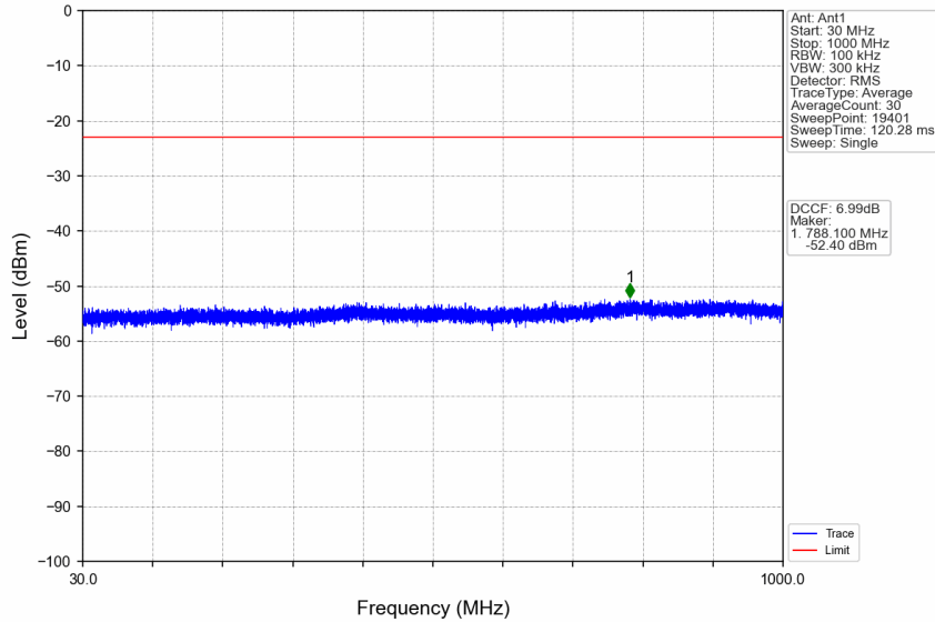
n38_15kHz_SISO_NTNV_10MHz_DFT-s-OFDM_QPSK_2615MHz_Edge_1RB_Right
