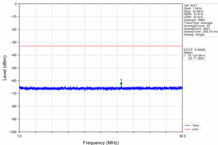
n38_15kHz_SISO_NTNV_10MHz_CP-OFDM QPSK_2575MHz_Edge_1RB_Left
