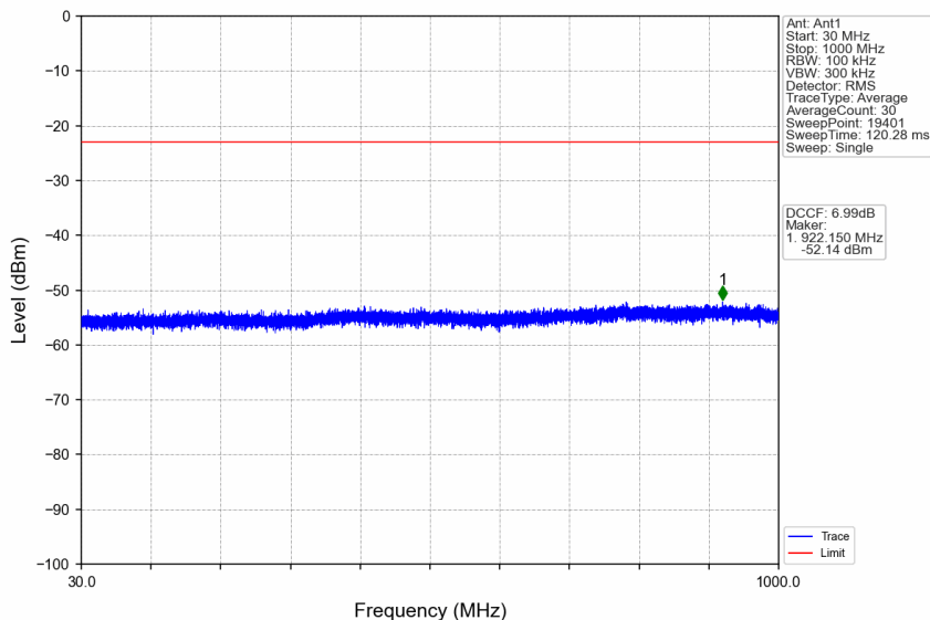
n38_15kHz_SISO_NTNV_10MHz_CP-OFDM QPSK_2615MHz_Edge_1RB_Right
