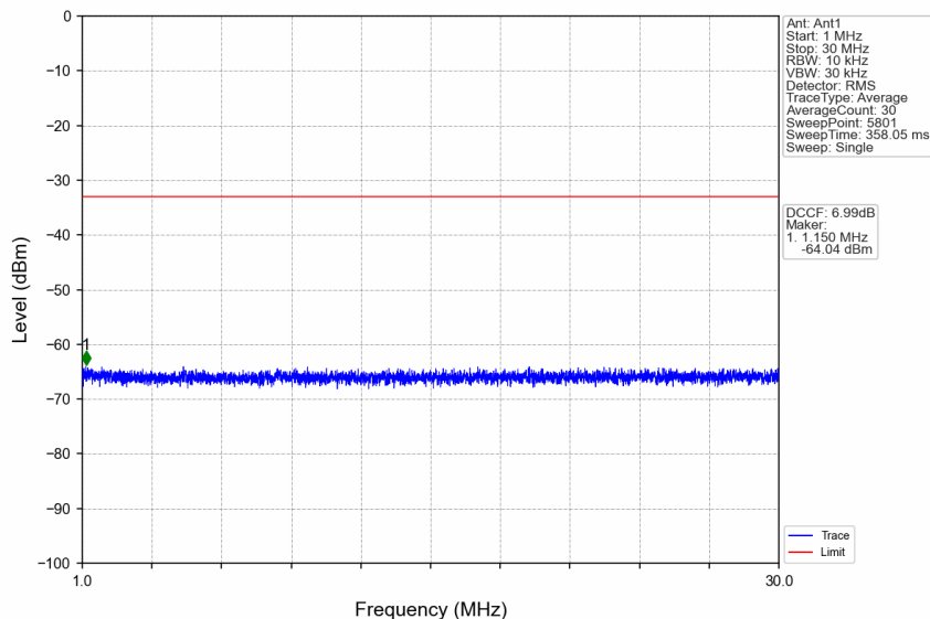
n38_15kHz_SISO_NTNV_10MHz_DFT-s-OFDM QPSK_2575MHz_Edge_1RB_Left
