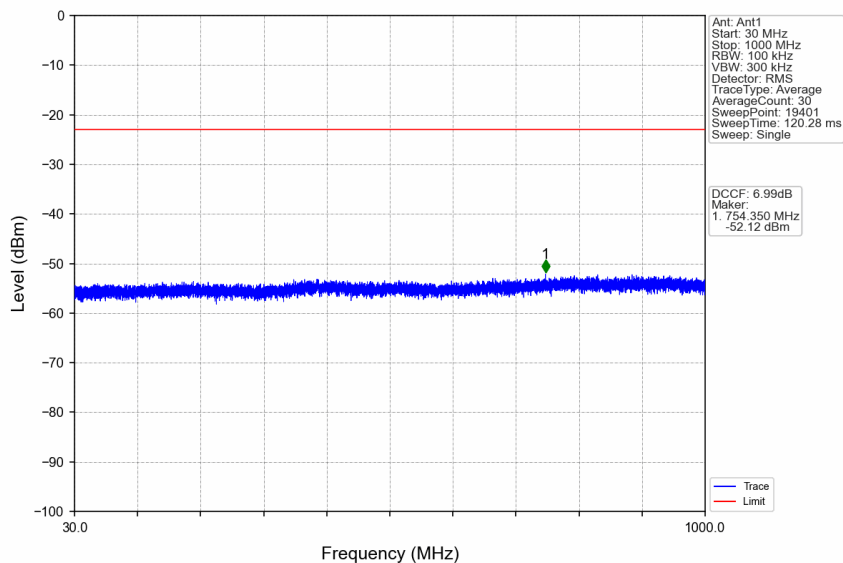
n38_15kHz_SISO_NTNV_5MHz_CP-OFDM QPSK_2572.5MHz_Edge_1RB_Left
