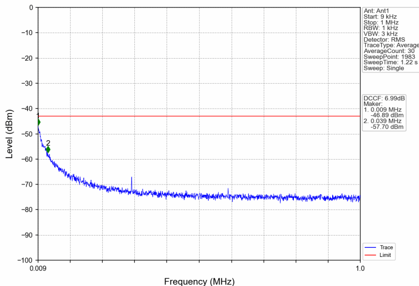
n38_15kHz_SISO_NTNV_10MHz_CP-OFDM QPSK_2615MHz_Edge_1RB_Right
