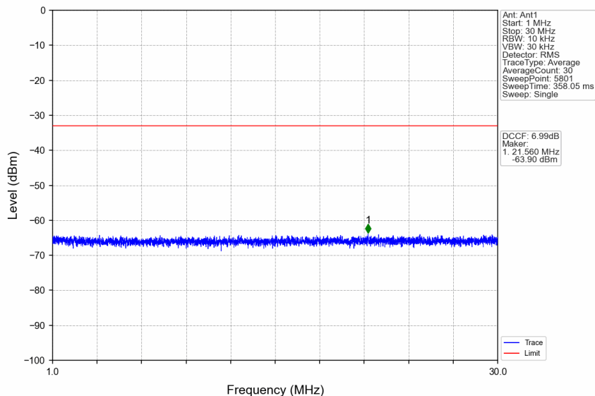
n38_15kHz_SISO_NTNV_10MHz_DFT-s-OFDM QPSK_2595MHz_Edge_1RB_Left
