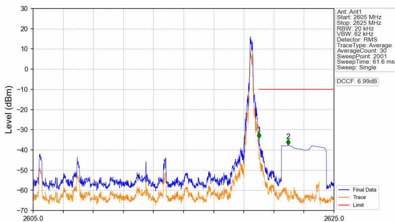
n38_15kHz_SISO_NTNV_15MHz_DFT-s-OFDM PI/2 BPSK_2612.5MHz_Edge_1RB_Right
