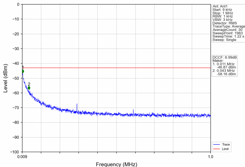
n38_15kHz_SISO_NTNV_5MHz_CP-OFDM QPSK_2617.5MHz_Edge_1RB_Right
