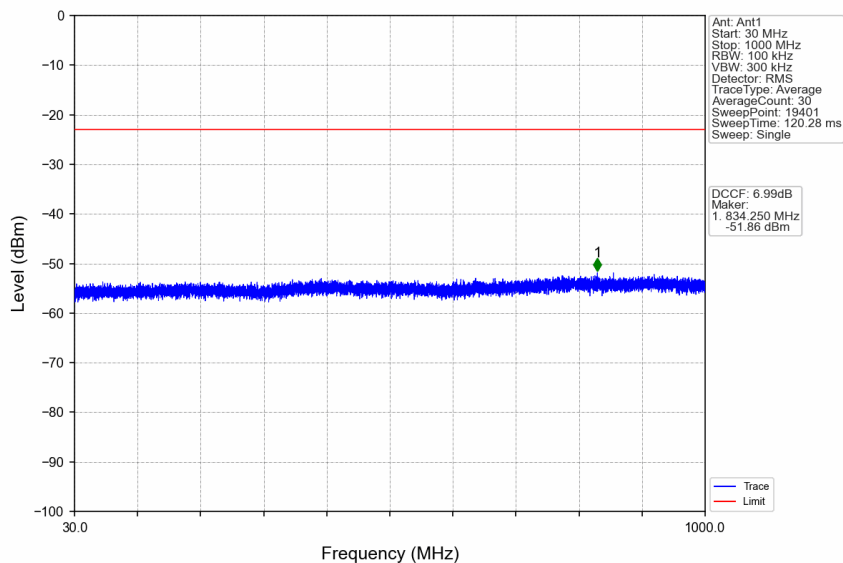
n38_15kHz_SISO_NTNV_10MHz_CP-OFDM QPSK_2575MHz_Edge_1RB_Left
