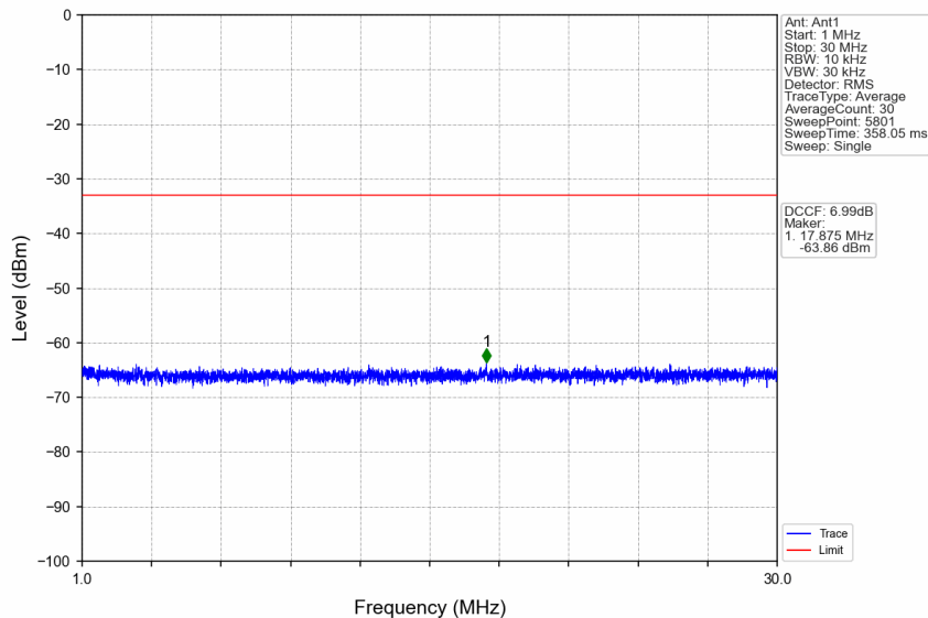
n38_15kHz_SISO_NTNV_10MHz_CP-OFDM QPSK_2615MHz_Edge_1RB_Right
