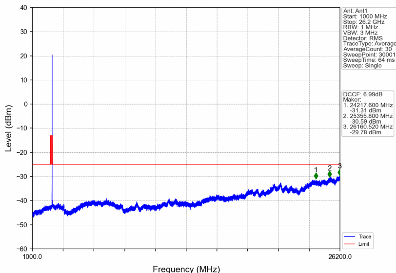
n38_15kHz_SISO_NTNV_10MHz_CP-OFDM QPSK_2615MHz_Edge_1RB_Right
