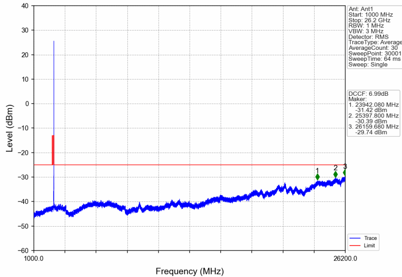
n38_15kHz_SISO_NTNV_10MHz_DFT-s-OFDM_QPSK_2615MHz_Edge_1RB_Right
