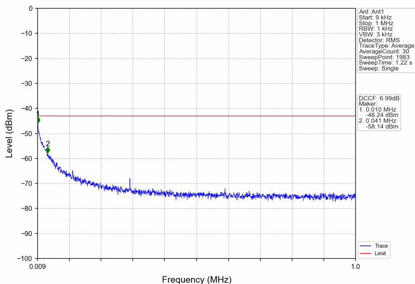
n38_15kHz_SISO_NTNV_10MHz_DFT-s-OFDM QPSK_2615MHz_Edge_1RB_Right
