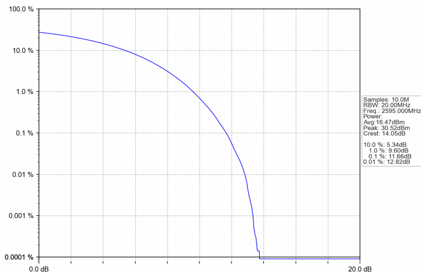
n38_30kHz_SISO_NTNV_30MHz_CP-OFDM 16 QAM_2595MHz_Outer_Full
