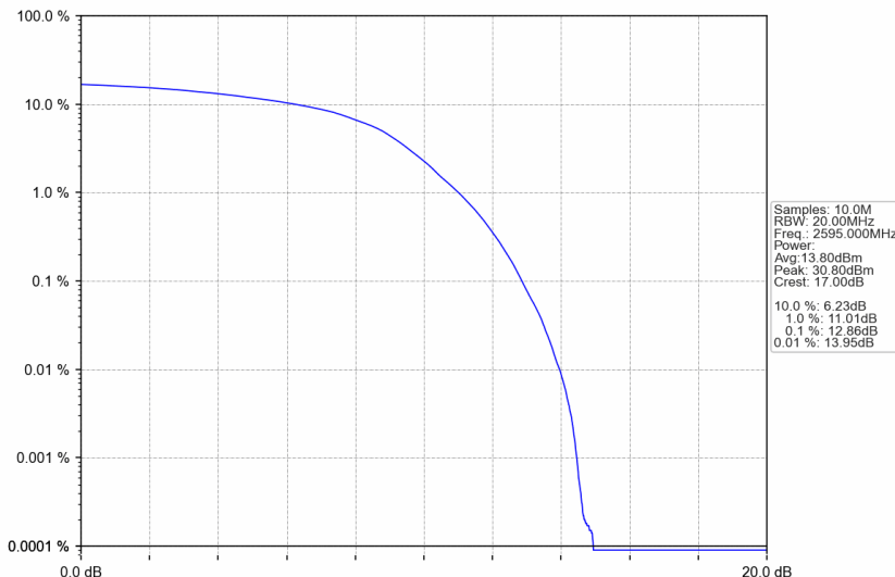
n38_30kHz_SISO_NTNV_30MHz_DFT-s-OFDM 64 QAM_2595MHz_Outer_Full
