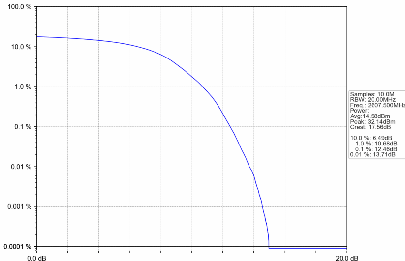
n38_30kHz_SISO_NTNV_25MHz_DFT-s-OFDM 64 QAM_2607.5MHz_Outer_Full
