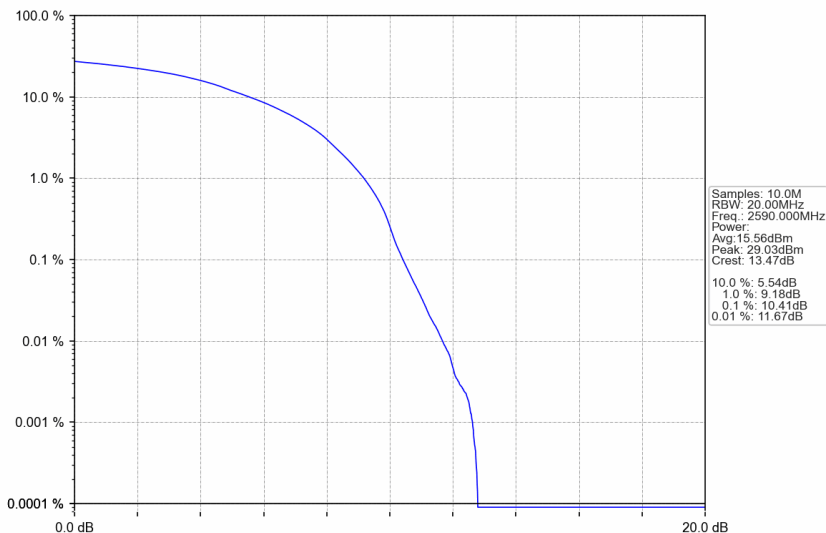
n38_30kHz_SISO_NTNV_40MHz_DFT-s-OFDM 64 QAM_2590MHz_Outer_Full
