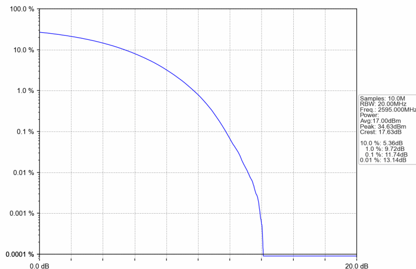
n38_30kHz_SISO_NTNV_25MHz_CP-OFDM 16 QAM_2595MHz_Outer_Full
