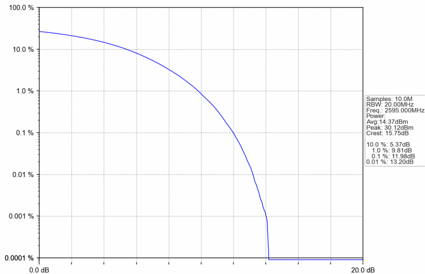
n38_30kHz_SISO_NTNV_40MHz_CP-OFDM 64 QAM_2595MHz_Outer_Full
