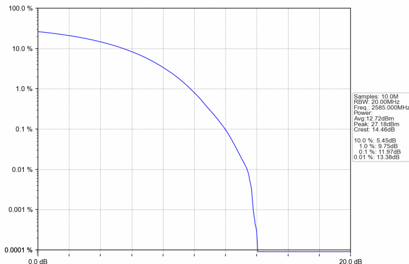
n38_30kHz_SISO_NTNV_30MHz_CP-OFDM 256 QAM_2585MHz_Outer_Full
