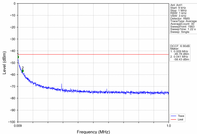
n38_15kHz_SISO_NTNV_5MHz_DFT-s-OFDM QPSK_2617.5MHz_Edge_1RB_Right
