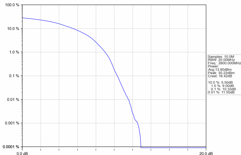
n38_30kHz_SISO_NTNV_40MHz_DFT-s-OFDM 256 QAM_2600MHz_Outer_Full
