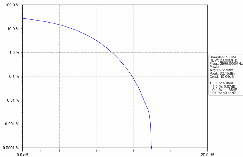
n38_30kHz_SISO_NTNV_25MHz_CP-OFDM 64 QAM_2595MHz_Outer_Full
