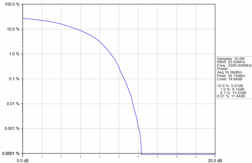
n38_30kHz_SISO_NTNV_40MHz_DFT-s-OFDM 16 QAM_2595MHz_Outer_Full
