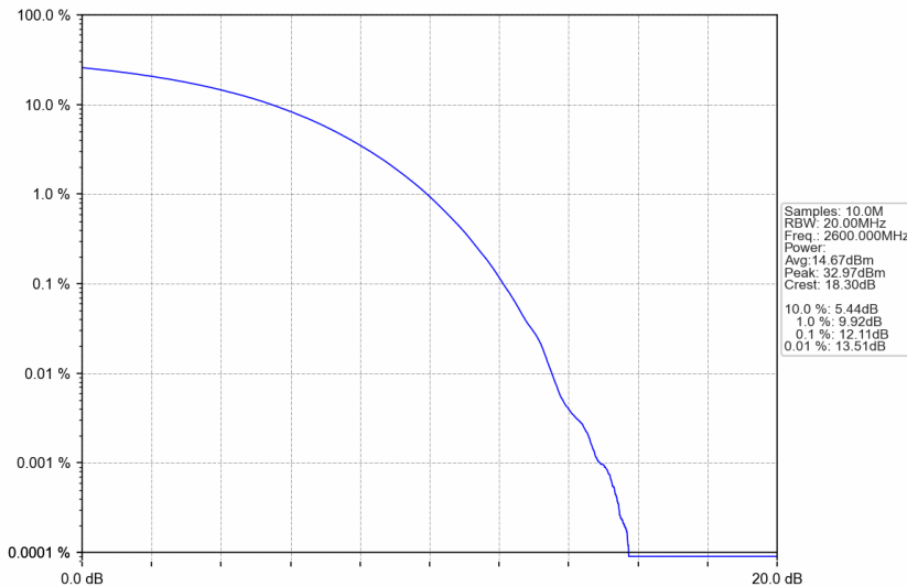
n38_30kHz_SISO_NTNV_40MHz_CP-OFDM QPSK_2600MHz_Outer_Full
