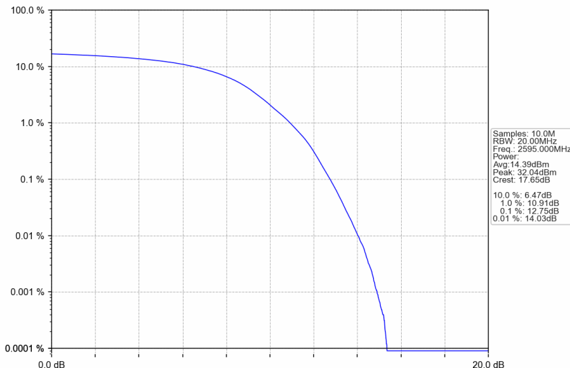
n38_30kHz_SISO_NTNV_25MHz_DFT-s-OFDM 64 QAM_2595MHz_Outer_Full
