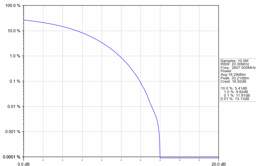
n38_30kHz_SISO_NTNV_25MHz_CP-OFDM 64 QAM_2607.5MHz_Outer_Full
