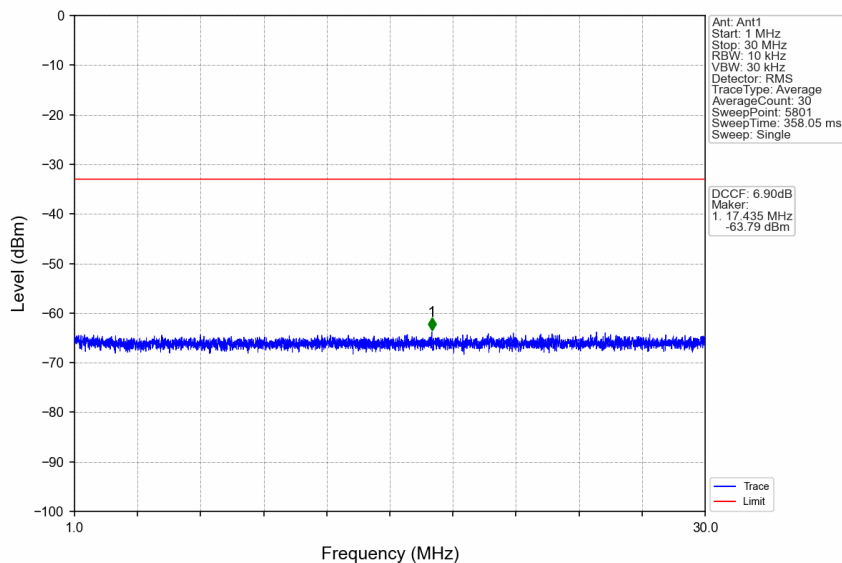
n38_15kHz_SISO_NTNV_5MHz_DFT-s-OFDM QPSK_2617.5MHz_Edge_1RB_Right
