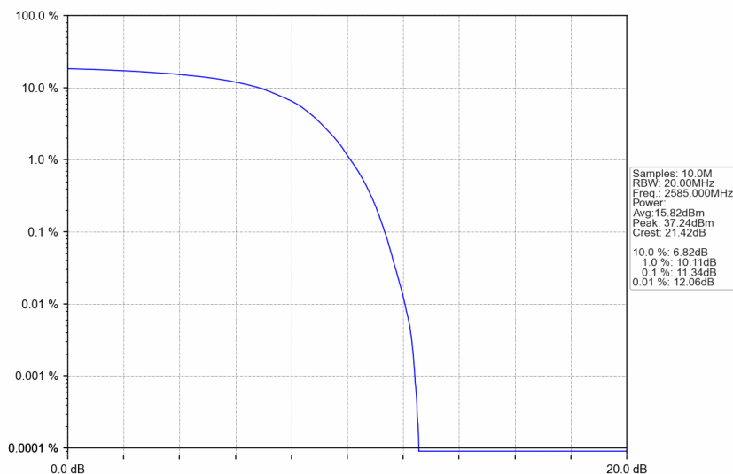
n38_30kHz_SISO_NTNV_30MHz_DFT-s-OFDM QPSK_2585MHz_Outer_Full
