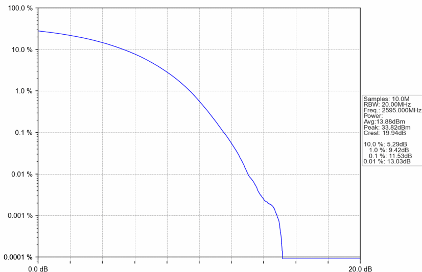
n38_30kHz_SISO_NTNV_25MHz_CP-OFDM 256 QAM_2595MHz_Outer_Full
