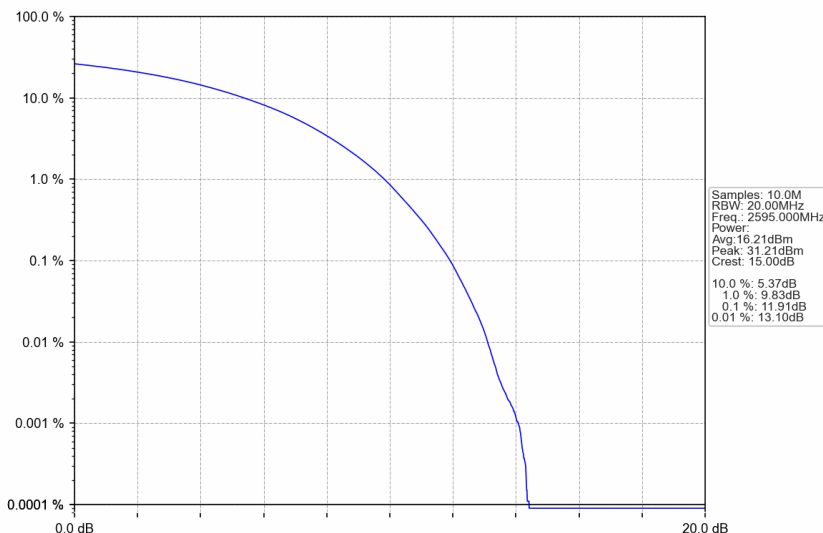
n38_30kHz_SISO_NTNV_30MHz_CP-OFDM QPSK_2595MHz_Outer_Full
