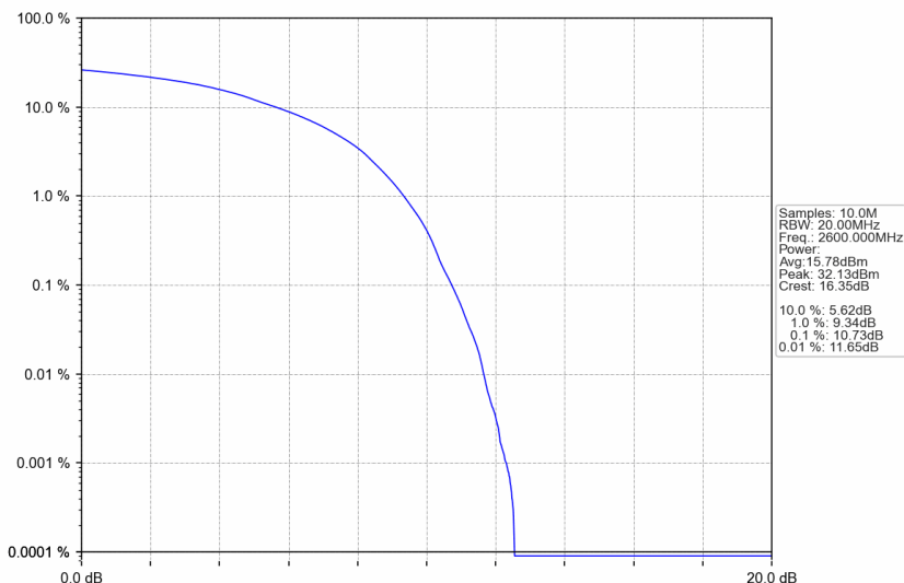
n38_30kHz_SISO_NTNV_40MHz_DFT-s-OFDM 16 QAM_2600MHz_Outer_Full
