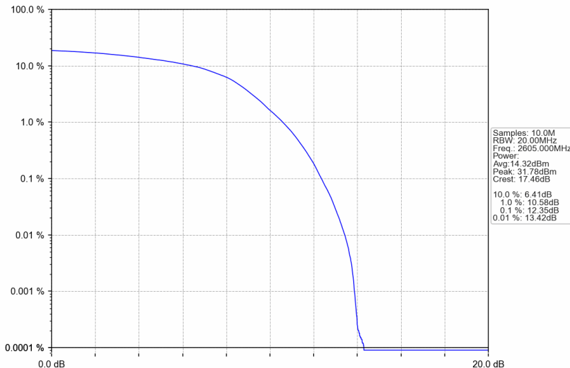
n38_30kHz_SISO_NTNV_30MHz_DFT-s-OFDM 64 QAM_2605MHz_Outer_Full
