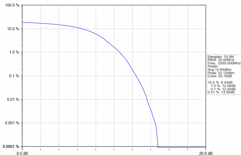
n38_30kHz_SISO_NTNV_25MHz_DFT-s-OFDM 256 QAM_2595MHz_Outer_Full
