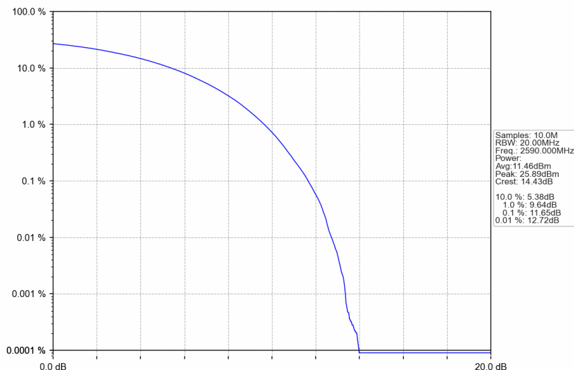
n38_30kHz_SISO_NTNV_40MHz_CP-OFDM 256 QAM_2590MHz_Outer_Full
