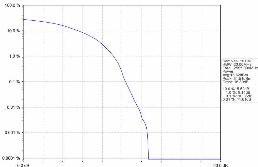
n38_30kHz_SISO_NTNV_40MHz_DFT-s-OFDM 64 QAM_2595MHz_Outer_Full
