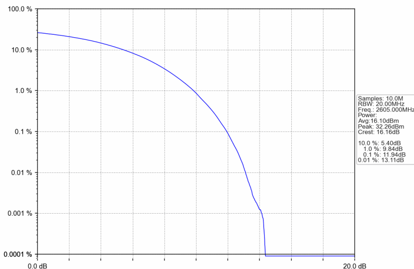
n38_30kHz_SISO_NTNV_30MHz_CP-OFDM QPSK_2605MHz_Outer_Full
