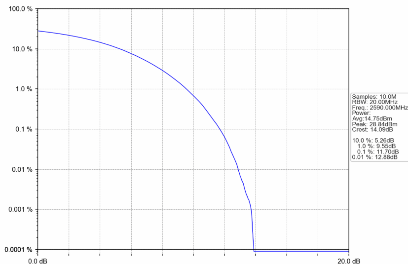
n38_30kHz_SISO_NTNV_40MHz_CP-OFDM 64 QAM_2590MHz_Outer_Full
