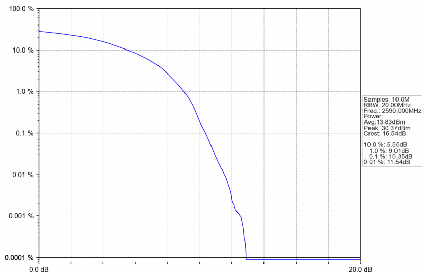
n38_30kHz_SISO_NTNV_40MHz_DFT-s-OFDM 256 QAM_2590MHz_Outer_Full
