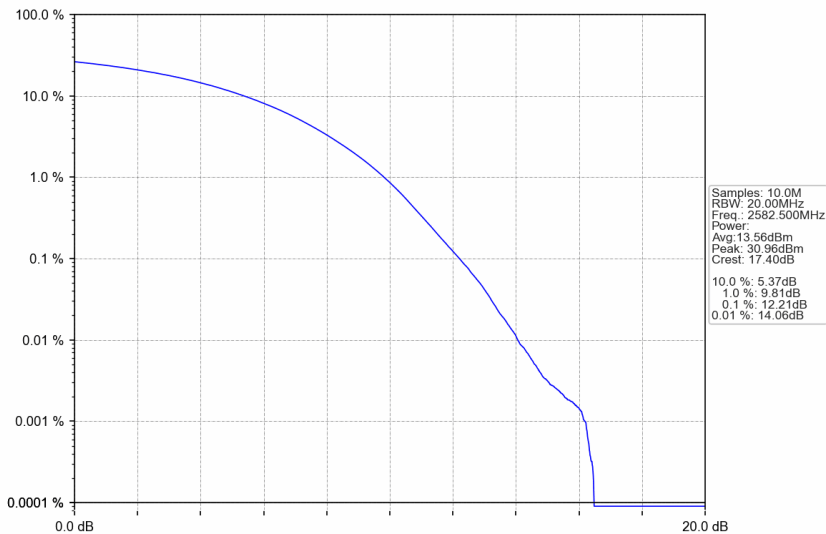
n38_30kHz_SISO_NTNV_25MHz_CP-OFDM 256 QAM_2582.5MHz_Outer_Full
