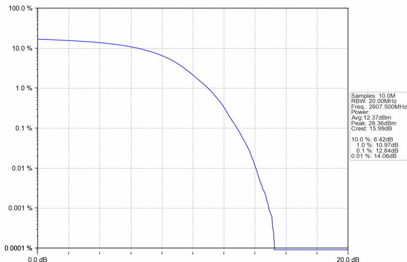
n38_30kHz_SISO_NTNV_25MHz_DFT-s-OFDM 256 QAM_2607.5MHz_Outer_Full
