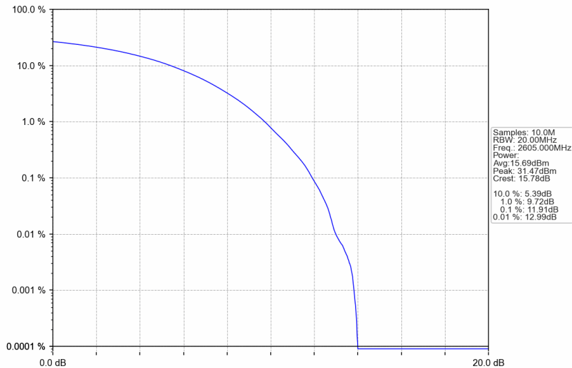
n38_30kHz_SISO_NTNV_30MHz_CP-OFDM 64 QAM_2605MHz_Outer_Full
