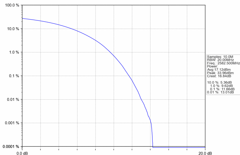
n38_30kHz_SISO_NTNV_25MHz_CP-OFDM QPSK_2582.5MHz_Outer_Full
