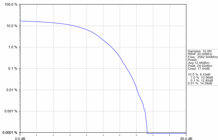
n38_30kHz_SISO_NTNV_25MHz_DFT-s-OFDM 256 QAM_2582.5MHz_Outer_Full
