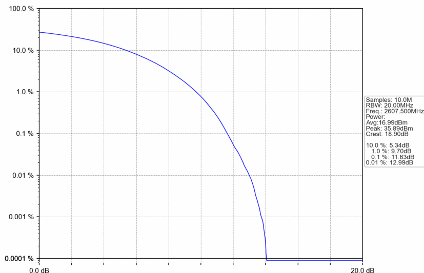
n38_30kHz_SISO_NTNV_25MHz_CP-OFDM 16 QAM_2607.5MHz_Outer_Full
