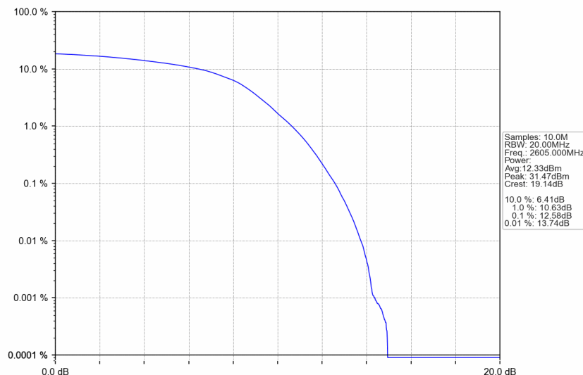
n38_30kHz_SISO_NTNV_30MHz_DFT-s-OFDM 256 QAM_2605MHz_Outer_Full
