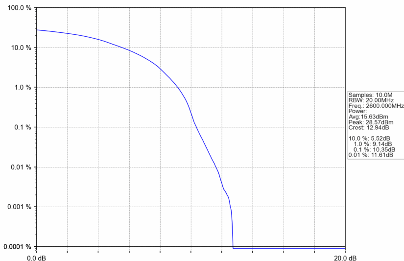
n38_30kHz_SISO_NTNV_40MHz_DFT-s-OFDM 64 QAM_2600MHz_Outer_Full
