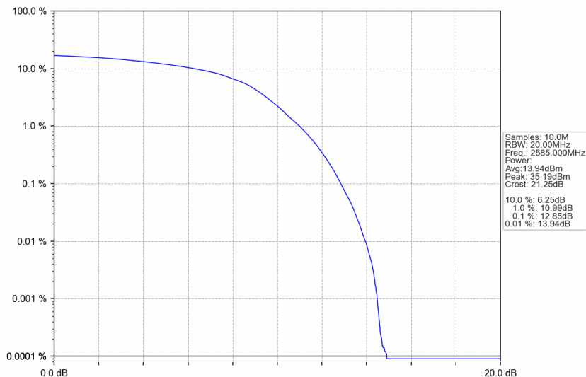
n38_30kHz_SISO_NTNV_30MHz_DFT-s-OFDM 64 QAM_2585MHz_Outer_Full
