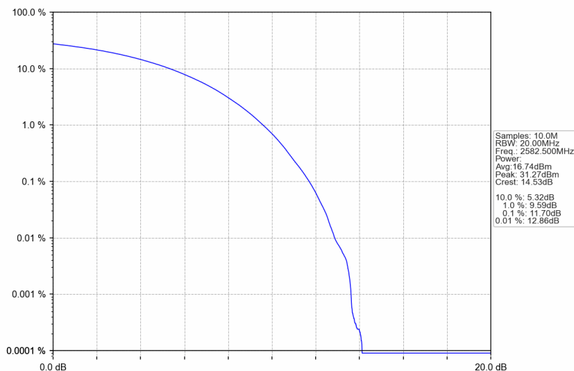
n38_30kHz_SISO_NTNV_25MHz_CP-OFDM 64 QAM_2582.5MHz_Outer_Full
