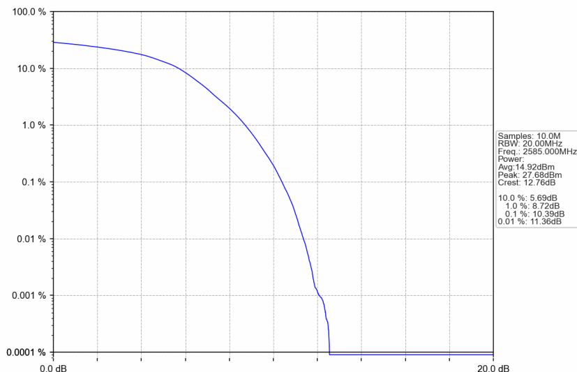
n38_30kHz_SISO_NTNV_30MHz_DFT-s-OFDM 256 QAM_2585MHz_Outer_Full
