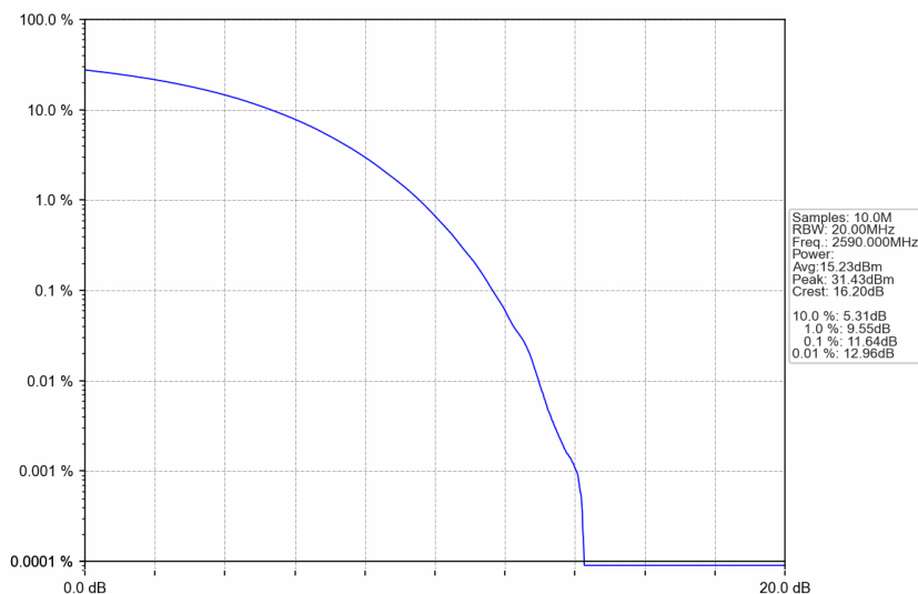
n38_30kHz_SISO_NTNV_40MHz_CP-OFDM QPSK_2590MHz_Outer_Full
