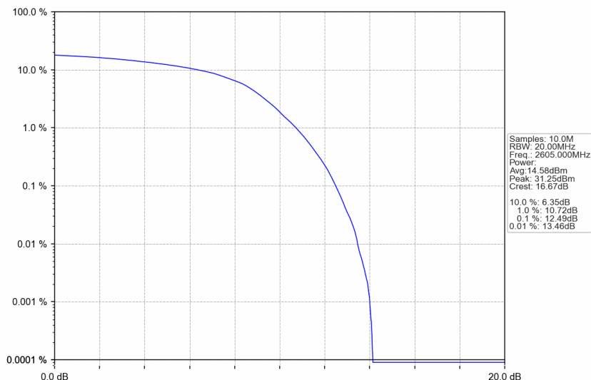
n38_30kHz_SISO_NTNV_30MHz_DFT-s-OFDM 16 QAM_2605MHz_Outer_Full
