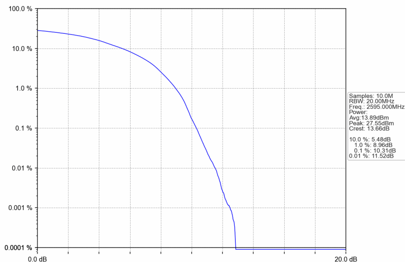
n38_30kHz_SISO_NTNV_40MHz_DFT-s-OFDM 256 QAM_2595MHz_Outer_Full
