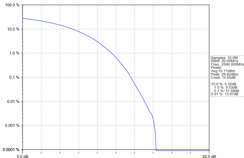
n38_30kHz_SISO_NTNV_40MHz_CP-OFDM 16 QAM_2590MHz_Outer_Full
