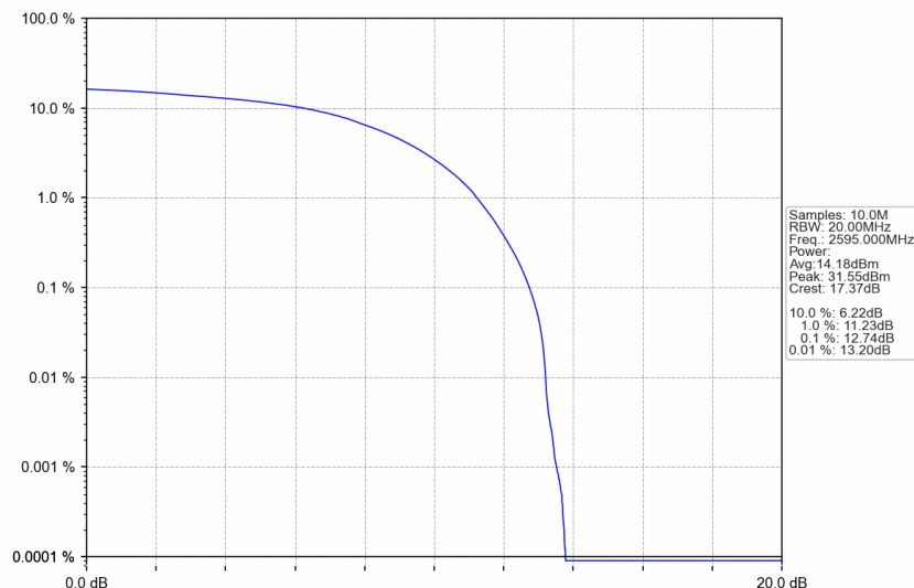
n38_30kHz_SISO_NTNV_40MHz_DFT-s-OFDM QPSK_2595MHz_Outer_Full
