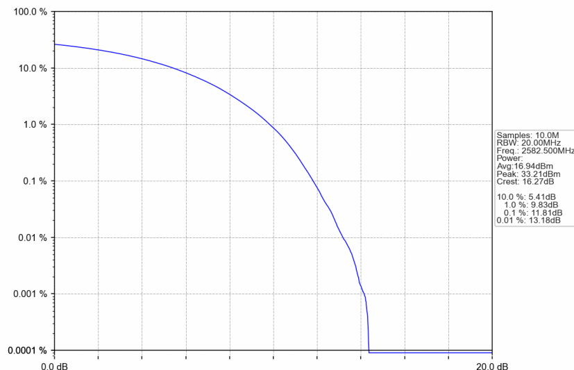
n38_30kHz_SISO_NTNV_25MHz_CP-OFDM 16 QAM_2582.5MHz_Outer_Full
