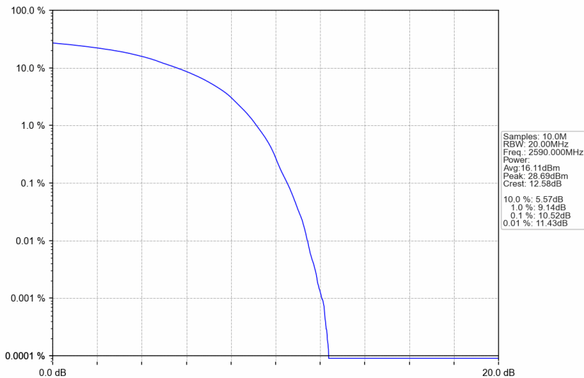
n38_30kHz_SISO_NTNV_40MHz_DFT-s-OFDM 16 QAM_2590MHz_Outer_Full
