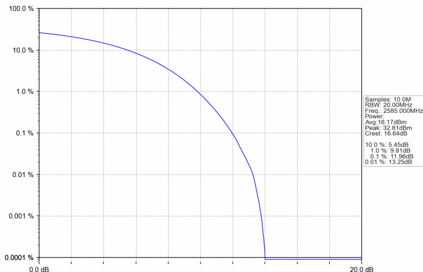
n38_30kHz_SISO_NTNV_30MHz_CP-OFDM 16 QAM_2585MHz_Outer_Full
