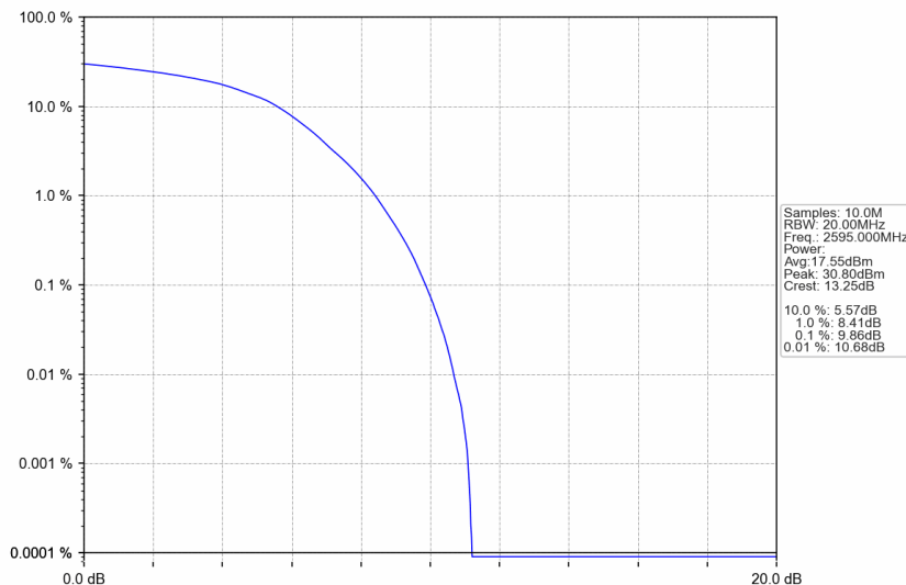
n38_30kHz_SISO_NTNV_30MHz_DFT-s-OFDM 16 QAM_2595MHz_Outer_Full
