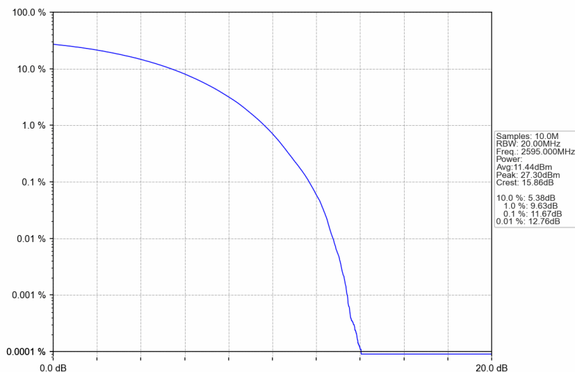
n38_30kHz_SISO_NTNV_40MHz_CP-OFDM 256 QAM_2595MHz_Outer_Full
