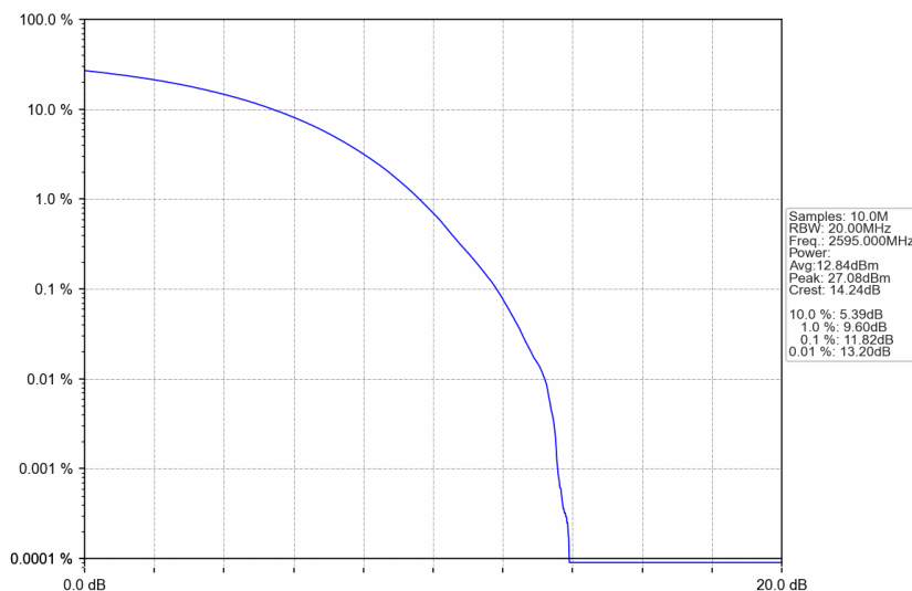
n38_30kHz_SISO_NTNV_30MHz_CP-OFDM 256 QAM_2595MHz_Outer_Full
