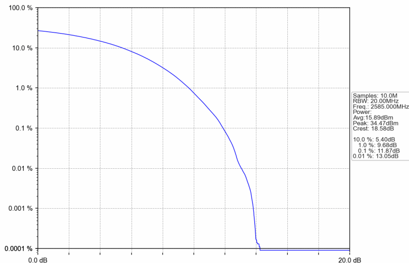
n38_30kHz_SISO_NTNV_30MHz_CP-OFDM 64 QAM_2585MHz_Outer_Full
