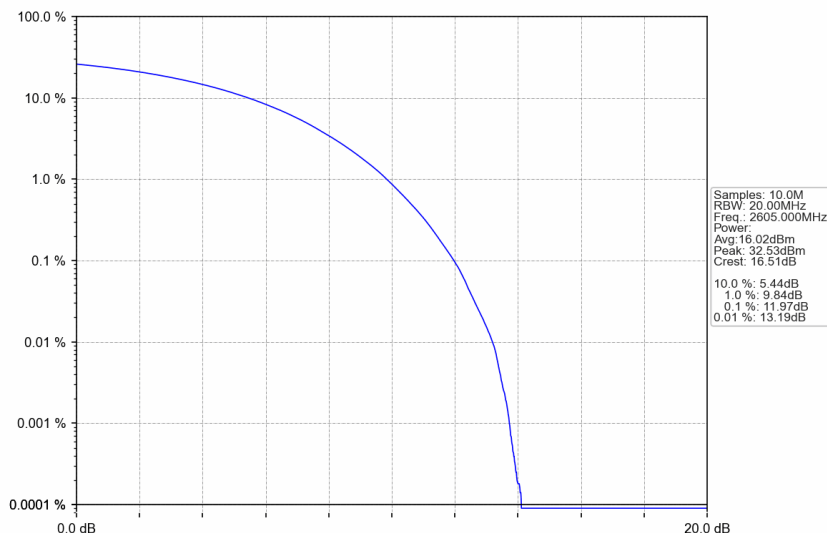
n38_30kHz_SISO_NTNV_30MHz_CP-OFDM 16 QAM_2605MHz_Outer_Full
