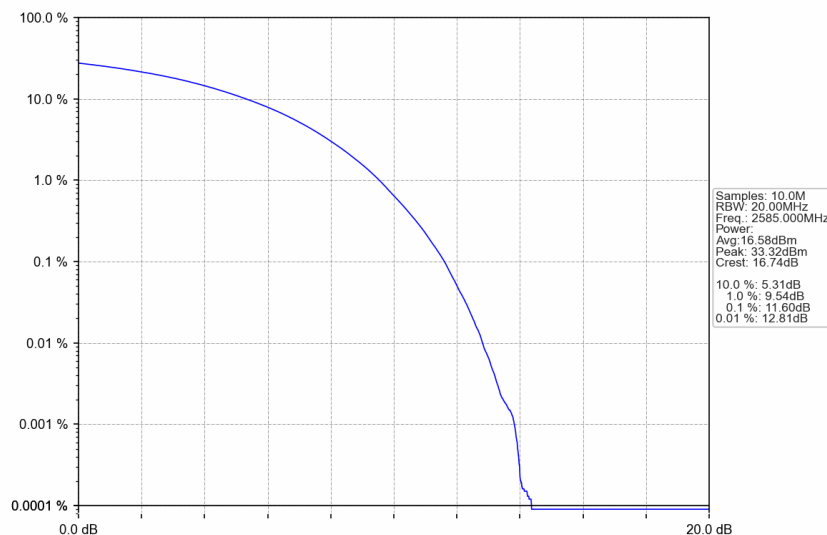
n38_30kHz_SISO_NTNV_30MHz_CP-OFDM QPSK_2585MHz_Outer_Full
