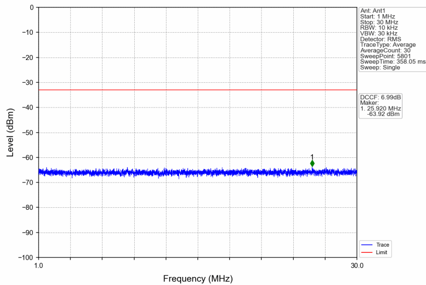
n38_15kHz_SISO_NTNV_5MHz_DFT-s-OFDM QPSK_2572.5MHz_Edge_1RB_Left
