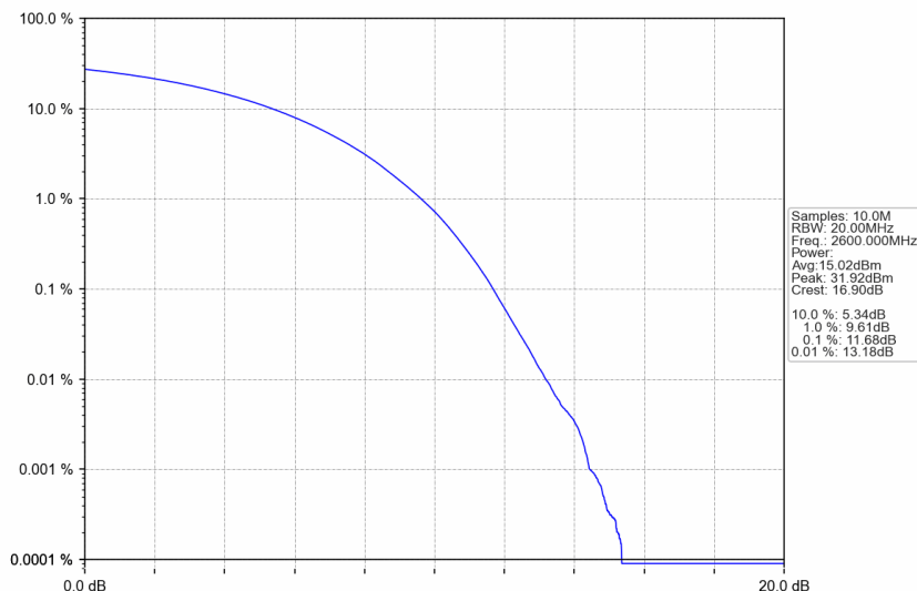
n38_30kHz_SISO_NTNV_40MHz_CP-OFDM 16 QAM_2600MHz_Outer_Full
