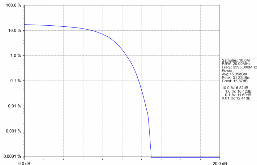
n38_30kHz_SISO_NTNV_30MHz_DFT-s-OFDM QPSK_2595MHz_Outer_Full
