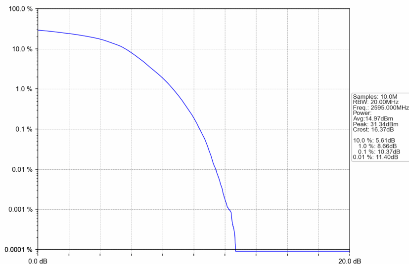
n38_30kHz_SISO_NTNV_30MHz_DFT-s-OFDM 256 QAM_2595MHz_Outer_Full
