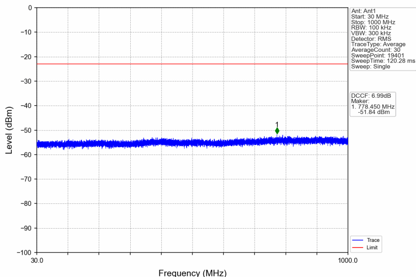
n38_15kHz_SISO_NTNV_5MHz_DFT-s-OFDM QPSK_2595MHz_Edge_1RB_Left
