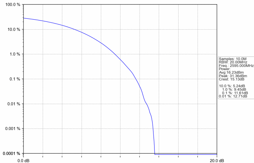
n38_30kHz_SISO_NTNV_30MHz_CP-OFDM 64 QAM_2595MHz_Outer_Full
