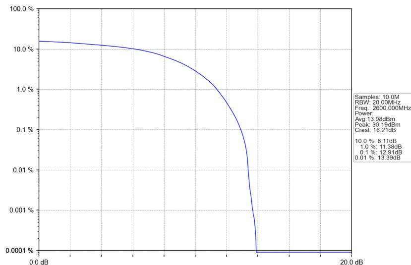
n38_30kHz_SISO_NTNV_40MHz_DFT-s-OFDM QPSK_2600MHz_Outer_Full
