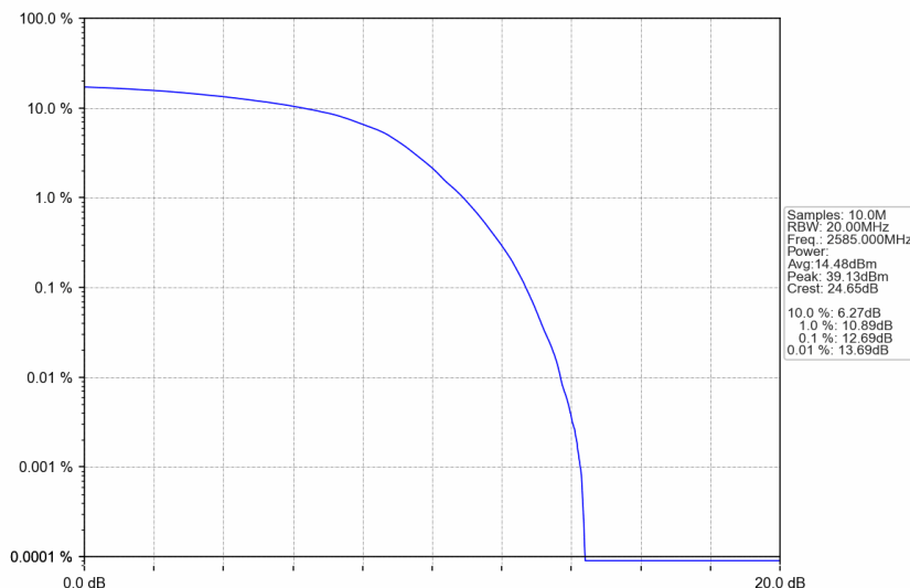
n38_30kHz_SISO_NTNV_30MHz_DFT-s-OFDM 16 QAM_2585MHz_Outer_Full
