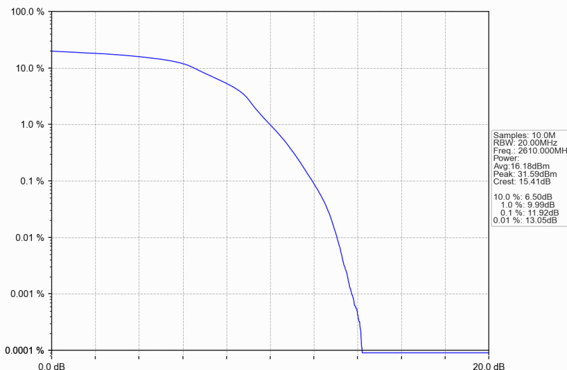
n38_30kHz_SISO_NTNV_20MHz_DFT-s-OFDM 16 QAM_2610MHz_Outer_Full
