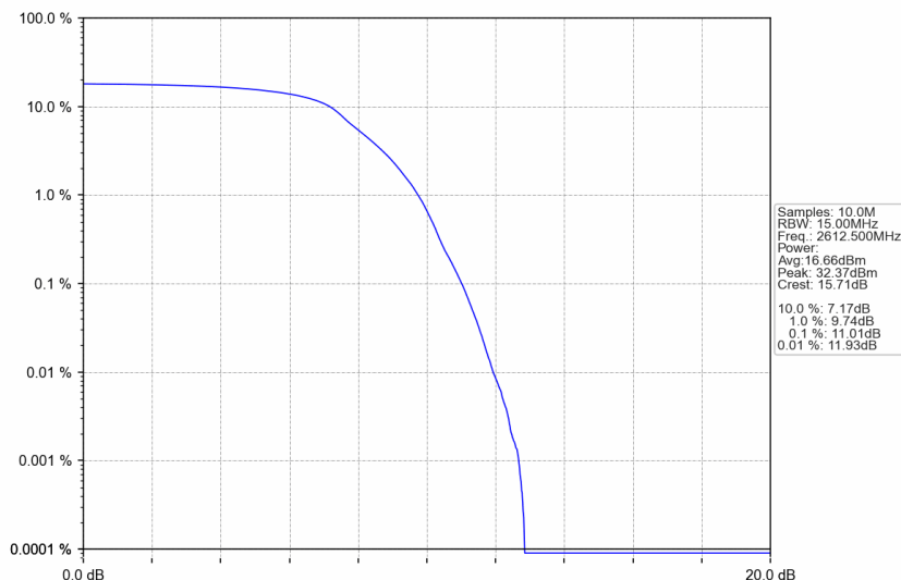
n38_30kHz_SISO_NTNV_15MHz_DFT-s-OFDM PI/2 BPSK_2612.5MHz_Outer_Full
