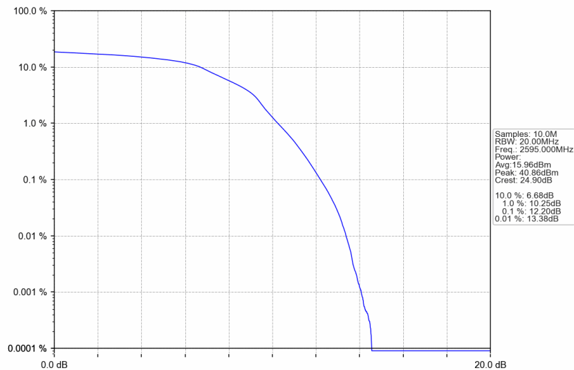
n38_30kHz_SISO_NTNV_20MHz_DFT-s-OFDM 16 QAM_2595MHz_Outer_Full
