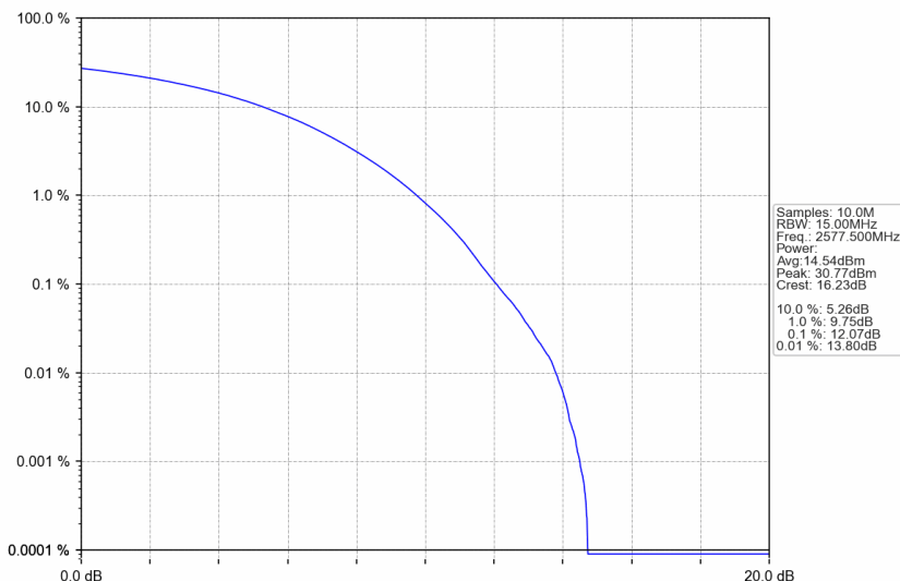
n38_30kHz_SISO_NTNV_15MHz_CP-OFDM 256 QAM_2577.5MHz_Outer_Full
