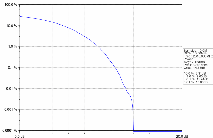
n38_30kHz_SISO_NTNV_10MHz_CP-OFDM 64 QAM_2615MHz_Outer_Full
