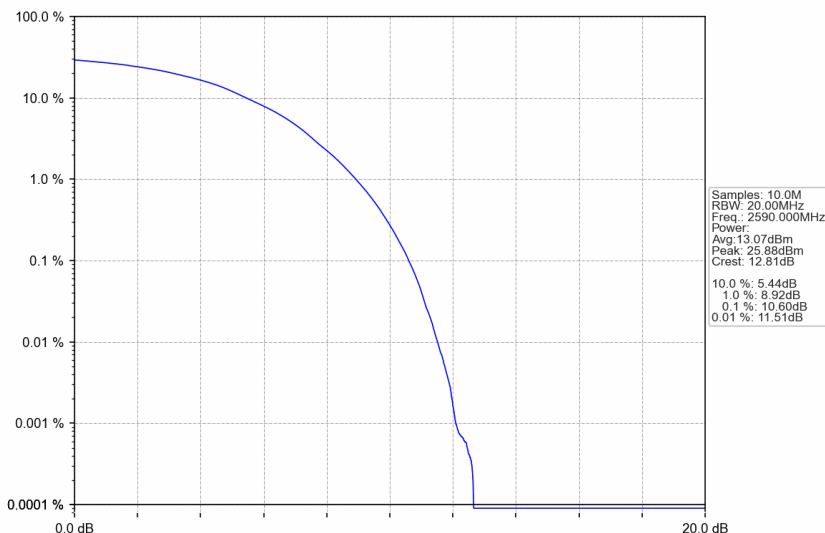
n38_15kHz_SISO_NTNV_40MHz_DFT-s-OFDM 256 QAM_2590MHz_Outer_Full
