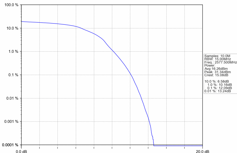
n38_30kHz_SISO_NTNV_15MHz_DFT-s-OFDM 16 QAM_2577.5MHz_Outer_Full
