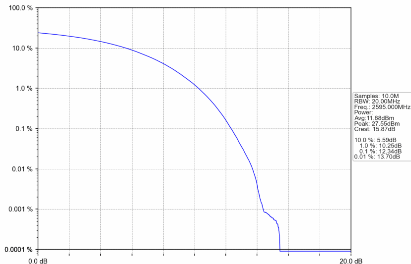
n38_15kHz_SISO_NTNV_30MHz_CP-OFDM 256 QAM_2595MHz_Outer_Full
