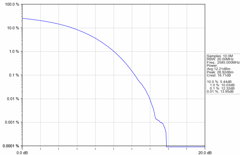
n38_15kHz_SISO_NTNV_30MHz_CP-OFDM 256 QAM_2585MHz_Outer_Full
