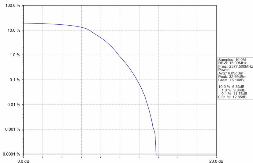
n38_30kHz_SISO_NTNV_15MHz_DFT-s-OFDM QPSK_2577.5MHz_Outer_Full
