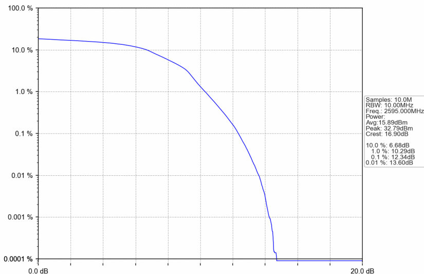
n38_30kHz_SISO_NTNV_10MHz_DFT-s-OFDM 16 QAM_2595MHz_Outer_Full
