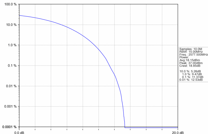
n38_30kHz_SISO_NTNV_15MHz_CP-OFDM 16 QAM_2577.5MHz_Outer_Full
