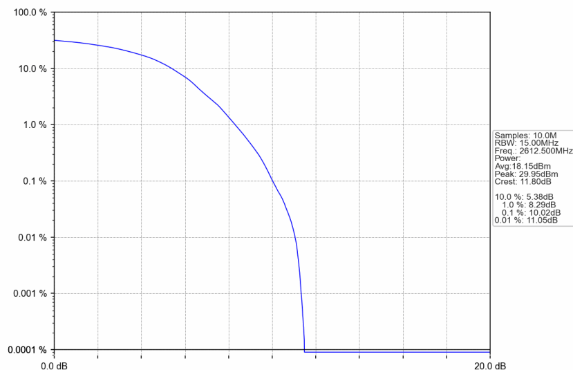
n38_30kHz_SISO_NTNV_15MHz_DFT-s-OFDM 64 QAM_2612.5MHz_Outer_Full
