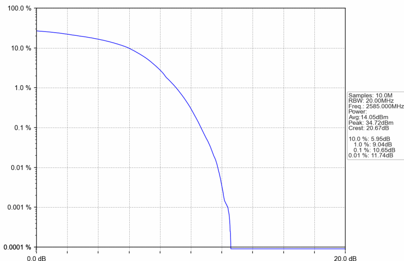
n38_15kHz_SISO_NTNV_30MHz_DFT-s-OFDM 256 QAM_2585MHz_Outer_Full
