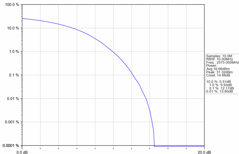
n38_15kHz_SISO_NTNV_10MHz_CP-OFDM 64 QAM_2575MHz_Outer_Full
