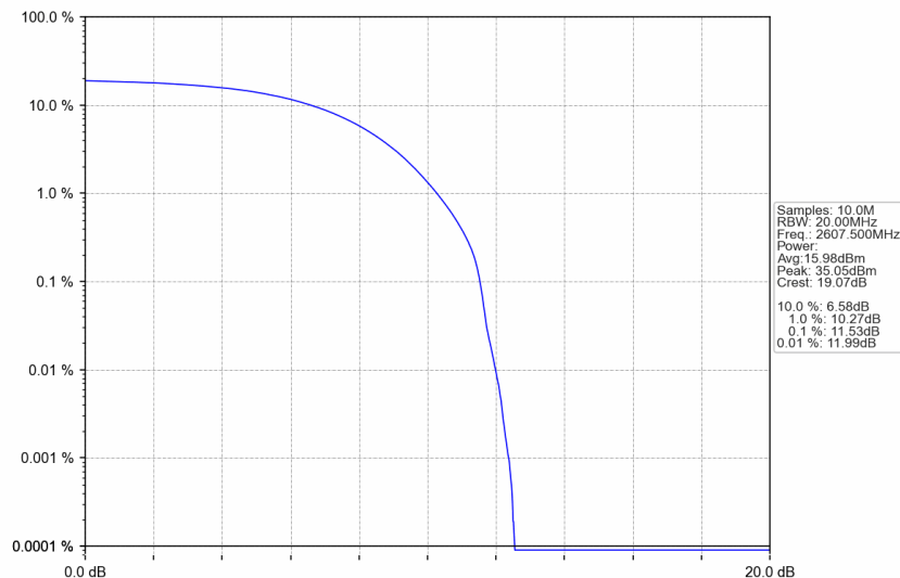
n38_15kHz_SISO_NTNV_25MHz_DFT-s-OFDM QPSK_2607.5MHz_Outer_Full
