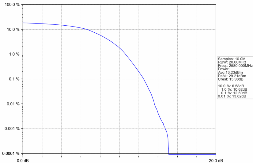
n38_15kHz_SISO_NTNV_20MHz_DFT-s-OFDM 256 QAM_2580MHz_Outer_Full
