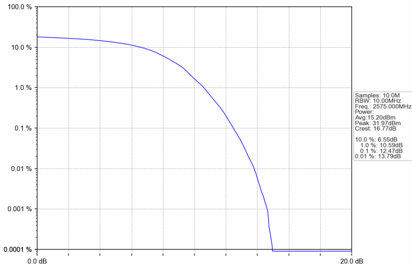
n38_15kHz_SISO_NTNV_10MHz_DFT-s-OFDM 64 QAM_2575MHz_Outer_Full
