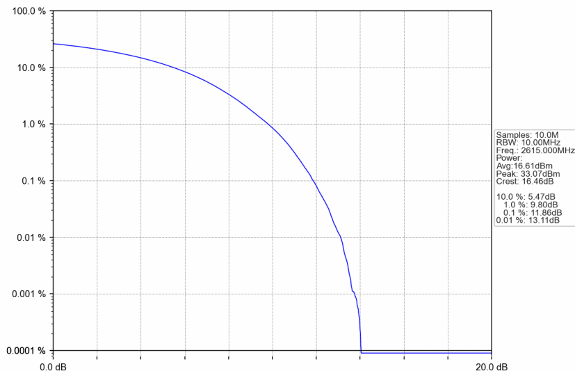
n38_15kHz_SISO_NTNV_10MHz_CP-OFDM 64 QAM_2615MHz_Outer_Full
