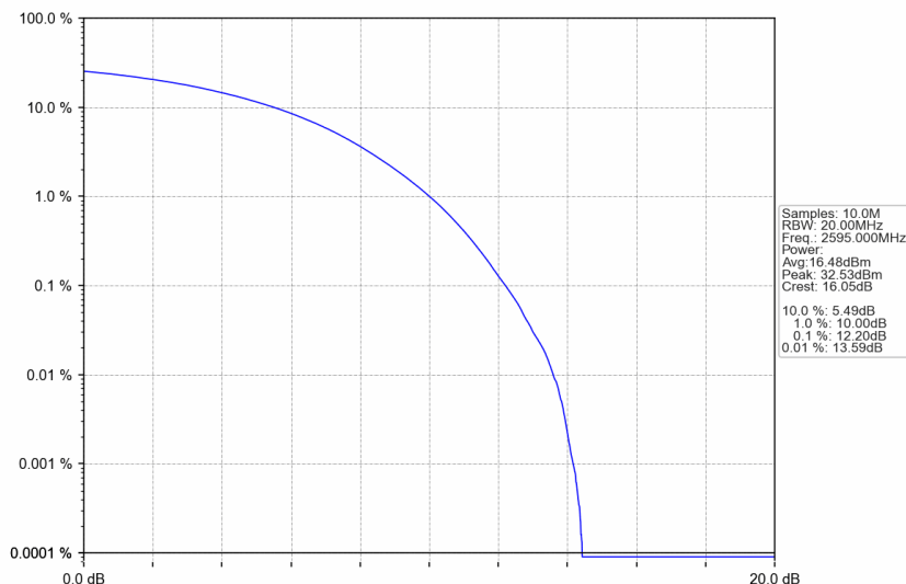
n38_15kHz_SISO_NTNV_20MHz_CP-OFDM 64 QAM_2595MHz_Outer_Full
