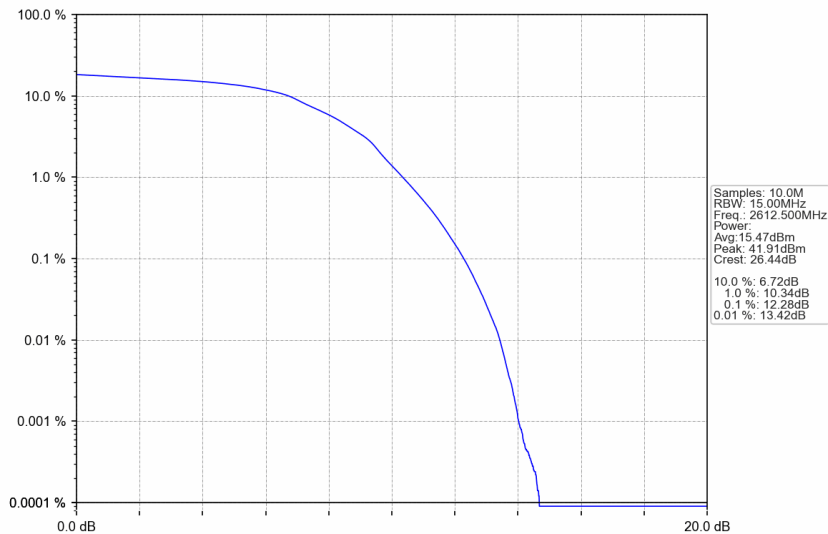
n38_15kHz_SISO_NTNV_15MHz_DFT-s-OFDM 16 QAM_2612.5MHz_Outer_Full
