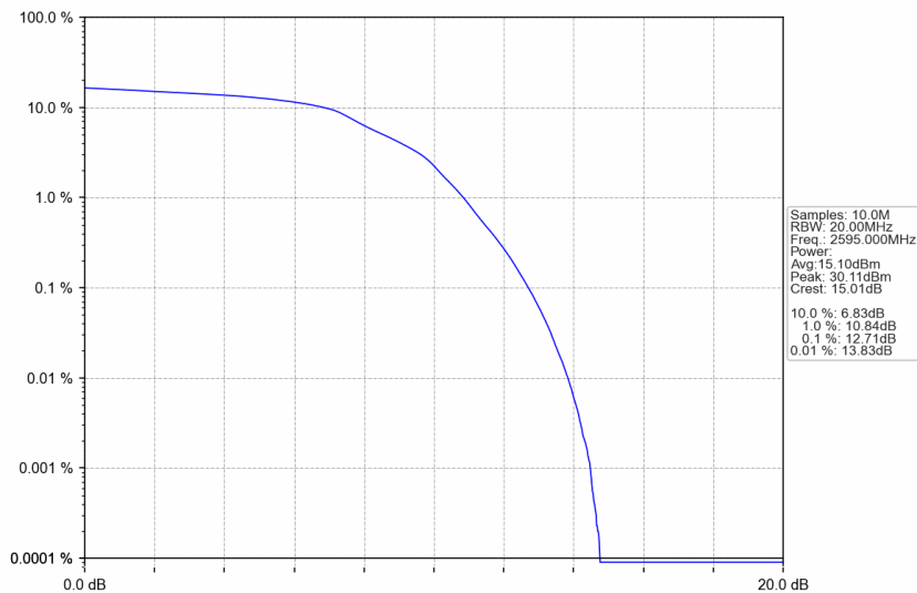
n38_15kHz_SISO_NTNV_20MHz_DFT-s-OFDM 16 QAM_2595MHz_Outer_Full
