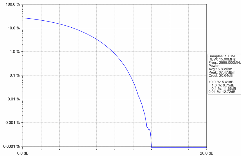
n38_15kHz_SISO_NTNV_15MHz_CP-OFDM 64 QAM_2595MHz_Outer_Full
