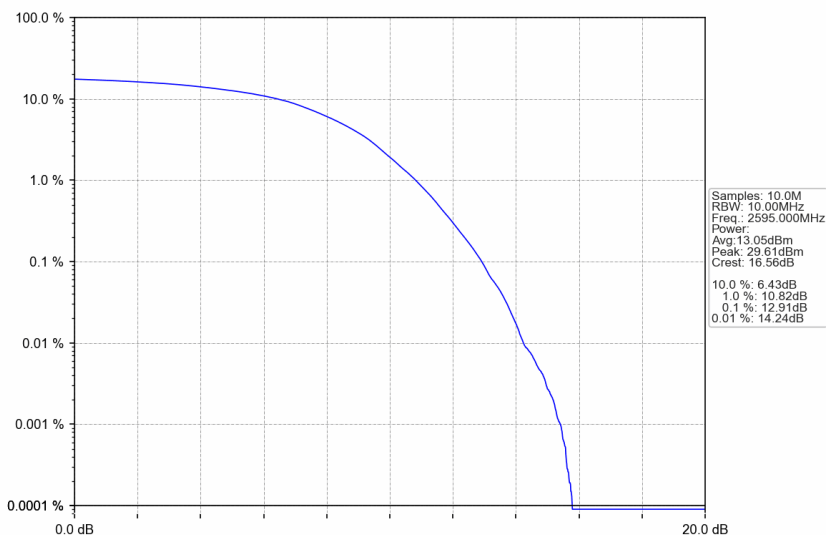
n38_15kHz_SISO_NTNV_10MHz_DFT-s-OFDM 256 QAM_2595MHz_Outer_Full
