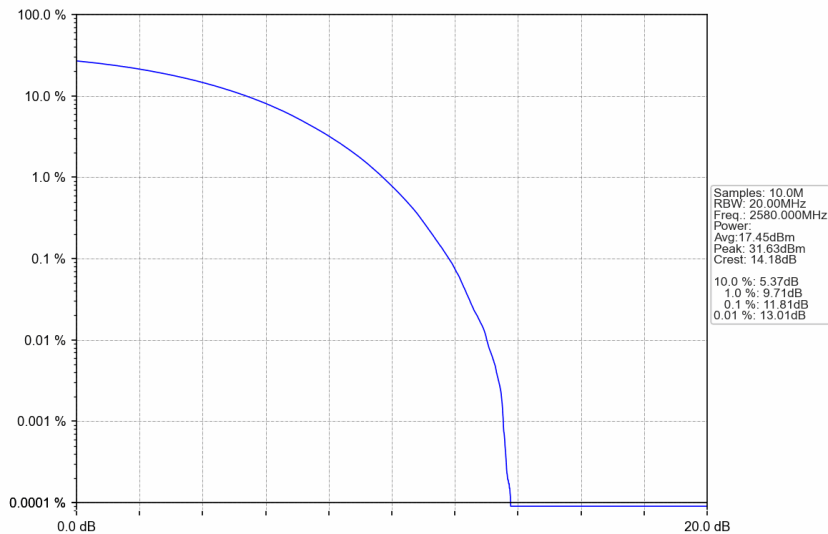
n38_15kHz_SISO_NTNV_20MHz_CP-OFDM 16 QAM_2580MHz_Outer_Full
