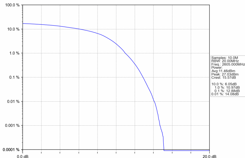
n38_15kHz_SISO_NTNV_30MHz_DFT-s-OFDM 256 QAM_2605MHz_Outer_Full
