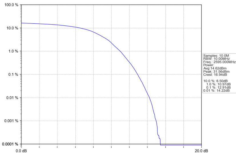
n38_15kHz_SISO_NTNV_10MHz_DFT-s-OFDM 64 QAM_2595MHz_Outer_Full
