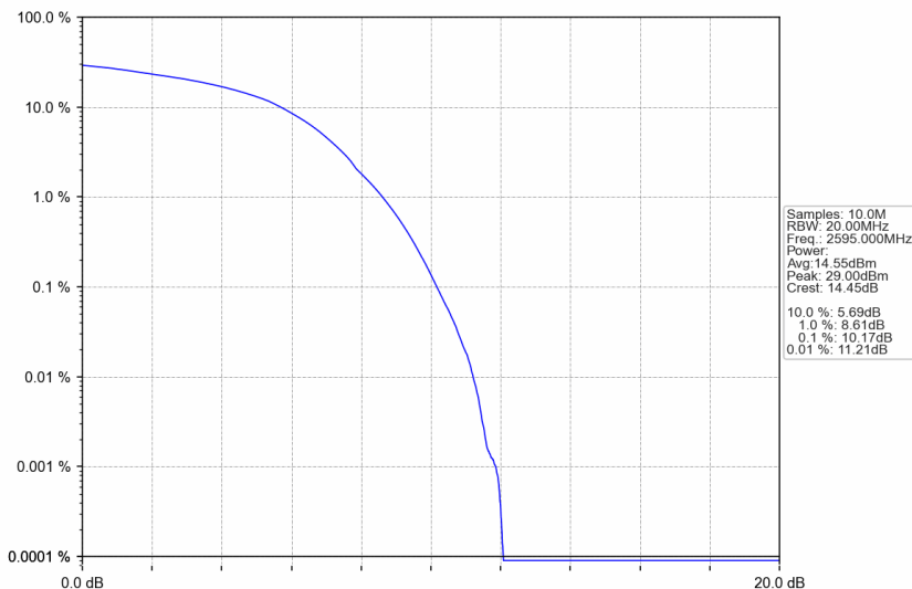
n38_15kHz_SISO_NTNV_30MHz_DFT-s-OFDM 256 QAM_2595MHz_Outer_Full
