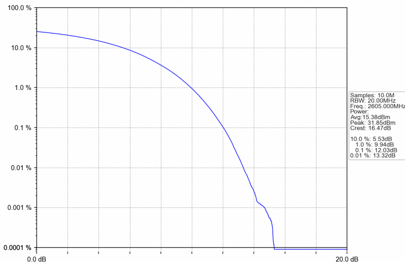
n38_15kHz_SISO_NTNV_30MHz_CP-OFDM QPSK_2605MHz_Outer_Full
