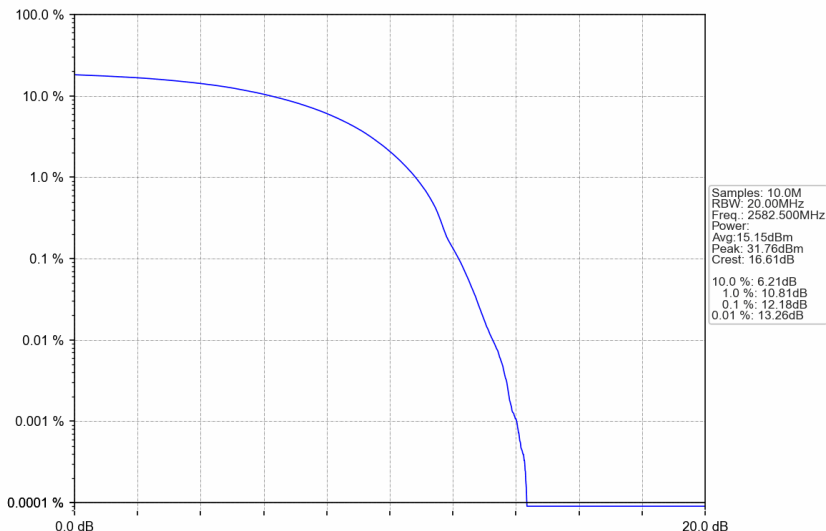
n38_15kHz_SISO_NTNV_25MHz_DFT-s-OFDM 16 QAM_2582.5MHz_Outer_Full
