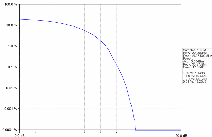
n38_15kHz_SISO_NTNV_25MHz_DFT-s-OFDM 256 QAM_2607.5MHz_Outer_Full
