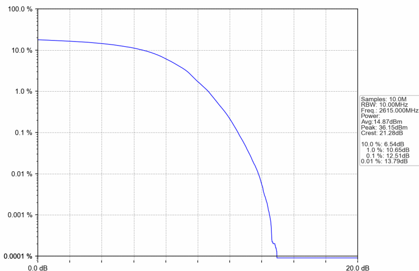
n38_15kHz_SISO_NTNV_10MHz_DFT-s-OFDM 64 QAM_2615MHz_Outer_Full
