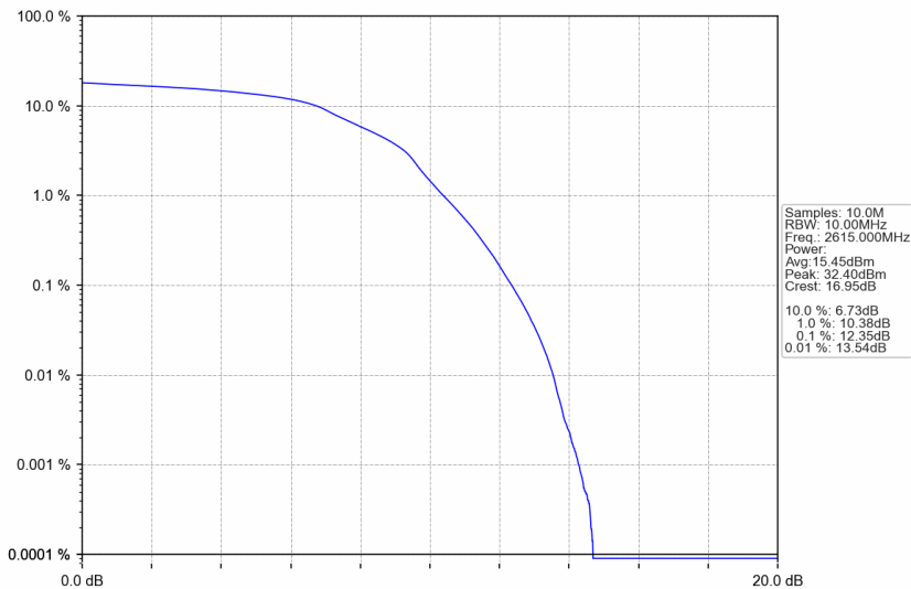
n38_15kHz_SISO_NTNV_10MHz_DFT-s-OFDM 16 QAM_2615MHz_Outer_Full
