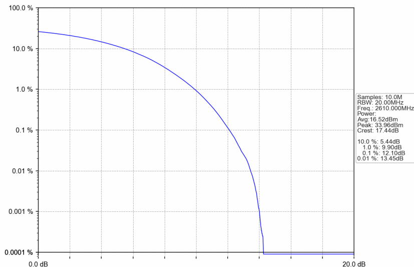
n38_15kHz_SISO_NTNV_20MHz_CP-OFDM 64 QAM_2610MHz_Outer_Full
