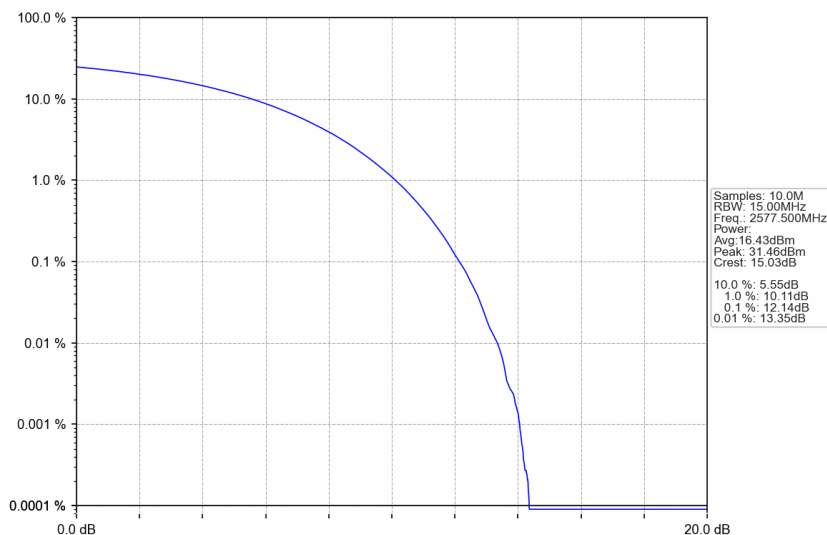
n38_15kHz_SISO_NTNV_15MHz_CP-OFDM 64 QAM_2577.5MHz_Outer_Full
