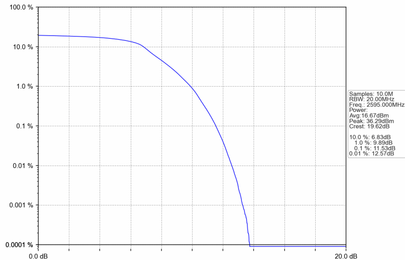
n38_15kHz_SISO_NTNV_20MHz_DFT-s-OFDM QPSK_2595MHz_Outer_Full
