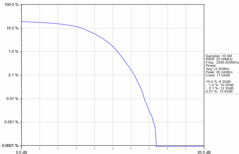
n38_15kHz_SISO_NTNV_20MHz_DFT-s-OFDM 256 QAM_2595MHz_Outer_Full
