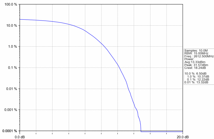
n38_15kHz_SISO_NTNV_15MHz_DFT-s-OFDM 256 QAM_2612.5MHz_Outer_Full
