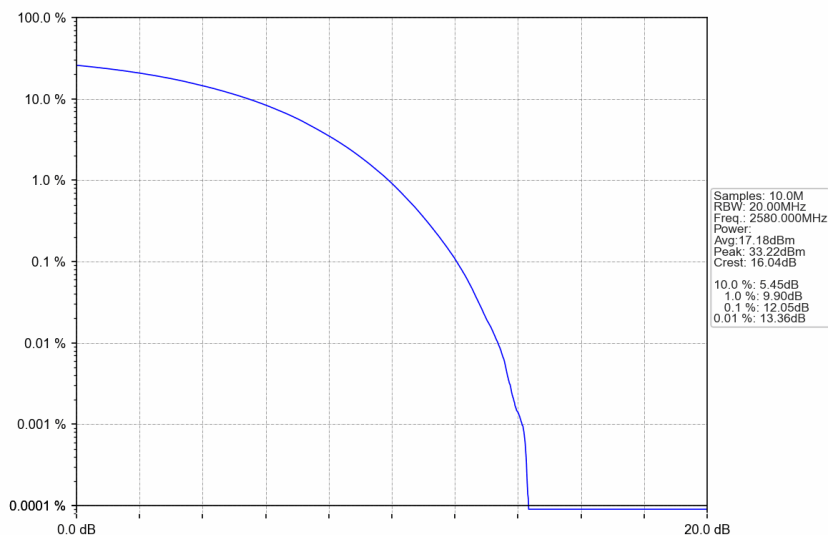
n38_15kHz_SISO_NTNV_20MHz_CP-OFDM QPSK_2580MHz_Outer_Full
