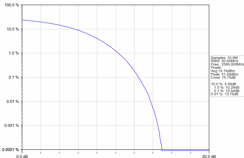
n38_15kHz_SISO_NTNV_25MHz_CP-OFDM QPSK_2595MHz_Outer_Full
