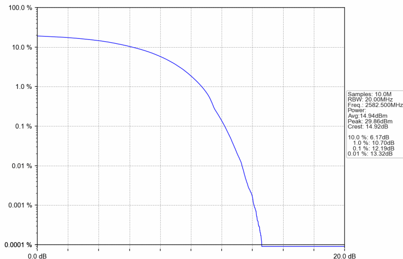
n38_15kHz_SISO_NTNV_25MHz_DFT-s-OFDM 64 QAM_2582.5MHz_Outer_Full
