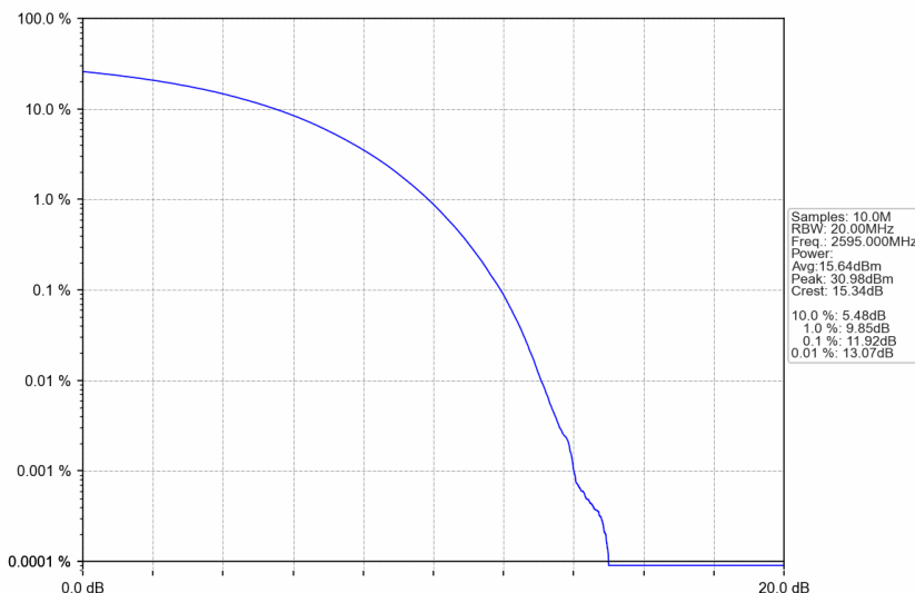
n38_15kHz_SISO_NTNV_30MHz_CP-OFDM QPSK_2595MHz_Outer_Full
