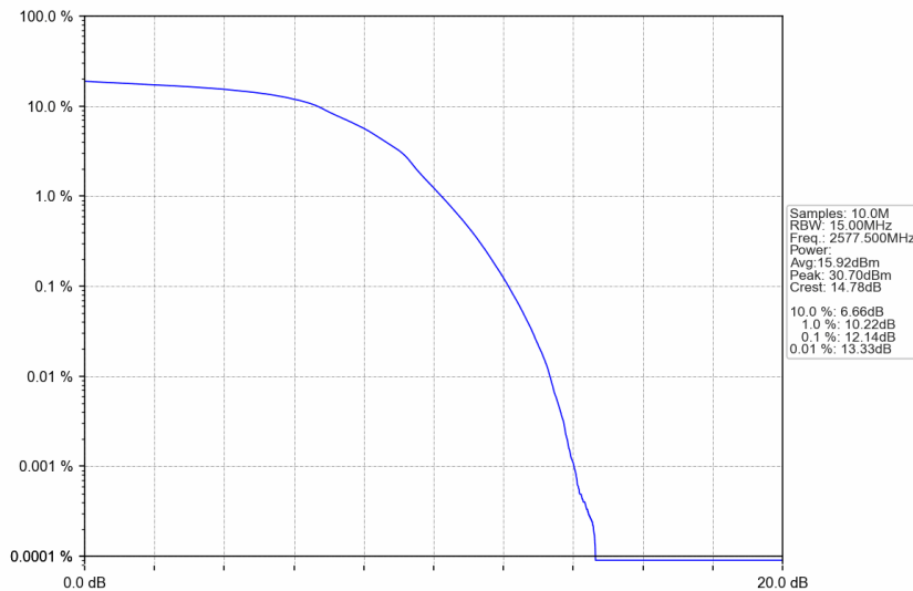
n38_15kHz_SISO_NTNV_15MHz_DFT-s-OFDM 16 QAM_2577.5MHz_Outer_Full
