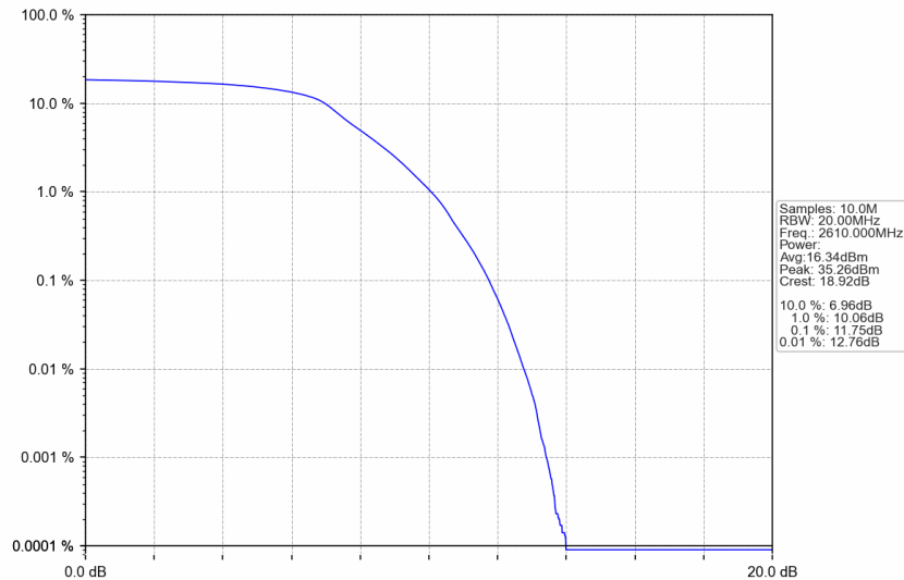
n38_15kHz_SISO_NTNV_20MHz_DFT-s-OFDM QPSK_2610MHz_Outer_Full
