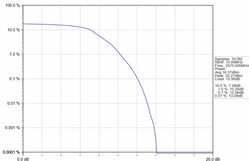
n38_15kHz_SISO_NTNV_10MHz_DFT-s-OFDM QPSK_2575MHz_Outer_Full
