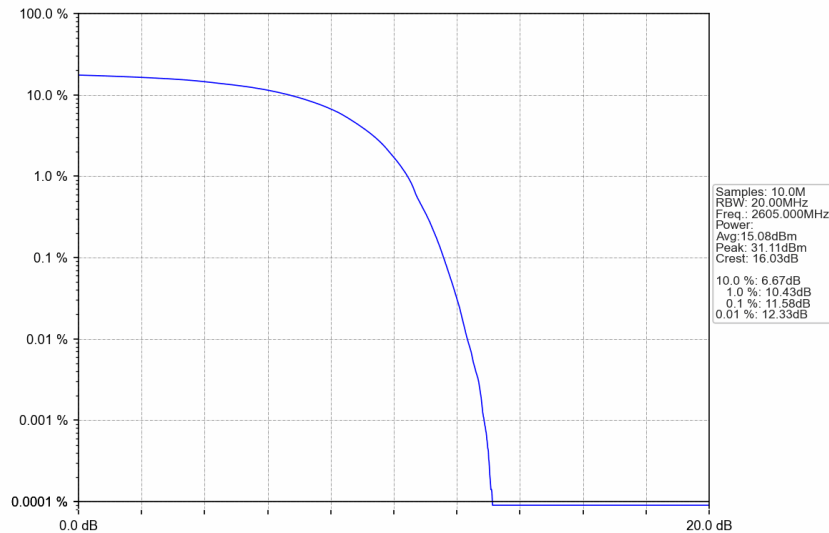
n38_15kHz_SISO_NTNV_30MHz_DFT-s-OFDM QPSK_2605MHz_Outer_Full
