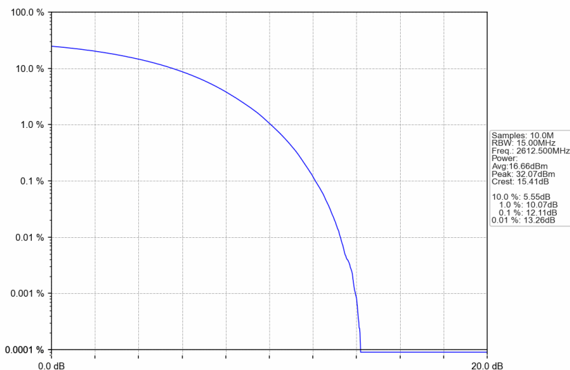
n38_15kHz_SISO_NTNV_15MHz_CP-OFDM QPSK_2612.5MHz_Outer_Full
