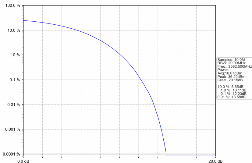
n38_15kHz_SISO_NTNV_25MHz_CP-OFDM QPSK_2582.5MHz_Outer_Full
