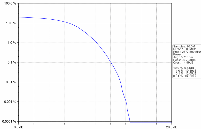
n38_15kHz_SISO_NTNV_15MHz_DFT-s-OFDM 64 QAM_2577.5MHz_Outer_Full
