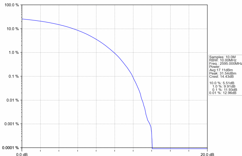
n38_15kHz_SISO_NTNV_10MHz_CP-OFDM QPSK_2595MHz_Outer_Full
