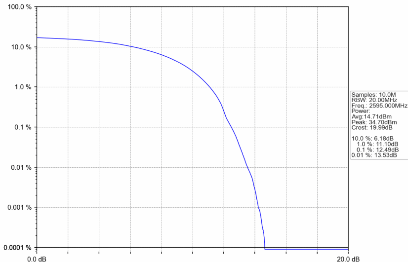
n38_15kHz_SISO_NTNV_25MHz_DFT-s-OFDM 16 QAM_2595MHz_Outer_Full
