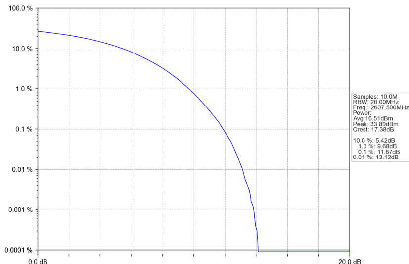
n38_15kHz_SISO_NTNV_25MHz_CP-OFDM 16 QAM_2607.5MHz_Outer_Full
