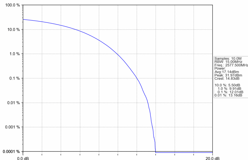
n38_15kHz_SISO_NTNV_15MHz_CP-OFDM 16 QAM_2577.5MHz_Outer_Full
