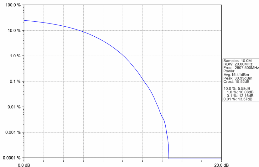
n38_15kHz_SISO_NTNV_25MHz_CP-OFDM 64 QAM_2607.5MHz_Outer_Full
