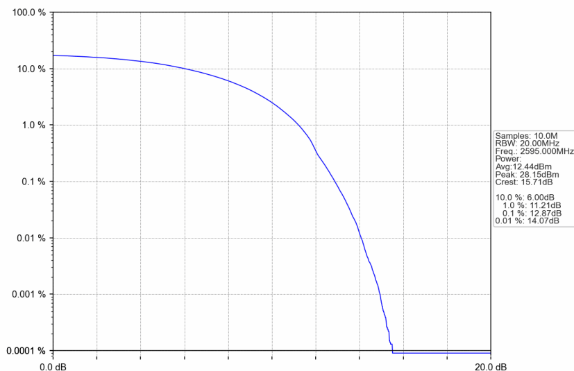
n38_15kHz_SISO_NTNV_25MHz_DFT-s-OFDM 256 QAM_2595MHz_Outer_Full
