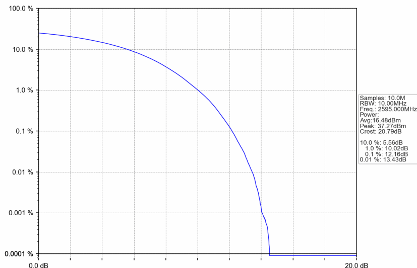
n38_15kHz_SISO_NTNV_10MHz_CP-OFDM 64 QAM_2595MHz_Outer_Full
