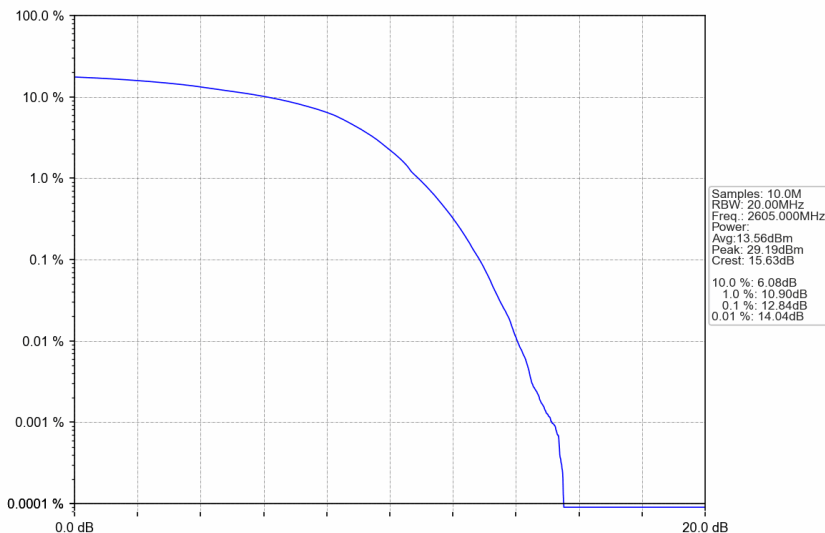
n38_15kHz_SISO_NTNV_30MHz_DFT-s-OFDM 64 QAM_2605MHz_Outer_Full
