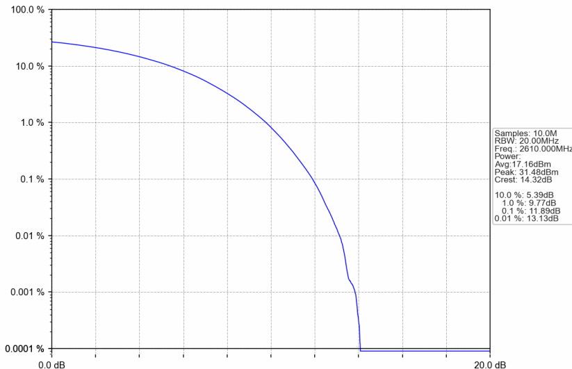
n38_15kHz_SISO_NTNV_20MHz_CP-OFDM QPSK_2610MHz_Outer_Full
