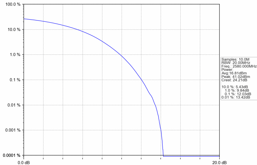
n38_15kHz_SISO_NTNV_20MHz_CP-OFDM 64 QAM_2580MHz_Outer_Full
