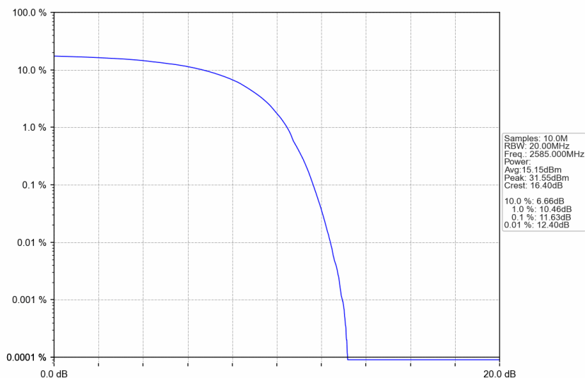
n38_15kHz_SISO_NTNV_30MHz_DFT-s-OFDM QPSK_2585MHz_Outer_Full
