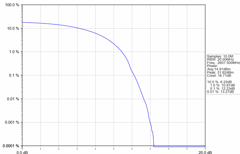
n38_15kHz_SISO_NTNV_25MHz_DFT-s-OFDM 16 QAM_2607.5MHz_Outer_Full
