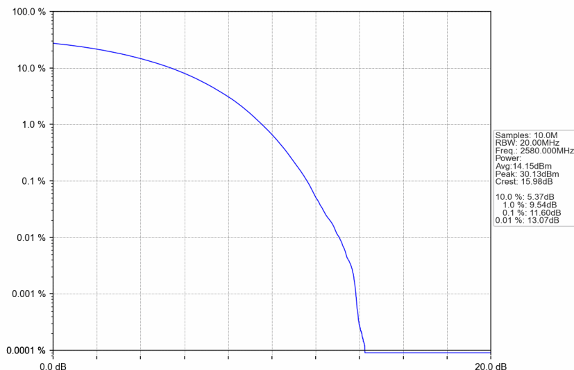
n38_15kHz_SISO_NTNV_20MHz_CP-OFDM 256 QAM_2580MHz_Outer_Full
