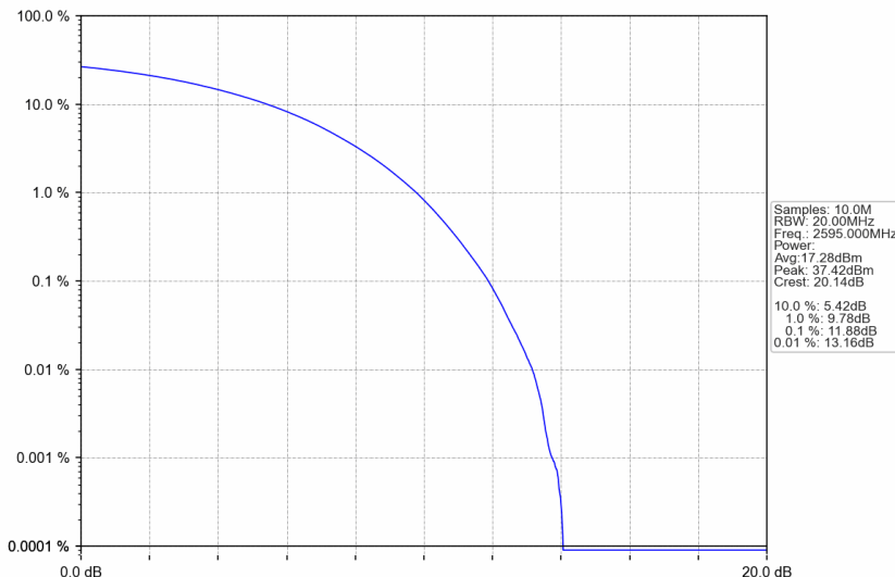
n38_15kHz_SISO_NTNV_20MHz_CP-OFDM QPSK_2595MHz_Outer_Full
