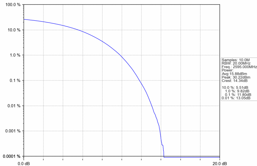
n38_15kHz_SISO_NTNV_25MHz_CP-OFDM 64 QAM_2595MHz_Outer_Full
