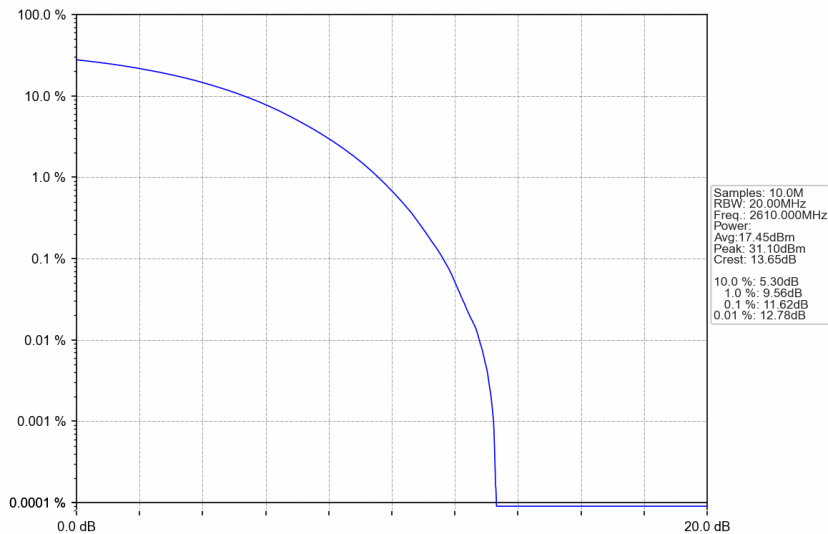
n38_15kHz_SISO_NTNV_20MHz_CP-OFDM 16 QAM_2610MHz_Outer_Full
