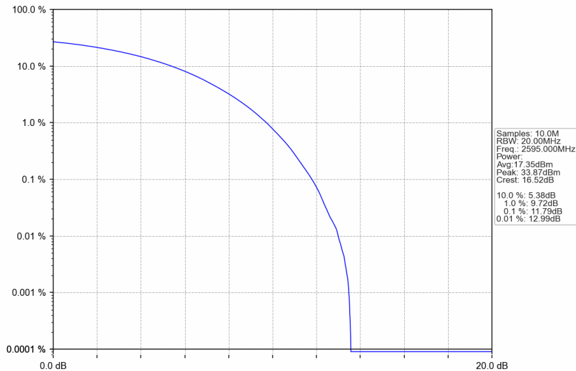
n38_15kHz_SISO_NTNV_20MHz_CP-OFDM 16 QAM_2595MHz_Outer_Full
