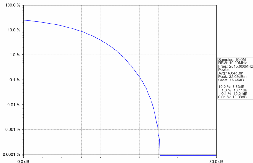
n38_15kHz_SISO_NTNV_10MHz_CP-OFDM 16 QAM_2615MHz_Outer_Full
