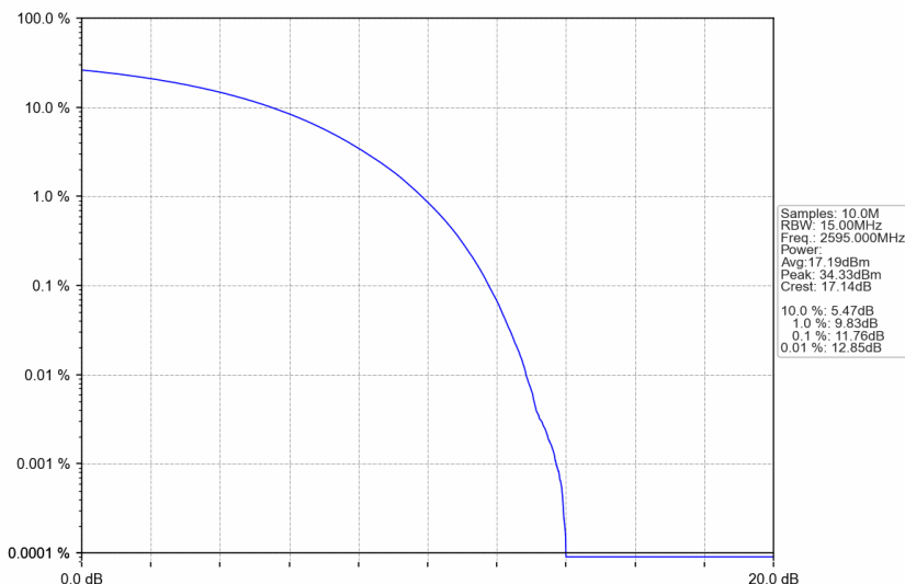
n38_15kHz_SISO_NTNV_15MHz_CP-OFDM QPSK_2595MHz_Outer_Full
