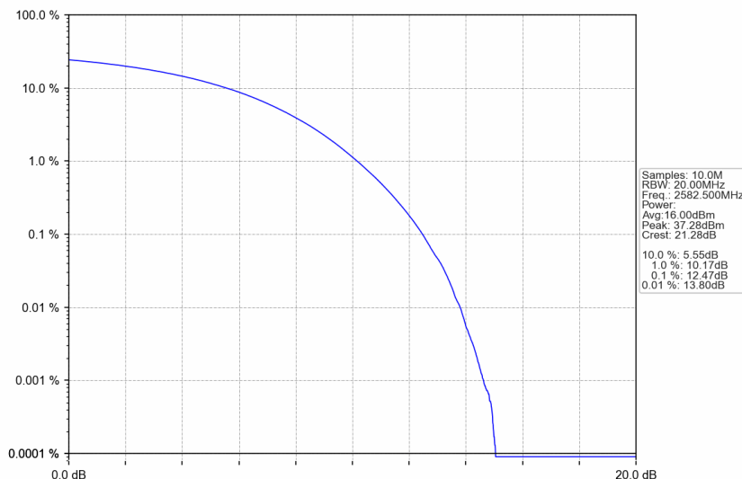
n38_15kHz_SISO_NTNV_25MHz_CP-OFDM 16 QAM_2582.5MHz_Outer_Full
