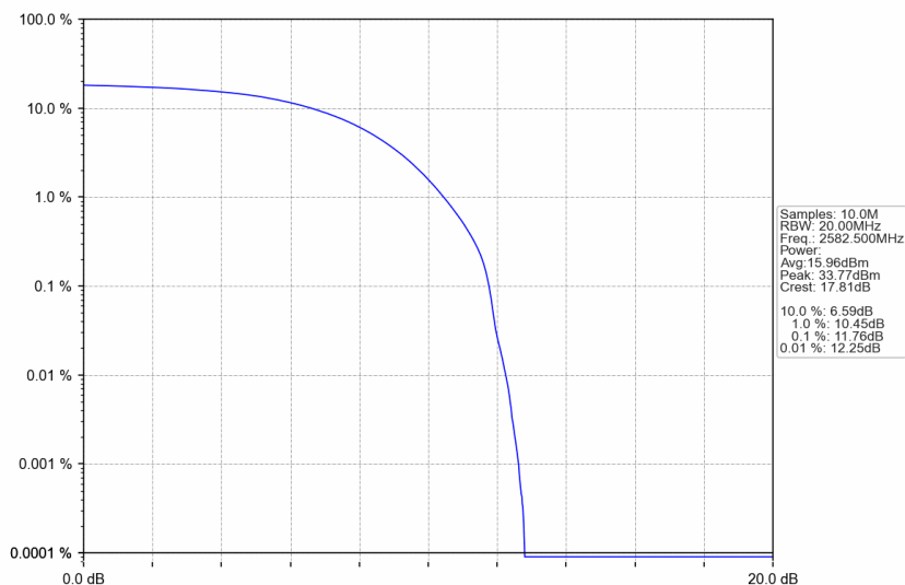
n38_15kHz_SISO_NTNV_25MHz_DFT-s-OFDM QPSK_2582.5MHz_Outer_Full
