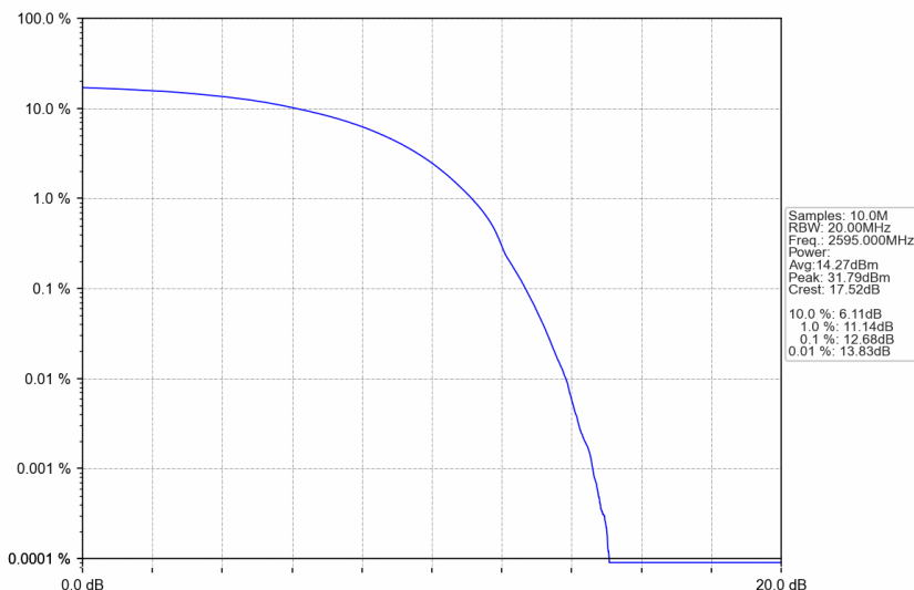
n38_15kHz_SISO_NTNV_25MHz_DFT-s-OFDM 64 QAM_2595MHz_Outer_Full
