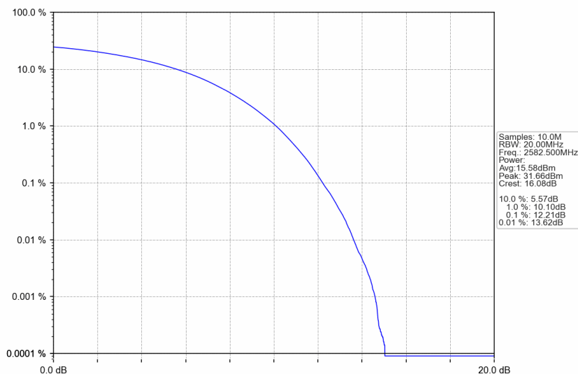
n38_15kHz_SISO_NTNV_25MHz_CP-OFDM 64 QAM_2582.5MHz_Outer_Full
