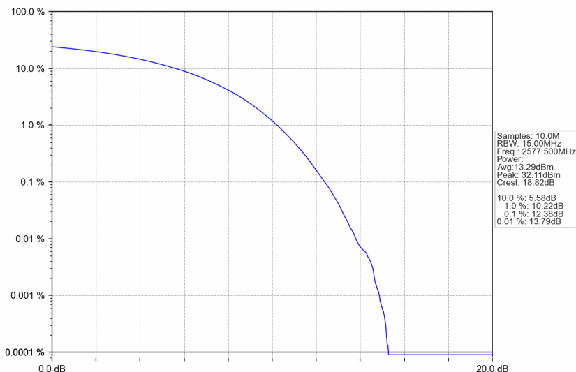
n38_15kHz_SISO_NTNV_15MHz_CP-OFDM 256 QAM_2577.5MHz_Outer_Full
