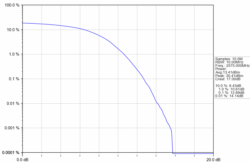
n38_15kHz_SISO_NTNV_10MHz_DFT-s-OFDM 256 QAM_2575MHz_Outer_Full
