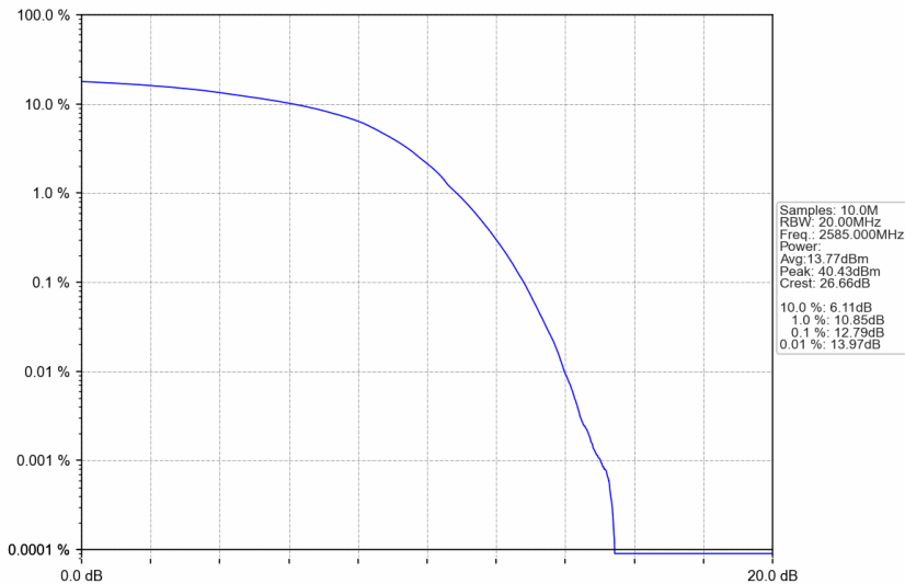
n38_15kHz_SISO_NTNV_30MHz_DFT-s-OFDM 64 QAM_2585MHz_Outer_Full
