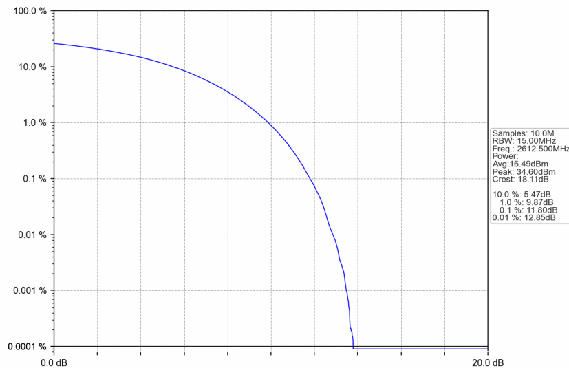
n38_15kHz_SISO_NTNV_15MHz_CP-OFDM 64 QAM_2612.5MHz_Outer_Full
