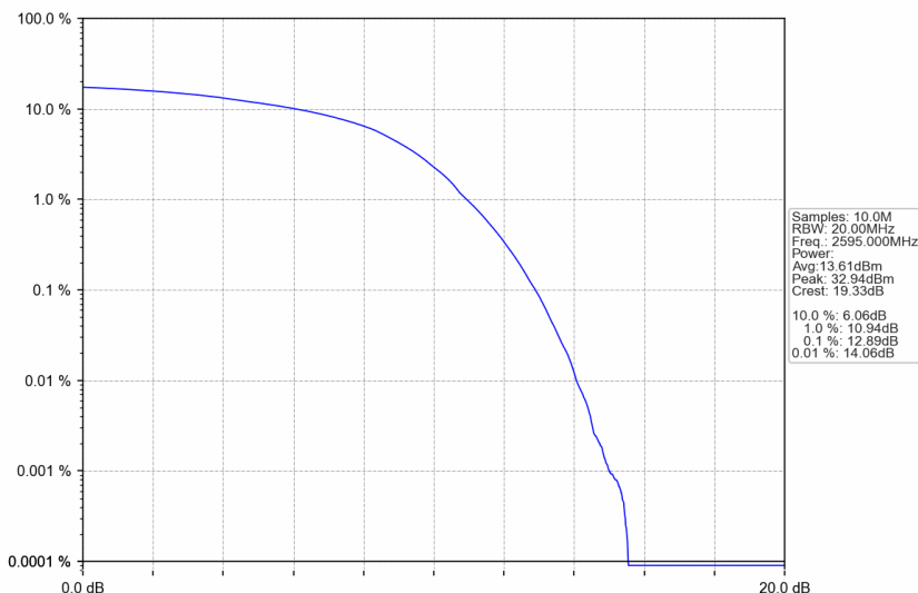
n38_15kHz_SISO_NTNV_30MHz_DFT-s-OFDM 64 QAM_2595MHz_Outer_Full
