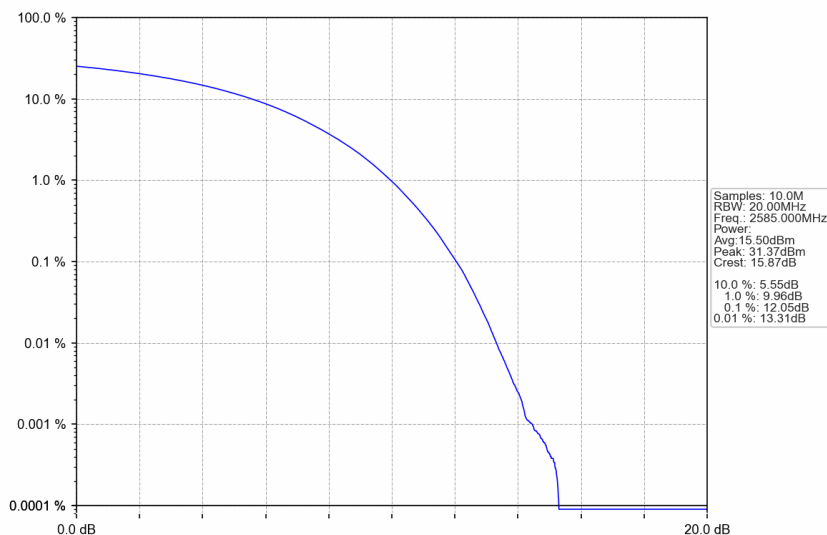
n38_15kHz_SISO_NTNV_30MHz_CP-OFDM QPSK_2585MHz_Outer_Full
