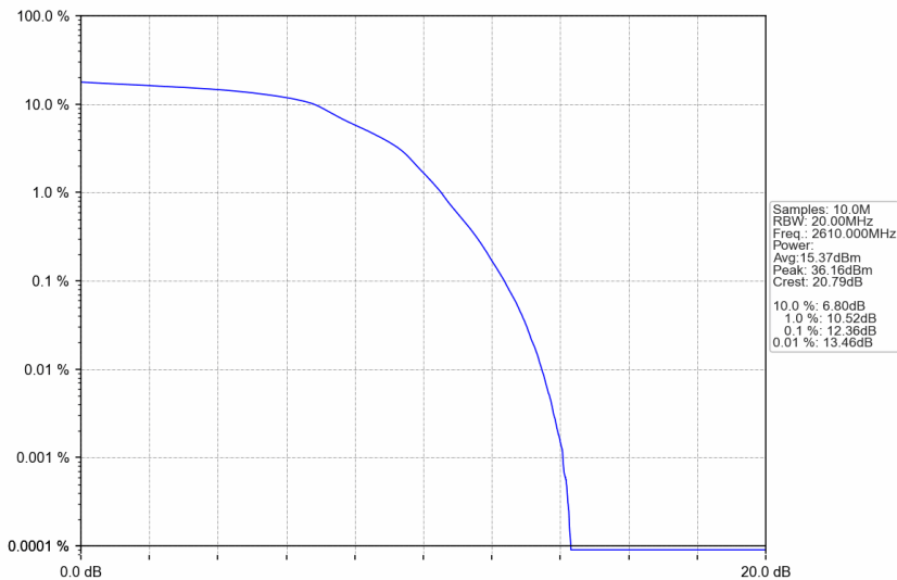
n38_15kHz_SISO_NTNV_20MHz_DFT-s-OFDM 16 QAM_2610MHz_Outer_Full
