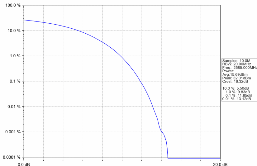
n38_15kHz_SISO_NTNV_30MHz_CP-OFDM 16 QAM_2585MHz_Outer_Full
