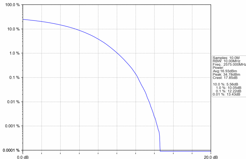
n38_15kHz_SISO_NTNV_10MHz_CP-OFDM QPSK_2575MHz_Outer_Full
