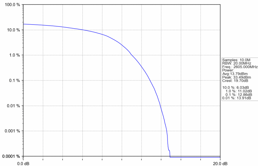
n38_15kHz_SISO_NTNV_30MHz_DFT-s-OFDM 16 QAM_2605MHz_Outer_Full
