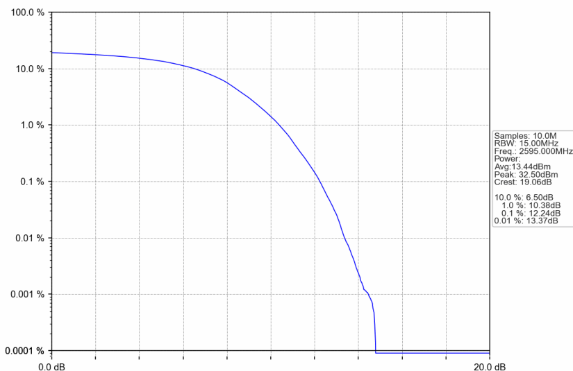
n38_15kHz_SISO_NTNV_15MHz_DFT-s-OFDM 256 QAM_2595MHz_Outer_Full
