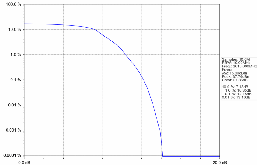
n38_15kHz_SISO_NTNV_10MHz_DFT-s-OFDM QPSK_2615MHz_Outer_Full
