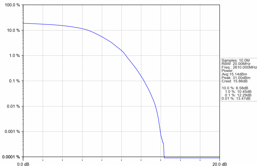
n38_15kHz_SISO_NTNV_20MHz_DFT-s-OFDM 64 QAM_2610MHz_Outer_Full
