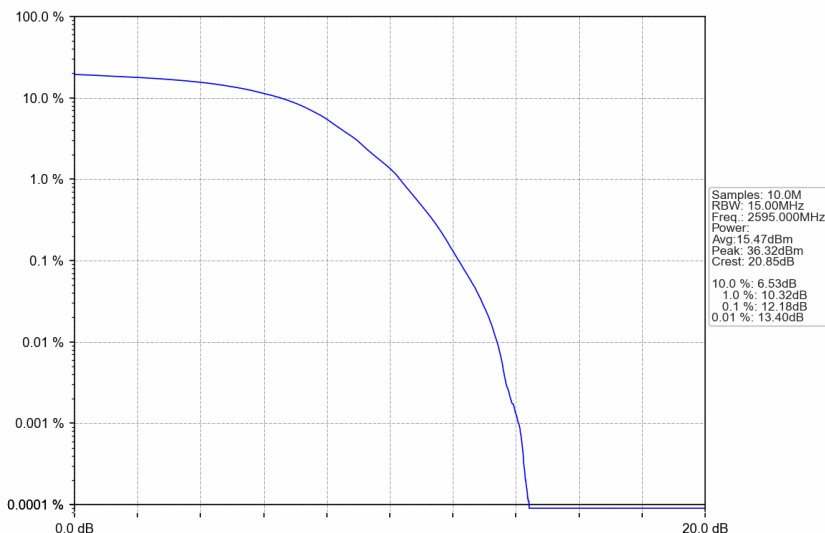
n38_15kHz_SISO_NTNV_15MHz_DFT-s-OFDM 64 QAM_2595MHz_Outer_Full
