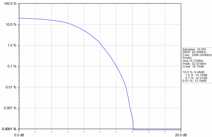
n38_15kHz_SISO_NTNV_20MHz_DFT-s-OFDM 64 QAM_2580MHz_Outer_Full
