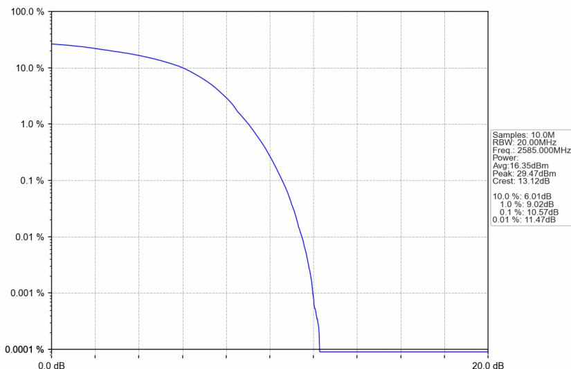
n38_15kHz_SISO_NTNV_30MHz_DFT-s-OFDM 16 QAM_2585MHz_Outer_Full
