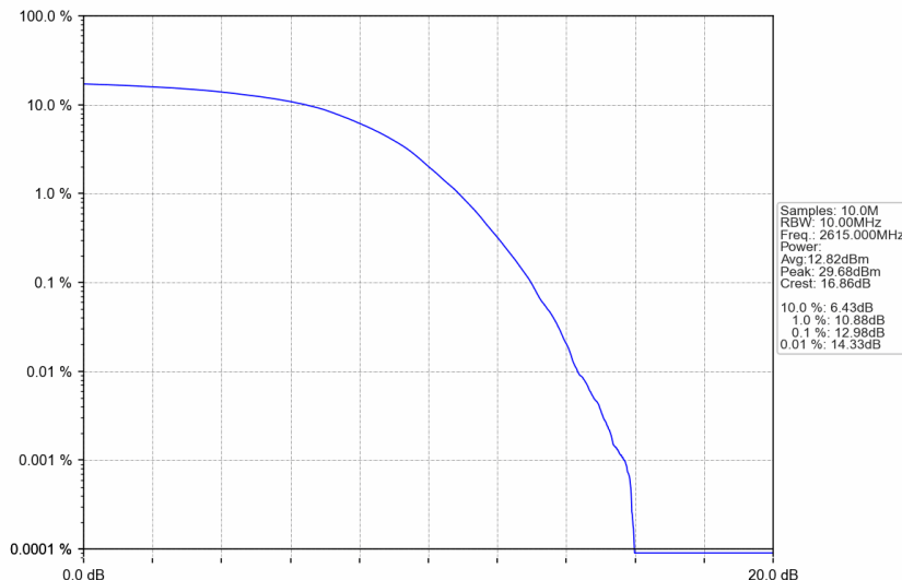
n38_15kHz_SISO_NTNV_10MHz_DFT-s-OFDM 256 QAM_2615MHz_Outer_Full
