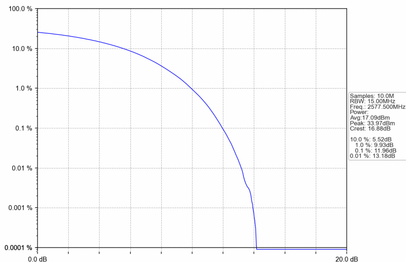
n38_15kHz_SISO_NTNV_15MHz_CP-OFDM QPSK_2577.5MHz_Outer_Full
