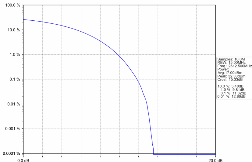
n38_15kHz_SISO_NTNV_15MHz_CP-OFDM 16 QAM_2612.5MHz_Outer_Full
