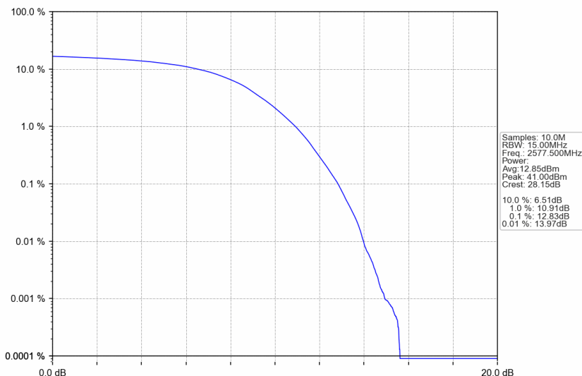
n38_15kHz_SISO_NTNV_15MHz_DFT-s-OFDM 256 QAM_2577.5MHz_Outer_Full
