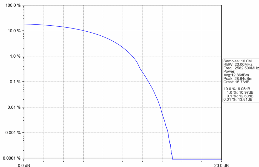
n38_15kHz_SISO_NTNV_25MHz_DFT-s-OFDM 256 QAM_2582.5MHz_Outer_Full
