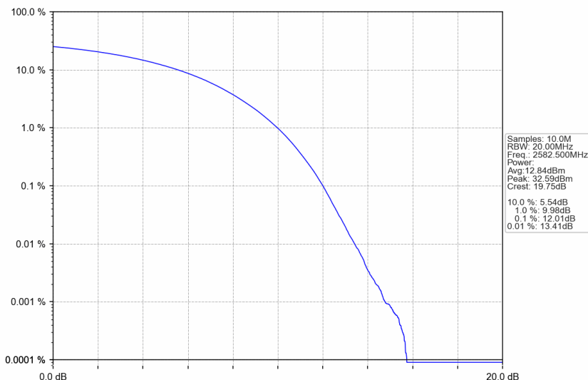
n38_15kHz_SISO_NTNV_25MHz_CP-OFDM 256 QAM_2582.5MHz_Outer_Full
