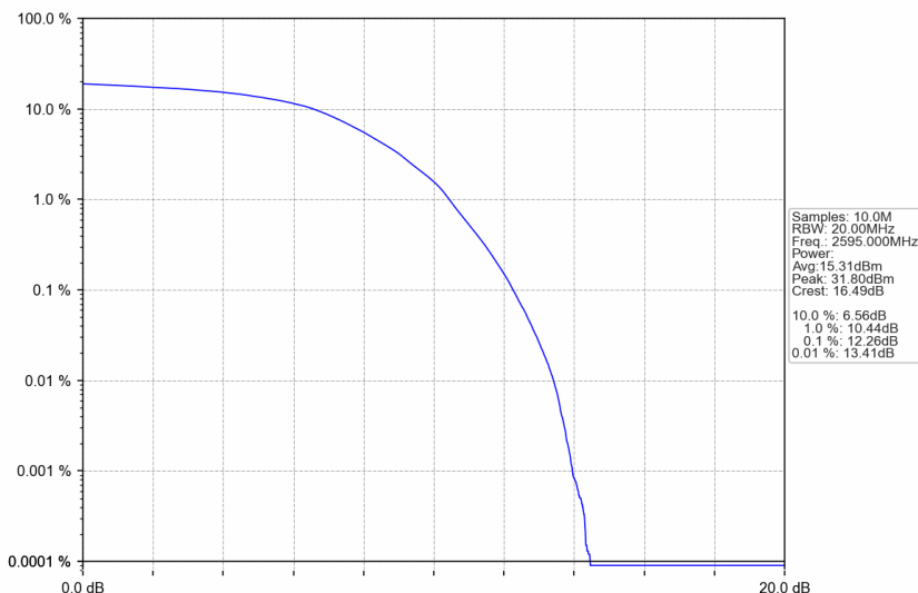
n38_15kHz_SISO_NTNV_20MHz_DFT-s-OFDM 64 QAM_2595MHz_Outer_Full
