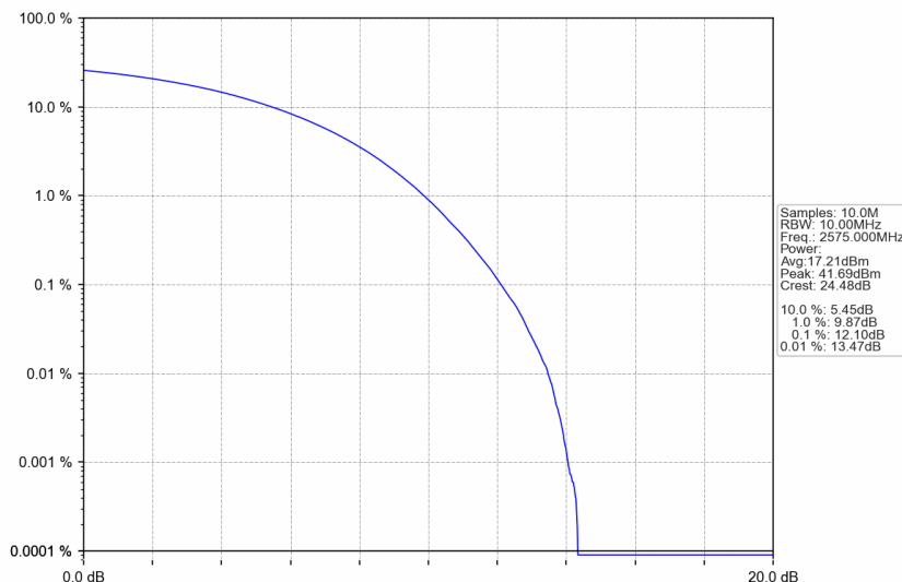
n38_15kHz_SISO_NTNV_10MHz_CP-OFDM 16 QAM_2575MHz_Outer_Full
