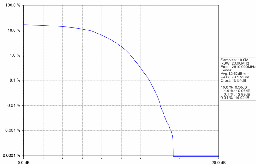
n38_15kHz_SISO_NTNV_20MHz_DFT-s-OFDM 256 QAM_2610MHz_Outer_Full
