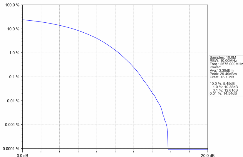
n38_15kHz_SISO_NTNV_10MHz_CP-OFDM 256 QAM_2575MHz_Outer_Full
