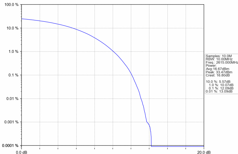
n38_15kHz_SISO_NTNV_10MHz_CP-OFDM QPSK_2615MHz_Outer_Full
