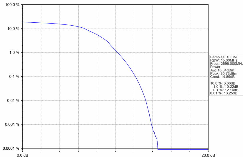
n38_15kHz_SISO_NTNV_15MHz_DFT-s-OFDM 16 QAM_2595MHz_Outer_Full
