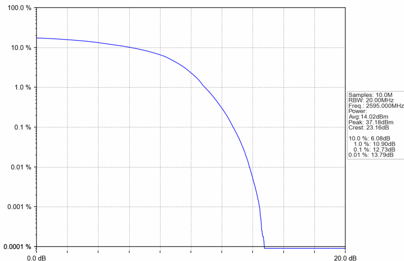
n38_15kHz_SISO_NTNV_30MHz_DFT-s-OFDM 16 QAM_2595MHz_Outer_Full
