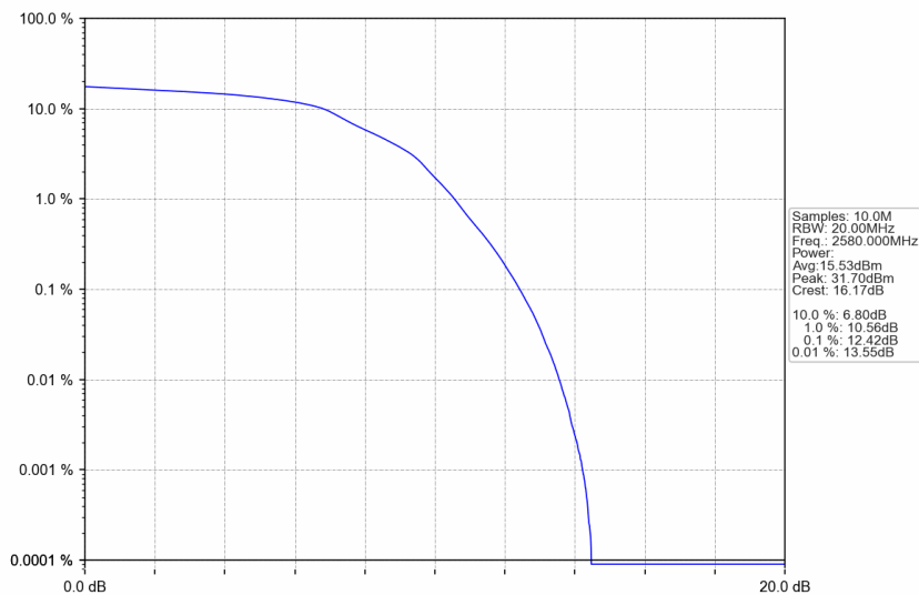
n38_15kHz_SISO_NTNV_20MHz_DFT-s-OFDM 16 QAM_2580MHz_Outer_Full
