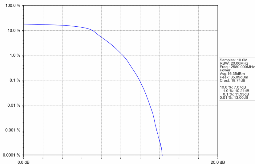
n38_15kHz_SISO_NTNV_20MHz_DFT-s-OFDM QPSK_2580MHz_Outer_Full
