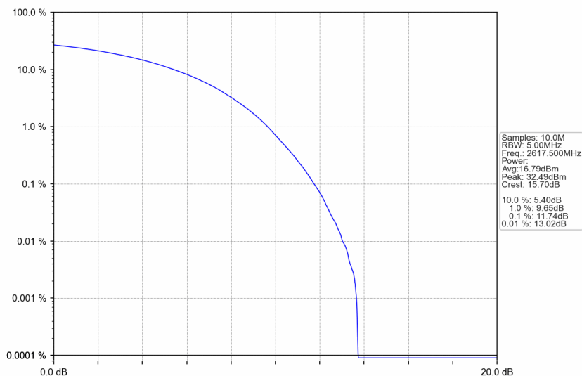
n38_15kHz_SISO_NTNV_5MHz_CP-OFDM 64 QAM_2617.5MHz_Outer_Full
