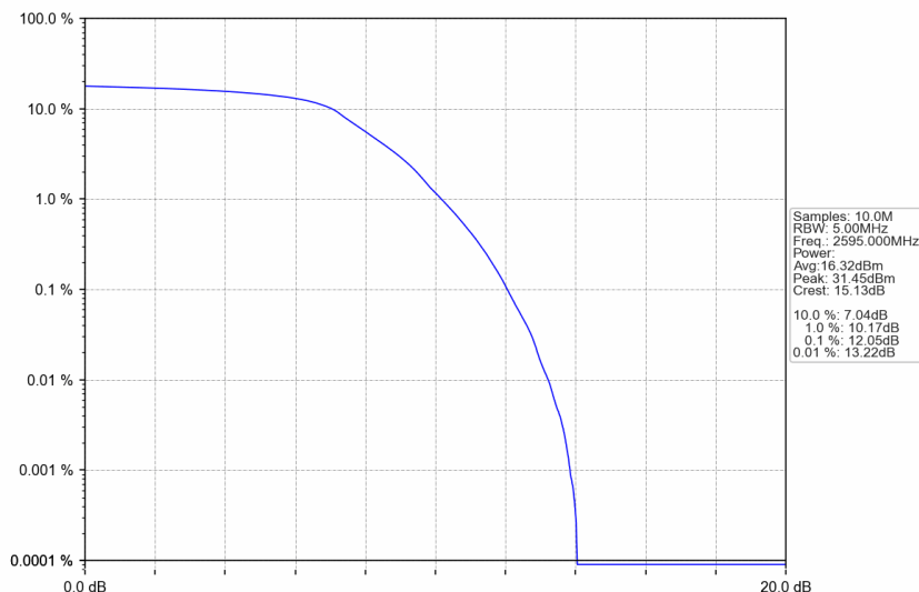
n38_15kHz_SISO_NTNV_5MHz_DFT-s-OFDM QPSK_2595MHz_Outer_Full
