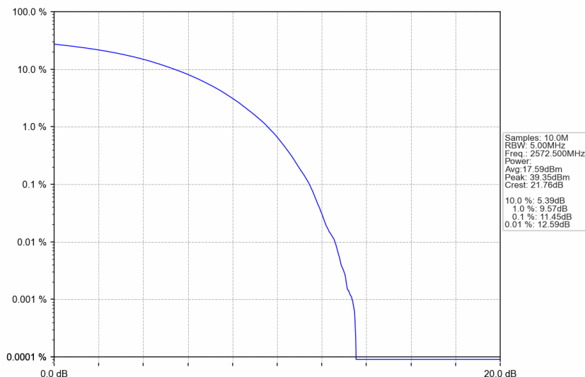
n38_15kHz_SISO_NTNV_5MHz_CP-OFDM 16 QAM_2572.5MHz_Outer_Full
