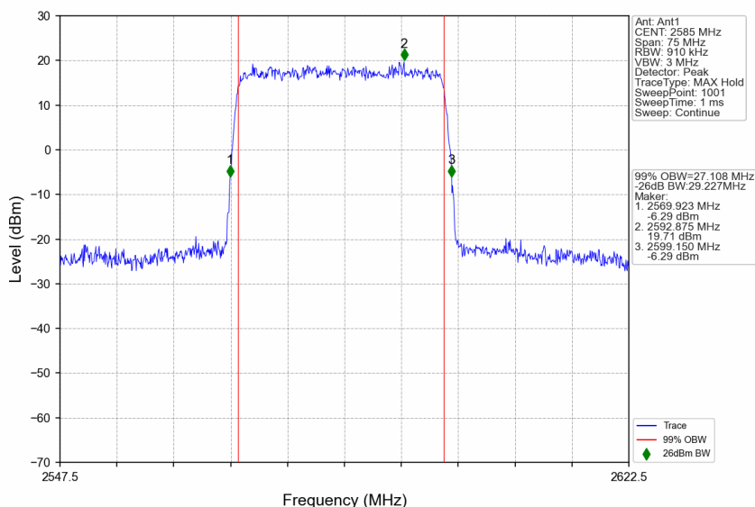
n38_30kHz_SISO_NTNV_30MHz_DFT-s-OFDM QPSK_2585MHz_Outer_Full
