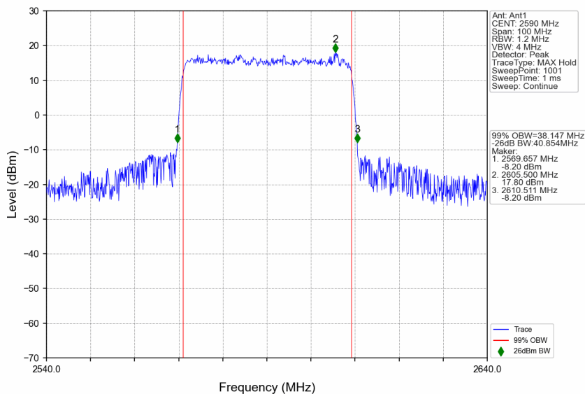
n38_30kHz_SISO_NTNV_40MHz_CP-OFDM QPSK_2590MHz_Outer_Full
