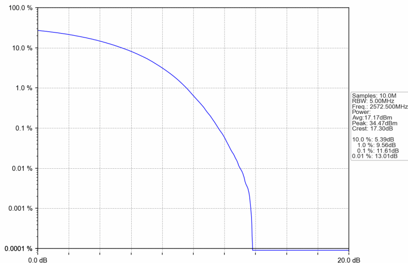
n38_15kHz_SISO_NTNV_5MHz_CP-OFDM 64 QAM_2572.5MHz_Outer_Full
