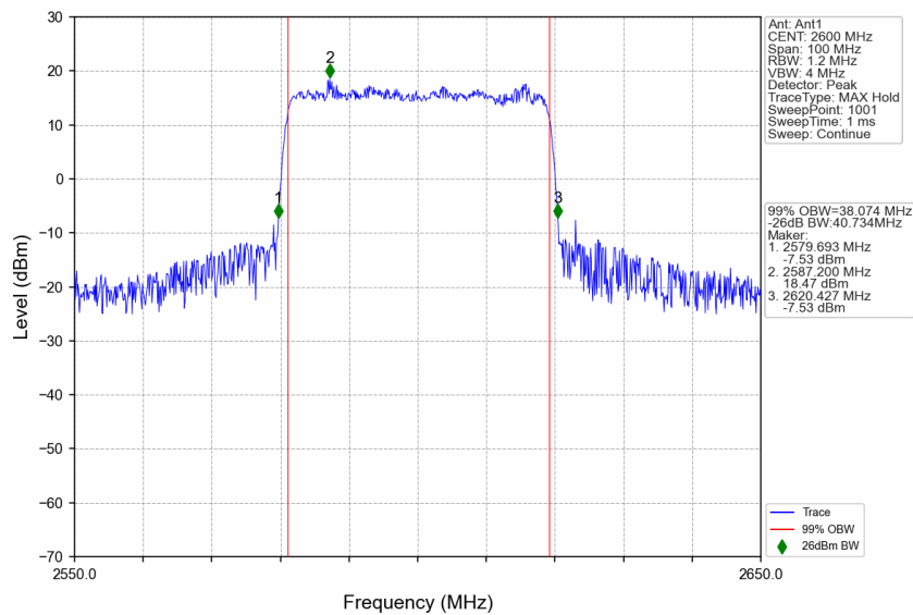
n38_30kHz_SISO_NTNV_40MHz_CP-OFDM QPSK_2600MHz_Outer_Full
