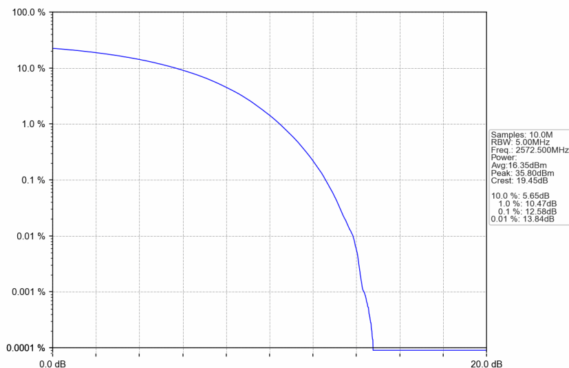
n38_15kHz_SISO_NTNV_5MHz_CP-OFDM QPSK_2572.5MHz_Outer_Full
