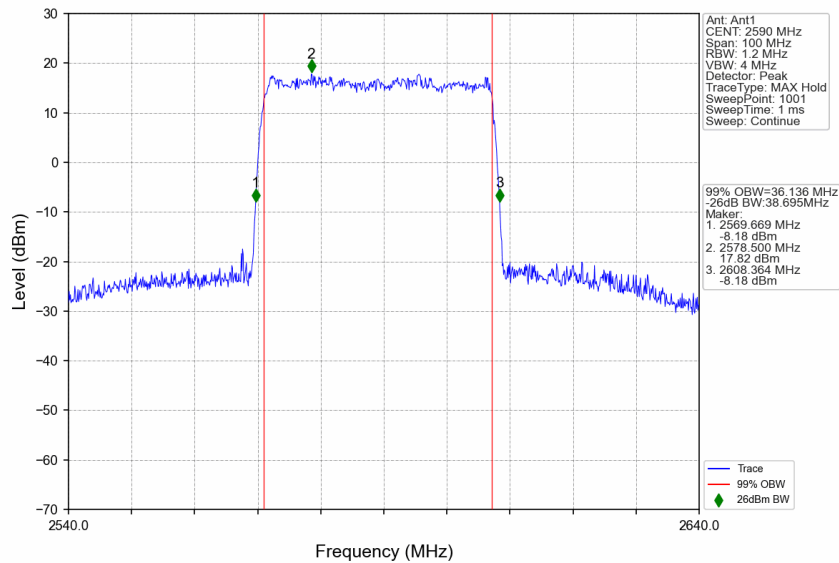
n38_30kHz_SISO_NTNV_40MHz_DFT-s-OFDM 64 QAM_2590MHz_Outer_Full
