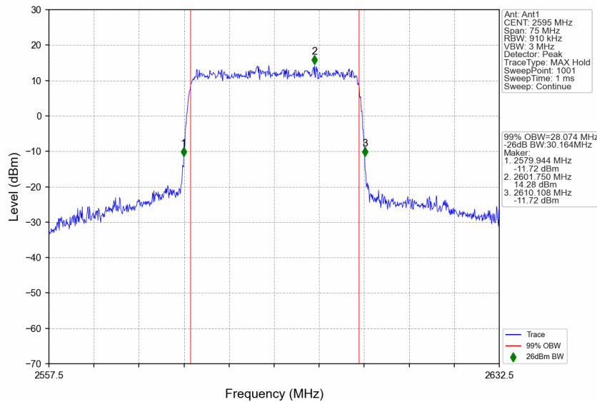
n38_30kHz_SISO_NTNV_30MHz_CP-OFDM 256 QAM_2595MHz_Outer_Full
