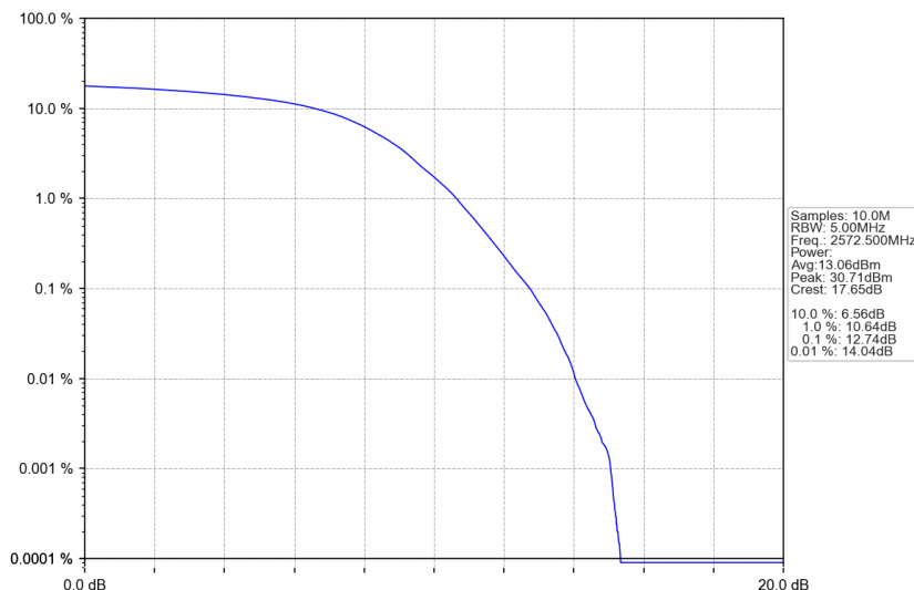
n38_15kHz_SISO_NTNV_5MHz_DFT-s-OFDM 256 QAM_2572.5MHz_Outer_Full
