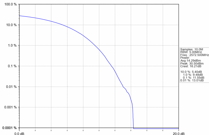
n38_15kHz_SISO_NTNV_5MHz_CP-OFDM 256 QAM_2572.5MHz_Outer_Full
