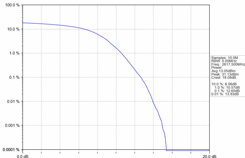
n38_15kHz_SISO_NTNV_5MHz_DFT-s-OFDM 256 QAM_2617.5MHz_Outer_Full
