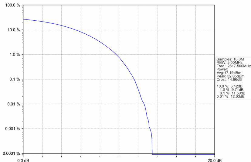
n38_15kHz_SISO_NTNV_5MHz_CP-OFDM 16 QAM_2617.5MHz_Outer_Full
