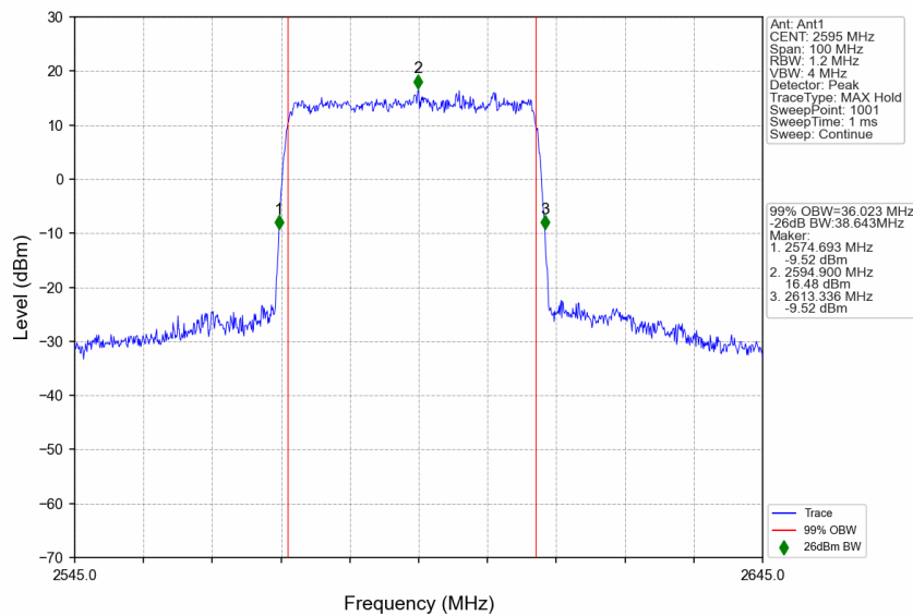
n38_30kHz_SISO_NTNV_40MHz_DFT-s-OFDM 256 QAM_2595MHz_Outer_Full
