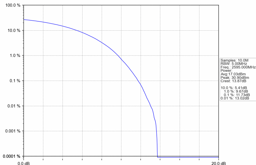
n38_15kHz_SISO_NTNV_5MHz_CP-OFDM 64 QAM_2595MHz_Outer_Full
