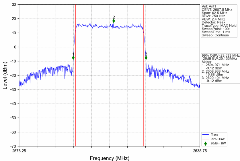
n38_30kHz_SISO_NTNV_25MHz_CP-OFDM 64 QAM_2607.5MHz_Outer_Full
