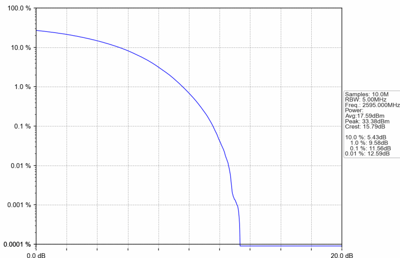
n38_15kHz_SISO_NTNV_5MHz_CP-OFDM QPSK_2595MHz_Outer_Full
