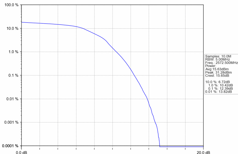
n38_15kHz_SISO_NTNV_5MHz_DFT-s-OFDM 16 QAM_2572.5MHz_Outer_Full
