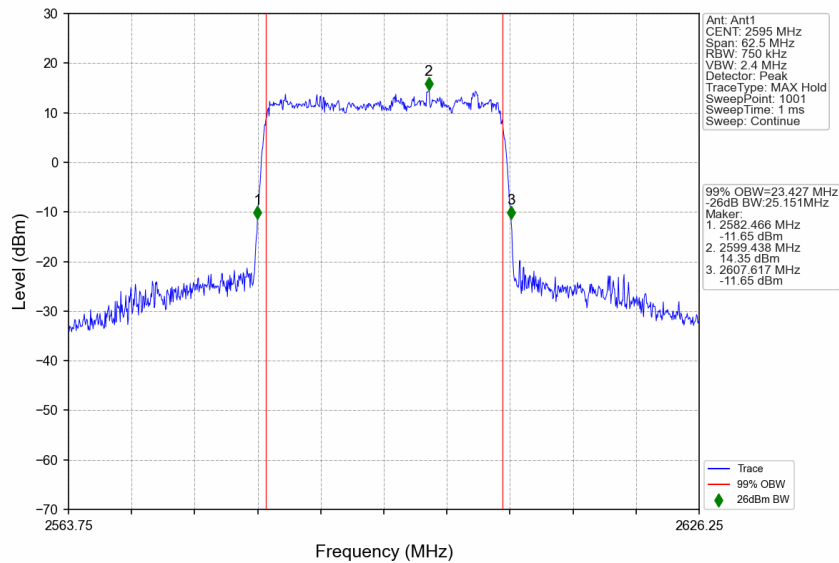
n38_30kHz_SISO_NTNV_25MHz_CP-OFDM 256 QAM_2595MHz_Outer_Full
