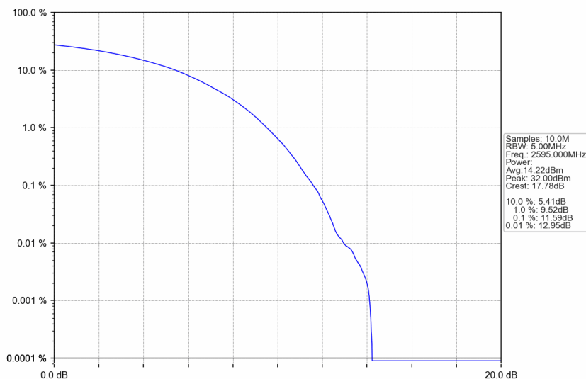
n38_15kHz_SISO_NTNV_5MHz_CP-OFDM 256 QAM_2595MHz_Outer_Full
