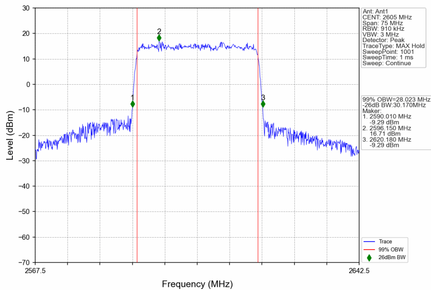
n38_30kHz_SISO_NTNV_30MHz_CP-OFDM 64 QAM_2605MHz_Outer_Full
