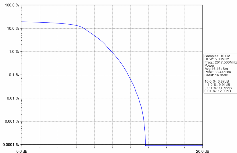
n38_15kHz_SISO_NTNV_5MHz_DFT-s-OFDM QPSK_2617.5MHz_Outer_Full
