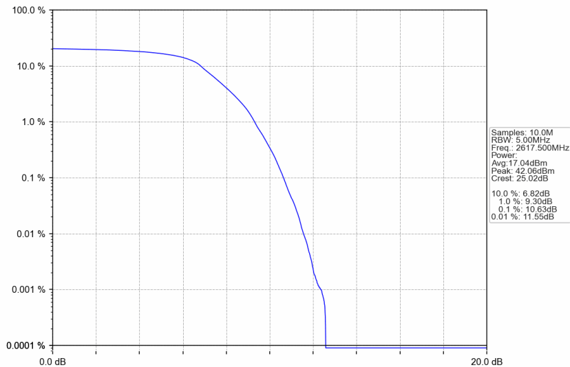
n38_15kHz_SISO_NTNV_5MHz_DFT-s-OFDM PI/2 BPSK_2617.5MHz_Outer_Full
