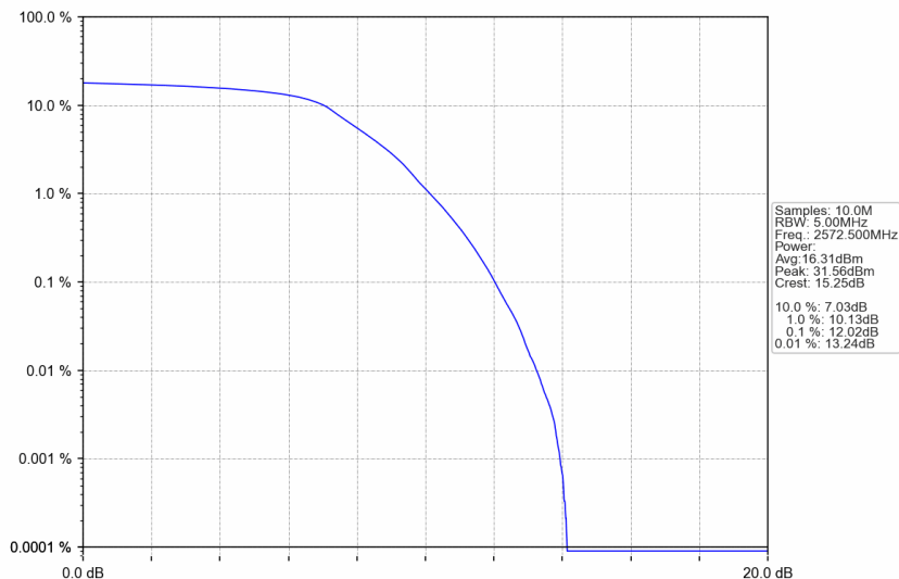
n38_15kHz_SISO_NTNV_5MHz_DFT-s-OFDM QPSK_2572.5MHz_Outer_Full
