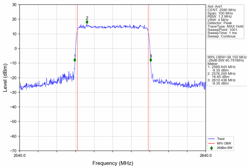
n38_30kHz_SISO_NTNV_40MHz_CP-OFDM 64 QAM_2590MHz_Outer_Full
