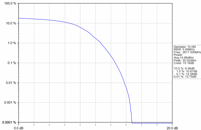
n38_15kHz_SISO_NTNV_5MHz_DFT-s-OFDM 64 QAM_2617.5MHz_Outer_Full
