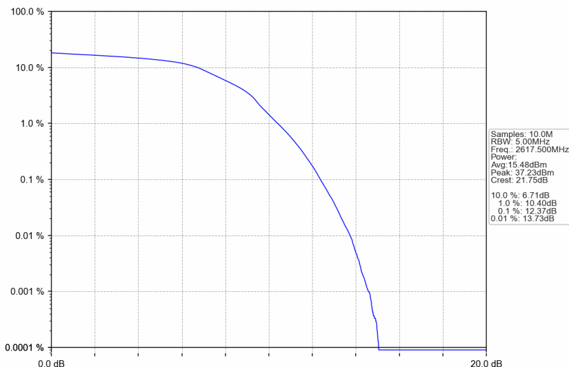
n38_15kHz_SISO_NTNV_5MHz_DFT-s-OFDM 16 QAM_2617.5MHz_Outer_Full
