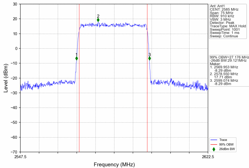
n38_30kHz_SISO_NTNV_30MHz_DFT-s-OFDM 64 QAM_2585MHz_Outer_Full
