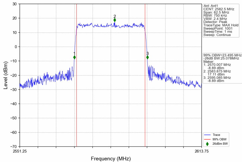
n38_30kHz_SISO_NTNV_25MHz_CP-OFDM 64 QAM_2582.5MHz_Outer_Full
