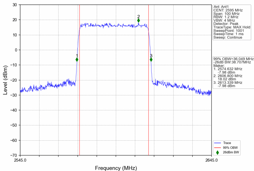
n38_30kHz_SISO_NTNV_40MHz_DFT-s-OFDM 16 QAM_2595MHz_Outer_Full
