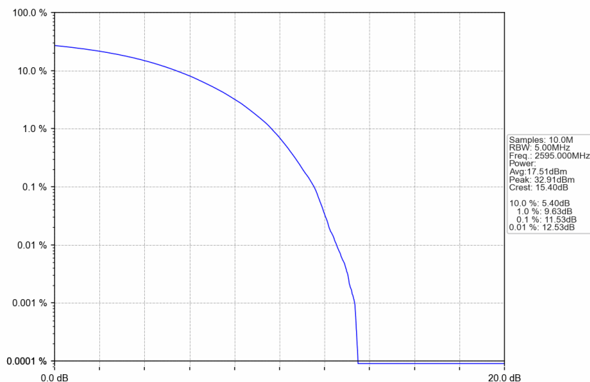
n38_15kHz_SISO_NTNV_5MHz_CP-OFDM 16 QAM_2595MHz_Outer_Full
