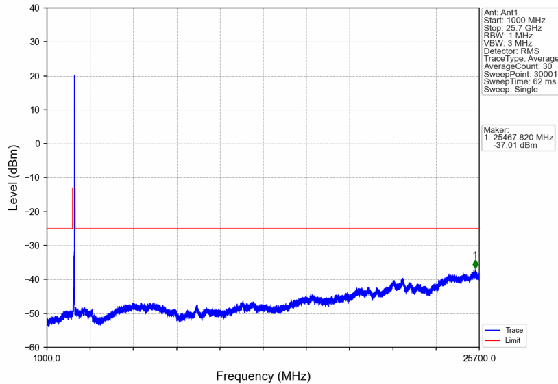
n7_30kHz_SiSO_NTNV_40MHz_CP-OFDM QPSK_2550MHz_Edge_1RB_Right
