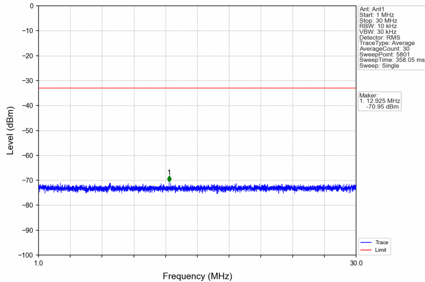
n7_30kHz_SISO_NTNV_50MHz_CP-OFDM QPSK_2545MHz_Edge_1RB_Right
