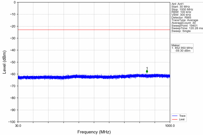
n7_30kHz_SISO_NTNV_50MHz_DFT-s-OFDM QPSK_2545MHz_Edge_1RB_Right
