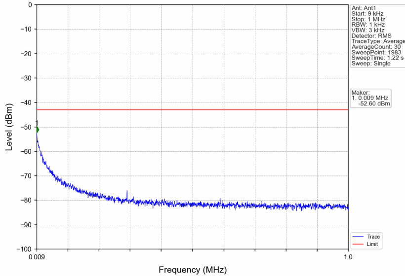
n7_30kHz_SiSO_NTNV_40MHz_CP-OFDM QPSK_2550MHz_Edge_1RB_Right
