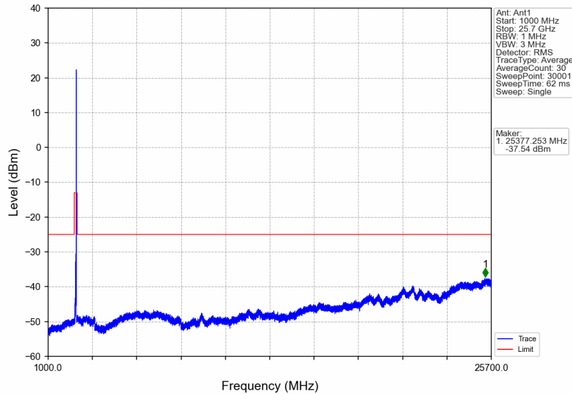
n7_30kHz_SISO_NTNV_50MHz_DFT-s-OFDM QPSK_2545MHz_Edge_1RB_Right
