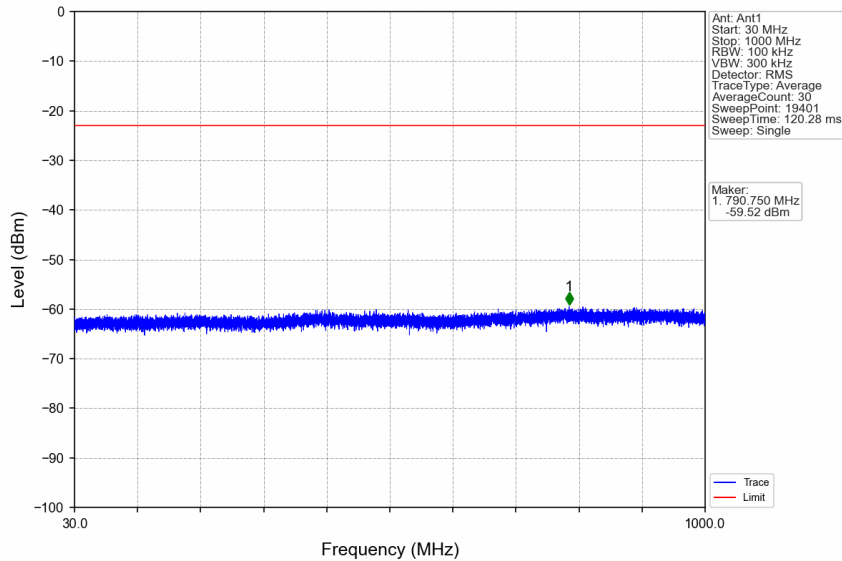
n7_30kHz_SISO_NTNV_50MHz_CP-OFDM QPSK_2525MHz_Edge_1RB_Left
