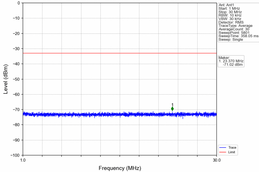
n7_30kHz_SISO_NTNV_50MHz_DFT-s-OFDM QPSK_2525MHz_Edge_1RB_Left
