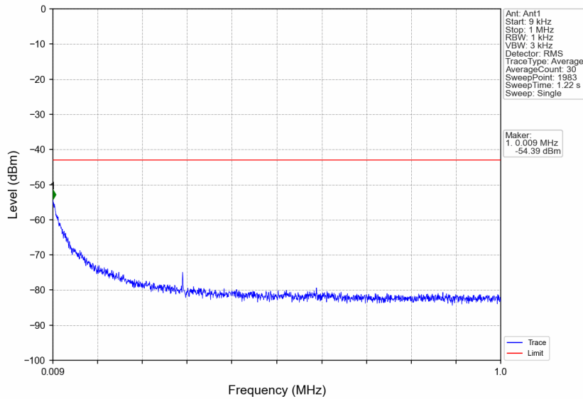
n7_30kHz_SISO_NTNV_50MHz_DFT-s-OFDM QPSK_2545MHz_Edge_1RB_Right
