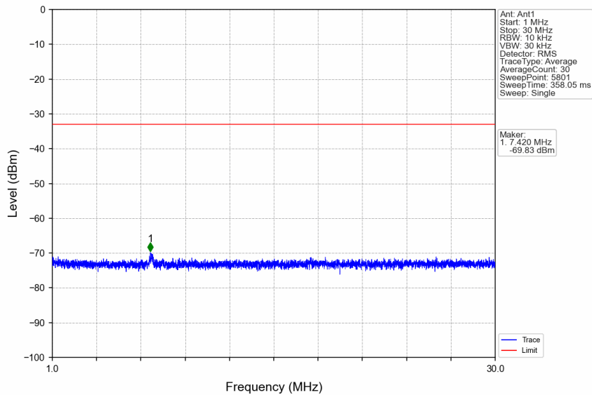
n7_30kHz_SISO_NTNV_50MHz_DFT-s-OFDM QPSK_2545MHz_Edge_1RB_Right
