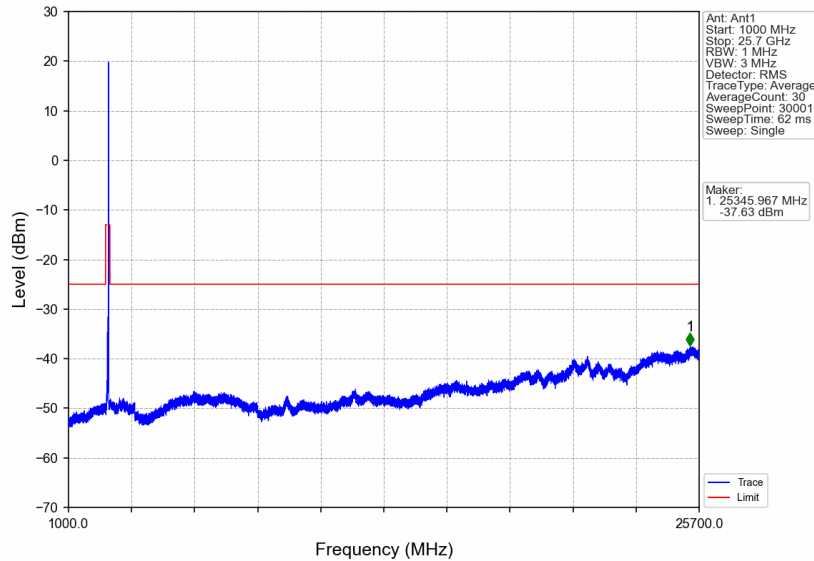
n7_30kHz_SiSO_NTNV_50MHz_CP-OFDM QPSK_2545MHz_Edge_1RB_Right
