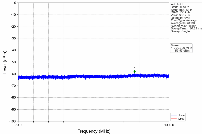
n7_30kHz_SISO_NTNV_50MHz_DFT-s-OFDM QPSK_2535MHz_Edge_1RB_Left
