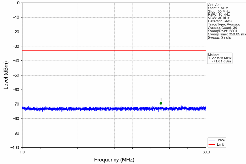
n7_30kHz_SISO_NTNV_50MHz_DFT-s-OFDM QPSK_2535MHz_Edge_1RB_Left
