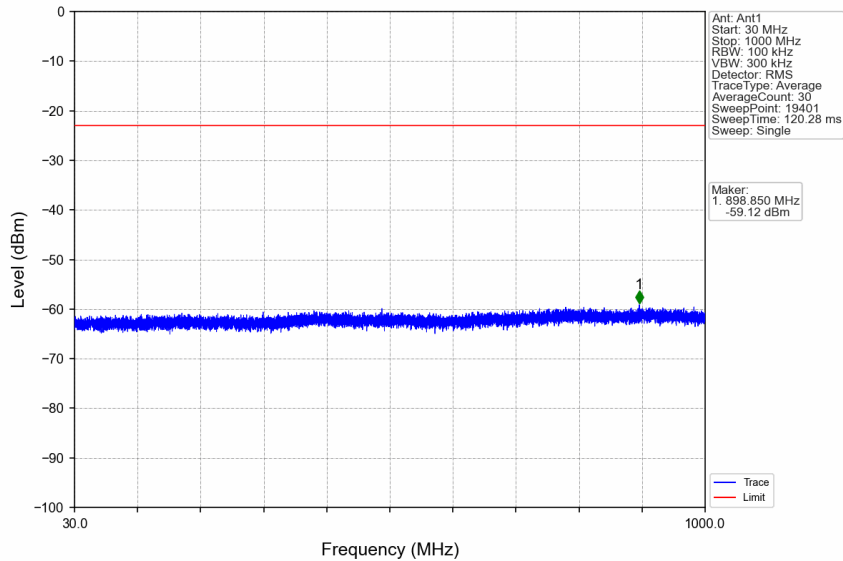
n7_30kHz_SISO_NTNV_50MHz_CP-OFDM QPSK_2535MHz_Edge_1RB_Left
