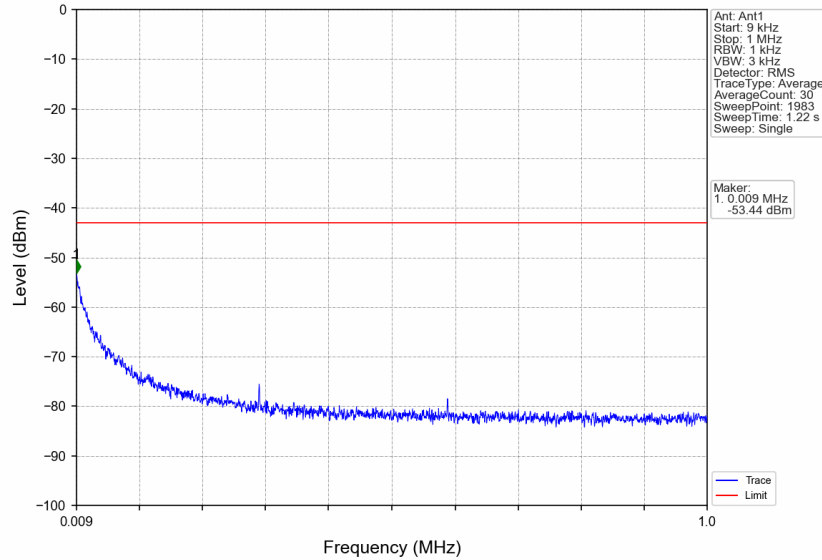
n7_30kHz_SISO_NTNV_50MHz_CP-OFDM QPSK_2545MHz_Edge_1RB_Right
