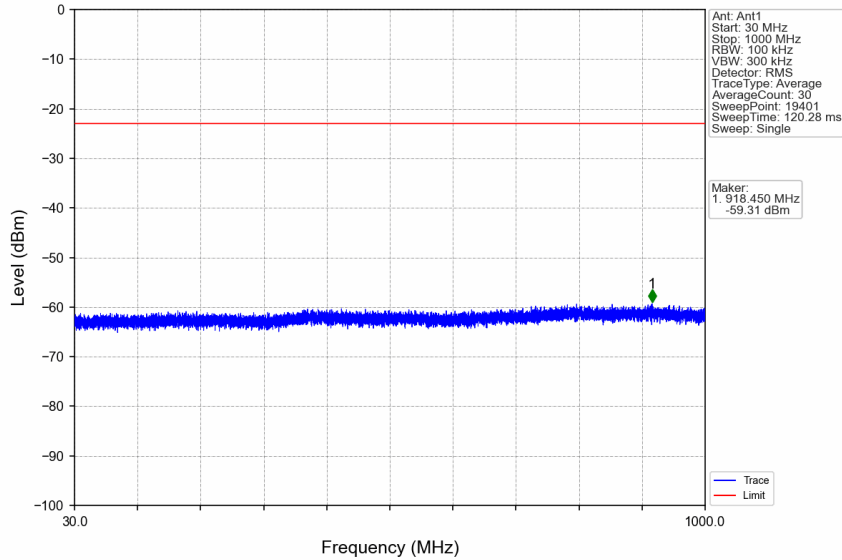
n7_30kHz_SiSO_NTNV_40MHz_CP-OFDM QPSK_2550MHz_Edge_1RB_Right
