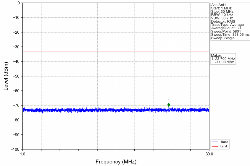
n7_30kHz_SISO_NTNV_40MHz_DFT-s-OFDM QPSK_2535MHz_Edge_1RB_Left
