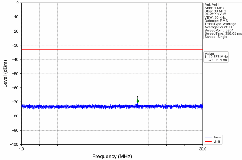
n7_30kHz_SISO_NTNV_30MHz_CP-OFDM QPSK_2535MHz_Edge_1RB_Left
