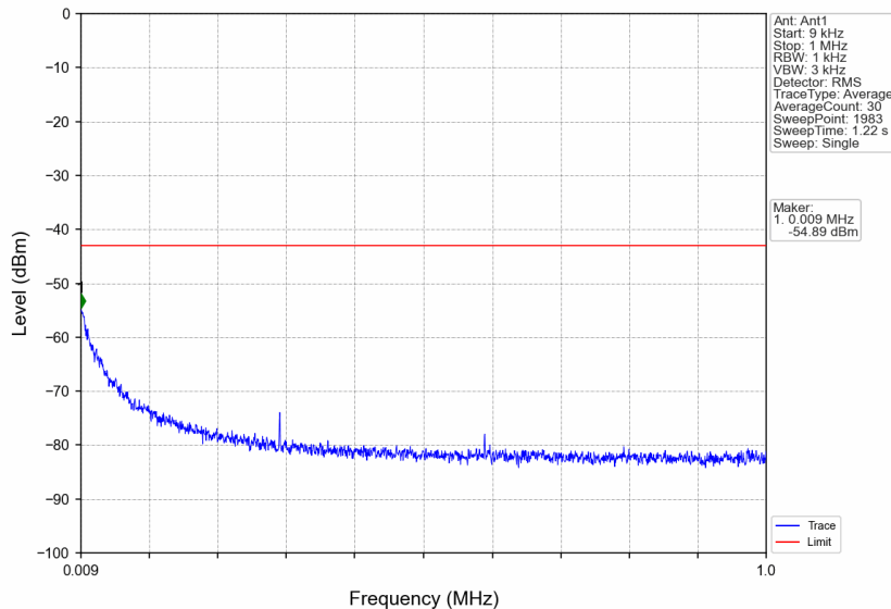
n7_30kHz_SISO_NTNV_30MHz_DFT-s-OFDM PI/2 BPSK_2515MHz_Edge_1RB_Left
