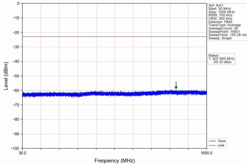
n7_30kHz_SISO_NTNV_40MHz_DFT-s-OFDM QPSK_2535MHz_Edge_1RB_Left
