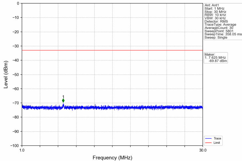
n7_30kHz_SISO_NTNV_40MHz_DFT-s-OFDM QPSK_2550MHz_Edge_1RB_Right
