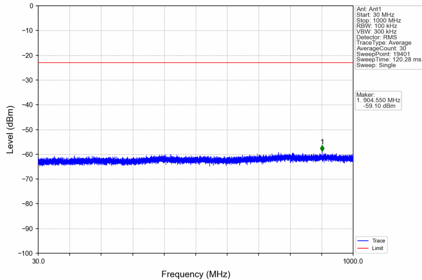
n7_30kHz_SISO_NTNV_30MHz_DFT-s-OFDM QPSK_2515MHz_Edge_1RB_Left
