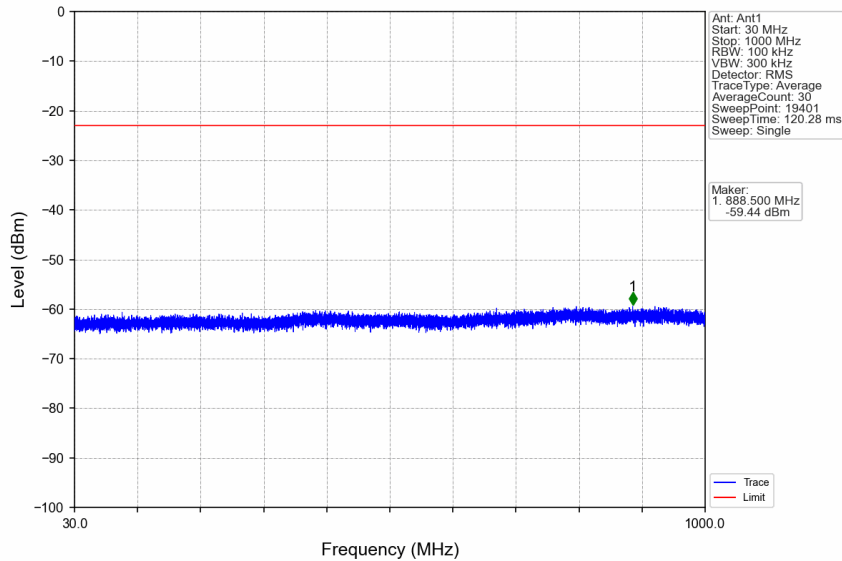
n7_30kHz_SISO_NTNV_40MHz_CP-OFDM QPSK_2520MHz_Edge_1RB_Left
