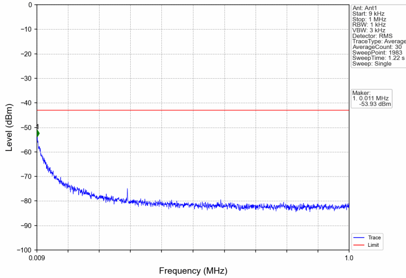
n7_30kHz_SiSO_NTNV_30MHz_CP-OFDM QPSK_2555MHz_Edge_1RB_Right
