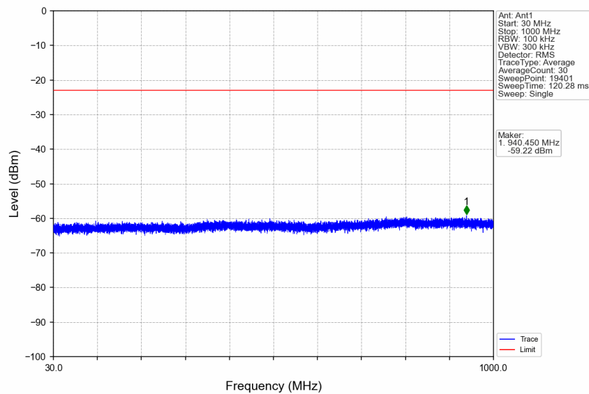
n7_30kHz_SISO_NTNV_40MHz_CP-OFDM QPSK_2535MHz_Edge_1RB_Left
