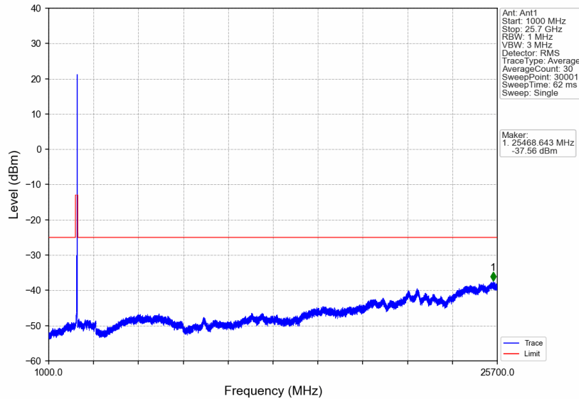
n7_30kHz_SISO_NTNV_30MHz_DFT-s-OFDM QPSK_2555MHz_Edge_1RB_Right
