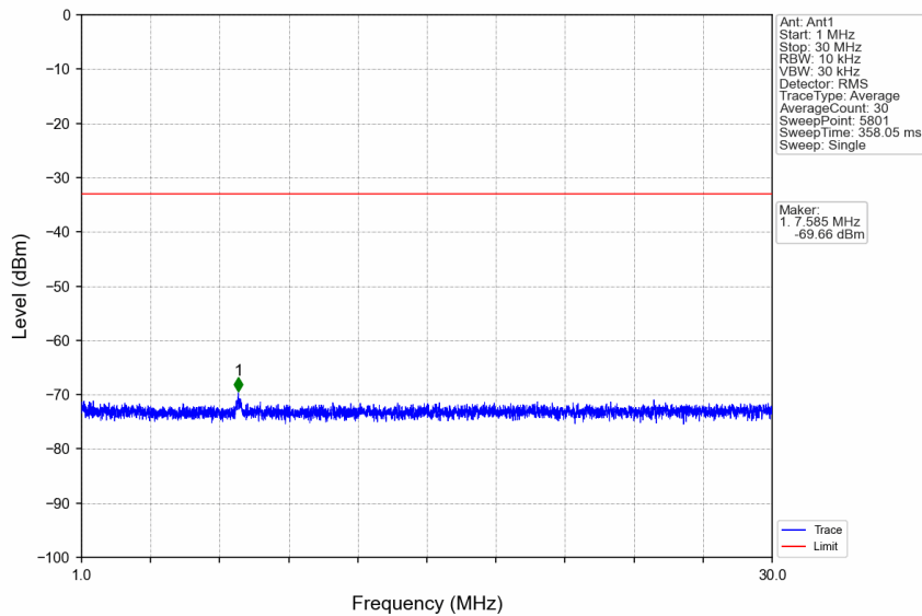
n7_30kHz_SISO_NTNV_30MHz_DFT-s-OFDM QPSK_2555MHz_Edge_1RB_Right
