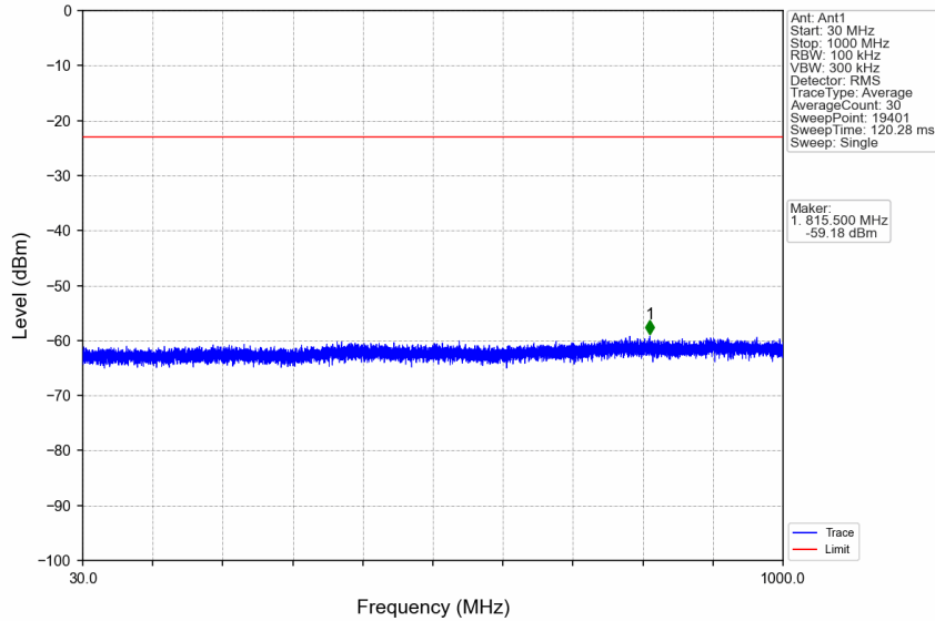
n7_30kHz_SISO_NTNV_30MHz_DFT-s-OFDM QPSK_2555MHz_Edge_1RB_Right
