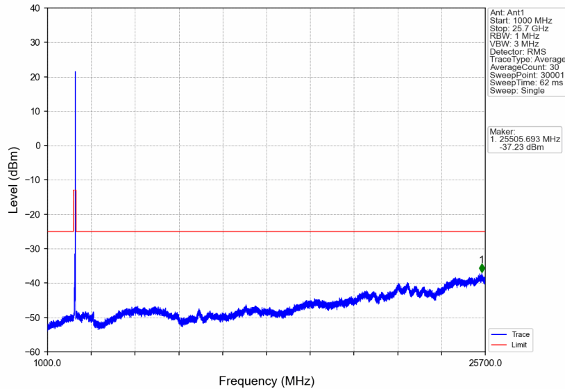
n7_30kHz_SISO_NTNV_40MHz_DFT-s-OFDM QPSK_2550MHz_Edge_1RB_Right
