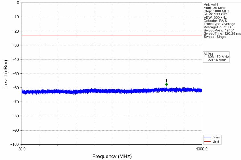
n7_30kHz_SISO_NTNV_30MHz_CP-OFDM QPSK_2555MHz_Edge_1RB_Right
