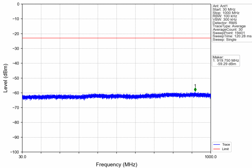
n7_30kHz_SISO_NTNV_30MHz_CP-OFDM QPSK_2515MHz_Edge_1RB_Left
