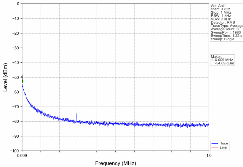
n7_30kHz_SISO_NTNV_30MHz_DFT-s-OFDM QPSK_2555MHz_Edge_1RB_Right
