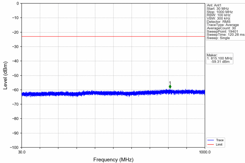
n7_30kHz_SISO_NTNV_40MHz_DFT-s-OFDM QPSK_2520MHz_Edge_1RB_Left
