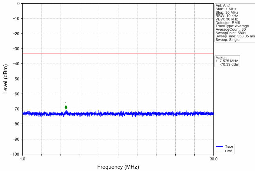
n7_30kHz_SiSO_NTNV_30MHz_CP-OFDM QPSK_2555MHz_Edge_1RB_Right
