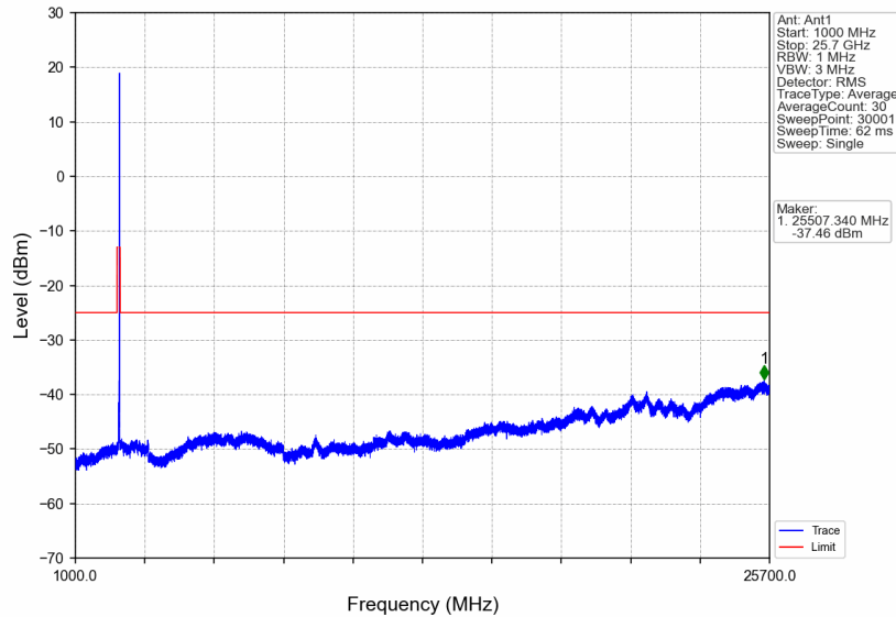
n7_30kHz_SISO_NTNV_20MHz_CP-OFDM QPSK_2560MHz_Edge_1RB_Right
