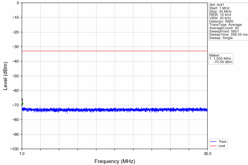
n7_30kHz_SISO_NTNV_25MHz_DFT-s-OFDM QPSK_2512.5MHz_Edge_1RB_Left
