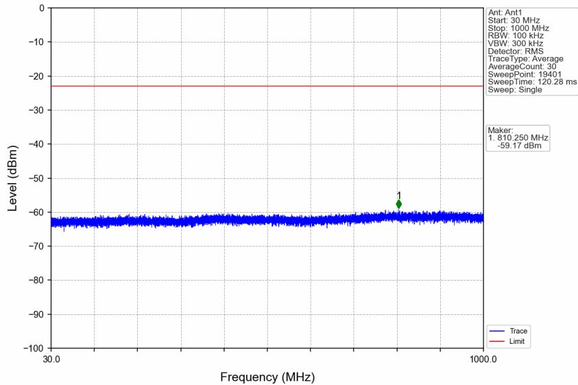
n7_30kHz_SISO_NTNV_20MHz_CP-OFDM_QPSK_2535MHz_Edge_1RB_Left
