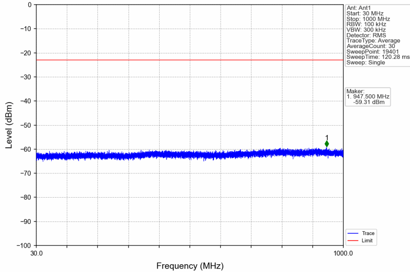
n7_30kHz_SISO_NTNV_20MHz_DFT-s-OFDM QPSK_2560MHz_Edge_1RB_Right
