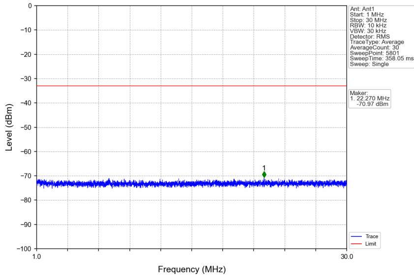
n7_30kHz_SISO_NTNV_20MHz_CP-OFDM QPSK_2560MHz_Edge_1RB_Right
