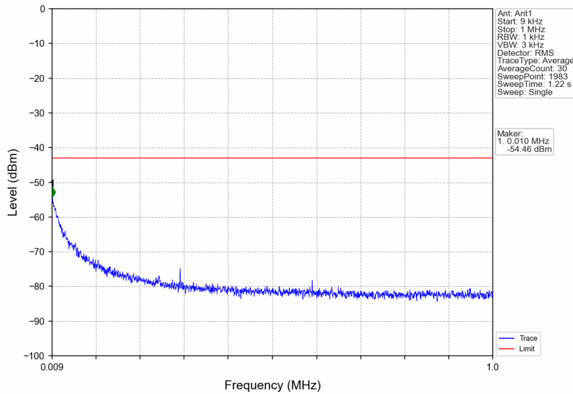
n7_30kHz_SISO_NTNV_20MHz_DFT-s-OFDM QPSK_2560MHz_Edge_1RB_Right
