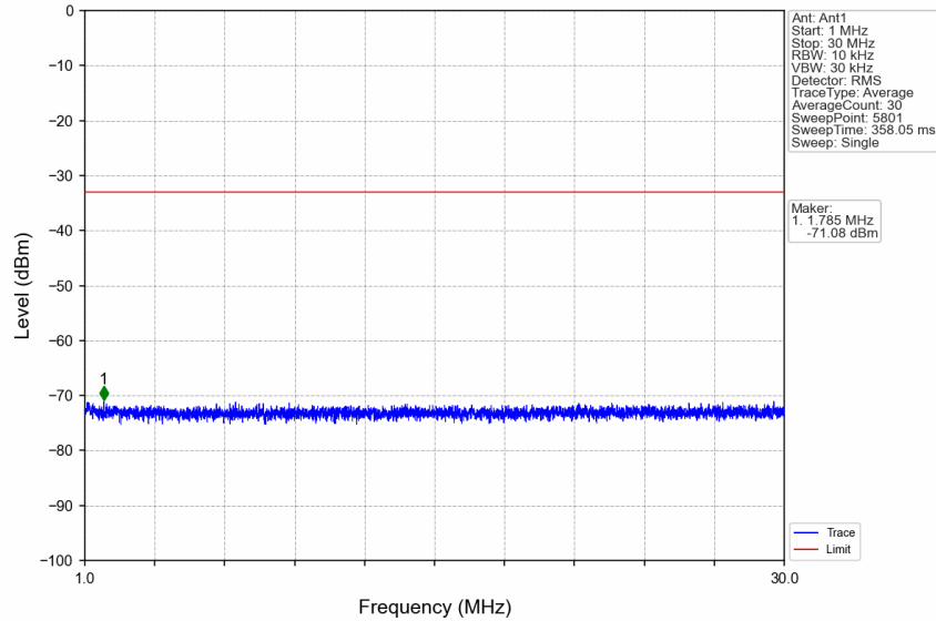
n7_30kHz_SISO_NTNV_20MHz_DFT-s-OFDM QPSK_2510MHz_Edge_1RB_Left
