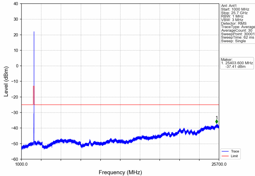
n7_30kHz_SISO_NTNV_25MHz_DFT-s-OFDM_QPSK_2557.5MHz_Edge_1RB_Right
