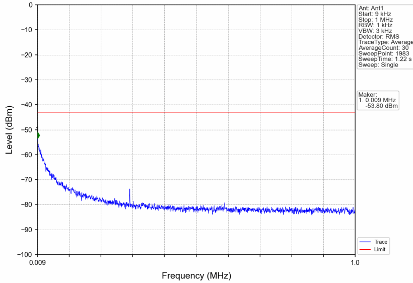
n7_30kHz_SISO_NTNV_25MHz_DFT-s-OFDM_QPSK_2557.5MHz_Edge_1RB_Right
