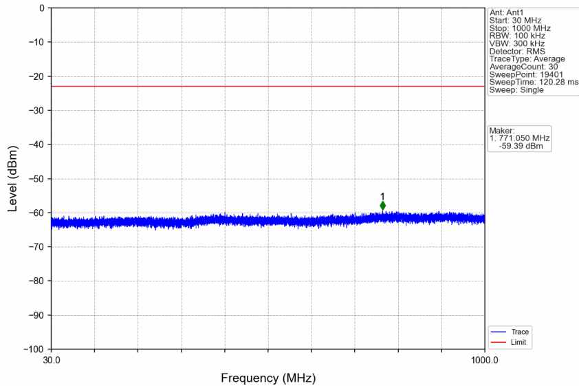
n7_30kHz_SISO_NTNV_25MHz_CP-OFDM QPSK_2512.5MHz_Edge_1RB_Left
