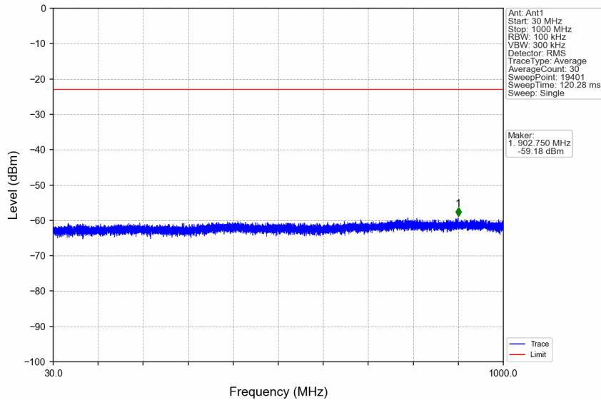
n7_30kHz_SISO_NTNV_20MHz_DFT-s-OFDM QPSK_2535MHz_Edge_1RB_Left
