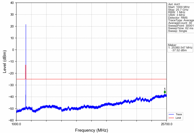
n7_30kHz_SISO_NTNV_20MHz_DFT-s-OFDM QPSK_2560MHz_Edge_1RB_Right
