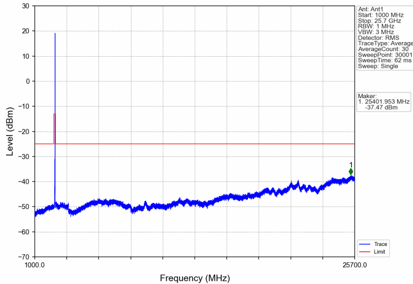
n7_30kHz_SISO_NTNV_25MHz_CP-OFDM QPSK_2557.5MHz_Edge_1RB_Right
