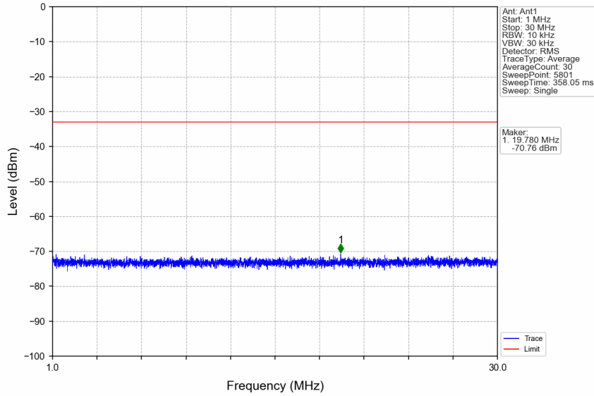
n7_30kHz_SISO_NTNV_25MHz_CP-OFDM QPSK_2512.5MHz_Edge_1RB_Left
