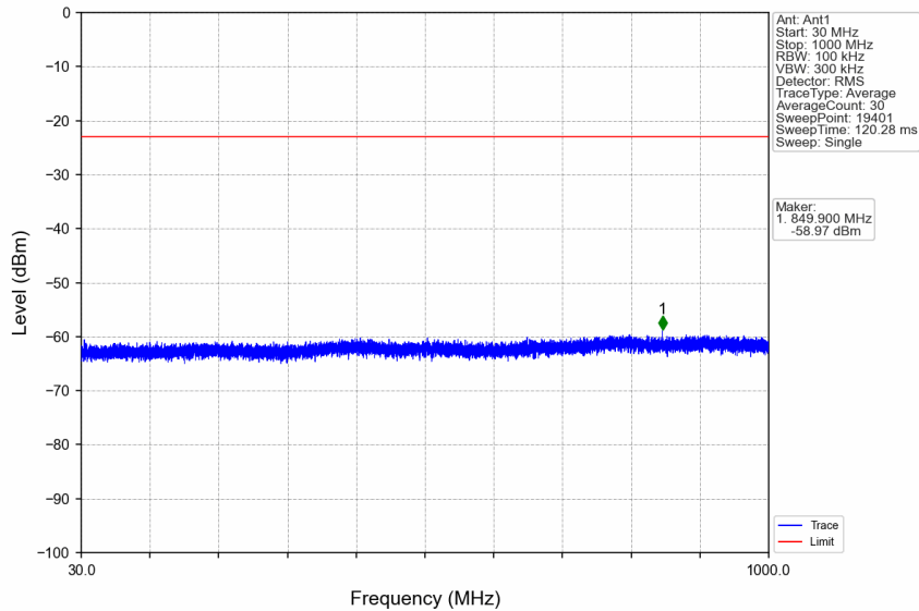
n7_30kHz_SISO_NTNV_25MHz_DFT-s-OFDM QPSK_2535MHz_Edge_1RB_Left
