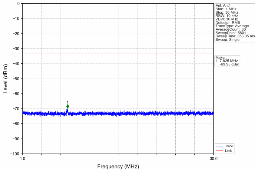
n7_30kHz_SISO_NTNV_25MHz_DFT-s-OFDM_QPSK_2557.5MHz_Edge_1RB_Right
