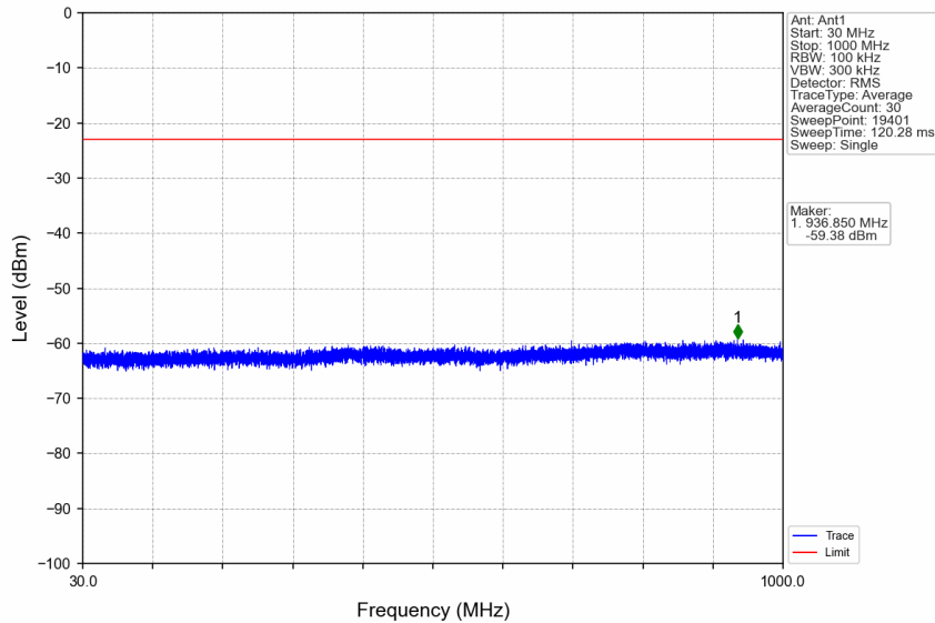
n7_30kHz_SISO_NTNV_25MHz_CP-OFDM QPSK_2535MHz_Edge_1RB_Left
