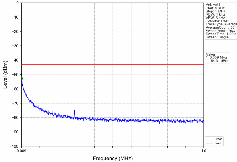
n7_30kHz_SISO_NTNV_25MHz_CP-OFDM QPSK_2557.5MHz_Edge_1RB_Right
