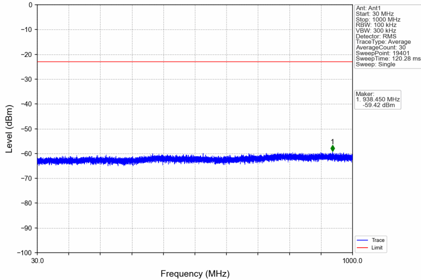
n7_30kHz_SISO_NTNV_25MHz_CP-OFDM QPSK_2557.5MHz_Edge_1RB_Right
