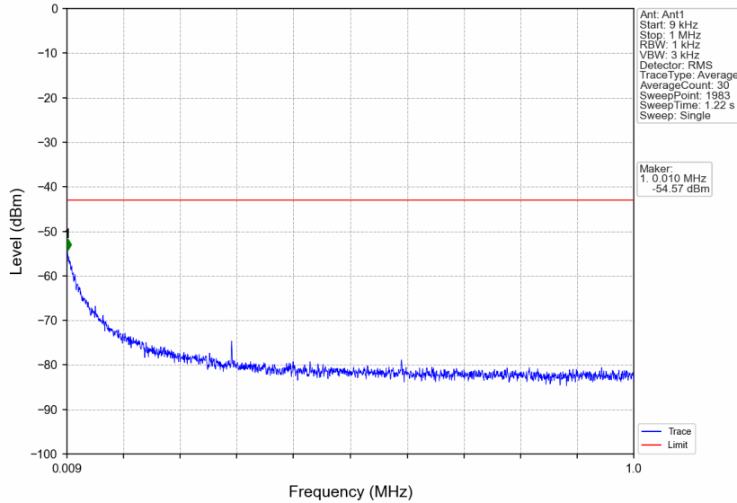
n7_30kHz_SISO_NTNV_20MHz_CP-OFDM QPSK_2560MHz_Edge_1RB_Right
