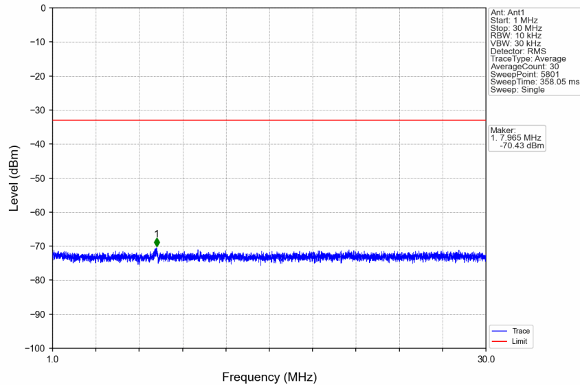
n7_30kHz_SISO_NTNV_15MHz_DFT-s-OFDM_QPSK_2562.5MHz_Edge_1RB_Right
