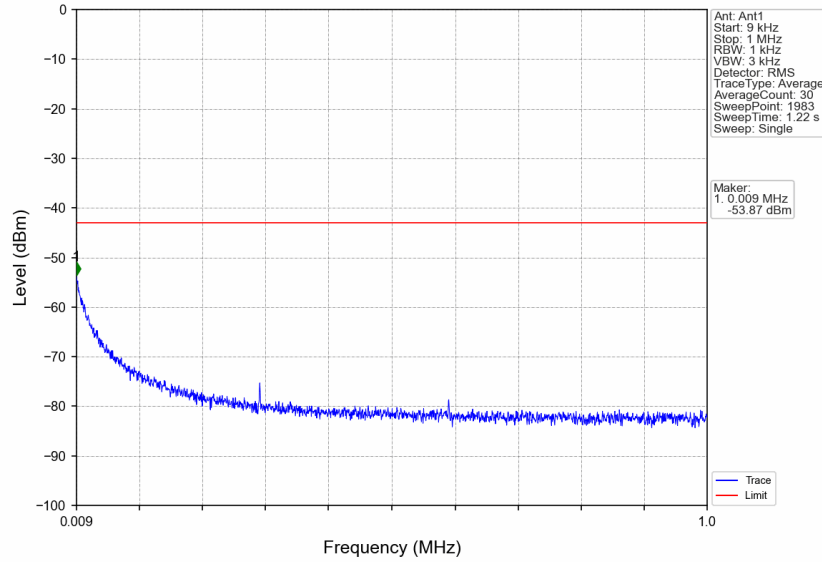
n7_30kHz_SISO_NTNV_10MHz_CP-OFDM QPSK_2565MHz_Edge_1RB_Right
