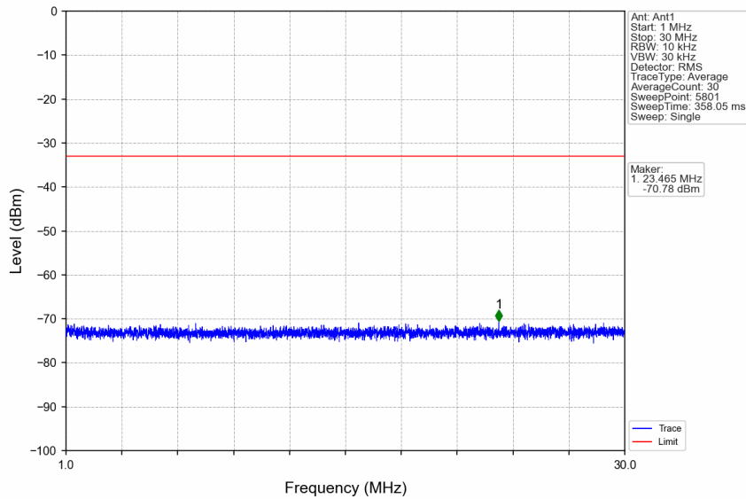
n7_30kHz_SISO_NTNV_15MHz_DFT-s-OFDM QPSK_2507.5MHz_Edge_1RB_Left
