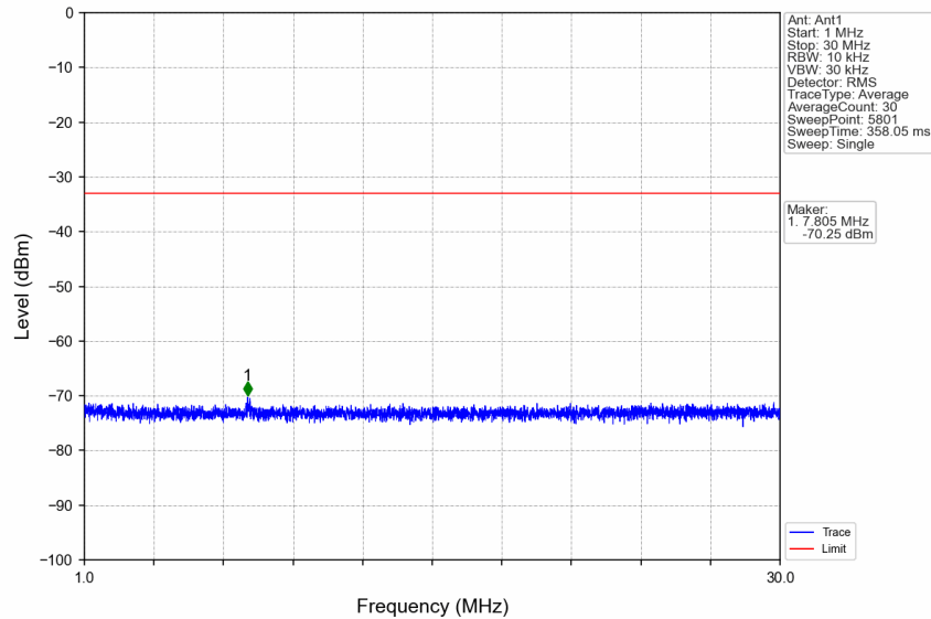
n7_30kHz_SISO_NTNV_10MHz_CP-OFDM QPSK_2565MHz_Edge_1RB_Right
