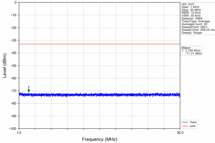
n7_30kHz_SISO_NTNV_10MHz_CP-OFDM QPSK_2535MHz_Edge_1RB_Left
