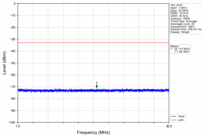
n7_30kHz_SISO_NTNV_15MHz_CP-OFDM QPSK_2507.5MHz_Edge_1RB_Left
