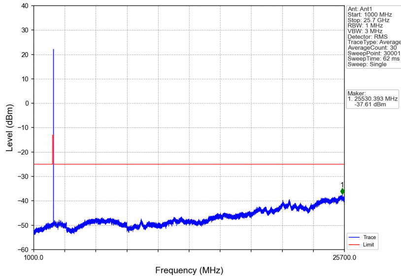
n7_30kHz_SISO_NTNV_10MHz_DFT-s-OFDM QPSK_2565MHz_Edge_1RB_Right
