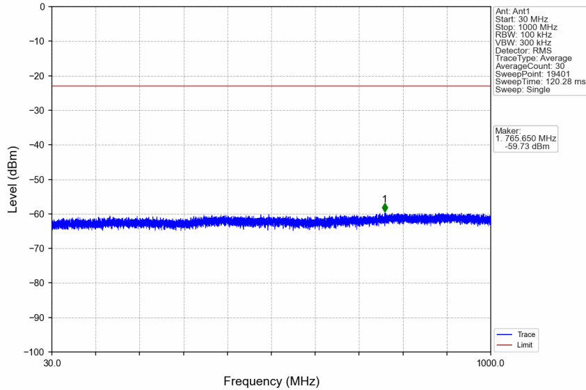
n7_30kHz_SISO_NTNV_10MHz_DFT-s-OFDM QPSK_2565MHz_Edge_1RB_Right
