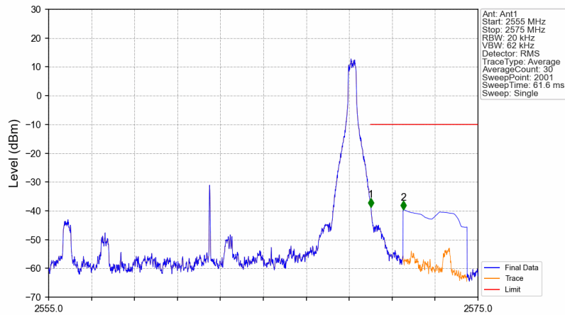
n7_30kHz_SISO_NTNV_15MHz_DFT-s-OFDM QPSK_2562.5MHz_Edge_1RB_Right
