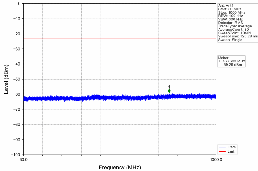
n7_30kHz_SISO_NTNV_10MHz_DFT-s-OFDM QPSK_2535MHz_Edge_1RB_Left
