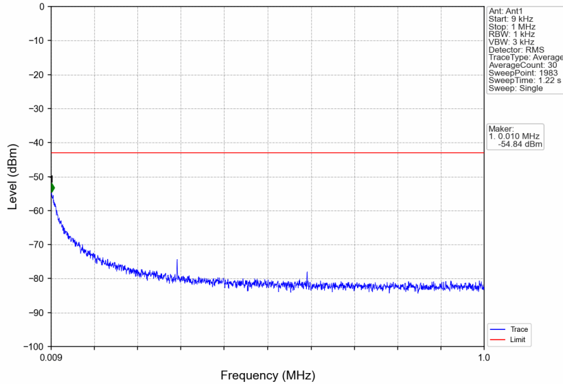
n7_30kHz_SISO_NTNV_15MHz_CP-OFDM QPSK_2562.5MHz_Edge_1RB_Right
