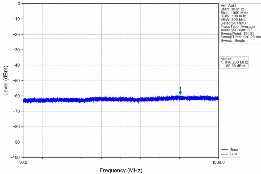
n7_30kHz_SISO_NTNV_10MHz_CP-OFDM QPSK_2535MHz_Edge_1RB_Left
