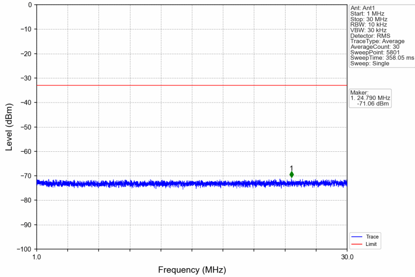
n7_30kHz_SISO_NTNV_15MHz_CP-OFDM QPSK_2535MHz_Edge_1RB_Left
