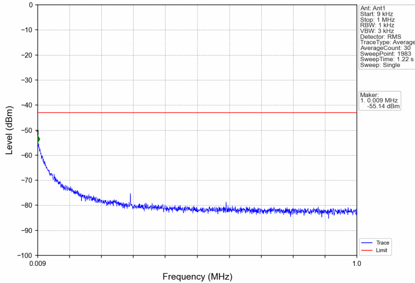
n7_30kHz_SISO_NTNV_10MHz_DFT-s-OFDM QPSK_2565MHz_Edge_1RB_Right
