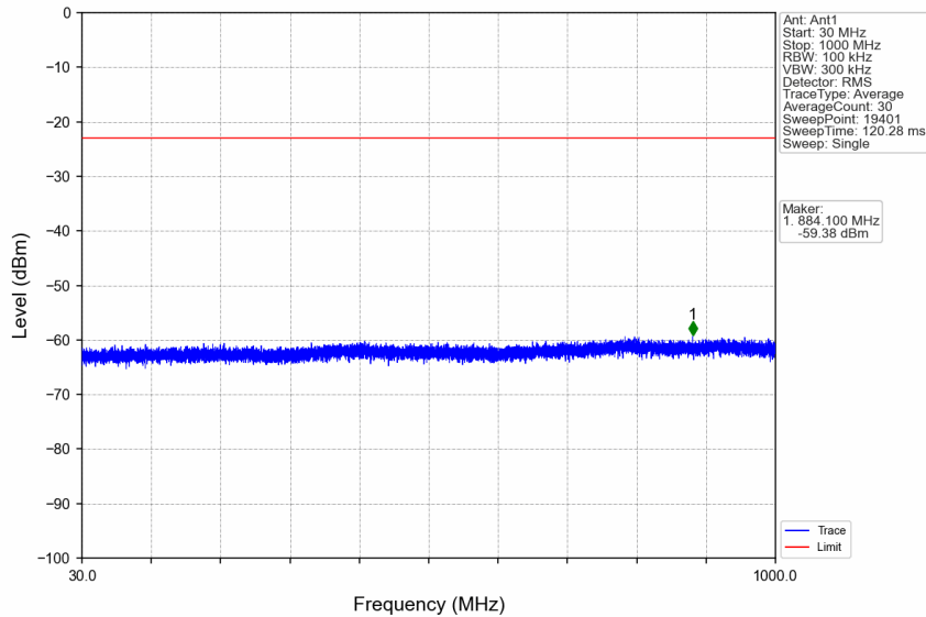
n7_30kHz_SISO_NTNV_10MHz_CP-OFDM QPSK_2505MHz_Edge_1RB_Left
