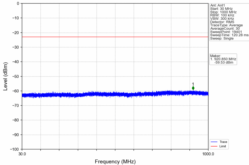
n7_30kHz_SISO_NTNV_10MHz_DFT-s-OFDM QPSK_2505MHz_Edge_1RB_Left
