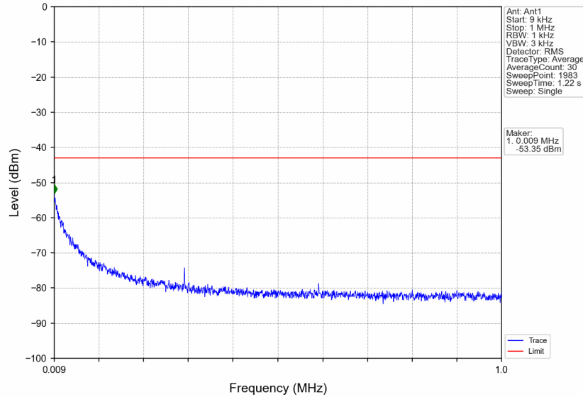
n7_30kHz_SISO_NTNV_15MHz_DFT-s-OFDM_QPSK_2562.5MHz_Edge_1RB_Right
