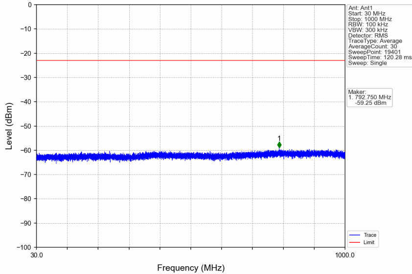
n7_30kHz_SISO_NTNV_15MHz_CP-OFDM QPSK_2562.5MHz_Edge_1RB_Right
