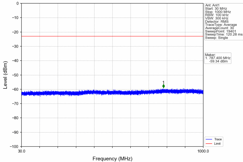
n7_30kHz_SISO_NTNV_15MHz_CP-OFDM QPSK_2535MHz_Edge_1RB_Left
