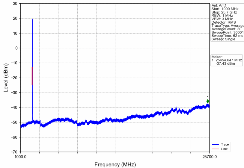
n7_30kHz_SISO_NTNV_15MHz_CP-OFDM QPSK_2562.5MHz_Edge_1RB_Right
