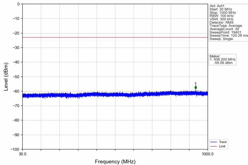
n7_15kHz_SISO_NTNV_50MHz_DFT-s-OFDM QPSK_2525MHz_Edge_1RB_Left
