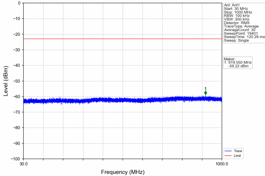
n7_15kHz_SISO_NTNV_40MHz_DFT-s-OFDM QPSK_2550MHz_Edge_1RB_Right
