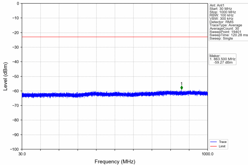
n7_15kHz_SISO_NTNV_40MHz_CP-OFDM QPSK_2535MHz_Edge_1RB_Left
