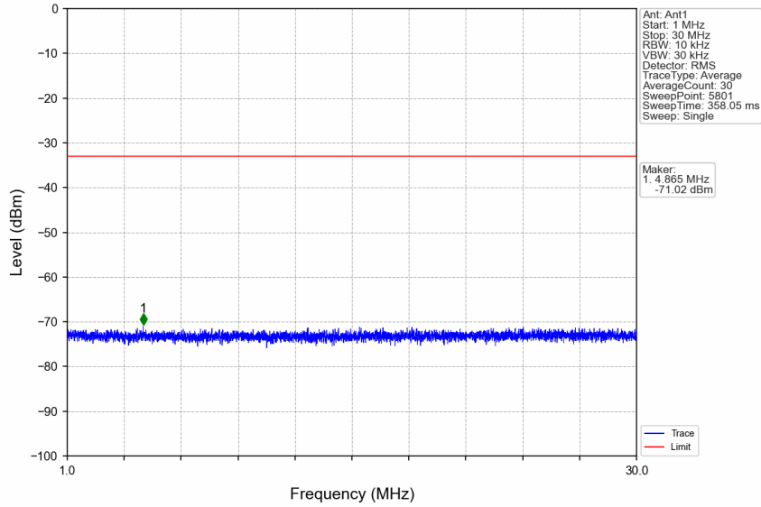
n7_15kHz_SISO_NTNV_50MHz_DFT-s-OFDM QPSK_2535MHz_Edge_1RB_Left
