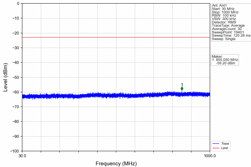
n7_15kHz_SISO_NTNV_50MHz_DFT-s-OFDM QPSK_2535MHz_Edge_1RB_Left
