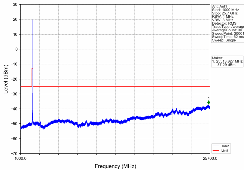
n7_15kHz_SISO_NTNV_40MHz_CP-OFDM QPSK_2550MHz_Edge_1RB_Right
