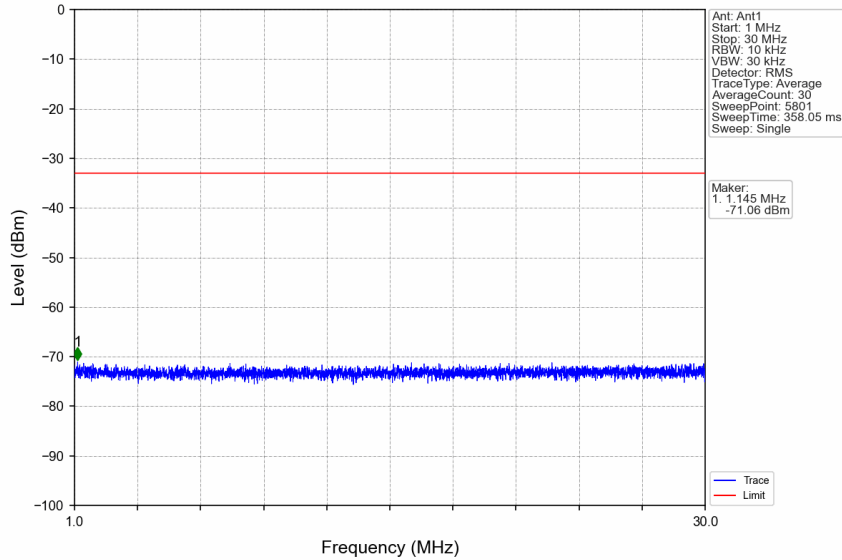
n7_15kHz_SISO_NTNV_40MHz_CP-OFDM QPSK_2520MHz_Edge_1RB_Left
