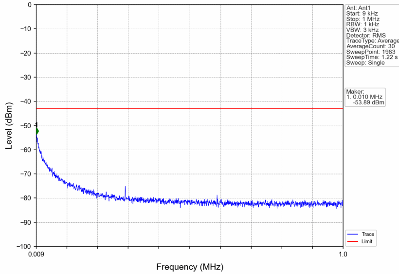
n7_15kHz_SISO_NTNV_40MHz_DFT-s-OFDM QPSK_2550MHz_Edge_1RB_Right
