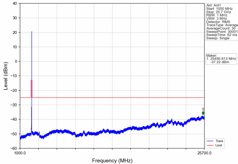
n7_15kHz_SiSO_NTNV_40MHz_CP-OFDM QPSK_2550MHz_Edge_1RB_Right
