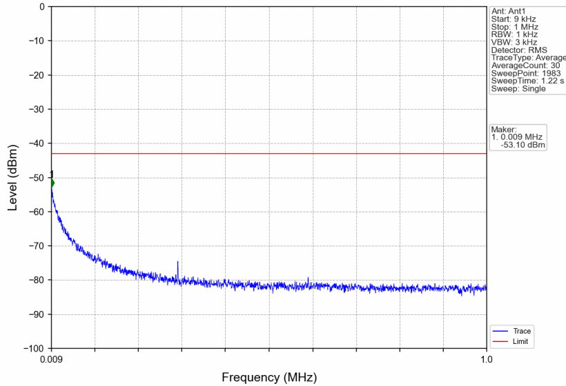
n7_15kHz_SISO_NTNV_50MHz_CP-OFDM QPSK_2545MHz_Edge_1RB_Right
