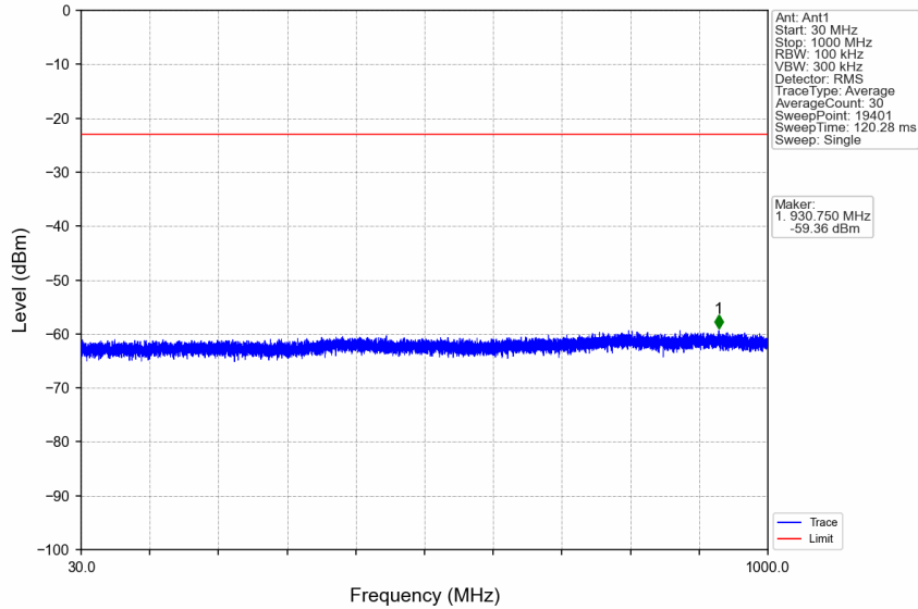
n7_15kHz_SISO_NTNV_50MHz_CP-OFDM QPSK_2545MHz_Edge_1RB_Right
