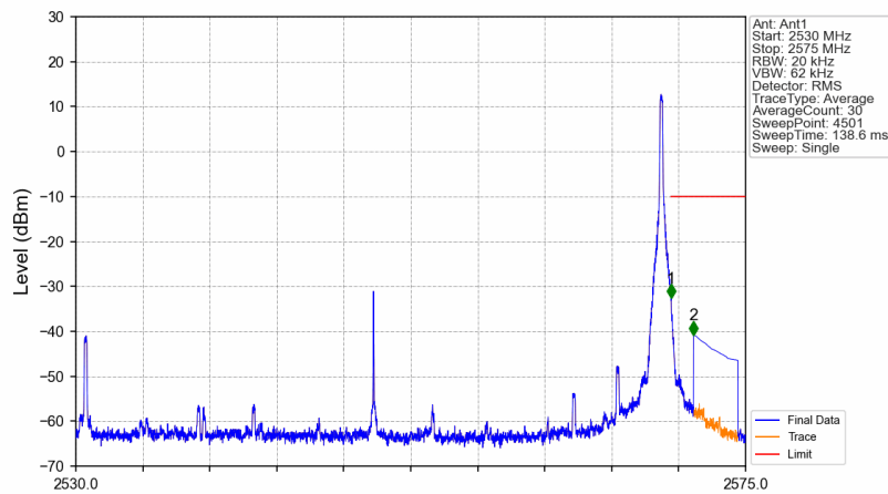
n7_15kHz_SISO_NTNV_40MHz_CP-OFDM QPSK_2550MHz_Edge_1RB_Right
