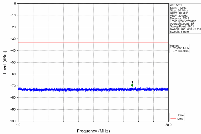
n7_15kHz_SISO_NTNV_50MHz_CP-OFDM QPSK_2535MHz_Edge_1RB_Left
