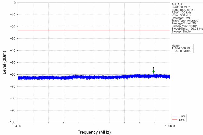
n7_15kHz_SISO_NTNV_40MHz_DFT-s-OFDM QPSK_2535MHz_Edge_1RB_Left
