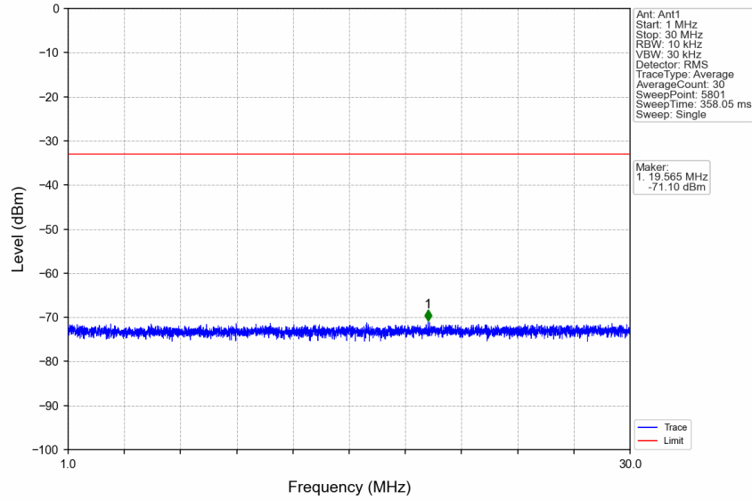
n7_15kHz_SISO_NTNV_50MHz_CP-OFDM QPSK_2525MHz_Edge_1RB_Left
