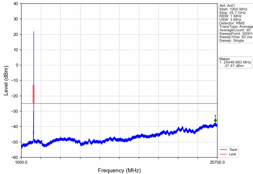
n7_15kHz_SISO_NTNV_40MHz_DFT-s-OFDM QPSK_2550MHz_Edge_1RB_Right
