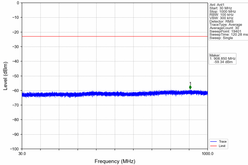
n7_15kHz_SiSO_NTNV_40MHz_CP-OFDM QPSK_2550MHz_Edge_1RB_Right
