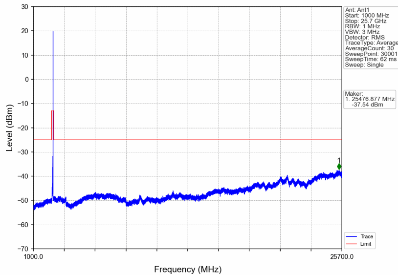
n7_15kHz_SISO_NTNV_50MHz_CP-OFDM QPSK_2545MHz_Edge_1RB_Right
