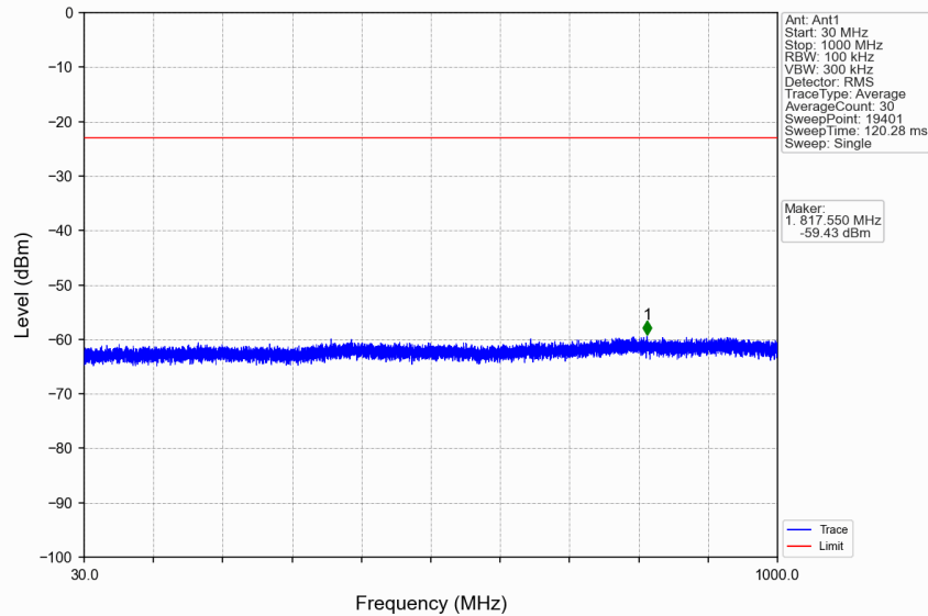
n7_15kHz_SISO_NTNV_50MHz_CP-OFDM QPSK_2525MHz_Edge_1RB_Left
