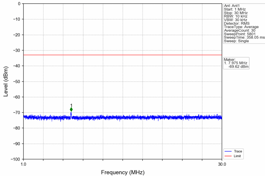
n7_15kHz_SISO_NTNV_50MHz_DFT-s-OFDM QPSK_2545MHz_Edge_1RB_Right
