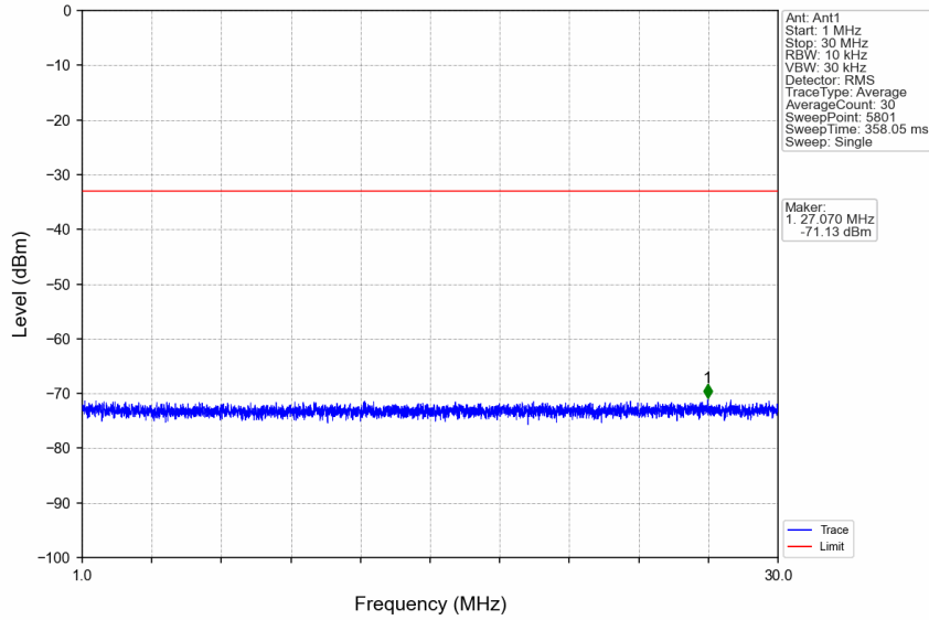
n7_15kHz_SISO_NTNV_40MHz_CP-OFDM QPSK_2535MHz_Edge_1RB_Left
