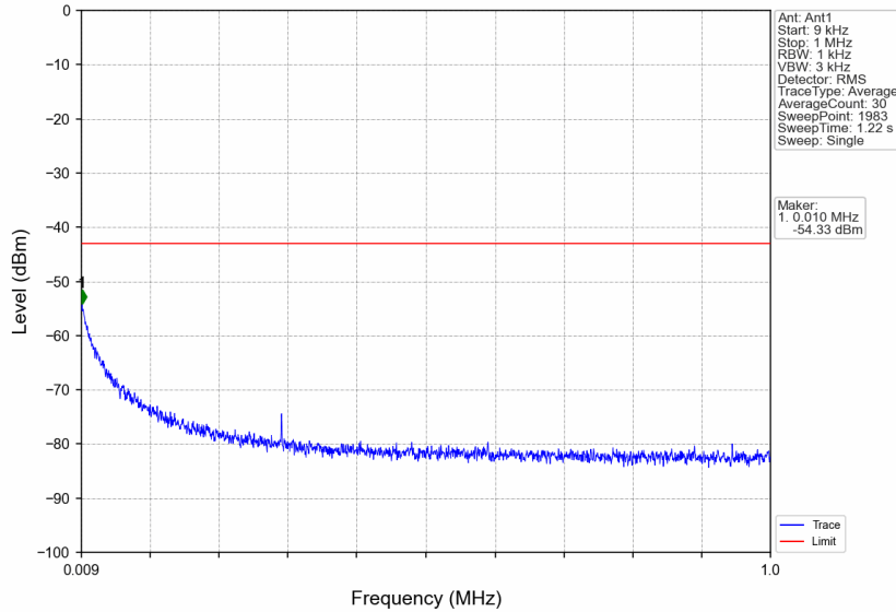
n7_15kHz_SISO_NTNV_50MHz_DFT-s-OFDM QPSK_2545MHz_Edge_1RB_Right
